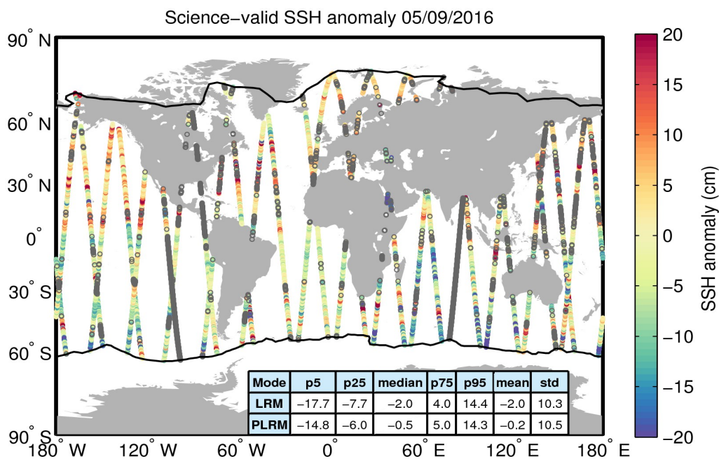
Figure 10. Geographical distribution of science-valid SSH anomaly data over oceans and lakes for 05/09/2016. The statistical values shown in the table refer to the SSH anomaly in cm and are calculated separately for LRM and PLRM regions. The black lines mark the outer limit of the Arctic and Antarctic polar polygons. Gray circles denote records that have been rejected based on the editing criteria described in Table 2.
