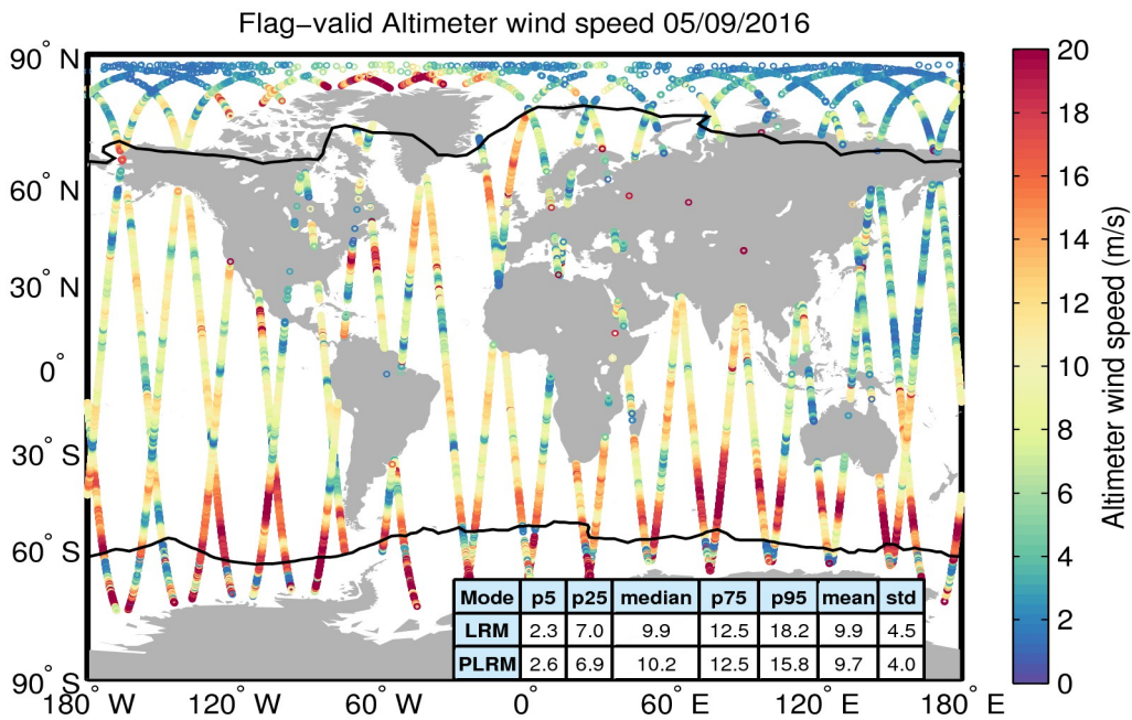
Figure 31. Geographical distribution of flag-valid wind data over oceans and lakes for 05/09/2016. The statistical values shown in the table refer to the wind in m/s and are calculated separately for LRM and PLRM regions. Measurements taken over polar polygons have been excluded from the computation of the statistical values. The black lines mark the outer limit of the Arctic and Antarctic polar polygons.
