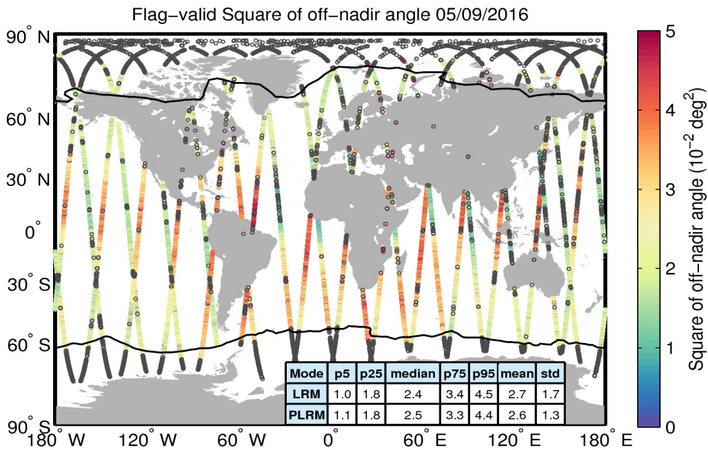
Figure 37. Geographical distribution of flag-valid mispointing data over oceans and lakes for 05/09/2016. The statistical values shown in the table refer to the mispointing in 10^{-2} deg 2 and are calculated separately for LRM and PLRM regions. Measurements taken over polar polygons have been excluded from the computation of the statistical values. The black lines mark the outer limit of the Arctic and Antarctic polar polygons. Gray circles denote negative values.
