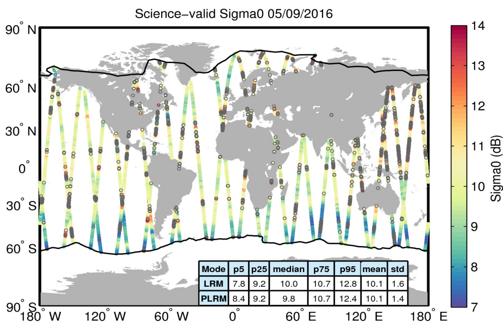
Figure 27. Geographical distribution of science-valid sigma0 data over oceans and lakes for 05/09/2016. The statistical values shown in the table refer to the sigma0 in dB and are calculated separately for LRM and PLRM regions. The black lines mark the outer limit of the Arctic and Antarctic polar polygons. Gray circles denote records that have been rejected based on the editing criteria described in Table 4.
