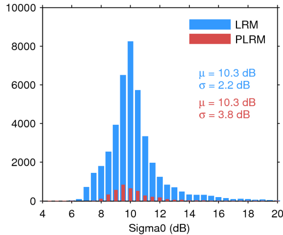
Figure 25. Histogram of flag-valid sigma0 over oceans and lakes for LRM (blue) and PLRM (red) for 05/09/2016. The mean ( \mu ) and standard deviation ( \sigma ) are also shown. Note that values outside [4 20] dB are excluded from the histogram for the sake of readability but not from the computation of \mu and \sigma .
