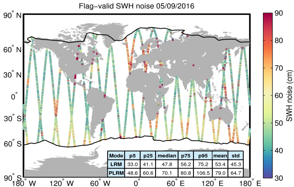
Figure 18. Geographical distribution of flag-valid 20-Hz SWH measurement noise over oceans and lakes for 05/09/2016. The statistical values shown in the table refer to the SWH noise and are calculated separately for LRM and PLRM regions. Measurements taken over polar polygons have been excluded from the computation of the statistical values. The black lines mark the outer limit of the Arctic and Antarctic polar polygons.
