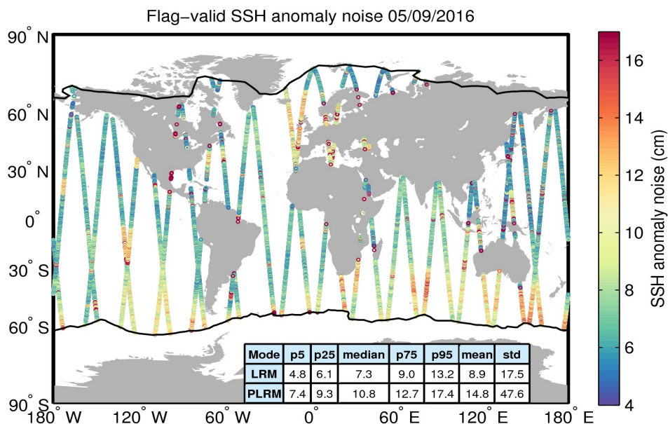
Figure 8. Geographical distribution of flag-valid 20-Hz SSH anomaly measurement noise over oceans and lakes for 05/09/2016. The statistical values shown in the table refer to the SSH anomaly noise and are calculated separately for LRM and PLRM regions. Measurements taken over polar polygons have been excluded from the computation of the statistical values. The black lines mark the outer limit of the Arctic and Antarctic polar polygons.
