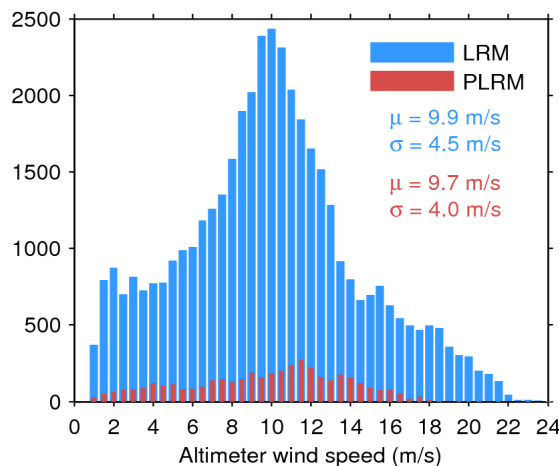
Figure 35. Histogram of science-valid wind over oceans and lakes for LRM (blue) and PLRM (red) for 05/09/2016. The mean ( \mu ) and standard deviation ( \sigma ) are also shown. Note that values larger than 24 m/s are excluded from the histogram for the sake of readability but not from the computation of \mu and \sigma .
