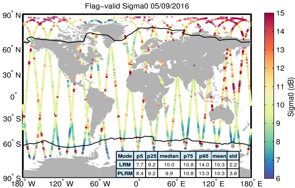
Figure 23. Geographical distribution of flag-valid sigma0 data over oceans and lakes for 05/09/2016. The statistical values shown in the table refer to the sigma0 in dB and are calculated separately for LRM and PLRM regions. Measurements taken over polar polygons have been excluded from the computation of the statistical values. The black lines mark the outer limit of the Arctic and Antarctic polar polygons.
