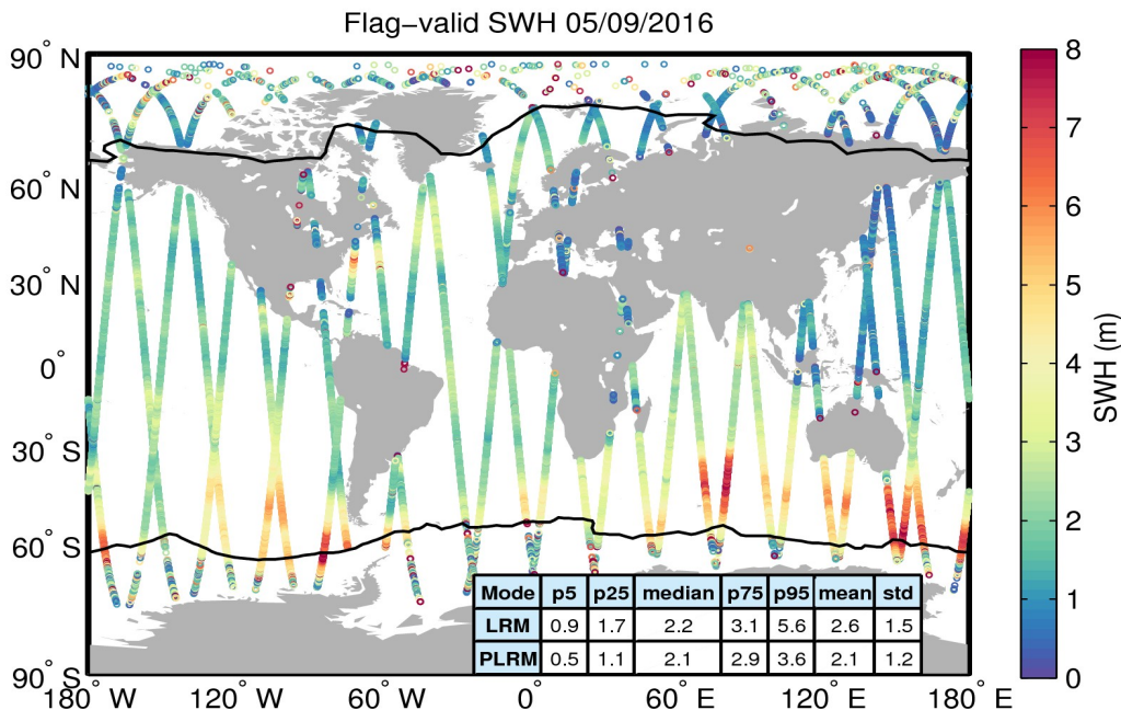
Figure 15. Geographical distribution of flag-valid SWH data over oceans and lakes for 05/09/2016. The statistical values shown in the table refer to the SWH in m and are calculated separately for LRM and PLRM regions. Measurements taken over polar polygons have been excluded from the computation of the statistical values. The black lines mark the outer limit of the Arctic and Antarctic polar polygons.
