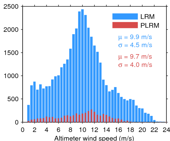
Figure 33. Histogram of flag-valid wind over oceans and lakes for LRM (blue) and PLRM (red) for 05/09/2016. The mean ( \mu ) and standard deviation ( \sigma ) are also shown. Note that values larger than 24 m/s are excluded from the histogram for the sake of readability but not from the computation of \mu and \sigma .
