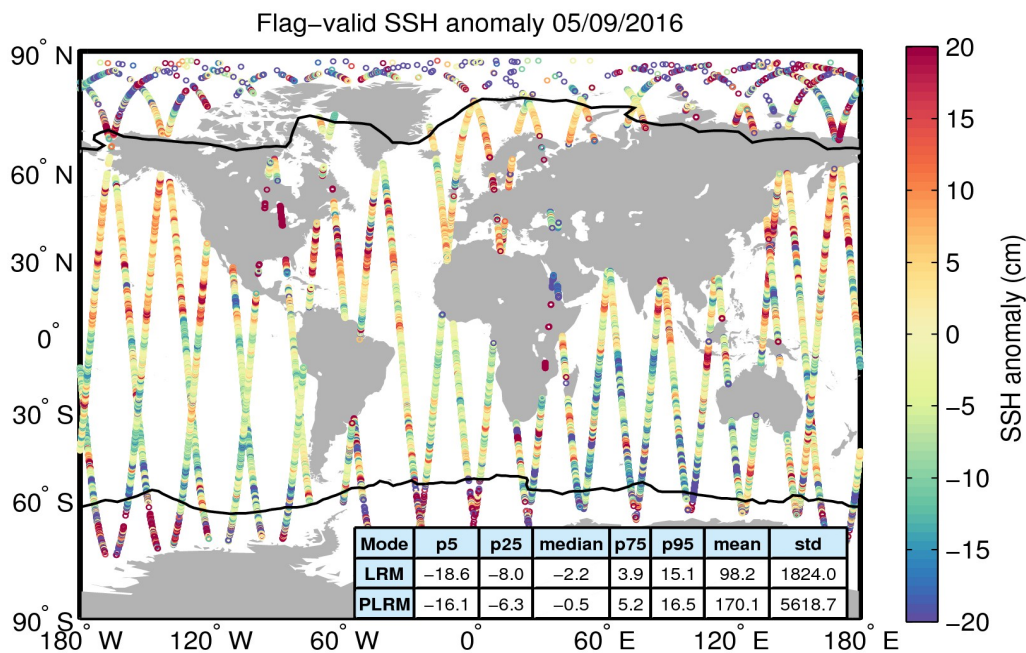
Figure 5. Geographical distribution of flag-valid 1-Hz SSH anomaly data over oceans and lakes for 05/09/2016. The statistical values shown in the table refer to the SSH anomaly in cm and are calculated separately for LRM and PLRM regions. Measurements taken over polar polygons have been excluded from the computation of the statistical values. The black lines mark the outer limit of the Arctic and Antarctic polar polygons.
