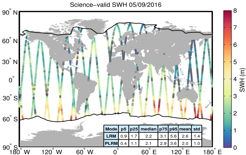
Figure 19. Geographical distribution of science-valid SWH data over oceans and lakes for 05/09/2016. The statistical values shown in the table refer to the SWH in m and are calculated separately for LRM and PLRM regions. The black lines mark the outer limit of the Arctic and Antarctic polar polygons. Gray circles denote records that have been rejected based on the editing criteria described in Table 3.
