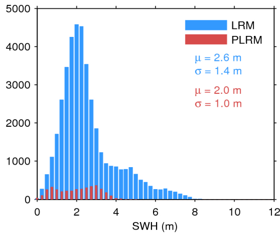
Figure 20. Histogram of science-valid SWH over oceans and lakes for LRM (blue) and PLRM (red) for 05/09/2016. The mean ( \mu ) and standard deviation ( \sigma ) are also shown. Note that values larger than 12 m are excluded from the histogram for the sake of readability but not from the computation of \mu and \sigma .
