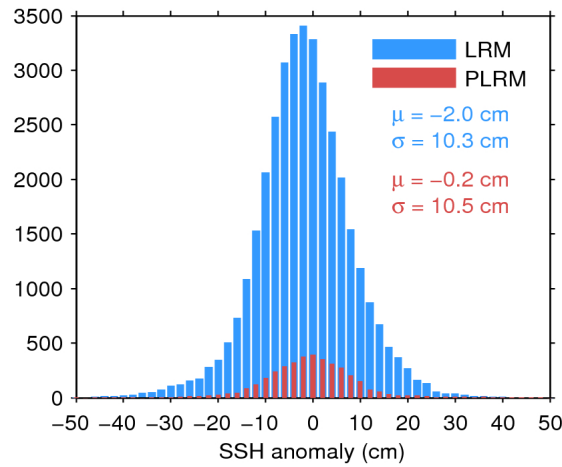
Figure 11. Histogram of science-valid SSH anomaly over oceans and lakes for LRM (blue) and PLRM (red) for 05/09/2016. The mean ( \mu ) and standard deviation ( \sigma ) are also shown. Note that values outside [-50 50] cm are excluded from the histogram for the sake of readability but not from the computation of \mu and \sigma .
