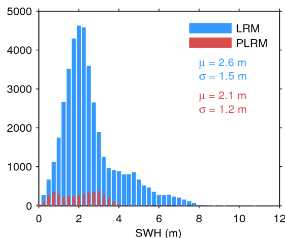
Figure 17. Histogram of flag-valid SWH over oceans and lakes for LRM (blue) and PLRM (red) for 05/09/2016. The mean ( \mu ) and standard deviation ( \sigma ) are also shown. Note that values larger than 12 m are excluded from the histogram for the sake of readability but not from the computation of \mu and \sigma .
