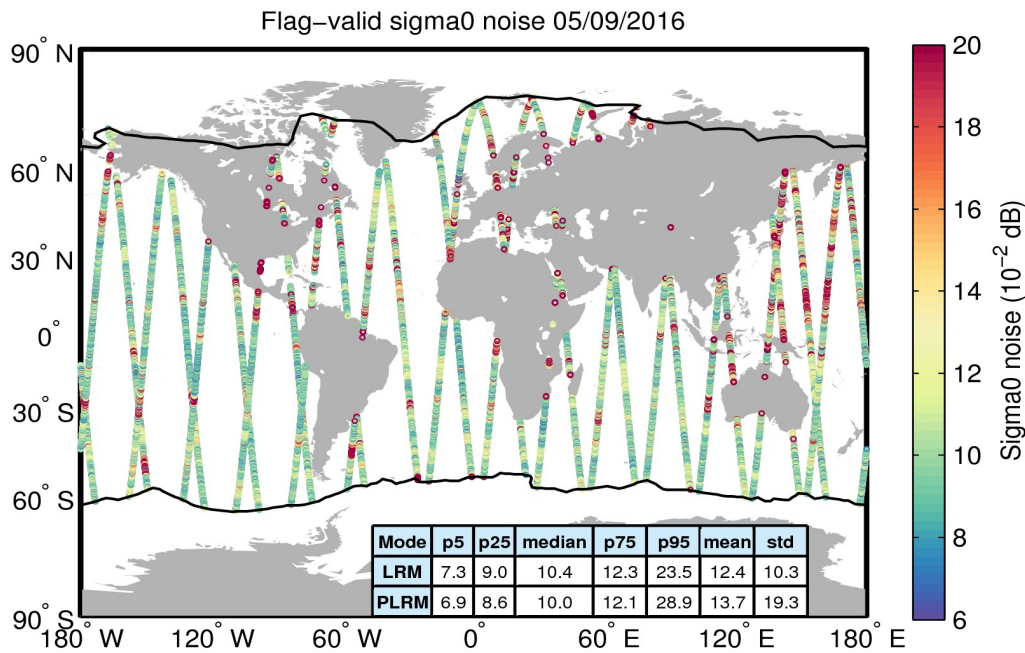
Figure 26. Geographical distribution of flag-valid 20-Hz sigma0 measurement noise over oceans and lakes for 05/09/2016. The statistical values shown in the table refer to the sigma0 noise and are calculated separately for LRM and PLRM regions. Measurements taken over polar polygons have been excluded from the computation of the statistical values. The black lines mark the outer limit of the Arctic and Antarctic polar polygons.
