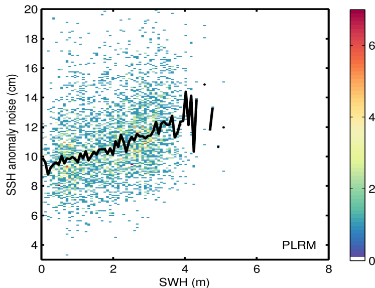
Figure 9. 2D histogram showing flag-valid SSH anomaly noise as a function of SWH for LRM (top) and PLRM (bottom) for 05/09/2016. The black line denotes the median SSH anomaly noise as a function of SWH.
