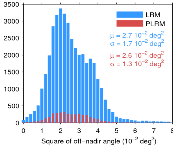
Figure 39. Histogram of flag-valid mispointing over oceans and lakes for LRM (blue) and PLRM (red) for 05/09/2016. Only positive values have been considered. The mean ( \mu ) and standard deviation ( \sigma ) are also shown. Note that values larger than 8 \cdot 10^{-2} \text{ deg}^2 are excluded from the histogram for the sake of readability but not from the computation of \mu and \sigma .
