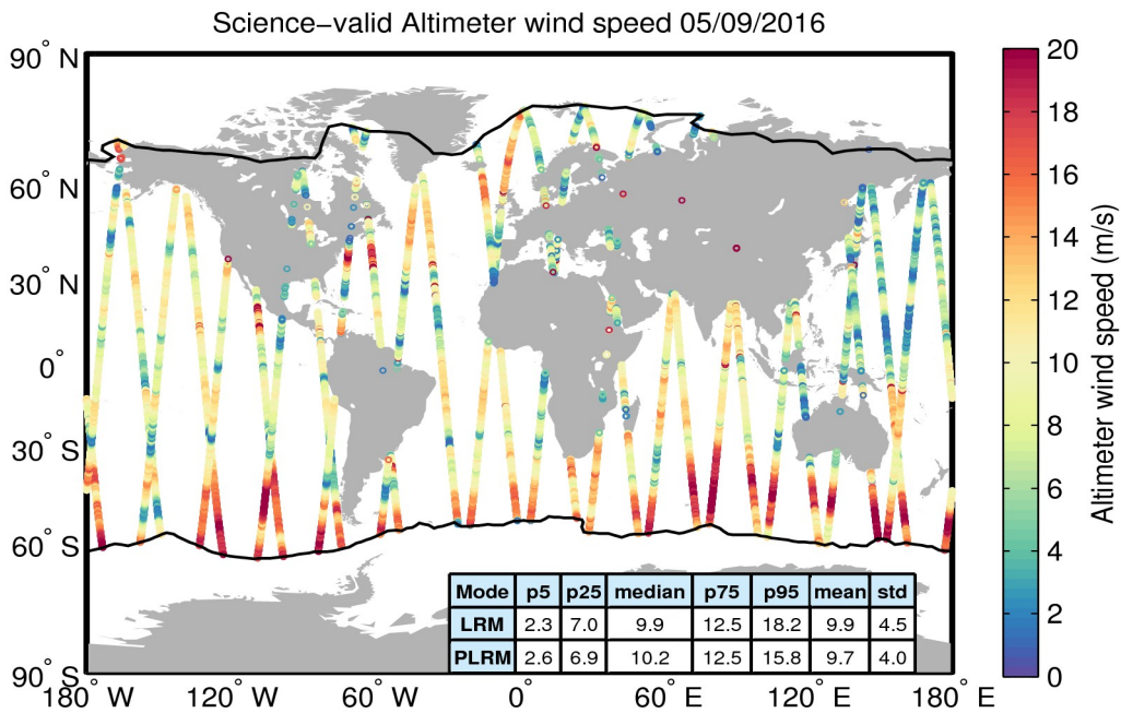
Figure 34. Geographical distribution of science-valid wind data over oceans and lakes for 05/09/2016. The statistical values shown in the table refer to the wind in m/s and are calculated separately for LRM and PLRM regions. The black lines mark the outer limit of the Arctic and Antarctic polar polygons. Gray circles denote records that have been rejected based on the editing criteria described in Table 5.
