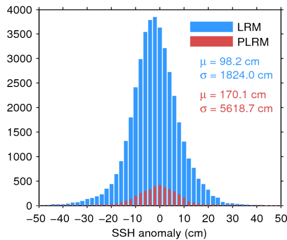
Figure 7. Histogram of flag-valid SSH anomaly over oceans and lakes for LRM (blue) and PLRM (red) for 05/09/2016. The mean ( \mu ) and standard deviation ( \sigma ) are also shown. Note that values outside [-50 50] cm are excluded from the histogram for the sake of readability but not from the computation of \mu and \sigma .
