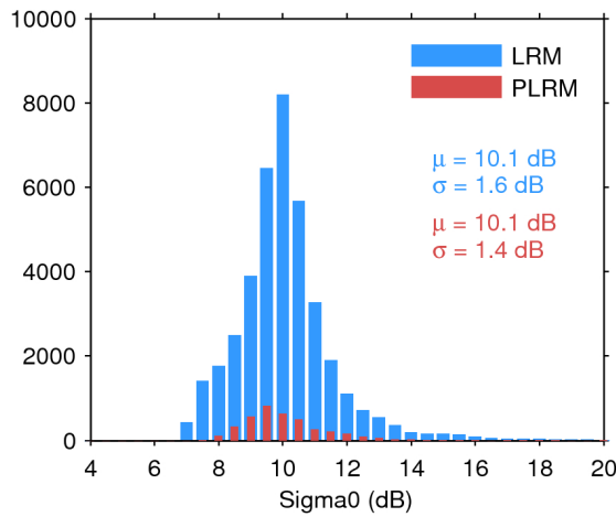
Figure 28. Histogram of science-valid sigma0 over oceans and lakes for LRM (blue) and PLRM (red) for 05/09/2016. The mean ( \mu ) and standard deviation ( \sigma ) are also shown. Note that values outside [4 20] dB are excluded from the histogram for the sake of readability but not from the computation of \mu and \sigma .
