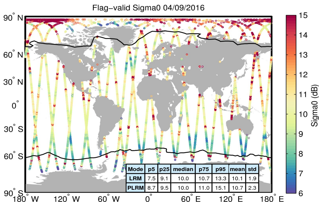
Figure 23. Geographical distribution of flag-valid sigma0 data over oceans and lakes for 04/09/2016. The statistical values shown in the table refer to the sigma0 in dB and are calculated separately for LRM and PLRM regions. Measurements taken over polar polygons have been excluded from the computation of the statistical values. The black lines mark the outer limit of the Arctic and Antarctic polar polygons.
