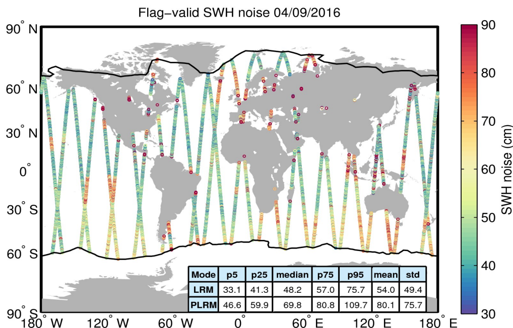
Figure 18. Geographical distribution of flag-valid 20-Hz SWH measurement noise over oceans and lakes for 04/09/2016. The statistical values shown in the table refer to the SWH noise and are calculated separately for LRM and PLRM regions. Measurements taken over polar polygons have been excluded from the computation of the statistical values. The black lines mark the outer limit of the Arctic and Antarctic polar polygons.
