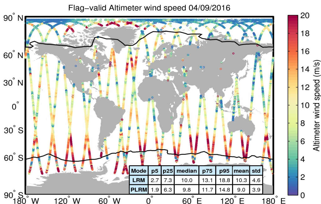
Figure 31. Geographical distribution of flag-valid wind data over oceans and lakes for 04/09/2016. The statistical values shown in the table refer to the wind in m/s and are calculated separately for LRM and PLRM regions. Measurements taken over polar polygons have been excluded from the computation of the statistical values. The black lines mark the outer limit of the Arctic and Antarctic polar polygons.
