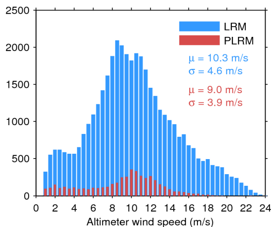
Figure 35. Histogram of science-valid wind over oceans and lakes for LRM (blue) and PLRM (red) for 04/09/2016. The mean ( \mu ) and standard deviation ( \sigma ) are also shown. Note that values larger than 24 m/s are excluded from the histogram for the sake of readability but not from the computation of \mu and \sigma .
