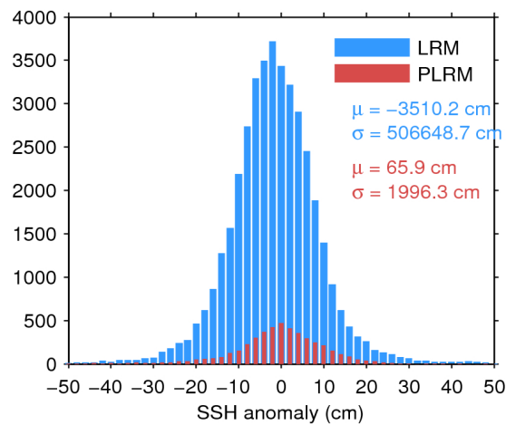
Figure 7. Histogram of flag-valid SSH anomaly over oceans and lakes for LRM (blue) and PLRM (red) for 04/09/2016. The mean ( \mu ) and standard deviation ( \sigma ) are also shown. Note that values outside [-50\ 50] cm are excluded from the histogram for the sake of readability but not from the computation of \mu and \sigma .
