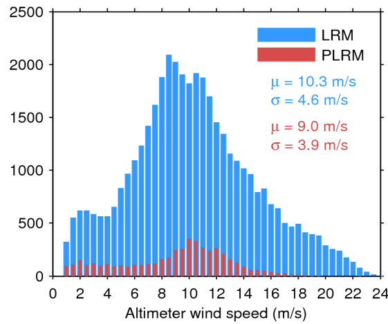
Figure 33. Histogram of flag-valid wind over oceans and lakes for LRM (blue) and PLRM (red) for 04/09/2016. The mean ( \mu ) and standard deviation ( \sigma ) are also shown. Note that values larger than 24 m/s are excluded from the histogram for the sake of readability but not from the computation of \mu and \sigma .
