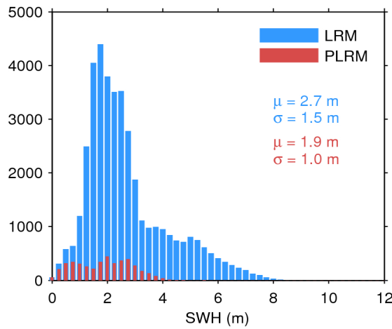
Figure 20. Histogram of science-valid SWH over oceans and lakes for LRM (blue) and PLRM (red) for 04/09/2016. The mean ( \mu ) and standard deviation ( \sigma ) are also shown. Note that values larger than 12 m are excluded from the histogram for the sake of readability but not from the computation of \mu and \sigma .
