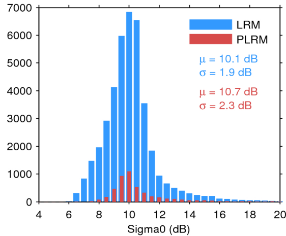
Figure 25. Histogram of flag-valid sigma0 over oceans and lakes for LRM (blue) and PLRM (red) for 04/09/2016. The mean ( \mu ) and standard deviation ( \sigma ) are also shown. Note that values outside [4 20] dB are excluded from the histogram for the sake of readability but not from the computation of \mu and \sigma .
