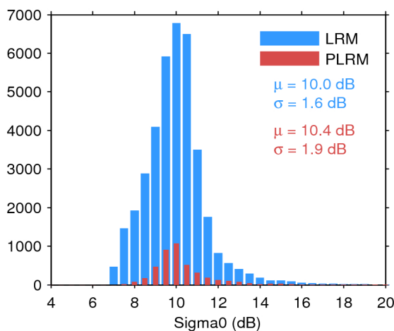
Figure 28. Histogram of science-valid sigma0 over oceans and lakes for LRM (blue) and PLRM (red) for 04/09/2016. The mean ( \mu ) and standard deviation ( \sigma ) are also shown. Note that values outside [4 20] dB are excluded from the histogram for the sake of readability but not from the computation of \mu and \sigma .
