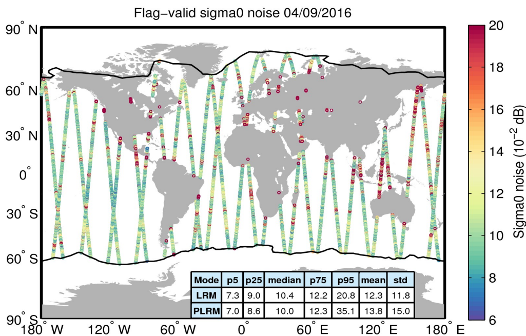
Figure 26. Geographical distribution of flag-valid 20-Hz sigma0 measurement noise over oceans and lakes for 04/09/2016. The statistical values shown in the table refer to the sigma0 noise and are calculated separately for LRM and PLRM regions. Measurements taken over polar polygons have been excluded from the computation of the statistical values. The black lines mark the outer limit of the Arctic and Antarctic polar polygons.
