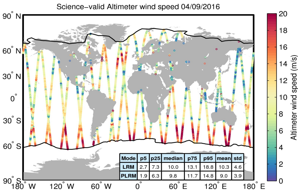
Figure 34. Geographical distribution of science-valid wind data over oceans and lakes for 04/09/2016. The statistical values shown in the table refer to the wind in m/s and are calculated separately for LRM and PLRM regions. The black lines mark the outer limit of the Arctic and Antarctic polar polygons. Gray circles denote records that have been rejected based on the editing criteria described in Table 5.
