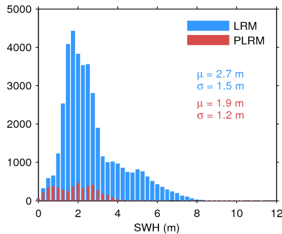
Figure 17. Histogram of flag-valid SWH over oceans and lakes for LRM (blue) and PLRM (red) for 04/09/2016. The mean ( \mu ) and standard deviation ( \sigma ) are also shown. Note that values larger than 12 m are excluded from the histogram for the sake of readability but not from the computation of \mu and \sigma .
