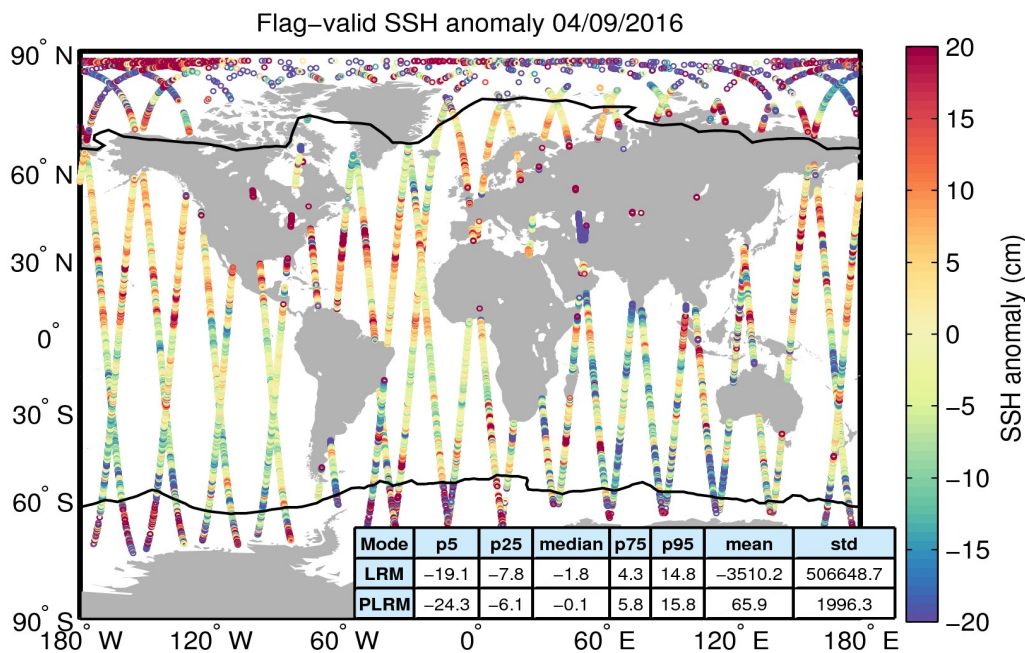
Figure 5. Geographical distribution of flag-valid 1-Hz SSH anomaly data over oceans and lakes for 04/09/2016. The statistical values shown in the table refer to the SSH anomaly in cm and are calculated separately for LRM and PLRM regions. Measurements taken over polar polygons have been excluded from the computation of the statistical values. The black lines mark the outer limit of the Arctic and Antarctic polar polygons.
