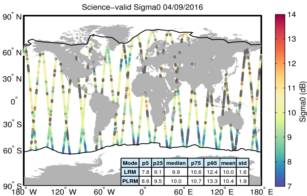
Figure 27. Geographical distribution of science-valid sigma0 data over oceans and lakes for 04/09/2016. The statistical values shown in the table refer to the sigma0 in dB and are calculated separately for LRM and PLRM regions. The black lines mark the outer limit of the Arctic and Antarctic polar polygons. Gray circles denote records that have been rejected based on the editing criteria described in Table 4.
