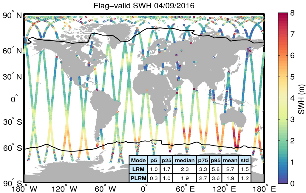
Figure 15. Geographical distribution of flag-valid SWH data over oceans and lakes for 04/09/2016. The statistical values shown in the table refer to the SWH in m and are calculated separately for LRM and PLRM regions. Measurements taken over polar polygons have been excluded from the computation of the statistical values. The black lines mark the outer limit of the Arctic and Antarctic polar polygons.
