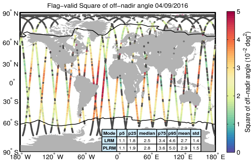
Figure 37. Geographical distribution of flag-valid mispointing data over oceans and lakes for 04/09/2016. The statistical values shown in the table refer to the mispointing in 10^{-2} deg 2 and are calculated separately for LRM and PLRM regions. Measurements taken over polar polygons have been excluded from the computation of the statistical values. The black lines mark the outer limit of the Arctic and Antarctic polar polygons. Gray circles denote negative values.
