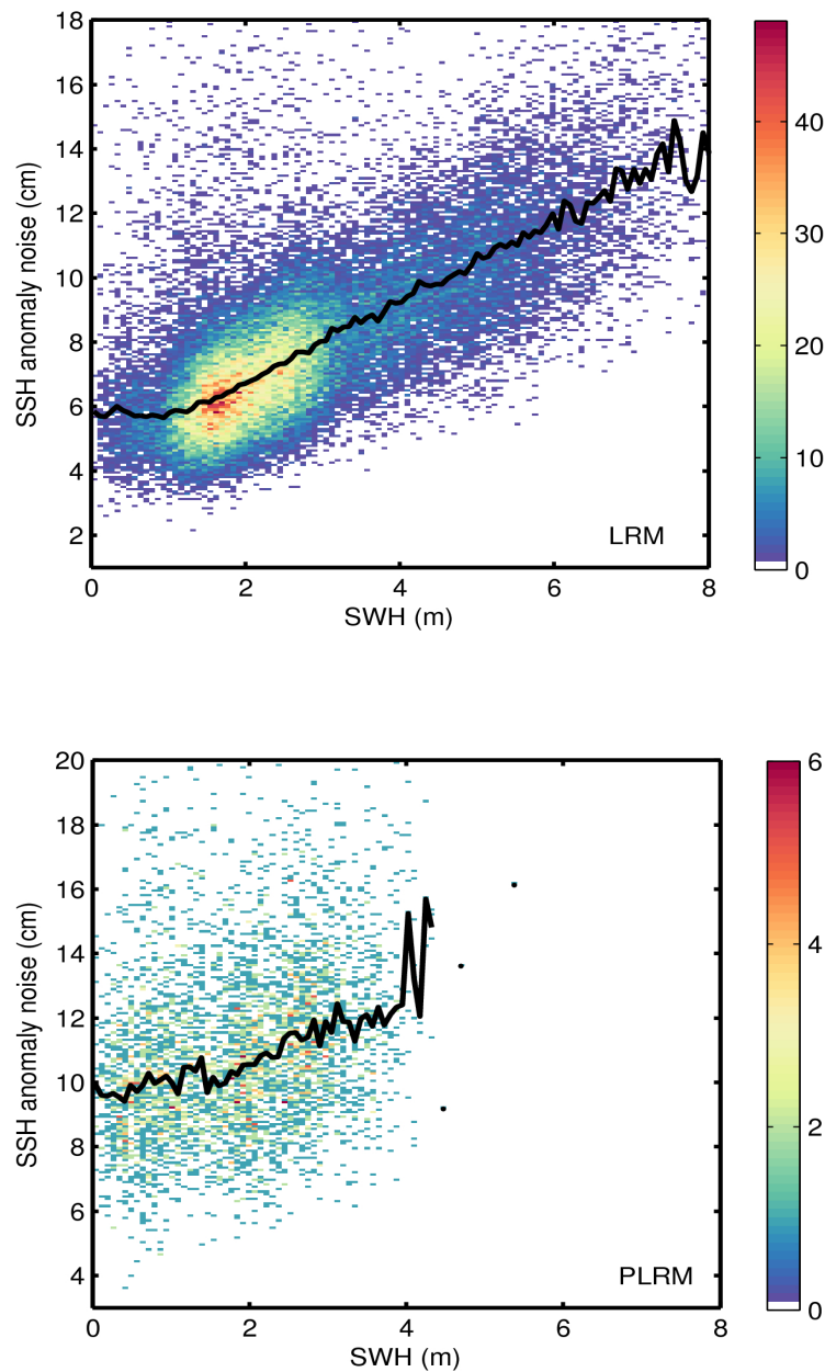
Figure 9. 2D histogram showing flag-valid SSH anomaly noise as a function of SWH for LRM (top) and PLRM (bottom) for 04/09/2016. The black line denotes the median SSH anomaly noise as a function of SWH.
