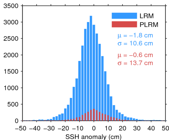
Figure 11. Histogram of science-valid SSH anomaly over oceans and lakes for LRM (blue) and PLRM (red) for 04/09/2016. The mean ( \mu ) and standard deviation ( \sigma ) are also shown. Note that values outside [-50 50] cm are excluded from the histogram for the sake of readability but not from the computation of \mu and \sigma .
