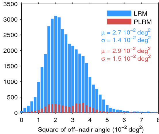
Figure 39. Histogram of flag-valid mispointing over oceans and lakes for LRM (blue) and PLRM (red) for 04/09/2016. Only positive values have been considered. The mean ( \mu ) and standard deviation ( \sigma ) are also shown. Note that values larger than 8 \cdot 10^{-2} \text{ deg}^2 are excluded from the histogram for the sake of readability but not from the computation of \mu and \sigma .
