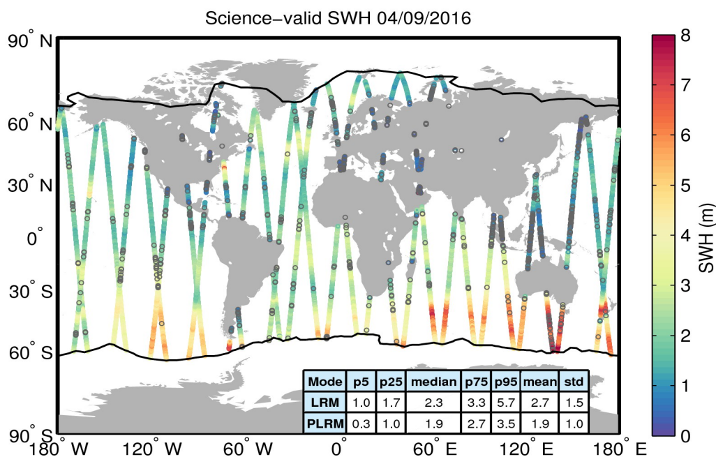
Figure 19. Geographical distribution of science-valid SWH data over oceans and lakes for 04/09/2016. The statistical values shown in the table refer to the SWH in m and are calculated separately for LRM and PLRM regions. The black lines mark the outer limit of the Arctic and Antarctic polar polygons. Gray circles denote records that have been rejected based on the editing criteria described in Table 3.
