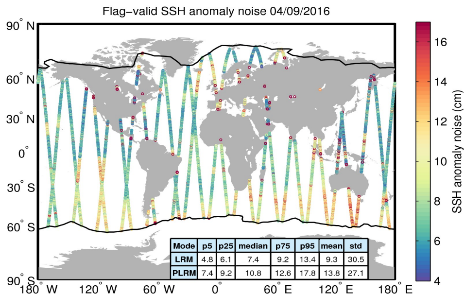
Figure 8. Geographical distribution of flag-valid 20-Hz SSH anomaly measurement noise over oceans and lakes for 04/09/2016. The statistical values shown in the table refer to the SSH anomaly noise and are calculated separately for LRM and PLRM regions. Measurements taken over polar polygons have been excluded from the computation of the statistical values. The black lines mark the outer limit of the Arctic and Antarctic polar polygons.
