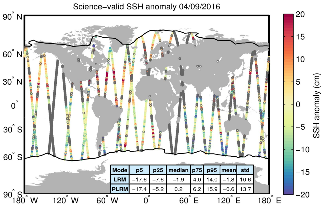
Figure 10. Geographical distribution of science-valid SSH anomaly data over oceans and lakes for 04/09/2016. The statistical values shown in the table refer to the SSH anomaly in cm and are calculated separately for LRM and PLRM regions. The black lines mark the outer limit of the Arctic and Antarctic polar polygons. Gray circles denote records that have been rejected based on the editing criteria described in Table 2.
