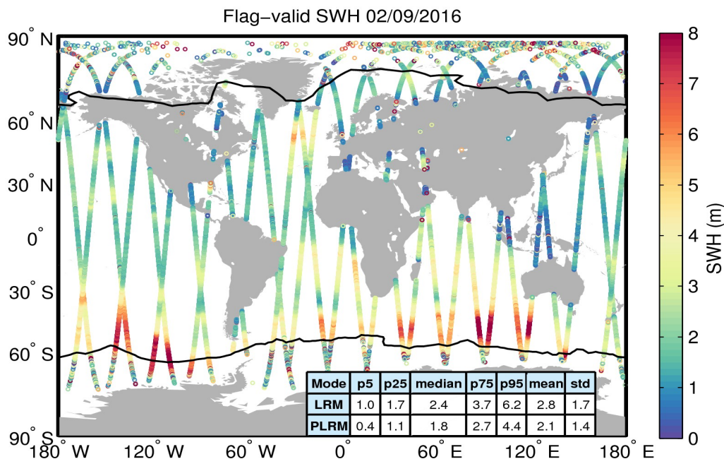
Figure 15. Geographical distribution of flag-valid SWH data over oceans and lakes for 02/09/2016. The statistical values shown in the table refer to the SWH in m and are calculated separately for LRM and PLRM regions. Measurements taken over polar polygons have been excluded from the computation of the statistical values. The black lines mark the outer limit of the Arctic and Antarctic polar polygons.
