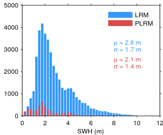
Figure 17. Histogram of flag-valid SWH over oceans and lakes for LRM (blue) and PLRM (red) for 02/09/2016. The mean ( \mu ) and standard deviation ( \sigma ) are also shown. Note that values larger than 12 m are excluded from the histogram for the sake of readability but not from the computation of \mu and \sigma .
