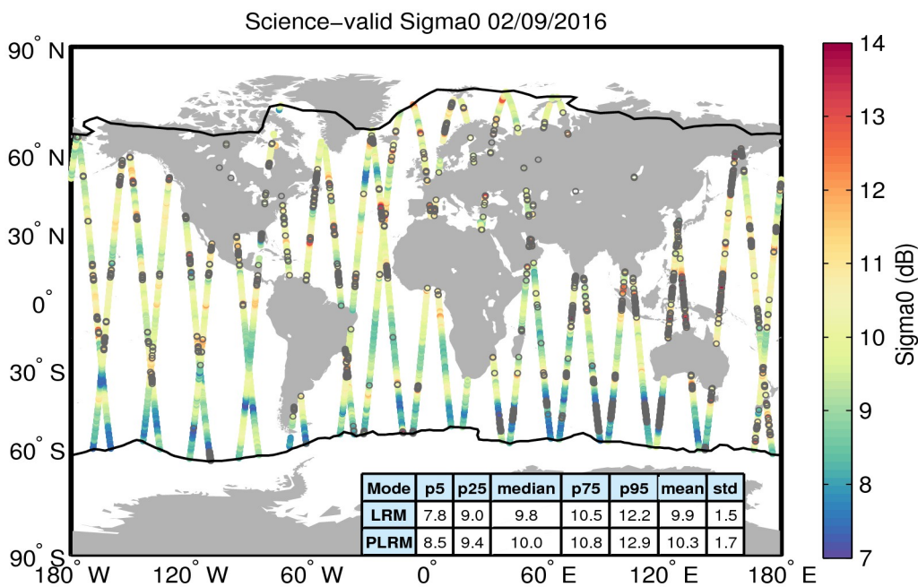
Figure 27. Geographical distribution of science-valid sigma0 data over oceans and lakes for 02/09/2016. The statistical values shown in the table refer to the sigma0 in dB and are calculated separately for LRM and PLRM regions. The black lines mark the outer limit of the Arctic and Antarctic polar polygons. Gray circles denote records that have been rejected based on the editing criteria described in Table 4.
