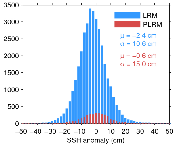
Figure 11. Histogram of science-valid SSH anomaly over oceans and lakes for LRM (blue) and PLRM (red) for 02/09/2016. The mean ( \mu ) and standard deviation ( \sigma ) are also shown. Note that values outside [-50 50] cm are excluded from the histogram for the sake of readability but not from the computation of \mu and \sigma .
