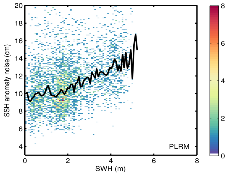
Figure 9. 2D histogram showing flag-valid SSH anomaly noise as a function of SWH for LRM (top) and PLRM (bottom) for 02/09/2016. The black line denotes the median SSH anomaly noise as a function of SWH.
