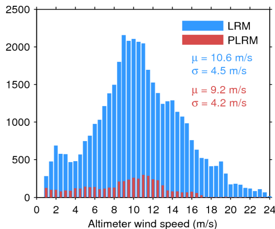
Figure 35. Histogram of science-valid wind over oceans and lakes for LRM (blue) and PLRM (red) for 02/09/2016. The mean ( \mu ) and standard deviation ( \sigma ) are also shown. Note that values larger than 24 m/s are excluded from the histogram for the sake of readability but not from the computation of \mu and \sigma .
