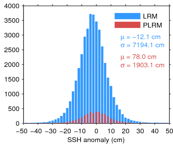
Figure 7. Histogram of flag-valid SSH anomaly over oceans and lakes for LRM (blue) and PLRM (red) for 02/09/2016. The mean ( \mu ) and standard deviation ( \sigma ) are also shown. Note that values outside [-50\ 50] cm are excluded from the histogram for the sake of readability but not from the computation of \mu and \sigma .
