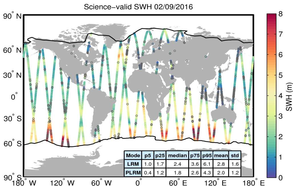
Figure 19. Geographical distribution of science-valid SWH data over oceans and lakes for 02/09/2016. The statistical values shown in the table refer to the SWH in m and are calculated separately for LRM and PLRM regions. The black lines mark the outer limit of the Arctic and Antarctic polar polygons. Gray circles denote records that have been rejected based on the editing criteria described in Table 3.
