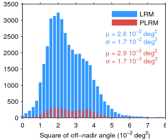
Figure 39. Histogram of flag-valid mispointing over oceans and lakes for LRM (blue) and PLRM (red) for 02/09/2016. Only positive values have been considered. The mean ( \mu ) and standard deviation ( \sigma ) are also shown. Note that values larger than 8 \cdot 10^{-2} \text{ deg}^2 are excluded from the histogram for the sake of readability but not from the computation of \mu and \sigma .
