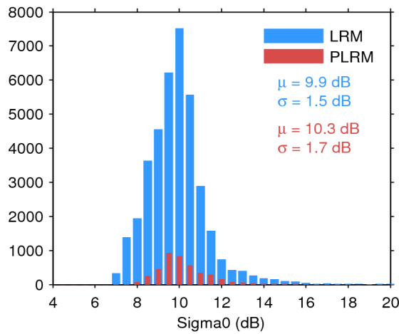
Figure 28. Histogram of science-valid sigma0 over oceans and lakes for LRM (blue) and PLRM (red) for 02/09/2016. The mean ( \mu ) and standard deviation ( \sigma ) are also shown. Note that values outside [4 20] dB are excluded from the histogram for the sake of readability but not from the computation of \mu and \sigma .
