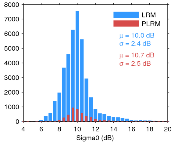
Figure 25. Histogram of flag-valid sigma0 over oceans and lakes for LRM (blue) and PLRM (red) for 02/09/2016. The mean ( \mu ) and standard deviation ( \sigma ) are also shown. Note that values outside [4 20] dB are excluded from the histogram for the sake of readability but not from the computation of \mu and \sigma .
