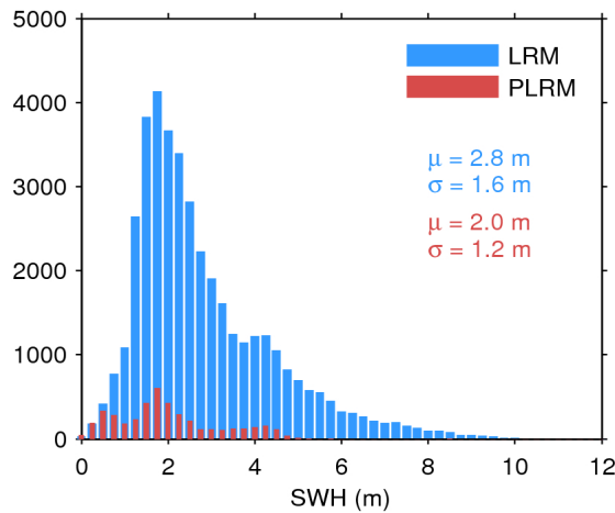
Figure 20. Histogram of science-valid SWH over oceans and lakes for LRM (blue) and PLRM (red) for 02/09/2016. The mean ( \mu ) and standard deviation ( \sigma ) are also shown. Note that values larger than 12 m are excluded from the histogram for the sake of readability but not from the computation of \mu and \sigma .
