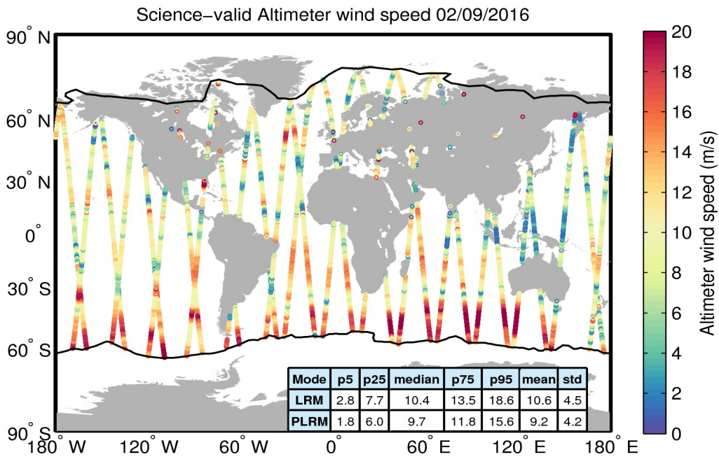
Figure 34. Geographical distribution of science-valid wind data over oceans and lakes for 02/09/2016. The statistical values shown in the table refer to the wind in m/s and are calculated separately for LRM and PLRM regions. The black lines mark the outer limit of the Arctic and Antarctic polar polygons. Gray circles denote records that have been rejected based on the editing criteria described in Table 5.
