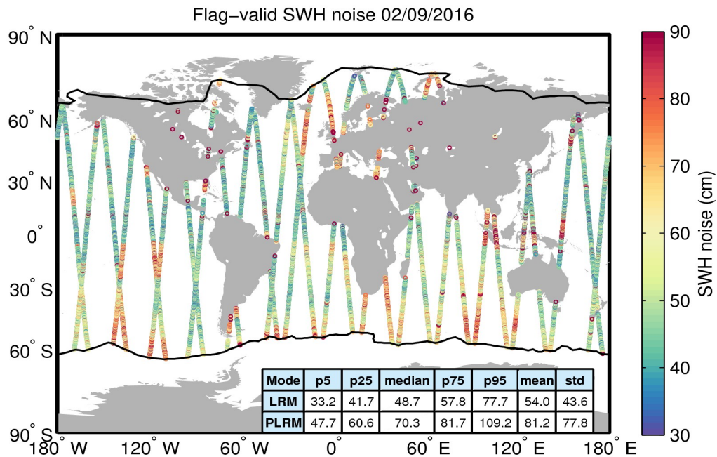
Figure 18. Geographical distribution of flag-valid 20-Hz SWH measurement noise over oceans and lakes for 02/09/2016. The statistical values shown in the table refer to the SWH noise and are calculated separately for LRM and PLRM regions. Measurements taken over polar polygons have been excluded from the computation of the statistical values. The black lines mark the outer limit of the Arctic and Antarctic polar polygons.
