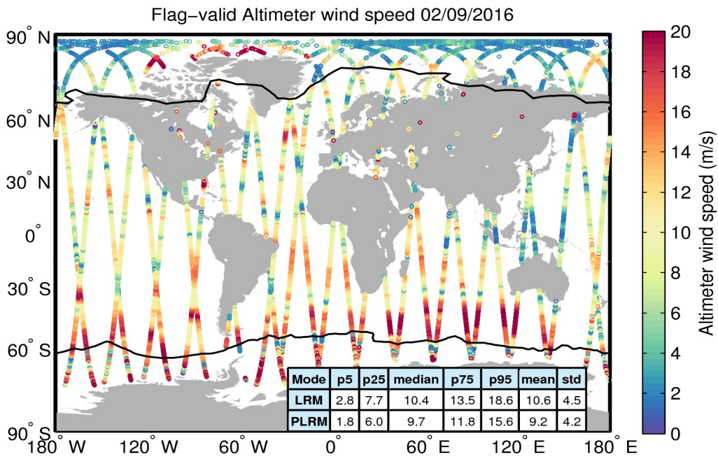
Figure 31. Geographical distribution of flag-valid wind data over oceans and lakes for 02/09/2016. The statistical values shown in the table refer to the wind in m/s and are calculated separately for LRM and PLRM regions. Measurements taken over polar polygons have been excluded from the computation of the statistical values. The black lines mark the outer limit of the Arctic and Antarctic polar polygons.
