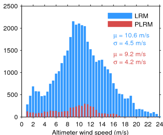
Figure 33. Histogram of flag-valid wind over oceans and lakes for LRM (blue) and PLRM (red) for 02/09/2016. The mean ( \mu ) and standard deviation ( \sigma ) are also shown. Note that values larger than 24 m/s are excluded from the histogram for the sake of readability but not from the computation of \mu and \sigma .
