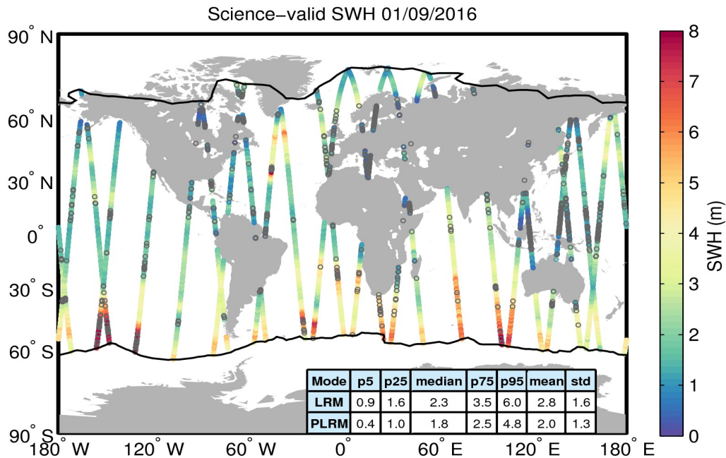
Figure 19. Geographical distribution of science-valid SWH data over oceans and lakes for 01/09/2016. The statistical values shown in the table refer to the SWH in m and are calculated separately for LRM and PLRM regions. The black lines mark the outer limit of the Arctic and Antarctic polar polygons. Gray circles denote records that have been rejected based on the editing criteria described in Table 3.
