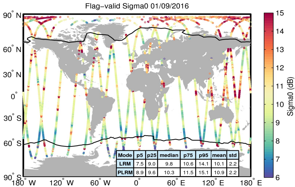
Figure 23. Geographical distribution of flag-valid sigma0 data over oceans and lakes for 01/09/2016. The statistical values shown in the table refer to the sigma0 in dB and are calculated separately for LRM and PLRM regions. Measurements taken over polar polygons have been excluded from the computation of the statistical values. The black lines mark the outer limit of the Arctic and Antarctic polar polygons.
