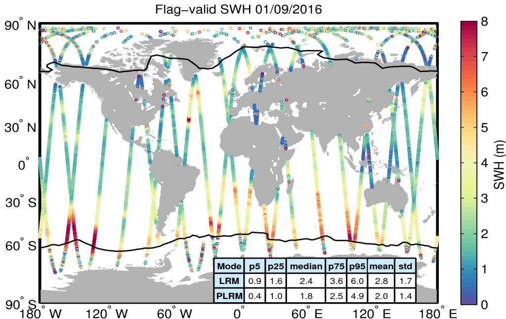
Figure 15. Geographical distribution of flag-valid SWH data over oceans and lakes for 01/09/2016. The statistical values shown in the table refer to the SWH in m and are calculated separately for LRM and PLRM regions. Measurements taken over polar polygons have been excluded from the computation of the statistical values. The black lines mark the outer limit of the Arctic and Antarctic polar polygons.
