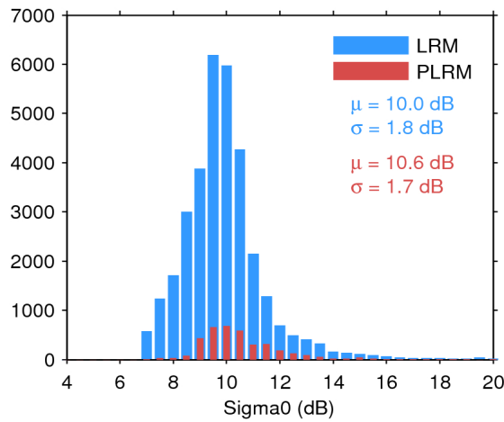
Figure 28. Histogram of science-valid sigma0 over oceans and lakes for LRM (blue) and PLRM (red) for 01/09/2016. The mean ( \mu ) and standard deviation ( \sigma ) are also shown. Note that values outside [4 20] dB are excluded from the histogram for the sake of readability but not from the computation of \mu and \sigma .
