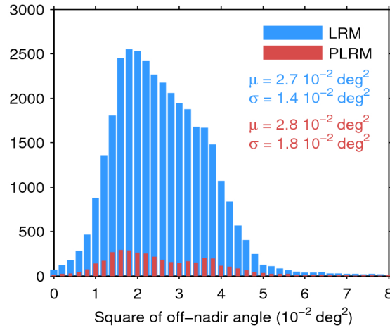
Figure 39. Histogram of flag-valid mispointing over oceans and lakes for LRM (blue) and PLRM (red) for 01/09/2016. Only positive values have been considered. The mean ( \mu ) and standard deviation ( \sigma ) are also shown. Note that values larger than 8 \cdot 10^{-2} \text{ deg}^2 are excluded from the histogram for the sake of readability but not from the computation of \mu and \sigma .
