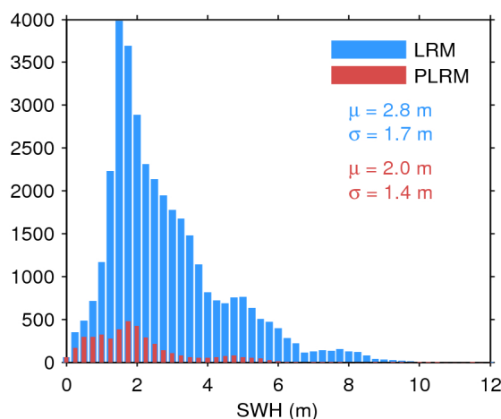
Figure 17. Histogram of flag-valid SWH over oceans and lakes for LRM (blue) and PLRM (red) for 01/09/2016. The mean ( \mu ) and standard deviation ( \sigma ) are also shown. Note that values larger than 12 m are excluded from the histogram for the sake of readability but not from the computation of \mu and \sigma .
