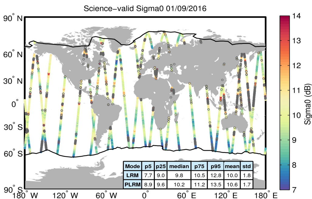
Figure 27. Geographical distribution of science-valid sigma0 data over oceans and lakes for 01/09/2016. The statistical values shown in the table refer to the sigma0 in dB and are calculated separately for LRM and PLRM regions. The black lines mark the outer limit of the Arctic and Antarctic polar polygons. Gray circles denote records that have been rejected based on the editing criteria described in Table 4.
