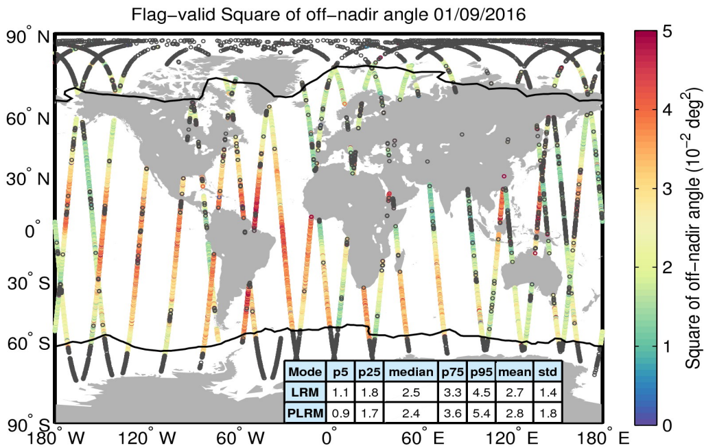
Figure 37. Geographical distribution of flag-valid mispointing data over oceans and lakes for 01/09/2016. The statistical values shown in the table refer to the mispointing in 10^{-2} deg 2 and are calculated separately for LRM and PLRM regions. Measurements taken over polar polygons have been excluded from the computation of the statistical values. The black lines mark the outer limit of the Arctic and Antarctic polar polygons. Gray circles denote negative values.
