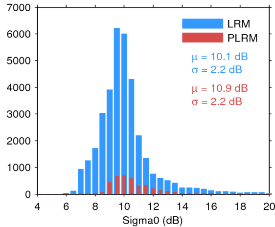
Figure 25. Histogram of flag-valid sigma0 over oceans and lakes for LRM (blue) and PLRM (red) for 01/09/2016. The mean ( \mu ) and standard deviation ( \sigma ) are also shown. Note that values outside [4 20] dB are excluded from the histogram for the sake of readability but not from the computation of \mu and \sigma .
