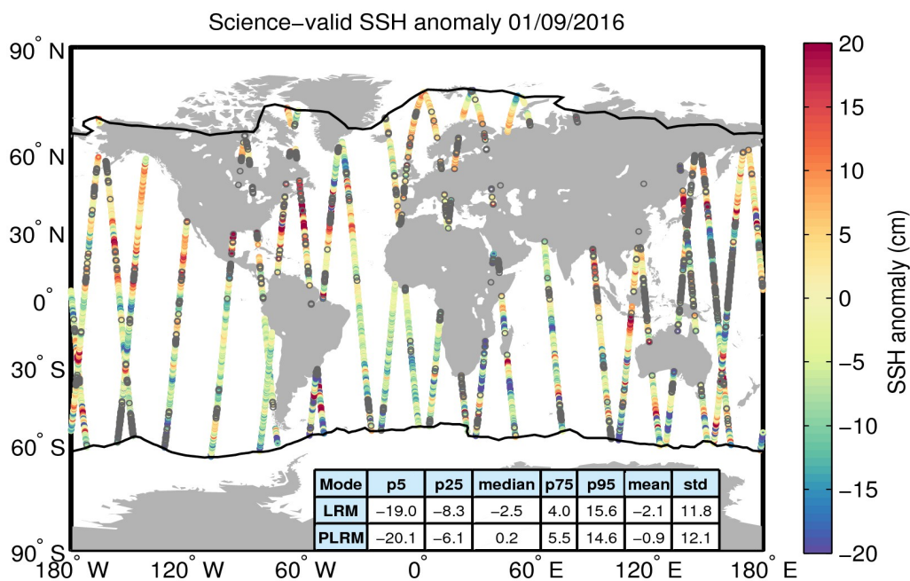
Figure 10. Geographical distribution of science-valid SSH anomaly data over oceans and lakes for 01/09/2016. The statistical values shown in the table refer to the SSH anomaly in cm and are calculated separately for LRM and PLRM regions. The black lines mark the outer limit of the Arctic and Antarctic polar polygons. Gray circles denote records that have been rejected based on the editing criteria described in Table 2.
