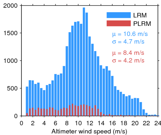
Figure 35. Histogram of science-valid wind over oceans and lakes for LRM (blue) and PLRM (red) for 01/09/2016. The mean ( \mu ) and standard deviation ( \sigma ) are also shown. Note that values larger than 24 m/s are excluded from the histogram for the sake of readability but not from the computation of \mu and \sigma .
