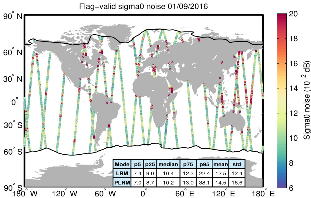
Figure 26. Geographical distribution of flag-valid 20-Hz sigma0 measurement noise over oceans and lakes for 01/09/2016. The statistical values shown in the table refer to the sigma0 noise and are calculated separately for LRM and PLRM regions. Measurements taken over polar polygons have been excluded from the computation of the statistical values. The black lines mark the outer limit of the Arctic and Antarctic polar polygons.
