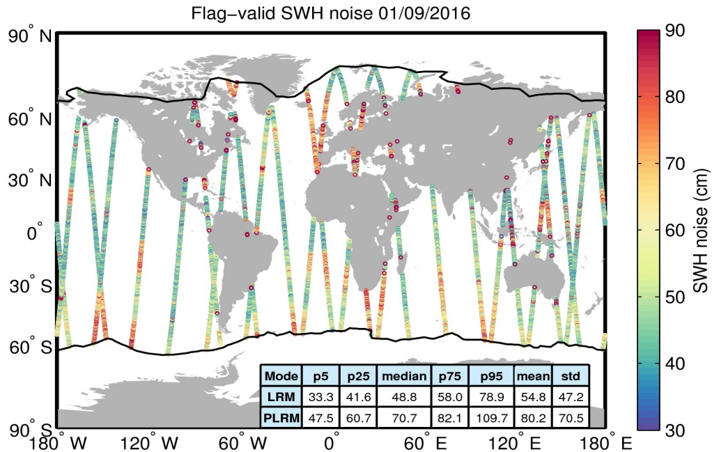
Figure 18. Geographical distribution of flag-valid 20-Hz SWH measurement noise over oceans and lakes for 01/09/2016. The statistical values shown in the table refer to the SWH noise and are calculated separately for LRM and PLRM regions. Measurements taken over polar polygons have been excluded from the computation of the statistical values. The black lines mark the outer limit of the Arctic and Antarctic polar polygons.
