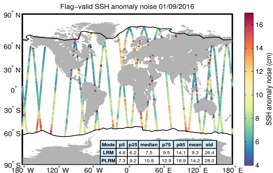
Figure 8. Geographical distribution of flag-valid 20-Hz SSH anomaly measurement noise over oceans and lakes for 01/09/2016. The statistical values shown in the table refer to the SSH anomaly noise and are calculated separately for LRM and PLRM regions. Measurements taken over polar polygons have been excluded from the computation of the statistical values. The black lines mark the outer limit of the Arctic and Antarctic polar polygons.
