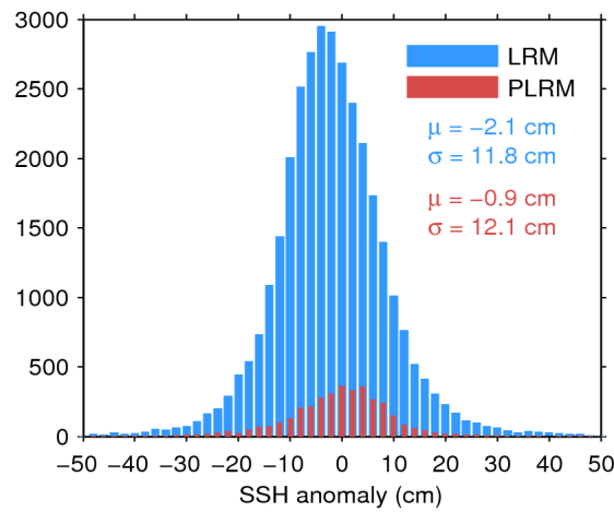
Figure 11. Histogram of science-valid SSH anomaly over oceans and lakes for LRM (blue) and PLRM (red) for 01/09/2016. The mean ( \mu ) and standard deviation ( \sigma ) are also shown. Note that values outside [-50\ 50] cm are excluded from the histogram for the sake of readability but not from the computation of \mu and \sigma .
