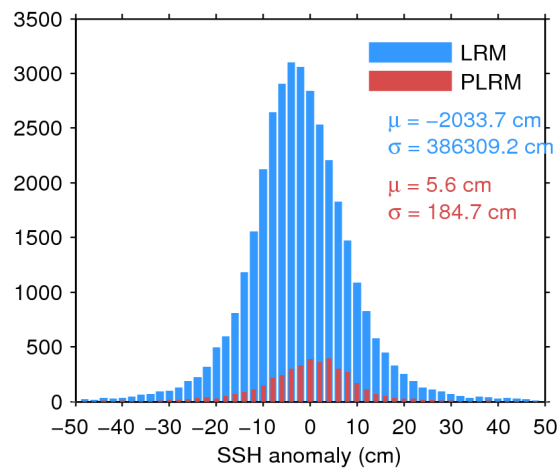
Figure 7. Histogram of flag-valid SSH anomaly over oceans and lakes for LRM (blue) and PLRM (red) for 01/09/2016. The mean ( \mu ) and standard deviation ( \sigma ) are also shown. Note that values outside [-50\ 50] cm are excluded from the histogram for the sake of readability but not from the computation of \mu and \sigma .
