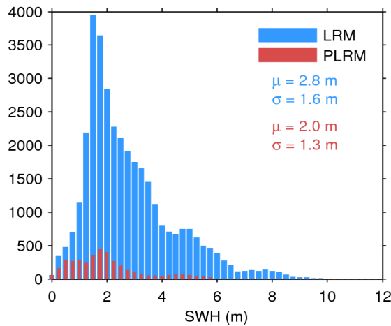
Figure 20. Histogram of science-valid SWH over oceans and lakes for LRM (blue) and PLRM (red) for 01/09/2016. The mean ( \mu ) and standard deviation ( \sigma ) are also shown. Note that values larger than 12 m are excluded from the histogram for the sake of readability but not from the computation of \mu and \sigma .
