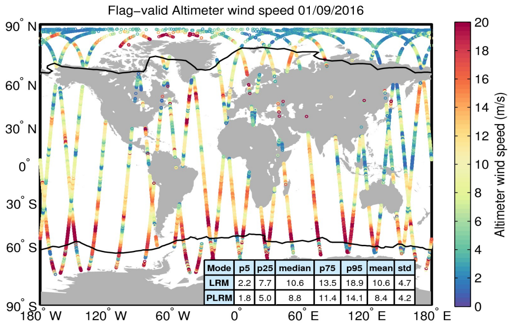
Figure 31. Geographical distribution of flag-valid wind data over oceans and lakes for 01/09/2016. The statistical values shown in the table refer to the wind in m/s and are calculated separately for LRM and PLRM regions. Measurements taken over polar polygons have been excluded from the computation of the statistical values. The black lines mark the outer limit of the Arctic and Antarctic polar polygons.
