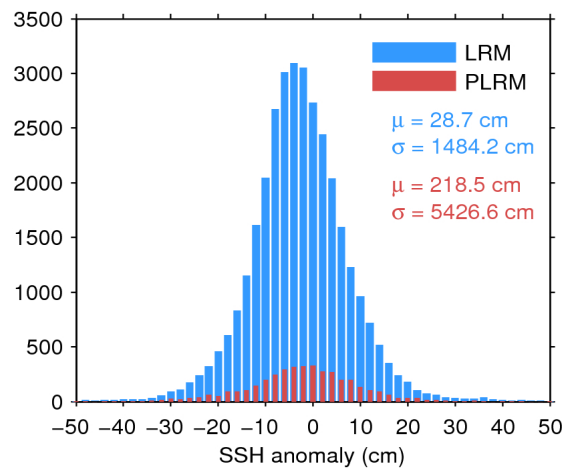
Figure 7. Histogram of flag-valid SSH anomaly over oceans and lakes for LRM (blue) and PLRM (red) for 31/08/2016. The mean ( \mu ) and standard deviation ( \sigma ) are also shown. Note that values outside [-50\ 50] cm are excluded from the histogram for the sake of readability but not from the computation of \mu and \sigma .
