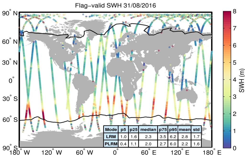
Figure 15. Geographical distribution of flag-valid SWH data over oceans and lakes for 31/08/2016. The statistical values shown in the table refer to the SWH in m and are calculated separately for LRM and PLRM regions. Measurements taken over polar polygons have been excluded from the computation of the statistical values. The black lines mark the outer limit of the Arctic and Antarctic polar polygons.
