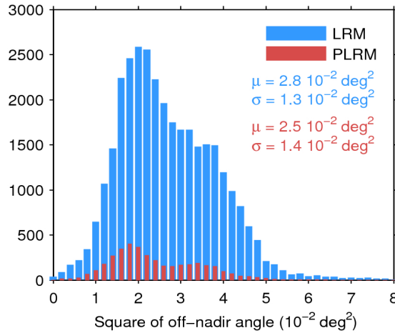
Figure 39. Histogram of flag-valid mispointing over oceans and lakes for LRM (blue) and PLRM (red) for 31/08/2016. Only positive values have been considered. The mean ( \mu ) and standard deviation ( \sigma ) are also shown. Note that values larger than 8 \cdot 10^{-2} \text{ deg}^2 are excluded from the histogram for the sake of readability but not from the computation of \mu and \sigma .
