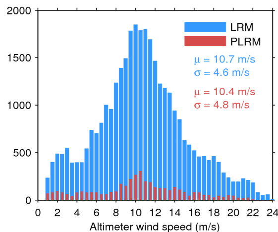
Figure 35. Histogram of science-valid wind over oceans and lakes for LRM (blue) and PLRM (red) for 31/08/2016. The mean ( \mu ) and standard deviation ( \sigma ) are also shown. Note that values larger than 24 m/s are excluded from the histogram for the sake of readability but not from the computation of \mu and \sigma .
