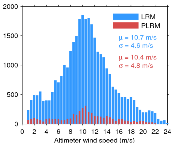
Figure 33. Histogram of flag-valid wind over oceans and lakes for LRM (blue) and PLRM (red) for 31/08/2016. The mean ( \mu ) and standard deviation ( \sigma ) are also shown. Note that values larger than 24 m/s are excluded from the histogram for the sake of readability but not from the computation of \mu and \sigma .
