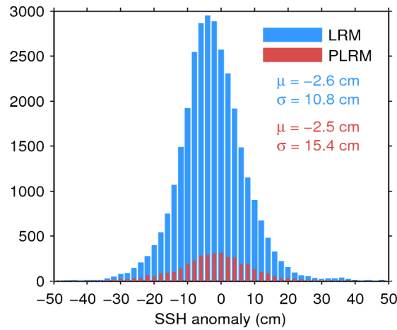
Figure 11. Histogram of science-valid SSH anomaly over oceans and lakes for LRM (blue) and PLRM (red) for 31/08/2016. The mean ( \mu ) and standard deviation ( \sigma ) are also shown. Note that values outside [-50 50] cm are excluded from the histogram for the sake of readability but not from the computation of \mu and \sigma .
