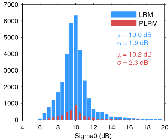
Figure 25. Histogram of flag-valid sigma0 over oceans and lakes for LRM (blue) and PLRM (red) for 31/08/2016. The mean ( \mu ) and standard deviation ( \sigma ) are also shown. Note that values outside [4 20] dB are excluded from the histogram for the sake of readability but not from the computation of \mu and \sigma .
