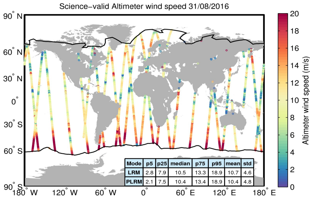
Figure 34. Geographical distribution of science-valid wind data over oceans and lakes for 31/08/2016. The statistical values shown in the table refer to the wind in m/s and are calculated separately for LRM and PLRM regions. The black lines mark the outer limit of the Arctic and Antarctic polar polygons. Gray circles denote records that have been rejected based on the editing criteria described in Table 5.
