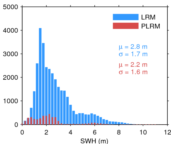
Figure 17. Histogram of flag-valid SWH over oceans and lakes for LRM (blue) and PLRM (red) for 31/08/2016. The mean ( \mu ) and standard deviation ( \sigma ) are also shown. Note that values larger than 12 m are excluded from the histogram for the sake of readability but not from the computation of \mu and \sigma .
