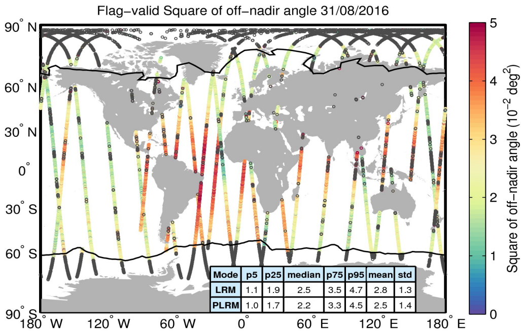
Figure 37. Geographical distribution of flag-valid mispointing data over oceans and lakes for 31/08/2016. The statistical values shown in the table refer to the mispointing in 10^{-2} deg 2 and are calculated separately for LRM and PLRM regions. Measurements taken over polar polygons have been excluded from the computation of the statistical values. The black lines mark the outer limit of the Arctic and Antarctic polar polygons. Gray circles denote negative values.
