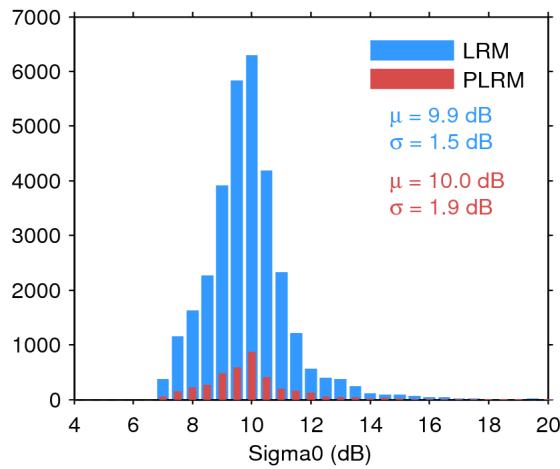
Figure 28. Histogram of science-valid sigma0 over oceans and lakes for LRM (blue) and PLRM (red) for 31/08/2016. The mean ( \mu ) and standard deviation ( \sigma ) are also shown. Note that values outside [4 20] dB are excluded from the histogram for the sake of readability but not from the computation of \mu and \sigma .
