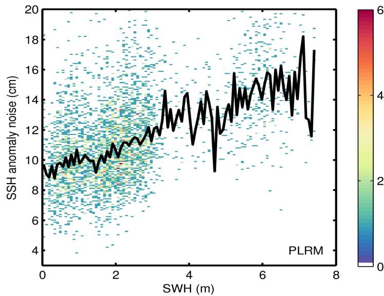
Figure 9. 2D histogram showing flag-valid SSH anomaly noise as a function of SWH for LRM (top) and PLRM (bottom) for 31/08/2016. The black line denotes the median SSH anomaly noise as a function of SWH.
