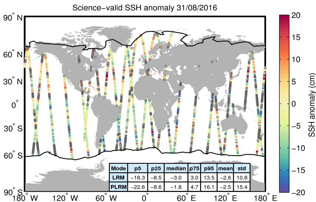
Figure 10. Geographical distribution of science-valid SSH anomaly data over oceans and lakes for 31/08/2016. The statistical values shown in the table refer to the SSH anomaly in cm and are calculated separately for LRM and PLRM regions. The black lines mark the outer limit of the Arctic and Antarctic polar polygons. Gray circles denote records that have been rejected based on the editing criteria described in Table 2.
