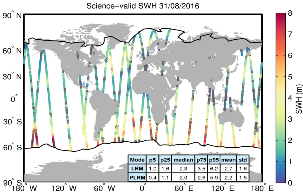
Figure 19. Geographical distribution of science-valid SWH data over oceans and lakes for 31/08/2016. The statistical values shown in the table refer to the SWH in m and are calculated separately for LRM and PLRM regions. The black lines mark the outer limit of the Arctic and Antarctic polar polygons. Gray circles denote records that have been rejected based on the editing criteria described in Table 3.
