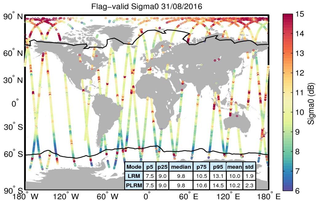
Figure 23. Geographical distribution of flag-valid sigma0 data over oceans and lakes for 31/08/2016. The statistical values shown in the table refer to the sigma0 in dB and are calculated separately for LRM and PLRM regions. Measurements taken over polar polygons have been excluded from the computation of the statistical values. The black lines mark the outer limit of the Arctic and Antarctic polar polygons.
