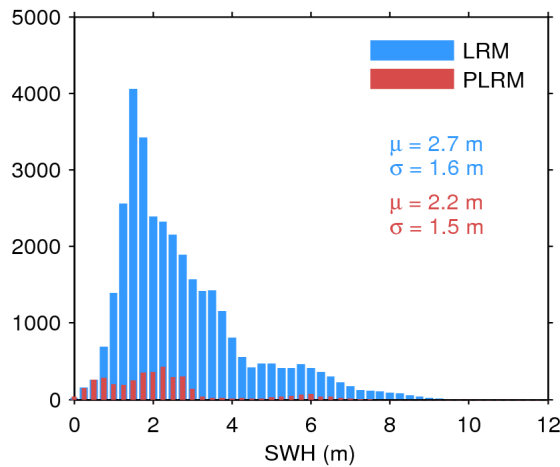
Figure 20. Histogram of science-valid SWH over oceans and lakes for LRM (blue) and PLRM (red) for 31/08/2016. The mean ( \mu ) and standard deviation ( \sigma ) are also shown. Note that values larger than 12 m are excluded from the histogram for the sake of readability but not from the computation of \mu and \sigma .
