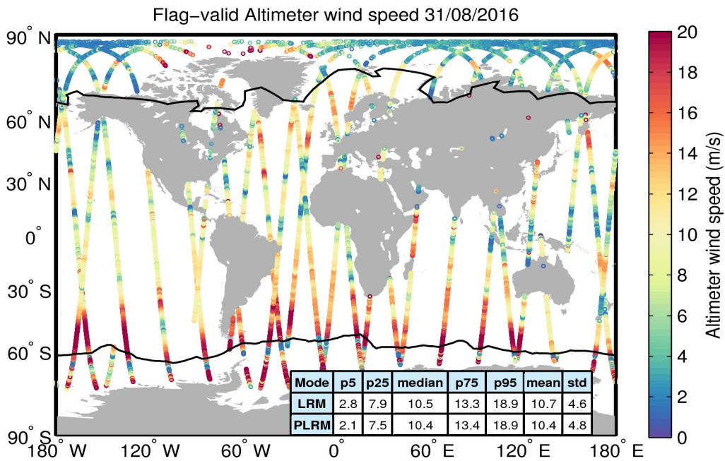
Figure 31. Geographical distribution of flag-valid wind data over oceans and lakes for 31/08/2016. The statistical values shown in the table refer to the wind in m/s and are calculated separately for LRM and PLRM regions. Measurements taken over polar polygons have been excluded from the computation of the statistical values. The black lines mark the outer limit of the Arctic and Antarctic polar polygons.
