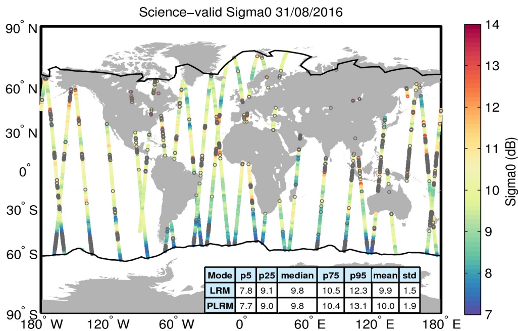
Figure 27. Geographical distribution of science-valid sigma0 data over oceans and lakes for 31/08/2016. The statistical values shown in the table refer to the sigma0 in dB and are calculated separately for LRM and PLRM regions. The black lines mark the outer limit of the Arctic and Antarctic polar polygons. Gray circles denote records that have been rejected based on the editing criteria described in Table 4.
