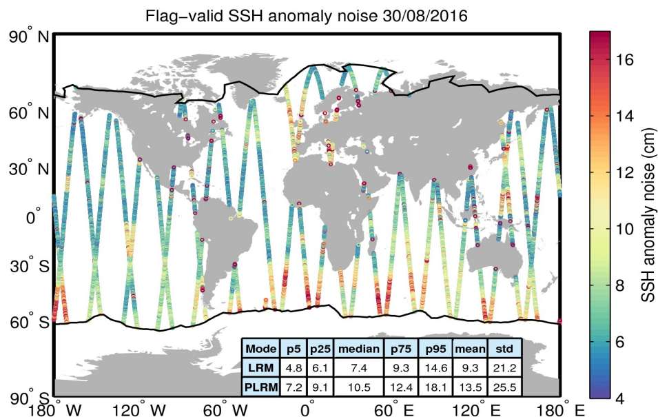
Figure 8. Geographical distribution of flag-valid 20-Hz SSH anomaly measurement noise over oceans and lakes for 30/08/2016. The statistical values shown in the table refer to the SSH anomaly noise and are calculated separately for LRM and PLRM regions. Measurements taken over polar polygons have been excluded from the computation of the statistical values. The black lines mark the outer limit of the Arctic and Antarctic polar polygons.
