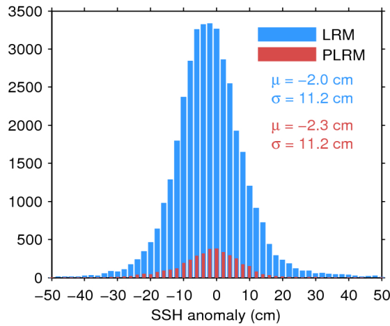
Figure 11. Histogram of science-valid SSH anomaly over oceans and lakes for LRM (blue) and PLRM (red) for 30/08/2016. The mean ( \mu ) and standard deviation ( \sigma ) are also shown. Note that values outside [-50\ 50] cm are excluded from the histogram for the sake of readability but not from the computation of \mu and \sigma .
