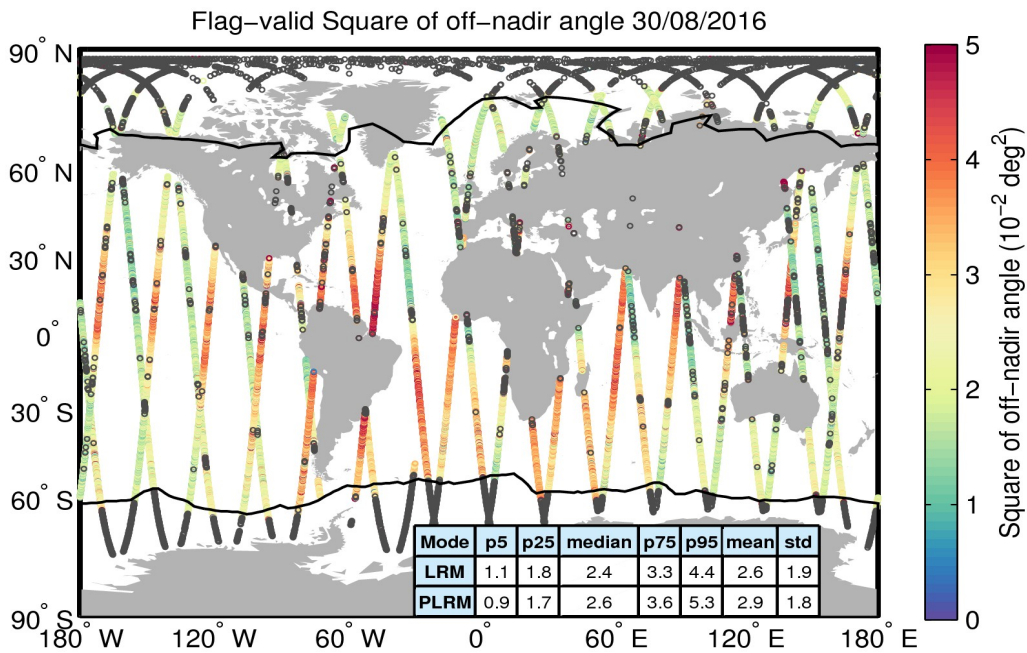
Figure 37. Geographical distribution of flag-valid mispointing data over oceans and lakes for 30/08/2016. The statistical values shown in the table refer to the mispointing in 10^{-2} deg 2 and are calculated separately for LRM and PLRM regions. Measurements taken over polar polygons have been excluded from the computation of the statistical values. The black lines mark the outer limit of the Arctic and Antarctic polar polygons. Gray circles denote negative values.
