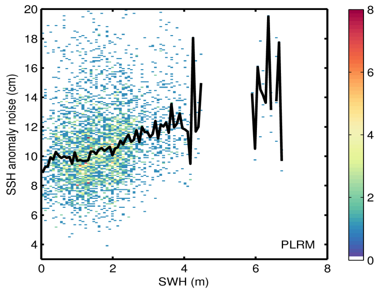
Figure 9. 2D histogram showing flag-valid SSH anomaly noise as a function of SWH for LRM (top) and PLRM (bottom) for 30/08/2016. The black line denotes the median SSH anomaly noise as a function of SWH.
