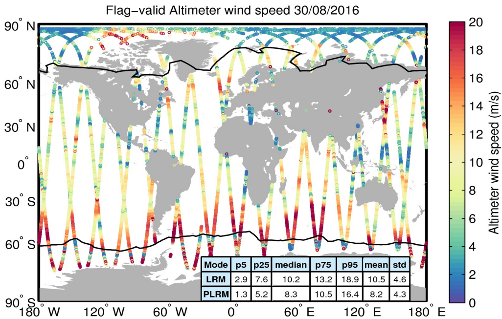
Figure 31. Geographical distribution of flag-valid wind data over oceans and lakes for 30/08/2016. The statistical values shown in the table refer to the wind in m/s and are calculated separately for LRM and PLRM regions. Measurements taken over polar polygons have been excluded from the computation of the statistical values. The black lines mark the outer limit of the Arctic and Antarctic polar polygons.
