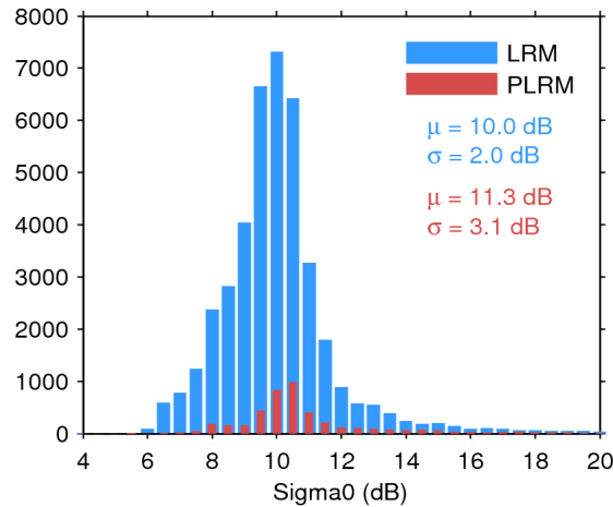
Figure 25. Histogram of flag-valid sigma0 over oceans and lakes for LRM (blue) and PLRM (red) for 30/08/2016. The mean ( \mu ) and standard deviation ( \sigma ) are also shown. Note that values outside [4 20] dB are excluded from the histogram for the sake of readability but not from the computation of \mu and \sigma .
