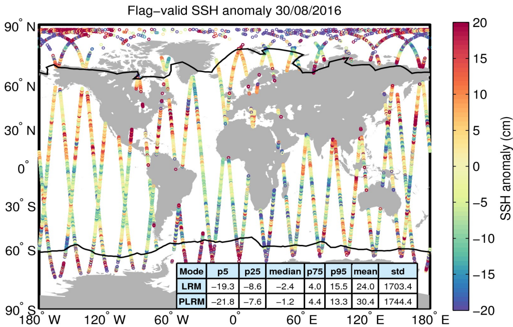
Figure 5. Geographical distribution of flag-valid 1-Hz SSH anomaly data over oceans and lakes for 30/08/2016. The statistical values shown in the table refer to the SSH anomaly in cm and are calculated separately for LRM and PLRM regions. Measurements taken over polar polygons have been excluded from the computation of the statistical values. The black lines mark the outer limit of the Arctic and Antarctic polar polygons.
