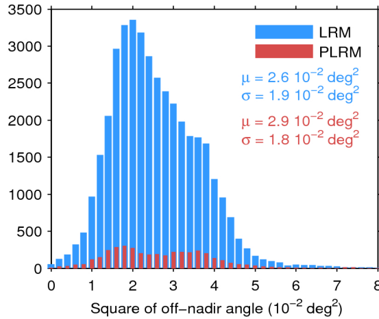
Figure 39. Histogram of flag-valid mispointing over oceans and lakes for LRM (blue) and PLRM (red) for 30/08/2016. Only positive values have been considered. The mean ( \mu ) and standard deviation ( \sigma ) are also shown. Note that values larger than 8 \cdot 10^{-2} \text{ deg}^2 are excluded from the histogram for the sake of readability but not from the computation of \mu and \sigma .
