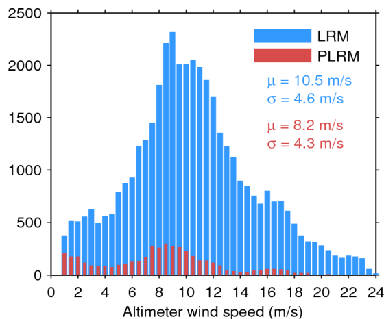
Figure 35. Histogram of science-valid wind over oceans and lakes for LRM (blue) and PLRM (red) for 30/08/2016. The mean ( \mu ) and standard deviation ( \sigma ) are also shown. Note that values larger than 24 m/s are excluded from the histogram for the sake of readability but not from the computation of \mu and \sigma .
