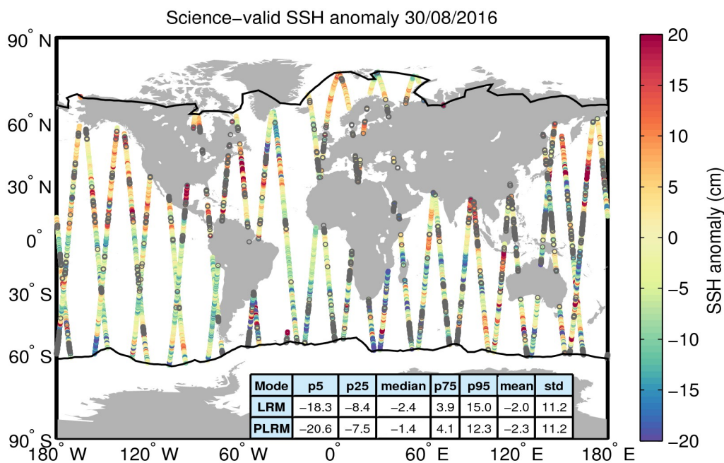
Figure 10. Geographical distribution of science-valid SSH anomaly data over oceans and lakes for 30/08/2016. The statistical values shown in the table refer to the SSH anomaly in cm and are calculated separately for LRM and PLRM regions. The black lines mark the outer limit of the Arctic and Antarctic polar polygons. Gray circles denote records that have been rejected based on the editing criteria described in Table 2.
