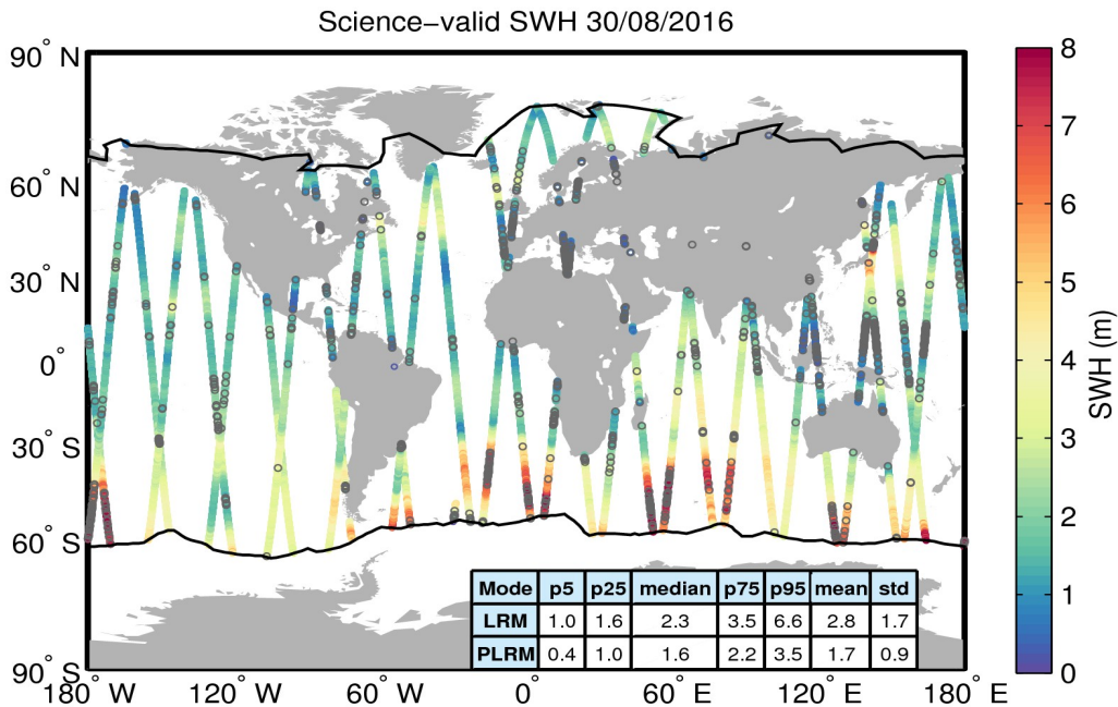
Figure 19. Geographical distribution of science-valid SWH data over oceans and lakes for 30/08/2016. The statistical values shown in the table refer to the SWH in m and are calculated separately for LRM and PLRM regions. The black lines mark the outer limit of the Arctic and Antarctic polar polygons. Gray circles denote records that have been rejected based on the editing criteria described in Table 3.
