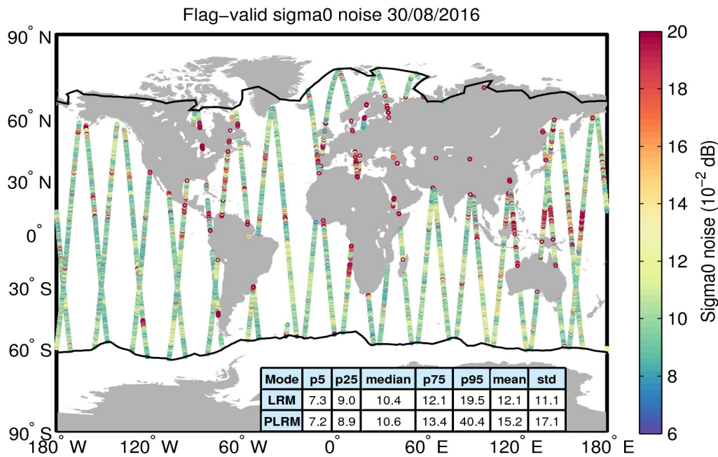
Figure 26. Geographical distribution of flag-valid 20-Hz sigma0 measurement noise over oceans and lakes for 30/08/2016. The statistical values shown in the table refer to the sigma0 noise and are calculated separately for LRM and PLRM regions. Measurements taken over polar polygons have been excluded from the computation of the statistical values. The black lines mark the outer limit of the Arctic and Antarctic polar polygons.
