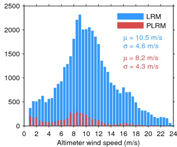
Figure 33. Histogram of flag-valid wind over oceans and lakes for LRM (blue) and PLRM (red) for 30/08/2016. The mean ( \mu ) and standard deviation ( \sigma ) are also shown. Note that values larger than 24 m/s are excluded from the histogram for the sake of readability but not from the computation of \mu and \sigma .
