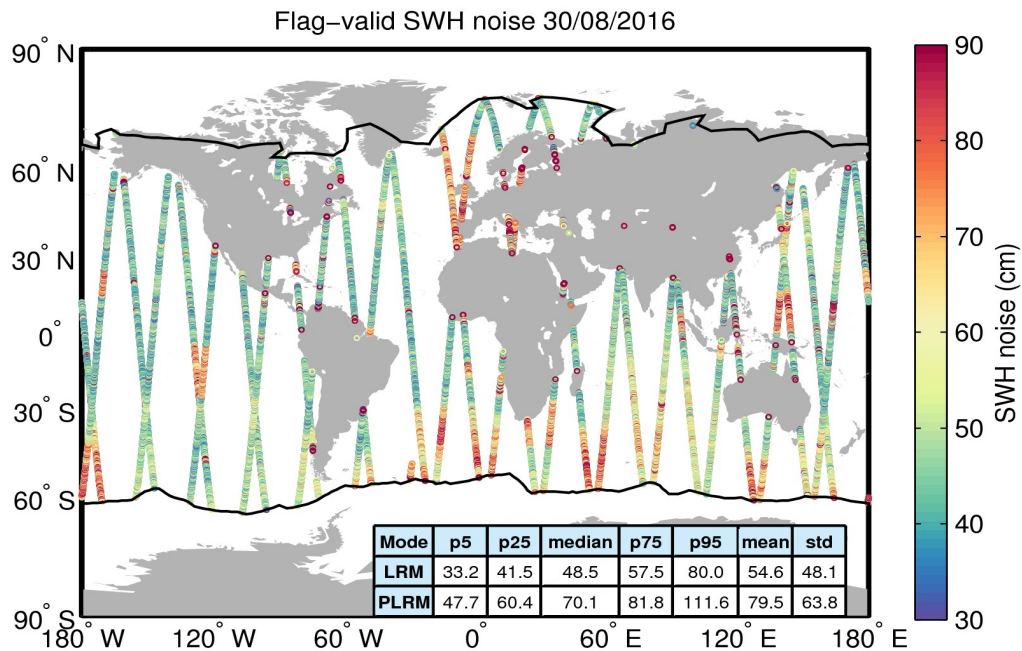
Figure 18. Geographical distribution of flag-valid 20-Hz SWH measurement noise over oceans and lakes for 30/08/2016. The statistical values shown in the table refer to the SWH noise and are calculated separately for LRM and PLRM regions. Measurements taken over polar polygons have been excluded from the computation of the statistical values. The black lines mark the outer limit of the Arctic and Antarctic polar polygons.
