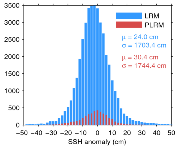
Figure 7. Histogram of flag-valid SSH anomaly over oceans and lakes for LRM (blue) and PLRM (red) for 30/08/2016. The mean ( \mu ) and standard deviation ( \sigma ) are also shown. Note that values outside [-50\ 50] cm are excluded from the histogram for the sake of readability but not from the computation of \mu and \sigma .
