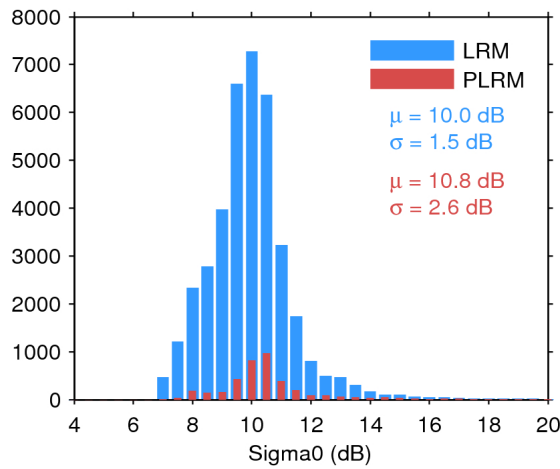
Figure 28. Histogram of science-valid sigma0 over oceans and lakes for LRM (blue) and PLRM (red) for 30/08/2016. The mean ( \mu ) and standard deviation ( \sigma ) are also shown. Note that values outside [4 20] dB are excluded from the histogram for the sake of readability but not from the computation of \mu and \sigma .
