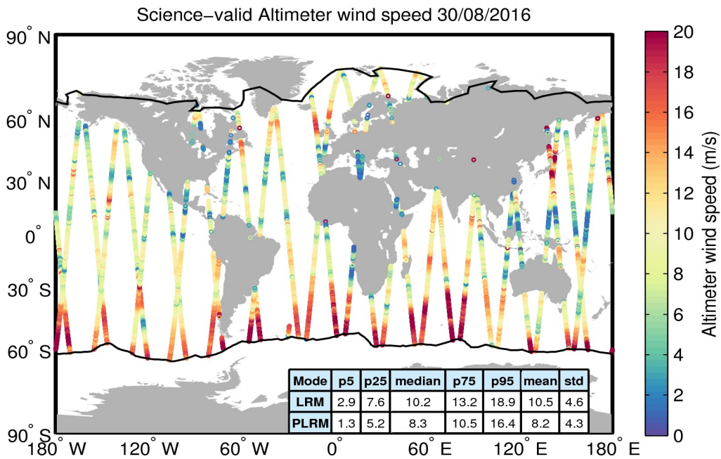
Figure 34. Geographical distribution of science-valid wind data over oceans and lakes for 30/08/2016. The statistical values shown in the table refer to the wind in m/s and are calculated separately for LRM and PLRM regions. The black lines mark the outer limit of the Arctic and Antarctic polar polygons. Gray circles denote records that have been rejected based on the editing criteria described in Table 5.
