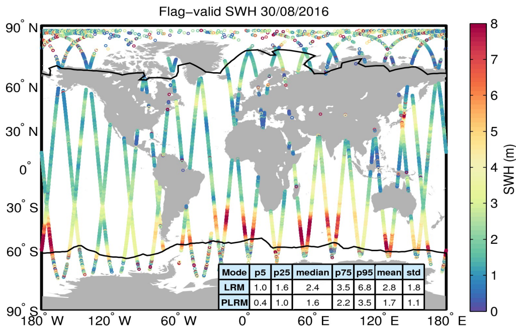
Figure 15. Geographical distribution of flag-valid SWH data over oceans and lakes for 30/08/2016. The statistical values shown in the table refer to the SWH in m and are calculated separately for LRM and PLRM regions. Measurements taken over polar polygons have been excluded from the computation of the statistical values. The black lines mark the outer limit of the Arctic and Antarctic polar polygons.
