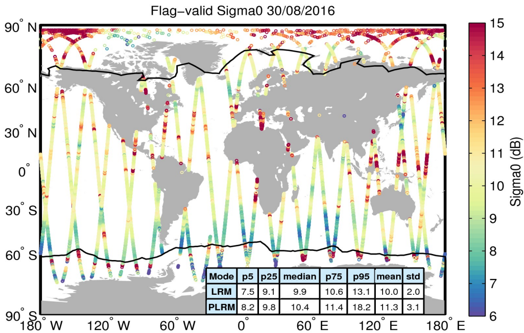
Figure 23. Geographical distribution of flag-valid sigma0 data over oceans and lakes for 30/08/2016. The statistical values shown in the table refer to the sigma0 in dB and are calculated separately for LRM and PLRM regions. Measurements taken over polar polygons have been excluded from the computation of the statistical values. The black lines mark the outer limit of the Arctic and Antarctic polar polygons.
