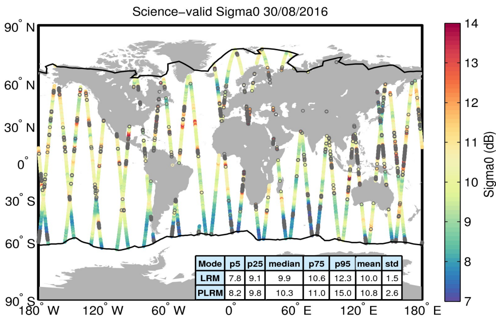
Figure 27. Geographical distribution of science-valid sigma0 data over oceans and lakes for 30/08/2016. The statistical values shown in the table refer to the sigma0 in dB and are calculated separately for LRM and PLRM regions. The black lines mark the outer limit of the Arctic and Antarctic polar polygons. Gray circles denote records that have been rejected based on the editing criteria described in Table 4.
