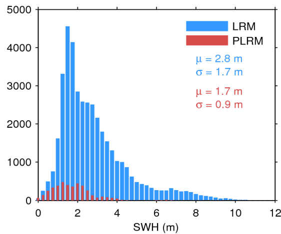
Figure 20. Histogram of science-valid SWH over oceans and lakes for LRM (blue) and PLRM (red) for 30/08/2016. The mean ( \mu ) and standard deviation ( \sigma ) are also shown. Note that values larger than 12 m are excluded from the histogram for the sake of readability but not from the computation of \mu and \sigma .
