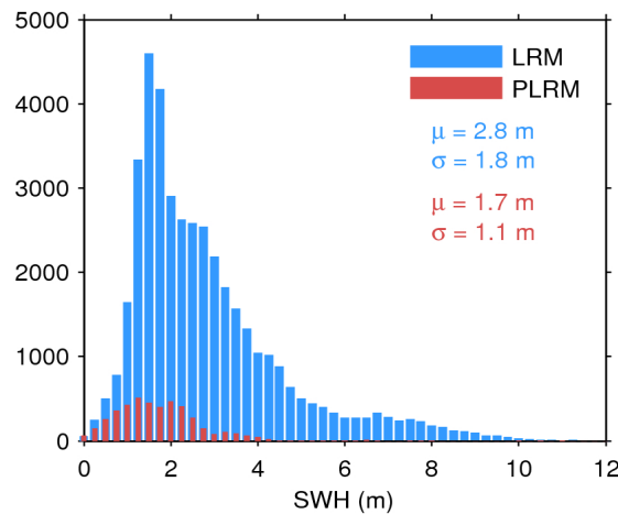
Figure 17. Histogram of flag-valid SWH over oceans and lakes for LRM (blue) and PLRM (red) for 30/08/2016. The mean ( \mu ) and standard deviation ( \sigma ) are also shown. Note that values larger than 12 m are excluded from the histogram for the sake of readability but not from the computation of \mu and \sigma .
