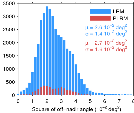
Figure 39. Histogram of flag-valid mispointing over oceans and lakes for LRM (blue) and PLRM (red) for 25/08/2016. Only positive values have been considered. The mean ( \mu ) and standard deviation ( \sigma ) are also shown. Note that values larger than 8 \cdot 10^{-2} \text{ deg}^2 are excluded from the histogram for the sake of readability but not from the computation of \mu and \sigma .
