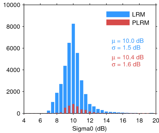
Figure 28. Histogram of science-valid sigma0 over oceans and lakes for LRM (blue) and PLRM (red) for 25/08/2016. The mean ( \mu ) and standard deviation ( \sigma ) are also shown. Note that values outside [4 20] dB are excluded from the histogram for the sake of readability but not from the computation of \mu and \sigma .
