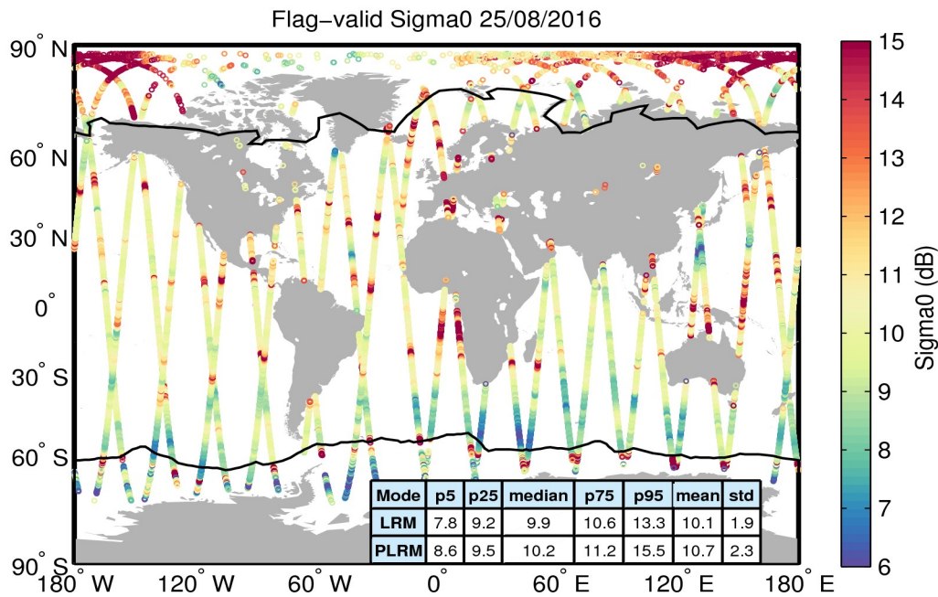
Figure 23. Geographical distribution of flag-valid sigma0 data over oceans and lakes for 25/08/2016. The statistical values shown in the table refer to the sigma0 in dB and are calculated separately for LRM and PLRM regions. Measurements taken over polar polygons have been excluded from the computation of the statistical values. The black lines mark the outer limit of the Arctic and Antarctic polar polygons.
