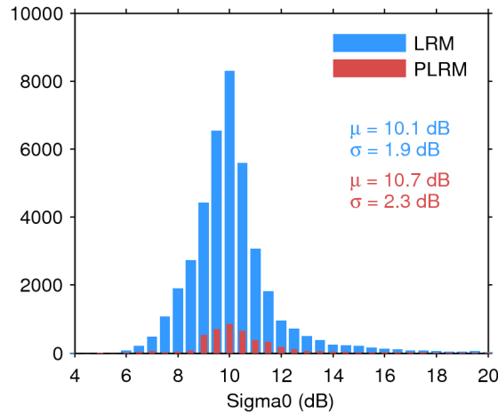
Figure 25. Histogram of flag-valid sigma0 over oceans and lakes for LRM (blue) and PLRM (red) for 25/08/2016. The mean ( \mu ) and standard deviation ( \sigma ) are also shown. Note that values outside [4 20] dB are excluded from the histogram for the sake of readability but not from the computation of \mu and \sigma .
