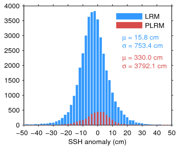
Figure 7. Histogram of flag-valid SSH anomaly over oceans and lakes for LRM (blue) and PLRM (red) for 25/08/2016. The mean ( \mu ) and standard deviation ( \sigma ) are also shown. Note that values outside [-50\ 50] cm are excluded from the histogram for the sake of readability but not from the computation of \mu and \sigma .
