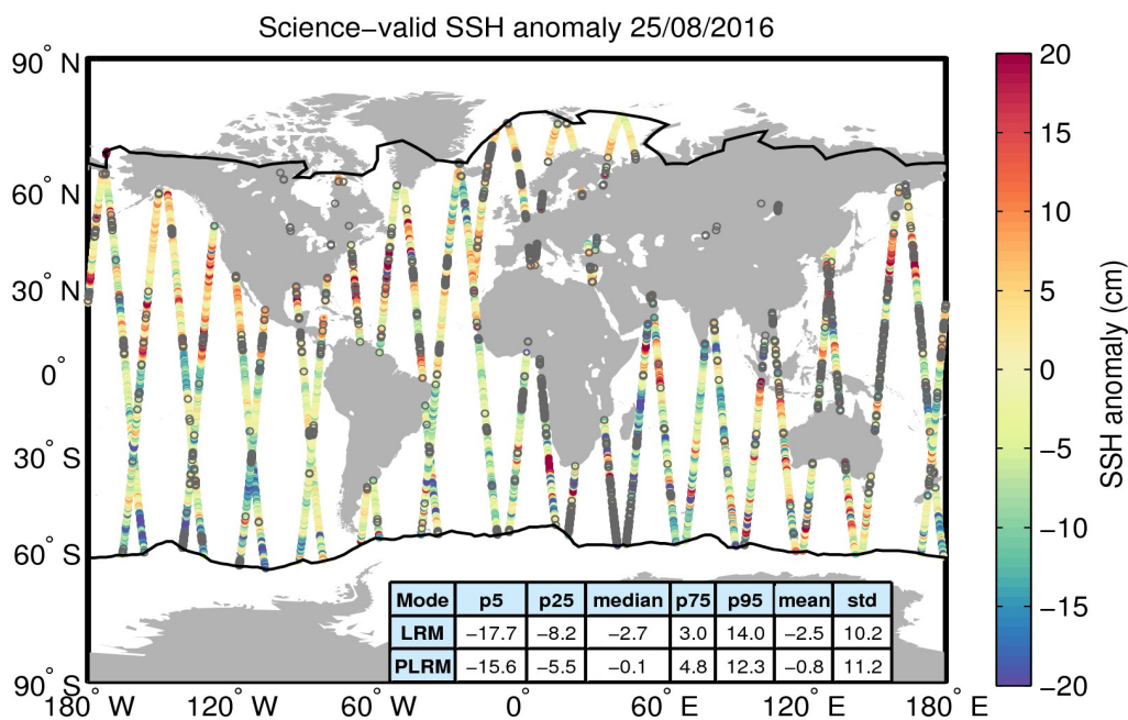
Figure 10. Geographical distribution of science-valid SSH anomaly data over oceans and lakes for 25/08/2016. The statistical values shown in the table refer to the SSH anomaly in cm and are calculated separately for LRM and PLRM regions. The black lines mark the outer limit of the Arctic and Antarctic polar polygons. Gray circles denote records that have been rejected based on the editing criteria described in Table 2.
