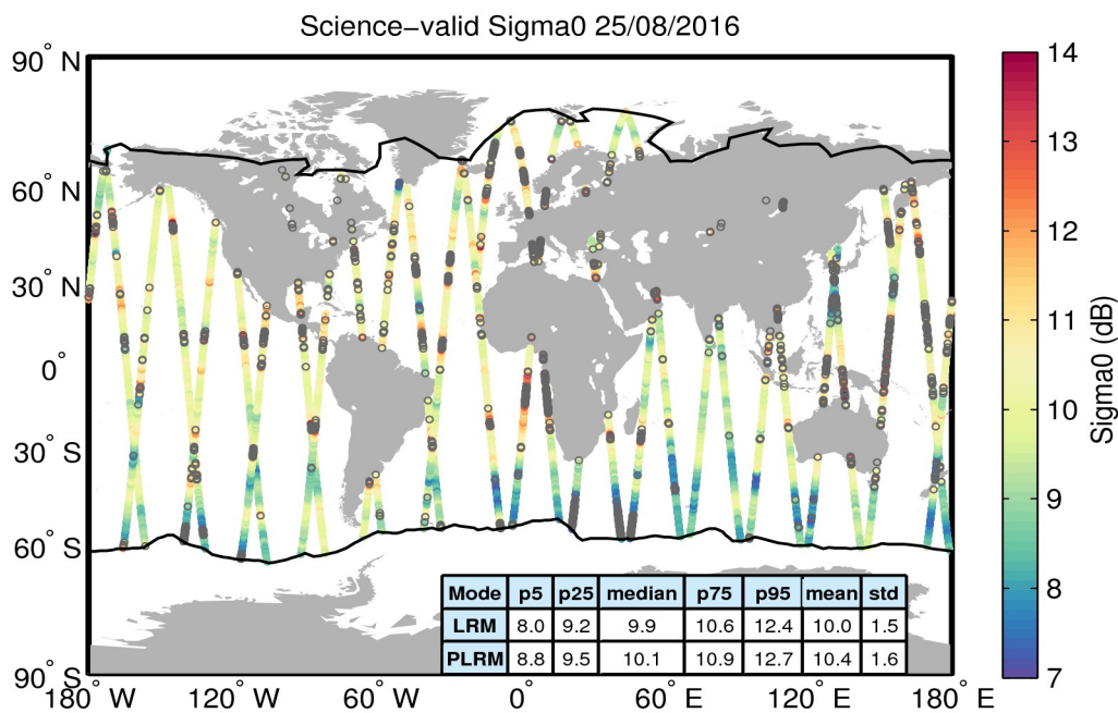
Figure 27. Geographical distribution of science-valid sigma0 data over oceans and lakes for 25/08/2016. The statistical values shown in the table refer to the sigma0 in dB and are calculated separately for LRM and PLRM regions. The black lines mark the outer limit of the Arctic and Antarctic polar polygons. Gray circles denote records that have been rejected based on the editing criteria described in Table 4.
