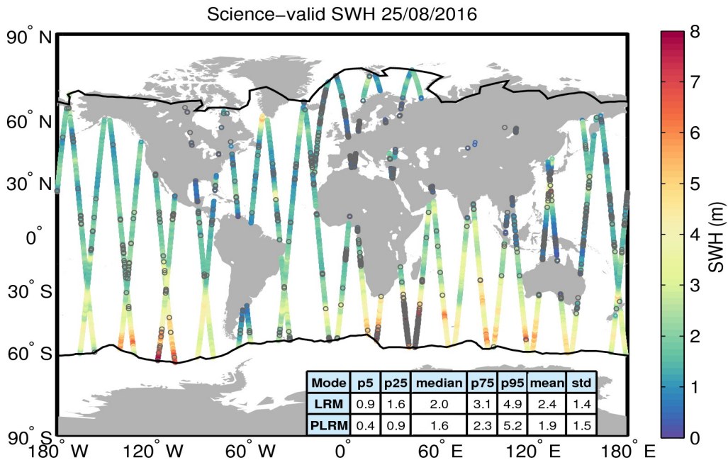
Figure 19. Geographical distribution of science-valid SWH data over oceans and lakes for 25/08/2016. The statistical values shown in the table refer to the SWH in m and are calculated separately for LRM and PLRM regions. The black lines mark the outer limit of the Arctic and Antarctic polar polygons. Gray circles denote records that have been rejected based on the editing criteria described in Table 3.
