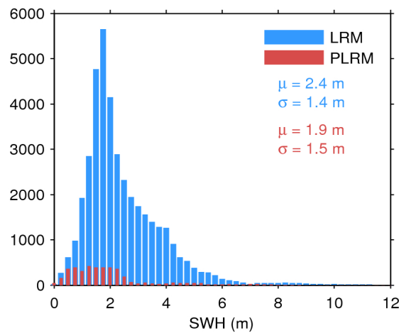
Figure 20. Histogram of science-valid SWH over oceans and lakes for LRM (blue) and PLRM (red) for 25/08/2016. The mean ( \mu ) and standard deviation ( \sigma ) are also shown. Note that values larger than 12 m are excluded from the histogram for the sake of readability but not from the computation of \mu and \sigma .
