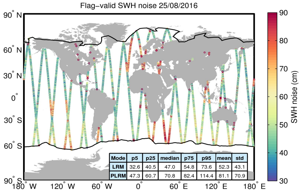
Figure 18. Geographical distribution of flag-valid 20-Hz SWH measurement noise over oceans and lakes for 25/08/2016. The statistical values shown in the table refer to the SWH noise and are calculated separately for LRM and PLRM regions. Measurements taken over polar polygons have been excluded from the computation of the statistical values. The black lines mark the outer limit of the Arctic and Antarctic polar polygons.
