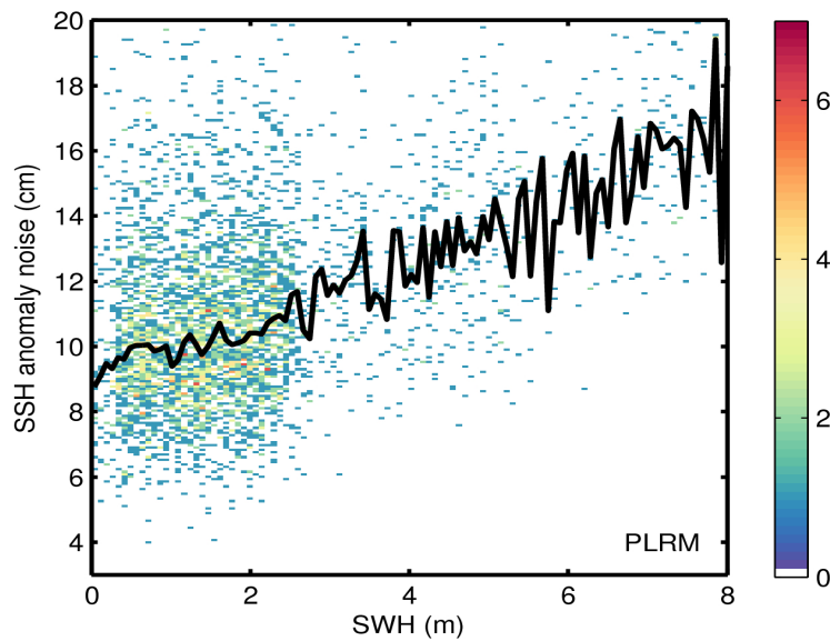
Figure 9. 2D histogram showing flag-valid SSH anomaly noise as a function of SWH for LRM (top) and PLRM (bottom) for 25/08/2016. The black line denotes the median SSH anomaly noise as a function of SWH.
