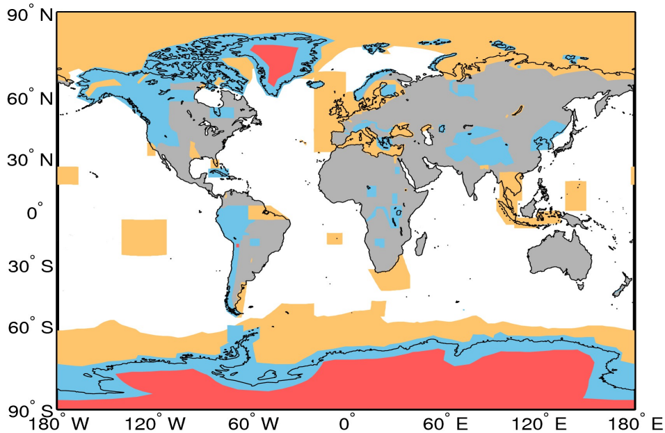
Figure A1. Extent of the regions defining the geographical mode mask for 25/08/2016. The regions where SAR, and SARIn are operated are denoted by the orange and blue polygons, respectively. LRM is operated over areas of the continental ice sheets (red polygons) and over oceans and land not covered by other modes.
