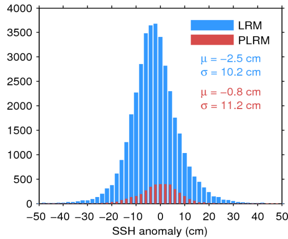
Figure 11. Histogram of science-valid SSH anomaly over oceans and lakes for LRM (blue) and PLRM (red) for 25/08/2016. The mean ( \mu ) and standard deviation ( \sigma ) are also shown. Note that values outside [-50 50] cm are excluded from the histogram for the sake of readability but not from the computation of \mu and \sigma .
