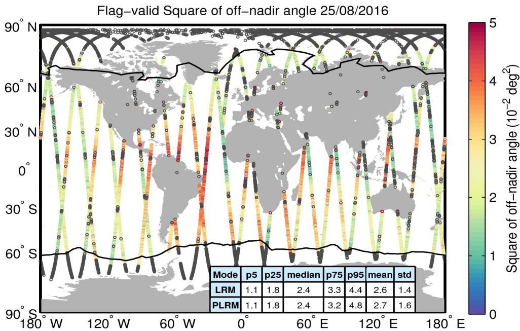
Figure 37. Geographical distribution of flag-valid mispointing data over oceans and lakes for 25/08/2016. The statistical values shown in the table refer to the mispointing in 10^{-2} deg 2 and are calculated separately for LRM and PLRM regions. Measurements taken over polar polygons have been excluded from the computation of the statistical values. The black lines mark the outer limit of the Arctic and Antarctic polar polygons. Gray circles denote negative values.
