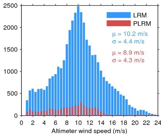
Figure 35. Histogram of science-valid wind over oceans and lakes for LRM (blue) and PLRM (red) for 25/08/2016. The mean ( \mu ) and standard deviation ( \sigma ) are also shown. Note that values larger than 24 m/s are excluded from the histogram for the sake of readability but not from the computation of \mu and \sigma .
