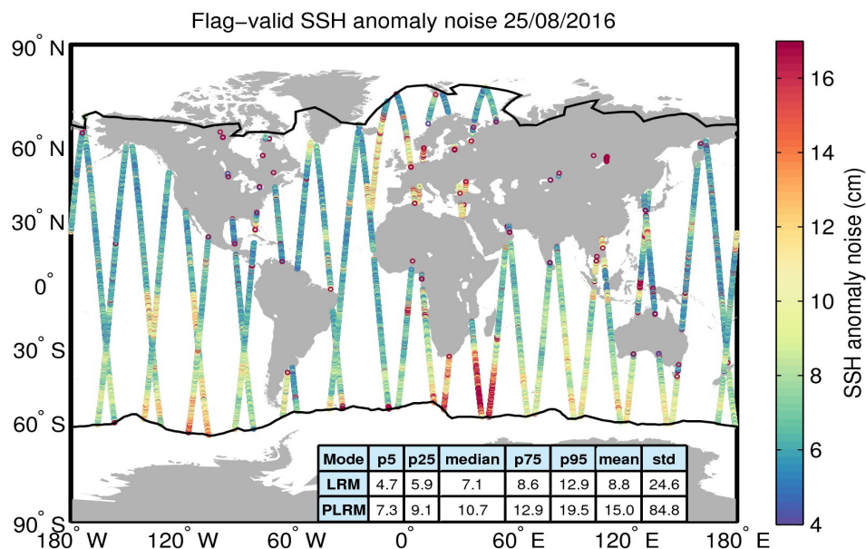
Figure 8. Geographical distribution of flag-valid 20-Hz SSH anomaly measurement noise over oceans and lakes for 25/08/2016. The statistical values shown in the table refer to the SSH anomaly noise and are calculated separately for LRM and PLRM regions. Measurements taken over polar polygons have been excluded from the computation of the statistical values. The black lines mark the outer limit of the Arctic and Antarctic polar polygons.
