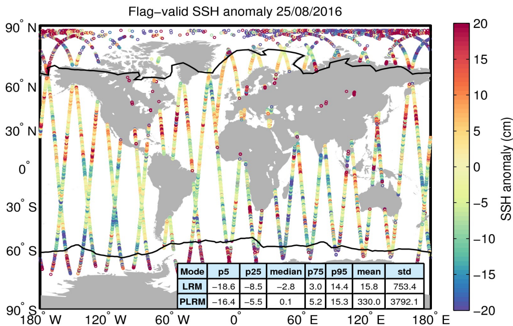
Figure 5. Geographical distribution of flag-valid 1-Hz SSH anomaly data over oceans and lakes for 25/08/2016. The statistical values shown in the table refer to the SSH anomaly in cm and are calculated separately for LRM and PLRM regions. Measurements taken over polar polygons have been excluded from the computation of the statistical values. The black lines mark the outer limit of the Arctic and Antarctic polar polygons.
