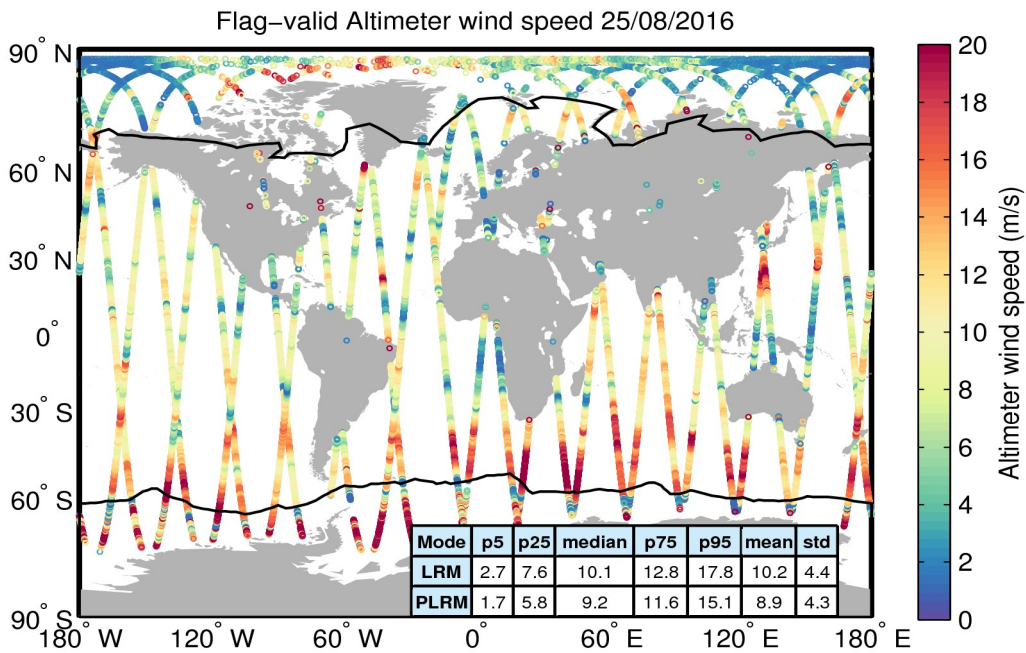
Figure 31. Geographical distribution of flag-valid wind data over oceans and lakes for 25/08/2016. The statistical values shown in the table refer to the wind in m/s and are calculated separately for LRM and PLRM regions. Measurements taken over polar polygons have been excluded from the computation of the statistical values. The black lines mark the outer limit of the Arctic and Antarctic polar polygons.
