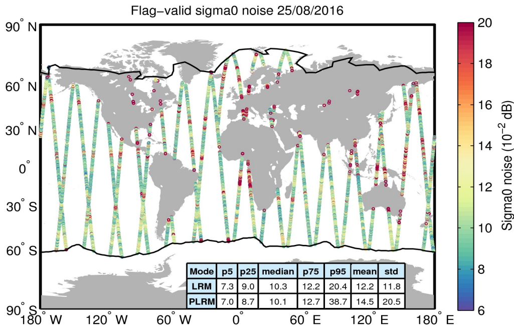
Figure 26. Geographical distribution of flag-valid 20-Hz sigma0 measurement noise over oceans and lakes for 25/08/2016. The statistical values shown in the table refer to the sigma0 noise and are calculated separately for LRM and PLRM regions. Measurements taken over polar polygons have been excluded from the computation of the statistical values. The black lines mark the outer limit of the Arctic and Antarctic polar polygons.
