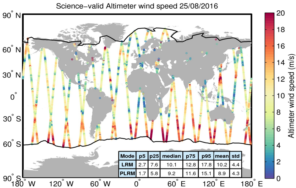
Figure 34. Geographical distribution of science-valid wind data over oceans and lakes for 25/08/2016. The statistical values shown in the table refer to the wind in m/s and are calculated separately for LRM and PLRM regions. The black lines mark the outer limit of the Arctic and Antarctic polar polygons. Gray circles denote records that have been rejected based on the editing criteria described in Table 5.
