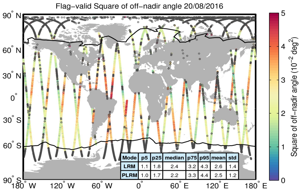
Figure 37. Geographical distribution of flag-valid mispointing data over oceans and lakes for 20/08/2016. The statistical values shown in the table refer to the mispointing in 10^{-2} deg 2 and are calculated separately for LRM and PLRM regions. Measurements taken over polar polygons have been excluded from the computation of the statistical values. The black lines mark the outer limit of the Arctic and Antarctic polar polygons. Gray circles denote negative values.
