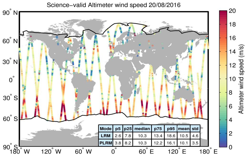
Figure 34. Geographical distribution of science-valid wind data over oceans and lakes for 20/08/2016. The statistical values shown in the table refer to the wind in m/s and are calculated separately for LRM and PLRM regions. The black lines mark the outer limit of the Arctic and Antarctic polar polygons. Gray circles denote records that have been rejected based on the editing criteria described in Table 5.
