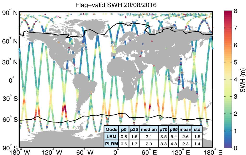
Figure 15. Geographical distribution of flag-valid SWH data over oceans and lakes for 20/08/2016. The statistical values shown in the table refer to the SWH in m and are calculated separately for LRM and PLRM regions. Measurements taken over polar polygons have been excluded from the computation of the statistical values. The black lines mark the outer limit of the Arctic and Antarctic polar polygons.
