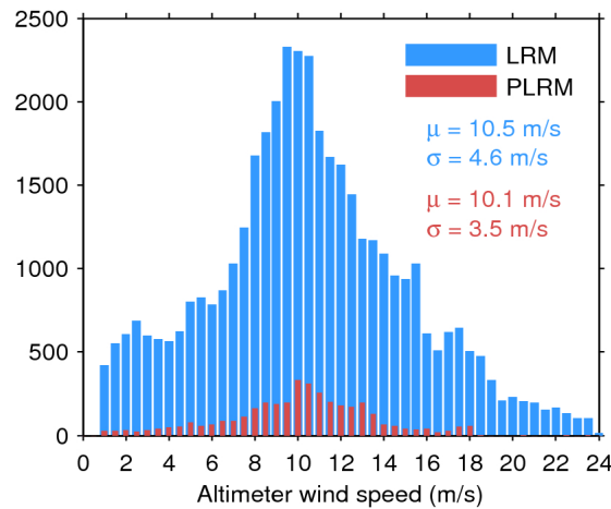
Figure 33. Histogram of flag-valid wind over oceans and lakes for LRM (blue) and PLRM (red) for 20/08/2016. The mean ( \mu ) and standard deviation ( \sigma ) are also shown. Note that values larger than 24 m/s are excluded from the histogram for the sake of readability but not from the computation of \mu and \sigma .
