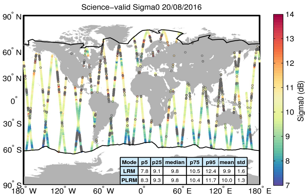
Figure 27. Geographical distribution of science-valid sigma0 data over oceans and lakes for 20/08/2016. The statistical values shown in the table refer to the sigma0 in dB and are calculated separately for LRM and PLRM regions. The black lines mark the outer limit of the Arctic and Antarctic polar polygons. Gray circles denote records that have been rejected based on the editing criteria described in Table 4.
