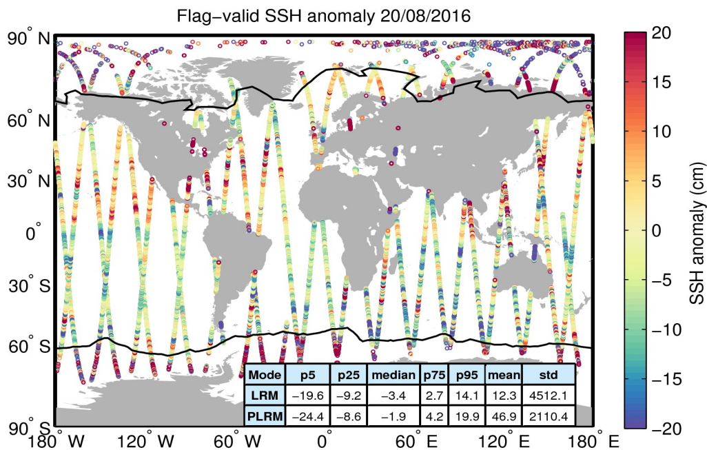
Figure 5. Geographical distribution of flag-valid 1-Hz SSH anomaly data over oceans and lakes for 20/08/2016. The statistical values shown in the table refer to the SSH anomaly in cm and are calculated separately for LRM and PLRM regions. Measurements taken over polar polygons have been excluded from the computation of the statistical values. The black lines mark the outer limit of the Arctic and Antarctic polar polygons.
