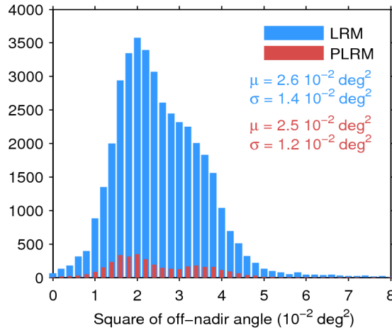
Figure 39. Histogram of flag-valid mispointing over oceans and lakes for LRM (blue) and PLRM (red) for 20/08/2016. Only positive values have been considered. The mean ( \mu ) and standard deviation ( \sigma ) are also shown. Note that values larger than 8 \cdot 10^{-2} \text{ deg}^2 are excluded from the histogram for the sake of readability but not from the computation of \mu and \sigma .
