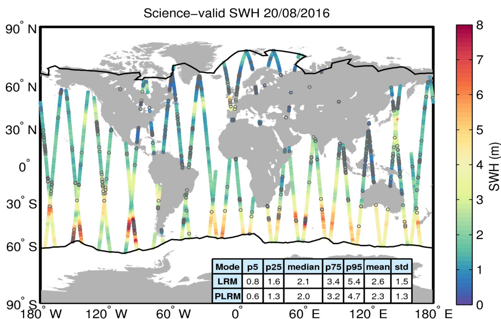
Figure 19. Geographical distribution of science-valid SWH data over oceans and lakes for 20/08/2016. The statistical values shown in the table refer to the SWH in m and are calculated separately for LRM and PLRM regions. The black lines mark the outer limit of the Arctic and Antarctic polar polygons. Gray circles denote records that have been rejected based on the editing criteria described in Table 3.
