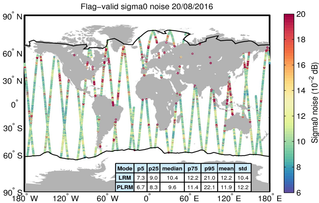
Figure 26. Geographical distribution of flag-valid 20-Hz sigma0 measurement noise over oceans and lakes for 20/08/2016. The statistical values shown in the table refer to the sigma0 noise and are calculated separately for LRM and PLRM regions. Measurements taken over polar polygons have been excluded from the computation of the statistical values. The black lines mark the outer limit of the Arctic and Antarctic polar polygons.
