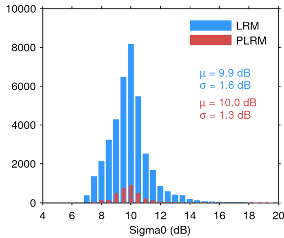
Figure 28. Histogram of science-valid sigma0 over oceans and lakes for LRM (blue) and PLRM (red) for 20/08/2016. The mean ( \mu ) and standard deviation ( \sigma ) are also shown. Note that values outside [4 20] dB are excluded from the histogram for the sake of readability but not from the computation of \mu and \sigma .
