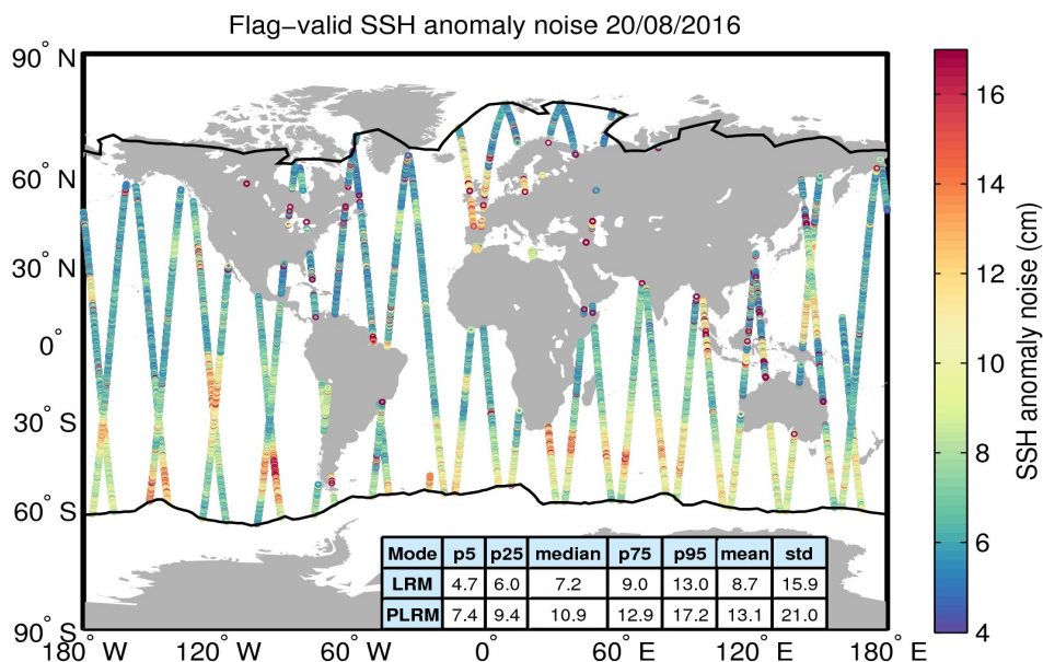
Figure 8. Geographical distribution of flag-valid 20-Hz SSH anomaly measurement noise over oceans and lakes for 20/08/2016. The statistical values shown in the table refer to the SSH anomaly noise and are calculated separately for LRM and PLRM regions. Measurements taken over polar polygons have been excluded from the computation of the statistical values. The black lines mark the outer limit of the Arctic and Antarctic polar polygons.
