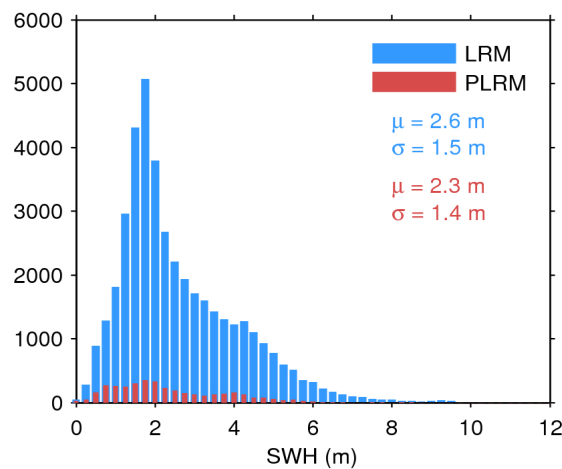
Figure 17. Histogram of flag-valid SWH over oceans and lakes for LRM (blue) and PLRM (red) for 20/08/2016. The mean ( \mu ) and standard deviation ( \sigma ) are also shown. Note that values larger than 12 m are excluded from the histogram for the sake of readability but not from the computation of \mu and \sigma .
