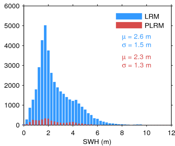
Figure 20. Histogram of science-valid SWH over oceans and lakes for LRM (blue) and PLRM (red) for 20/08/2016. The mean ( \mu ) and standard deviation ( \sigma ) are also shown. Note that values larger than 12 m are excluded from the histogram for the sake of readability but not from the computation of \mu and \sigma .
