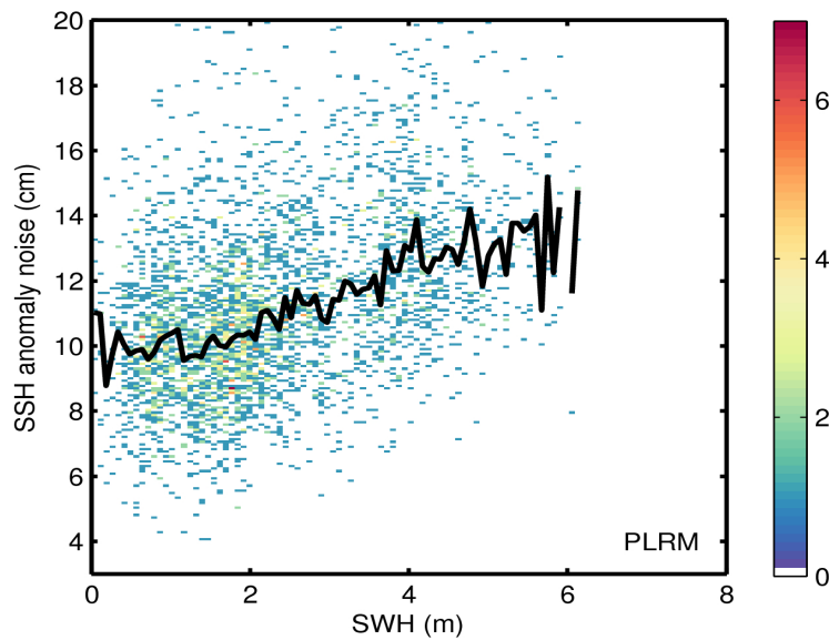
Figure 9. 2D histogram showing flag-valid SSH anomaly noise as a function of SWH for LRM (top) and PLRM (bottom) for 20/08/2016. The black line denotes the median SSH anomaly noise as a function of SWH.
