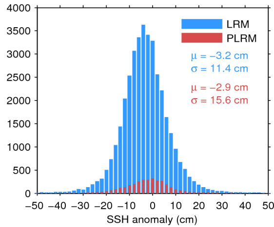
Figure 11. Histogram of science-valid SSH anomaly over oceans and lakes for LRM (blue) and PLRM (red) for 20/08/2016. The mean ( \mu ) and standard deviation ( \sigma ) are also shown. Note that values outside [-50 50] cm are excluded from the histogram for the sake of readability but not from the computation of \mu and \sigma .
