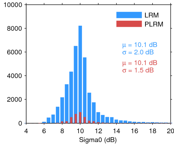
Figure 25. Histogram of flag-valid sigma0 over oceans and lakes for LRM (blue) and PLRM (red) for 20/08/2016. The mean ( \mu ) and standard deviation ( \sigma ) are also shown. Note that values outside [4 20] dB are excluded from the histogram for the sake of readability but not from the computation of \mu and \sigma .
