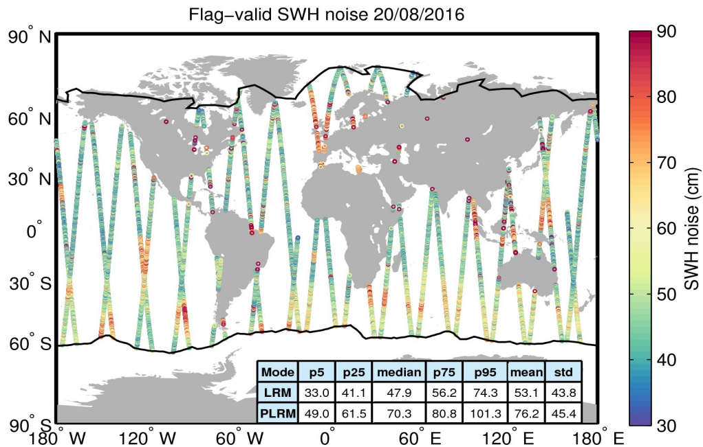
Figure 18. Geographical distribution of flag-valid 20-Hz SWH measurement noise over oceans and lakes for 20/08/2016. The statistical values shown in the table refer to the SWH noise and are calculated separately for LRM and PLRM regions. Measurements taken over polar polygons have been excluded from the computation of the statistical values. The black lines mark the outer limit of the Arctic and Antarctic polar polygons.
