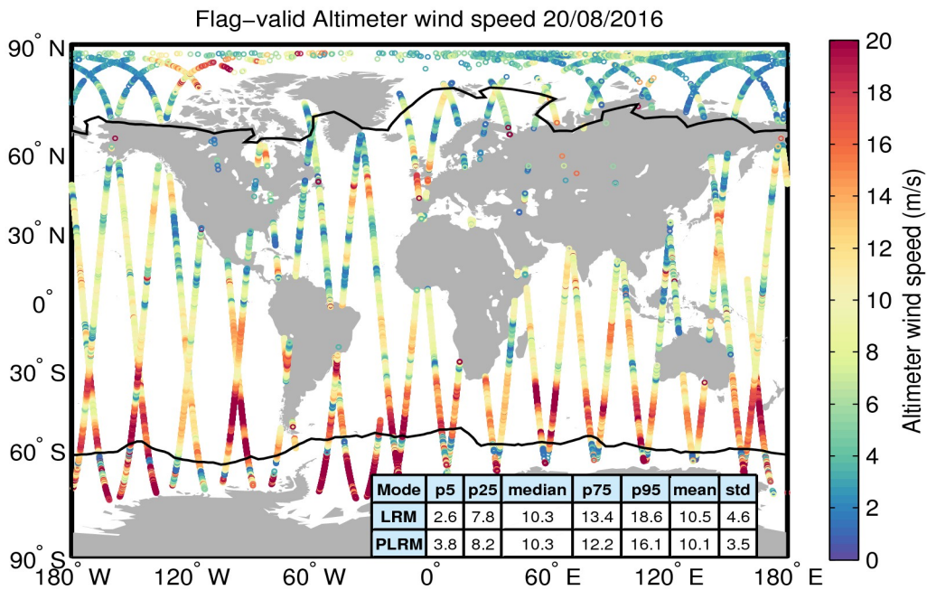
Figure 31. Geographical distribution of flag-valid wind data over oceans and lakes for 20/08/2016. The statistical values shown in the table refer to the wind in m/s and are calculated separately for LRM and PLRM regions. Measurements taken over polar polygons have been excluded from the computation of the statistical values. The black lines mark the outer limit of the Arctic and Antarctic polar polygons.
