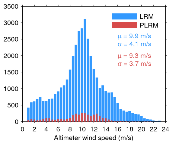
Figure 35. Histogram of science-valid wind over oceans and lakes for LRM (blue) and PLRM (red) for 16/08/2016. The mean ( \mu ) and standard deviation ( \sigma ) are also shown. Note that values larger than 24 m/s are excluded from the histogram for the sake of readability but not from the computation of \mu and \sigma .
