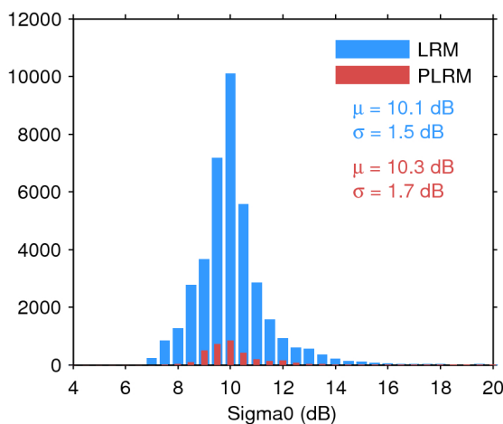
Figure 28. Histogram of science-valid sigma0 over oceans and lakes for LRM (blue) and PLRM (red) for 16/08/2016. The mean ( \mu ) and standard deviation ( \sigma ) are also shown. Note that values outside [4 20] dB are excluded from the histogram for the sake of readability but not from the computation of \mu and \sigma .
