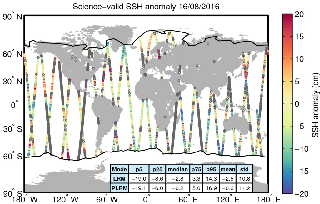
Figure 10. Geographical distribution of science-valid SSH anomaly data over oceans and lakes for 16/08/2016. The statistical values shown in the table refer to the SSH anomaly in cm and are calculated separately for LRM and PLRM regions. The black lines mark the outer limit of the Arctic and Antarctic polar polygons. Gray circles denote records that have been rejected based on the editing criteria described in Table 2.
