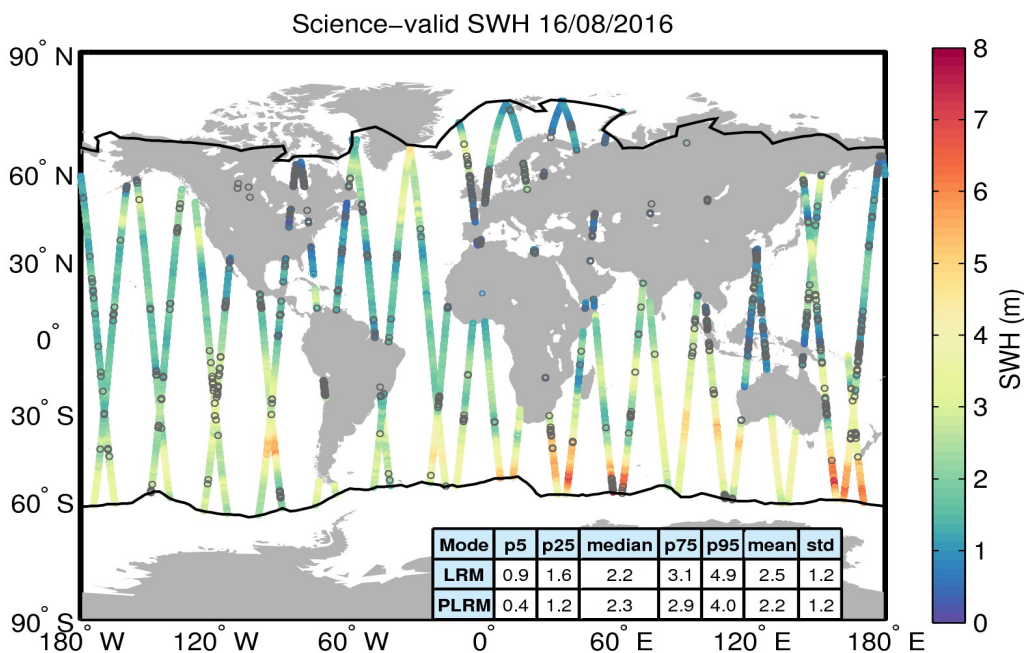
Figure 19. Geographical distribution of science-valid SWH data over oceans and lakes for 16/08/2016. The statistical values shown in the table refer to the SWH in m and are calculated separately for LRM and PLRM regions. The black lines mark the outer limit of the Arctic and Antarctic polar polygons. Gray circles denote records that have been rejected based on the editing criteria described in Table 3.
