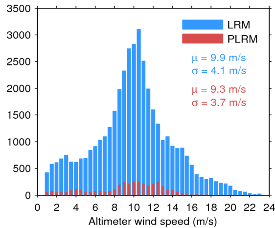
Figure 33. Histogram of flag-valid wind over oceans and lakes for LRM (blue) and PLRM (red) for 16/08/2016. The mean ( \mu ) and standard deviation ( \sigma ) are also shown. Note that values larger than 24 m/s are excluded from the histogram for the sake of readability but not from the computation of \mu and \sigma .
