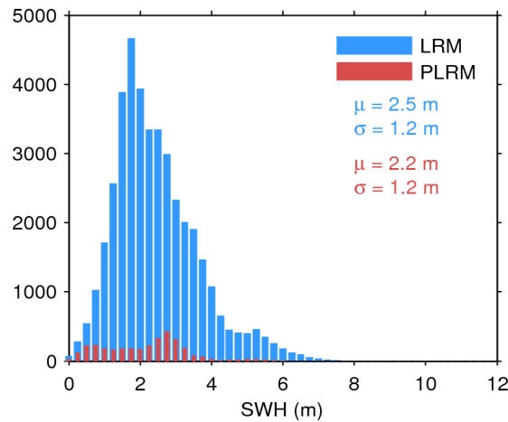
Figure 20. Histogram of science-valid SWH over oceans and lakes for LRM (blue) and PLRM (red) for 16/08/2016. The mean ( \mu ) and standard deviation ( \sigma ) are also shown. Note that values larger than 12 m are excluded from the histogram for the sake of readability but not from the computation of \mu and \sigma .
