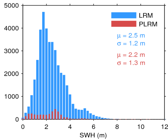
Figure 17. Histogram of flag-valid SWH over oceans and lakes for LRM (blue) and PLRM (red) for 16/08/2016. The mean ( \mu ) and standard deviation ( \sigma ) are also shown. Note that values larger than 12 m are excluded from the histogram for the sake of readability but not from the computation of \mu and \sigma .
