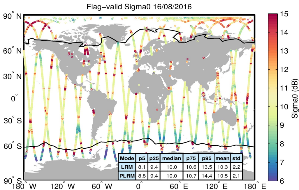
Figure 23. Geographical distribution of flag-valid sigma0 data over oceans and lakes for 16/08/2016. The statistical values shown in the table refer to the sigma0 in dB and are calculated separately for LRM and PLRM regions. Measurements taken over polar polygons have been excluded from the computation of the statistical values. The black lines mark the outer limit of the Arctic and Antarctic polar polygons.
