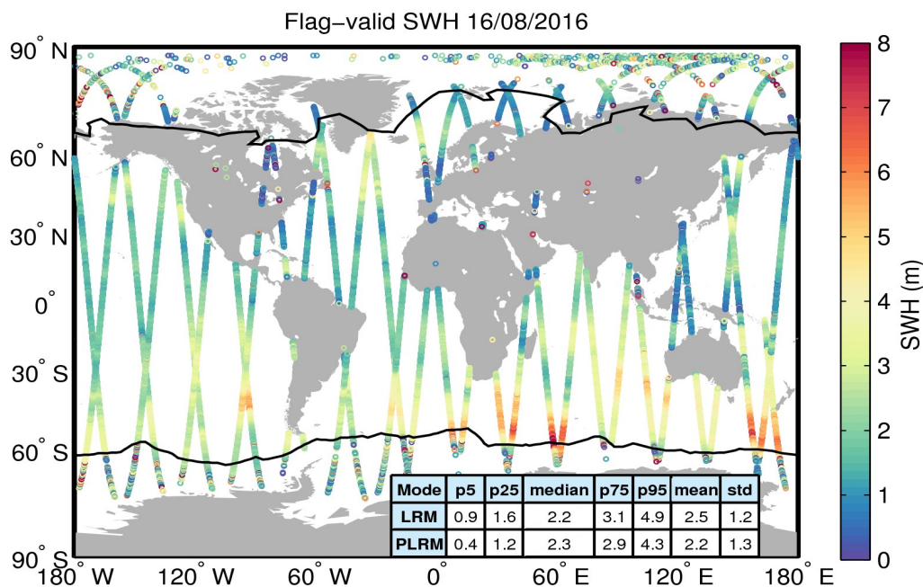
Figure 15. Geographical distribution of flag-valid SWH data over oceans and lakes for 16/08/2016. The statistical values shown in the table refer to the SWH in m and are calculated separately for LRM and PLRM regions. Measurements taken over polar polygons have been excluded from the computation of the statistical values. The black lines mark the outer limit of the Arctic and Antarctic polar polygons.
