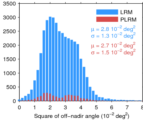
Figure 39. Histogram of flag-valid mispointing over oceans and lakes for LRM (blue) and PLRM (red) for 16/08/2016. Only positive values have been considered. The mean ( \mu ) and standard deviation ( \sigma ) are also shown. Note that values larger than 8 \cdot 10^{-2} \text{ deg}^2 are excluded from the histogram for the sake of readability but not from the computation of \mu and \sigma .
