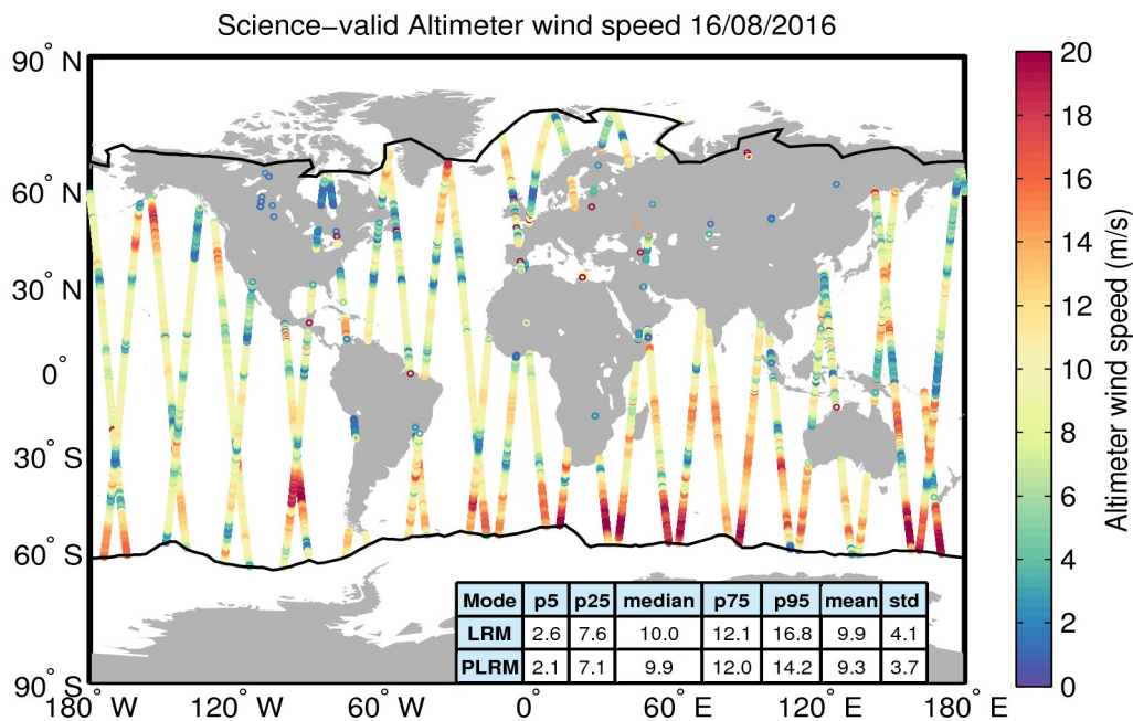
Figure 34. Geographical distribution of science-valid wind data over oceans and lakes for 16/08/2016. The statistical values shown in the table refer to the wind in m/s and are calculated separately for LRM and PLRM regions. The black lines mark the outer limit of the Arctic and Antarctic polar polygons. Gray circles denote records that have been rejected based on the editing criteria described in Table 5.
