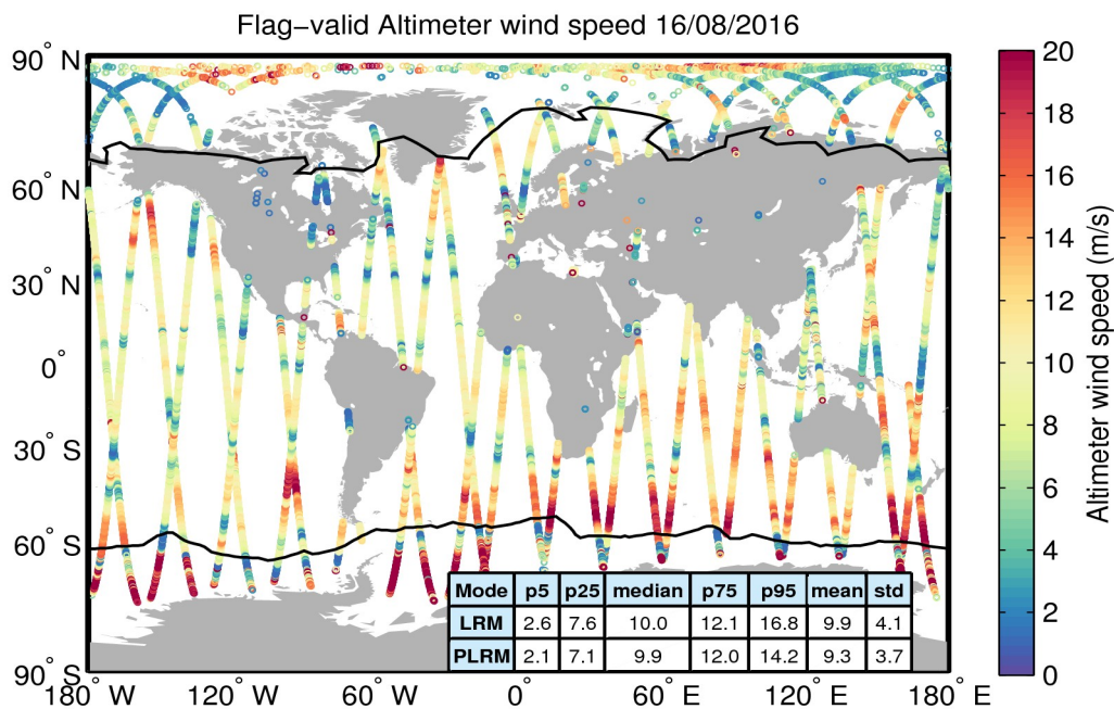
Figure 31. Geographical distribution of flag-valid wind data over oceans and lakes for 16/08/2016. The statistical values shown in the table refer to the wind in m/s and are calculated separately for LRM and PLRM regions. Measurements taken over polar polygons have been excluded from the computation of the statistical values. The black lines mark the outer limit of the Arctic and Antarctic polar polygons.
