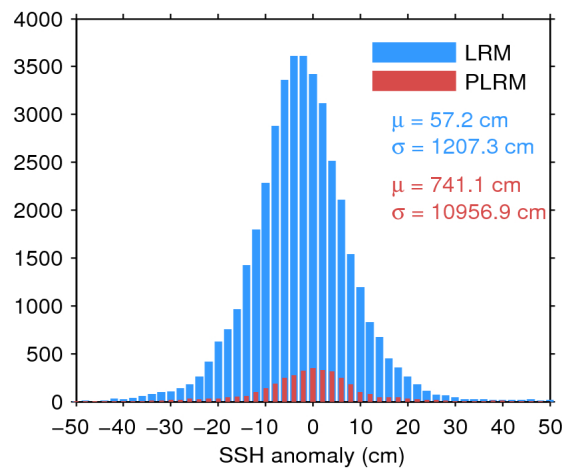
Figure 7. Histogram of flag-valid SSH anomaly over oceans and lakes for LRM (blue) and PLRM (red) for 16/08/2016. The mean ( \mu ) and standard deviation ( \sigma ) are also shown. Note that values outside [-50\ 50] cm are excluded from the histogram for the sake of readability but not from the computation of \mu and \sigma .
