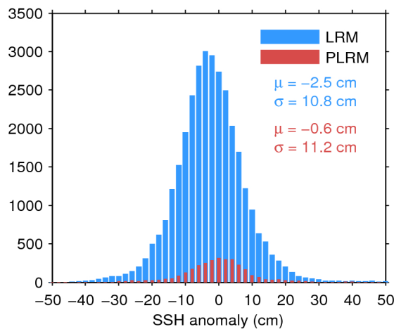
Figure 11. Histogram of science-valid SSH anomaly over oceans and lakes for LRM (blue) and PLRM (red) for 16/08/2016. The mean ( \mu ) and standard deviation ( \sigma ) are also shown. Note that values outside [-50 50] cm are excluded from the histogram for the sake of readability but not from the computation of \mu and \sigma .
