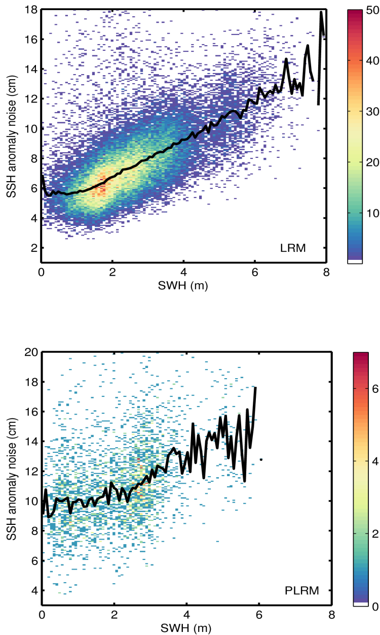
Figure 9. 2D histogram showing flag-valid SSH anomaly noise as a function of SWH for LRM (top) and PLRM (bottom) for 16/08/2016. The black line denotes the median SSH anomaly noise as a function of SWH.
