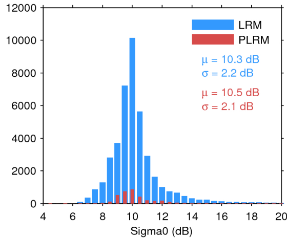
Figure 25. Histogram of flag-valid sigma0 over oceans and lakes for LRM (blue) and PLRM (red) for 16/08/2016. The mean ( \mu ) and standard deviation ( \sigma ) are also shown. Note that values outside [4 20] dB are excluded from the histogram for the sake of readability but not from the computation of \mu and \sigma .
