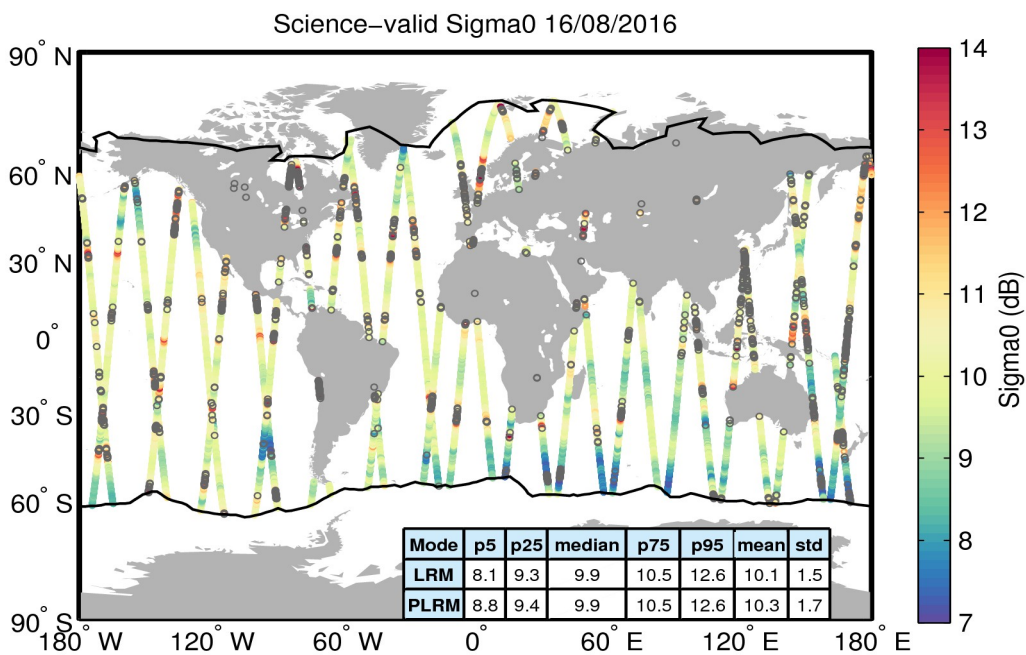
Figure 27. Geographical distribution of science-valid sigma0 data over oceans and lakes for 16/08/2016. The statistical values shown in the table refer to the sigma0 in dB and are calculated separately for LRM and PLRM regions. The black lines mark the outer limit of the Arctic and Antarctic polar polygons. Gray circles denote records that have been rejected based on the editing criteria described in Table 4.
