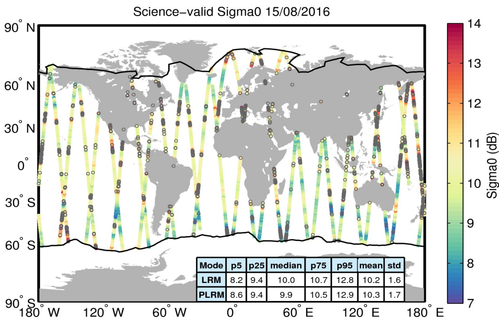
Figure 27. Geographical distribution of science-valid sigma0 data over oceans and lakes for 15/08/2016. The statistical values shown in the table refer to the sigma0 in dB and are calculated separately for LRM and PLRM regions. The black lines mark the outer limit of the Arctic and Antarctic polar polygons. Gray circles denote records that have been rejected based on the editing criteria described in Table 4.
