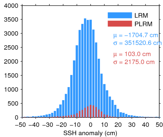
Figure 7. Histogram of flag-valid SSH anomaly over oceans and lakes for LRM (blue) and PLRM (red) for 15/08/2016. The mean ( \mu ) and standard deviation ( \sigma ) are also shown. Note that values outside [-50 \ 50] cm are excluded from the histogram for the sake of readability but not from the computation of \mu and \sigma .
