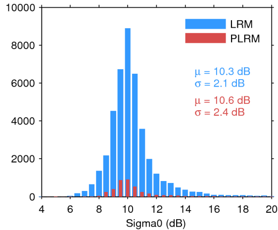
Figure 25. Histogram of flag-valid sigma0 over oceans and lakes for LRM (blue) and PLRM (red) for 15/08/2016. The mean ( \mu ) and standard deviation ( \sigma ) are also shown. Note that values outside [4 20] dB are excluded from the histogram for the sake of readability but not from the computation of \mu and \sigma .
