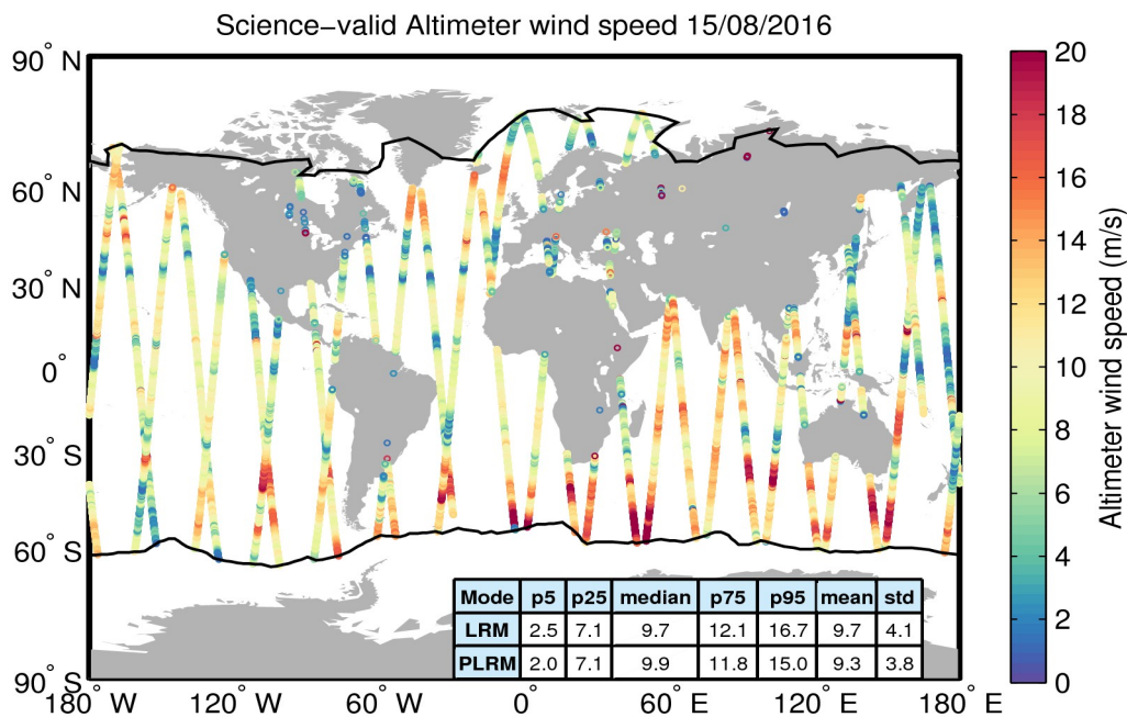
Figure 34. Geographical distribution of science-valid wind data over oceans and lakes for 15/08/2016. The statistical values shown in the table refer to the wind in m/s and are calculated separately for LRM and PLRM regions. The black lines mark the outer limit of the Arctic and Antarctic polar polygons. Gray circles denote records that have been rejected based on the editing criteria described in Table 5.
