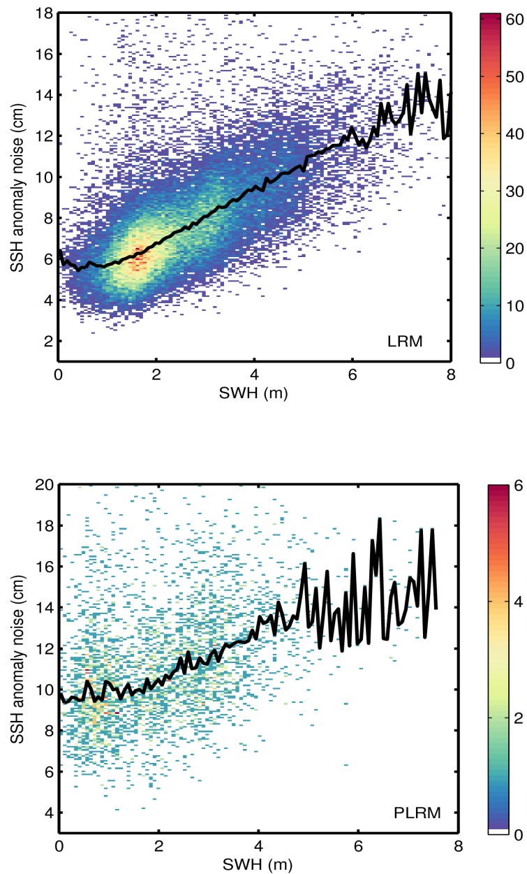
Figure 9. 2D histogram showing flag-valid SSH anomaly noise as a function of SWH for LRM (top) and PLRM (bottom) for 15/08/2016. The black line denotes the median SSH anomaly noise as a function of SWH.
