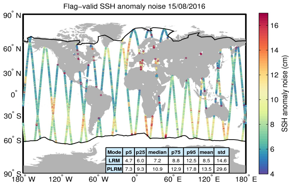
Figure 8. Geographical distribution of flag-valid 20-Hz SSH anomaly measurement noise over oceans and lakes for 15/08/2016. The statistical values shown in the table refer to the SSH anomaly noise and are calculated separately for LRM and PLRM regions. Measurements taken over polar polygons have been excluded from the computation of the statistical values. The black lines mark the outer limit of the Arctic and Antarctic polar polygons.
