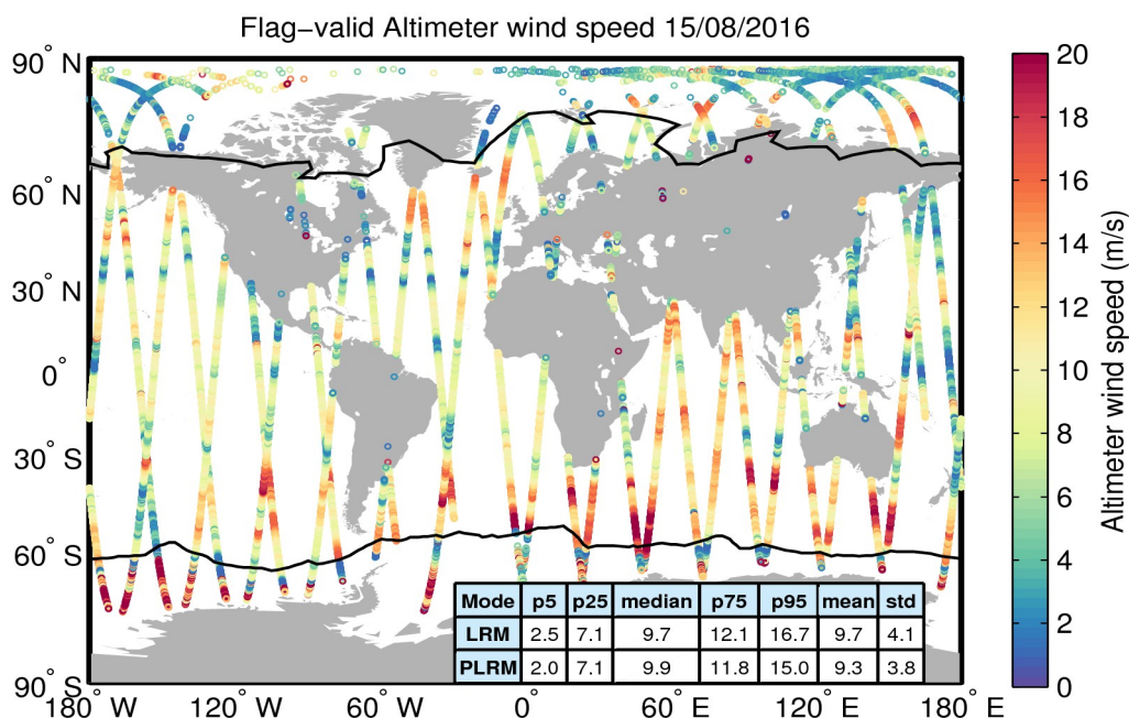
Figure 31. Geographical distribution of flag-valid wind data over oceans and lakes for 15/08/2016. The statistical values shown in the table refer to the wind in m/s and are calculated separately for LRM and PLRM regions. Measurements taken over polar polygons have been excluded from the computation of the statistical values. The black lines mark the outer limit of the Arctic and Antarctic polar polygons.
