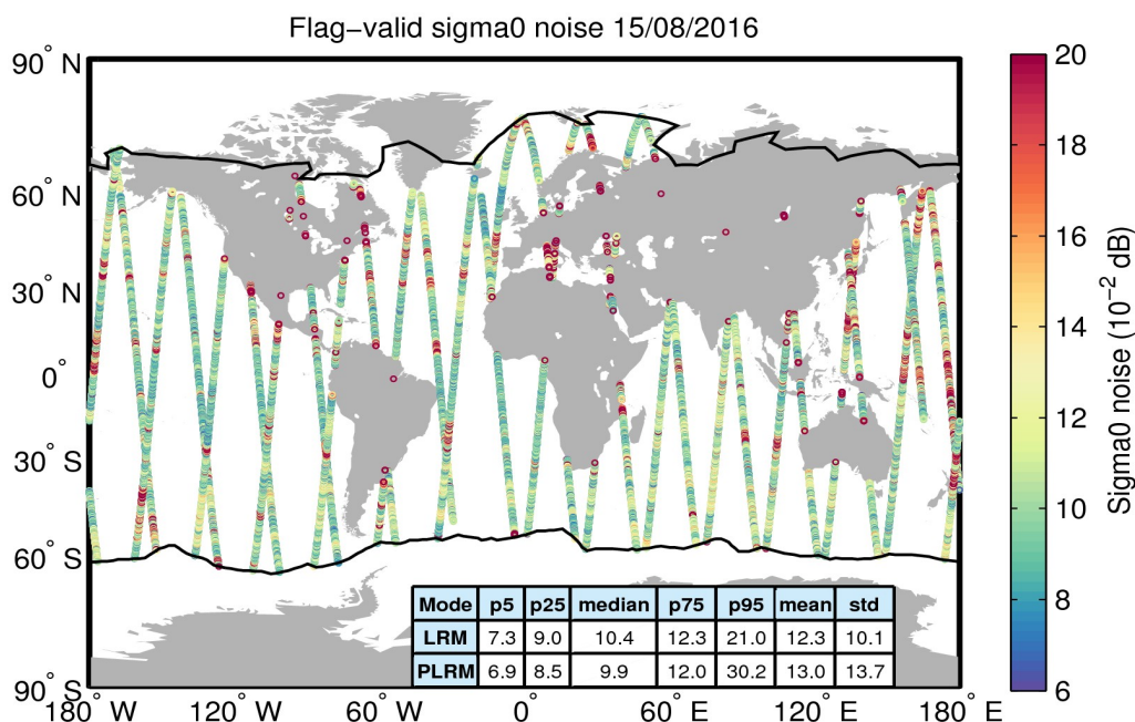
Figure 26. Geographical distribution of flag-valid 20-Hz sigma0 measurement noise over oceans and lakes for 15/08/2016. The statistical values shown in the table refer to the sigma0 noise and are calculated separately for LRM and PLRM regions. Measurements taken over polar polygons have been excluded from the computation of the statistical values. The black lines mark the outer limit of the Arctic and Antarctic polar polygons.
