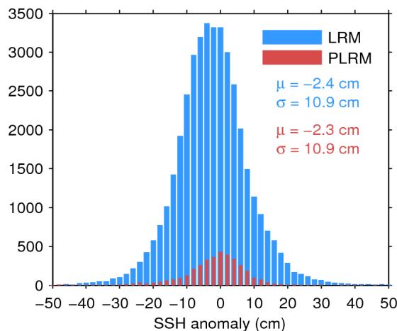
Figure 11. Histogram of science-valid SSH anomaly over oceans and lakes for LRM (blue) and PLRM (red) for 15/08/2016. The mean ( \mu ) and standard deviation ( \sigma ) are also shown. Note that values outside [-50 50] cm are excluded from the histogram for the sake of readability but not from the computation of \mu and \sigma .
