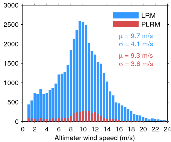
Figure 33. Histogram of flag-valid wind over oceans and lakes for LRM (blue) and PLRM (red) for 15/08/2016. The mean ( \mu ) and standard deviation ( \sigma ) are also shown. Note that values larger than 24 m/s are excluded from the histogram for the sake of readability but not from the computation of \mu and \sigma .
