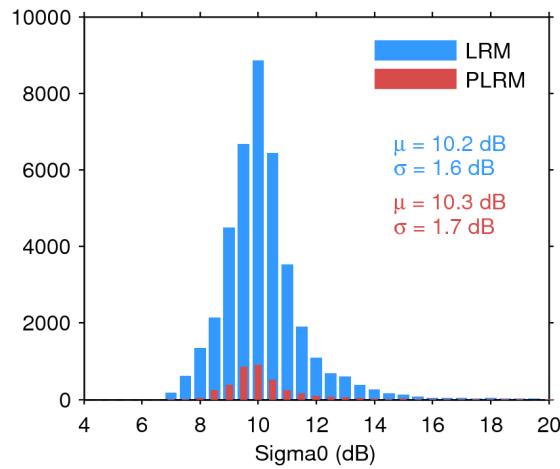
Figure 28. Histogram of science-valid sigma0 over oceans and lakes for LRM (blue) and PLRM (red) for 15/08/2016. The mean ( \mu ) and standard deviation ( \sigma ) are also shown. Note that values outside [4 20] dB are excluded from the histogram for the sake of readability but not from the computation of \mu and \sigma .
