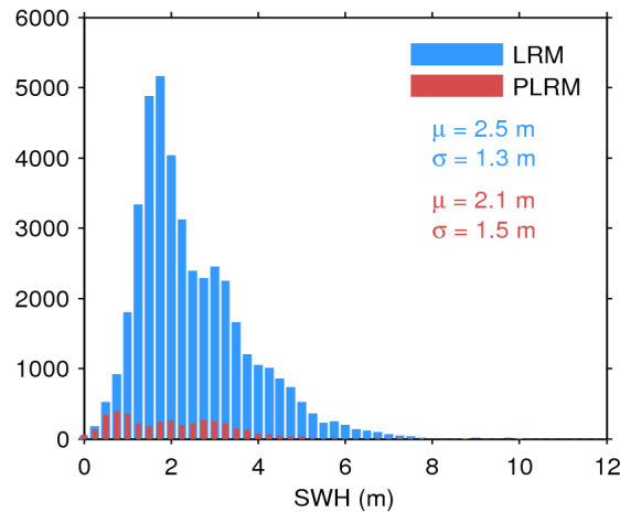
Figure 17. Histogram of flag-valid SWH over oceans and lakes for LRM (blue) and PLRM (red) for 15/08/2016. The mean ( \mu ) and standard deviation ( \sigma ) are also shown. Note that values larger than 12 m are excluded from the histogram for the sake of readability but not from the computation of \mu and \sigma .
