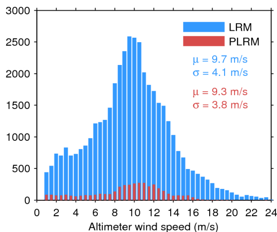
Figure 35. Histogram of science-valid wind over oceans and lakes for LRM (blue) and PLRM (red) for 15/08/2016. The mean ( \mu ) and standard deviation ( \sigma ) are also shown. Note that values larger than 24 m/s are excluded from the histogram for the sake of readability but not from the computation of \mu and \sigma .
