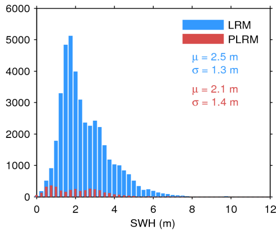
Figure 20. Histogram of science-valid SWH over oceans and lakes for LRM (blue) and PLRM (red) for 15/08/2016. The mean ( \mu ) and standard deviation ( \sigma ) are also shown. Note that values larger than 12 m are excluded from the histogram for the sake of readability but not from the computation of \mu and \sigma .
