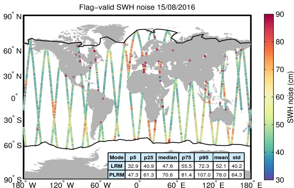
Figure 18. Geographical distribution of flag-valid 20-Hz SWH measurement noise over oceans and lakes for 15/08/2016. The statistical values shown in the table refer to the SWH noise and are calculated separately for LRM and PLRM regions. Measurements taken over polar polygons have been excluded from the computation of the statistical values. The black lines mark the outer limit of the Arctic and Antarctic polar polygons.
