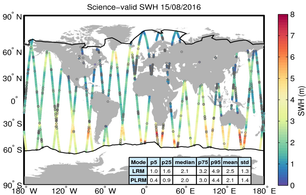
Figure 19. Geographical distribution of science-valid SWH data over oceans and lakes for 15/08/2016. The statistical values shown in the table refer to the SWH in m and are calculated separately for LRM and PLRM regions. The black lines mark the outer limit of the Arctic and Antarctic polar polygons. Gray circles denote records that have been rejected based on the editing criteria described in Table 3.
