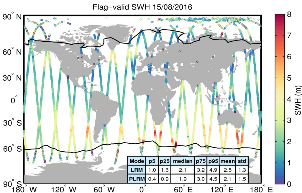
Figure 15. Geographical distribution of flag-valid SWH data over oceans and lakes for 15/08/2016. The statistical values shown in the table refer to the SWH in m and are calculated separately for LRM and PLRM regions. Measurements taken over polar polygons have been excluded from the computation of the statistical values. The black lines mark the outer limit of the Arctic and Antarctic polar polygons.
