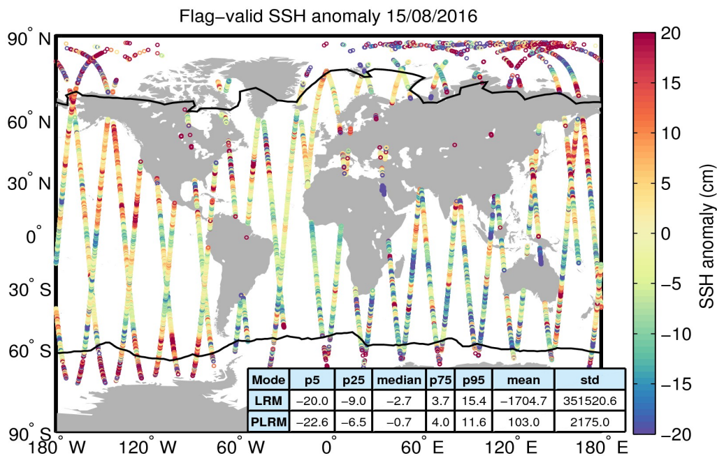
Figure 5. Geographical distribution of flag-valid 1-Hz SSH anomaly data over oceans and lakes for 15/08/2016. The statistical values shown in the table refer to the SSH anomaly in cm and are calculated separately for LRM and PLRM regions. Measurements taken over polar polygons have been excluded from the computation of the statistical values. The black lines mark the outer limit of the Arctic and Antarctic polar polygons.
