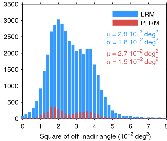
Figure 39. Histogram of flag-valid mispointing over oceans and lakes for LRM (blue) and PLRM (red) for 15/08/2016. Only positive values have been considered. The mean ( \mu ) and standard deviation ( \sigma ) are also shown. Note that values larger than 8 \cdot 10^{-2} \text{ deg}^2 are excluded from the histogram for the sake of readability but not from the computation of \mu and \sigma .
