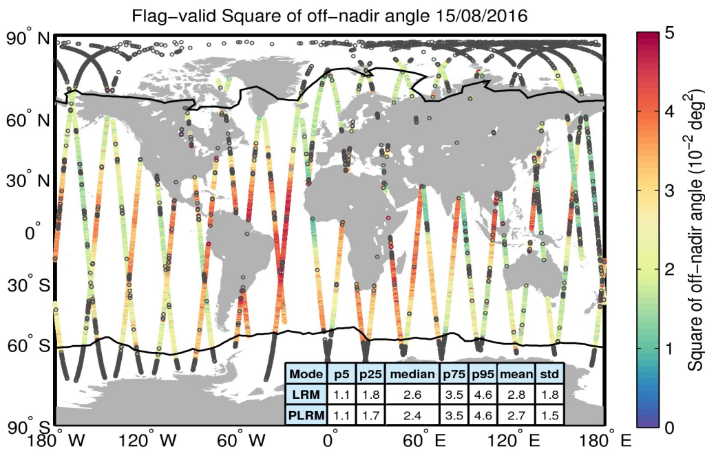
Figure 37. Geographical distribution of flag-valid mispointing data over oceans and lakes for 15/08/2016. The statistical values shown in the table refer to the mispointing in 10^{-2} deg 2 and are calculated separately for LRM and PLRM regions. Measurements taken over polar polygons have been excluded from the computation of the statistical values. The black lines mark the outer limit of the Arctic and Antarctic polar polygons. Gray circles denote negative values.
