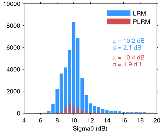
Figure 25. Histogram of flag-valid sigma0 over oceans and lakes for LRM (blue) and PLRM (red) for 14/08/2016. The mean ( \mu ) and standard deviation ( \sigma ) are also shown. Note that values outside [4 20] dB are excluded from the histogram for the sake of readability but not from the computation of \mu and \sigma .
