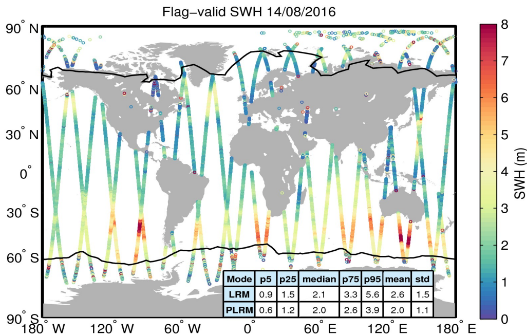
Figure 15. Geographical distribution of flag-valid SWH data over oceans and lakes for 14/08/2016. The statistical values shown in the table refer to the SWH in m and are calculated separately for LRM and PLRM regions. Measurements taken over polar polygons have been excluded from the computation of the statistical values. The black lines mark the outer limit of the Arctic and Antarctic polar polygons.
