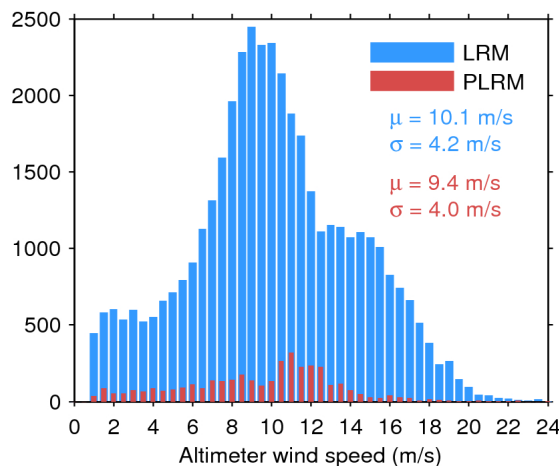
Figure 35. Histogram of science-valid wind over oceans and lakes for LRM (blue) and PLRM (red) for 14/08/2016. The mean ( \mu ) and standard deviation ( \sigma ) are also shown. Note that values larger than 24 m/s are excluded from the histogram for the sake of readability but not from the computation of \mu and \sigma .
