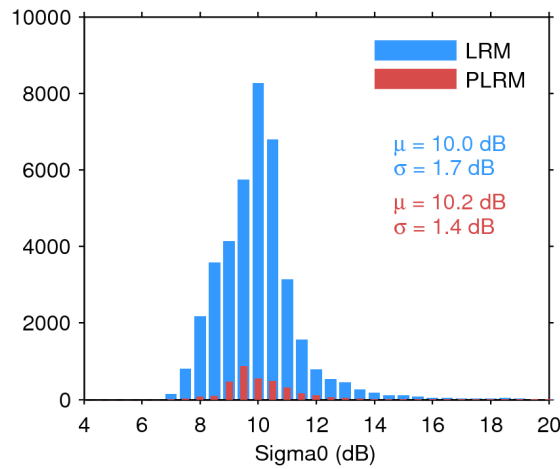
Figure 28. Histogram of science-valid sigma0 over oceans and lakes for LRM (blue) and PLRM (red) for 14/08/2016. The mean ( \mu ) and standard deviation ( \sigma ) are also shown. Note that values outside [4 20] dB are excluded from the histogram for the sake of readability but not from the computation of \mu and \sigma .
