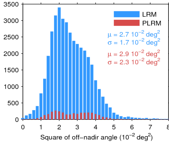
Figure 39. Histogram of flag-valid mispointing over oceans and lakes for LRM (blue) and PLRM (red) for 14/08/2016. Only positive values have been considered. The mean ( \mu ) and standard deviation ( \sigma ) are also shown. Note that values larger than 8 \cdot 10^{-2} \text{ deg}^2 are excluded from the histogram for the sake of readability but not from the computation of \mu and \sigma .
