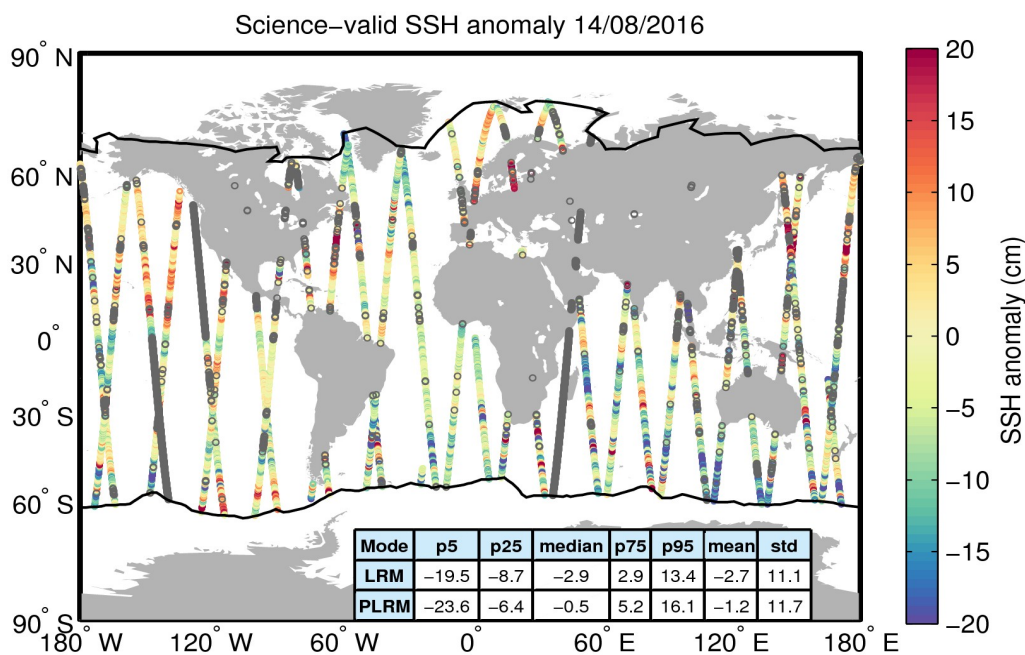
Figure 10. Geographical distribution of science-valid SSH anomaly data over oceans and lakes for 14/08/2016. The statistical values shown in the table refer to the SSH anomaly in cm and are calculated separately for LRM and PLRM regions. The black lines mark the outer limit of the Arctic and Antarctic polar polygons. Gray circles denote records that have been rejected based on the editing criteria described in Table 2.
