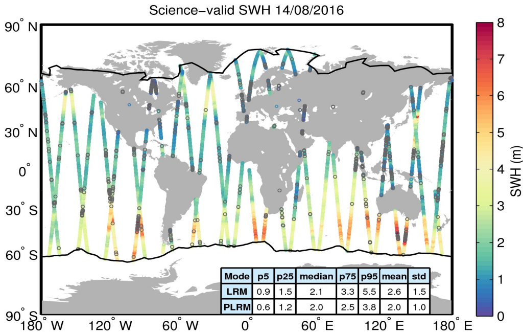
Figure 19. Geographical distribution of science-valid SWH data over oceans and lakes for 14/08/2016. The statistical values shown in the table refer to the SWH in m and are calculated separately for LRM and PLRM regions. The black lines mark the outer limit of the Arctic and Antarctic polar polygons. Gray circles denote records that have been rejected based on the editing criteria described in Table 3.
