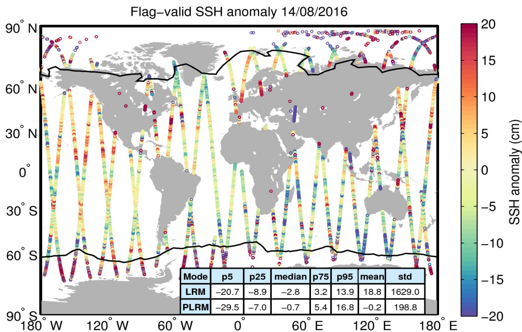
Figure 5. Geographical distribution of flag-valid 1-Hz SSH anomaly data over oceans and lakes for 14/08/2016. The statistical values shown in the table refer to the SSH anomaly in cm and are calculated separately for LRM and PLRM regions. Measurements taken over polar polygons have been excluded from the computation of the statistical values. The black lines mark the outer limit of the Arctic and Antarctic polar polygons.
