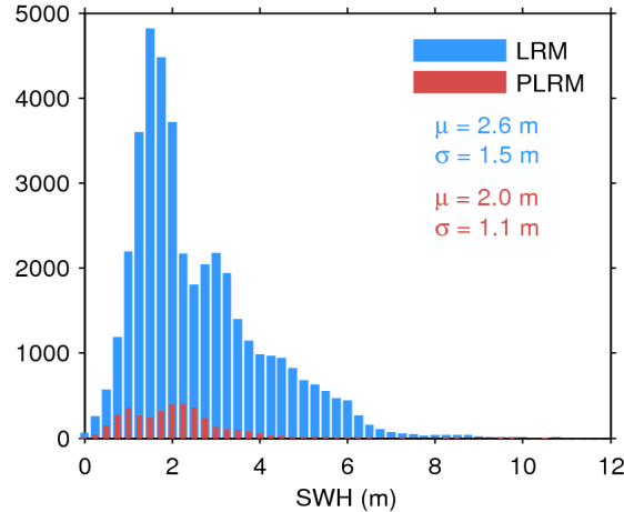
Figure 17. Histogram of flag-valid SWH over oceans and lakes for LRM (blue) and PLRM (red) for 14/08/2016. The mean ( \mu ) and standard deviation ( \sigma ) are also shown. Note that values larger than 12 m are excluded from the histogram for the sake of readability but not from the computation of \mu and \sigma .
