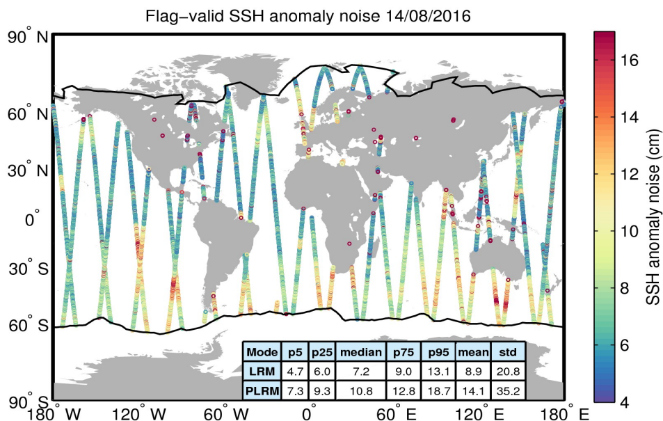
Figure 8. Geographical distribution of flag-valid 20-Hz SSH anomaly measurement noise over oceans and lakes for 14/08/2016. The statistical values shown in the table refer to the SSH anomaly noise and are calculated separately for LRM and PLRM regions. Measurements taken over polar polygons have been excluded from the computation of the statistical values. The black lines mark the outer limit of the Arctic and Antarctic polar polygons.
