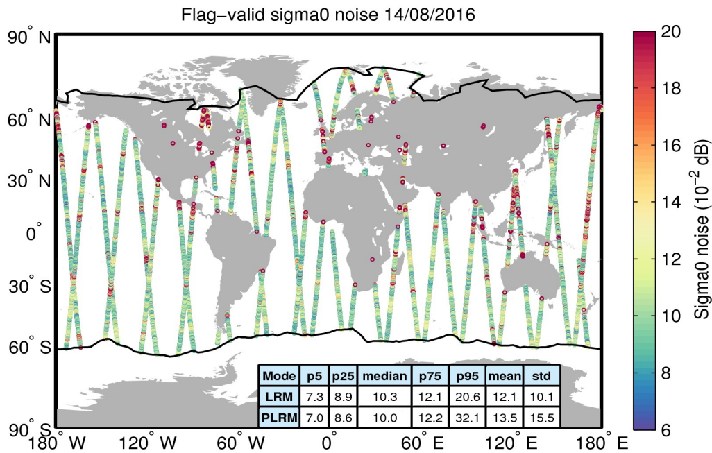
Figure 26. Geographical distribution of flag-valid 20-Hz sigma0 measurement noise over oceans and lakes for 14/08/2016. The statistical values shown in the table refer to the sigma0 noise and are calculated separately for LRM and PLRM regions. Measurements taken over polar polygons have been excluded from the computation of the statistical values. The black lines mark the outer limit of the Arctic and Antarctic polar polygons.
