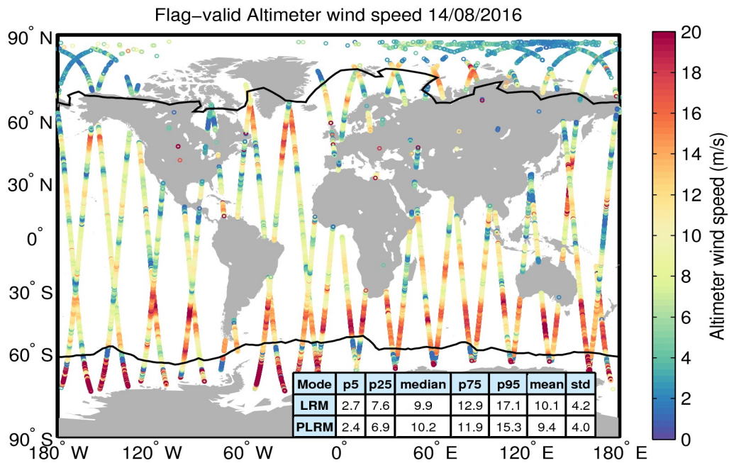
Figure 31. Geographical distribution of flag-valid wind data over oceans and lakes for 14/08/2016. The statistical values shown in the table refer to the wind in m/s and are calculated separately for LRM and PLRM regions. Measurements taken over polar polygons have been excluded from the computation of the statistical values. The black lines mark the outer limit of the Arctic and Antarctic polar polygons.
