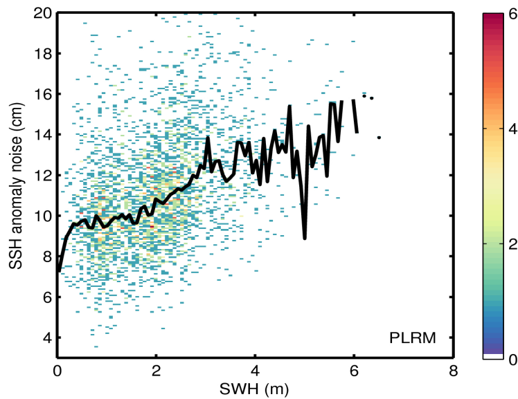
Figure 9. 2D histogram showing flag-valid SSH anomaly noise as a function of SWH for LRM (top) and PLRM (bottom) for 14/08/2016. The black line denotes the median SSH anomaly noise as a function of SWH.
