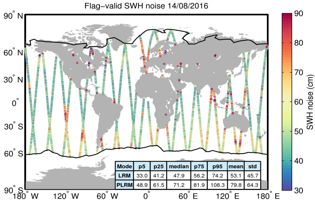
Figure 18. Geographical distribution of flag-valid 20-Hz SWH measurement noise over oceans and lakes for 14/08/2016. The statistical values shown in the table refer to the SWH noise and are calculated separately for LRM and PLRM regions. Measurements taken over polar polygons have been excluded from the computation of the statistical values. The black lines mark the outer limit of the Arctic and Antarctic polar polygons.
