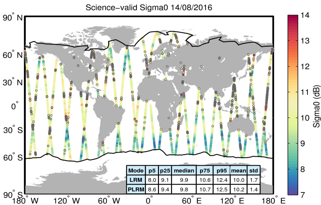
Figure 27. Geographical distribution of science-valid sigma0 data over oceans and lakes for 14/08/2016. The statistical values shown in the table refer to the sigma0 in dB and are calculated separately for LRM and PLRM regions. The black lines mark the outer limit of the Arctic and Antarctic polar polygons. Gray circles denote records that have been rejected based on the editing criteria described in Table 4.
