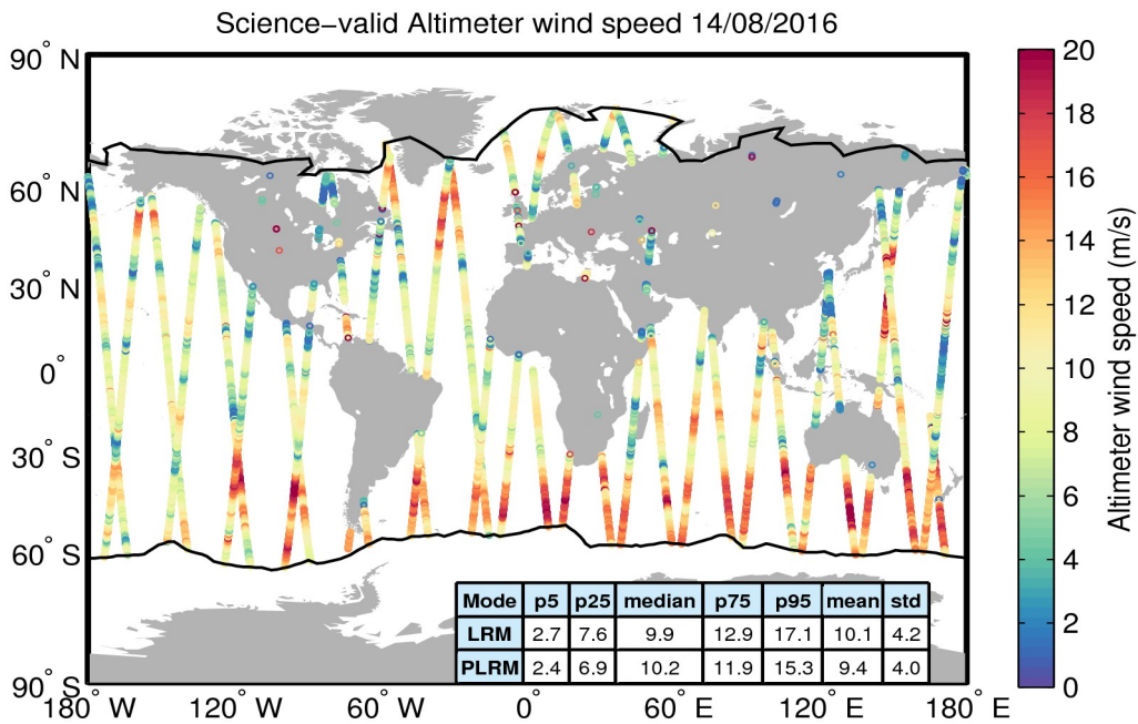
Figure 34. Geographical distribution of science-valid wind data over oceans and lakes for 14/08/2016. The statistical values shown in the table refer to the wind in m/s and are calculated separately for LRM and PLRM regions. The black lines mark the outer limit of the Arctic and Antarctic polar polygons. Gray circles denote records that have been rejected based on the editing criteria described in Table 5.
