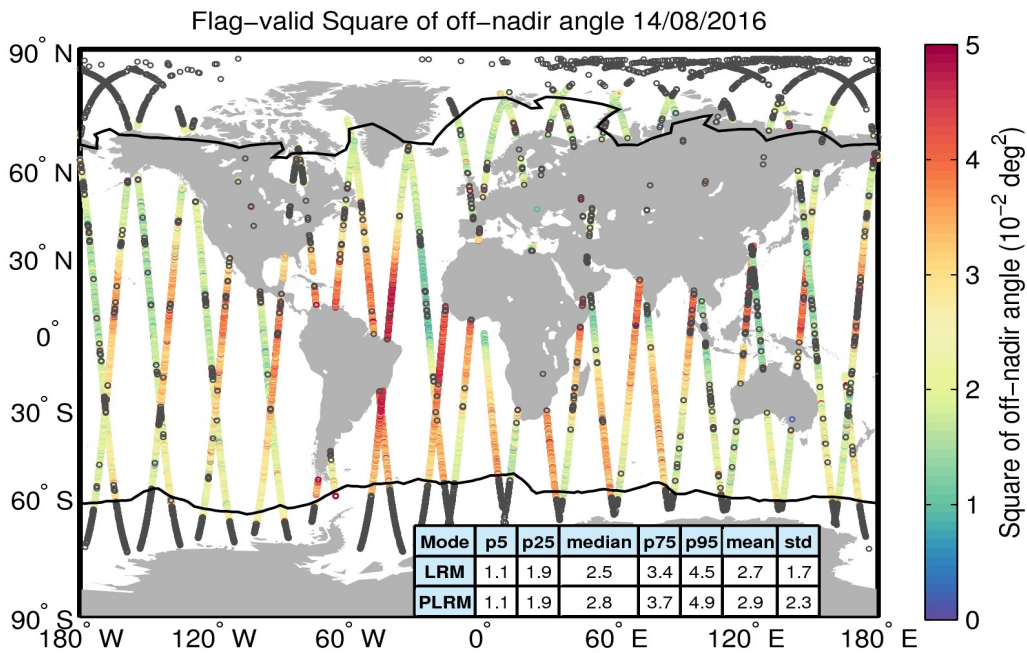
Figure 37. Geographical distribution of flag-valid mispointing data over oceans and lakes for 14/08/2016. The statistical values shown in the table refer to the mispointing in 10^{-2} \text{ deg}^2 and are calculated separately for LRM and PLRM regions. Measurements taken over polar polygons have been excluded from the computation of the statistical values. The black lines mark the outer limit of the Arctic and Antarctic polar polygons. Gray circles denote negative values.
