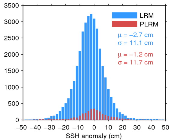
Figure 11. Histogram of science-valid SSH anomaly over oceans and lakes for LRM (blue) and PLRM (red) for 14/08/2016. The mean ( \mu ) and standard deviation ( \sigma ) are also shown. Note that values outside [-50 50] cm are excluded from the histogram for the sake of readability but not from the computation of \mu and \sigma .
