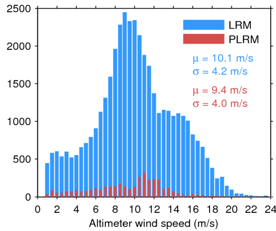
Figure 33. Histogram of flag-valid wind over oceans and lakes for LRM (blue) and PLRM (red) for 14/08/2016. The mean ( \mu ) and standard deviation ( \sigma ) are also shown. Note that values larger than 24 m/s are excluded from the histogram for the sake of readability but not from the computation of \mu and \sigma .
