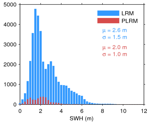
Figure 20. Histogram of science-valid SWH over oceans and lakes for LRM (blue) and PLRM (red) for 14/08/2016. The mean ( \mu ) and standard deviation ( \sigma ) are also shown. Note that values larger than 12 m are excluded from the histogram for the sake of readability but not from the computation of \mu and \sigma .
