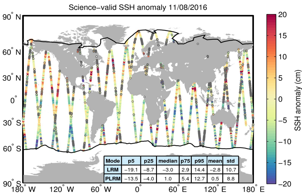
Figure 10. Geographical distribution of science-valid SSH anomaly data over oceans and lakes for 11/08/2016. The statistical values shown in the table refer to the SSH anomaly in cm and are calculated separately for LRM and PLRM regions. The black lines mark the outer limit of the Arctic and Antarctic polar polygons. Gray circles denote records that have been rejected based on the editing criteria described in Table 2.
