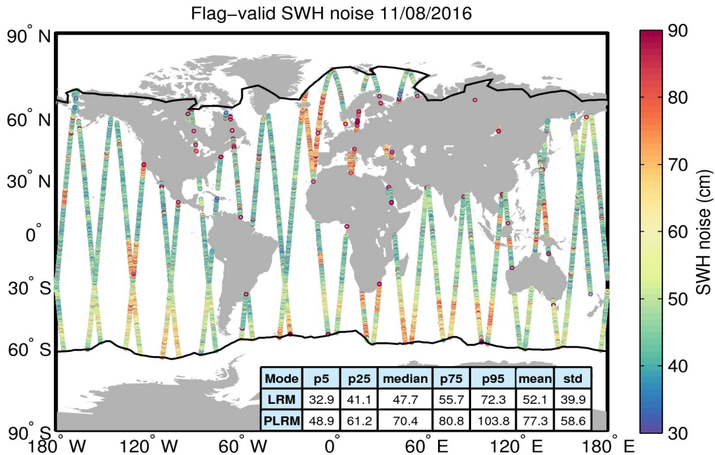
Figure 18. Geographical distribution of flag-valid 20-Hz SWH measurement noise over oceans and lakes for 11/08/2016. The statistical values shown in the table refer to the SWH noise and are calculated separately for LRM and PLRM regions. Measurements taken over polar polygons have been excluded from the computation of the statistical values. The black lines mark the outer limit of the Arctic and Antarctic polar polygons.
