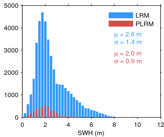
Figure 20. Histogram of science-valid SWH over oceans and lakes for LRM (blue) and PLRM (red) for 11/08/2016. The mean ( \mu ) and standard deviation ( \sigma ) are also shown. Note that values larger than 12 m are excluded from the histogram for the sake of readability but not from the computation of \mu and \sigma .
