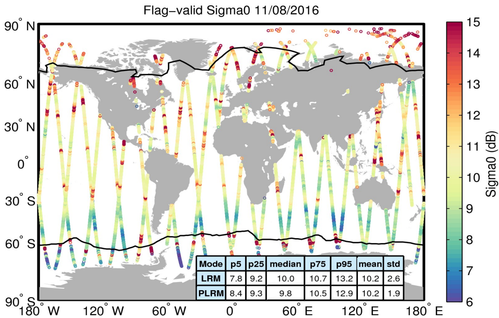
Figure 23. Geographical distribution of flag-valid sigma0 data over oceans and lakes for 11/08/2016. The statistical values shown in the table refer to the sigma0 in dB and are calculated separately for LRM and PLRM regions. Measurements taken over polar polygons have been excluded from the computation of the statistical values. The black lines mark the outer limit of the Arctic and Antarctic polar polygons.
