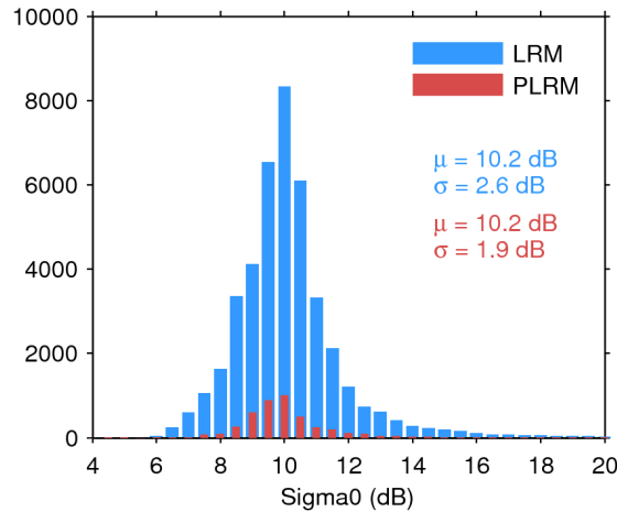
Figure 25. Histogram of flag-valid sigma0 over oceans and lakes for LRM (blue) and PLRM (red) for 11/08/2016. The mean ( \mu ) and standard deviation ( \sigma ) are also shown. Note that values outside [4 20] dB are excluded from the histogram for the sake of readability but not from the computation of \mu and \sigma .
