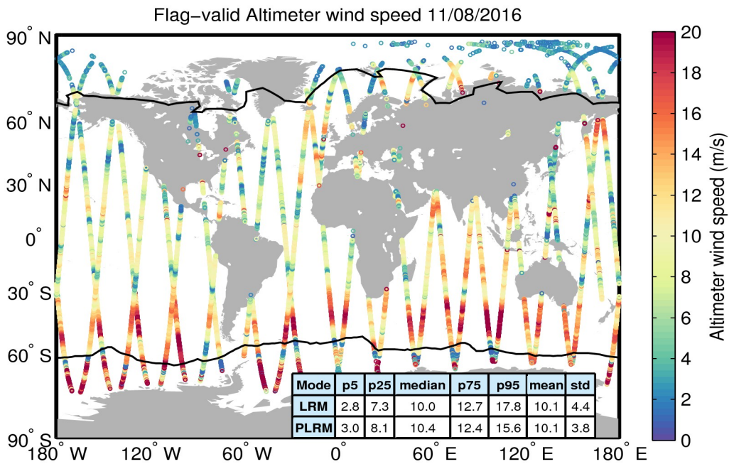
Figure 31. Geographical distribution of flag-valid wind data over oceans and lakes for 11/08/2016. The statistical values shown in the table refer to the wind in m/s and are calculated separately for LRM and PLRM regions. Measurements taken over polar polygons have been excluded from the computation of the statistical values. The black lines mark the outer limit of the Arctic and Antarctic polar polygons.
