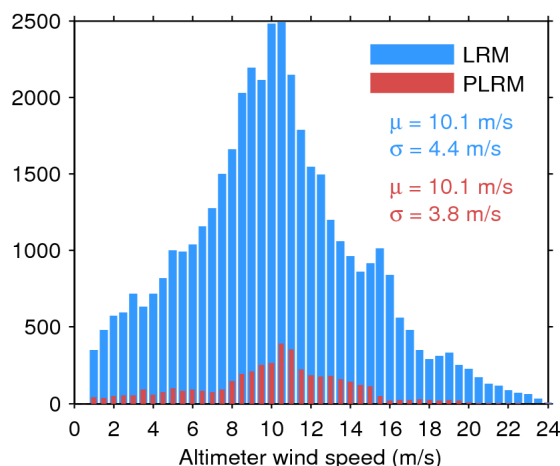
Figure 33. Histogram of flag-valid wind over oceans and lakes for LRM (blue) and PLRM (red) for 11/08/2016. The mean ( \mu ) and standard deviation ( \sigma ) are also shown. Note that values larger than 24 m/s are excluded from the histogram for the sake of readability but not from the computation of \mu and \sigma .
