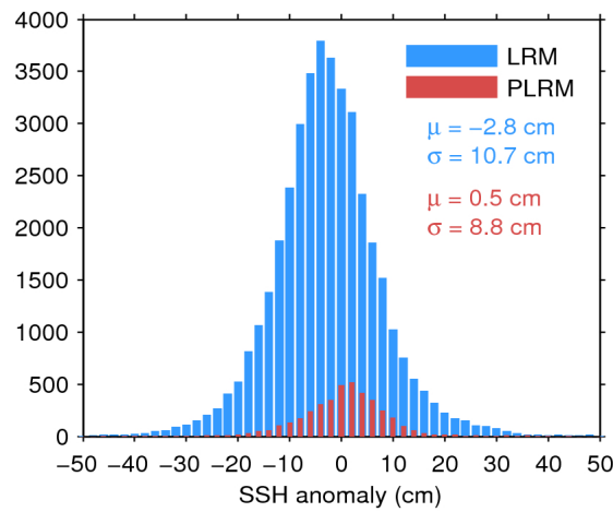
Figure 11. Histogram of science-valid SSH anomaly over oceans and lakes for LRM (blue) and PLRM (red) for 11/08/2016. The mean ( \mu ) and standard deviation ( \sigma ) are also shown. Note that values outside [-50\ 50] cm are excluded from the histogram for the sake of readability but not from the computation of \mu and \sigma .
