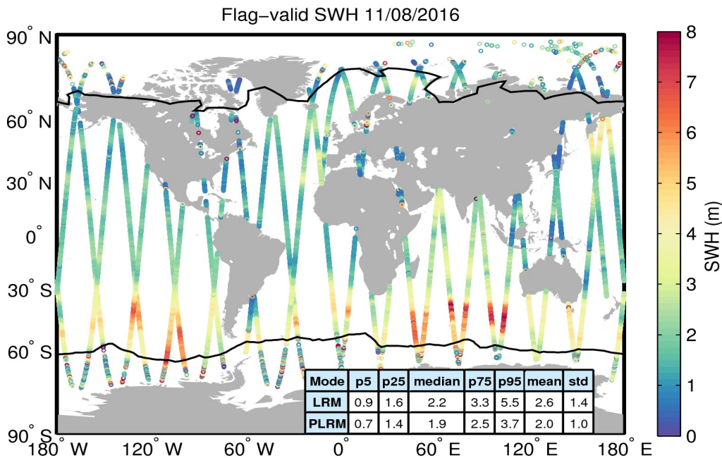
Figure 15. Geographical distribution of flag-valid SWH data over oceans and lakes for 11/08/2016. The statistical values shown in the table refer to the SWH in m and are calculated separately for LRM and PLRM regions. Measurements taken over polar polygons have been excluded from the computation of the statistical values. The black lines mark the outer limit of the Arctic and Antarctic polar polygons.
