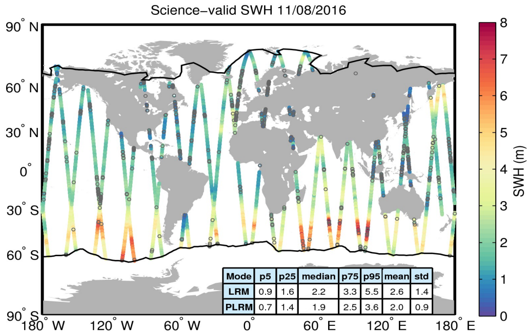
Figure 19. Geographical distribution of science-valid SWH data over oceans and lakes for 11/08/2016. The statistical values shown in the table refer to the SWH in m and are calculated separately for LRM and PLRM regions. The black lines mark the outer limit of the Arctic and Antarctic polar polygons. Gray circles denote records that have been rejected based on the editing criteria described in Table 3.
