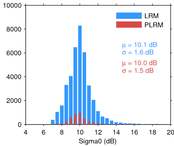
Figure 28. Histogram of science-valid sigma0 over oceans and lakes for LRM (blue) and PLRM (red) for 11/08/2016. The mean ( \mu ) and standard deviation ( \sigma ) are also shown. Note that values outside [4 20] dB are excluded from the histogram for the sake of readability but not from the computation of \mu and \sigma .
