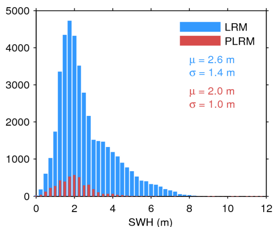
Figure 17. Histogram of flag-valid SWH over oceans and lakes for LRM (blue) and PLRM (red) for 11/08/2016. The mean ( \mu ) and standard deviation ( \sigma ) are also shown. Note that values larger than 12 m are excluded from the histogram for the sake of readability but not from the computation of \mu and \sigma .
