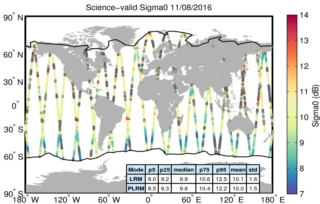
Figure 27. Geographical distribution of science-valid sigma0 data over oceans and lakes for 11/08/2016. The statistical values shown in the table refer to the sigma0 in dB and are calculated separately for LRM and PLRM regions. The black lines mark the outer limit of the Arctic and Antarctic polar polygons. Gray circles denote records that have been rejected based on the editing criteria described in Table 4.
