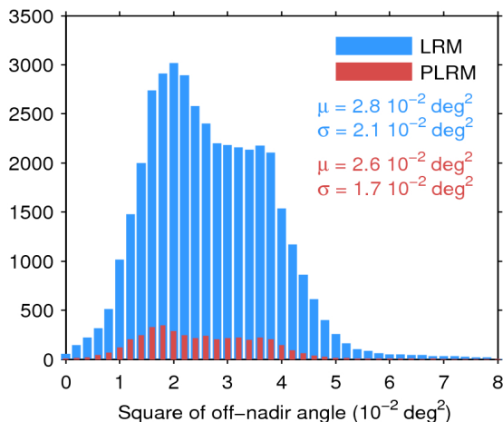
Figure 39. Histogram of flag-valid mispointing over oceans and lakes for LRM (blue) and PLRM (red) for 11/08/2016. Only positive values have been considered. The mean ( \mu ) and standard deviation ( \sigma ) are also shown. Note that values larger than 8 \cdot 10^{-2} \text{ deg}^2 are excluded from the histogram for the sake of readability but not from the computation of \mu and \sigma .
