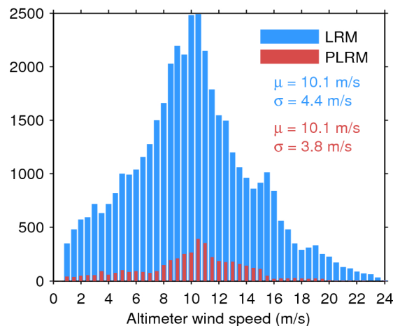
Figure 35. Histogram of science-valid wind over oceans and lakes for LRM (blue) and PLRM (red) for 11/08/2016. The mean ( \mu ) and standard deviation ( \sigma ) are also shown. Note that values larger than 24 m/s are excluded from the histogram for the sake of readability but not from the computation of \mu and \sigma .
