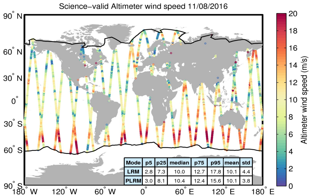
Figure 34. Geographical distribution of science-valid wind data over oceans and lakes for 11/08/2016. The statistical values shown in the table refer to the wind in m/s and are calculated separately for LRM and PLRM regions. The black lines mark the outer limit of the Arctic and Antarctic polar polygons. Gray circles denote records that have been rejected based on the editing criteria described in Table 5.
