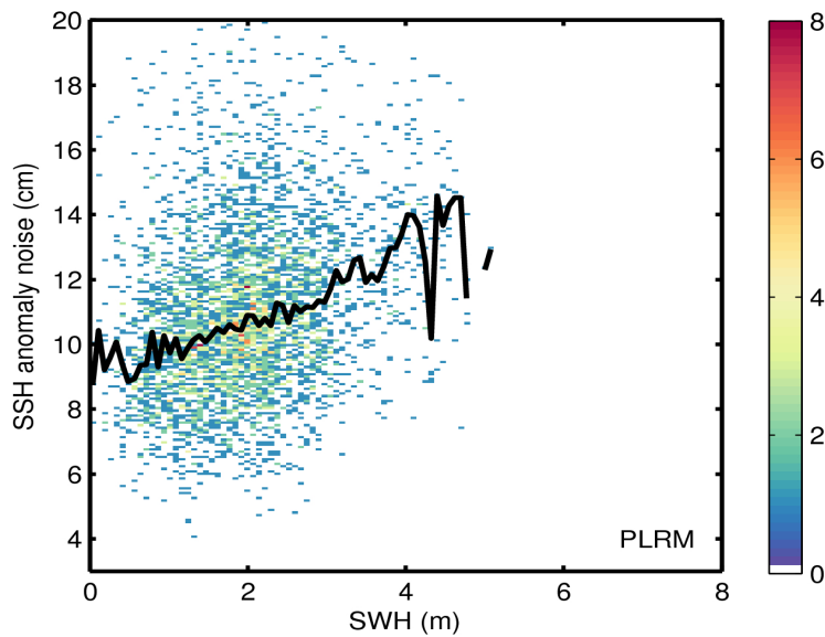
Figure 9. 2D histogram showing flag-valid SSH anomaly noise as a function of SWH for LRM (top) and PLRM (bottom) for 11/08/2016. The black line denotes the median SSH anomaly noise as a function of SWH.
