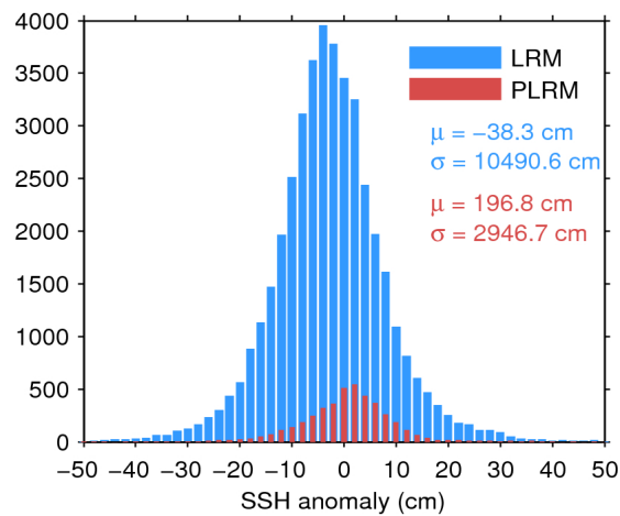
Figure 7. Histogram of flag-valid SSH anomaly over oceans and lakes for LRM (blue) and PLRM (red) for 11/08/2016. The mean ( \mu ) and standard deviation ( \sigma ) are also shown. Note that values outside [-50 50] cm are excluded from the histogram for the sake of readability but not from the computation of \mu and \sigma .
