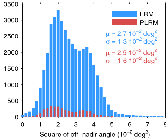
Figure 39. Histogram of flag-valid mispointing over oceans and lakes for LRM (blue) and PLRM (red) for 09/08/2016. Only positive values have been considered. The mean ( \mu ) and standard deviation ( \sigma ) are also shown. Note that values larger than 8 \cdot 10^{-2} \text{ deg}^2 are excluded from the histogram for the sake of readability but not from the computation of \mu and \sigma .
