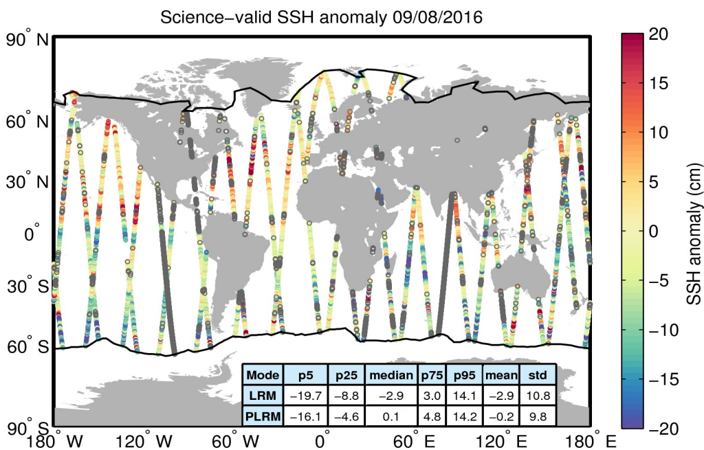
Figure 10. Geographical distribution of science-valid SSH anomaly data over oceans and lakes for 09/08/2016. The statistical values shown in the table refer to the SSH anomaly in cm and are calculated separately for LRM and PLRM regions. The black lines mark the outer limit of the Arctic and Antarctic polar polygons. Gray circles denote records that have been rejected based on the editing criteria described in Table 2.
