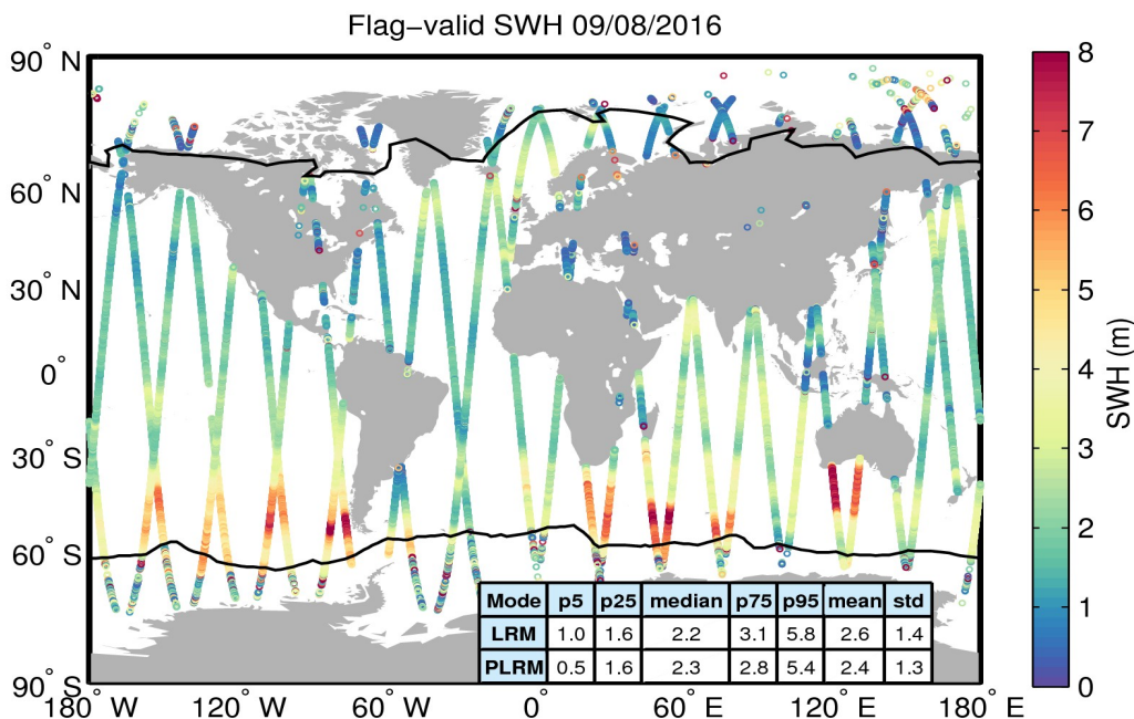
Figure 15. Geographical distribution of flag-valid SWH data over oceans and lakes for 09/08/2016. The statistical values shown in the table refer to the SWH in m and are calculated separately for LRM and PLRM regions. Measurements taken over polar polygons have been excluded from the computation of the statistical values. The black lines mark the outer limit of the Arctic and Antarctic polar polygons.
