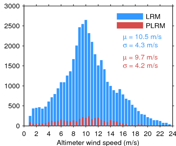
Figure 35. Histogram of science-valid wind over oceans and lakes for LRM (blue) and PLRM (red) for 09/08/2016. The mean ( \mu ) and standard deviation ( \sigma ) are also shown. Note that values larger than 24 m/s are excluded from the histogram for the sake of readability but not from the computation of \mu and \sigma .
