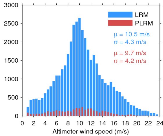
Figure 33. Histogram of flag-valid wind over oceans and lakes for LRM (blue) and PLRM (red) for 09/08/2016. The mean ( \mu ) and standard deviation ( \sigma ) are also shown. Note that values larger than 24 m/s are excluded from the histogram for the sake of readability but not from the computation of \mu and \sigma .
