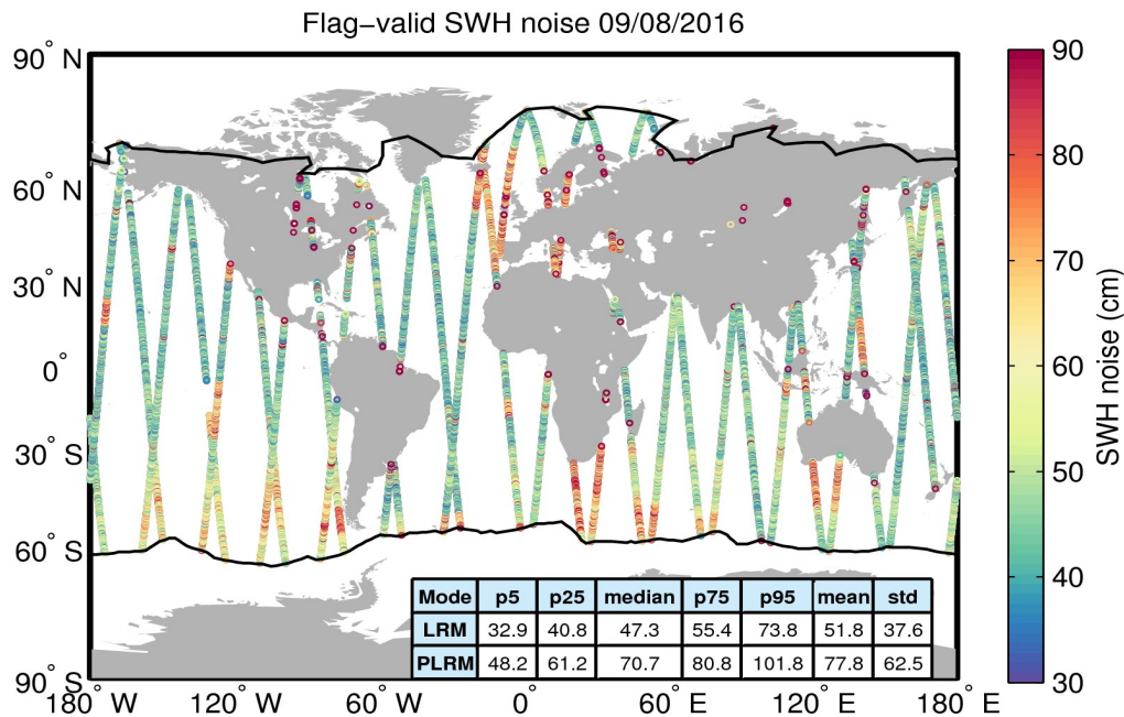
Figure 18. Geographical distribution of flag-valid 20-Hz SWH measurement noise over oceans and lakes for 09/08/2016. The statistical values shown in the table refer to the SWH noise and are calculated separately for LRM and PLRM regions. Measurements taken over polar polygons have been excluded from the computation of the statistical values. The black lines mark the outer limit of the Arctic and Antarctic polar polygons.
