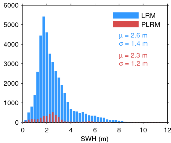
Figure 20. Histogram of science-valid SWH over oceans and lakes for LRM (blue) and PLRM (red) for 09/08/2016. The mean ( \mu ) and standard deviation ( \sigma ) are also shown. Note that values larger than 12 m are excluded from the histogram for the sake of readability but not from the computation of \mu and \sigma .
