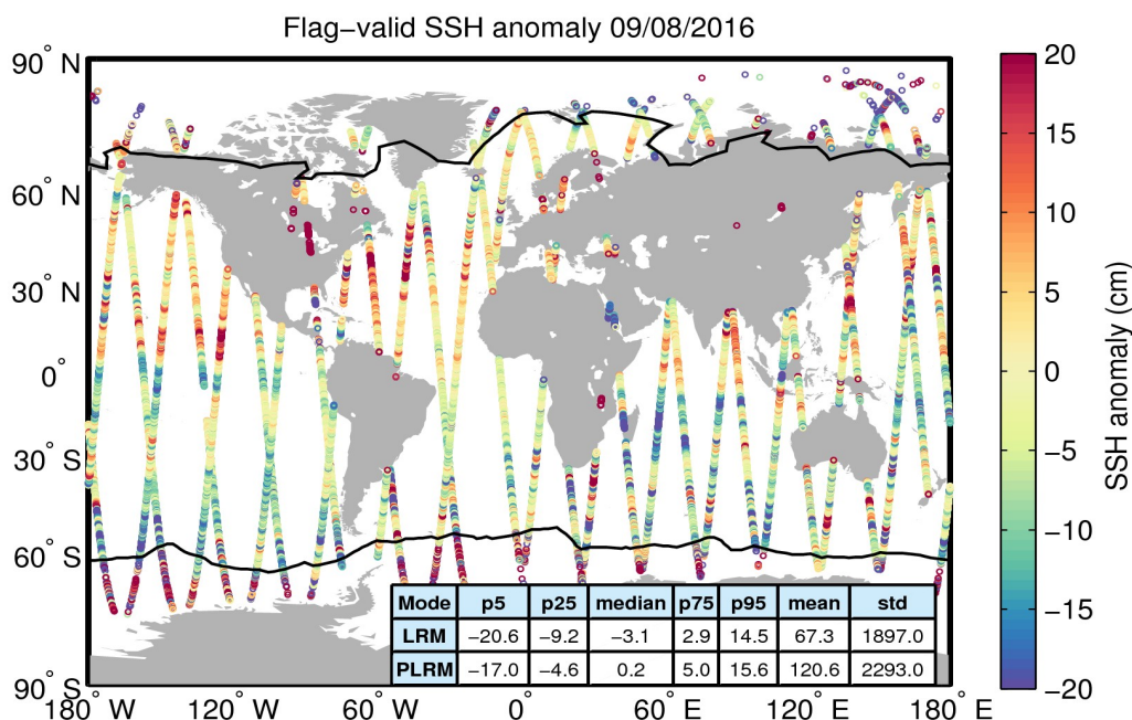
Figure 5. Geographical distribution of flag-valid 1-Hz SSH anomaly data over oceans and lakes for 09/08/2016. The statistical values shown in the table refer to the SSH anomaly in cm and are calculated separately for LRM and PLRM regions. Measurements taken over polar polygons have been excluded from the computation of the statistical values. The black lines mark the outer limit of the Arctic and Antarctic polar polygons.
