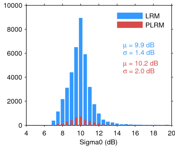
Figure 28. Histogram of science-valid sigma0 over oceans and lakes for LRM (blue) and PLRM (red) for 09/08/2016. The mean ( \mu ) and standard deviation ( \sigma ) are also shown. Note that values outside [4 20] dB are excluded from the histogram for the sake of readability but not from the computation of \mu and \sigma .
