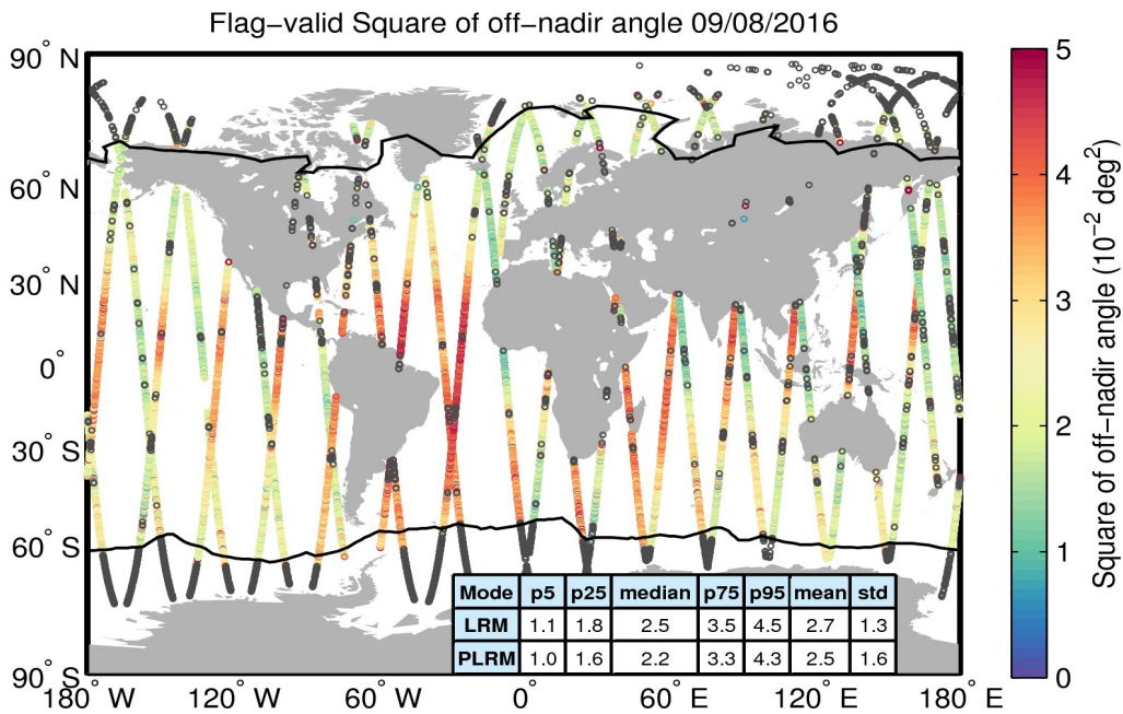
Figure 37. Geographical distribution of flag-valid mispointing data over oceans and lakes for 09/08/2016. The statistical values shown in the table refer to the mispointing in 10^{-2} deg 2 and are calculated separately for LRM and PLRM regions. Measurements taken over polar polygons have been excluded from the computation of the statistical values. The black lines mark the outer limit of the Arctic and Antarctic polar polygons. Gray circles denote negative values.
