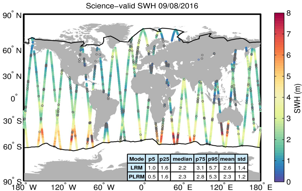
Figure 19. Geographical distribution of science-valid SWH data over oceans and lakes for 09/08/2016. The statistical values shown in the table refer to the SWH in m and are calculated separately for LRM and PLRM regions. The black lines mark the outer limit of the Arctic and Antarctic polar polygons. Gray circles denote records that have been rejected based on the editing criteria described in Table 3.
