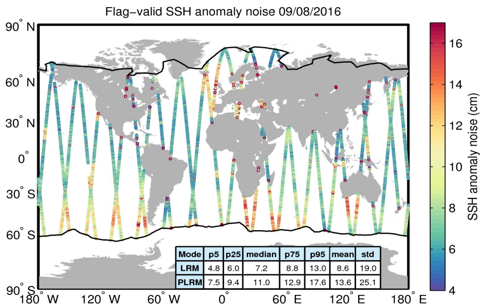
Figure 8. Geographical distribution of flag-valid 20-Hz SSH anomaly measurement noise over oceans and lakes for 09/08/2016. The statistical values shown in the table refer to the SSH anomaly noise and are calculated separately for LRM and PLRM regions. Measurements taken over polar polygons have been excluded from the computation of the statistical values. The black lines mark the outer limit of the Arctic and Antarctic polar polygons.
