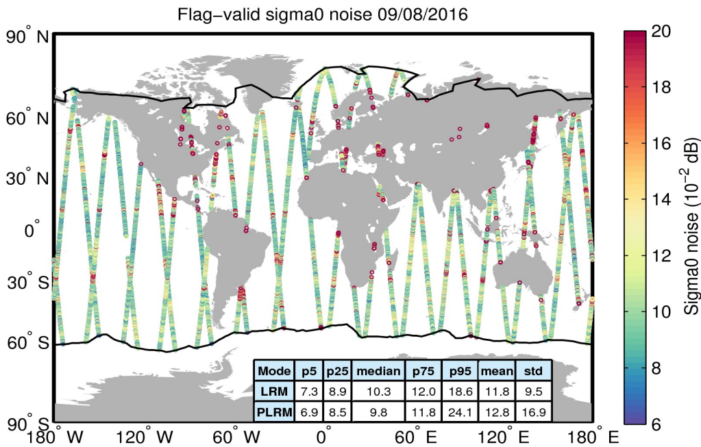
Figure 26. Geographical distribution of flag-valid 20-Hz sigma0 measurement noise over oceans and lakes for 09/08/2016. The statistical values shown in the table refer to the sigma0 noise and are calculated separately for LRM and PLRM regions. Measurements taken over polar polygons have been excluded from the computation of the statistical values. The black lines mark the outer limit of the Arctic and Antarctic polar polygons.
