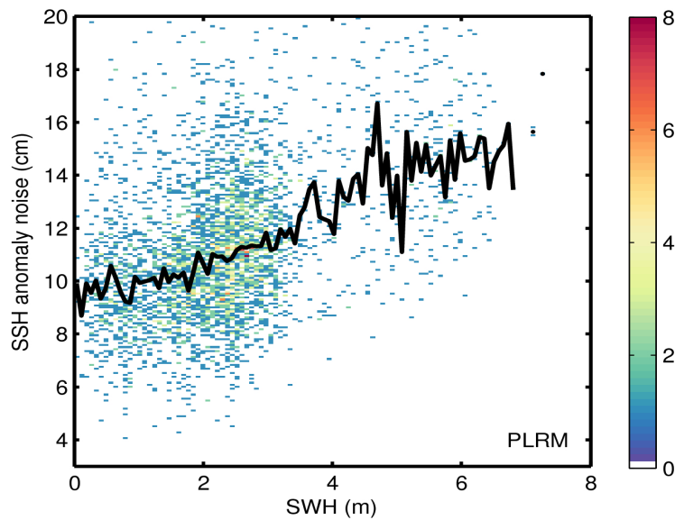
Figure 9. 2D histogram showing flag-valid SSH anomaly noise as a function of SWH for LRM (top) and PLRM (bottom) for 09/08/2016. The black line denotes the median SSH anomaly noise as a function of SWH.
