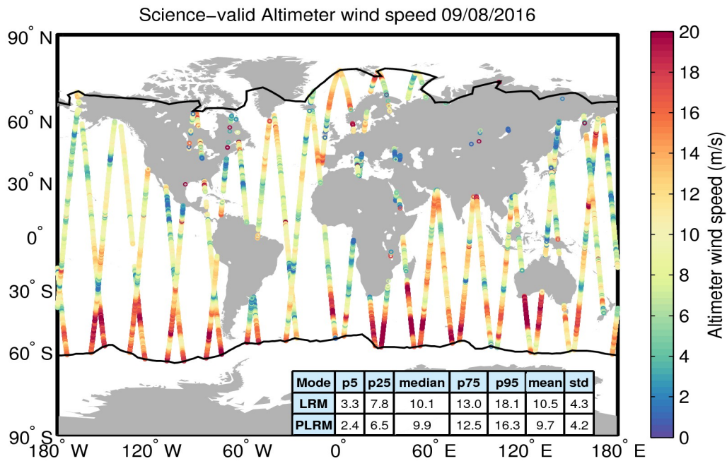
Figure 34. Geographical distribution of science-valid wind data over oceans and lakes for 09/08/2016. The statistical values shown in the table refer to the wind in m/s and are calculated separately for LRM and PLRM regions. The black lines mark the outer limit of the Arctic and Antarctic polar polygons. Gray circles denote records that have been rejected based on the editing criteria described in Table 5.
