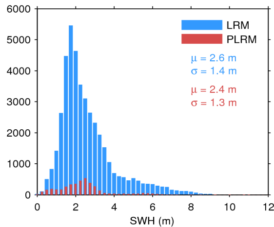
Figure 17. Histogram of flag-valid SWH over oceans and lakes for LRM (blue) and PLRM (red) for 09/08/2016. The mean ( \mu ) and standard deviation ( \sigma ) are also shown. Note that values larger than 12 m are excluded from the histogram for the sake of readability but not from the computation of \mu and \sigma .
