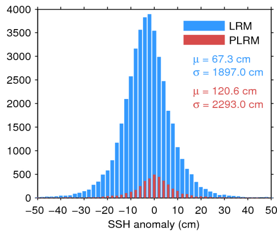
Figure 7. Histogram of flag-valid SSH anomaly over oceans and lakes for LRM (blue) and PLRM (red) for 09/08/2016. The mean ( \mu ) and standard deviation ( \sigma ) are also shown. Note that values outside [-50\ 50] cm are excluded from the histogram for the sake of readability but not from the computation of \mu and \sigma .
