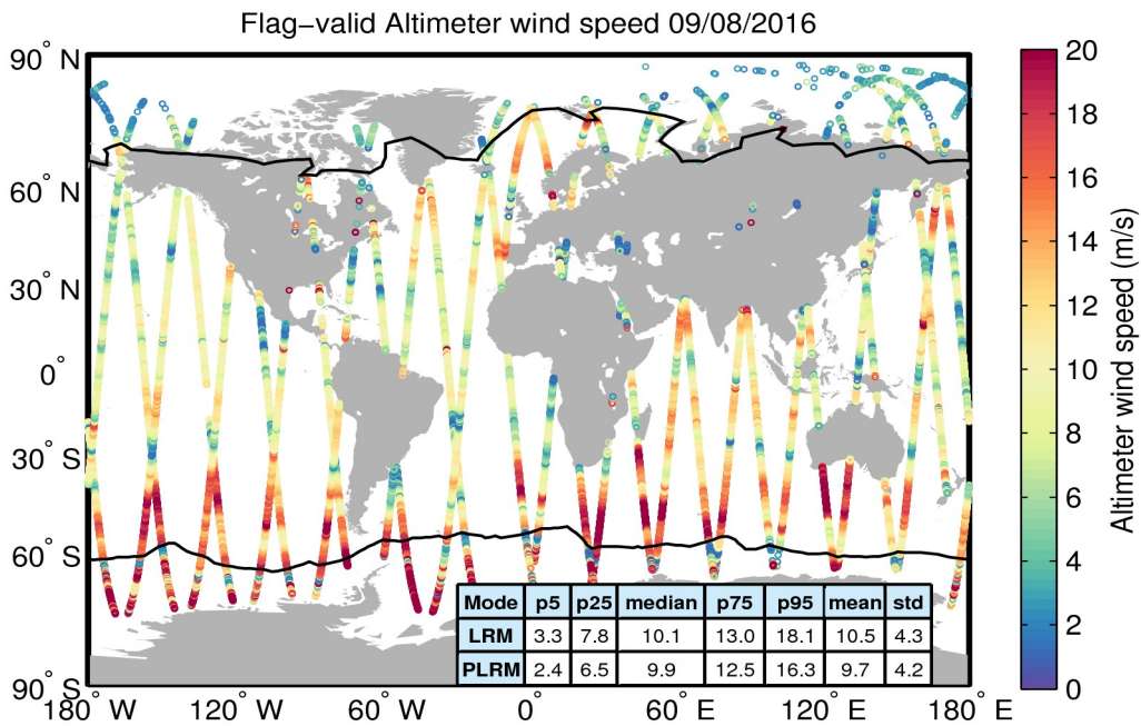
Figure 31. Geographical distribution of flag-valid wind data over oceans and lakes for 09/08/2016. The statistical values shown in the table refer to the wind in m/s and are calculated separately for LRM and PLRM regions. Measurements taken over polar polygons have been excluded from the computation of the statistical values. The black lines mark the outer limit of the Arctic and Antarctic polar polygons.
