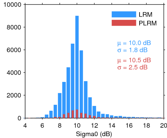
Figure 25. Histogram of flag-valid sigma0 over oceans and lakes for LRM (blue) and PLRM (red) for 09/08/2016. The mean ( \mu ) and standard deviation ( \sigma ) are also shown. Note that values outside [4 20] dB are excluded from the histogram for the sake of readability but not from the computation of \mu and \sigma .
