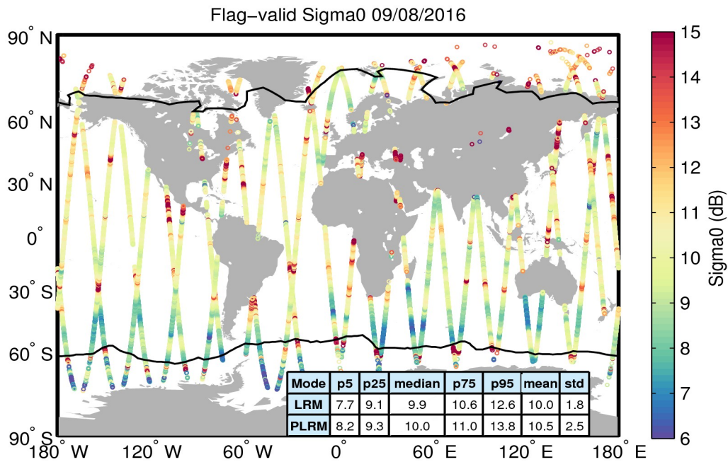
Figure 23. Geographical distribution of flag-valid sigma0 data over oceans and lakes for 09/08/2016. The statistical values shown in the table refer to the sigma0 in dB and are calculated separately for LRM and PLRM regions. Measurements taken over polar polygons have been excluded from the computation of the statistical values. The black lines mark the outer limit of the Arctic and Antarctic polar polygons.
