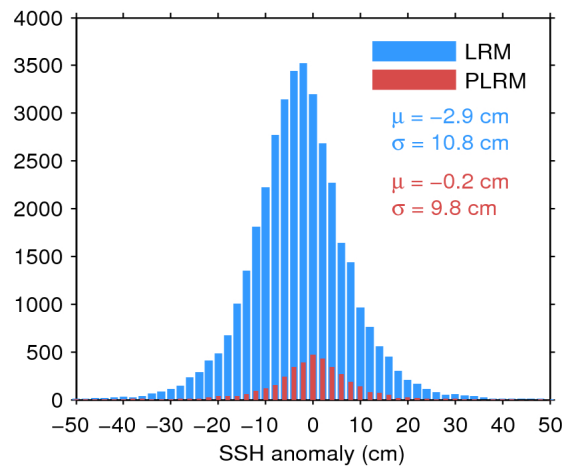
Figure 11. Histogram of science-valid SSH anomaly over oceans and lakes for LRM (blue) and PLRM (red) for 09/08/2016. The mean ( \mu ) and standard deviation ( \sigma ) are also shown. Note that values outside [-50\ 50] cm are excluded from the histogram for the sake of readability but not from the computation of \mu and \sigma .
