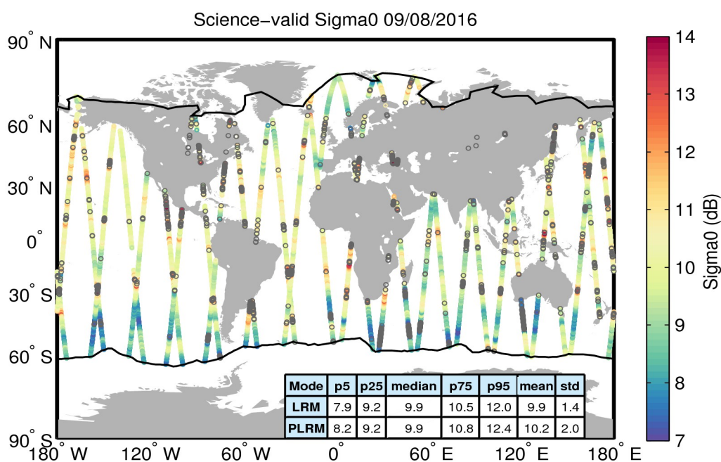
Figure 27. Geographical distribution of science-valid sigma0 data over oceans and lakes for 09/08/2016. The statistical values shown in the table refer to the sigma0 in dB and are calculated separately for LRM and PLRM regions. The black lines mark the outer limit of the Arctic and Antarctic polar polygons. Gray circles denote records that have been rejected based on the editing criteria described in Table 4.
