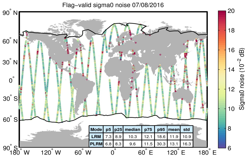
Figure 26. Geographical distribution of flag-valid 20-Hz sigma0 measurement noise over oceans and lakes for 07/08/2016. The statistical values shown in the table refer to the sigma0 noise and are calculated separately for LRM and PLRM regions. Measurements taken over polar polygons have been excluded from the computation of the statistical values. The black lines mark the outer limit of the Arctic and Antarctic polar polygons.
