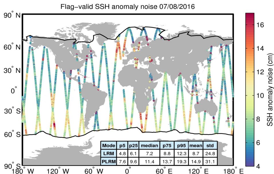
Figure 8. Geographical distribution of flag-valid 20-Hz SSH anomaly measurement noise over oceans and lakes for 07/08/2016. The statistical values shown in the table refer to the SSH anomaly noise and are calculated separately for LRM and PLRM regions. Measurements taken over polar polygons have been excluded from the computation of the statistical values. The black lines mark the outer limit of the Arctic and Antarctic polar polygons.
