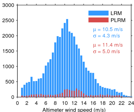
Figure 33. Histogram of flag-valid wind over oceans and lakes for LRM (blue) and PLRM (red) for 07/08/2016. The mean ( \mu ) and standard deviation ( \sigma ) are also shown. Note that values larger than 24 m/s are excluded from the histogram for the sake of readability but not from the computation of \mu and \sigma .
