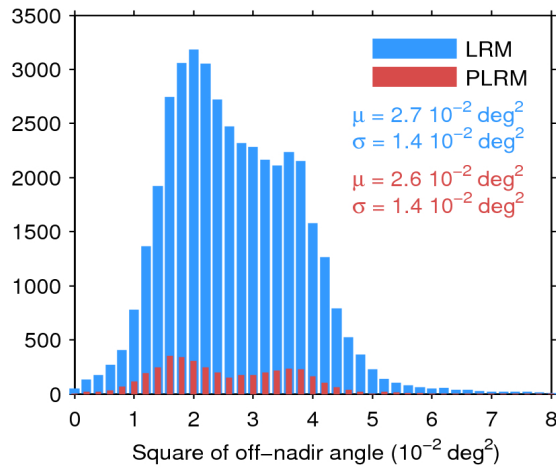
Figure 39. Histogram of flag-valid mispointing over oceans and lakes for LRM (blue) and PLRM (red) for 07/08/2016. Only positive values have been considered. The mean ( \mu ) and standard deviation ( \sigma ) are also shown. Note that values larger than 8 \cdot 10^{-2} \text{ deg}^2 are excluded from the histogram for the sake of readability but not from the computation of \mu and \sigma .
