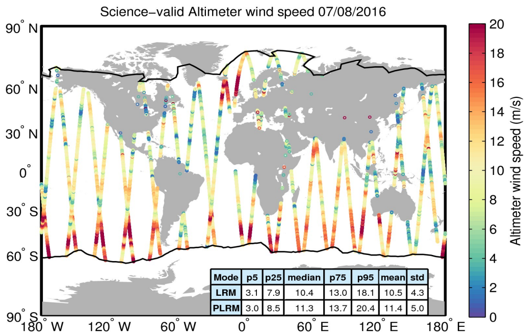
Figure 34. Geographical distribution of science-valid wind data over oceans and lakes for 07/08/2016. The statistical values shown in the table refer to the wind in m/s and are calculated separately for LRM and PLRM regions. The black lines mark the outer limit of the Arctic and Antarctic polar polygons. Gray circles denote records that have been rejected based on the editing criteria described in Table 5.
