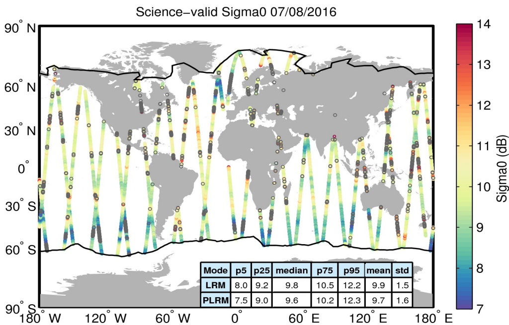
Figure 27. Geographical distribution of science-valid sigma0 data over oceans and lakes for 07/08/2016. The statistical values shown in the table refer to the sigma0 in dB and are calculated separately for LRM and PLRM regions. The black lines mark the outer limit of the Arctic and Antarctic polar polygons. Gray circles denote records that have been rejected based on the editing criteria described in Table 4.
