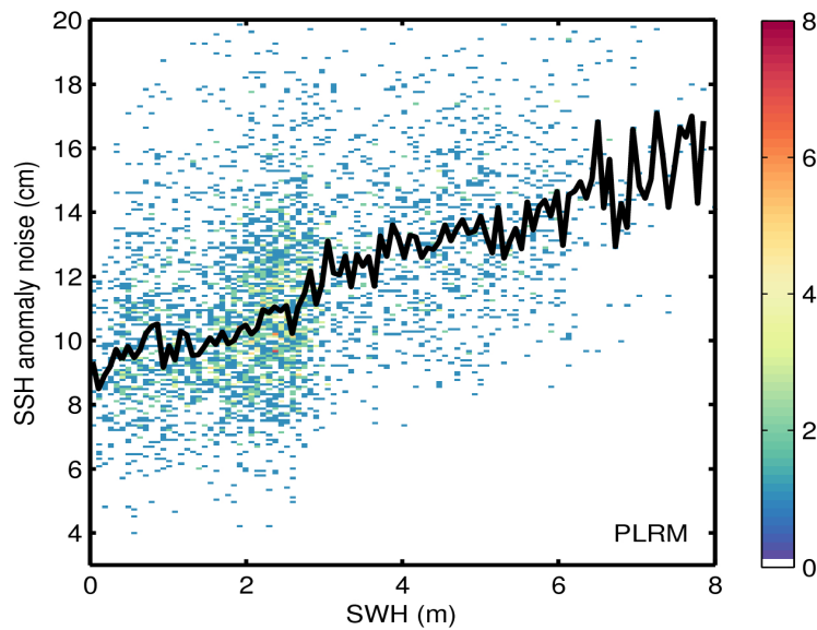
Figure 9. 2D histogram showing flag-valid SSH anomaly noise as a function of SWH for LRM (top) and PLRM (bottom) for 07/08/2016. The black line denotes the median SSH anomaly noise as a function of SWH.
