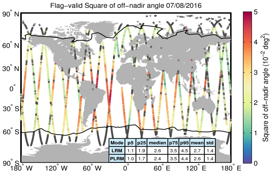
Figure 37. Geographical distribution of flag-valid mispointing data over oceans and lakes for 07/08/2016. The statistical values shown in the table refer to the mispointing in 10^{-2} deg 2 and are calculated separately for LRM and PLRM regions. Measurements taken over polar polygons have been excluded from the computation of the statistical values. The black lines mark the outer limit of the Arctic and Antarctic polar polygons. Gray circles denote negative values.
