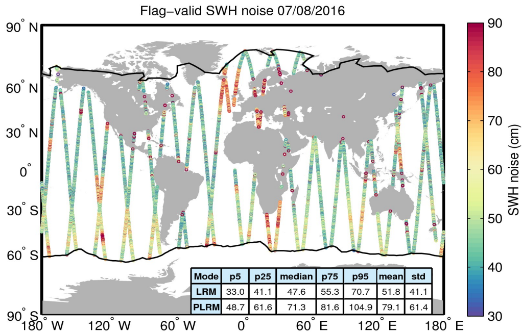
Figure 18. Geographical distribution of flag-valid 20-Hz SWH measurement noise over oceans and lakes for 07/08/2016. The statistical values shown in the table refer to the SWH noise and are calculated separately for LRM and PLRM regions. Measurements taken over polar polygons have been excluded from the computation of the statistical values. The black lines mark the outer limit of the Arctic and Antarctic polar polygons.
