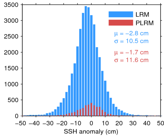
Figure 11. Histogram of science-valid SSH anomaly over oceans and lakes for LRM (blue) and PLRM (red) for 07/08/2016. The mean ( \mu ) and standard deviation ( \sigma ) are also shown. Note that values outside [-50\ 50] cm are excluded from the histogram for the sake of readability but not from the computation of \mu and \sigma .
