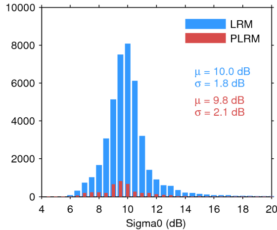
Figure 25. Histogram of flag-valid sigma0 over oceans and lakes for LRM (blue) and PLRM (red) for 07/08/2016. The mean ( \mu ) and standard deviation ( \sigma ) are also shown. Note that values outside [4 20] dB are excluded from the histogram for the sake of readability but not from the computation of \mu and \sigma .
