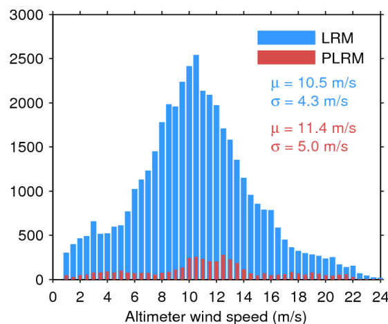
Figure 35. Histogram of science-valid wind over oceans and lakes for LRM (blue) and PLRM (red) for 07/08/2016. The mean ( \mu ) and standard deviation ( \sigma ) are also shown. Note that values larger than 24 m/s are excluded from the histogram for the sake of readability but not from the computation of \mu and \sigma .
