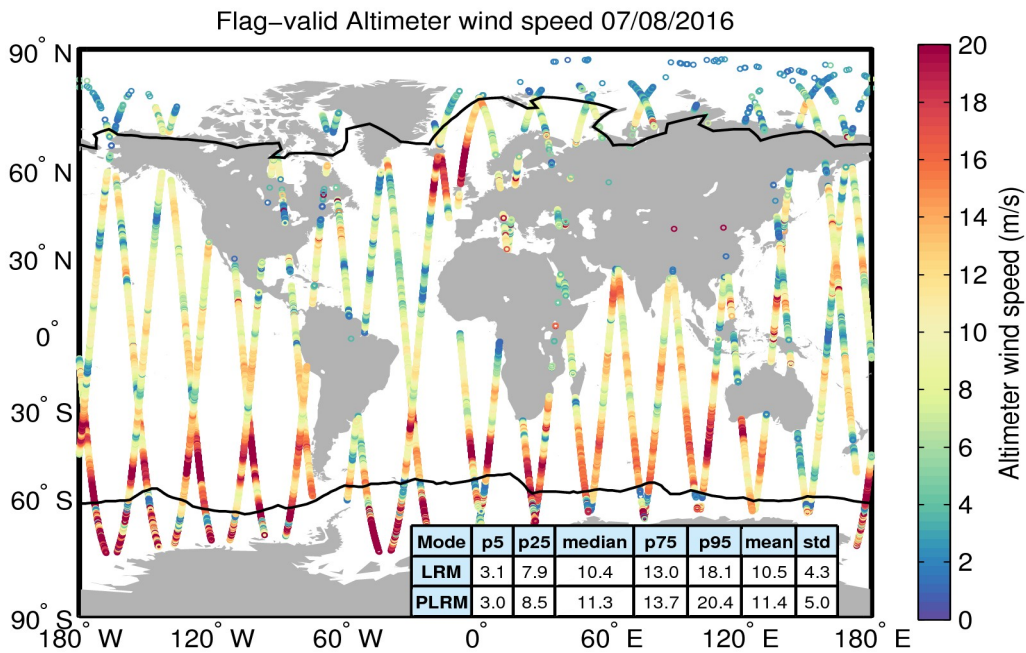
Figure 31. Geographical distribution of flag-valid wind data over oceans and lakes for 07/08/2016. The statistical values shown in the table refer to the wind in m/s and are calculated separately for LRM and PLRM regions. Measurements taken over polar polygons have been excluded from the computation of the statistical values. The black lines mark the outer limit of the Arctic and Antarctic polar polygons.
