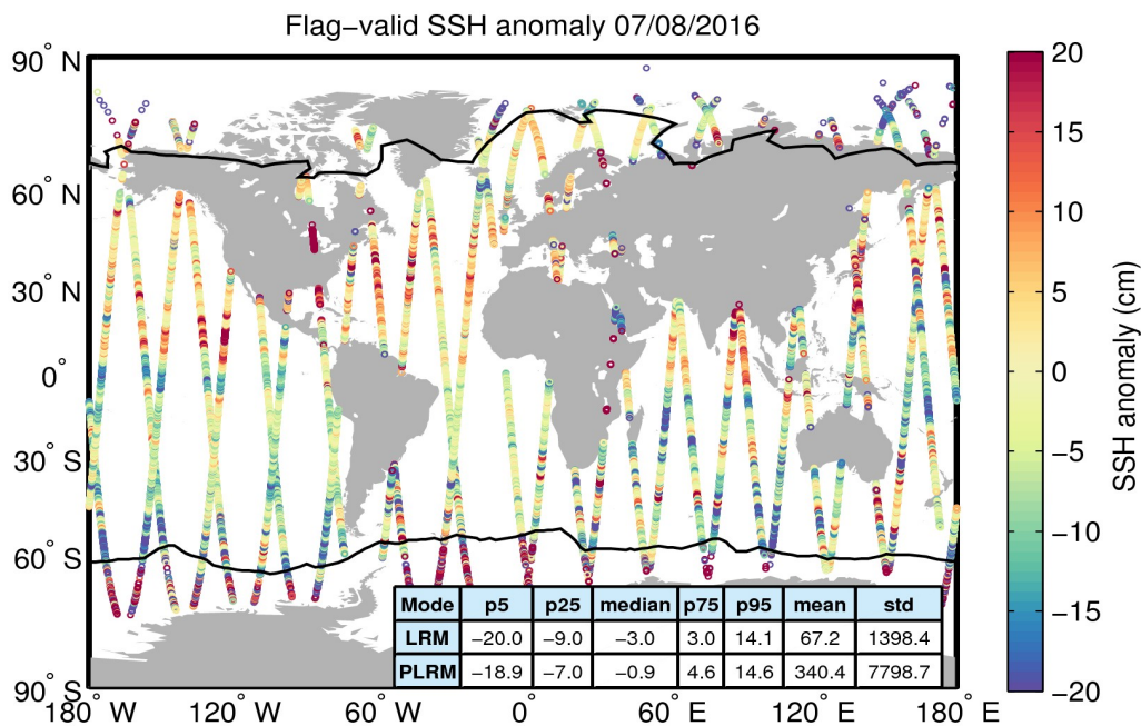
Figure 5. Geographical distribution of flag-valid 1-Hz SSH anomaly data over oceans and lakes for 07/08/2016. The statistical values shown in the table refer to the SSH anomaly in cm and are calculated separately for LRM and PLRM regions. Measurements taken over polar polygons have been excluded from the computation of the statistical values. The black lines mark the outer limit of the Arctic and Antarctic polar polygons.
