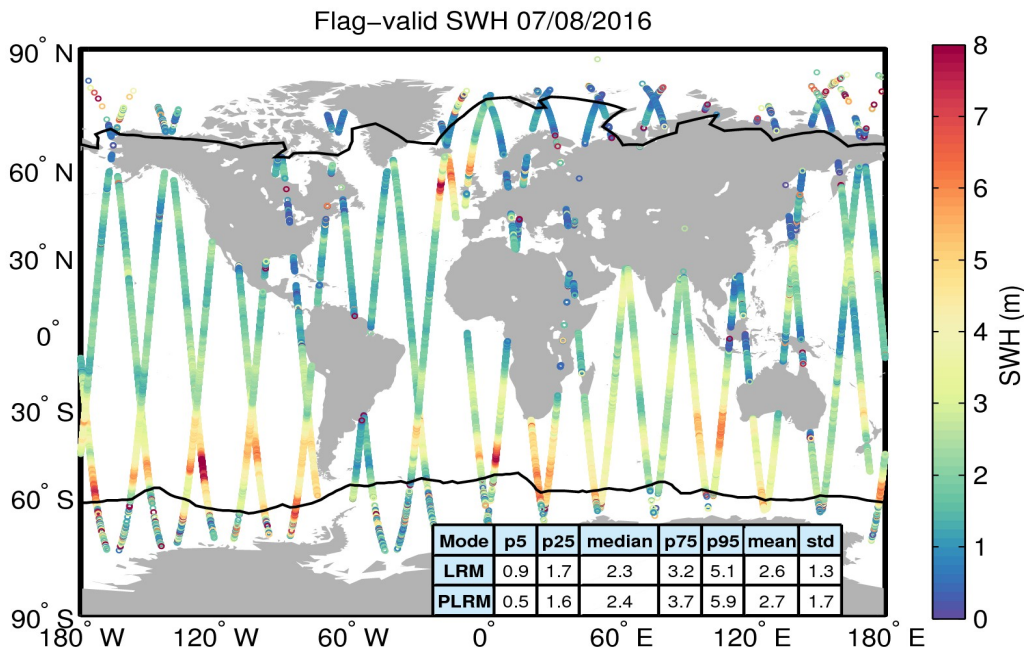
Figure 15. Geographical distribution of flag-valid SWH data over oceans and lakes for 07/08/2016. The statistical values shown in the table refer to the SWH in m and are calculated separately for LRM and PLRM regions. Measurements taken over polar polygons have been excluded from the computation of the statistical values. The black lines mark the outer limit of the Arctic and Antarctic polar polygons.
