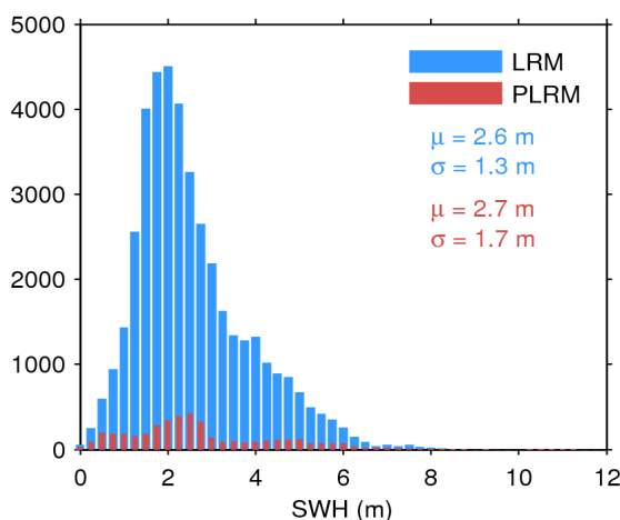
Figure 17. Histogram of flag-valid SWH over oceans and lakes for LRM (blue) and PLRM (red) for 07/08/2016. The mean ( \mu ) and standard deviation ( \sigma ) are also shown. Note that values larger than 12 m are excluded from the histogram for the sake of readability but not from the computation of \mu and \sigma .
