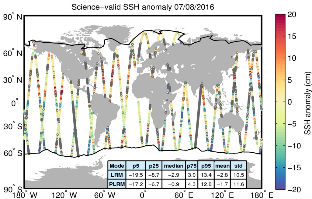
Figure 10. Geographical distribution of science-valid SSH anomaly data over oceans and lakes for 07/08/2016. The statistical values shown in the table refer to the SSH anomaly in cm and are calculated separately for LRM and PLRM regions. The black lines mark the outer limit of the Arctic and Antarctic polar polygons. Gray circles denote records that have been rejected based on the editing criteria described in Table 2.
