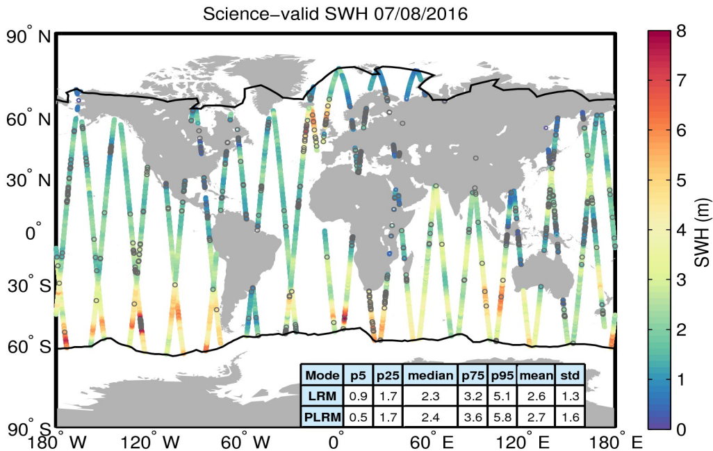
Figure 19. Geographical distribution of science-valid SWH data over oceans and lakes for 07/08/2016. The statistical values shown in the table refer to the SWH in m and are calculated separately for LRM and PLRM regions. The black lines mark the outer limit of the Arctic and Antarctic polar polygons. Gray circles denote records that have been rejected based on the editing criteria described in Table 3.
