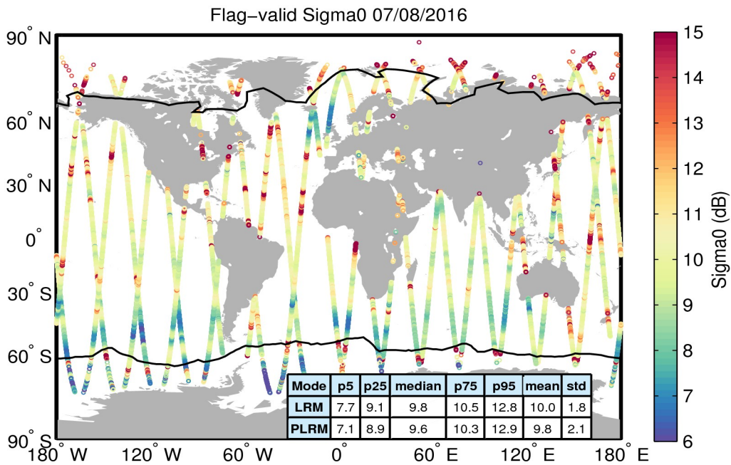
Figure 23. Geographical distribution of flag-valid sigma0 data over oceans and lakes for 07/08/2016. The statistical values shown in the table refer to the sigma0 in dB and are calculated separately for LRM and PLRM regions. Measurements taken over polar polygons have been excluded from the computation of the statistical values. The black lines mark the outer limit of the Arctic and Antarctic polar polygons.
