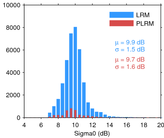
Figure 28. Histogram of science-valid sigma0 over oceans and lakes for LRM (blue) and PLRM (red) for 07/08/2016. The mean ( \mu ) and standard deviation ( \sigma ) are also shown. Note that values outside [4 20] dB are excluded from the histogram for the sake of readability but not from the computation of \mu and \sigma .
