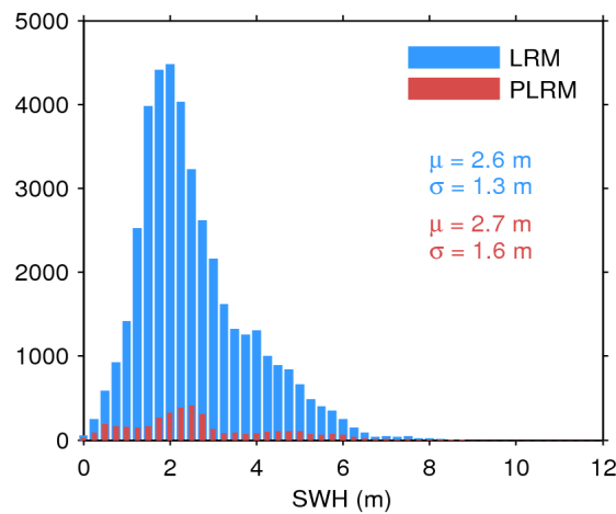
Figure 20. Histogram of science-valid SWH over oceans and lakes for LRM (blue) and PLRM (red) for 07/08/2016. The mean ( \mu ) and standard deviation ( \sigma ) are also shown. Note that values larger than 12 m are excluded from the histogram for the sake of readability but not from the computation of \mu and \sigma .
