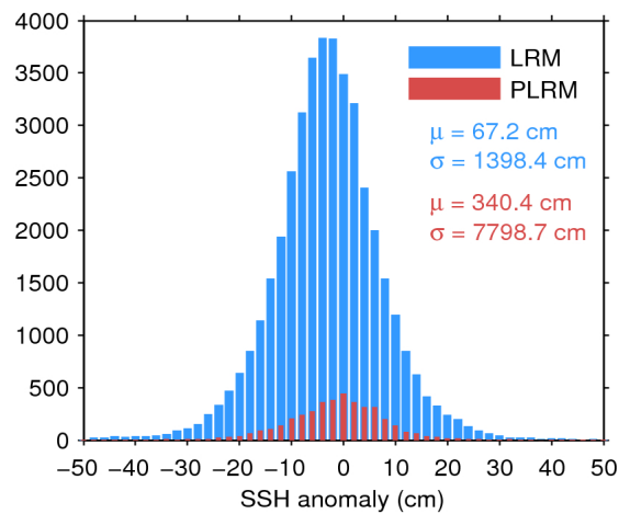
Figure 7. Histogram of flag-valid SSH anomaly over oceans and lakes for LRM (blue) and PLRM (red) for 07/08/2016. The mean ( \mu ) and standard deviation ( \sigma ) are also shown. Note that values outside [-50\ 50] cm are excluded from the histogram for the sake of readability but not from the computation of \mu and \sigma .
