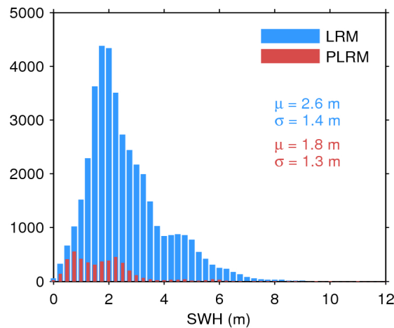
Figure 17. Histogram of flag-valid SWH over oceans and lakes for LRM (blue) and PLRM (red) for 06/08/2016. The mean ( \mu ) and standard deviation ( \sigma ) are also shown. Note that values larger than 12 m are excluded from the histogram for the sake of readability but not from the computation of \mu and \sigma .
