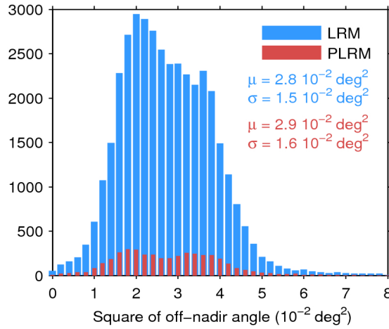
Figure 39. Histogram of flag-valid mispointing over oceans and lakes for LRM (blue) and PLRM (red) for 06/08/2016. Only positive values have been considered. The mean ( \mu ) and standard deviation ( \sigma ) are also shown. Note that values larger than 8 \cdot 10^{-2} \text{ deg}^2 are excluded from the histogram for the sake of readability but not from the computation of \mu and \sigma .
