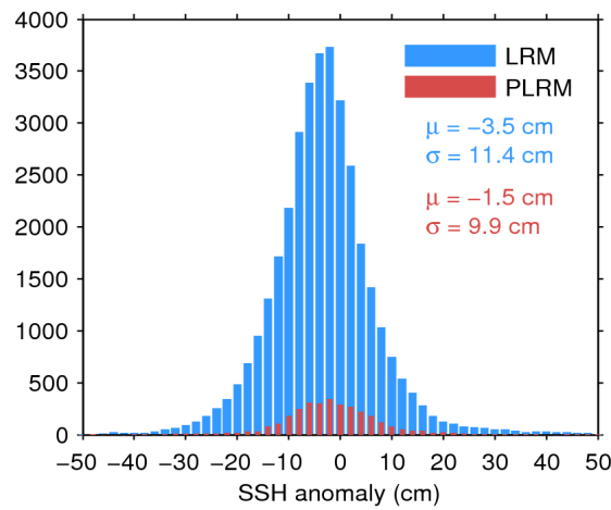
Figure 11. Histogram of science-valid SSH anomaly over oceans and lakes for LRM (blue) and PLRM (red) for 06/08/2016. The mean ( \mu ) and standard deviation ( \sigma ) are also shown. Note that values outside [-50\ 50] cm are excluded from the histogram for the sake of readability but not from the computation of \mu and \sigma .
