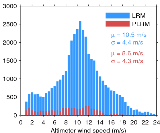
Figure 33. Histogram of flag-valid wind over oceans and lakes for LRM (blue) and PLRM (red) for 06/08/2016. The mean ( \mu ) and standard deviation ( \sigma ) are also shown. Note that values larger than 24 m/s are excluded from the histogram for the sake of readability but not from the computation of \mu and \sigma .
