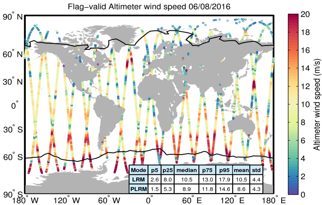
Figure 31. Geographical distribution of flag-valid wind data over oceans and lakes for 06/08/2016. The statistical values shown in the table refer to the wind in m/s and are calculated separately for LRM and PLRM regions. Measurements taken over polar polygons have been excluded from the computation of the statistical values. The black lines mark the outer limit of the Arctic and Antarctic polar polygons.
