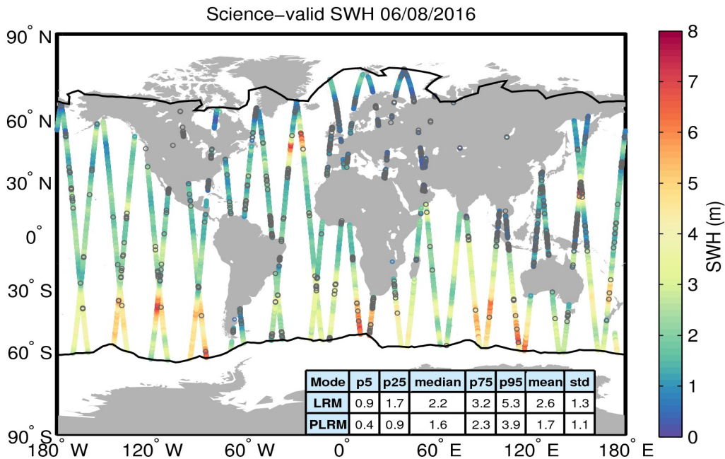
Figure 19. Geographical distribution of science-valid SWH data over oceans and lakes for 06/08/2016. The statistical values shown in the table refer to the SWH in m and are calculated separately for LRM and PLRM regions. The black lines mark the outer limit of the Arctic and Antarctic polar polygons. Gray circles denote records that have been rejected based on the editing criteria described in Table 3.
