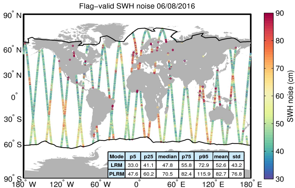
Figure 18. Geographical distribution of flag-valid 20-Hz SWH measurement noise over oceans and lakes for 06/08/2016. The statistical values shown in the table refer to the SWH noise and are calculated separately for LRM and PLRM regions. Measurements taken over polar polygons have been excluded from the computation of the statistical values. The black lines mark the outer limit of the Arctic and Antarctic polar polygons.
