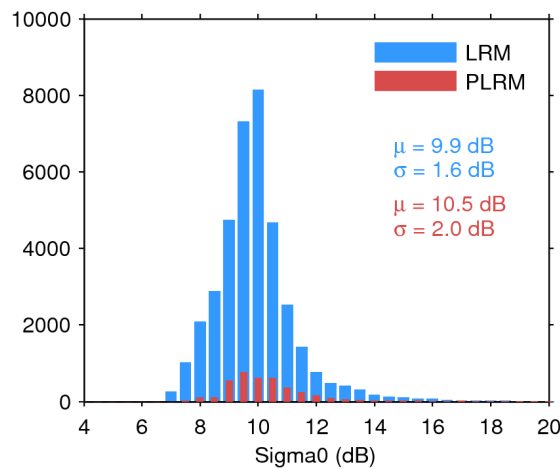
Figure 28. Histogram of science-valid sigma0 over oceans and lakes for LRM (blue) and PLRM (red) for 06/08/2016. The mean ( \mu ) and standard deviation ( \sigma ) are also shown. Note that values outside [4 20] dB are excluded from the histogram for the sake of readability but not from the computation of \mu and \sigma .
