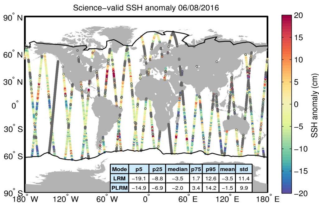
Figure 10. Geographical distribution of science-valid SSH anomaly data over oceans and lakes for 06/08/2016. The statistical values shown in the table refer to the SSH anomaly in cm and are calculated separately for LRM and PLRM regions. The black lines mark the outer limit of the Arctic and Antarctic polar polygons. Gray circles denote records that have been rejected based on the editing criteria described in Table 2.
