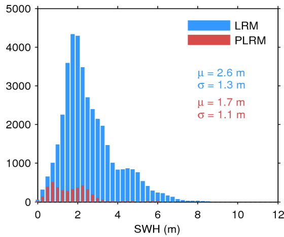
Figure 20. Histogram of science-valid SWH over oceans and lakes for LRM (blue) and PLRM (red) for 06/08/2016. The mean ( \mu ) and standard deviation ( \sigma ) are also shown. Note that values larger than 12 m are excluded from the histogram for the sake of readability but not from the computation of \mu and \sigma .
