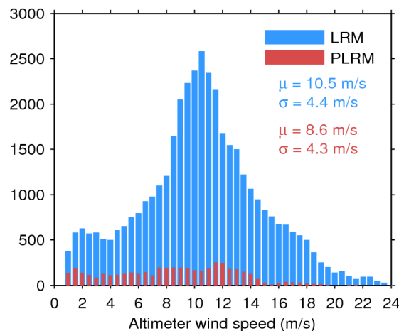
Figure 35. Histogram of science-valid wind over oceans and lakes for LRM (blue) and PLRM (red) for 06/08/2016. The mean ( \mu ) and standard deviation ( \sigma ) are also shown. Note that values larger than 24 m/s are excluded from the histogram for the sake of readability but not from the computation of \mu and \sigma .
