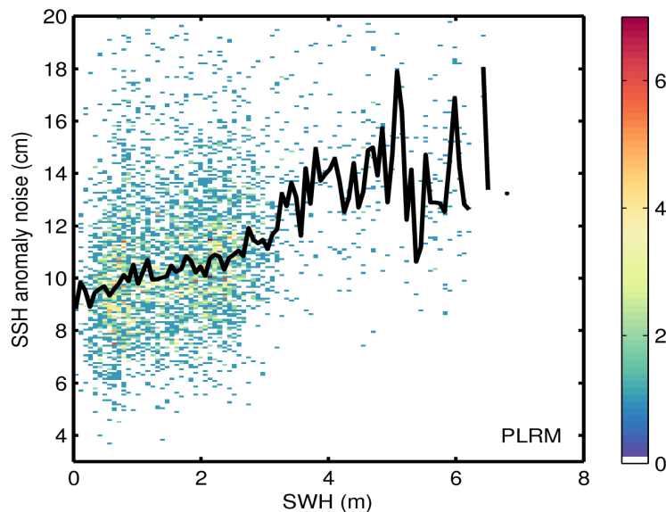
Figure 9. 2D histogram showing flag-valid SSH anomaly noise as a function of SWH for LRM (top) and PLRM (bottom) for 06/08/2016. The black line denotes the median SSH anomaly noise as a function of SWH.
