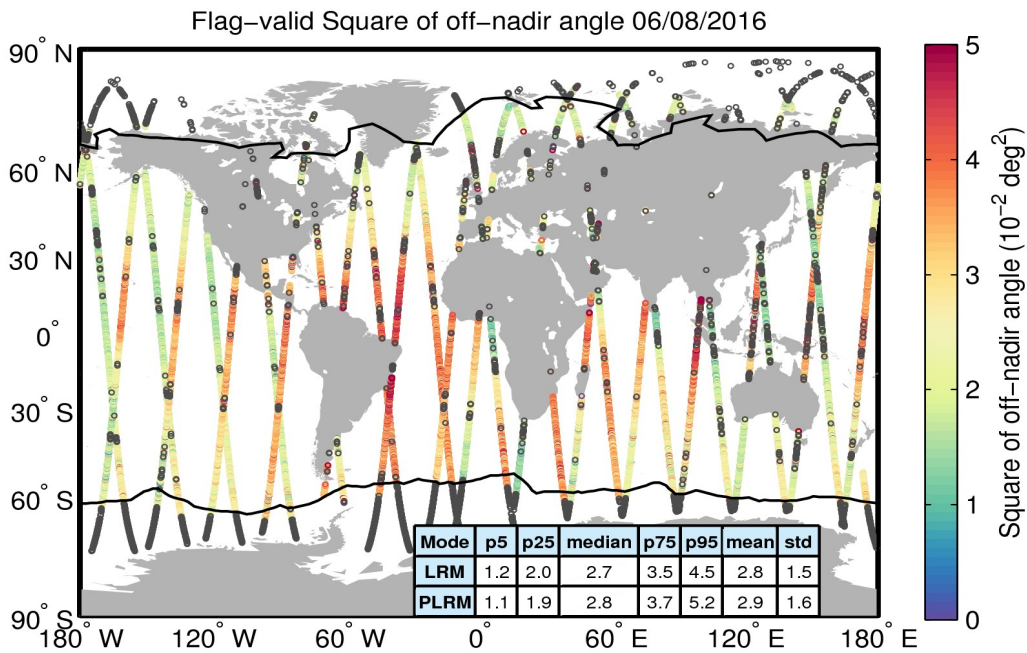
Figure 37. Geographical distribution of flag-valid mispointing data over oceans and lakes for 06/08/2016. The statistical values shown in the table refer to the mispointing in 10^{-2} \text{ deg}^2 and are calculated separately for LRM and PLRM regions. Measurements taken over polar polygons have been excluded from the computation of the statistical values. The black lines mark the outer limit of the Arctic and Antarctic polar polygons. Gray circles denote negative values.
