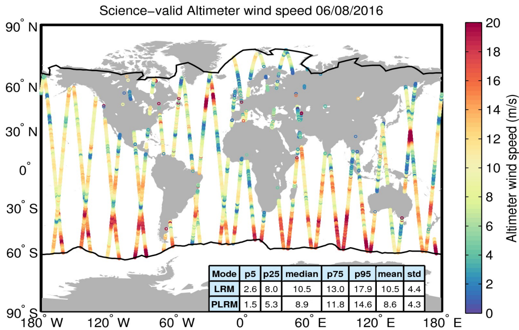
Figure 34. Geographical distribution of science-valid wind data over oceans and lakes for 06/08/2016. The statistical values shown in the table refer to the wind in m/s and are calculated separately for LRM and PLRM regions. The black lines mark the outer limit of the Arctic and Antarctic polar polygons. Gray circles denote records that have been rejected based on the editing criteria described in Table 5.
