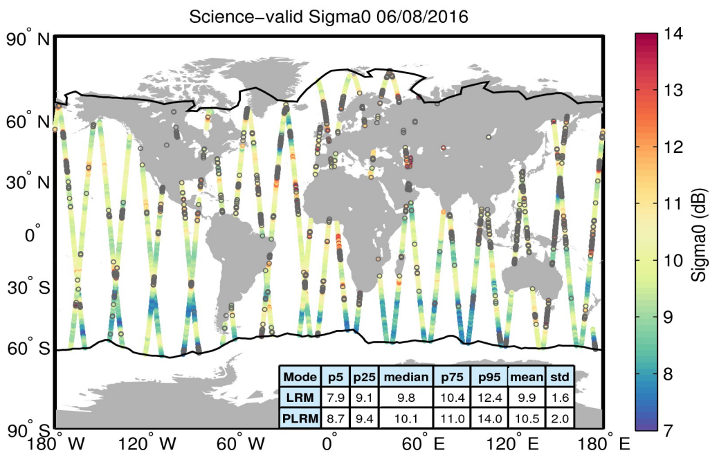
Figure 27. Geographical distribution of science-valid sigma0 data over oceans and lakes for 06/08/2016. The statistical values shown in the table refer to the sigma0 in dB and are calculated separately for LRM and PLRM regions. The black lines mark the outer limit of the Arctic and Antarctic polar polygons. Gray circles denote records that have been rejected based on the editing criteria described in Table 4.
