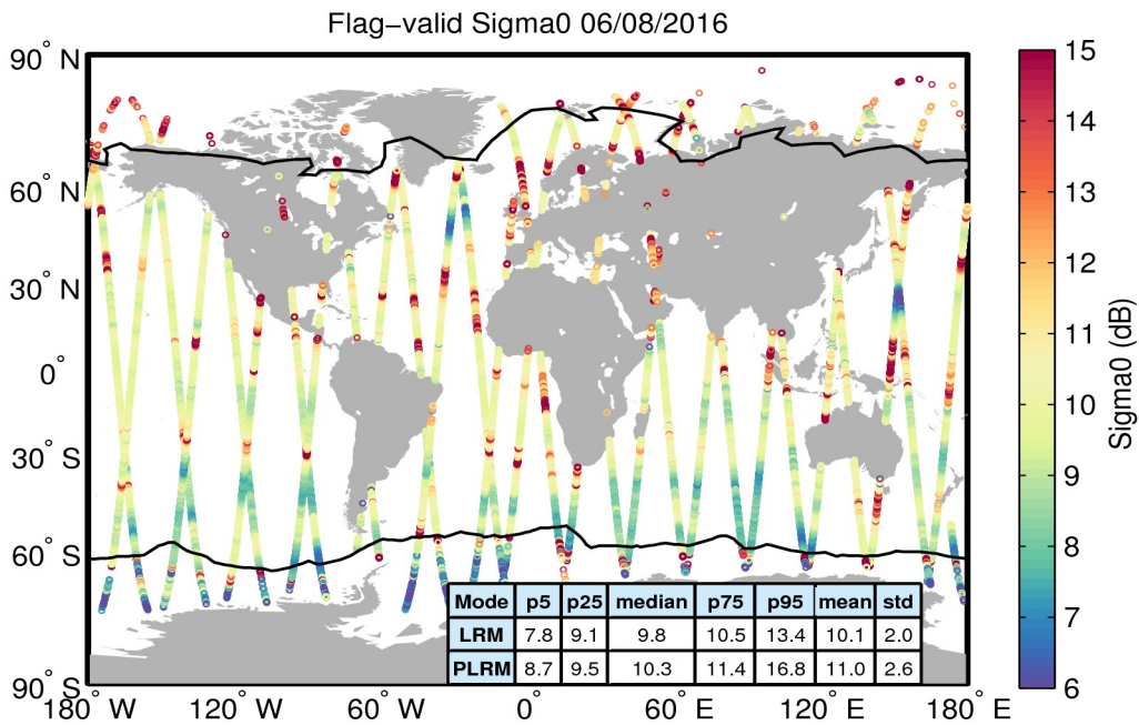
Figure 23. Geographical distribution of flag-valid sigma0 data over oceans and lakes for 06/08/2016. The statistical values shown in the table refer to the sigma0 in dB and are calculated separately for LRM and PLRM regions. Measurements taken over polar polygons have been excluded from the computation of the statistical values. The black lines mark the outer limit of the Arctic and Antarctic polar polygons.
