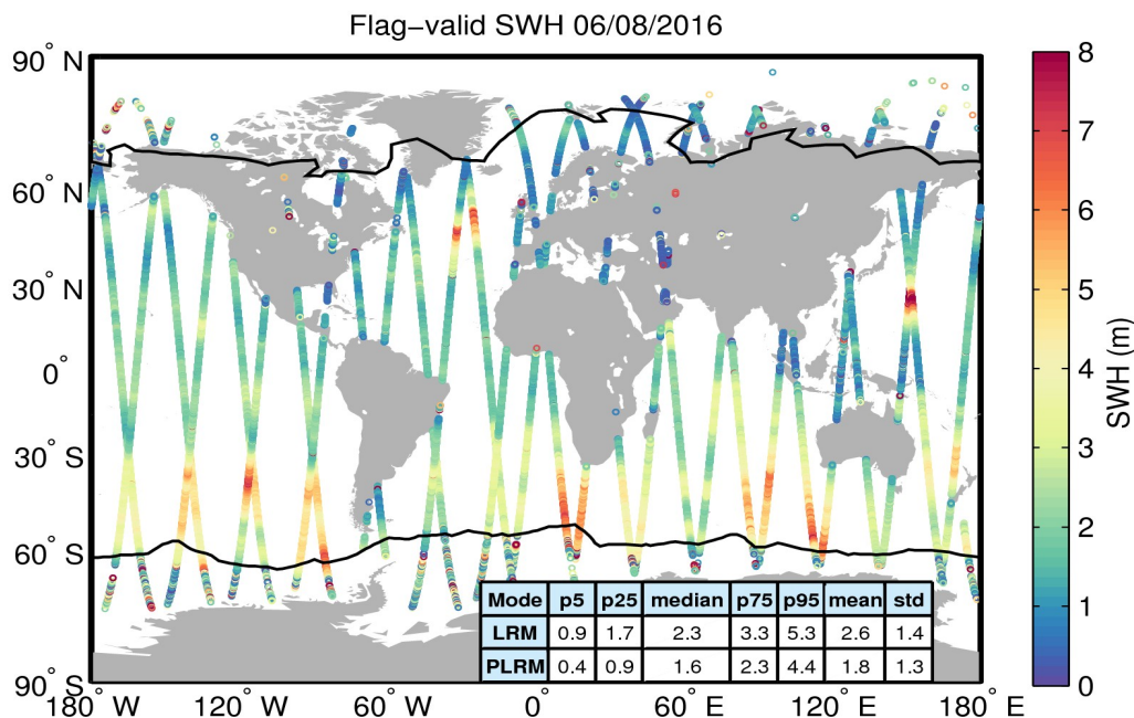
Figure 15. Geographical distribution of flag-valid SWH data over oceans and lakes for 06/08/2016. The statistical values shown in the table refer to the SWH in m and are calculated separately for LRM and PLRM regions. Measurements taken over polar polygons have been excluded from the computation of the statistical values. The black lines mark the outer limit of the Arctic and Antarctic polar polygons.
