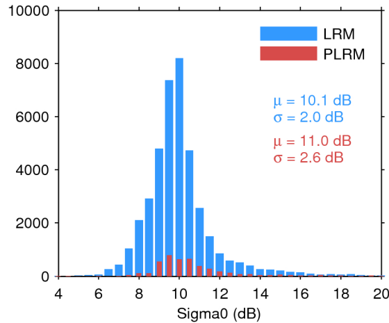
Figure 25. Histogram of flag-valid sigma0 over oceans and lakes for LRM (blue) and PLRM (red) for 06/08/2016. The mean ( \mu ) and standard deviation ( \sigma ) are also shown. Note that values outside [4 20] dB are excluded from the histogram for the sake of readability but not from the computation of \mu and \sigma .
