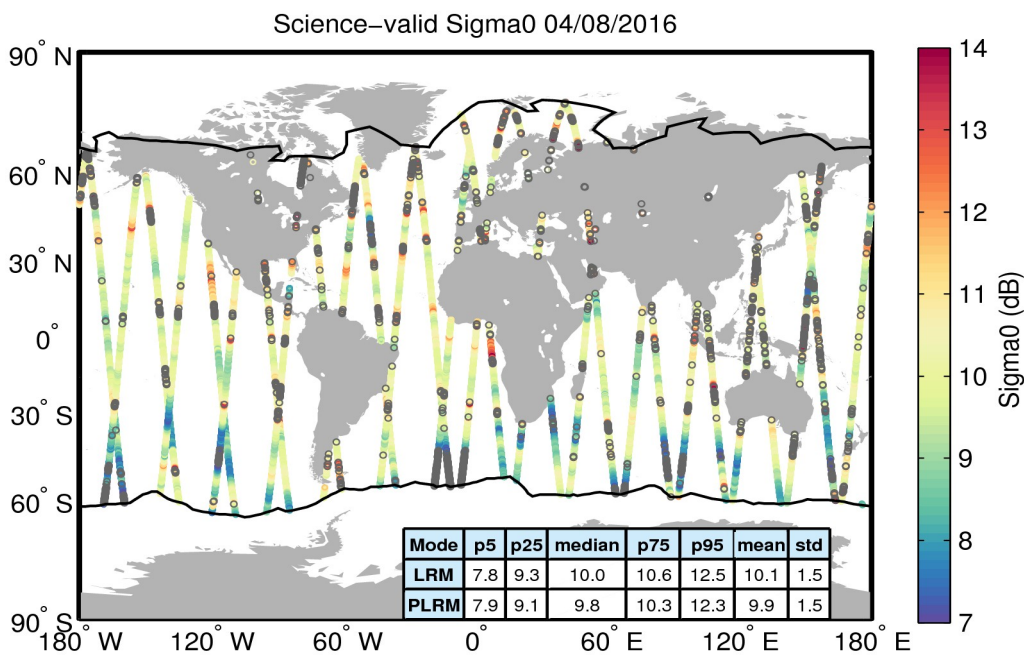
Figure 27. Geographical distribution of science-valid sigma0 data over oceans and lakes for 04/08/2016. The statistical values shown in the table refer to the sigma0 in dB and are calculated separately for LRM and PLRM regions. The black lines mark the outer limit of the Arctic and Antarctic polar polygons. Gray circles denote records that have been rejected based on the editing criteria described in Table 4.
