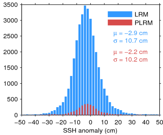
Figure 11. Histogram of science-valid SSH anomaly over oceans and lakes for LRM (blue) and PLRM (red) for 04/08/2016. The mean ( \mu ) and standard deviation ( \sigma ) are also shown. Note that values outside [-50\ 50] cm are excluded from the histogram for the sake of readability but not from the computation of \mu and \sigma .
