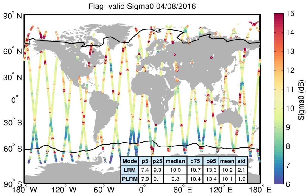
Figure 23. Geographical distribution of flag-valid sigma0 data over oceans and lakes for 04/08/2016. The statistical values shown in the table refer to the sigma0 in dB and are calculated separately for LRM and PLRM regions. Measurements taken over polar polygons have been excluded from the computation of the statistical values. The black lines mark the outer limit of the Arctic and Antarctic polar polygons.
