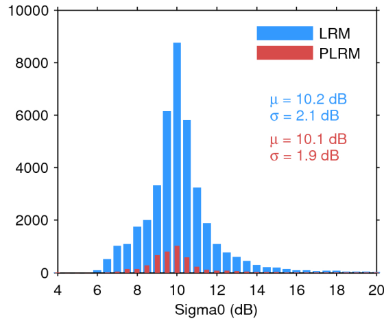
Figure 25. Histogram of flag-valid sigma0 over oceans and lakes for LRM (blue) and PLRM (red) for 04/08/2016. The mean ( \mu ) and standard deviation ( \sigma ) are also shown. Note that values outside [4 20] dB are excluded from the histogram for the sake of readability but not from the computation of \mu and \sigma .
