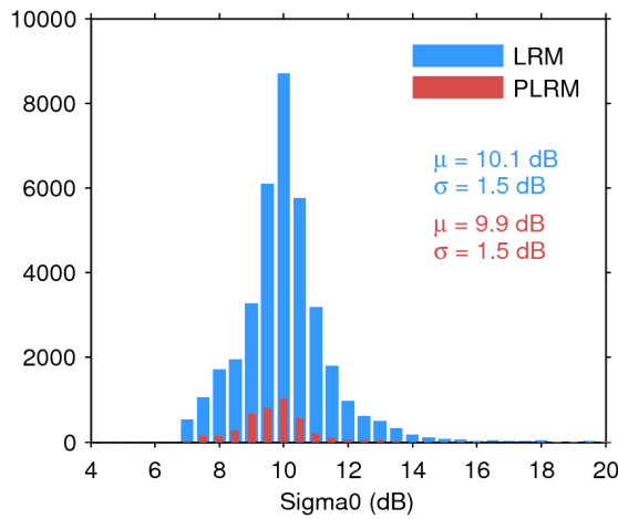
Figure 28. Histogram of science-valid sigma0 over oceans and lakes for LRM (blue) and PLRM (red) for 04/08/2016. The mean ( \mu ) and standard deviation ( \sigma ) are also shown. Note that values outside [4 20] dB are excluded from the histogram for the sake of readability but not from the computation of \mu and \sigma .
