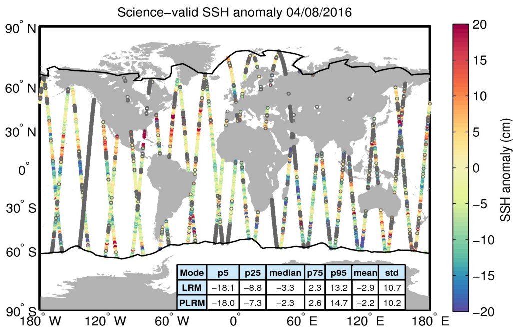
Figure 10. Geographical distribution of science-valid SSH anomaly data over oceans and lakes for 04/08/2016. The statistical values shown in the table refer to the SSH anomaly in cm and are calculated separately for LRM and PLRM regions. The black lines mark the outer limit of the Arctic and Antarctic polar polygons. Gray circles denote records that have been rejected based on the editing criteria described in Table 2.
