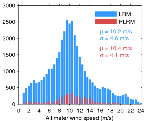
Figure 33. Histogram of flag-valid wind over oceans and lakes for LRM (blue) and PLRM (red) for 04/08/2016. The mean ( \mu ) and standard deviation ( \sigma ) are also shown. Note that values larger than 24 m/s are excluded from the histogram for the sake of readability but not from the computation of \mu and \sigma .
