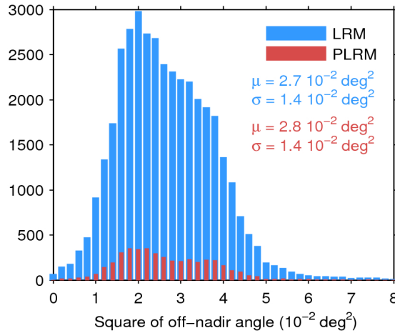
Figure 39. Histogram of flag-valid mispointing over oceans and lakes for LRM (blue) and PLRM (red) for 04/08/2016. Only positive values have been considered. The mean ( \mu ) and standard deviation ( \sigma ) are also shown. Note that values larger than 8 \cdot 10^{-2} \text{ deg}^2 are excluded from the histogram for the sake of readability but not from the computation of \mu and \sigma .
