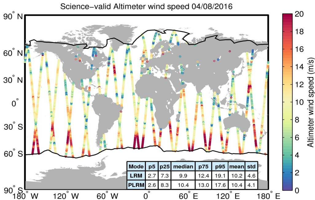
Figure 34. Geographical distribution of science-valid wind data over oceans and lakes for 04/08/2016. The statistical values shown in the table refer to the wind in m/s and are calculated separately for LRM and PLRM regions. The black lines mark the outer limit of the Arctic and Antarctic polar polygons. Gray circles denote records that have been rejected based on the editing criteria described in Table 5.
