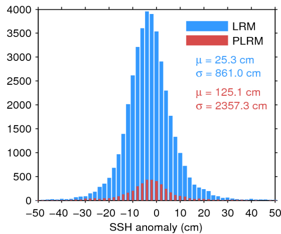
Figure 7. Histogram of flag-valid SSH anomaly over oceans and lakes for LRM (blue) and PLRM (red) for 04/08/2016. The mean ( \mu ) and standard deviation ( \sigma ) are also shown. Note that values outside [-50\ 50] cm are excluded from the histogram for the sake of readability but not from the computation of \mu and \sigma .
