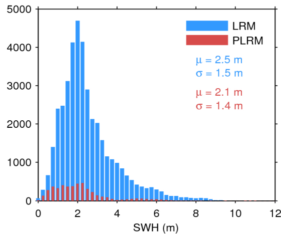
Figure 17. Histogram of flag-valid SWH over oceans and lakes for LRM (blue) and PLRM (red) for 04/08/2016. The mean ( \mu ) and standard deviation ( \sigma ) are also shown. Note that values larger than 12 m are excluded from the histogram for the sake of readability but not from the computation of \mu and \sigma .
