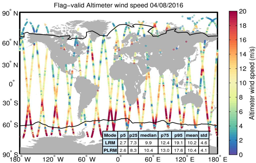
Figure 31. Geographical distribution of flag-valid wind data over oceans and lakes for 04/08/2016. The statistical values shown in the table refer to the wind in m/s and are calculated separately for LRM and PLRM regions. Measurements taken over polar polygons have been excluded from the computation of the statistical values. The black lines mark the outer limit of the Arctic and Antarctic polar polygons.
