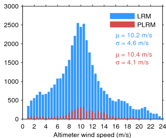
Figure 35. Histogram of science-valid wind over oceans and lakes for LRM (blue) and PLRM (red) for 04/08/2016. The mean ( \mu ) and standard deviation ( \sigma ) are also shown. Note that values larger than 24 m/s are excluded from the histogram for the sake of readability but not from the computation of \mu and \sigma .
