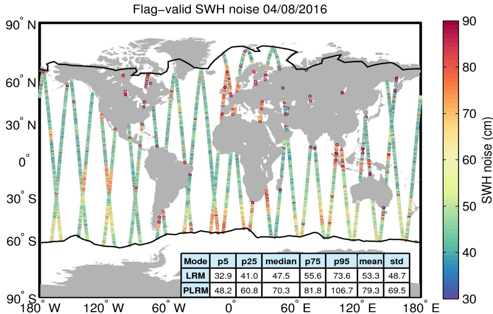
Figure 18. Geographical distribution of flag-valid 20-Hz SWH measurement noise over oceans and lakes for 04/08/2016. The statistical values shown in the table refer to the SWH noise and are calculated separately for LRM and PLRM regions. Measurements taken over polar polygons have been excluded from the computation of the statistical values. The black lines mark the outer limit of the Arctic and Antarctic polar polygons.
