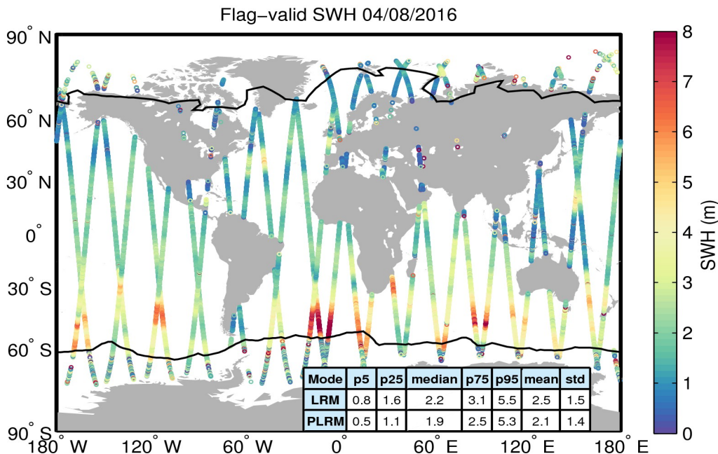
Figure 15. Geographical distribution of flag-valid SWH data over oceans and lakes for 04/08/2016. The statistical values shown in the table refer to the SWH in m and are calculated separately for LRM and PLRM regions. Measurements taken over polar polygons have been excluded from the computation of the statistical values. The black lines mark the outer limit of the Arctic and Antarctic polar polygons.
