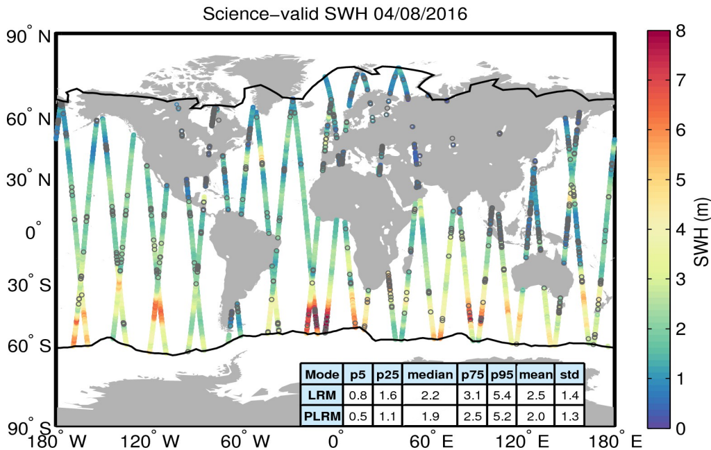
Figure 19. Geographical distribution of science-valid SWH data over oceans and lakes for 04/08/2016. The statistical values shown in the table refer to the SWH in m and are calculated separately for LRM and PLRM regions. The black lines mark the outer limit of the Arctic and Antarctic polar polygons. Gray circles denote records that have been rejected based on the editing criteria described in Table 3.
