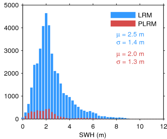
Figure 20. Histogram of science-valid SWH over oceans and lakes for LRM (blue) and PLRM (red) for 04/08/2016. The mean ( \mu ) and standard deviation ( \sigma ) are also shown. Note that values larger than 12 m are excluded from the histogram for the sake of readability but not from the computation of \mu and \sigma .
