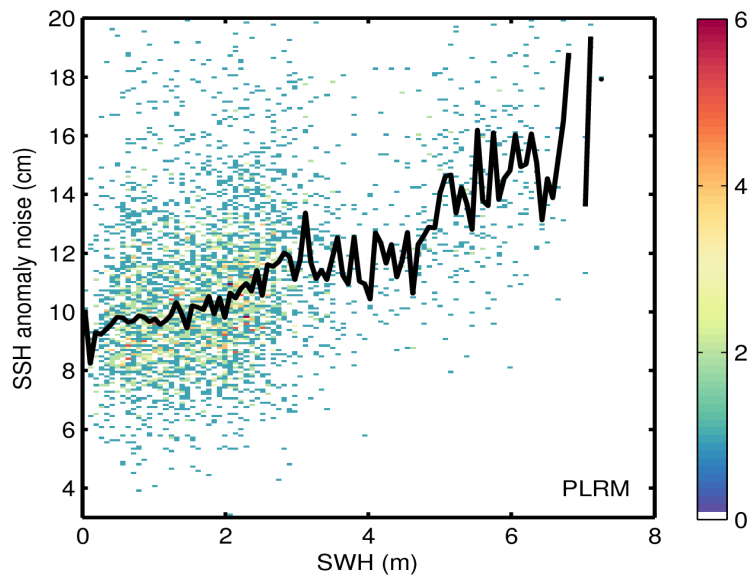
Figure 9. 2D histogram showing flag-valid SSH anomaly noise as a function of SWH for LRM (top) and PLRM (bottom) for 04/08/2016. The black line denotes the median SSH anomaly noise as a function of SWH.
