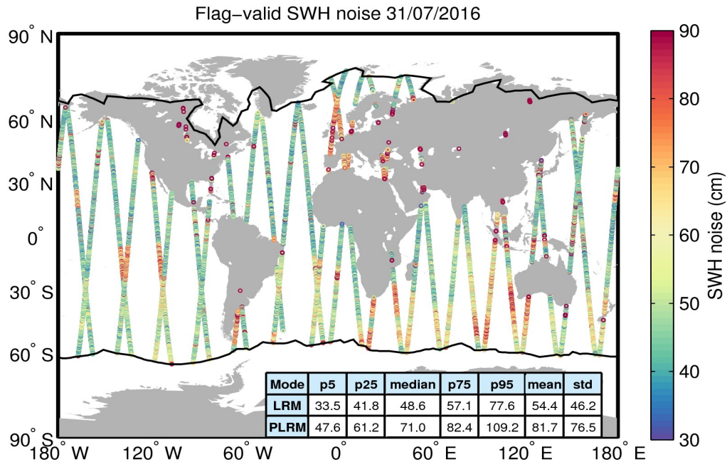
Figure 18. Geographical distribution of flag-valid 20-Hz SWH measurement noise over oceans and lakes for 31/07/2016. The statistical values shown in the table refer to the SWH noise and are calculated separately for LRM and PLRM regions. Measurements taken over polar polygons have been excluded from the computation of the statistical values. The black lines mark the outer limit of the Arctic and Antarctic polar polygons.
