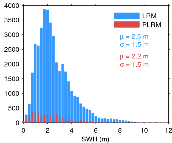
Figure 17. Histogram of flag-valid SWH over oceans and lakes for LRM (blue) and PLRM (red) for 31/07/2016. The mean ( \mu ) and standard deviation ( \sigma ) are also shown. Note that values larger than 12 m are excluded from the histogram for the sake of readability but not from the computation of \mu and \sigma .
