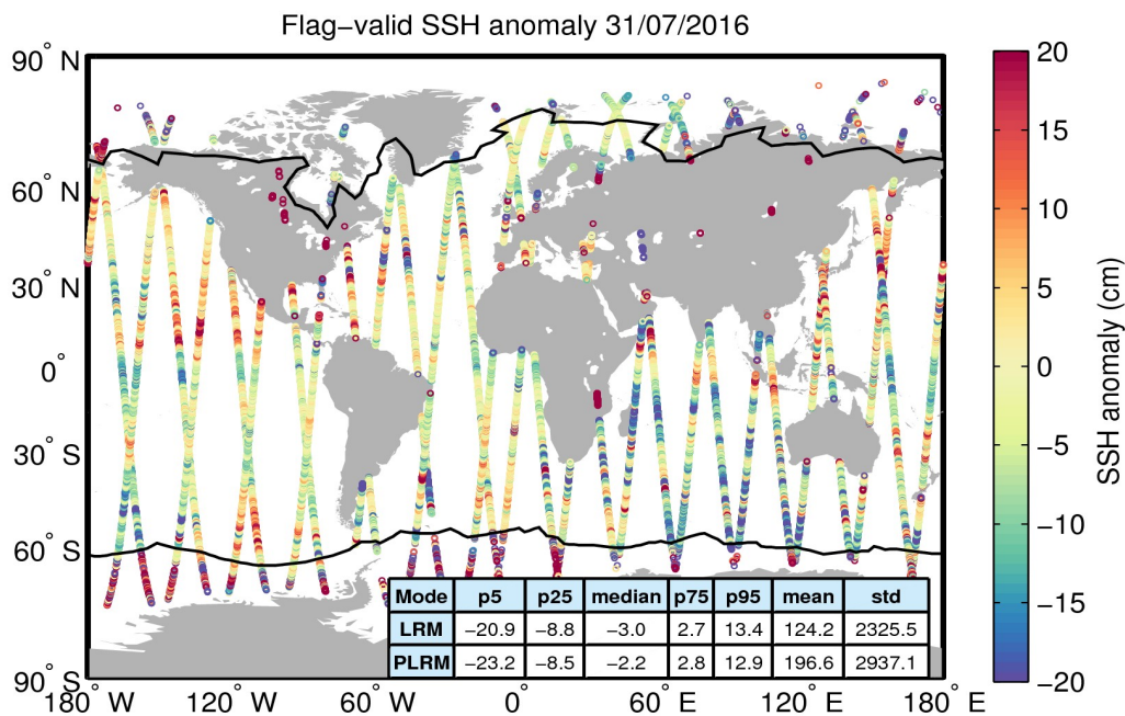
Figure 5. Geographical distribution of flag-valid 1-Hz SSH anomaly data over oceans and lakes for 31/07/2016. The statistical values shown in the table refer to the SSH anomaly in cm and are calculated separately for LRM and PLRM regions. Measurements taken over polar polygons have been excluded from the computation of the statistical values. The black lines mark the outer limit of the Arctic and Antarctic polar polygons.
