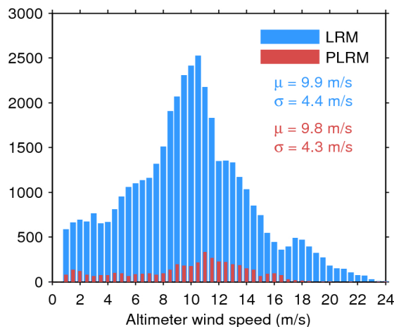
Figure 35. Histogram of science-valid wind over oceans and lakes for LRM (blue) and PLRM (red) for 31/07/2016. The mean ( \mu ) and standard deviation ( \sigma ) are also shown. Note that values larger than 24 m/s are excluded from the histogram for the sake of readability but not from the computation of \mu and \sigma .
