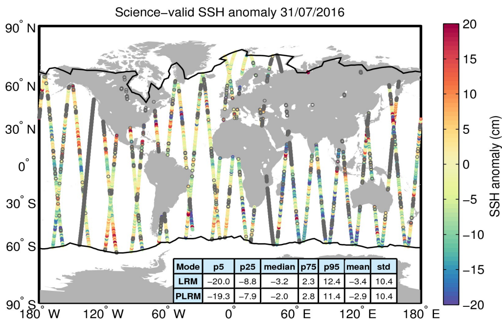
Figure 10. Geographical distribution of science-valid SSH anomaly data over oceans and lakes for 31/07/2016. The statistical values shown in the table refer to the SSH anomaly in cm and are calculated separately for LRM and PLRM regions. The black lines mark the outer limit of the Arctic and Antarctic polar polygons. Gray circles denote records that have been rejected based on the editing criteria described in Table 2.
