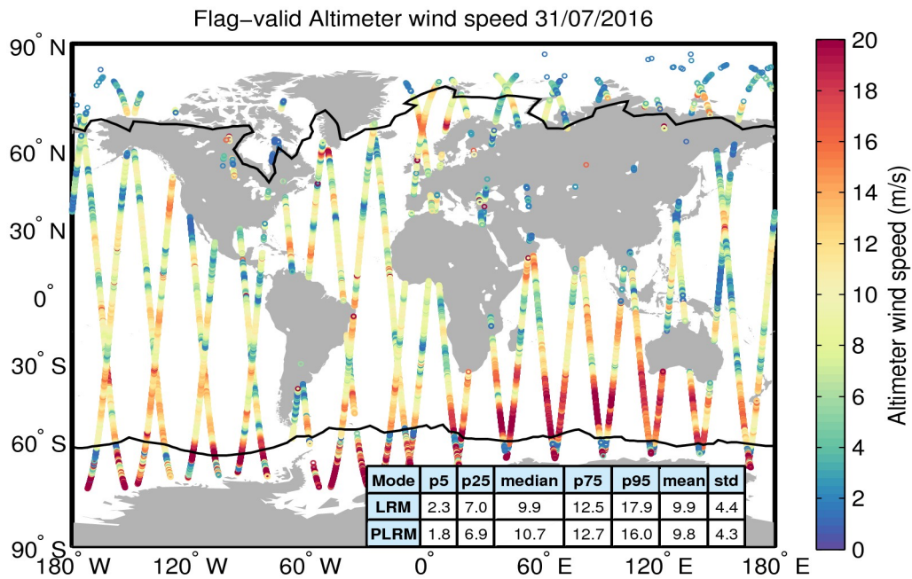
Figure 31. Geographical distribution of flag-valid wind data over oceans and lakes for 31/07/2016. The statistical values shown in the table refer to the wind in m/s and are calculated separately for LRM and PLRM regions. Measurements taken over polar polygons have been excluded from the computation of the statistical values. The black lines mark the outer limit of the Arctic and Antarctic polar polygons.
