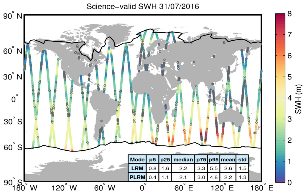
Figure 19. Geographical distribution of science-valid SWH data over oceans and lakes for 31/07/2016. The statistical values shown in the table refer to the SWH in m and are calculated separately for LRM and PLRM regions. The black lines mark the outer limit of the Arctic and Antarctic polar polygons. Gray circles denote records that have been rejected based on the editing criteria described in Table 3.
