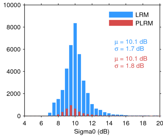
Figure 28. Histogram of science-valid sigma0 over oceans and lakes for LRM (blue) and PLRM (red) for 31/07/2016. The mean ( \mu ) and standard deviation ( \sigma ) are also shown. Note that values outside [4 20] dB are excluded from the histogram for the sake of readability but not from the computation of \mu and \sigma .
