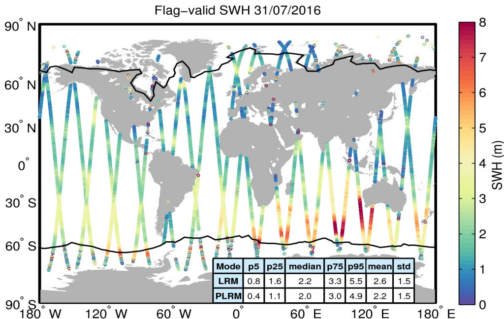
Figure 15. Geographical distribution of flag-valid SWH data over oceans and lakes for 31/07/2016. The statistical values shown in the table refer to the SWH in m and are calculated separately for LRM and PLRM regions. Measurements taken over polar polygons have been excluded from the computation of the statistical values. The black lines mark the outer limit of the Arctic and Antarctic polar polygons.
