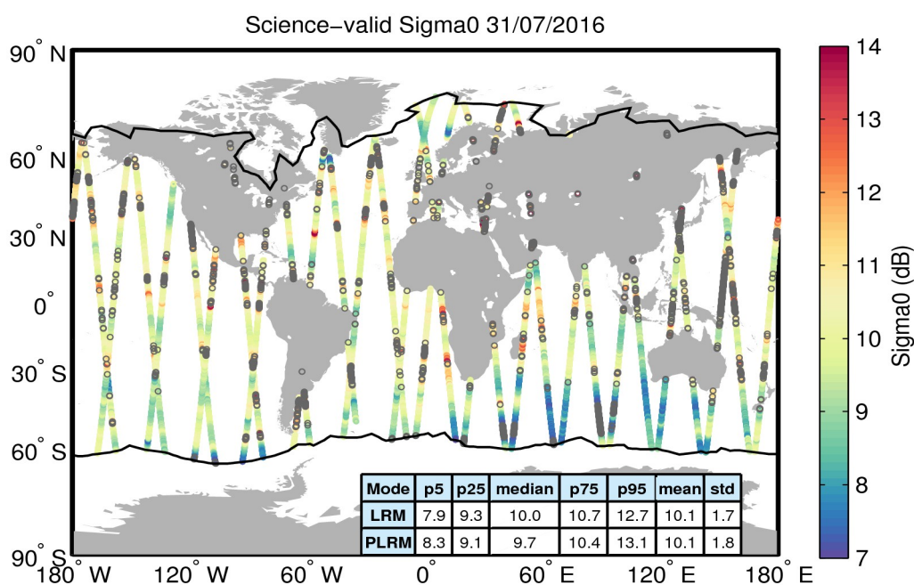
Figure 27. Geographical distribution of science-valid sigma0 data over oceans and lakes for 31/07/2016. The statistical values shown in the table refer to the sigma0 in dB and are calculated separately for LRM and PLRM regions. The black lines mark the outer limit of the Arctic and Antarctic polar polygons. Gray circles denote records that have been rejected based on the editing criteria described in Table 4.
