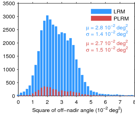
Figure 39. Histogram of flag-valid mispointing over oceans and lakes for LRM (blue) and PLRM (red) for 31/07/2016. Only positive values have been considered. The mean ( \mu ) and standard deviation ( \sigma ) are also shown. Note that values larger than 8 \cdot 10^{-2} \text{ deg}^2 are excluded from the histogram for the sake of readability but not from the computation of \mu and \sigma .
