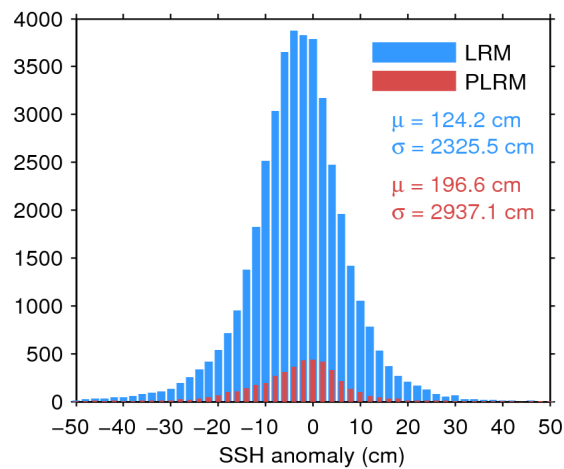
Figure 7. Histogram of flag-valid SSH anomaly over oceans and lakes for LRM (blue) and PLRM (red) for 31/07/2016. The mean ( \mu ) and standard deviation ( \sigma ) are also shown. Note that values outside [-50 50] cm are excluded from the histogram for the sake of readability but not from the computation of \mu and \sigma .
