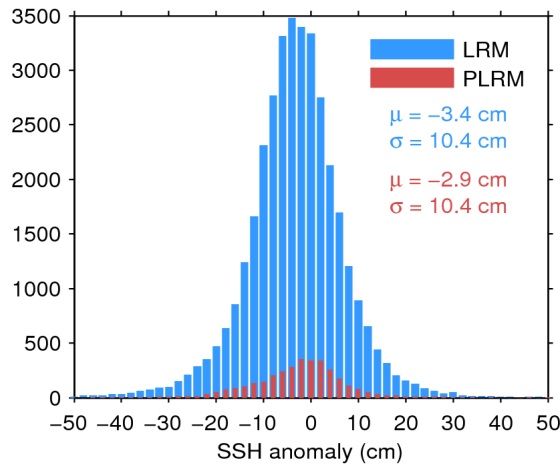
Figure 11. Histogram of science-valid SSH anomaly over oceans and lakes for LRM (blue) and PLRM (red) for 31/07/2016. The mean ( \mu ) and standard deviation ( \sigma ) are also shown. Note that values outside [-50\ 50] cm are excluded from the histogram for the sake of readability but not from the computation of \mu and \sigma .
