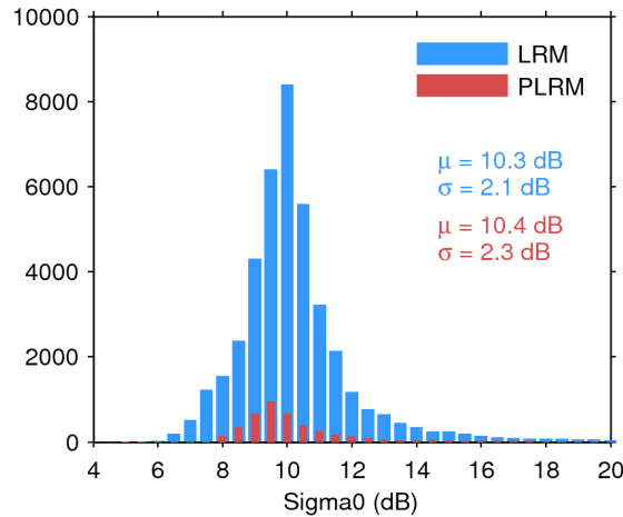
Figure 25. Histogram of flag-valid sigma0 over oceans and lakes for LRM (blue) and PLRM (red) for 31/07/2016. The mean ( \mu ) and standard deviation ( \sigma ) are also shown. Note that values outside [4 20] dB are excluded from the histogram for the sake of readability but not from the computation of \mu and \sigma .
