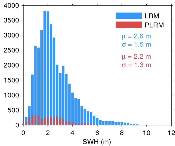
Figure 20. Histogram of science-valid SWH over oceans and lakes for LRM (blue) and PLRM (red) for 31/07/2016. The mean ( \mu ) and standard deviation ( \sigma ) are also shown. Note that values larger than 12 m are excluded from the histogram for the sake of readability but not from the computation of \mu and \sigma .
