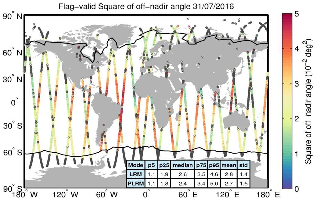
Figure 37. Geographical distribution of flag-valid mispointing data over oceans and lakes for 31/07/2016. The statistical values shown in the table refer to the mispointing in 10^{-2} deg 2 and are calculated separately for LRM and PLRM regions. Measurements taken over polar polygons have been excluded from the computation of the statistical values. The black lines mark the outer limit of the Arctic and Antarctic polar polygons. Gray circles denote negative values.
