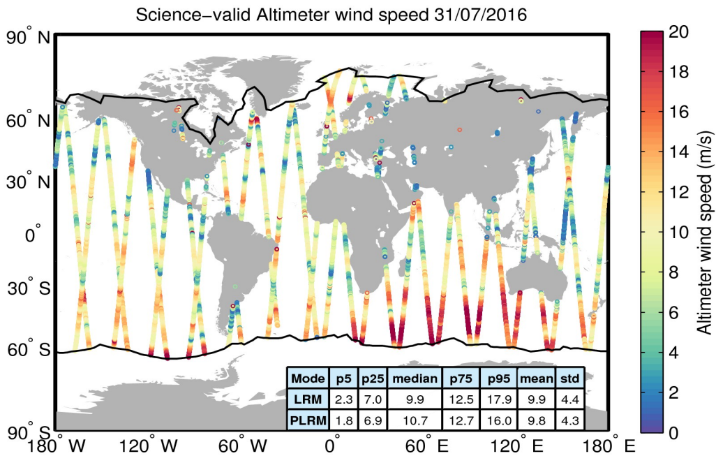
Figure 34. Geographical distribution of science-valid wind data over oceans and lakes for 31/07/2016. The statistical values shown in the table refer to the wind in m/s and are calculated separately for LRM and PLRM regions. The black lines mark the outer limit of the Arctic and Antarctic polar polygons. Gray circles denote records that have been rejected based on the editing criteria described in Table 5.
