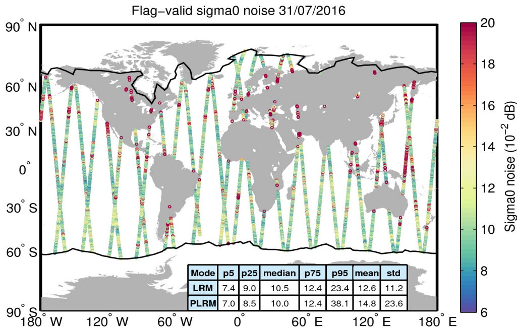
Figure 26. Geographical distribution of flag-valid 20-Hz sigma0 measurement noise over oceans and lakes for 31/07/2016. The statistical values shown in the table refer to the sigma0 noise and are calculated separately for LRM and PLRM regions. Measurements taken over polar polygons have been excluded from the computation of the statistical values. The black lines mark the outer limit of the Arctic and Antarctic polar polygons.
