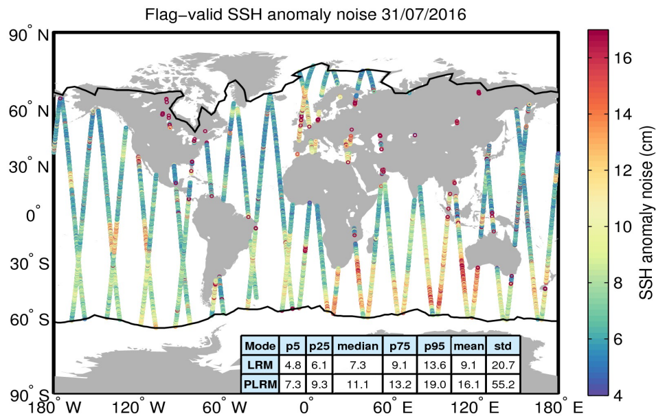
Figure 8. Geographical distribution of flag-valid 20-Hz SSH anomaly measurement noise over oceans and lakes for 31/07/2016. The statistical values shown in the table refer to the SSH anomaly noise and are calculated separately for LRM and PLRM regions. Measurements taken over polar polygons have been excluded from the computation of the statistical values. The black lines mark the outer limit of the Arctic and Antarctic polar polygons.
