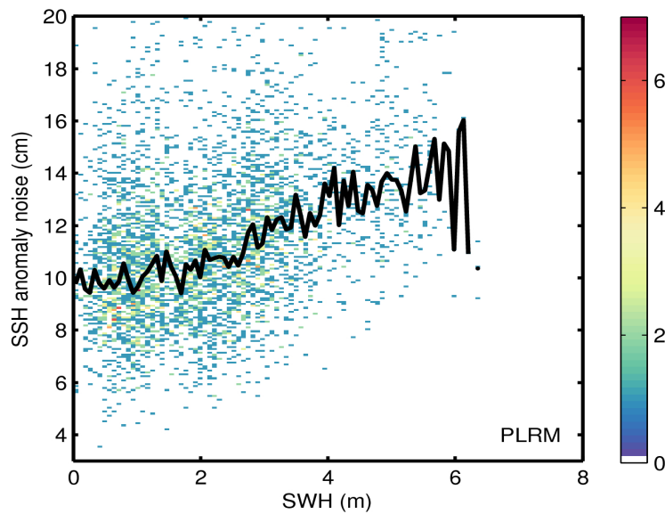
Figure 9. 2D histogram showing flag-valid SSH anomaly noise as a function of SWH for LRM (top) and PLRM (bottom) for 31/07/2016. The black line denotes the median SSH anomaly noise as a function of SWH.
