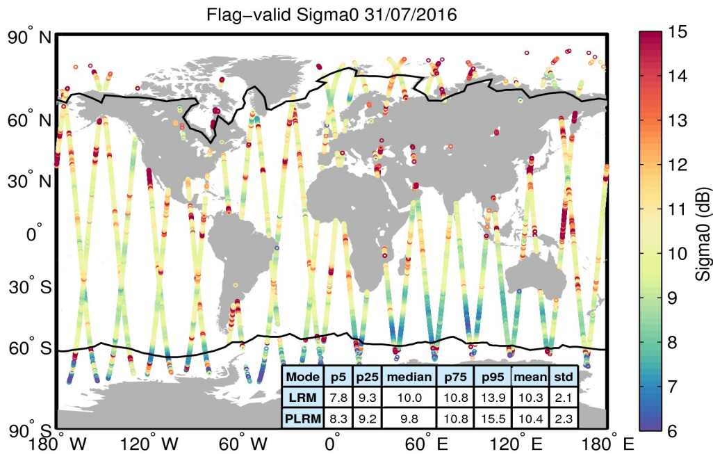
Figure 23. Geographical distribution of flag-valid sigma0 data over oceans and lakes for 31/07/2016. The statistical values shown in the table refer to the sigma0 in dB and are calculated separately for LRM and PLRM regions. Measurements taken over polar polygons have been excluded from the computation of the statistical values. The black lines mark the outer limit of the Arctic and Antarctic polar polygons.
