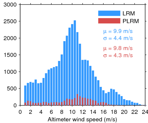
Figure 33. Histogram of flag-valid wind over oceans and lakes for LRM (blue) and PLRM (red) for 31/07/2016. The mean ( \mu ) and standard deviation ( \sigma ) are also shown. Note that values larger than 24 m/s are excluded from the histogram for the sake of readability but not from the computation of \mu and \sigma .
