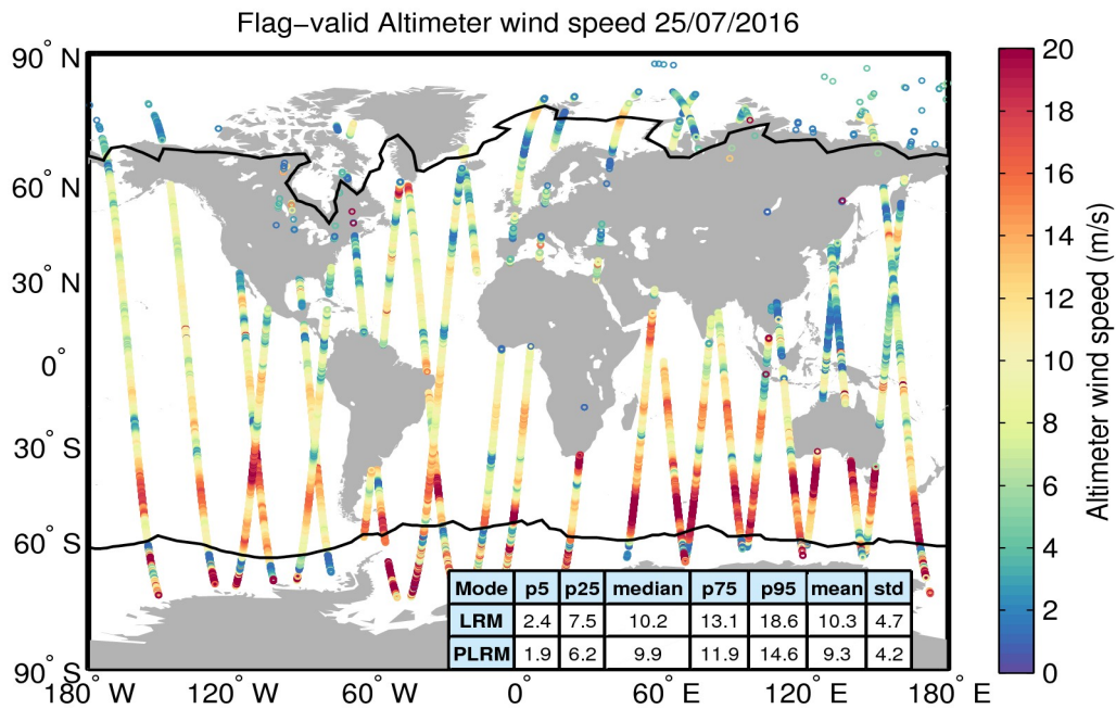
Figure 31. Geographical distribution of flag-valid wind data over oceans and lakes for 25/07/2016. The statistical values shown in the table refer to the wind in m/s and are calculated separately for LRM and PLRM regions. Measurements taken over polar polygons have been excluded from the computation of the statistical values. The black lines mark the outer limit of the Arctic and Antarctic polar polygons.
