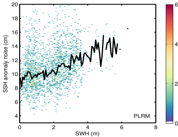
Figure 9. 2D histogram showing flag-valid SSH anomaly noise as a function of SWH for LRM (top) and PLRM (bottom) for 25/07/2016. The black line denotes the median SSH anomaly noise as a function of SWH.
