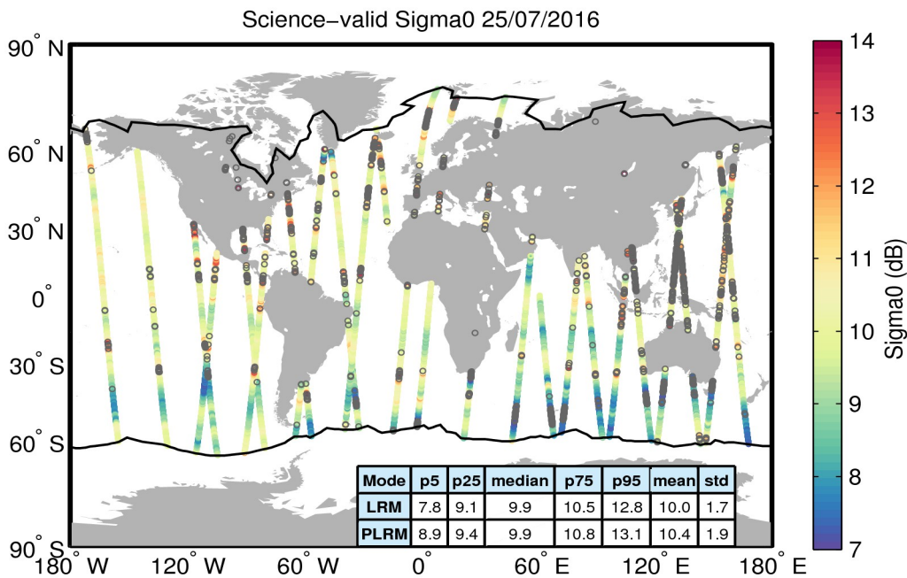
Figure 27. Geographical distribution of science-valid sigma0 data over oceans and lakes for 25/07/2016. The statistical values shown in the table refer to the sigma0 in dB and are calculated separately for LRM and PLRM regions. The black lines mark the outer limit of the Arctic and Antarctic polar polygons. Gray circles denote records that have been rejected based on the editing criteria described in Table 4.
