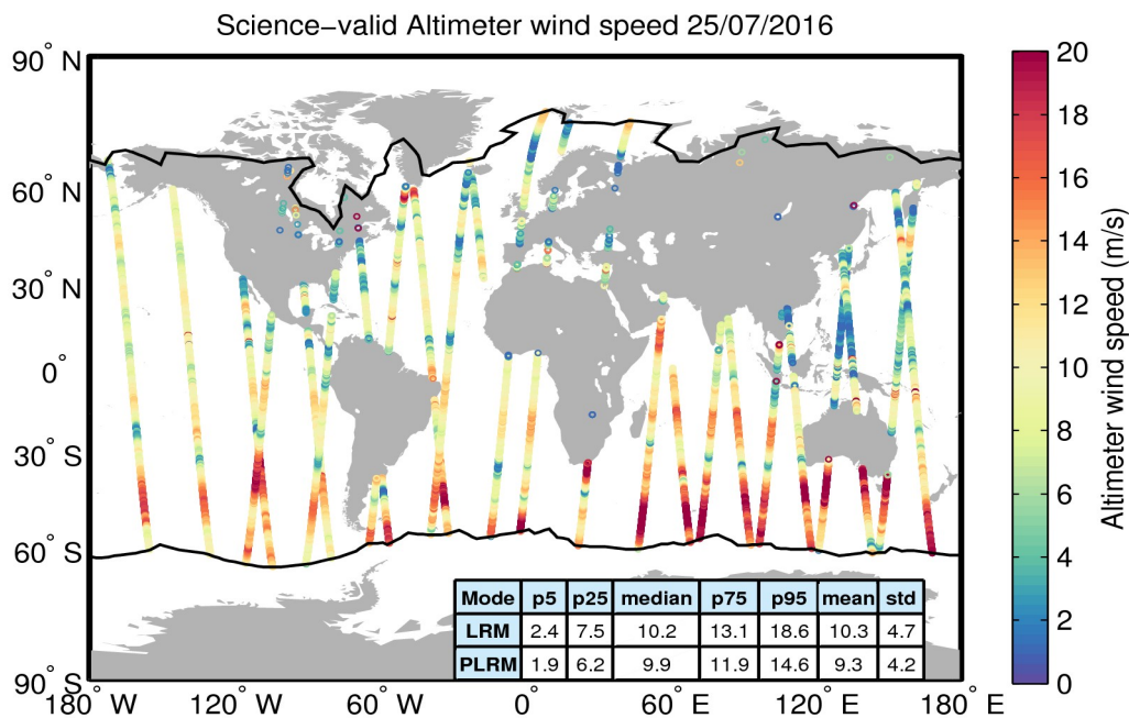
Figure 34. Geographical distribution of science-valid wind data over oceans and lakes for 25/07/2016. The statistical values shown in the table refer to the wind in m/s and are calculated separately for LRM and PLRM regions. The black lines mark the outer limit of the Arctic and Antarctic polar polygons. Gray circles denote records that have been rejected based on the editing criteria described in Table 5.
