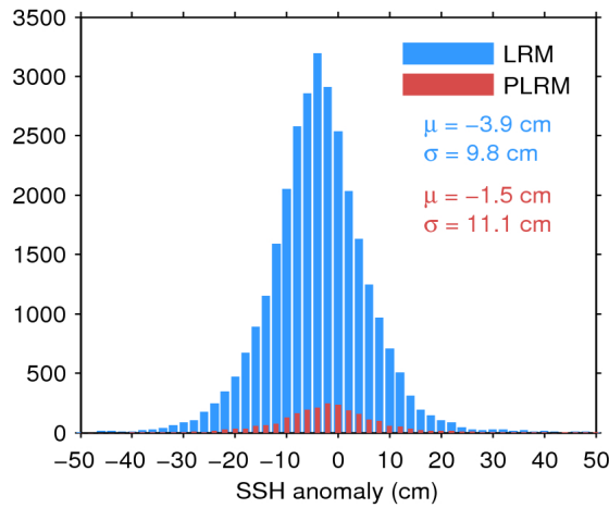
Figure 11. Histogram of science-valid SSH anomaly over oceans and lakes for LRM (blue) and PLRM (red) for 25/07/2016. The mean ( \mu ) and standard deviation ( \sigma ) are also shown. Note that values outside [-50 50] cm are excluded from the histogram for the sake of readability but not from the computation of \mu and \sigma .
