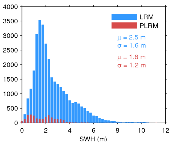
Figure 17. Histogram of flag-valid SWH over oceans and lakes for LRM (blue) and PLRM (red) for 25/07/2016. The mean ( \mu ) and standard deviation ( \sigma ) are also shown. Note that values larger than 12 m are excluded from the histogram for the sake of readability but not from the computation of \mu and \sigma .
