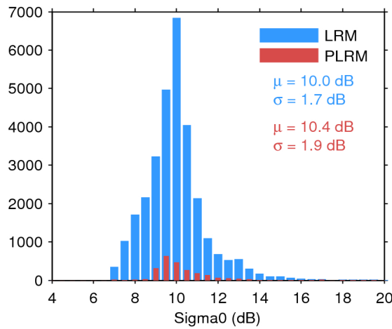
Figure 28. Histogram of science-valid sigma0 over oceans and lakes for LRM (blue) and PLRM (red) for 25/07/2016. The mean ( \mu ) and standard deviation ( \sigma ) are also shown. Note that values outside [4 20] dB are excluded from the histogram for the sake of readability but not from the computation of \mu and \sigma .
