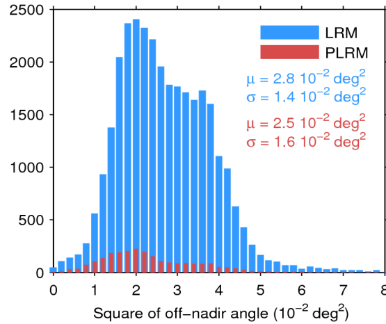
Figure 39. Histogram of flag-valid mispointing over oceans and lakes for LRM (blue) and PLRM (red) for 25/07/2016. Only positive values have been considered. The mean ( \mu ) and standard deviation ( \sigma ) are also shown. Note that values larger than 8 \cdot 10^{-2} \text{ deg}^2 are excluded from the histogram for the sake of readability but not from the computation of \mu and \sigma .
