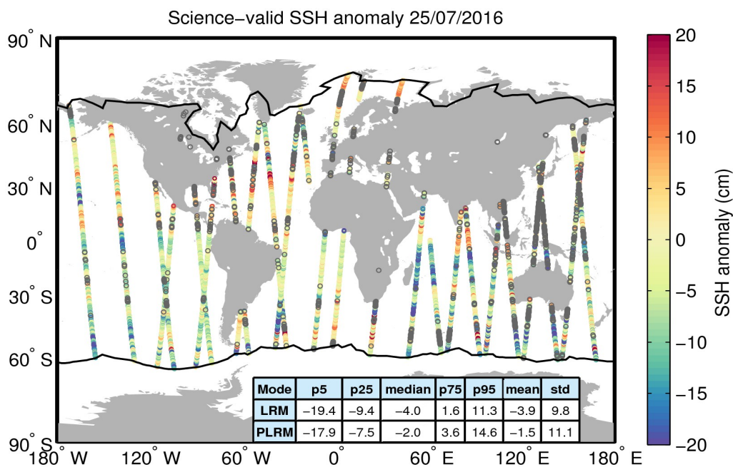
Figure 10. Geographical distribution of science-valid SSH anomaly data over oceans and lakes for 25/07/2016. The statistical values shown in the table refer to the SSH anomaly in cm and are calculated separately for LRM and PLRM regions. The black lines mark the outer limit of the Arctic and Antarctic polar polygons. Gray circles denote records that have been rejected based on the editing criteria described in Table 2.
