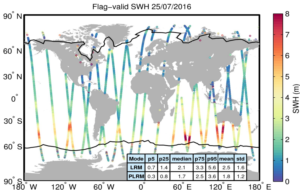
Figure 15. Geographical distribution of flag-valid SWH data over oceans and lakes for 25/07/2016. The statistical values shown in the table refer to the SWH in m and are calculated separately for LRM and PLRM regions. Measurements taken over polar polygons have been excluded from the computation of the statistical values. The black lines mark the outer limit of the Arctic and Antarctic polar polygons.
