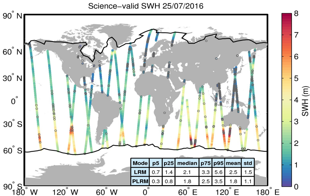
Figure 19. Geographical distribution of science-valid SWH data over oceans and lakes for 25/07/2016. The statistical values shown in the table refer to the SWH in m and are calculated separately for LRM and PLRM regions. The black lines mark the outer limit of the Arctic and Antarctic polar polygons. Gray circles denote records that have been rejected based on the editing criteria described in Table 3.
