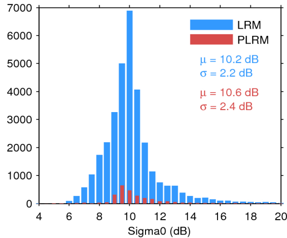
Figure 25. Histogram of flag-valid sigma0 over oceans and lakes for LRM (blue) and PLRM (red) for 25/07/2016. The mean ( \mu ) and standard deviation ( \sigma ) are also shown. Note that values outside [4 20] dB are excluded from the histogram for the sake of readability but not from the computation of \mu and \sigma .
