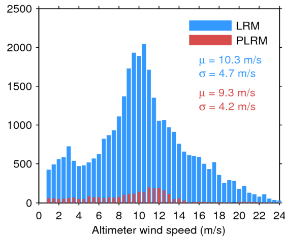
Figure 33. Histogram of flag-valid wind over oceans and lakes for LRM (blue) and PLRM (red) for 25/07/2016. The mean ( \mu ) and standard deviation ( \sigma ) are also shown. Note that values larger than 24 m/s are excluded from the histogram for the sake of readability but not from the computation of \mu and \sigma .
