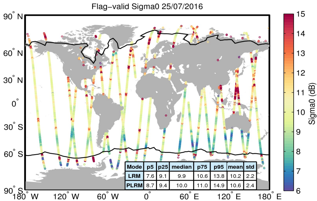
Figure 23. Geographical distribution of flag-valid sigma0 data over oceans and lakes for 25/07/2016. The statistical values shown in the table refer to the sigma0 in dB and are calculated separately for LRM and PLRM regions. Measurements taken over polar polygons have been excluded from the computation of the statistical values. The black lines mark the outer limit of the Arctic and Antarctic polar polygons.
