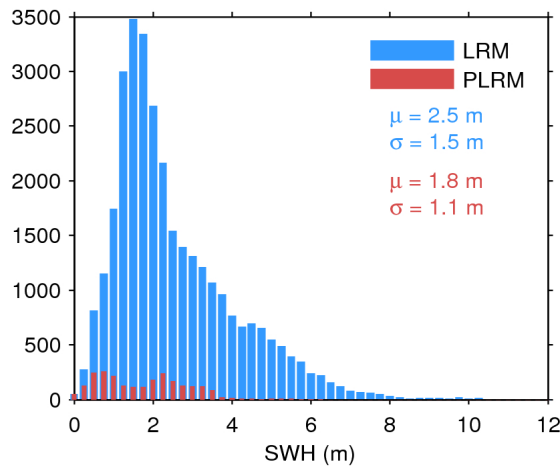
Figure 20. Histogram of science-valid SWH over oceans and lakes for LRM (blue) and PLRM (red) for 25/07/2016. The mean ( \mu ) and standard deviation ( \sigma ) are also shown. Note that values larger than 12 m are excluded from the histogram for the sake of readability but not from the computation of \mu and \sigma .
