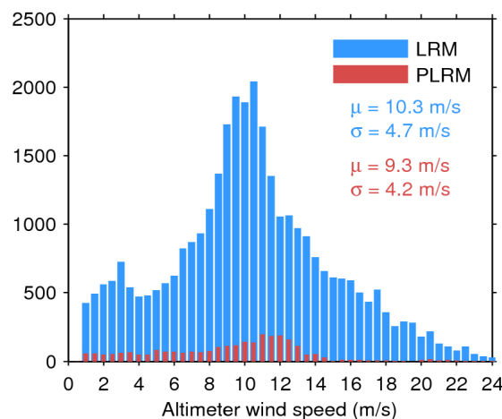
Figure 35. Histogram of science-valid wind over oceans and lakes for LRM (blue) and PLRM (red) for 25/07/2016. The mean ( \mu ) and standard deviation ( \sigma ) are also shown. Note that values larger than 24 m/s are excluded from the histogram for the sake of readability but not from the computation of \mu and \sigma .
