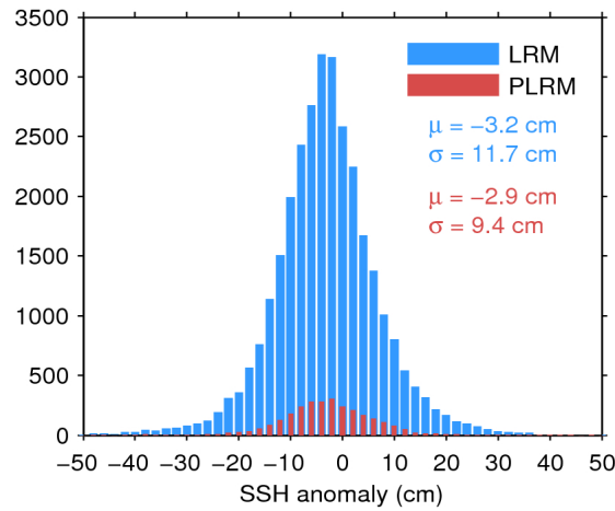
Figure 11. Histogram of science-valid SSH anomaly over oceans and lakes for LRM (blue) and PLRM (red) for 21/07/2016. The mean ( \mu ) and standard deviation ( \sigma ) are also shown. Note that values outside [-50\ 50] cm are excluded from the histogram for the sake of readability but not from the computation of \mu and \sigma .
