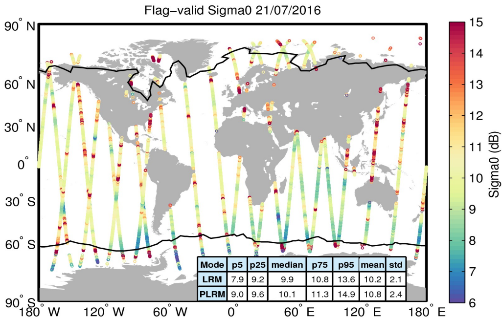
Figure 23. Geographical distribution of flag-valid sigma0 data over oceans and lakes for 21/07/2016. The statistical values shown in the table refer to the sigma0 in dB and are calculated separately for LRM and PLRM regions. Measurements taken over polar polygons have been excluded from the computation of the statistical values. The black lines mark the outer limit of the Arctic and Antarctic polar polygons.
