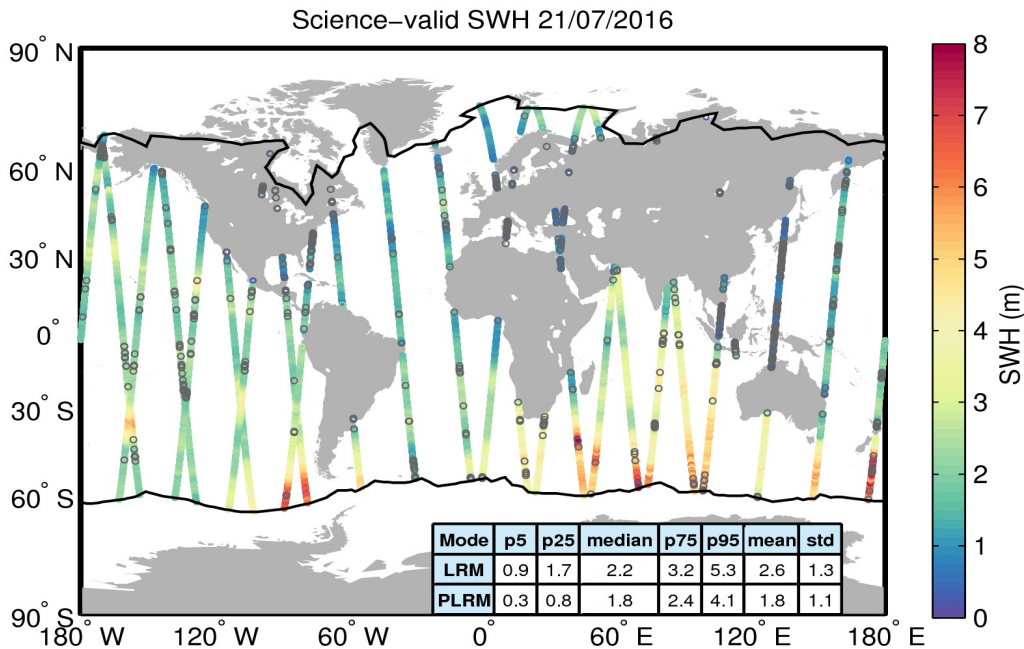
Figure 19. Geographical distribution of science-valid SWH data over oceans and lakes for 21/07/2016. The statistical values shown in the table refer to the SWH in m and are calculated separately for LRM and PLRM regions. The black lines mark the outer limit of the Arctic and Antarctic polar polygons. Gray circles denote records that have been rejected based on the editing criteria described in Table 3.
