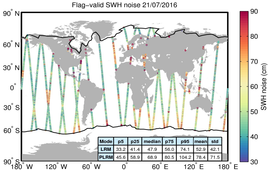
Figure 18. Geographical distribution of flag-valid 20-Hz SWH measurement noise over oceans and lakes for 21/07/2016. The statistical values shown in the table refer to the SWH noise and are calculated separately for LRM and PLRM regions. Measurements taken over polar polygons have been excluded from the computation of the statistical values. The black lines mark the outer limit of the Arctic and Antarctic polar polygons.
