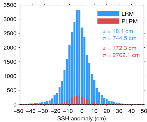
Figure 7. Histogram of flag-valid SSH anomaly over oceans and lakes for LRM (blue) and PLRM (red) for 21/07/2016. The mean ( \mu ) and standard deviation ( \sigma ) are also shown. Note that values outside [-50\ 50] cm are excluded from the histogram for the sake of readability but not from the computation of \mu and \sigma .
