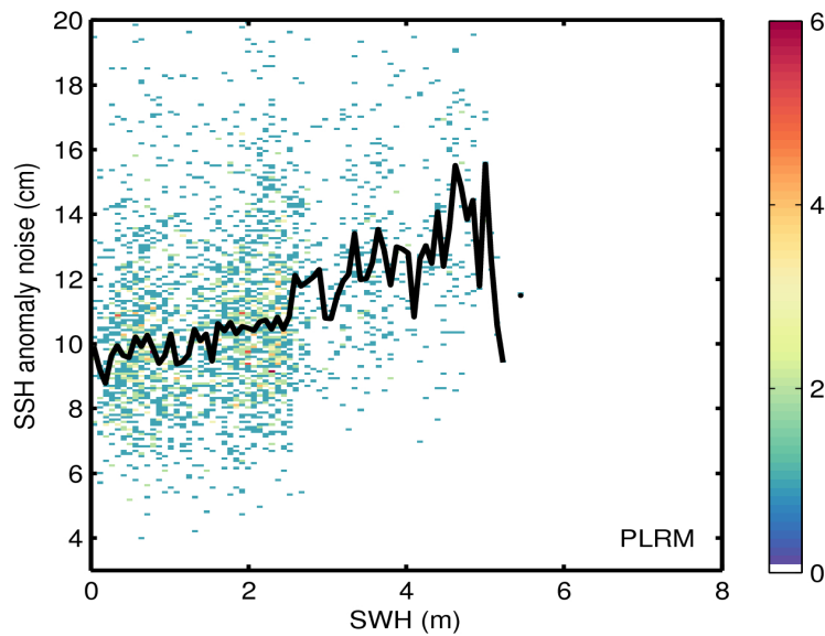
Figure 9. 2D histogram showing flag-valid SSH anomaly noise as a function of SWH for LRM (top) and PLRM (bottom) for 21/07/2016. The black line denotes the median SSH anomaly noise as a function of SWH.
