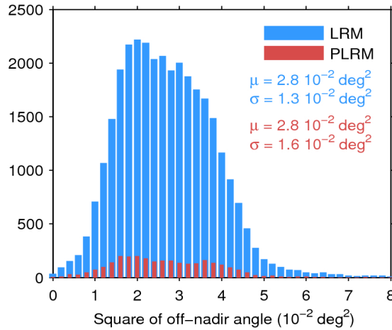
Figure 39. Histogram of flag-valid mispointing over oceans and lakes for LRM (blue) and PLRM (red) for 21/07/2016. Only positive values have been considered. The mean ( \mu ) and standard deviation ( \sigma ) are also shown. Note that values larger than 8 \cdot 10^{-2} \text{ deg}^2 are excluded from the histogram for the sake of readability but not from the computation of \mu and \sigma .
