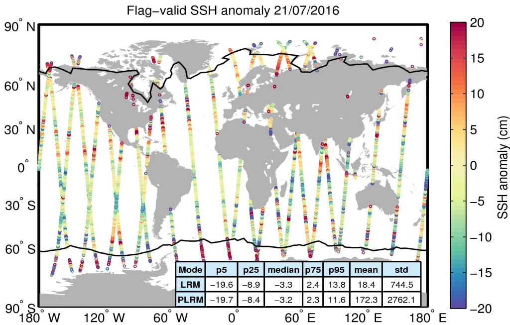
Figure 5. Geographical distribution of flag-valid 1-Hz SSH anomaly data over oceans and lakes for 21/07/2016. The statistical values shown in the table refer to the SSH anomaly in cm and are calculated separately for LRM and PLRM regions. Measurements taken over polar polygons have been excluded from the computation of the statistical values. The black lines mark the outer limit of the Arctic and Antarctic polar polygons.
