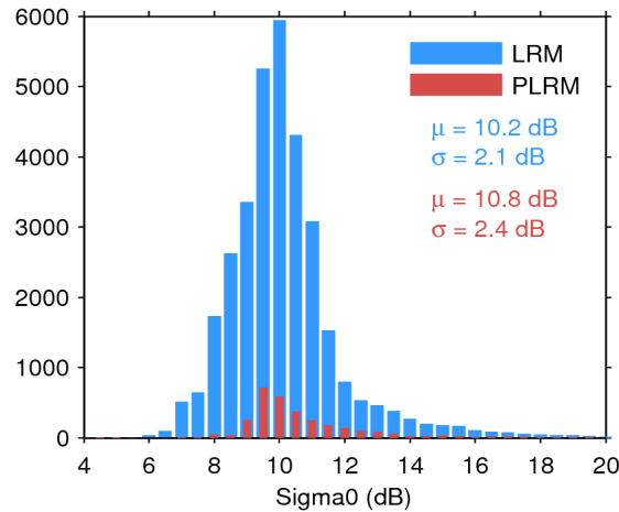
Figure 25. Histogram of flag-valid sigma0 over oceans and lakes for LRM (blue) and PLRM (red) for 21/07/2016. The mean ( \mu ) and standard deviation ( \sigma ) are also shown. Note that values outside [4 20] dB are excluded from the histogram for the sake of readability but not from the computation of \mu and \sigma .
