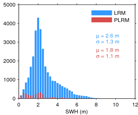
Figure 20. Histogram of science-valid SWH over oceans and lakes for LRM (blue) and PLRM (red) for 21/07/2016. The mean ( \mu ) and standard deviation ( \sigma ) are also shown. Note that values larger than 12 m are excluded from the histogram for the sake of readability but not from the computation of \mu and \sigma .
