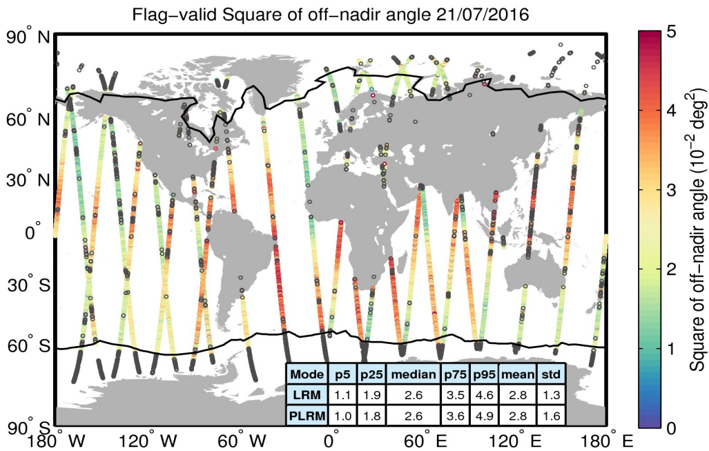
Figure 37. Geographical distribution of flag-valid mispointing data over oceans and lakes for 21/07/2016. The statistical values shown in the table refer to the mispointing in 10^{-2} deg 2 and are calculated separately for LRM and PLRM regions. Measurements taken over polar polygons have been excluded from the computation of the statistical values. The black lines mark the outer limit of the Arctic and Antarctic polar polygons. Gray circles denote negative values.
