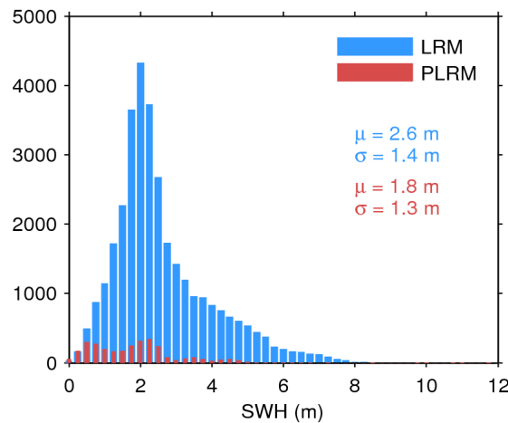
Figure 17. Histogram of flag-valid SWH over oceans and lakes for LRM (blue) and PLRM (red) for 21/07/2016. The mean ( \mu ) and standard deviation ( \sigma ) are also shown. Note that values larger than 12 m are excluded from the histogram for the sake of readability but not from the computation of \mu and \sigma .
