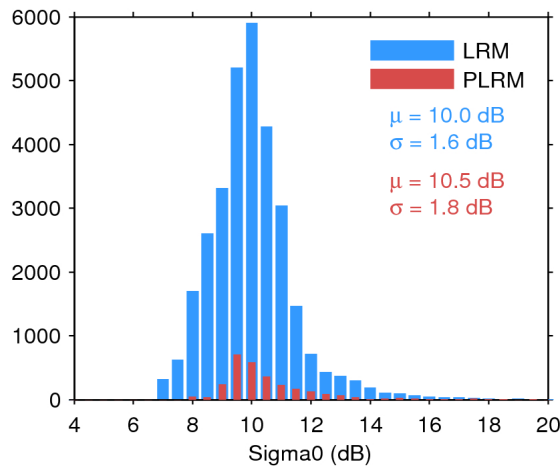
Figure 28. Histogram of science-valid sigma0 over oceans and lakes for LRM (blue) and PLRM (red) for 21/07/2016. The mean ( \mu ) and standard deviation ( \sigma ) are also shown. Note that values outside [4 20] dB are excluded from the histogram for the sake of readability but not from the computation of \mu and \sigma .
