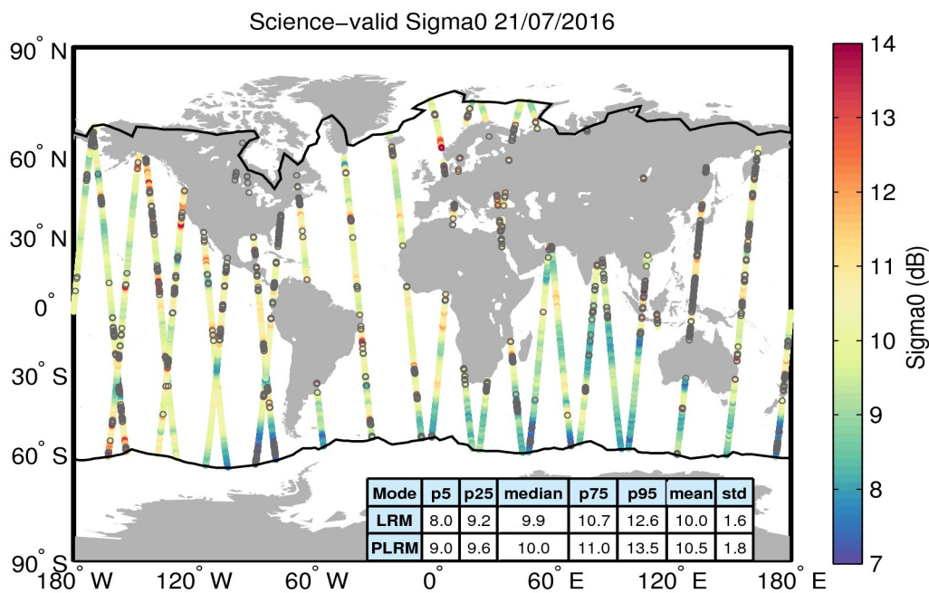
Figure 27. Geographical distribution of science-valid sigma0 data over oceans and lakes for 21/07/2016. The statistical values shown in the table refer to the sigma0 in dB and are calculated separately for LRM and PLRM regions. The black lines mark the outer limit of the Arctic and Antarctic polar polygons. Gray circles denote records that have been rejected based on the editing criteria described in Table 4.
