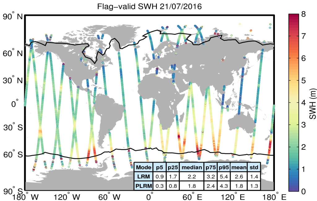
Figure 15. Geographical distribution of flag-valid SWH data over oceans and lakes for 21/07/2016. The statistical values shown in the table refer to the SWH in m and are calculated separately for LRM and PLRM regions. Measurements taken over polar polygons have been excluded from the computation of the statistical values. The black lines mark the outer limit of the Arctic and Antarctic polar polygons.
