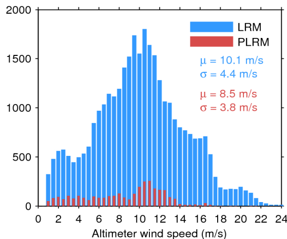
Figure 35. Histogram of science-valid wind over oceans and lakes for LRM (blue) and PLRM (red) for 21/07/2016. The mean ( \mu ) and standard deviation ( \sigma ) are also shown. Note that values larger than 24 m/s are excluded from the histogram for the sake of readability but not from the computation of \mu and \sigma .
