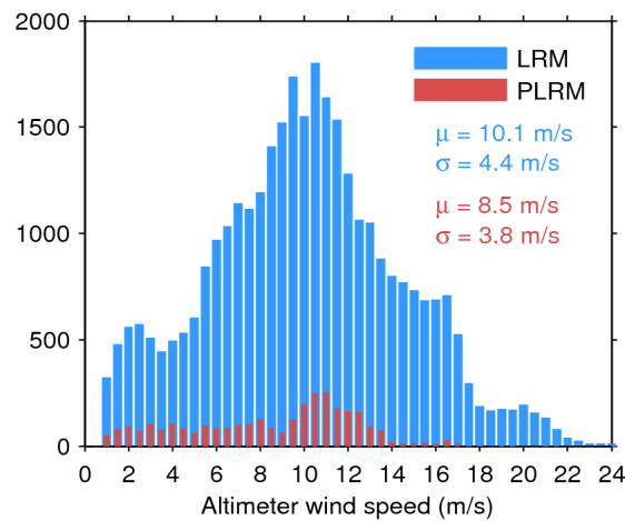
Figure 33. Histogram of flag-valid wind over oceans and lakes for LRM (blue) and PLRM (red) for 21/07/2016. The mean ( \mu ) and standard deviation ( \sigma ) are also shown. Note that values larger than 24 m/s are excluded from the histogram for the sake of readability but not from the computation of \mu and \sigma .
