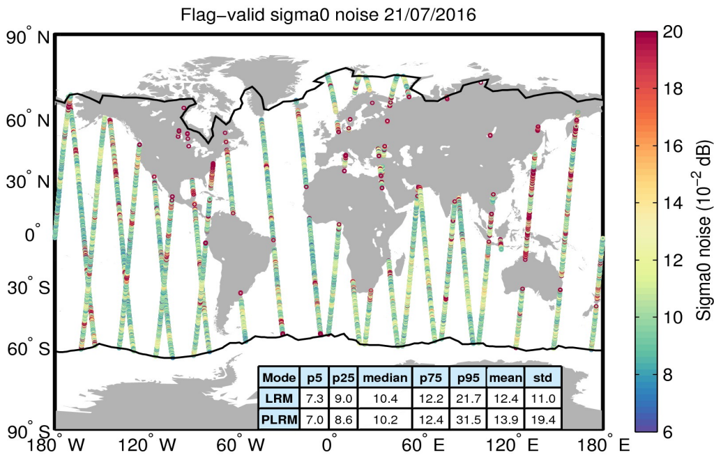
Figure 26. Geographical distribution of flag-valid 20-Hz sigma0 measurement noise over oceans and lakes for 21/07/2016. The statistical values shown in the table refer to the sigma0 noise and are calculated separately for LRM and PLRM regions. Measurements taken over polar polygons have been excluded from the computation of the statistical values. The black lines mark the outer limit of the Arctic and Antarctic polar polygons.
