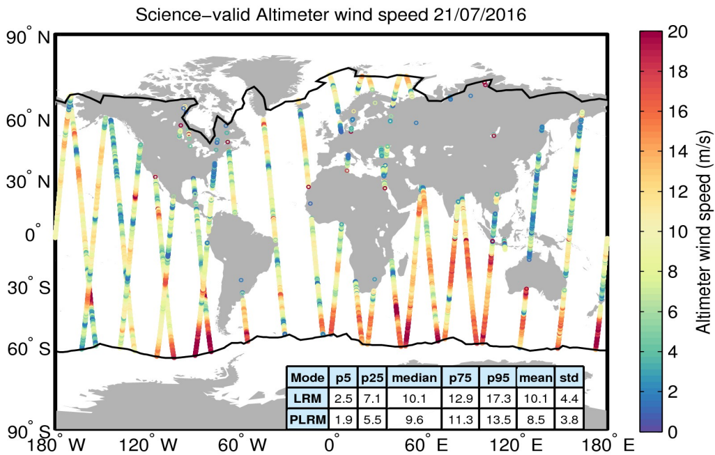
Figure 34. Geographical distribution of science-valid wind data over oceans and lakes for 21/07/2016. The statistical values shown in the table refer to the wind in m/s and are calculated separately for LRM and PLRM regions. The black lines mark the outer limit of the Arctic and Antarctic polar polygons. Gray circles denote records that have been rejected based on the editing criteria described in Table 5.
