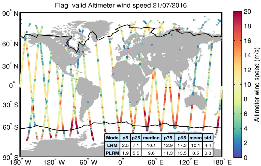
Figure 31. Geographical distribution of flag-valid wind data over oceans and lakes for 21/07/2016. The statistical values shown in the table refer to the wind in m/s and are calculated separately for LRM and PLRM regions. Measurements taken over polar polygons have been excluded from the computation of the statistical values. The black lines mark the outer limit of the Arctic and Antarctic polar polygons.
