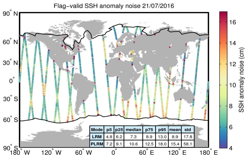
Figure 8. Geographical distribution of flag-valid 20-Hz SSH anomaly measurement noise over oceans and lakes for 21/07/2016. The statistical values shown in the table refer to the SSH anomaly noise and are calculated separately for LRM and PLRM regions. Measurements taken over polar polygons have been excluded from the computation of the statistical values. The black lines mark the outer limit of the Arctic and Antarctic polar polygons.
