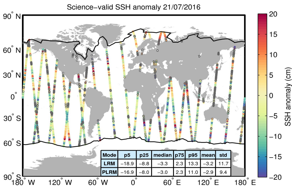
Figure 10. Geographical distribution of science-valid SSH anomaly data over oceans and lakes for 21/07/2016. The statistical values shown in the table refer to the SSH anomaly in cm and are calculated separately for LRM and PLRM regions. The black lines mark the outer limit of the Arctic and Antarctic polar polygons. Gray circles denote records that have been rejected based on the editing criteria described in Table 2.
