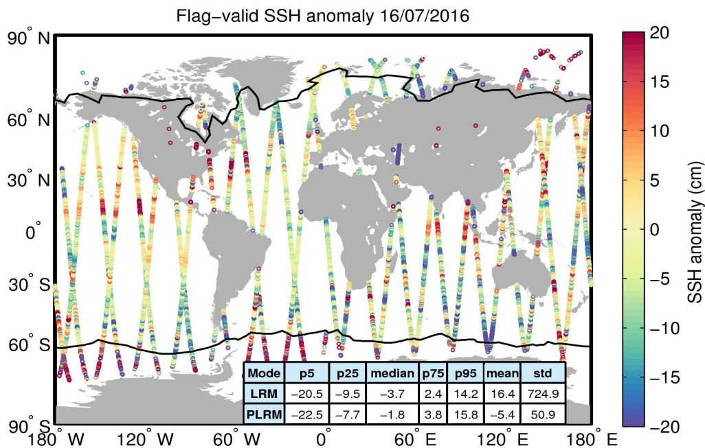
Figure 5. Geographical distribution of flag-valid 1-Hz SSH anomaly data over oceans and lakes for 16/07/2016. The statistical values shown in the table refer to the SSH anomaly in cm and are calculated separately for LRM and PLRM regions. Measurements taken over polar polygons have been excluded from the computation of the statistical values. The black lines mark the outer limit of the Arctic and Antarctic polar polygons.
