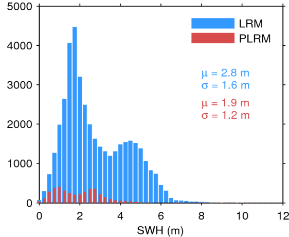
Figure 17. Histogram of flag-valid SWH over oceans and lakes for LRM (blue) and PLRM (red) for 16/07/2016. The mean ( \mu ) and standard deviation ( \sigma ) are also shown. Note that values larger than 12 m are excluded from the histogram for the sake of readability but not from the computation of \mu and \sigma .
