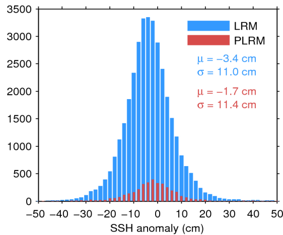
Figure 11. Histogram of science-valid SSH anomaly over oceans and lakes for LRM (blue) and PLRM (red) for 16/07/2016. The mean ( \mu ) and standard deviation ( \sigma ) are also shown. Note that values outside [-50\ 50] cm are excluded from the histogram for the sake of readability but not from the computation of \mu and \sigma .
