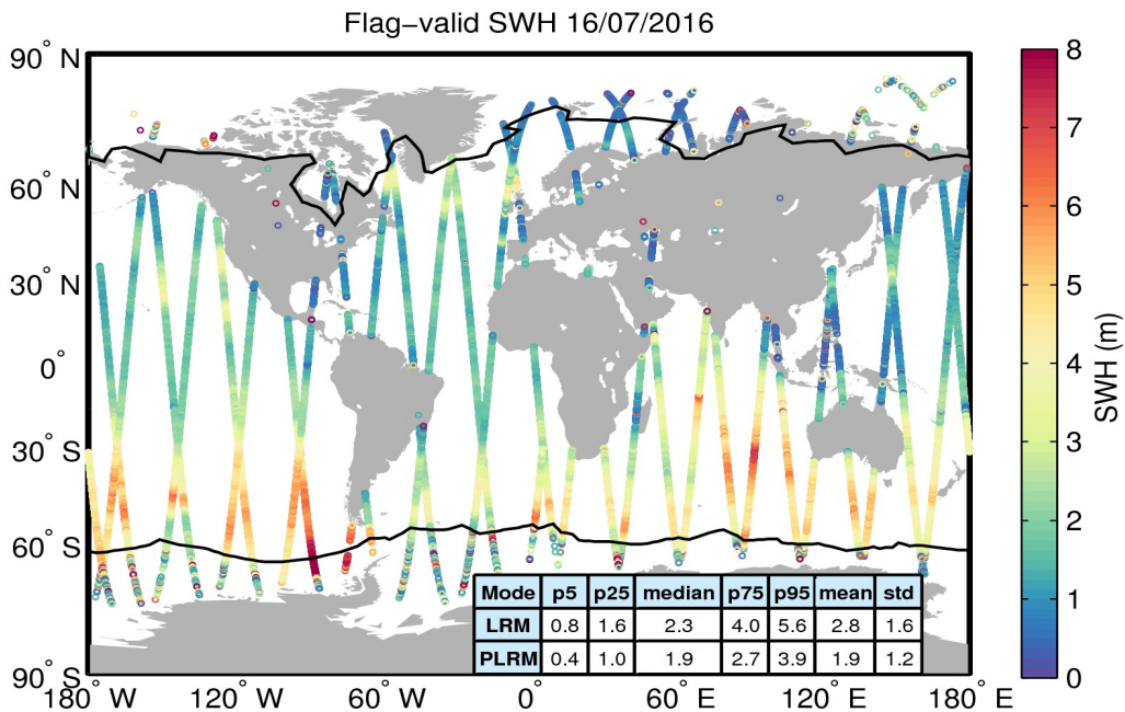
Figure 15. Geographical distribution of flag-valid SWH data over oceans and lakes for 16/07/2016. The statistical values shown in the table refer to the SWH in m and are calculated separately for LRM and PLRM regions. Measurements taken over polar polygons have been excluded from the computation of the statistical values. The black lines mark the outer limit of the Arctic and Antarctic polar polygons.
