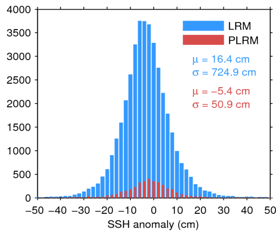
Figure 7. Histogram of flag-valid SSH anomaly over oceans and lakes for LRM (blue) and PLRM (red) for 16/07/2016. The mean ( \mu ) and standard deviation ( \sigma ) are also shown. Note that values outside [-50 50] cm are excluded from the histogram for the sake of readability but not from the computation of \mu and \sigma .
