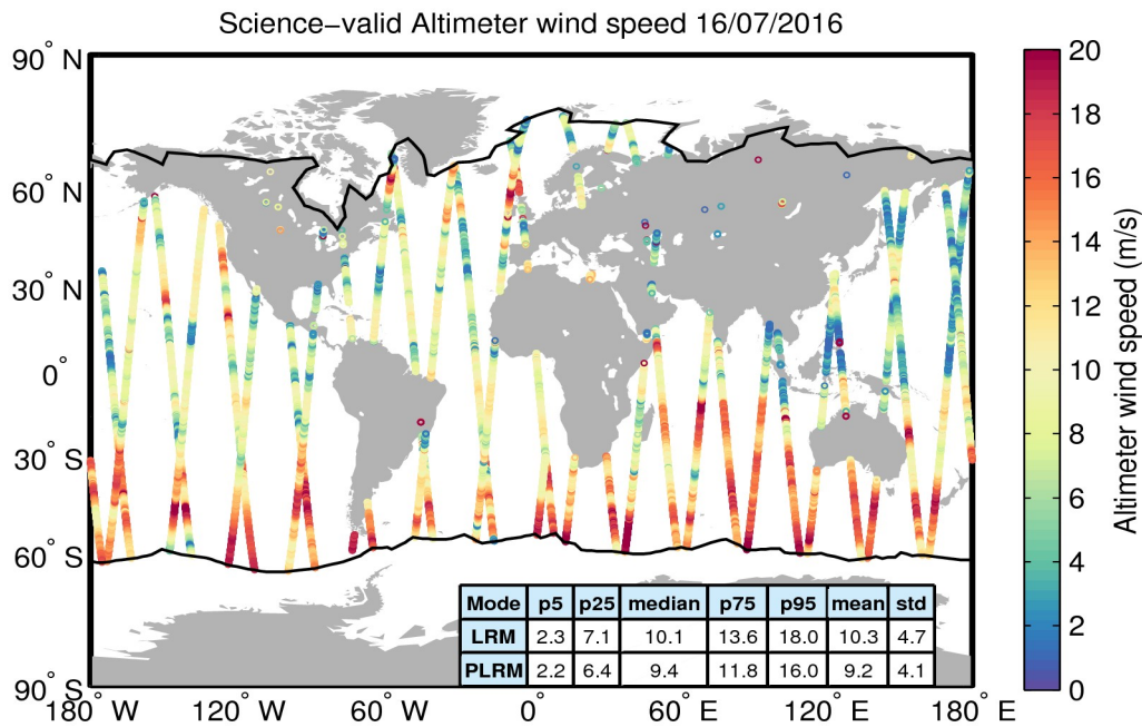
Figure 34. Geographical distribution of science-valid wind data over oceans and lakes for 16/07/2016. The statistical values shown in the table refer to the wind in m/s and are calculated separately for LRM and PLRM regions. The black lines mark the outer limit of the Arctic and Antarctic polar polygons. Gray circles denote records that have been rejected based on the editing criteria described in Table 5.
