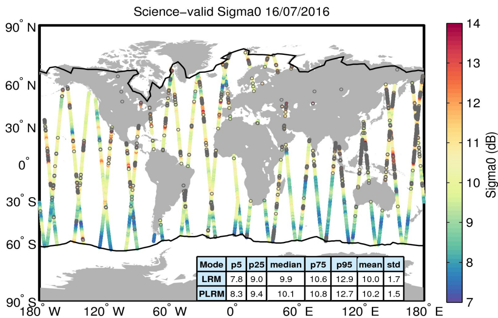
Figure 27. Geographical distribution of science-valid sigma0 data over oceans and lakes for 16/07/2016. The statistical values shown in the table refer to the sigma0 in dB and are calculated separately for LRM and PLRM regions. The black lines mark the outer limit of the Arctic and Antarctic polar polygons. Gray circles denote records that have been rejected based on the editing criteria described in Table 4.
