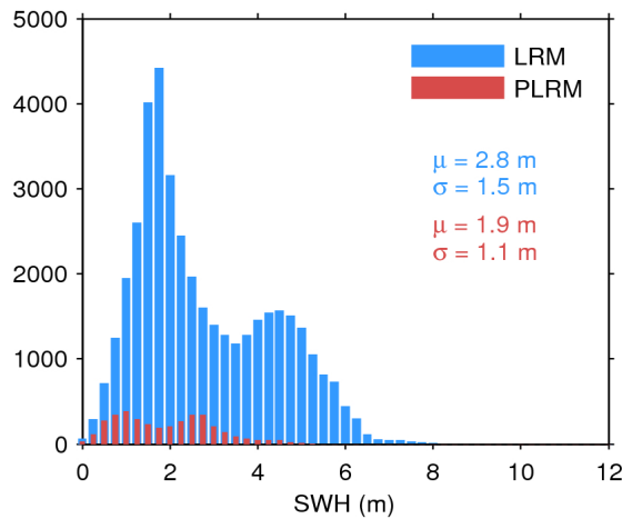
Figure 20. Histogram of science-valid SWH over oceans and lakes for LRM (blue) and PLRM (red) for 16/07/2016. The mean ( \mu ) and standard deviation ( \sigma ) are also shown. Note that values larger than 12 m are excluded from the histogram for the sake of readability but not from the computation of \mu and \sigma .
