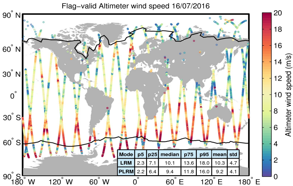
Figure 31. Geographical distribution of flag-valid wind data over oceans and lakes for 16/07/2016. The statistical values shown in the table refer to the wind in m/s and are calculated separately for LRM and PLRM regions. Measurements taken over polar polygons have been excluded from the computation of the statistical values. The black lines mark the outer limit of the Arctic and Antarctic polar polygons.
