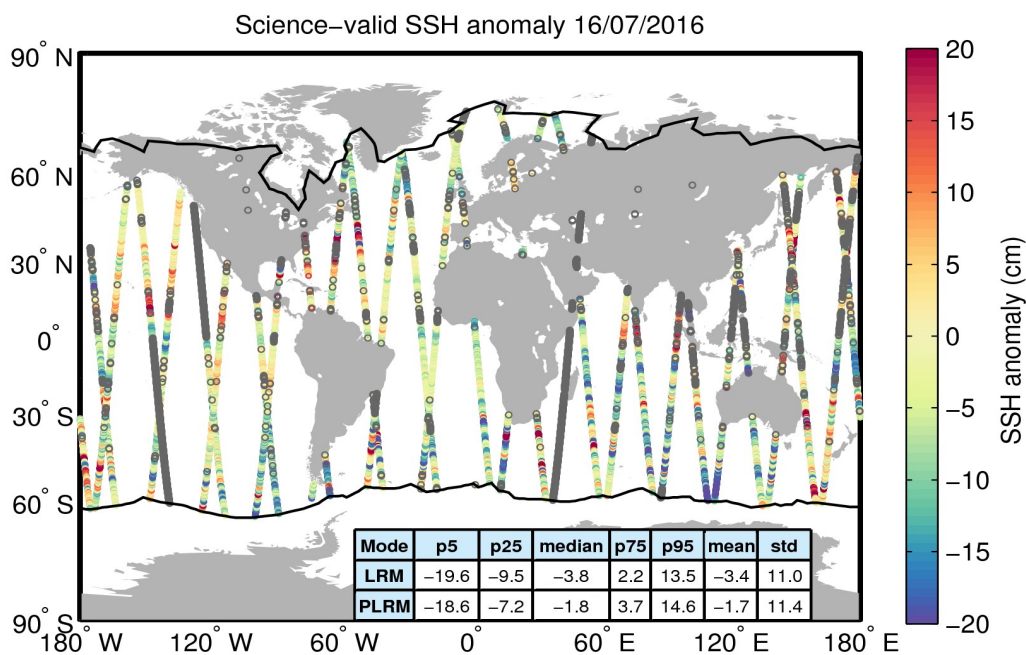
Figure 10. Geographical distribution of science-valid SSH anomaly data over oceans and lakes for 16/07/2016. The statistical values shown in the table refer to the SSH anomaly in cm and are calculated separately for LRM and PLRM regions. The black lines mark the outer limit of the Arctic and Antarctic polar polygons. Gray circles denote records that have been rejected based on the editing criteria described in Table 2.
