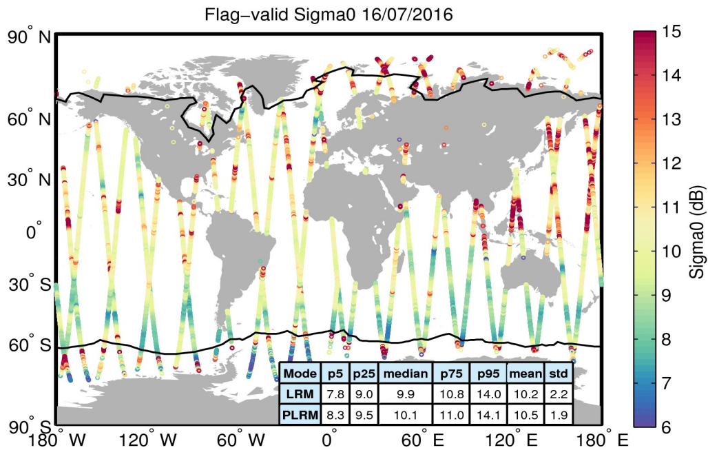
Figure 23. Geographical distribution of flag-valid sigma0 data over oceans and lakes for 16/07/2016. The statistical values shown in the table refer to the sigma0 in dB and are calculated separately for LRM and PLRM regions. Measurements taken over polar polygons have been excluded from the computation of the statistical values. The black lines mark the outer limit of the Arctic and Antarctic polar polygons.
