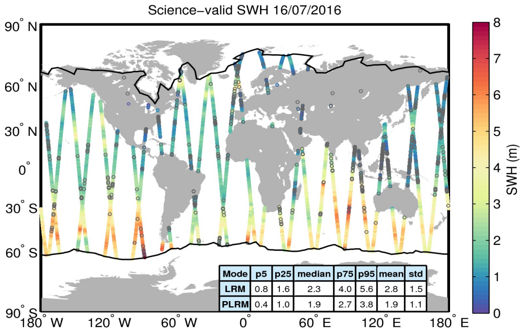
Figure 19. Geographical distribution of science-valid SWH data over oceans and lakes for 16/07/2016. The statistical values shown in the table refer to the SWH in m and are calculated separately for LRM and PLRM regions. The black lines mark the outer limit of the Arctic and Antarctic polar polygons. Gray circles denote records that have been rejected based on the editing criteria described in Table 3.
