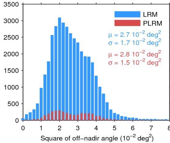
Figure 39. Histogram of flag-valid mispointing over oceans and lakes for LRM (blue) and PLRM (red) for 16/07/2016. Only positive values have been considered. The mean ( \mu ) and standard deviation ( \sigma ) are also shown. Note that values larger than 8 \cdot 10^{-2} \text{ deg}^2 are excluded from the histogram for the sake of readability but not from the computation of \mu and \sigma .
