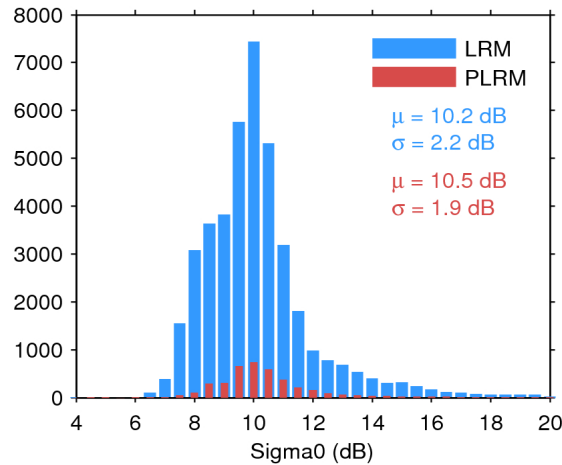
Figure 25. Histogram of flag-valid sigma0 over oceans and lakes for LRM (blue) and PLRM (red) for 16/07/2016. The mean ( \mu ) and standard deviation ( \sigma ) are also shown. Note that values outside [4 20] dB are excluded from the histogram for the sake of readability but not from the computation of \mu and \sigma .
