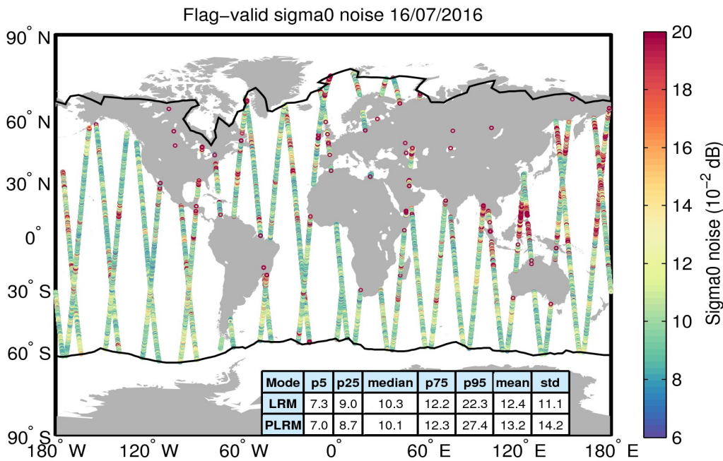
Figure 26. Geographical distribution of flag-valid 20-Hz sigma0 measurement noise over oceans and lakes for 16/07/2016. The statistical values shown in the table refer to the sigma0 noise and are calculated separately for LRM and PLRM regions. Measurements taken over polar polygons have been excluded from the computation of the statistical values. The black lines mark the outer limit of the Arctic and Antarctic polar polygons.
