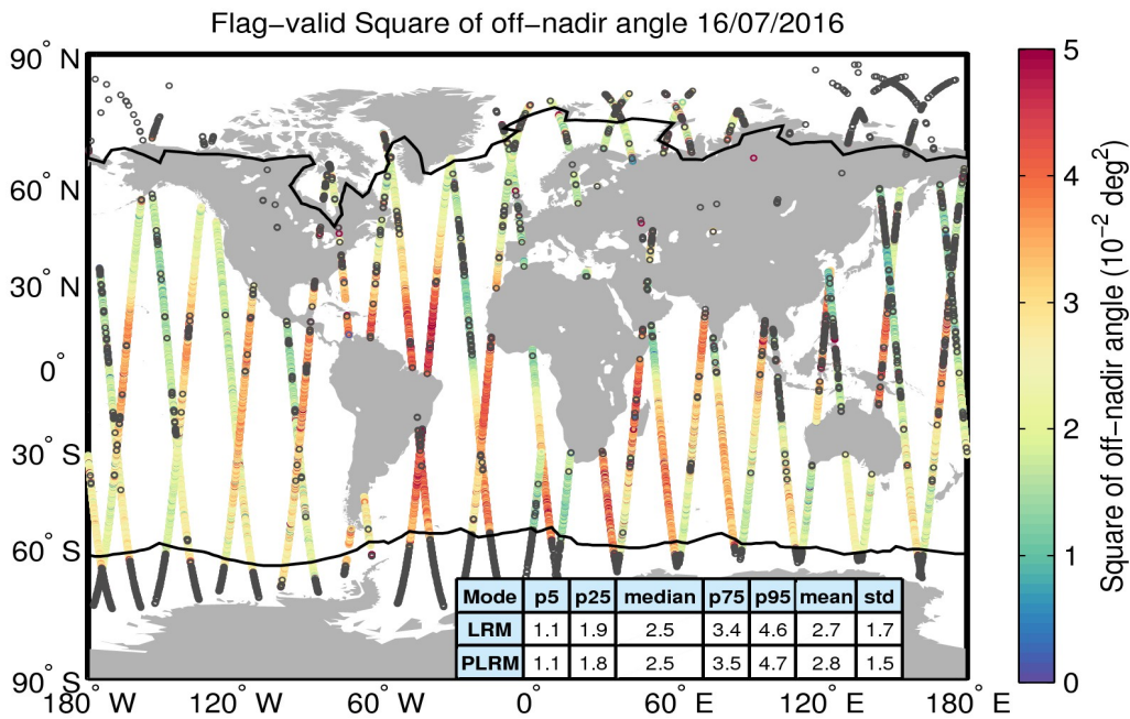
Figure 37. Geographical distribution of flag-valid mispointing data over oceans and lakes for 16/07/2016. The statistical values shown in the table refer to the mispointing in 10^{-2} \text{ deg}^2 and are calculated separately for LRM and PLRM regions. Measurements taken over polar polygons have been excluded from the computation of the statistical values. The black lines mark the outer limit of the Arctic and Antarctic polar polygons. Gray circles denote negative values.
