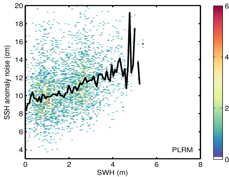
Figure 9. 2D histogram showing flag-valid SSH anomaly noise as a function of SWH for LRM (top) and PLRM (bottom) for 16/07/2016. The black line denotes the median SSH anomaly noise as a function of SWH.
