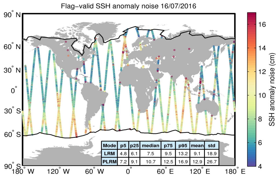
Figure 8. Geographical distribution of flag-valid 20-Hz SSH anomaly measurement noise over oceans and lakes for 16/07/2016. The statistical values shown in the table refer to the SSH anomaly noise and are calculated separately for LRM and PLRM regions. Measurements taken over polar polygons have been excluded from the computation of the statistical values. The black lines mark the outer limit of the Arctic and Antarctic polar polygons.
