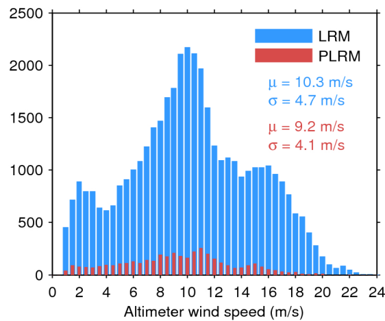
Figure 33. Histogram of flag-valid wind over oceans and lakes for LRM (blue) and PLRM (red) for 16/07/2016. The mean ( \mu ) and standard deviation ( \sigma ) are also shown. Note that values larger than 24 m/s are excluded from the histogram for the sake of readability but not from the computation of \mu and \sigma .
