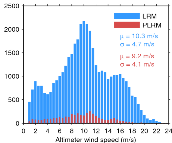
Figure 35. Histogram of science-valid wind over oceans and lakes for LRM (blue) and PLRM (red) for 16/07/2016. The mean ( \mu ) and standard deviation ( \sigma ) are also shown. Note that values larger than 24 m/s are excluded from the histogram for the sake of readability but not from the computation of \mu and \sigma .
