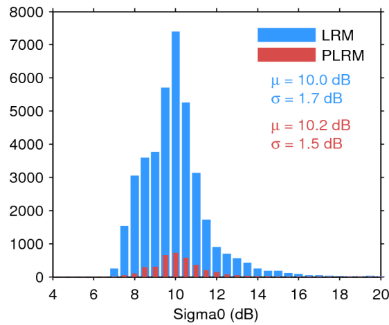
Figure 28. Histogram of science-valid sigma0 over oceans and lakes for LRM (blue) and PLRM (red) for 16/07/2016. The mean ( \mu ) and standard deviation ( \sigma ) are also shown. Note that values outside [4 20] dB are excluded from the histogram for the sake of readability but not from the computation of \mu and \sigma .
