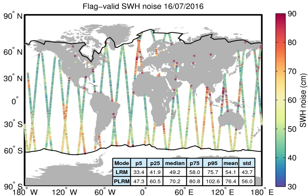
Figure 18. Geographical distribution of flag-valid 20-Hz SWH measurement noise over oceans and lakes for 16/07/2016. The statistical values shown in the table refer to the SWH noise and are calculated separately for LRM and PLRM regions. Measurements taken over polar polygons have been excluded from the computation of the statistical values. The black lines mark the outer limit of the Arctic and Antarctic polar polygons.
