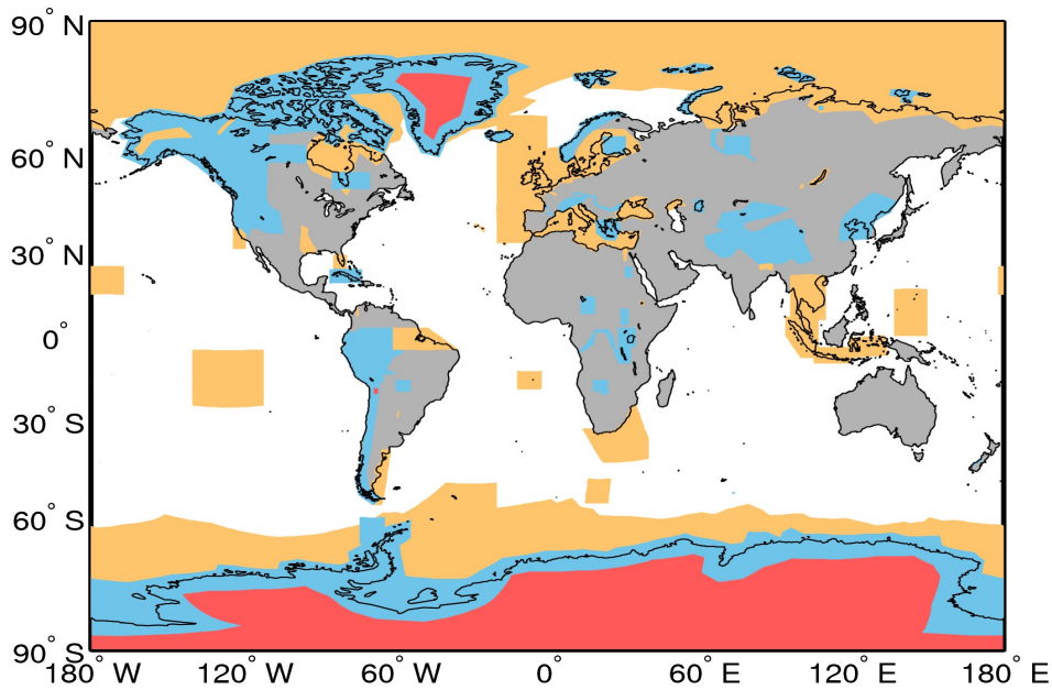
Figure A1. Extent of the regions defining the geographical mode mask for 10/07/2016. The regions where SAR, and SARIn are operated are denoted by the orange and blue polygons, respectively. LRM is operated over areas of the continental ice sheets (red polygons) and over oceans and land not covered by other modes.
