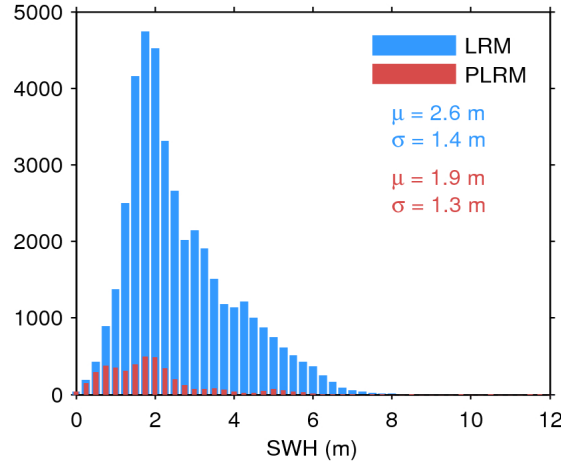
Figure 17. Histogram of flag-valid SWH over oceans and lakes for LRM (blue) and PLRM (red) for 10/07/2016. The mean ( \mu ) and standard deviation ( \sigma ) are also shown. Note that values larger than 12 m are excluded from the histogram for the sake of readability but not from the computation of \mu and \sigma .
