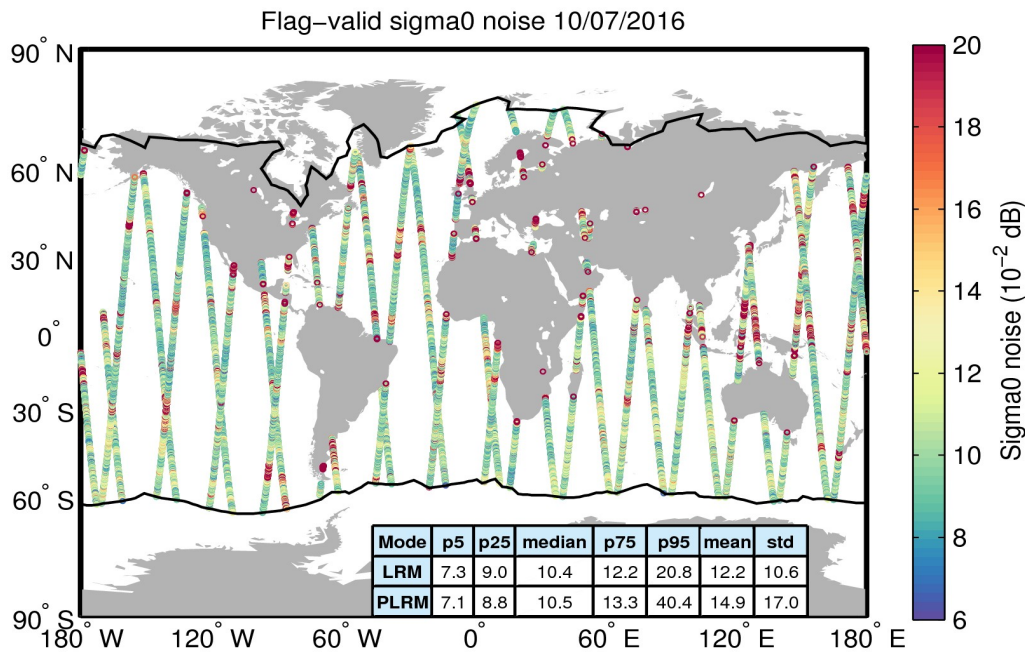
Figure 26. Geographical distribution of flag-valid 20-Hz sigma0 measurement noise over oceans and lakes for 10/07/2016. The statistical values shown in the table refer to the sigma0 noise and are calculated separately for LRM and PLRM regions. Measurements taken over polar polygons have been excluded from the computation of the statistical values. The black lines mark the outer limit of the Arctic and Antarctic polar polygons.
