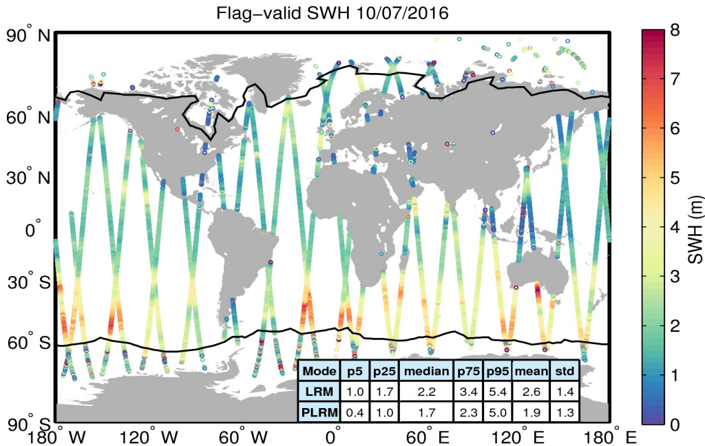
Figure 15. Geographical distribution of flag-valid SWH data over oceans and lakes for 10/07/2016. The statistical values shown in the table refer to the SWH in m and are calculated separately for LRM and PLRM regions. Measurements taken over polar polygons have been excluded from the computation of the statistical values. The black lines mark the outer limit of the Arctic and Antarctic polar polygons.
