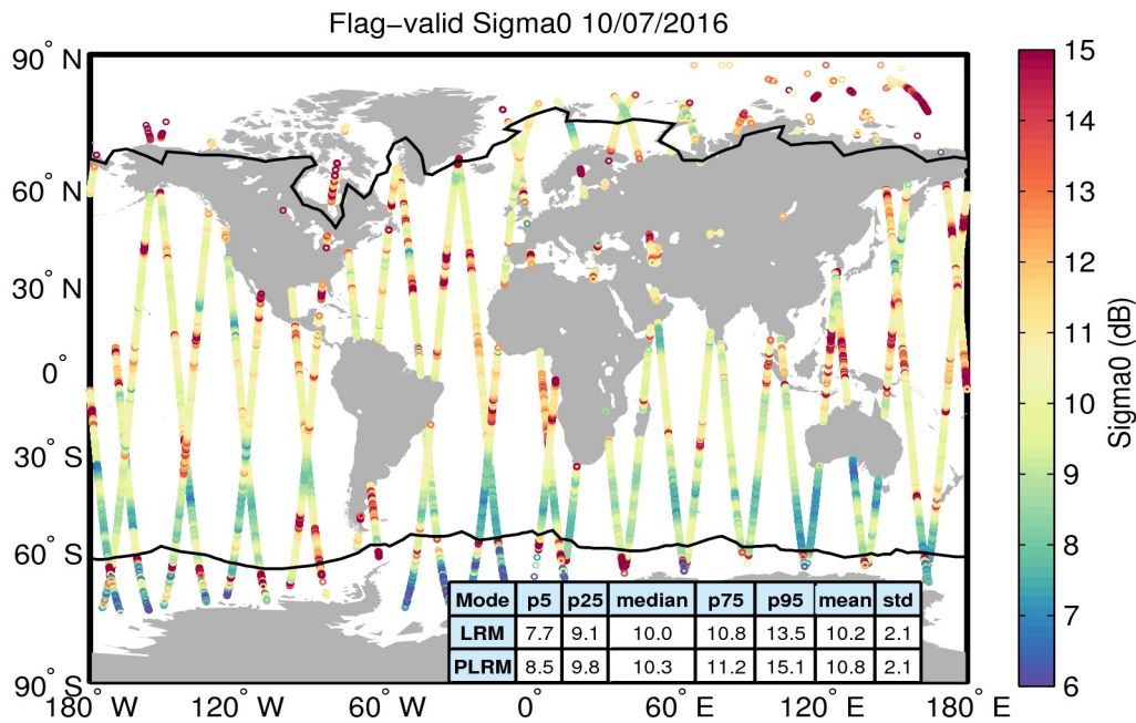
Figure 23. Geographical distribution of flag-valid sigma0 data over oceans and lakes for 10/07/2016. The statistical values shown in the table refer to the sigma0 in dB and are calculated separately for LRM and PLRM regions. Measurements taken over polar polygons have been excluded from the computation of the statistical values. The black lines mark the outer limit of the Arctic and Antarctic polar polygons.
