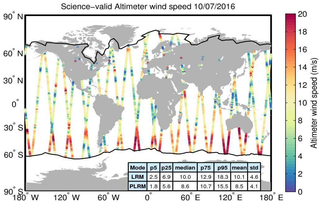
Figure 34. Geographical distribution of science-valid wind data over oceans and lakes for 10/07/2016. The statistical values shown in the table refer to the wind in m/s and are calculated separately for LRM and PLRM regions. The black lines mark the outer limit of the Arctic and Antarctic polar polygons. Gray circles denote records that have been rejected based on the editing criteria described in Table 5.
