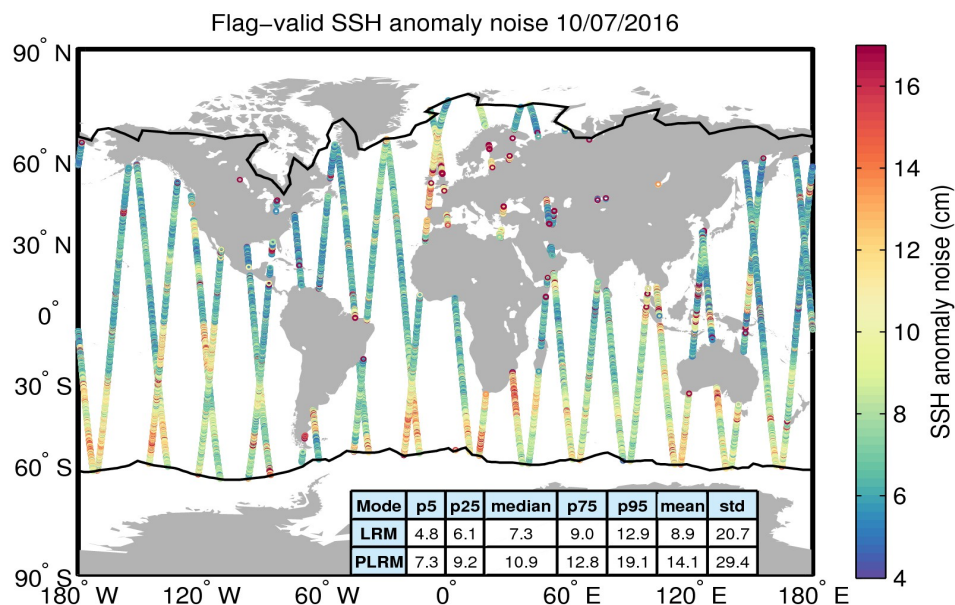
Figure 8. Geographical distribution of flag-valid 20-Hz SSH anomaly measurement noise over oceans and lakes for 10/07/2016. The statistical values shown in the table refer to the SSH anomaly noise and are calculated separately for LRM and PLRM regions. Measurements taken over polar polygons have been excluded from the computation of the statistical values. The black lines mark the outer limit of the Arctic and Antarctic polar polygons.
