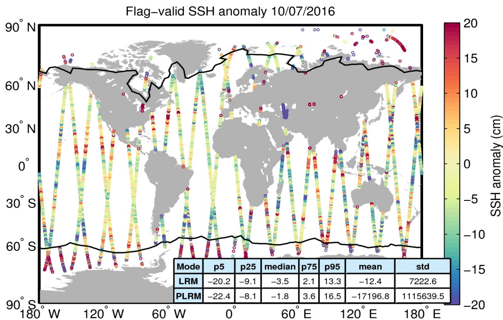
Figure 5. Geographical distribution of flag-valid 1-Hz SSH anomaly data over oceans and lakes for 10/07/2016. The statistical values shown in the table refer to the SSH anomaly in cm and are calculated separately for LRM and PLRM regions. Measurements taken over polar polygons have been excluded from the computation of the statistical values. The black lines mark the outer limit of the Arctic and Antarctic polar polygons.
