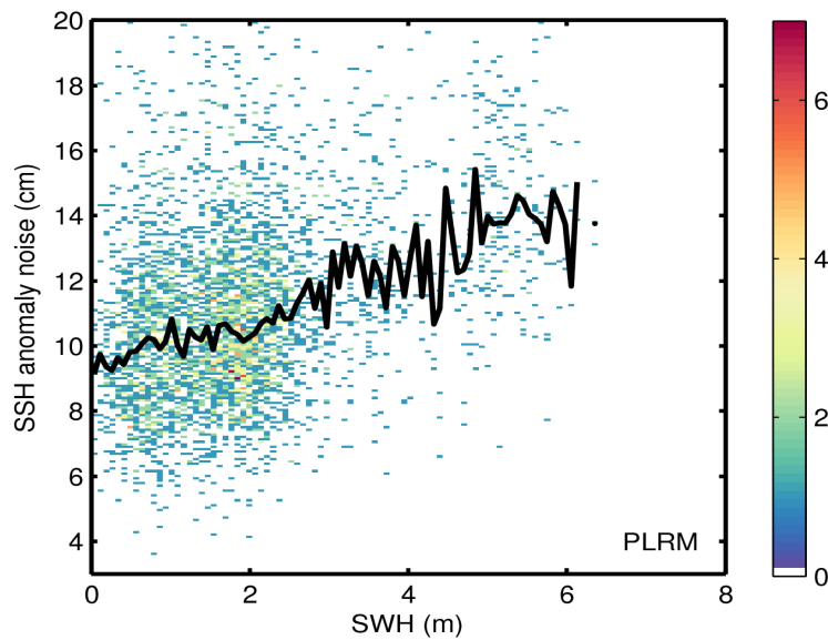
Figure 9. 2D histogram showing flag-valid SSH anomaly noise as a function of SWH for LRM (top) and PLRM (bottom) for 10/07/2016. The black line denotes the median SSH anomaly noise as a function of SWH.
