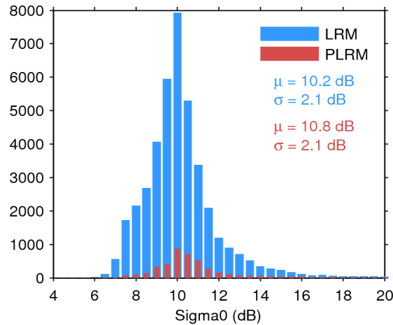
Figure 25. Histogram of flag-valid sigma0 over oceans and lakes for LRM (blue) and PLRM (red) for 10/07/2016. The mean ( \mu ) and standard deviation ( \sigma ) are also shown. Note that values outside [4 20] dB are excluded from the histogram for the sake of readability but not from the computation of \mu and \sigma .
