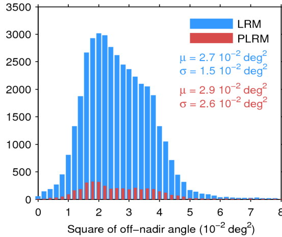
Figure 39. Histogram of flag-valid mispointing over oceans and lakes for LRM (blue) and PLRM (red) for 10/07/2016. Only positive values have been considered. The mean ( \mu ) and standard deviation ( \sigma ) are also shown. Note that values larger than 8 \cdot 10^{-2} \text{ deg}^2 are excluded from the histogram for the sake of readability but not from the computation of \mu and \sigma .
