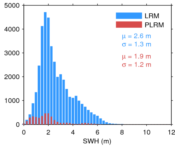
Figure 20. Histogram of science-valid SWH over oceans and lakes for LRM (blue) and PLRM (red) for 10/07/2016. The mean ( \mu ) and standard deviation ( \sigma ) are also shown. Note that values larger than 12 m are excluded from the histogram for the sake of readability but not from the computation of \mu and \sigma .
