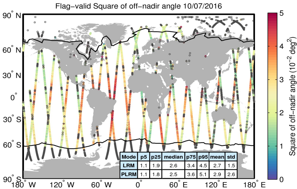
Figure 37. Geographical distribution of flag-valid mispointing data over oceans and lakes for 10/07/2016. The statistical values shown in the table refer to the mispointing in 10^{-2} deg 2 and are calculated separately for LRM and PLRM regions. Measurements taken over polar polygons have been excluded from the computation of the statistical values. The black lines mark the outer limit of the Arctic and Antarctic polar polygons. Gray circles denote negative values.
