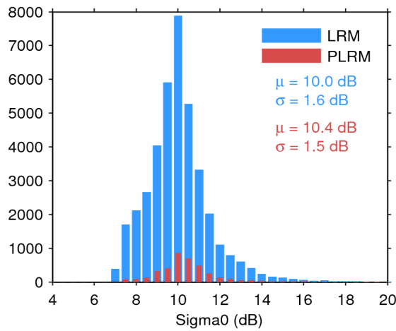
Figure 28. Histogram of science-valid sigma0 over oceans and lakes for LRM (blue) and PLRM (red) for 10/07/2016. The mean ( \mu ) and standard deviation ( \sigma ) are also shown. Note that values outside [4 20] dB are excluded from the histogram for the sake of readability but not from the computation of \mu and \sigma .
