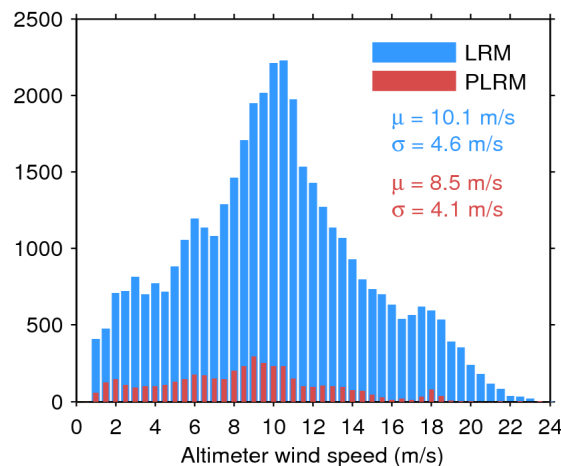
Figure 35. Histogram of science-valid wind over oceans and lakes for LRM (blue) and PLRM (red) for 10/07/2016. The mean ( \mu ) and standard deviation ( \sigma ) are also shown. Note that values larger than 24 m/s are excluded from the histogram for the sake of readability but not from the computation of \mu and \sigma .
