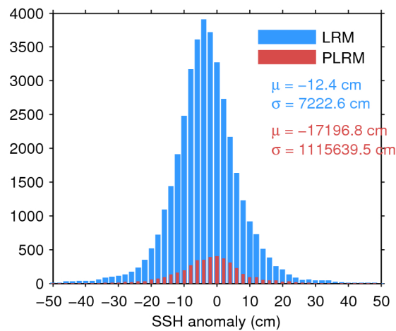
Figure 7. Histogram of flag-valid SSH anomaly over oceans and lakes for LRM (blue) and PLRM (red) for 10/07/2016. The mean ( \mu ) and standard deviation ( \sigma ) are also shown. Note that values outside [-50 \ 50] cm are excluded from the histogram for the sake of readability but not from the computation of \mu and \sigma .
