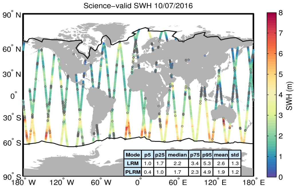
Figure 19. Geographical distribution of science-valid SWH data over oceans and lakes for 10/07/2016. The statistical values shown in the table refer to the SWH in m and are calculated separately for LRM and PLRM regions. The black lines mark the outer limit of the Arctic and Antarctic polar polygons. Gray circles denote records that have been rejected based on the editing criteria described in Table 3.
