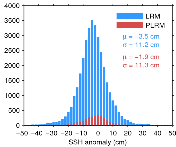
Figure 11. Histogram of science-valid SSH anomaly over oceans and lakes for LRM (blue) and PLRM (red) for 10/07/2016. The mean ( \mu ) and standard deviation ( \sigma ) are also shown. Note that values outside [-50 50] cm are excluded from the histogram for the sake of readability but not from the computation of \mu and \sigma .
