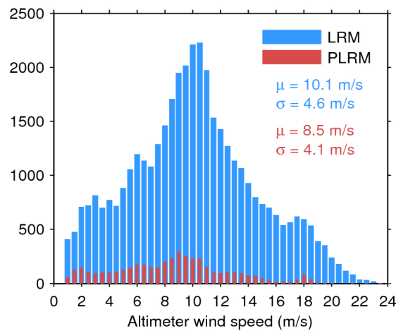
Figure 33. Histogram of flag-valid wind over oceans and lakes for LRM (blue) and PLRM (red) for 10/07/2016. The mean ( \mu ) and standard deviation ( \sigma ) are also shown. Note that values larger than 24 m/s are excluded from the histogram for the sake of readability but not from the computation of \mu and \sigma .
