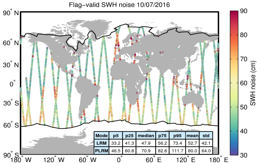
Figure 18. Geographical distribution of flag-valid 20-Hz SWH measurement noise over oceans and lakes for 10/07/2016. The statistical values shown in the table refer to the SWH noise and are calculated separately for LRM and PLRM regions. Measurements taken over polar polygons have been excluded from the computation of the statistical values. The black lines mark the outer limit of the Arctic and Antarctic polar polygons.
