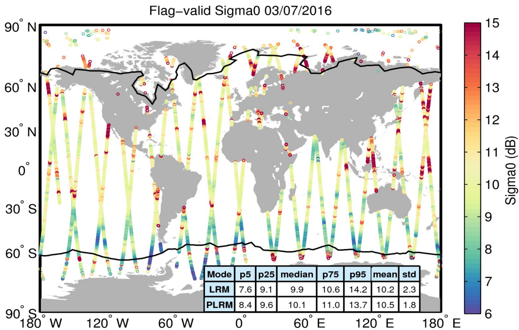
Figure 23. Geographical distribution of flag-valid sigma0 data over oceans and lakes for 03/07/2016. The statistical values shown in the table refer to the sigma0 in dB and are calculated separately for LRM and PLRM regions. Measurements taken over polar polygons have been excluded from the computation of the statistical values. The black lines mark the outer limit of the Arctic and Antarctic polar polygons.
