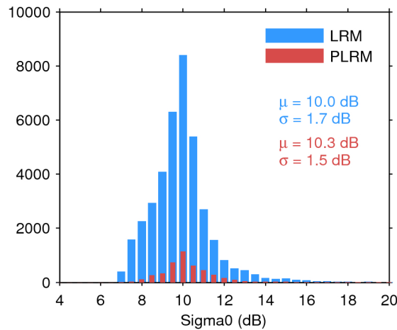
Figure 28. Histogram of science-valid sigma0 over oceans and lakes for LRM (blue) and PLRM (red) for 03/07/2016. The mean ( \mu ) and standard deviation ( \sigma ) are also shown. Note that values outside [4 20] dB are excluded from the histogram for the sake of readability but not from the computation of \mu and \sigma .
