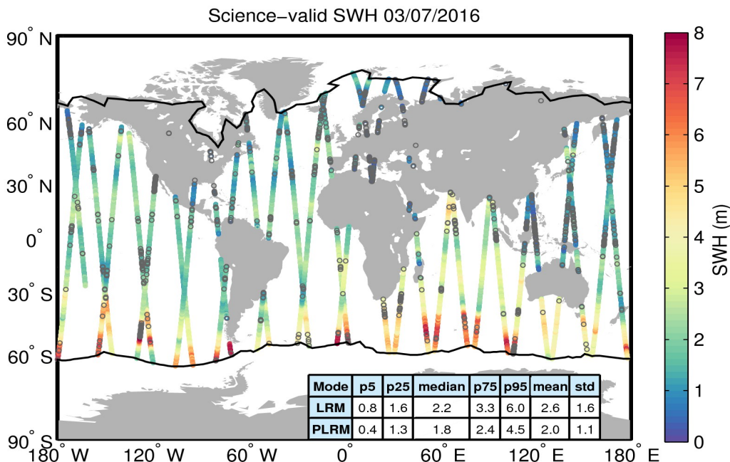
Figure 19. Geographical distribution of science-valid SWH data over oceans and lakes for 03/07/2016. The statistical values shown in the table refer to the SWH in m and are calculated separately for LRM and PLRM regions. The black lines mark the outer limit of the Arctic and Antarctic polar polygons. Gray circles denote records that have been rejected based on the editing criteria described in Table 3.
