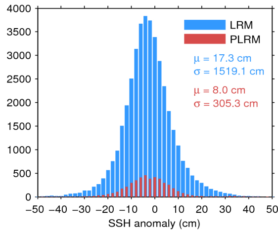
Figure 7. Histogram of flag-valid SSH anomaly over oceans and lakes for LRM (blue) and PLRM (red) for 03/07/2016. The mean ( \mu ) and standard deviation ( \sigma ) are also shown. Note that values outside [-50\ 50] cm are excluded from the histogram for the sake of readability but not from the computation of \mu and \sigma .
