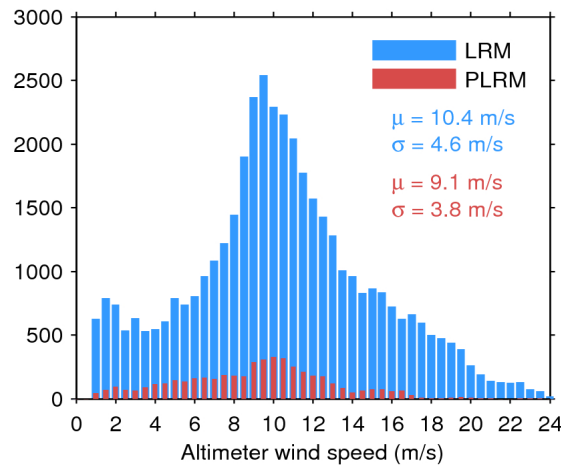
Figure 33. Histogram of flag-valid wind over oceans and lakes for LRM (blue) and PLRM (red) for 03/07/2016. The mean ( \mu ) and standard deviation ( \sigma ) are also shown. Note that values larger than 24 m/s are excluded from the histogram for the sake of readability but not from the computation of \mu and \sigma .
