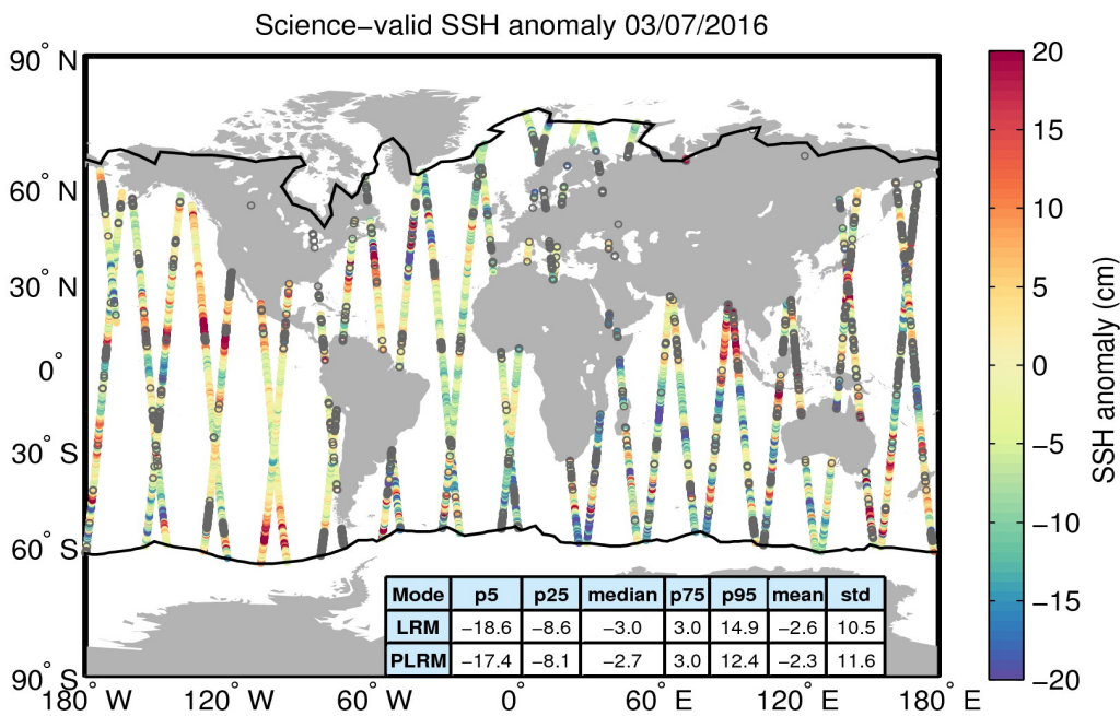
Figure 10. Geographical distribution of science-valid SSH anomaly data over oceans and lakes for 03/07/2016. The statistical values shown in the table refer to the SSH anomaly in cm and are calculated separately for LRM and PLRM regions. The black lines mark the outer limit of the Arctic and Antarctic polar polygons. Gray circles denote records that have been rejected based on the editing criteria described in Table 2.
