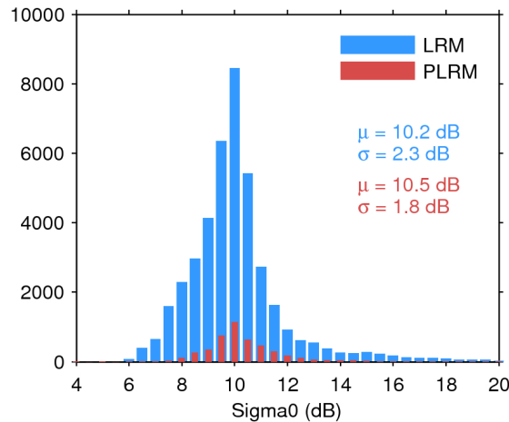
Figure 25. Histogram of flag-valid sigma0 over oceans and lakes for LRM (blue) and PLRM (red) for 03/07/2016. The mean ( \mu ) and standard deviation ( \sigma ) are also shown. Note that values outside [4 20] dB are excluded from the histogram for the sake of readability but not from the computation of \mu and \sigma .
