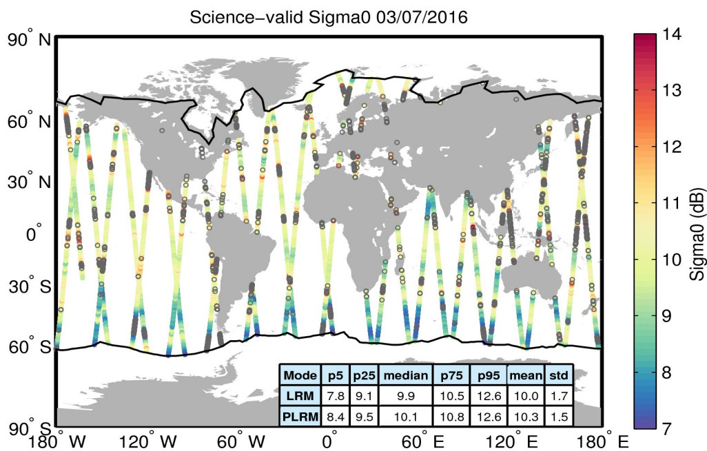
Figure 27. Geographical distribution of science-valid sigma0 data over oceans and lakes for 03/07/2016. The statistical values shown in the table refer to the sigma0 in dB and are calculated separately for LRM and PLRM regions. The black lines mark the outer limit of the Arctic and Antarctic polar polygons. Gray circles denote records that have been rejected based on the editing criteria described in Table 4.
