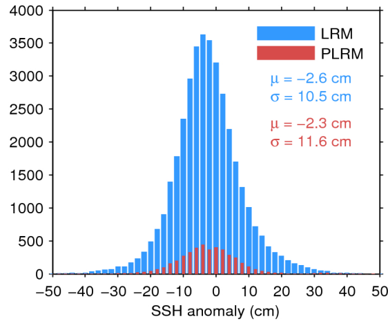
Figure 11. Histogram of science-valid SSH anomaly over oceans and lakes for LRM (blue) and PLRM (red) for 03/07/2016. The mean ( \mu ) and standard deviation ( \sigma ) are also shown. Note that values outside [-50 50] cm are excluded from the histogram for the sake of readability but not from the computation of \mu and \sigma .
