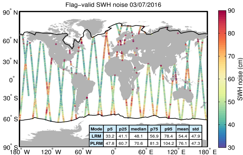
Figure 18. Geographical distribution of flag-valid 20-Hz SWH measurement noise over oceans and lakes for 03/07/2016. The statistical values shown in the table refer to the SWH noise and are calculated separately for LRM and PLRM regions. Measurements taken over polar polygons have been excluded from the computation of the statistical values. The black lines mark the outer limit of the Arctic and Antarctic polar polygons.
