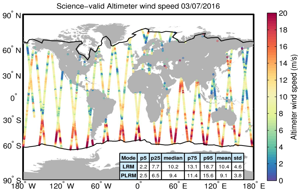
Figure 34. Geographical distribution of science-valid wind data over oceans and lakes for 03/07/2016. The statistical values shown in the table refer to the wind in m/s and are calculated separately for LRM and PLRM regions. The black lines mark the outer limit of the Arctic and Antarctic polar polygons. Gray circles denote records that have been rejected based on the editing criteria described in Table 5.
