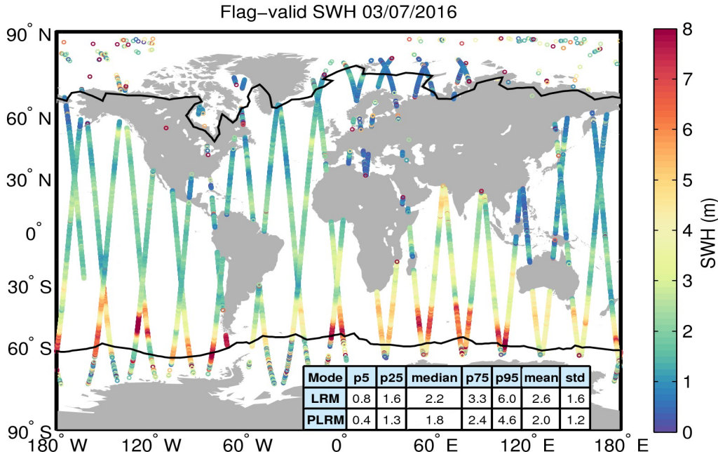
Figure 15. Geographical distribution of flag-valid SWH data over oceans and lakes for 03/07/2016. The statistical values shown in the table refer to the SWH in m and are calculated separately for LRM and PLRM regions. Measurements taken over polar polygons have been excluded from the computation of the statistical values. The black lines mark the outer limit of the Arctic and Antarctic polar polygons.
