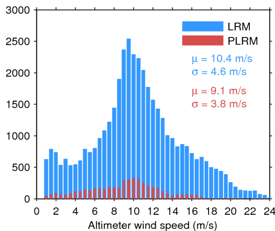
Figure 35. Histogram of science-valid wind over oceans and lakes for LRM (blue) and PLRM (red) for 03/07/2016. The mean ( \mu ) and standard deviation ( \sigma ) are also shown. Note that values larger than 24 m/s are excluded from the histogram for the sake of readability but not from the computation of \mu and \sigma .
