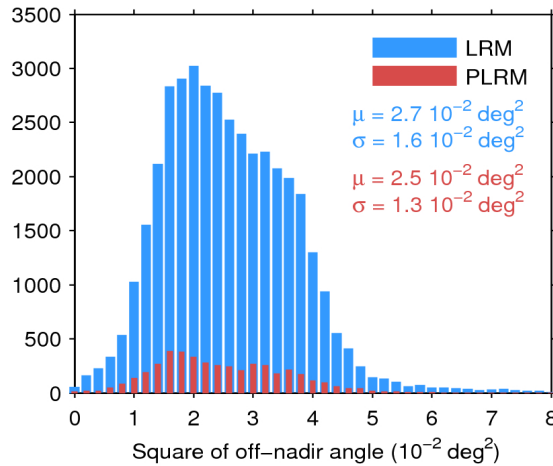
Figure 39. Histogram of flag-valid mispointing over oceans and lakes for LRM (blue) and PLRM (red) for 03/07/2016. Only positive values have been considered. The mean ( \mu ) and standard deviation ( \sigma ) are also shown. Note that values larger than 8 \cdot 10^{-2} \text{ deg}^2 are excluded from the histogram for the sake of readability but not from the computation of \mu and \sigma .
