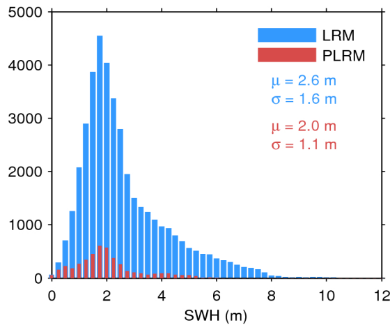
Figure 20. Histogram of science-valid SWH over oceans and lakes for LRM (blue) and PLRM (red) for 03/07/2016. The mean ( \mu ) and standard deviation ( \sigma ) are also shown. Note that values larger than 12 m are excluded from the histogram for the sake of readability but not from the computation of \mu and \sigma .
