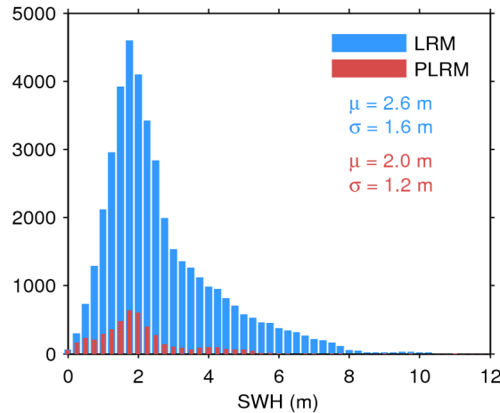
Figure 17. Histogram of flag-valid SWH over oceans and lakes for LRM (blue) and PLRM (red) for 03/07/2016. The mean ( \mu ) and standard deviation ( \sigma ) are also shown. Note that values larger than 12 m are excluded from the histogram for the sake of readability but not from the computation of \mu and \sigma .
