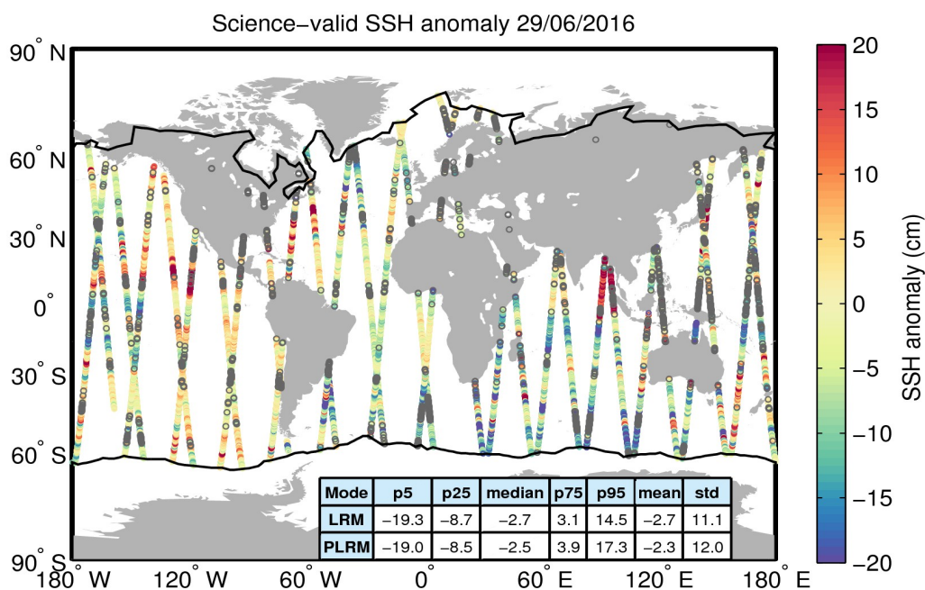
Figure 10. Geographical distribution of science-valid SSH anomaly data over oceans and lakes for 29/06/2016. The statistical values shown in the table refer to the SSH anomaly in cm and are calculated separately for LRM and PLRM regions. The black lines mark the outer limit of the Arctic and Antarctic polar polygons. Gray circles denote records that have been rejected based on the editing criteria described in Table 2.
