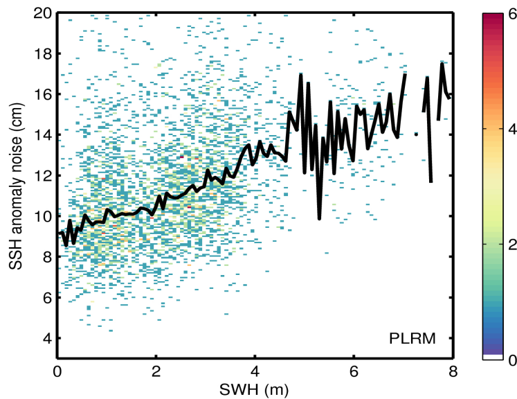
Figure 9. 2D histogram showing flag-valid SSH anomaly noise as a function of SWH for LRM (top) and PLRM (bottom) for 29/06/2016. The black line denotes the median SSH anomaly noise as a function of SWH.
