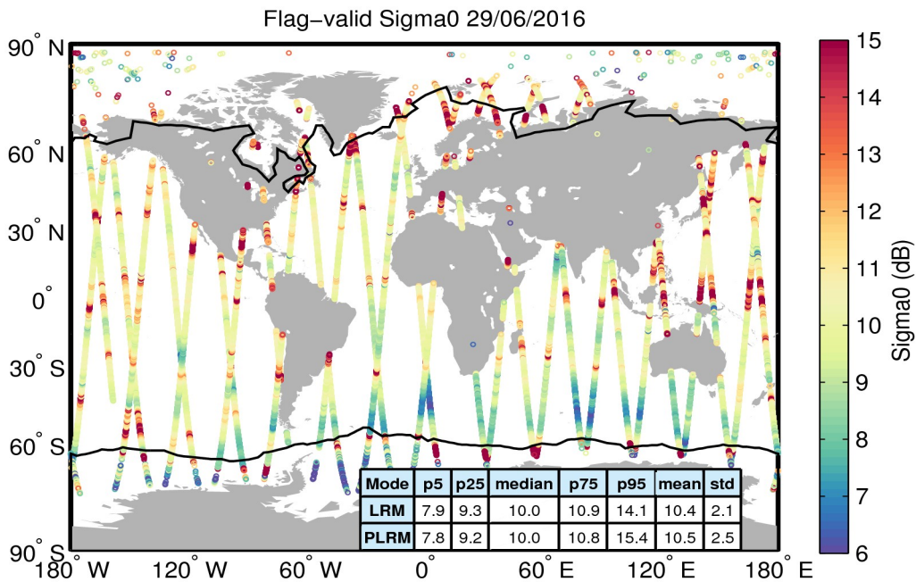
Figure 23. Geographical distribution of flag-valid sigma0 data over oceans and lakes for 29/06/2016. The statistical values shown in the table refer to the sigma0 in dB and are calculated separately for LRM and PLRM regions. Measurements taken over polar polygons have been excluded from the computation of the statistical values. The black lines mark the outer limit of the Arctic and Antarctic polar polygons.
