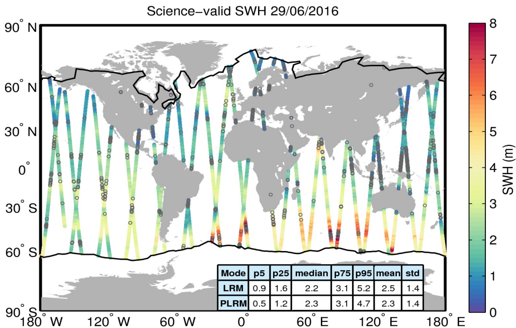
Figure 19. Geographical distribution of science-valid SWH data over oceans and lakes for 29/06/2016. The statistical values shown in the table refer to the SWH in m and are calculated separately for LRM and PLRM regions. The black lines mark the outer limit of the Arctic and Antarctic polar polygons. Gray circles denote records that have been rejected based on the editing criteria described in Table 3.
