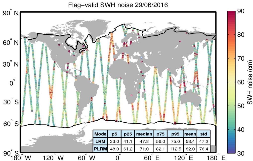
Figure 18. Geographical distribution of flag-valid 20-Hz SWH measurement noise over oceans and lakes for 29/06/2016. The statistical values shown in the table refer to the SWH noise and are calculated separately for LRM and PLRM regions. Measurements taken over polar polygons have been excluded from the computation of the statistical values. The black lines mark the outer limit of the Arctic and Antarctic polar polygons.
