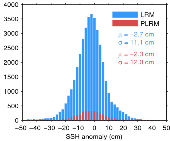
Figure 11. Histogram of science-valid SSH anomaly over oceans and lakes for LRM (blue) and PLRM (red) for 29/06/2016. The mean ( \mu ) and standard deviation ( \sigma ) are also shown. Note that values outside [-50 50] cm are excluded from the histogram for the sake of readability but not from the computation of \mu and \sigma .
