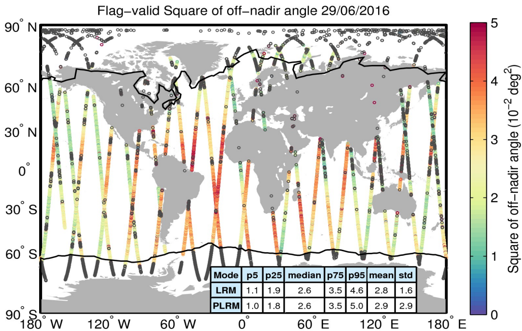
Figure 37. Geographical distribution of flag-valid mispointing data over oceans and lakes for 29/06/2016. The statistical values shown in the table refer to the mispointing in 10^{-2} deg 2 and are calculated separately for LRM and PLRM regions. Measurements taken over polar polygons have been excluded from the computation of the statistical values. The black lines mark the outer limit of the Arctic and Antarctic polar polygons. Gray circles denote negative values.
