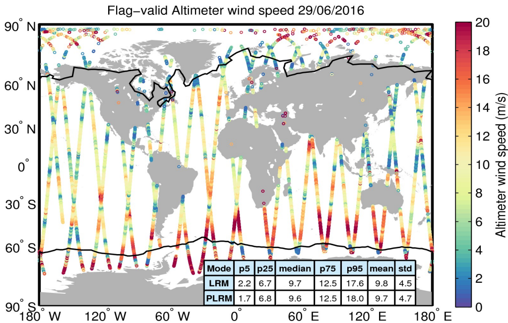
Figure 31. Geographical distribution of flag-valid wind data over oceans and lakes for 29/06/2016. The statistical values shown in the table refer to the wind in m/s and are calculated separately for LRM and PLRM regions. Measurements taken over polar polygons have been excluded from the computation of the statistical values. The black lines mark the outer limit of the Arctic and Antarctic polar polygons.
