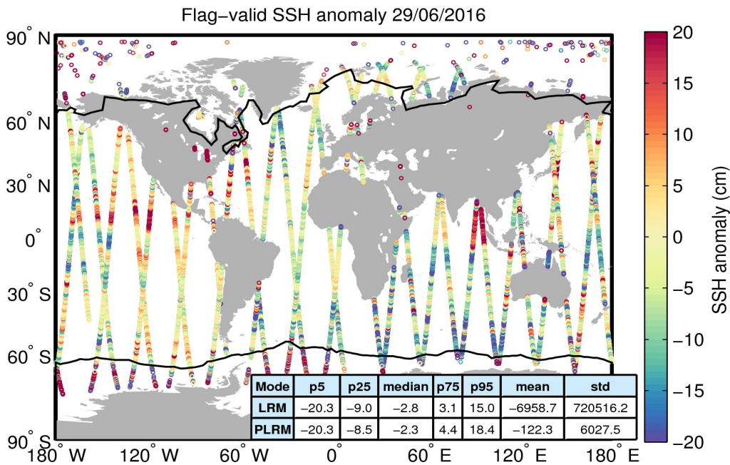
Figure 5. Geographical distribution of flag-valid 1-Hz SSH anomaly data over oceans and lakes for 29/06/2016. The statistical values shown in the table refer to the SSH anomaly in cm and are calculated separately for LRM and PLRM regions. Measurements taken over polar polygons have been excluded from the computation of the statistical values. The black lines mark the outer limit of the Arctic and Antarctic polar polygons.
