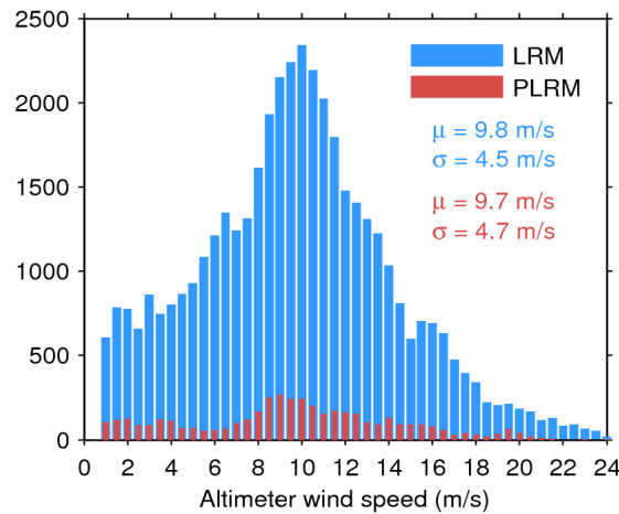
Figure 33. Histogram of flag-valid wind over oceans and lakes for LRM (blue) and PLRM (red) for 29/06/2016. The mean ( \mu ) and standard deviation ( \sigma ) are also shown. Note that values larger than 24 m/s are excluded from the histogram for the sake of readability but not from the computation of \mu and \sigma .
