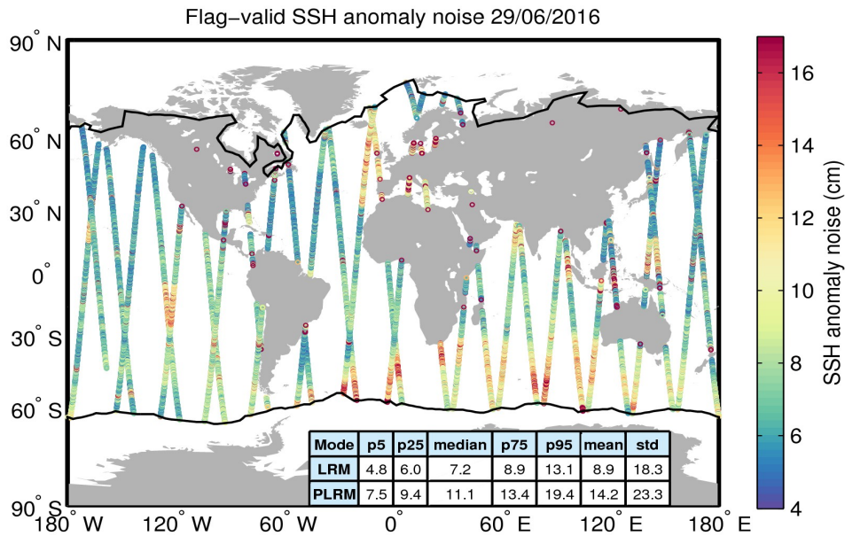
Figure 8. Geographical distribution of flag-valid 20-Hz SSH anomaly measurement noise over oceans and lakes for 29/06/2016. The statistical values shown in the table refer to the SSH anomaly noise and are calculated separately for LRM and PLRM regions. Measurements taken over polar polygons have been excluded from the computation of the statistical values. The black lines mark the outer limit of the Arctic and Antarctic polar polygons.
