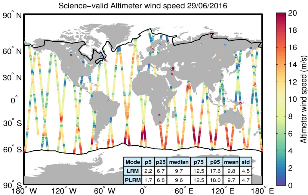
Figure 34. Geographical distribution of science-valid wind data over oceans and lakes for 29/06/2016. The statistical values shown in the table refer to the wind in m/s and are calculated separately for LRM and PLRM regions. The black lines mark the outer limit of the Arctic and Antarctic polar polygons. Gray circles denote records that have been rejected based on the editing criteria described in Table 5.
