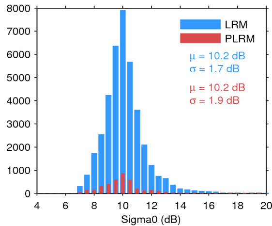
Figure 28. Histogram of science-valid sigma0 over oceans and lakes for LRM (blue) and PLRM (red) for 29/06/2016. The mean ( \mu ) and standard deviation ( \sigma ) are also shown. Note that values outside [4 20] dB are excluded from the histogram for the sake of readability but not from the computation of \mu and \sigma .
