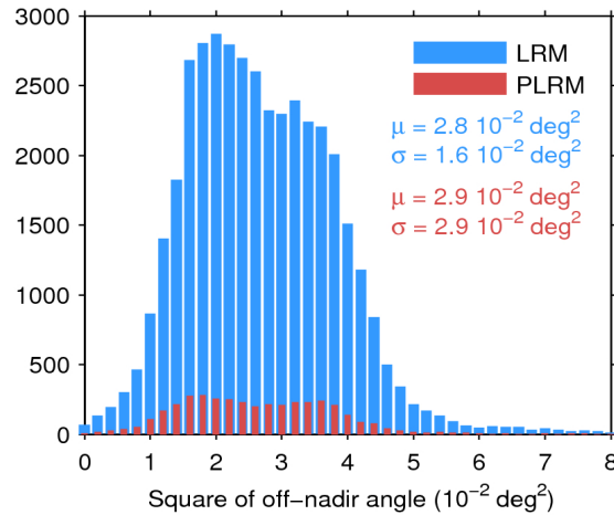
Figure 39. Histogram of flag-valid mispointing over oceans and lakes for LRM (blue) and PLRM (red) for 29/06/2016. Only positive values have been considered. The mean ( \mu ) and standard deviation ( \sigma ) are also shown. Note that values larger than 8 \cdot 10^{-2} \text{ deg}^2 are excluded from the histogram for the sake of readability but not from the computation of \mu and \sigma .
