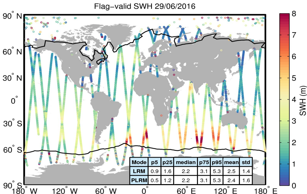
Figure 15. Geographical distribution of flag-valid SWH data over oceans and lakes for 29/06/2016. The statistical values shown in the table refer to the SWH in m and are calculated separately for LRM and PLRM regions. Measurements taken over polar polygons have been excluded from the computation of the statistical values. The black lines mark the outer limit of the Arctic and Antarctic polar polygons.
