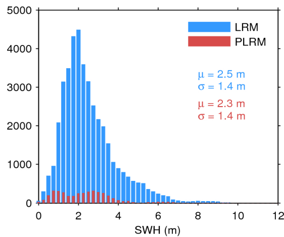
Figure 20. Histogram of science-valid SWH over oceans and lakes for LRM (blue) and PLRM (red) for 29/06/2016. The mean ( \mu ) and standard deviation ( \sigma ) are also shown. Note that values larger than 12 m are excluded from the histogram for the sake of readability but not from the computation of \mu and \sigma .
