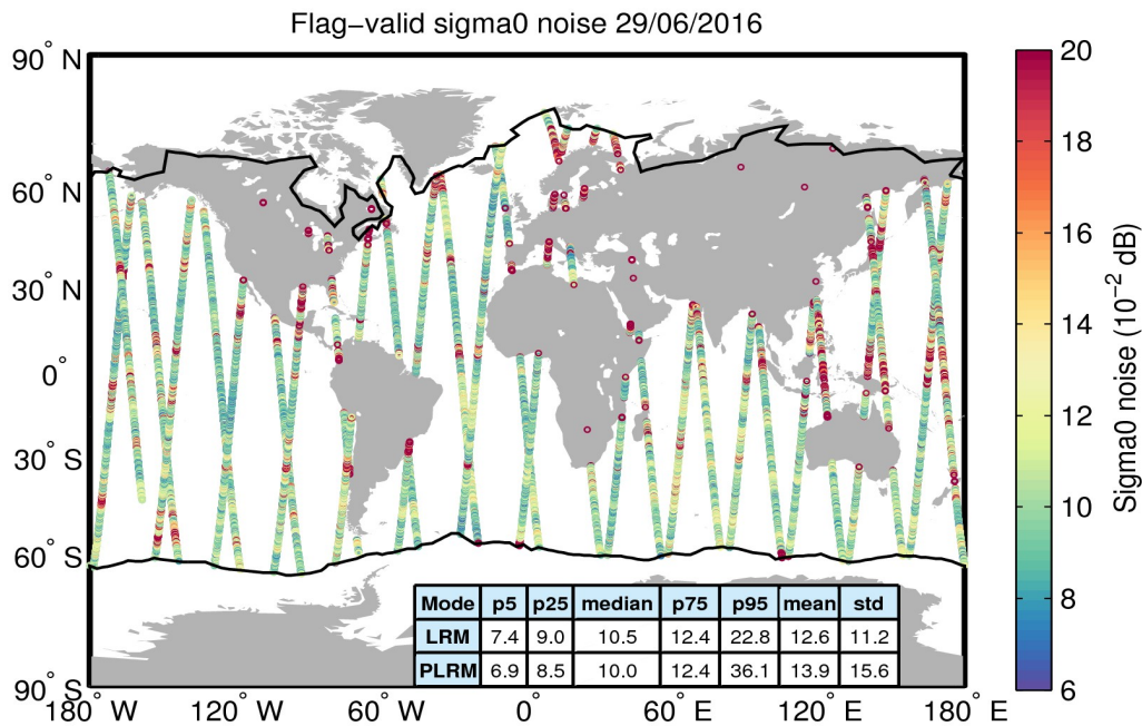
Figure 26. Geographical distribution of flag-valid 20-Hz sigma0 measurement noise over oceans and lakes for 29/06/2016. The statistical values shown in the table refer to the sigma0 noise and are calculated separately for LRM and PLRM regions. Measurements taken over polar polygons have been excluded from the computation of the statistical values. The black lines mark the outer limit of the Arctic and Antarctic polar polygons.
