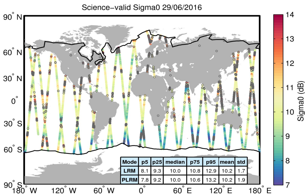
Figure 27. Geographical distribution of science-valid sigma0 data over oceans and lakes for 29/06/2016. The statistical values shown in the table refer to the sigma0 in dB and are calculated separately for LRM and PLRM regions. The black lines mark the outer limit of the Arctic and Antarctic polar polygons. Gray circles denote records that have been rejected based on the editing criteria described in Table 4.
