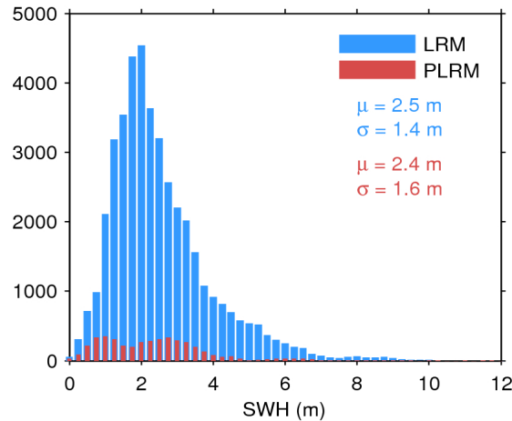
Figure 17. Histogram of flag-valid SWH over oceans and lakes for LRM (blue) and PLRM (red) for 29/06/2016. The mean ( \mu ) and standard deviation ( \sigma ) are also shown. Note that values larger than 12 m are excluded from the histogram for the sake of readability but not from the computation of \mu and \sigma .
