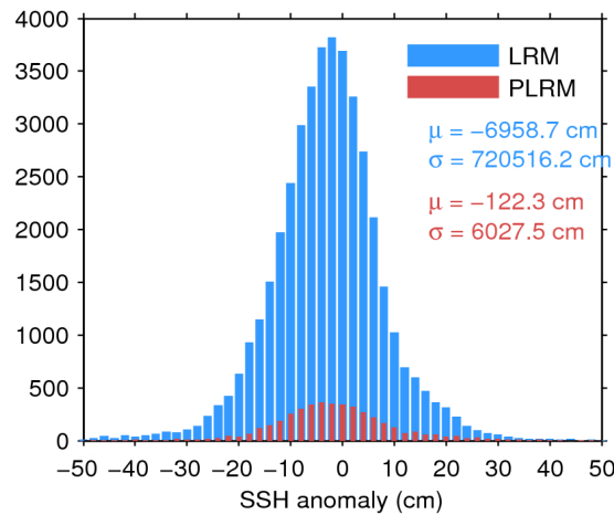
Figure 7. Histogram of flag-valid SSH anomaly over oceans and lakes for LRM (blue) and PLRM (red) for 29/06/2016. The mean ( \mu ) and standard deviation ( \sigma ) are also shown. Note that values outside [-50\ 50] cm are excluded from the histogram for the sake of readability but not from the computation of \mu and \sigma .
