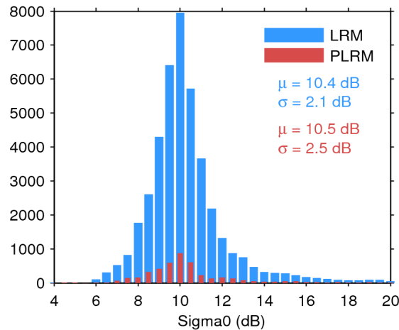
Figure 25. Histogram of flag-valid sigma0 over oceans and lakes for LRM (blue) and PLRM (red) for 29/06/2016. The mean ( \mu ) and standard deviation ( \sigma ) are also shown. Note that values outside [4 20] dB are excluded from the histogram for the sake of readability but not from the computation of \mu and \sigma .
