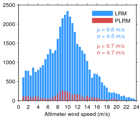
Figure 35. Histogram of science-valid wind over oceans and lakes for LRM (blue) and PLRM (red) for 29/06/2016. The mean ( \mu ) and standard deviation ( \sigma ) are also shown. Note that values larger than 24 m/s are excluded from the histogram for the sake of readability but not from the computation of \mu and \sigma .
