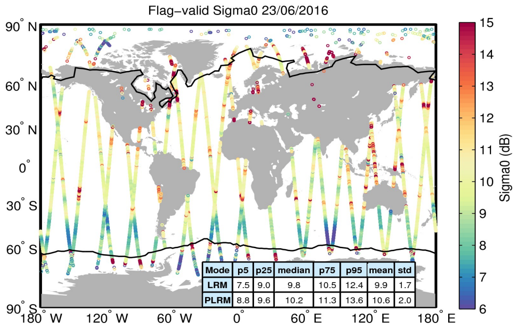
Figure 23. Geographical distribution of flag-valid sigma0 data over oceans and lakes for 23/06/2016. The statistical values shown in the table refer to the sigma0 in dB and are calculated separately for LRM and PLRM regions. Measurements taken over polar polygons have been excluded from the computation of the statistical values. The black lines mark the outer limit of the Arctic and Antarctic polar polygons.
