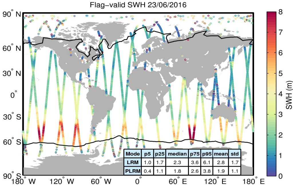
Figure 15. Geographical distribution of flag-valid SWH data over oceans and lakes for 23/06/2016. The statistical values shown in the table refer to the SWH in m and are calculated separately for LRM and PLRM regions. Measurements taken over polar polygons have been excluded from the computation of the statistical values. The black lines mark the outer limit of the Arctic and Antarctic polar polygons.
