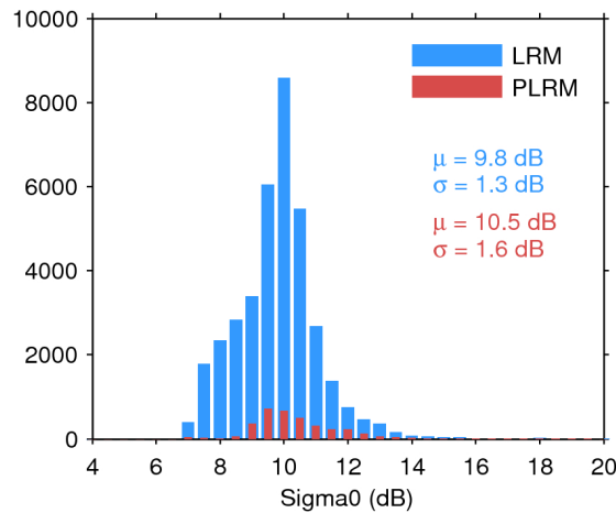
Figure 28. Histogram of science-valid sigma0 over oceans and lakes for LRM (blue) and PLRM (red) for 23/06/2016. The mean ( \mu ) and standard deviation ( \sigma ) are also shown. Note that values outside [4 20] dB are excluded from the histogram for the sake of readability but not from the computation of \mu and \sigma .
