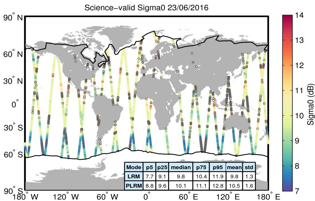
Figure 27. Geographical distribution of science-valid sigma0 data over oceans and lakes for 23/06/2016. The statistical values shown in the table refer to the sigma0 in dB and are calculated separately for LRM and PLRM regions. The black lines mark the outer limit of the Arctic and Antarctic polar polygons. Gray circles denote records that have been rejected based on the editing criteria described in Table 4.
