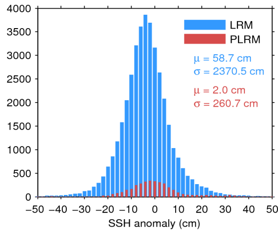
Figure 7. Histogram of flag-valid SSH anomaly over oceans and lakes for LRM (blue) and PLRM (red) for 23/06/2016. The mean ( \mu ) and standard deviation ( \sigma ) are also shown. Note that values outside [-50 \ 50] cm are excluded from the histogram for the sake of readability but not from the computation of \mu and \sigma .
