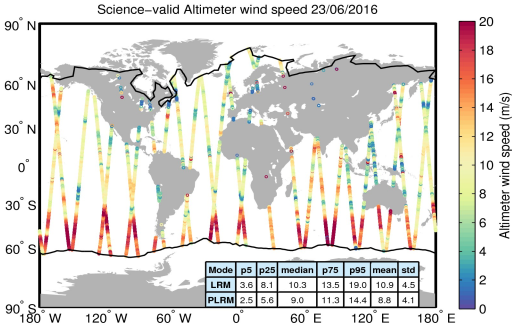
Figure 34. Geographical distribution of science-valid wind data over oceans and lakes for 23/06/2016. The statistical values shown in the table refer to the wind in m/s and are calculated separately for LRM and PLRM regions. The black lines mark the outer limit of the Arctic and Antarctic polar polygons. Gray circles denote records that have been rejected based on the editing criteria described in Table 5.
