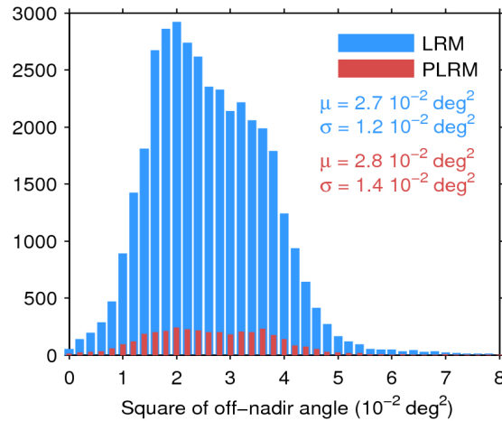
Figure 39. Histogram of flag-valid mispointing over oceans and lakes for LRM (blue) and PLRM (red) for 23/06/2016. Only positive values have been considered. The mean ( \mu ) and standard deviation ( \sigma ) are also shown. Note that values larger than 8 \cdot 10^{-2} \text{ deg}^2 are excluded from the histogram for the sake of readability but not from the computation of \mu and \sigma .
