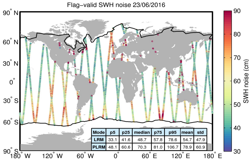
Figure 18. Geographical distribution of flag-valid 20-Hz SWH measurement noise over oceans and lakes for 23/06/2016. The statistical values shown in the table refer to the SWH noise and are calculated separately for LRM and PLRM regions. Measurements taken over polar polygons have been excluded from the computation of the statistical values. The black lines mark the outer limit of the Arctic and Antarctic polar polygons.
