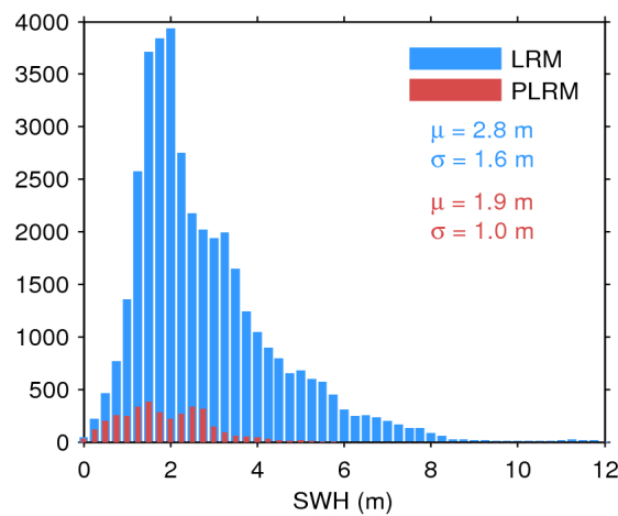
Figure 20. Histogram of science-valid SWH over oceans and lakes for LRM (blue) and PLRM (red) for 23/06/2016. The mean ( \mu ) and standard deviation ( \sigma ) are also shown. Note that values larger than 12 m are excluded from the histogram for the sake of readability but not from the computation of \mu and \sigma .
