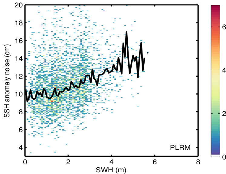
Figure 9. 2D histogram showing flag-valid SSH anomaly noise as a function of SWH for LRM (top) and PLRM (bottom) for 23/06/2016. The black line denotes the median SSH anomaly noise as a function of SWH.
