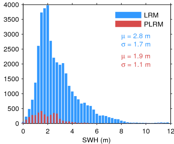
Figure 17. Histogram of flag-valid SWH over oceans and lakes for LRM (blue) and PLRM (red) for 23/06/2016. The mean ( \mu ) and standard deviation ( \sigma ) are also shown. Note that values larger than 12 m are excluded from the histogram for the sake of readability but not from the computation of \mu and \sigma .
