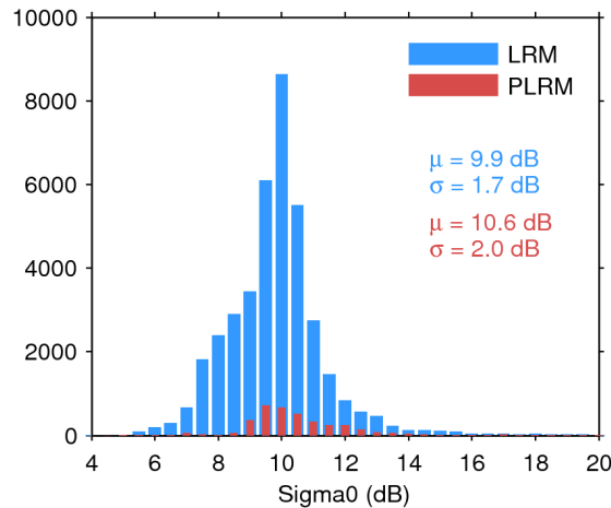
Figure 25. Histogram of flag-valid sigma0 over oceans and lakes for LRM (blue) and PLRM (red) for 23/06/2016. The mean ( \mu ) and standard deviation ( \sigma ) are also shown. Note that values outside [4 20] dB are excluded from the histogram for the sake of readability but not from the computation of \mu and \sigma .
