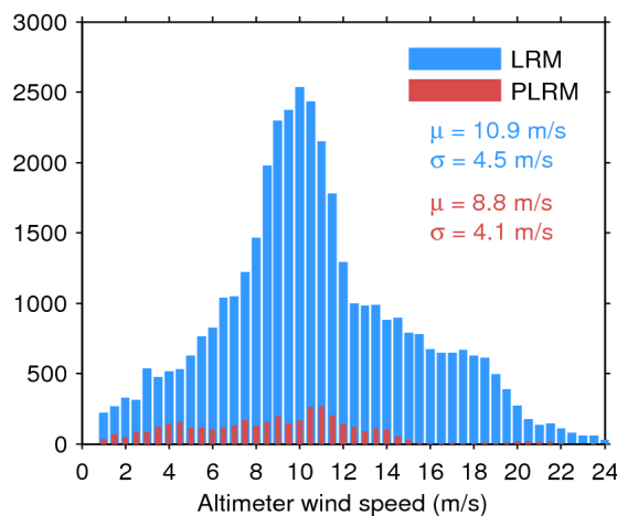
Figure 35. Histogram of science-valid wind over oceans and lakes for LRM (blue) and PLRM (red) for 23/06/2016. The mean ( \mu ) and standard deviation ( \sigma ) are also shown. Note that values larger than 24 m/s are excluded from the histogram for the sake of readability but not from the computation of \mu and \sigma .
