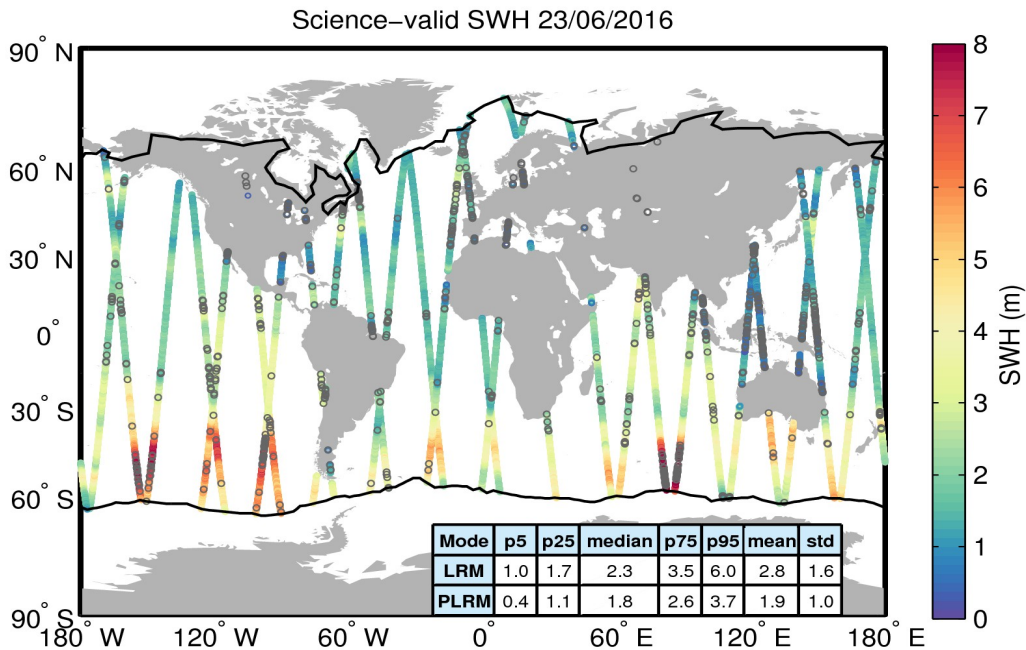
Figure 19. Geographical distribution of science-valid SWH data over oceans and lakes for 23/06/2016. The statistical values shown in the table refer to the SWH in m and are calculated separately for LRM and PLRM regions. The black lines mark the outer limit of the Arctic and Antarctic polar polygons. Gray circles denote records that have been rejected based on the editing criteria described in Table 3.
