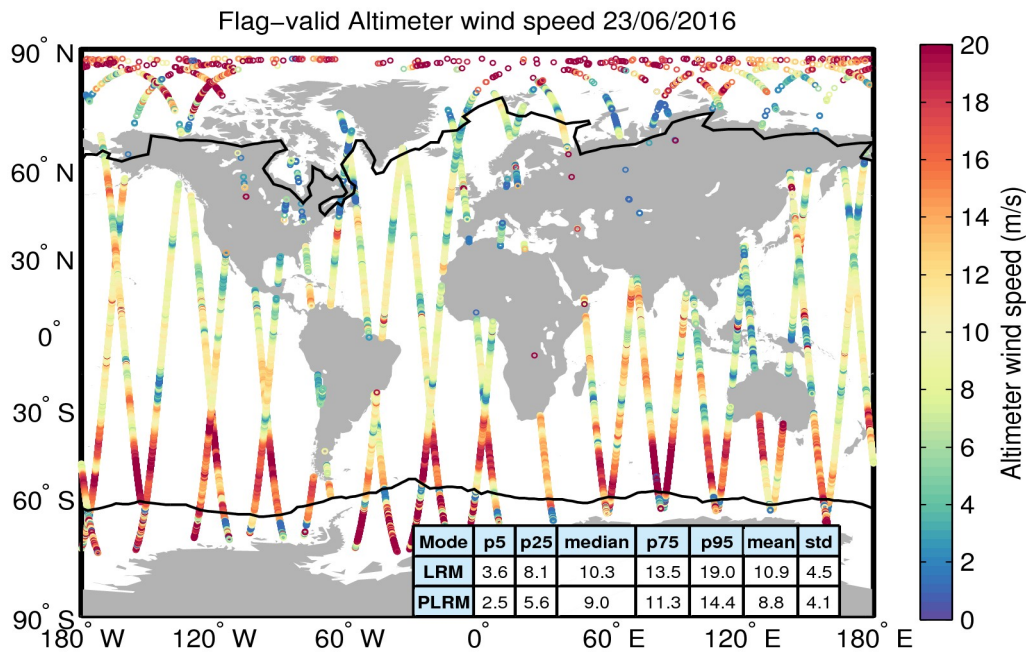
Figure 31. Geographical distribution of flag-valid wind data over oceans and lakes for 23/06/2016. The statistical values shown in the table refer to the wind in m/s and are calculated separately for LRM and PLRM regions. Measurements taken over polar polygons have been excluded from the computation of the statistical values. The black lines mark the outer limit of the Arctic and Antarctic polar polygons.
