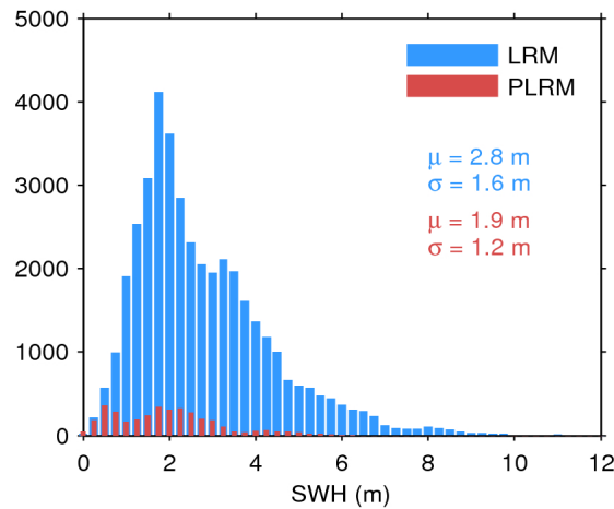
Figure 20. Histogram of science-valid SWH over oceans and lakes for LRM (blue) and PLRM (red) for 22/06/2016. The mean ( \mu ) and standard deviation ( \sigma ) are also shown. Note that values larger than 12 m are excluded from the histogram for the sake of readability but not from the computation of \mu and \sigma .
