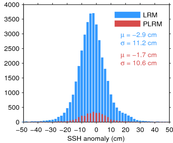
Figure 11. Histogram of science-valid SSH anomaly over oceans and lakes for LRM (blue) and PLRM (red) for 22/06/2016. The mean ( \mu ) and standard deviation ( \sigma ) are also shown. Note that values outside [-50 50] cm are excluded from the histogram for the sake of readability but not from the computation of \mu and \sigma .
