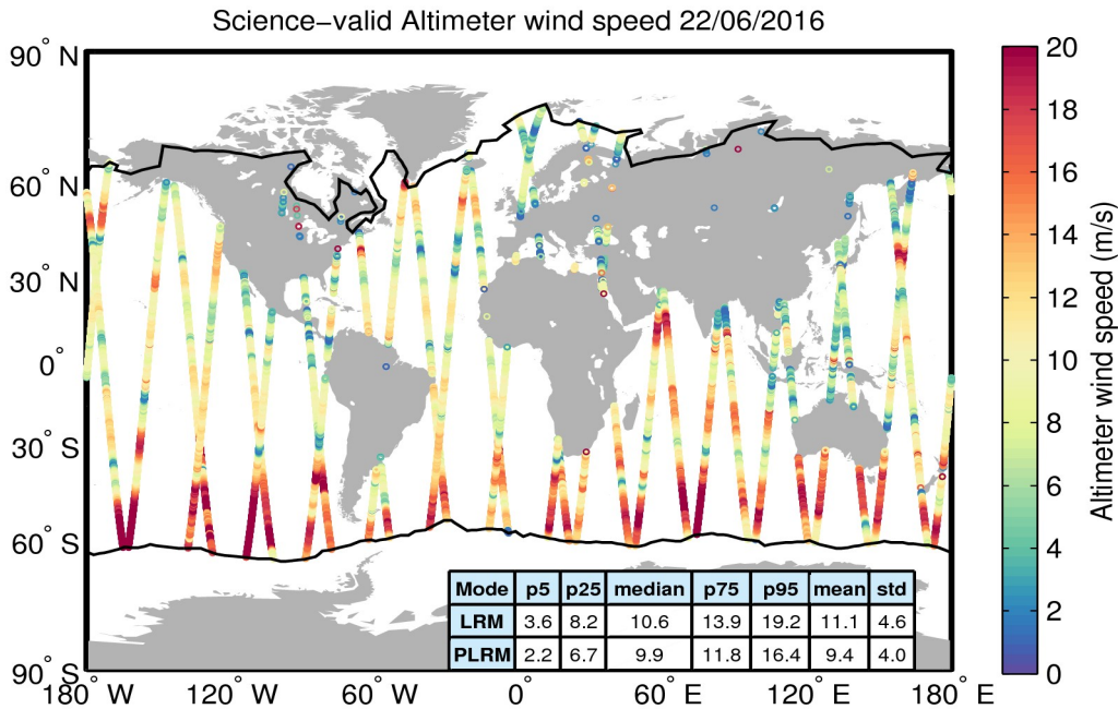
Figure 34. Geographical distribution of science-valid wind data over oceans and lakes for 22/06/2016. The statistical values shown in the table refer to the wind in m/s and are calculated separately for LRM and PLRM regions. The black lines mark the outer limit of the Arctic and Antarctic polar polygons. Gray circles denote records that have been rejected based on the editing criteria described in Table 5.
