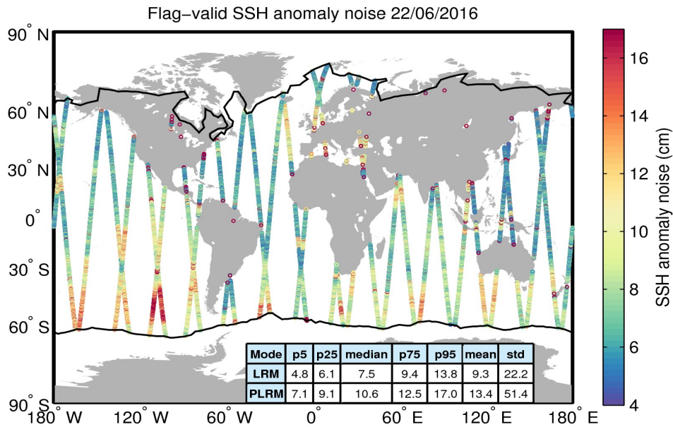
Figure 8. Geographical distribution of flag-valid 20-Hz SSH anomaly measurement noise over oceans and lakes for 22/06/2016. The statistical values shown in the table refer to the SSH anomaly noise and are calculated separately for LRM and PLRM regions. Measurements taken over polar polygons have been excluded from the computation of the statistical values. The black lines mark the outer limit of the Arctic and Antarctic polar polygons.
