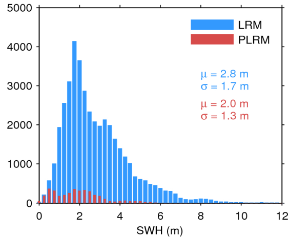
Figure 17. Histogram of flag-valid SWH over oceans and lakes for LRM (blue) and PLRM (red) for 22/06/2016. The mean ( \mu ) and standard deviation ( \sigma ) are also shown. Note that values larger than 12 m are excluded from the histogram for the sake of readability but not from the computation of \mu and \sigma .
