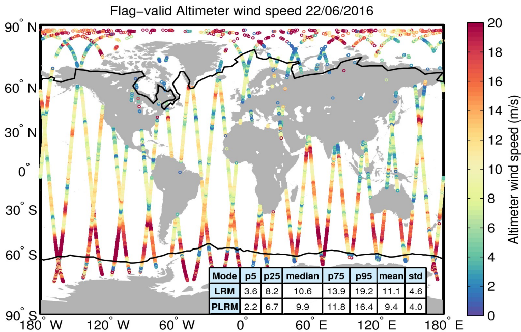
Figure 31. Geographical distribution of flag-valid wind data over oceans and lakes for 22/06/2016. The statistical values shown in the table refer to the wind in m/s and are calculated separately for LRM and PLRM regions. Measurements taken over polar polygons have been excluded from the computation of the statistical values. The black lines mark the outer limit of the Arctic and Antarctic polar polygons.
