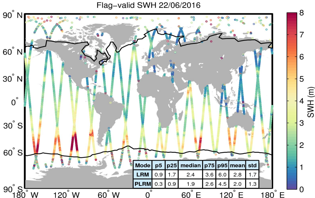
Figure 15. Geographical distribution of flag-valid SWH data over oceans and lakes for 22/06/2016. The statistical values shown in the table refer to the SWH in m and are calculated separately for LRM and PLRM regions. Measurements taken over polar polygons have been excluded from the computation of the statistical values. The black lines mark the outer limit of the Arctic and Antarctic polar polygons.
