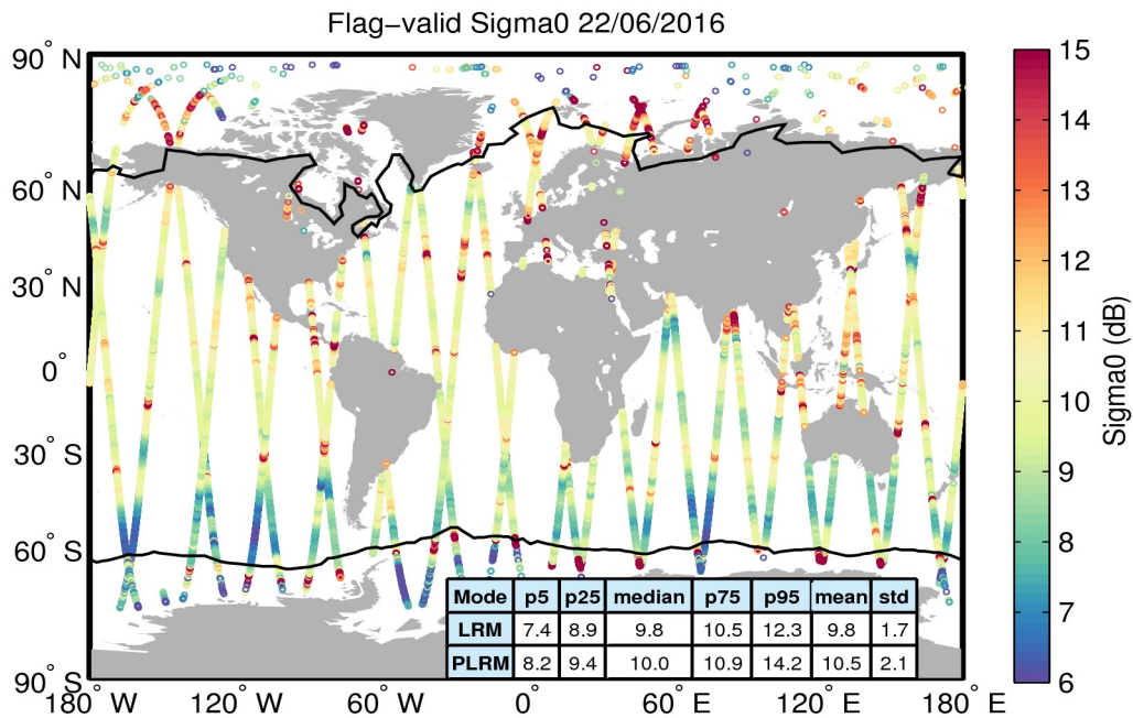
Figure 23. Geographical distribution of flag-valid sigma0 data over oceans and lakes for 22/06/2016. The statistical values shown in the table refer to the sigma0 in dB and are calculated separately for LRM and PLRM regions. Measurements taken over polar polygons have been excluded from the computation of the statistical values. The black lines mark the outer limit of the Arctic and Antarctic polar polygons.
