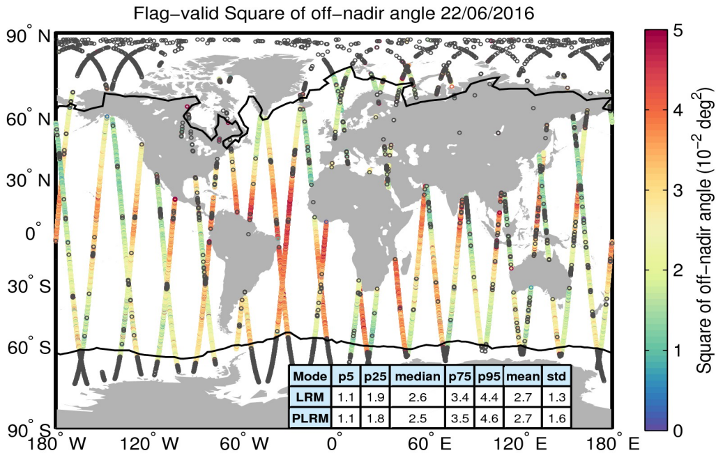
Figure 37. Geographical distribution of flag-valid mispointing data over oceans and lakes for 22/06/2016. The statistical values shown in the table refer to the mispointing in 10^{-2} deg 2 and are calculated separately for LRM and PLRM regions. Measurements taken over polar polygons have been excluded from the computation of the statistical values. The black lines mark the outer limit of the Arctic and Antarctic polar polygons. Gray circles denote negative values.
