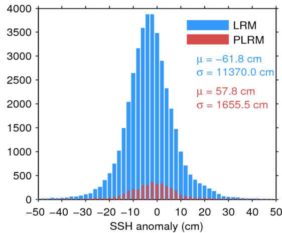
Figure 7. Histogram of flag-valid SSH anomaly over oceans and lakes for LRM (blue) and PLRM (red) for 22/06/2016. The mean ( \mu ) and standard deviation ( \sigma ) are also shown. Note that values outside [-50 50] cm are excluded from the histogram for the sake of readability but not from the computation of \mu and \sigma .
