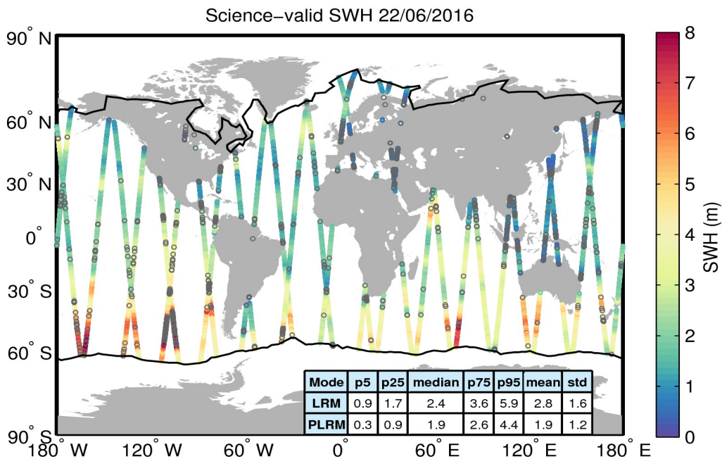
Figure 19. Geographical distribution of science-valid SWH data over oceans and lakes for 22/06/2016. The statistical values shown in the table refer to the SWH in m and are calculated separately for LRM and PLRM regions. The black lines mark the outer limit of the Arctic and Antarctic polar polygons. Gray circles denote records that have been rejected based on the editing criteria described in Table 3.
