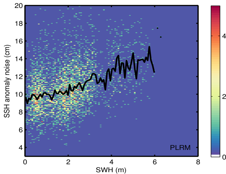
Figure 9. 2D histogram showing flag-valid SSH anomaly noise as a function of SWH for LRM (top) and PLRM (bottom) for 22/06/2016. The black line denotes the median SSH anomaly noise as a function of SWH.
