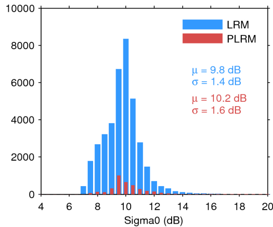
Figure 28. Histogram of science-valid sigma0 over oceans and lakes for LRM (blue) and PLRM (red) for 22/06/2016. The mean ( \mu ) and standard deviation ( \sigma ) are also shown. Note that values outside [4 20] dB are excluded from the histogram for the sake of readability but not from the computation of \mu and \sigma .
