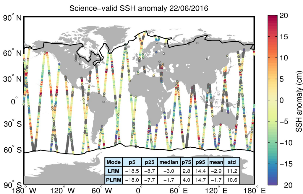
Figure 10. Geographical distribution of science-valid SSH anomaly data over oceans and lakes for 22/06/2016. The statistical values shown in the table refer to the SSH anomaly in cm and are calculated separately for LRM and PLRM regions. The black lines mark the outer limit of the Arctic and Antarctic polar polygons. Gray circles denote records that have been rejected based on the editing criteria described in Table 2.
