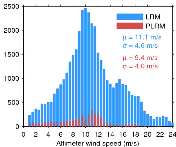
Figure 35. Histogram of science-valid wind over oceans and lakes for LRM (blue) and PLRM (red) for 22/06/2016. The mean ( \mu ) and standard deviation ( \sigma ) are also shown. Note that values larger than 24 m/s are excluded from the histogram for the sake of readability but not from the computation of \mu and \sigma .
