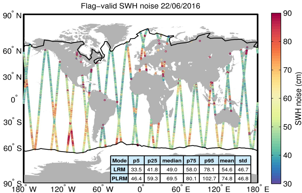
Figure 18. Geographical distribution of flag-valid 20-Hz SWH measurement noise over oceans and lakes for 22/06/2016. The statistical values shown in the table refer to the SWH noise and are calculated separately for LRM and PLRM regions. Measurements taken over polar polygons have been excluded from the computation of the statistical values. The black lines mark the outer limit of the Arctic and Antarctic polar polygons.
