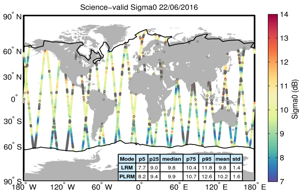
Figure 27. Geographical distribution of science-valid sigma0 data over oceans and lakes for 22/06/2016. The statistical values shown in the table refer to the sigma0 in dB and are calculated separately for LRM and PLRM regions. The black lines mark the outer limit of the Arctic and Antarctic polar polygons. Gray circles denote records that have been rejected based on the editing criteria described in Table 4.
