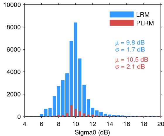
Figure 25. Histogram of flag-valid sigma0 over oceans and lakes for LRM (blue) and PLRM (red) for 22/06/2016. The mean ( \mu ) and standard deviation ( \sigma ) are also shown. Note that values outside [4 20] dB are excluded from the histogram for the sake of readability but not from the computation of \mu and \sigma .
