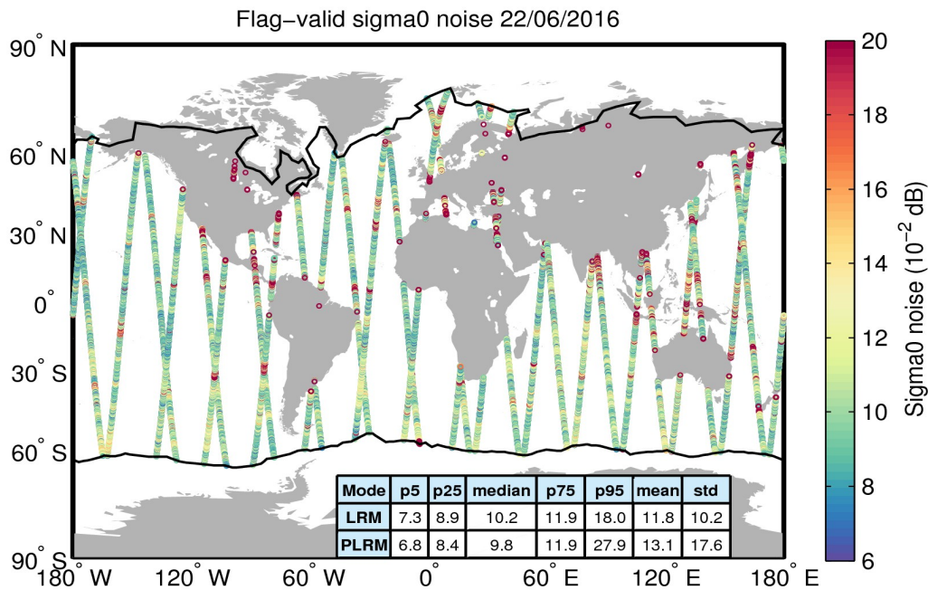
Figure 26. Geographical distribution of flag-valid 20-Hz sigma0 measurement noise over oceans and lakes for 22/06/2016. The statistical values shown in the table refer to the sigma0 noise and are calculated separately for LRM and PLRM regions. Measurements taken over polar polygons have been excluded from the computation of the statistical values. The black lines mark the outer limit of the Arctic and Antarctic polar polygons.
