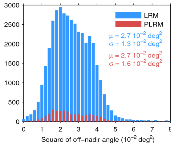
Figure 39. Histogram of flag-valid mispointing over oceans and lakes for LRM (blue) and PLRM (red) for 22/06/2016. Only positive values have been considered. The mean ( \mu ) and standard deviation ( \sigma ) are also shown. Note that values larger than 8 \cdot 10^{-2} \text{ deg}^2 are excluded from the histogram for the sake of readability but not from the computation of \mu and \sigma .
