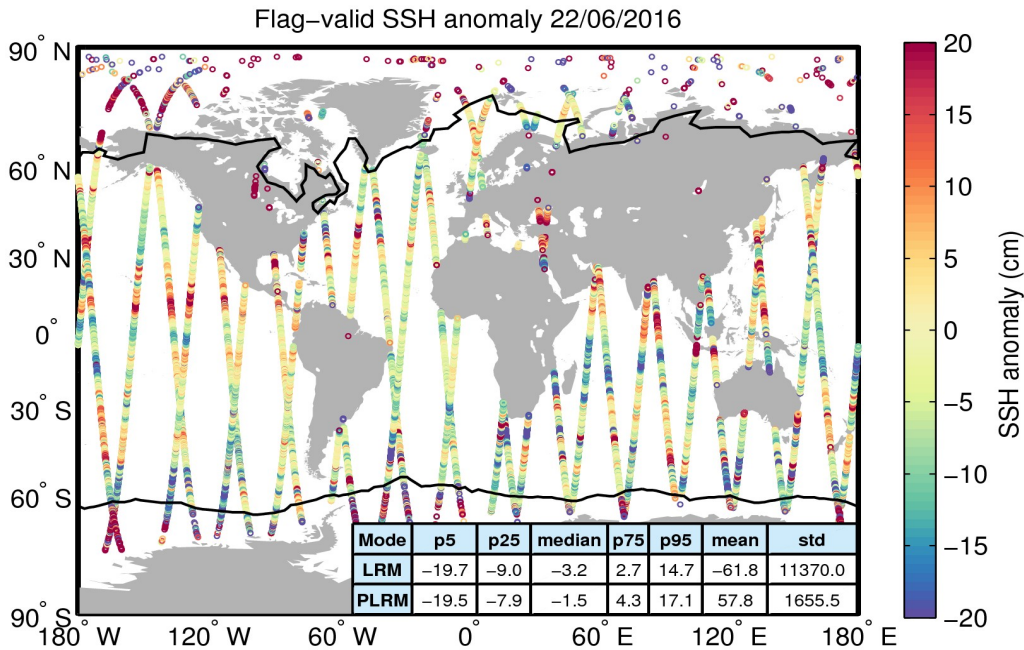
Figure 5. Geographical distribution of flag-valid 1-Hz SSH anomaly data over oceans and lakes for 22/06/2016. The statistical values shown in the table refer to the SSH anomaly in cm and are calculated separately for LRM and PLRM regions. Measurements taken over polar polygons have been excluded from the computation of the statistical values. The black lines mark the outer limit of the Arctic and Antarctic polar polygons.
