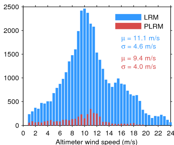
Figure 33. Histogram of flag-valid wind over oceans and lakes for LRM (blue) and PLRM (red) for 22/06/2016. The mean ( \mu ) and standard deviation ( \sigma ) are also shown. Note that values larger than 24 m/s are excluded from the histogram for the sake of readability but not from the computation of \mu and \sigma .
