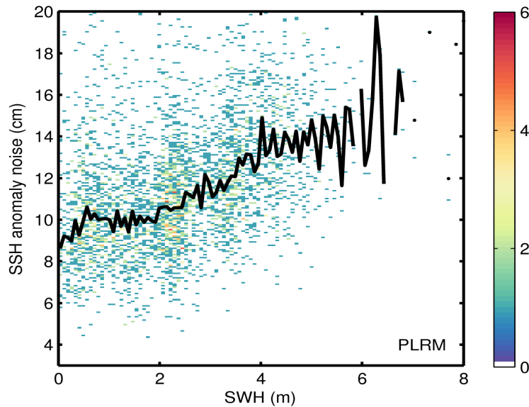
Figure 9. 2D histogram showing flag-valid SSH anomaly noise as a function of SWH for LRM (top) and PLRM (bottom) for 20/06/2016. The black line denotes the median SSH anomaly noise as a function of SWH.
