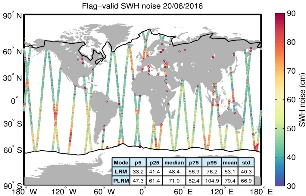
Figure 18. Geographical distribution of flag-valid 20-Hz SWH measurement noise over oceans and lakes for 20/06/2016. The statistical values shown in the table refer to the SWH noise and are calculated separately for LRM and PLRM regions. Measurements taken over polar polygons have been excluded from the computation of the statistical values. The black lines mark the outer limit of the Arctic and Antarctic polar polygons.
