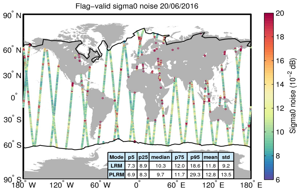
Figure 26. Geographical distribution of flag-valid 20-Hz sigma0 measurement noise over oceans and lakes for 20/06/2016. The statistical values shown in the table refer to the sigma0 noise and are calculated separately for LRM and PLRM regions. Measurements taken over polar polygons have been excluded from the computation of the statistical values. The black lines mark the outer limit of the Arctic and Antarctic polar polygons.
