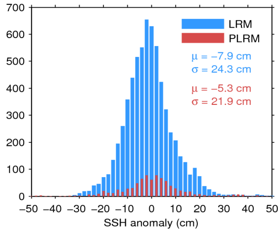
Figure 11. Histogram of science-valid SSH anomaly over oceans and lakes for LRM (blue) and PLRM (red) for 20/06/2016. The mean ( \mu ) and standard deviation ( \sigma ) are also shown. Note that values outside [-50 50] cm are excluded from the histogram for the sake of readability but not from the computation of \mu and \sigma .
