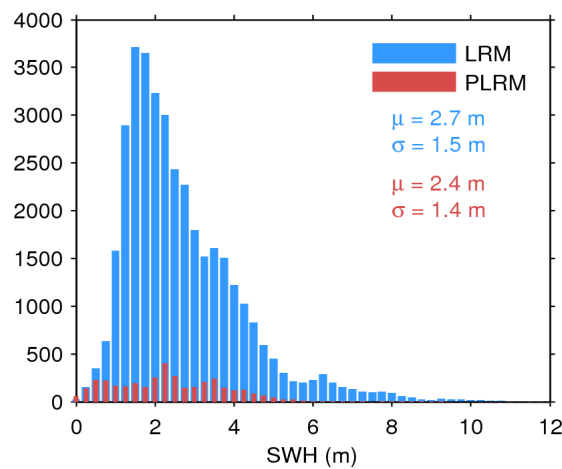
Figure 20. Histogram of science-valid SWH over oceans and lakes for LRM (blue) and PLRM (red) for 20/06/2016. The mean ( \mu ) and standard deviation ( \sigma ) are also shown. Note that values larger than 12 m are excluded from the histogram for the sake of readability but not from the computation of \mu and \sigma .
