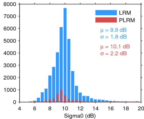
Figure 25. Histogram of flag-valid sigma0 over oceans and lakes for LRM (blue) and PLRM (red) for 20/06/2016. The mean ( \mu ) and standard deviation ( \sigma ) are also shown. Note that values outside [4 20] dB are excluded from the histogram for the sake of readability but not from the computation of \mu and \sigma .
