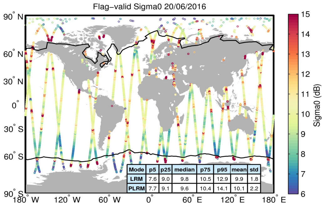
Figure 23. Geographical distribution of flag-valid sigma0 data over oceans and lakes for 20/06/2016. The statistical values shown in the table refer to the sigma0 in dB and are calculated separately for LRM and PLRM regions. Measurements taken over polar polygons have been excluded from the computation of the statistical values. The black lines mark the outer limit of the Arctic and Antarctic polar polygons.
