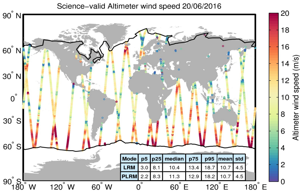
Figure 34. Geographical distribution of science-valid wind data over oceans and lakes for 20/06/2016. The statistical values shown in the table refer to the wind in m/s and are calculated separately for LRM and PLRM regions. The black lines mark the outer limit of the Arctic and Antarctic polar polygons. Gray circles denote records that have been rejected based on the editing criteria described in Table 5.
