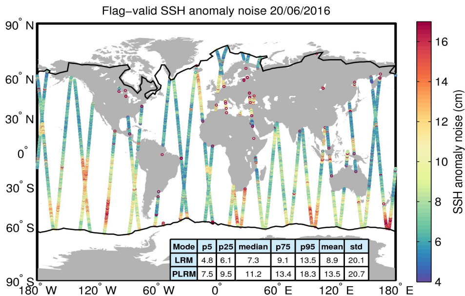
Figure 8. Geographical distribution of flag-valid 20-Hz SSH anomaly measurement noise over oceans and lakes for 20/06/2016. The statistical values shown in the table refer to the SSH anomaly noise and are calculated separately for LRM and PLRM regions. Measurements taken over polar polygons have been excluded from the computation of the statistical values. The black lines mark the outer limit of the Arctic and Antarctic polar polygons.
