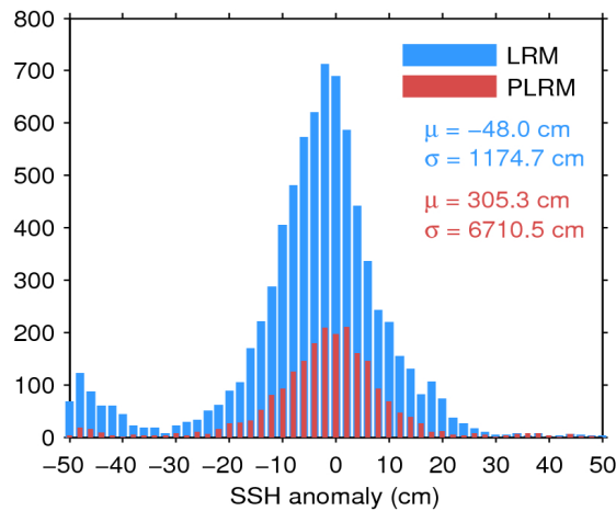
Figure 7. Histogram of flag-valid SSH anomaly over oceans and lakes for LRM (blue) and PLRM (red) for 20/06/2016. The mean ( \mu ) and standard deviation ( \sigma ) are also shown. Note that values outside [-50\ 50] cm are excluded from the histogram for the sake of readability but not from the computation of \mu and \sigma .
