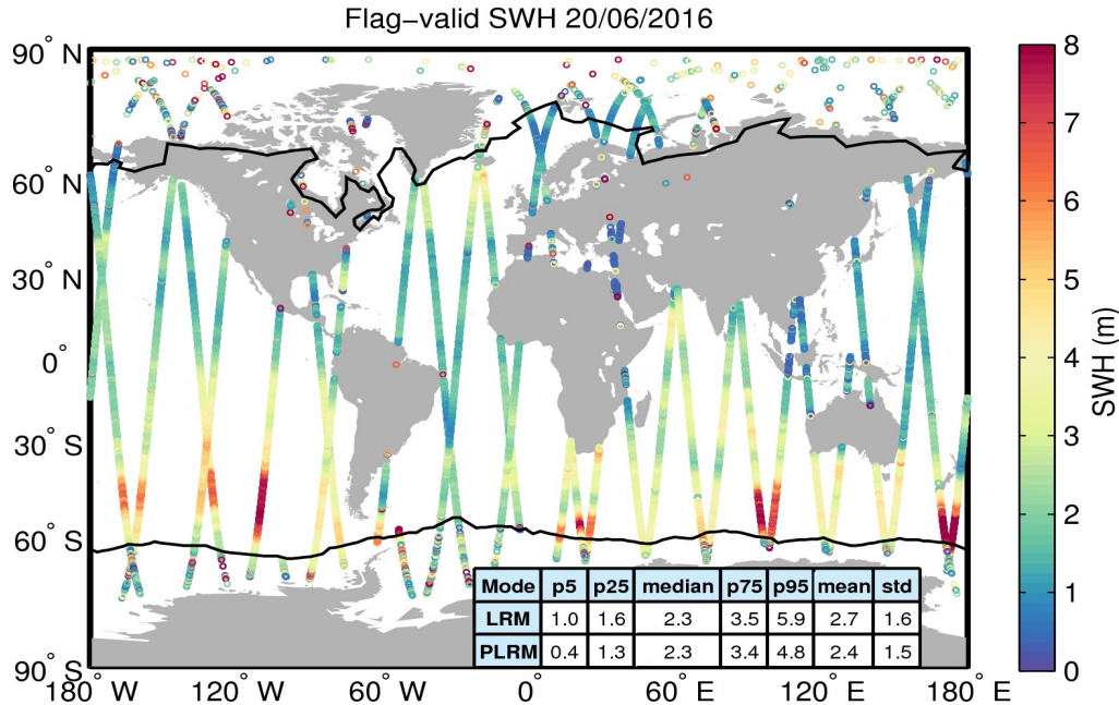
Figure 15. Geographical distribution of flag-valid SWH data over oceans and lakes for 20/06/2016. The statistical values shown in the table refer to the SWH in m and are calculated separately for LRM and PLRM regions. Measurements taken over polar polygons have been excluded from the computation of the statistical values. The black lines mark the outer limit of the Arctic and Antarctic polar polygons.
