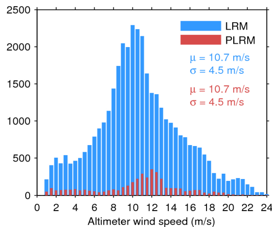
Figure 35. Histogram of science-valid wind over oceans and lakes for LRM (blue) and PLRM (red) for 20/06/2016. The mean ( \mu ) and standard deviation ( \sigma ) are also shown. Note that values larger than 24 m/s are excluded from the histogram for the sake of readability but not from the computation of \mu and \sigma .
