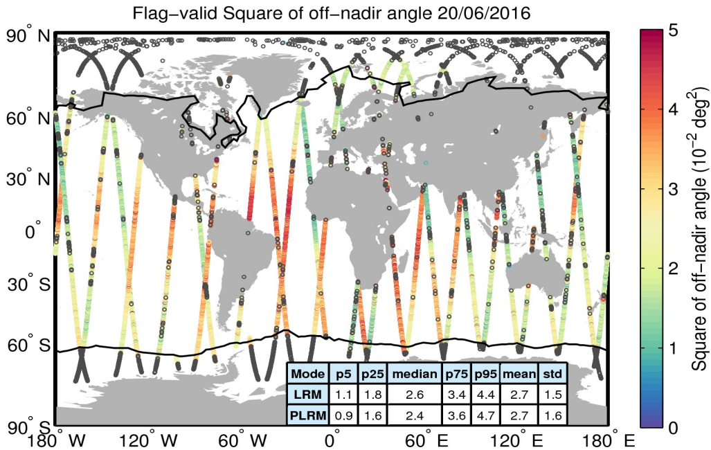
Figure 37. Geographical distribution of flag-valid mispointing data over oceans and lakes for 20/06/2016. The statistical values shown in the table refer to the mispointing in 10^{-2} deg 2 and are calculated separately for LRM and PLRM regions. Measurements taken over polar polygons have been excluded from the computation of the statistical values. The black lines mark the outer limit of the Arctic and Antarctic polar polygons. Gray circles denote negative values.
