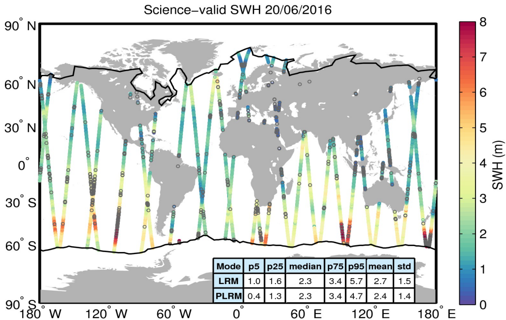
Figure 19. Geographical distribution of science-valid SWH data over oceans and lakes for 20/06/2016. The statistical values shown in the table refer to the SWH in m and are calculated separately for LRM and PLRM regions. The black lines mark the outer limit of the Arctic and Antarctic polar polygons. Gray circles denote records that have been rejected based on the editing criteria described in Table 3.
