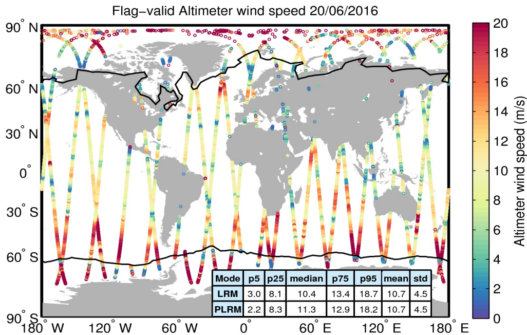
Figure 31. Geographical distribution of flag-valid wind data over oceans and lakes for 20/06/2016. The statistical values shown in the table refer to the wind in m/s and are calculated separately for LRM and PLRM regions. Measurements taken over polar polygons have been excluded from the computation of the statistical values. The black lines mark the outer limit of the Arctic and Antarctic polar polygons.
