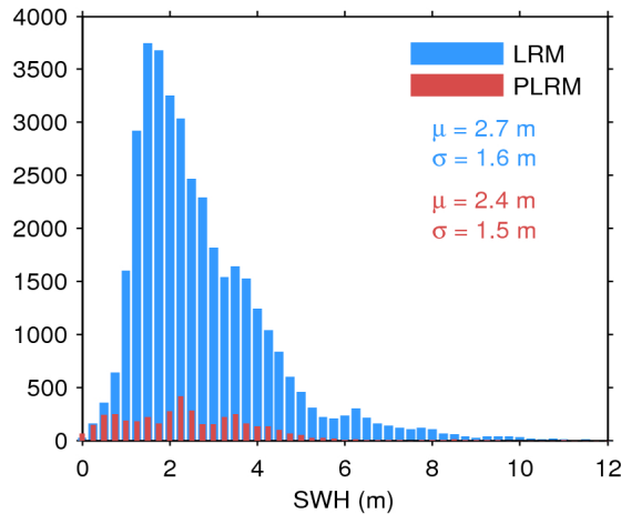
Figure 17. Histogram of flag-valid SWH over oceans and lakes for LRM (blue) and PLRM (red) for 20/06/2016. The mean ( \mu ) and standard deviation ( \sigma ) are also shown. Note that values larger than 12 m are excluded from the histogram for the sake of readability but not from the computation of \mu and \sigma .
