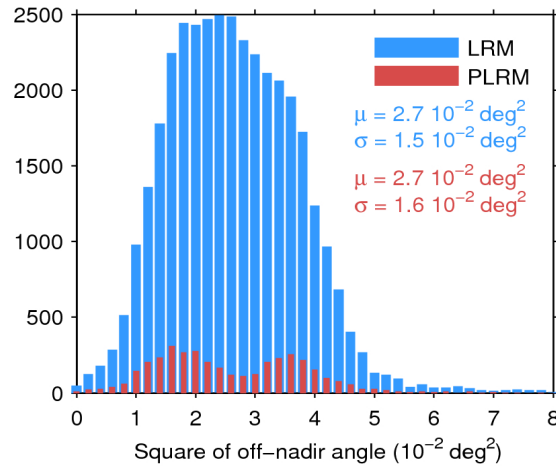
Figure 39. Histogram of flag-valid mispointing over oceans and lakes for LRM (blue) and PLRM (red) for 20/06/2016. Only positive values have been considered. The mean ( \mu ) and standard deviation ( \sigma ) are also shown. Note that values larger than 8 \cdot 10^{-2} \text{ deg}^2 are excluded from the histogram for the sake of readability but not from the computation of \mu and \sigma .
