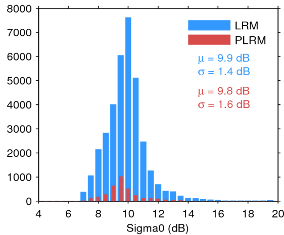
Figure 28. Histogram of science-valid sigma0 over oceans and lakes for LRM (blue) and PLRM (red) for 20/06/2016. The mean ( \mu ) and standard deviation ( \sigma ) are also shown. Note that values outside [4 20] dB are excluded from the histogram for the sake of readability but not from the computation of \mu and \sigma .
