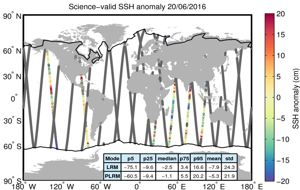
Figure 10. Geographical distribution of science-valid SSH anomaly data over oceans and lakes for 20/06/2016. The statistical values shown in the table refer to the SSH anomaly in cm and are calculated separately for LRM and PLRM regions. The black lines mark the outer limit of the Arctic and Antarctic polar polygons. Gray circles denote records that have been rejected based on the editing criteria described in Table 2.
