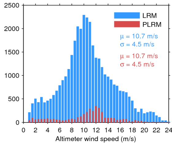
Figure 33. Histogram of flag-valid wind over oceans and lakes for LRM (blue) and PLRM (red) for 20/06/2016. The mean ( \mu ) and standard deviation ( \sigma ) are also shown. Note that values larger than 24 m/s are excluded from the histogram for the sake of readability but not from the computation of \mu and \sigma .
