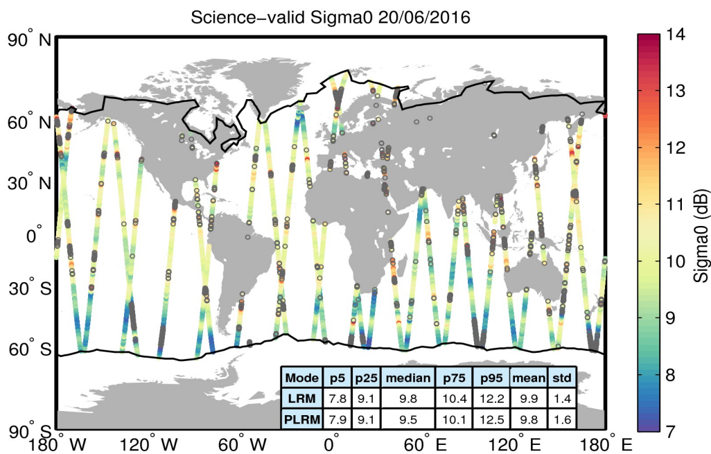
Figure 27. Geographical distribution of science-valid sigma0 data over oceans and lakes for 20/06/2016. The statistical values shown in the table refer to the sigma0 in dB and are calculated separately for LRM and PLRM regions. The black lines mark the outer limit of the Arctic and Antarctic polar polygons. Gray circles denote records that have been rejected based on the editing criteria described in Table 4.
