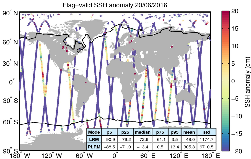
Figure 5. Geographical distribution of flag-valid 1-Hz SSH anomaly data over oceans and lakes for 20/06/2016. The statistical values shown in the table refer to the SSH anomaly in cm and are calculated separately for LRM and PLRM regions. Measurements taken over polar polygons have been excluded from the computation of the statistical values. The black lines mark the outer limit of the Arctic and Antarctic polar polygons.
