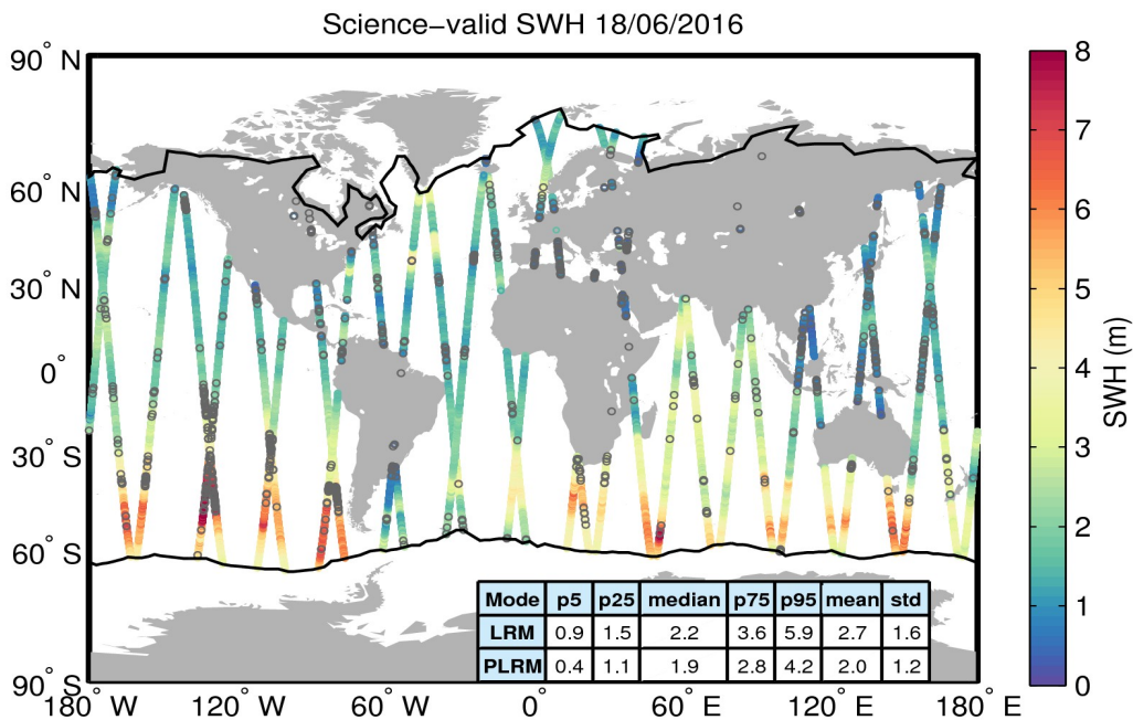
Figure 19. Geographical distribution of science-valid SWH data over oceans and lakes for 18/06/2016. The statistical values shown in the table refer to the SWH in m and are calculated separately for LRM and PLRM regions. The black lines mark the outer limit of the Arctic and Antarctic polar polygons. Gray circles denote records that have been rejected based on the editing criteria described in Table 3.
