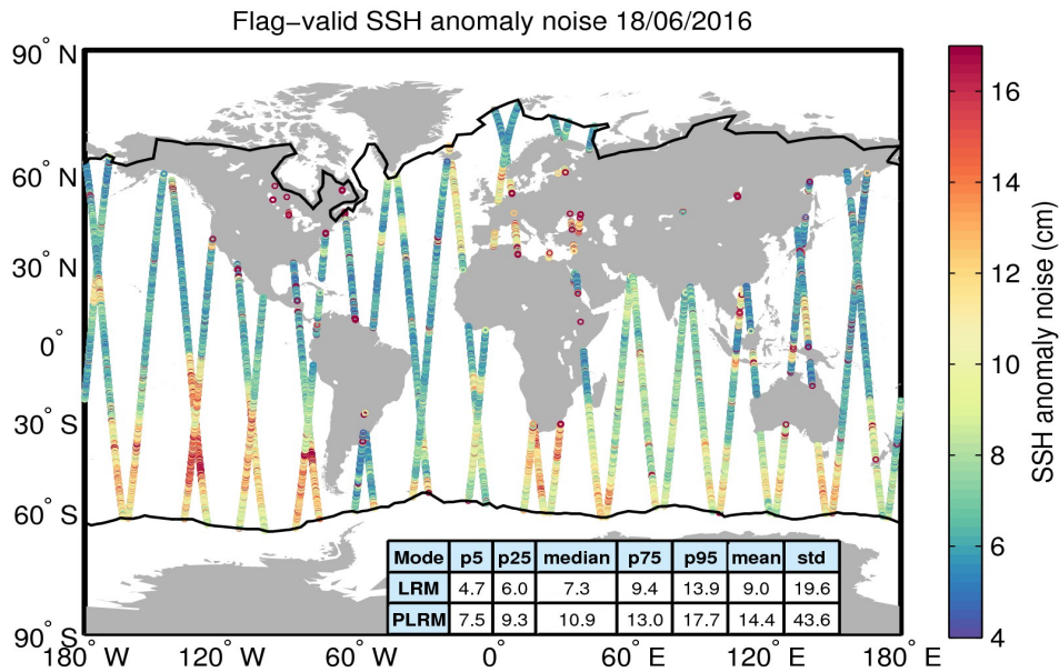
Figure 8. Geographical distribution of flag-valid 20-Hz SSH anomaly measurement noise over oceans and lakes for 18/06/2016. The statistical values shown in the table refer to the SSH anomaly noise and are calculated separately for LRM and PLRM regions. Measurements taken over polar polygons have been excluded from the computation of the statistical values. The black lines mark the outer limit of the Arctic and Antarctic polar polygons.
