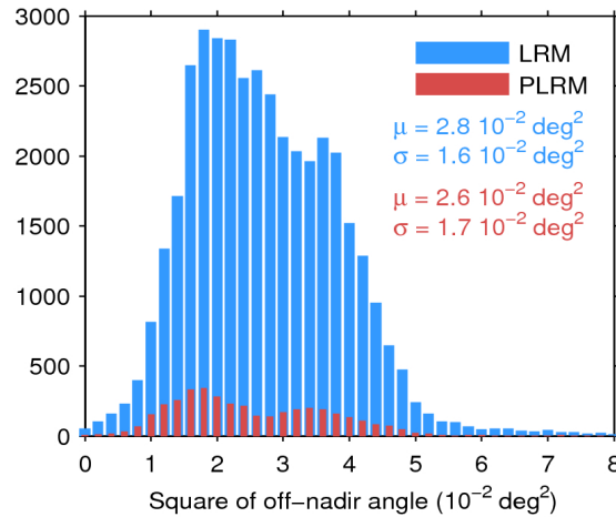
Figure 39. Histogram of flag-valid mispointing over oceans and lakes for LRM (blue) and PLRM (red) for 18/06/2016. Only positive values have been considered. The mean ( \mu ) and standard deviation ( \sigma ) are also shown. Note that values larger than 8 \cdot 10^{-2} \text{ deg}^2 are excluded from the histogram for the sake of readability but not from the computation of \mu and \sigma .
