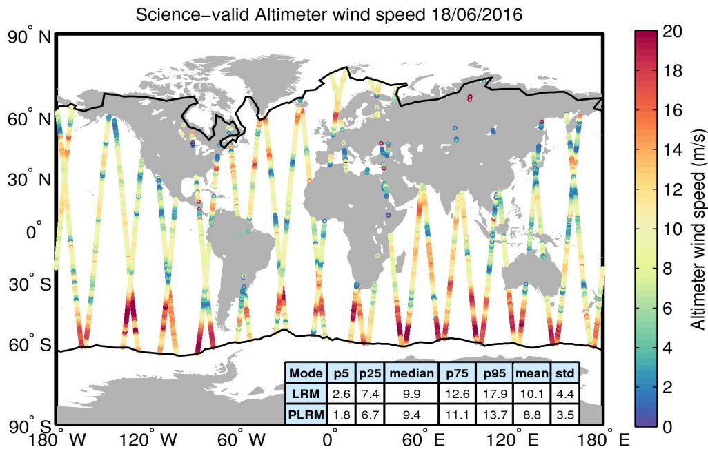
Figure 34. Geographical distribution of science-valid wind data over oceans and lakes for 18/06/2016. The statistical values shown in the table refer to the wind in m/s and are calculated separately for LRM and PLRM regions. The black lines mark the outer limit of the Arctic and Antarctic polar polygons. Gray circles denote records that have been rejected based on the editing criteria described in Table 5.
