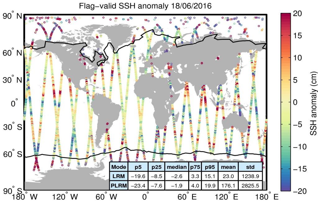
Figure 5. Geographical distribution of flag-valid 1-Hz SSH anomaly data over oceans and lakes for 18/06/2016. The statistical values shown in the table refer to the SSH anomaly in cm and are calculated separately for LRM and PLRM regions. Measurements taken over polar polygons have been excluded from the computation of the statistical values. The black lines mark the outer limit of the Arctic and Antarctic polar polygons.
