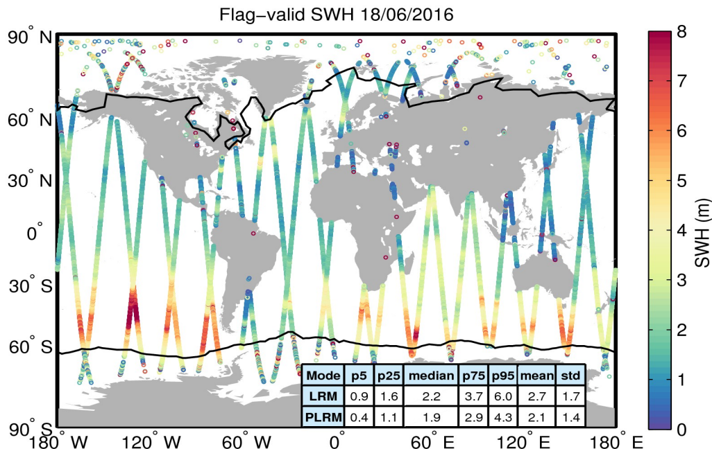
Figure 15. Geographical distribution of flag-valid SWH data over oceans and lakes for 18/06/2016. The statistical values shown in the table refer to the SWH in m and are calculated separately for LRM and PLRM regions. Measurements taken over polar polygons have been excluded from the computation of the statistical values. The black lines mark the outer limit of the Arctic and Antarctic polar polygons.
