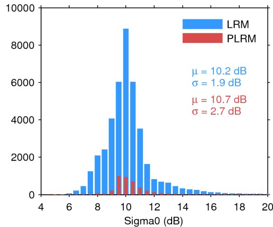
Figure 25. Histogram of flag-valid sigma0 over oceans and lakes for LRM (blue) and PLRM (red) for 18/06/2016. The mean ( \mu ) and standard deviation ( \sigma ) are also shown. Note that values outside [4 20] dB are excluded from the histogram for the sake of readability but not from the computation of \mu and \sigma .
