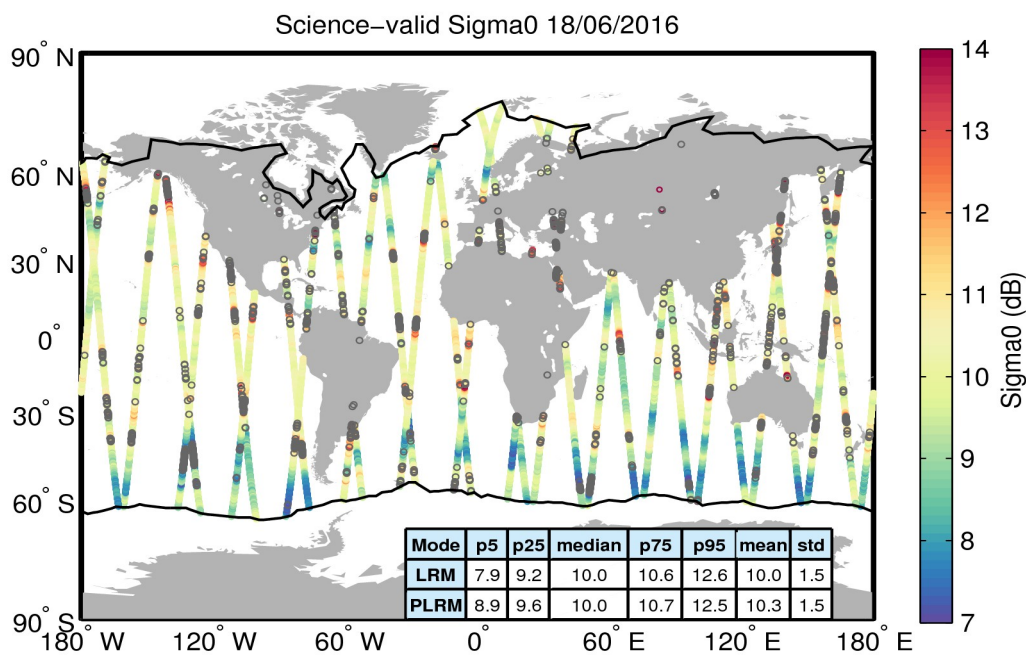
Figure 27. Geographical distribution of science-valid sigma0 data over oceans and lakes for 18/06/2016. The statistical values shown in the table refer to the sigma0 in dB and are calculated separately for LRM and PLRM regions. The black lines mark the outer limit of the Arctic and Antarctic polar polygons. Gray circles denote records that have been rejected based on the editing criteria described in Table 4.
