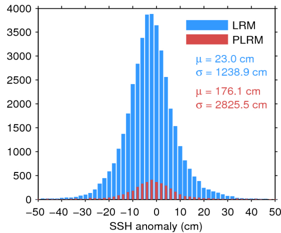
Figure 7. Histogram of flag-valid SSH anomaly over oceans and lakes for LRM (blue) and PLRM (red) for 18/06/2016. The mean ( \mu ) and standard deviation ( \sigma ) are also shown. Note that values outside [-50 50] cm are excluded from the histogram for the sake of readability but not from the computation of \mu and \sigma .
