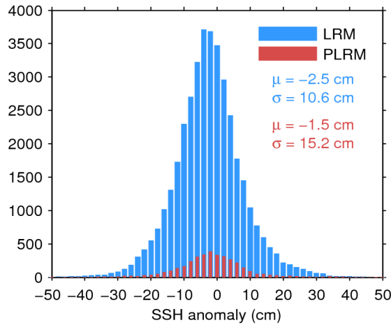
Figure 11. Histogram of science-valid SSH anomaly over oceans and lakes for LRM (blue) and PLRM (red) for 18/06/2016. The mean ( \mu ) and standard deviation ( \sigma ) are also shown. Note that values outside [-50 50] cm are excluded from the histogram for the sake of readability but not from the computation of \mu and \sigma .
