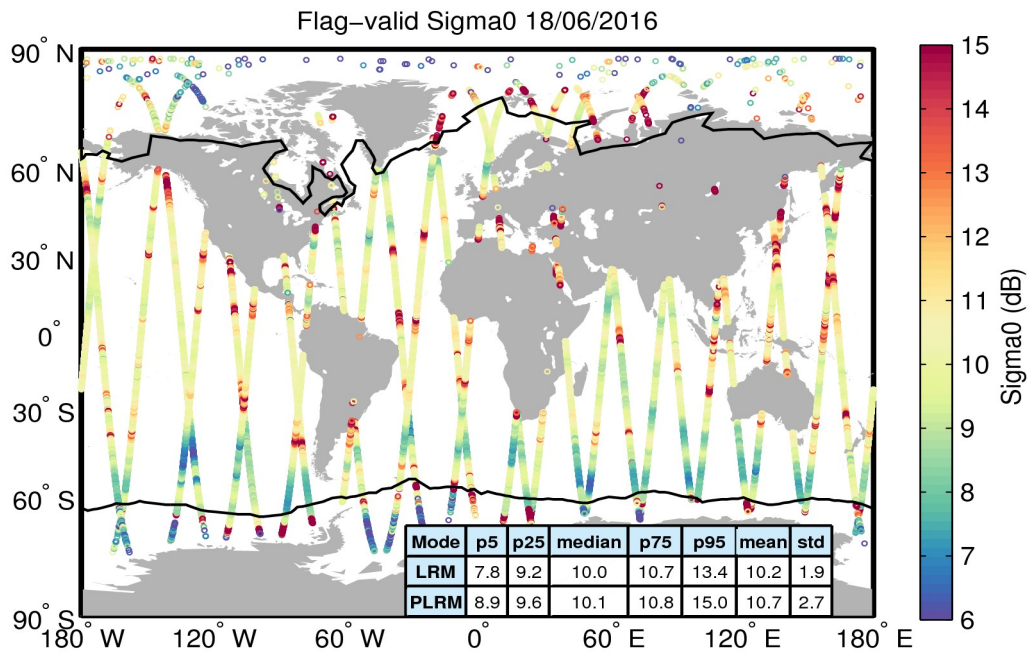
Figure 23. Geographical distribution of flag-valid sigma0 data over oceans and lakes for 18/06/2016. The statistical values shown in the table refer to the sigma0 in dB and are calculated separately for LRM and PLRM regions. Measurements taken over polar polygons have been excluded from the computation of the statistical values. The black lines mark the outer limit of the Arctic and Antarctic polar polygons.
