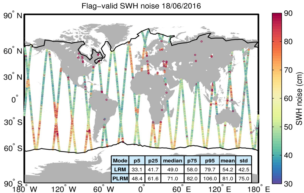
Figure 18. Geographical distribution of flag-valid 20-Hz SWH measurement noise over oceans and lakes for 18/06/2016. The statistical values shown in the table refer to the SWH noise and are calculated separately for LRM and PLRM regions. Measurements taken over polar polygons have been excluded from the computation of the statistical values. The black lines mark the outer limit of the Arctic and Antarctic polar polygons.
