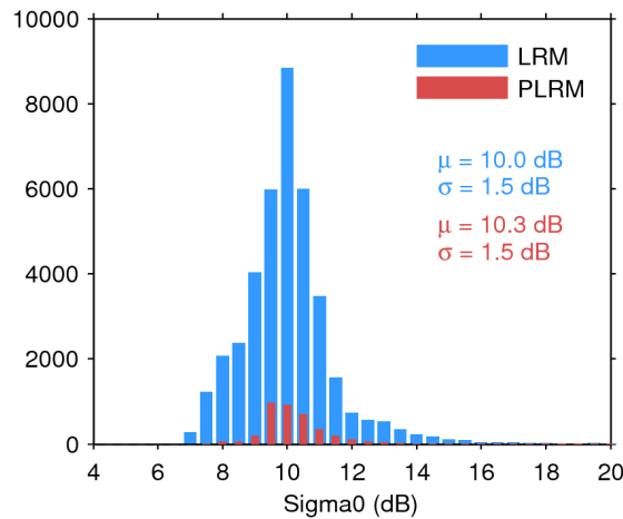
Figure 28. Histogram of science-valid sigma0 over oceans and lakes for LRM (blue) and PLRM (red) for 18/06/2016. The mean ( \mu ) and standard deviation ( \sigma ) are also shown. Note that values outside [4 20] dB are excluded from the histogram for the sake of readability but not from the computation of \mu and \sigma .
