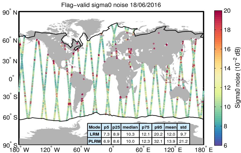
Figure 26. Geographical distribution of flag-valid 20-Hz sigma0 measurement noise over oceans and lakes for 18/06/2016. The statistical values shown in the table refer to the sigma0 noise and are calculated separately for LRM and PLRM regions. Measurements taken over polar polygons have been excluded from the computation of the statistical values. The black lines mark the outer limit of the Arctic and Antarctic polar polygons.
