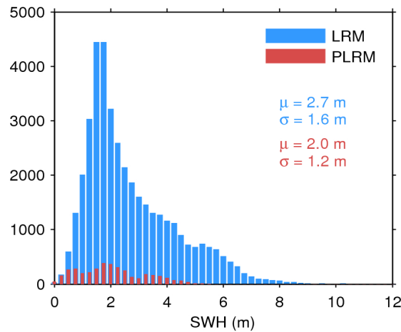
Figure 20. Histogram of science-valid SWH over oceans and lakes for LRM (blue) and PLRM (red) for 18/06/2016. The mean ( \mu ) and standard deviation ( \sigma ) are also shown. Note that values larger than 12 m are excluded from the histogram for the sake of readability but not from the computation of \mu and \sigma .
