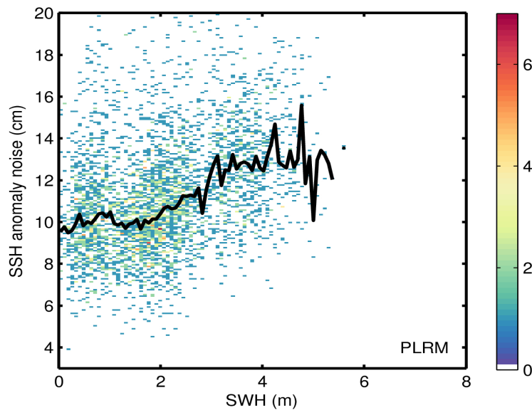
Figure 9. 2D histogram showing flag-valid SSH anomaly noise as a function of SWH for LRM (top) and PLRM (bottom) for 18/06/2016. The black line denotes the median SSH anomaly noise as a function of SWH.
