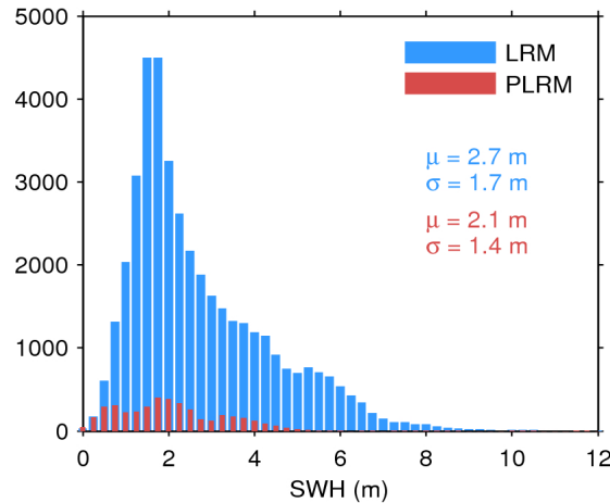
Figure 17. Histogram of flag-valid SWH over oceans and lakes for LRM (blue) and PLRM (red) for 18/06/2016. The mean ( \mu ) and standard deviation ( \sigma ) are also shown. Note that values larger than 12 m are excluded from the histogram for the sake of readability but not from the computation of \mu and \sigma .
