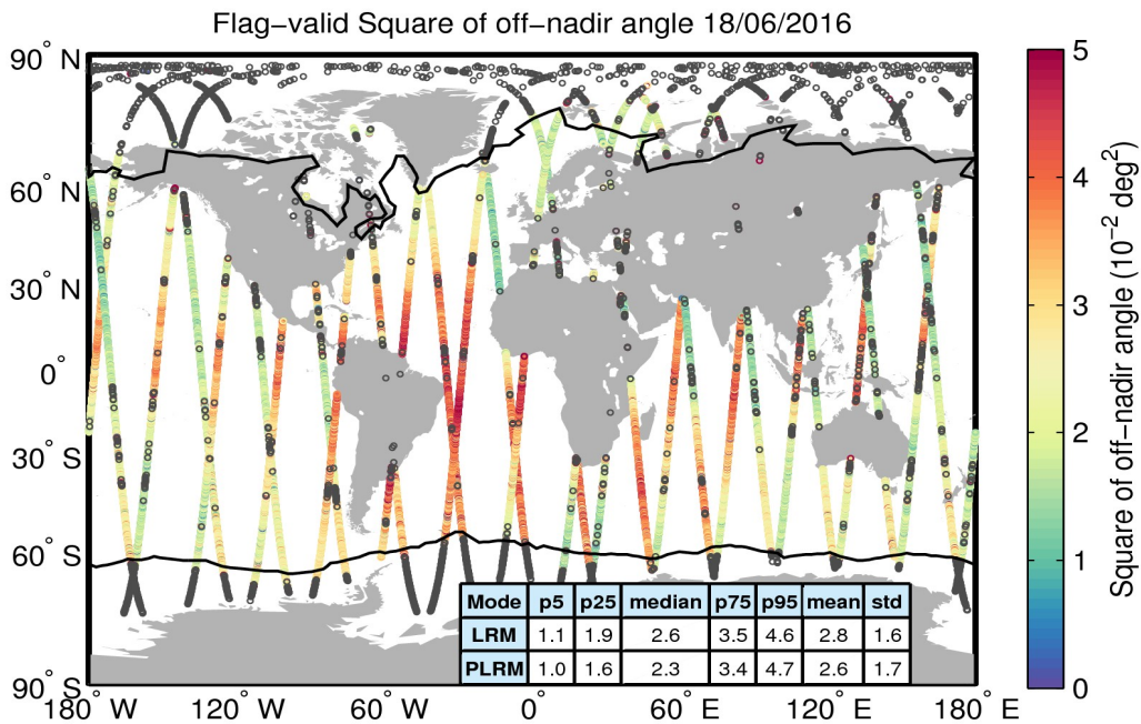
Figure 37. Geographical distribution of flag-valid mispointing data over oceans and lakes for 18/06/2016. The statistical values shown in the table refer to the mispointing in 10^{-2} deg 2 and are calculated separately for LRM and PLRM regions. Measurements taken over polar polygons have been excluded from the computation of the statistical values. The black lines mark the outer limit of the Arctic and Antarctic polar polygons. Gray circles denote negative values.
