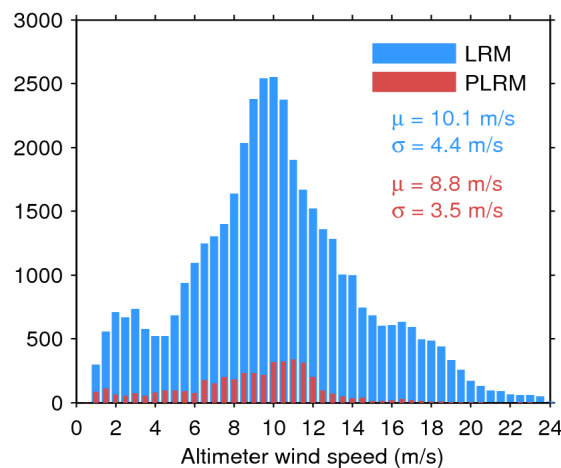
Figure 35. Histogram of science-valid wind over oceans and lakes for LRM (blue) and PLRM (red) for 18/06/2016. The mean ( \mu ) and standard deviation ( \sigma ) are also shown. Note that values larger than 24 m/s are excluded from the histogram for the sake of readability but not from the computation of \mu and \sigma .
