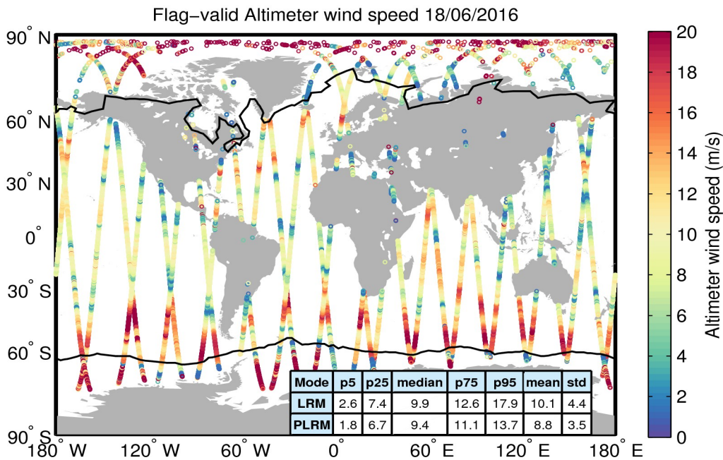
Figure 31. Geographical distribution of flag-valid wind data over oceans and lakes for 18/06/2016. The statistical values shown in the table refer to the wind in m/s and are calculated separately for LRM and PLRM regions. Measurements taken over polar polygons have been excluded from the computation of the statistical values. The black lines mark the outer limit of the Arctic and Antarctic polar polygons.
