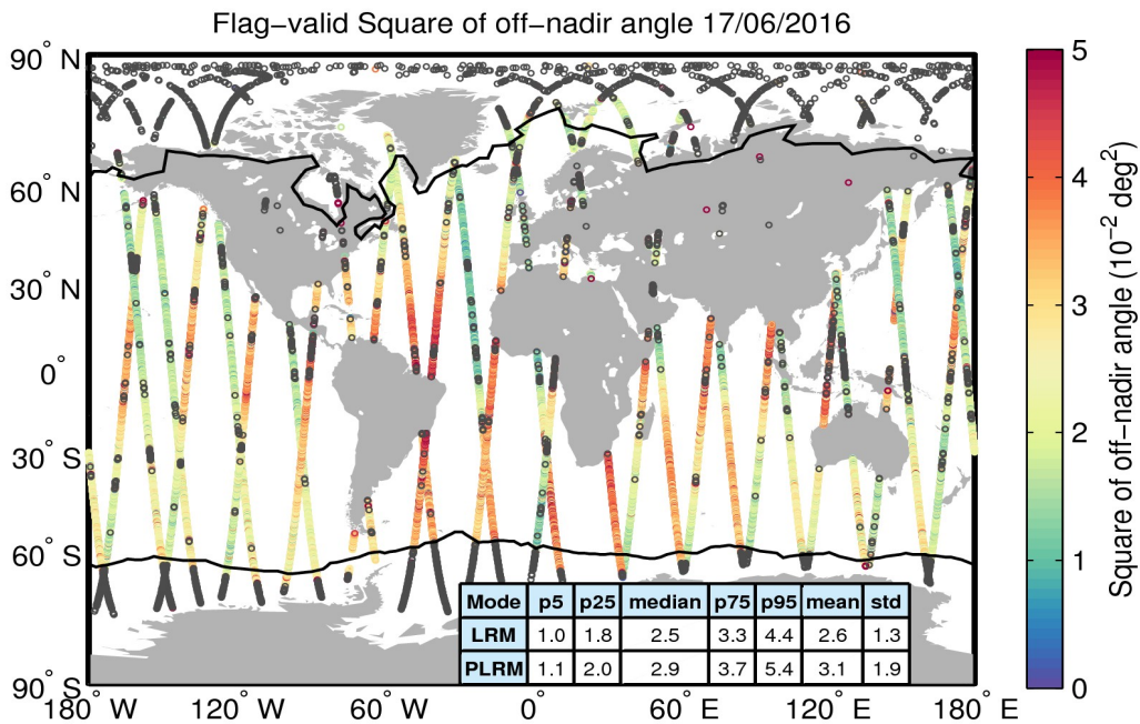
Figure 37. Geographical distribution of flag-valid mispointing data over oceans and lakes for 17/06/2016. The statistical values shown in the table refer to the mispointing in 10^{-2} deg 2 and are calculated separately for LRM and PLRM regions. Measurements taken over polar polygons have been excluded from the computation of the statistical values. The black lines mark the outer limit of the Arctic and Antarctic polar polygons. Gray circles denote negative values.
