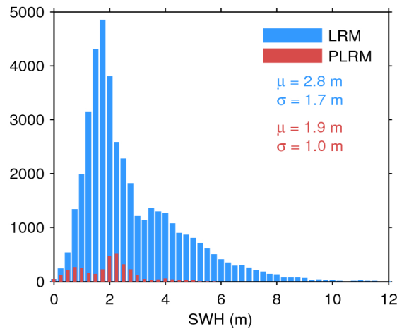
Figure 20. Histogram of science-valid SWH over oceans and lakes for LRM (blue) and PLRM (red) for 17/06/2016. The mean ( \mu ) and standard deviation ( \sigma ) are also shown. Note that values larger than 12 m are excluded from the histogram for the sake of readability but not from the computation of \mu and \sigma .
