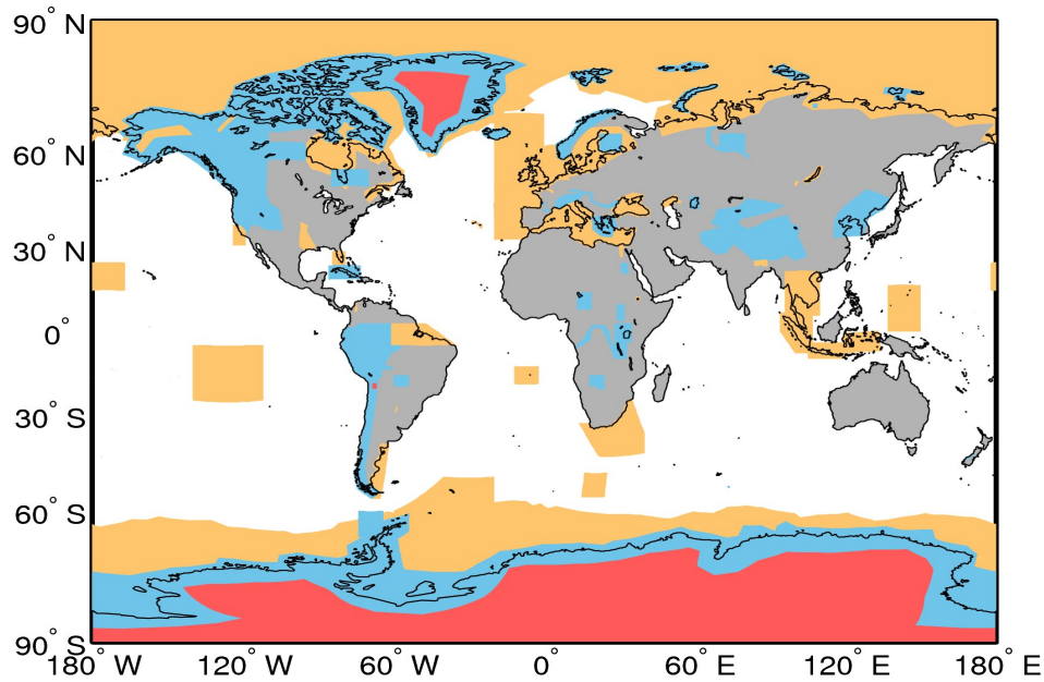
Figure A1. Extent of the regions defining the geographical mode mask for 17/06/2016. The regions where SAR, and SARIn are operated are denoted by the orange and blue polygons, respectively. LRM is operated over areas of the continental ice sheets (red polygons) and over oceans and land not covered by other modes.
