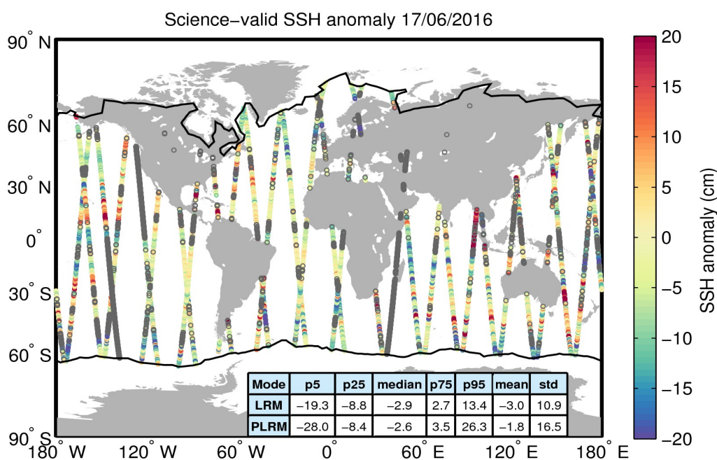
Figure 10. Geographical distribution of science-valid SSH anomaly data over oceans and lakes for 17/06/2016. The statistical values shown in the table refer to the SSH anomaly in cm and are calculated separately for LRM and PLRM regions. The black lines mark the outer limit of the Arctic and Antarctic polar polygons. Gray circles denote records that have been rejected based on the editing criteria described in Table 2.
