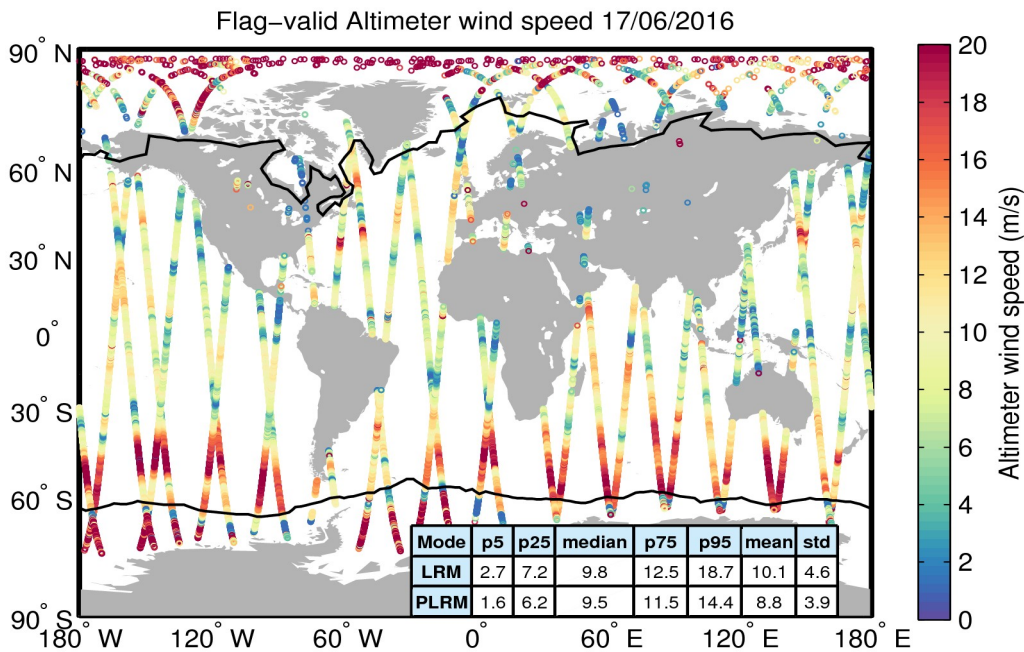
Figure 31. Geographical distribution of flag-valid wind data over oceans and lakes for 17/06/2016. The statistical values shown in the table refer to the wind in m/s and are calculated separately for LRM and PLRM regions. Measurements taken over polar polygons have been excluded from the computation of the statistical values. The black lines mark the outer limit of the Arctic and Antarctic polar polygons.
