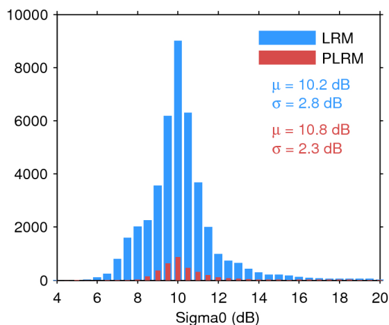
Figure 25. Histogram of flag-valid sigma0 over oceans and lakes for LRM (blue) and PLRM (red) for 17/06/2016. The mean ( \mu ) and standard deviation ( \sigma ) are also shown. Note that values outside [4 20] dB are excluded from the histogram for the sake of readability but not from the computation of \mu and \sigma .
