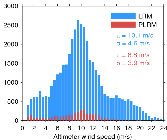
Figure 35. Histogram of science-valid wind over oceans and lakes for LRM (blue) and PLRM (red) for 17/06/2016. The mean ( \mu ) and standard deviation ( \sigma ) are also shown. Note that values larger than 24 m/s are excluded from the histogram for the sake of readability but not from the computation of \mu and \sigma .
