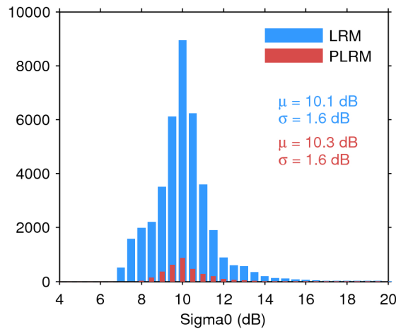
Figure 28. Histogram of science-valid sigma0 over oceans and lakes for LRM (blue) and PLRM (red) for 17/06/2016. The mean ( \mu ) and standard deviation ( \sigma ) are also shown. Note that values outside [4 20] dB are excluded from the histogram for the sake of readability but not from the computation of \mu and \sigma .
