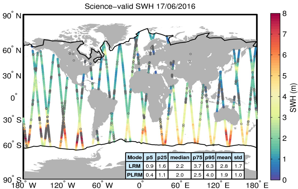
Figure 19. Geographical distribution of science-valid SWH data over oceans and lakes for 17/06/2016. The statistical values shown in the table refer to the SWH in m and are calculated separately for LRM and PLRM regions. The black lines mark the outer limit of the Arctic and Antarctic polar polygons. Gray circles denote records that have been rejected based on the editing criteria described in Table 3.
