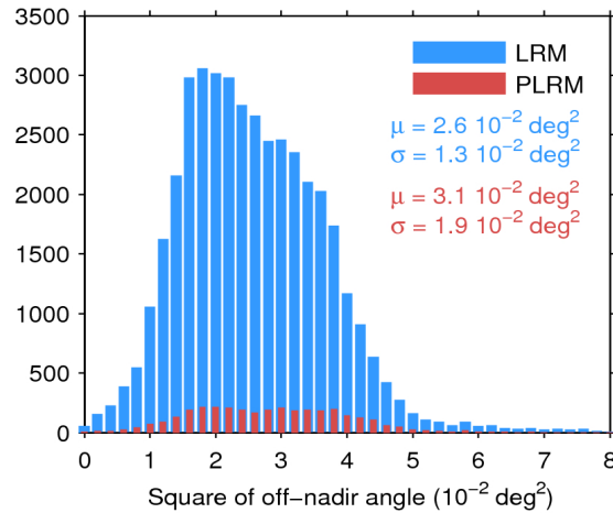
Figure 39. Histogram of flag-valid mispointing over oceans and lakes for LRM (blue) and PLRM (red) for 17/06/2016. Only positive values have been considered. The mean ( \mu ) and standard deviation ( \sigma ) are also shown. Note that values larger than 8 \cdot 10^{-2} \text{ deg}^2 are excluded from the histogram for the sake of readability but not from the computation of \mu and \sigma .
