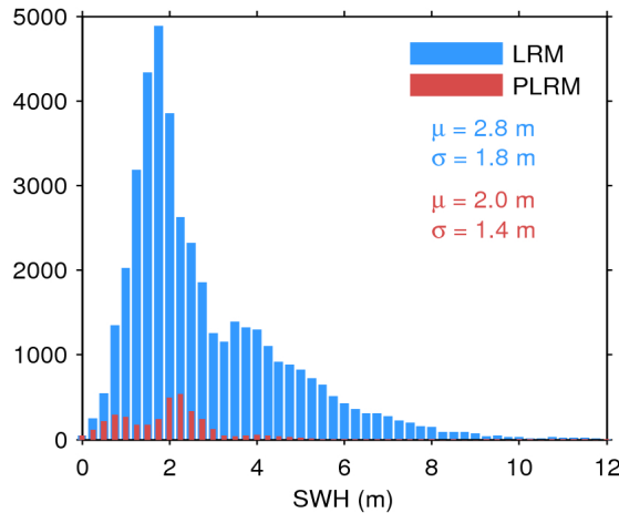
Figure 17. Histogram of flag-valid SWH over oceans and lakes for LRM (blue) and PLRM (red) for 17/06/2016. The mean ( \mu ) and standard deviation ( \sigma ) are also shown. Note that values larger than 12 m are excluded from the histogram for the sake of readability but not from the computation of \mu and \sigma .
