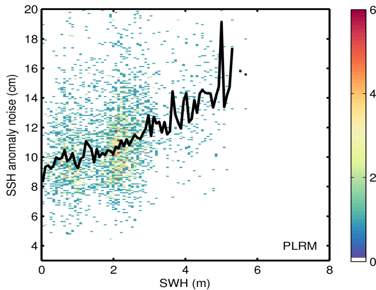
Figure 9. 2D histogram showing flag-valid SSH anomaly noise as a function of SWH for LRM (top) and PLRM (bottom) for 17/06/2016. The black line denotes the median SSH anomaly noise as a function of SWH.
