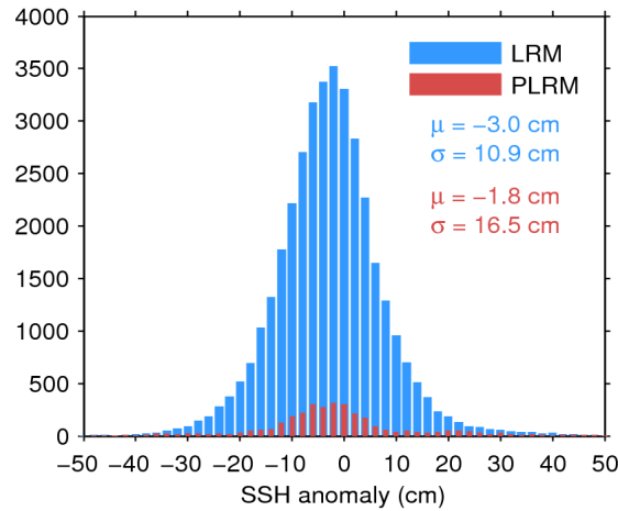
Figure 11. Histogram of science-valid SSH anomaly over oceans and lakes for LRM (blue) and PLRM (red) for 17/06/2016. The mean ( \mu ) and standard deviation ( \sigma ) are also shown. Note that values outside [-50 50] cm are excluded from the histogram for the sake of readability but not from the computation of \mu and \sigma .
