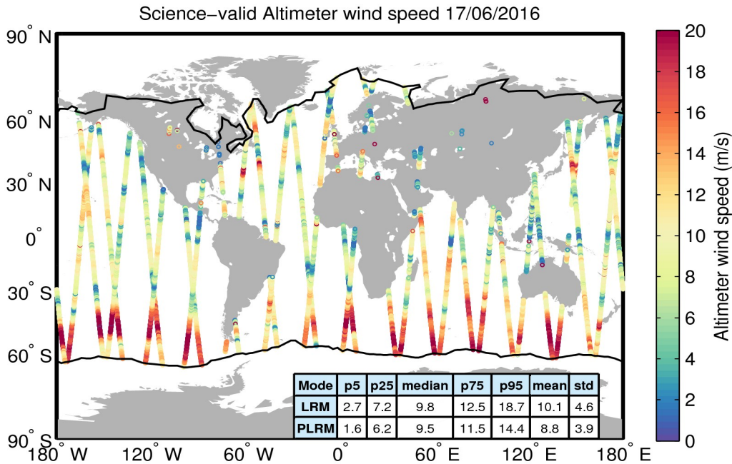
Figure 34. Geographical distribution of science-valid wind data over oceans and lakes for 17/06/2016. The statistical values shown in the table refer to the wind in m/s and are calculated separately for LRM and PLRM regions. The black lines mark the outer limit of the Arctic and Antarctic polar polygons. Gray circles denote records that have been rejected based on the editing criteria described in Table 5.
