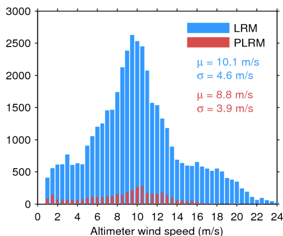
Figure 33. Histogram of flag-valid wind over oceans and lakes for LRM (blue) and PLRM (red) for 17/06/2016. The mean ( \mu ) and standard deviation ( \sigma ) are also shown. Note that values larger than 24 m/s are excluded from the histogram for the sake of readability but not from the computation of \mu and \sigma .
