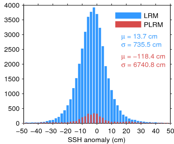
Figure 7. Histogram of flag-valid SSH anomaly over oceans and lakes for LRM (blue) and PLRM (red) for 17/06/2016. The mean ( \mu ) and standard deviation ( \sigma ) are also shown. Note that values outside [-50 50] cm are excluded from the histogram for the sake of readability but not from the computation of \mu and \sigma .
