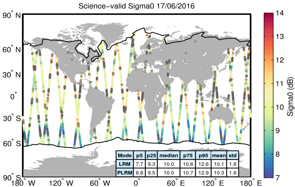
Figure 27. Geographical distribution of science-valid sigma0 data over oceans and lakes for 17/06/2016. The statistical values shown in the table refer to the sigma0 in dB and are calculated separately for LRM and PLRM regions. The black lines mark the outer limit of the Arctic and Antarctic polar polygons. Gray circles denote records that have been rejected based on the editing criteria described in Table 4.
