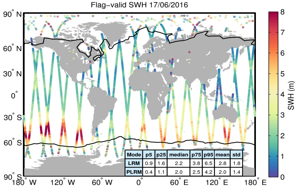
Figure 15. Geographical distribution of flag-valid SWH data over oceans and lakes for 17/06/2016. The statistical values shown in the table refer to the SWH in m and are calculated separately for LRM and PLRM regions. Measurements taken over polar polygons have been excluded from the computation of the statistical values. The black lines mark the outer limit of the Arctic and Antarctic polar polygons.
