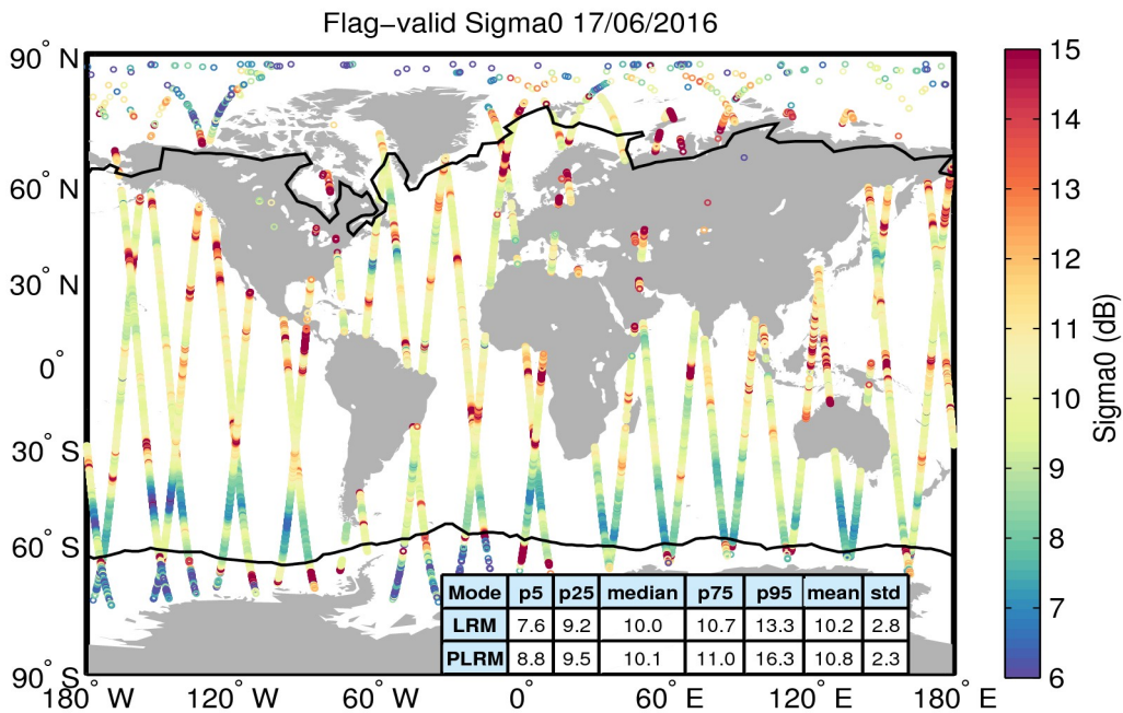
Figure 23. Geographical distribution of flag-valid sigma0 data over oceans and lakes for 17/06/2016. The statistical values shown in the table refer to the sigma0 in dB and are calculated separately for LRM and PLRM regions. Measurements taken over polar polygons have been excluded from the computation of the statistical values. The black lines mark the outer limit of the Arctic and Antarctic polar polygons.
