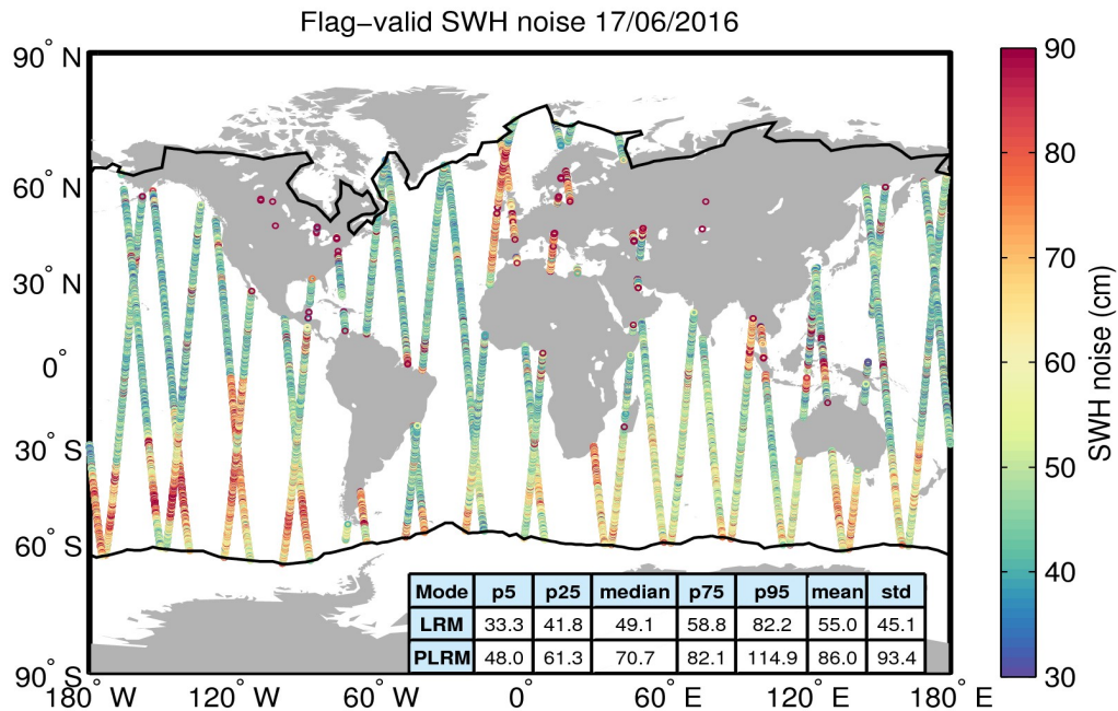
Figure 18. Geographical distribution of flag-valid 20-Hz SWH measurement noise over oceans and lakes for 17/06/2016. The statistical values shown in the table refer to the SWH noise and are calculated separately for LRM and PLRM regions. Measurements taken over polar polygons have been excluded from the computation of the statistical values. The black lines mark the outer limit of the Arctic and Antarctic polar polygons.
