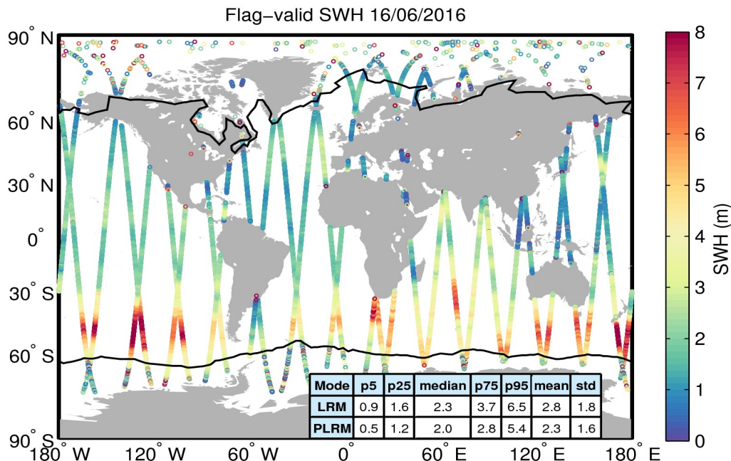
Figure 15. Geographical distribution of flag-valid SWH data over oceans and lakes for 16/06/2016. The statistical values shown in the table refer to the SWH in m and are calculated separately for LRM and PLRM regions. Measurements taken over polar polygons have been excluded from the computation of the statistical values. The black lines mark the outer limit of the Arctic and Antarctic polar polygons.
