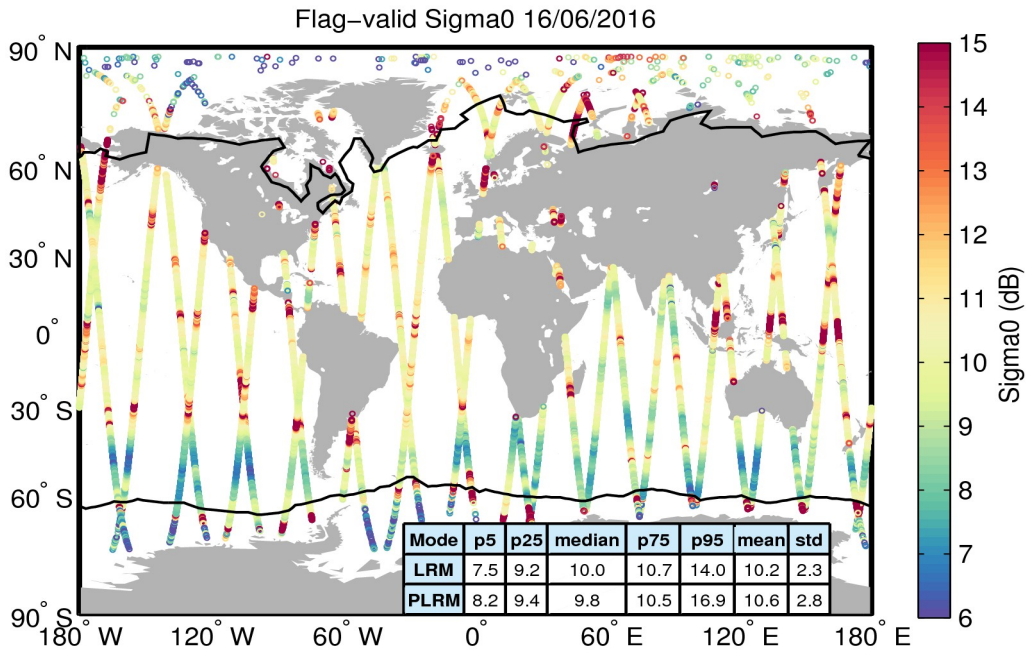
Figure 23. Geographical distribution of flag-valid sigma0 data over oceans and lakes for 16/06/2016. The statistical values shown in the table refer to the sigma0 in dB and are calculated separately for LRM and PLRM regions. Measurements taken over polar polygons have been excluded from the computation of the statistical values. The black lines mark the outer limit of the Arctic and Antarctic polar polygons.
