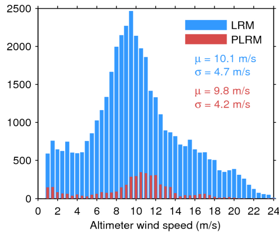
Figure 33. Histogram of flag-valid wind over oceans and lakes for LRM (blue) and PLRM (red) for 16/06/2016. The mean ( \mu ) and standard deviation ( \sigma ) are also shown. Note that values larger than 24 m/s are excluded from the histogram for the sake of readability but not from the computation of \mu and \sigma .
