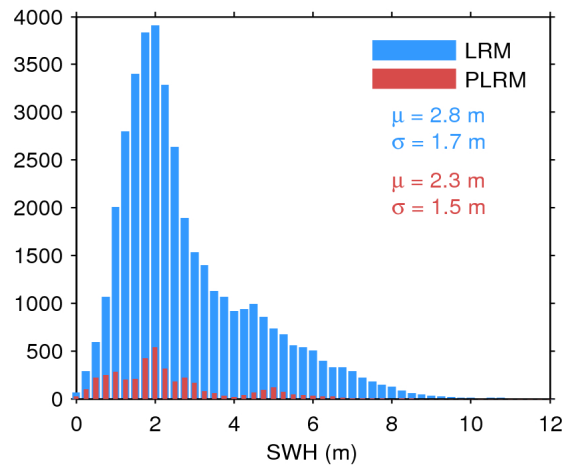
Figure 20. Histogram of science-valid SWH over oceans and lakes for LRM (blue) and PLRM (red) for 16/06/2016. The mean ( \mu ) and standard deviation ( \sigma ) are also shown. Note that values larger than 12 m are excluded from the histogram for the sake of readability but not from the computation of \mu and \sigma .
