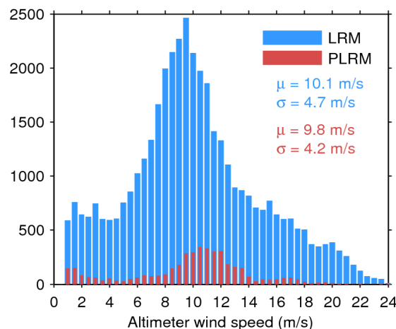
Figure 35. Histogram of science-valid wind over oceans and lakes for LRM (blue) and PLRM (red) for 16/06/2016. The mean ( \mu ) and standard deviation ( \sigma ) are also shown. Note that values larger than 24 m/s are excluded from the histogram for the sake of readability but not from the computation of \mu and \sigma .
