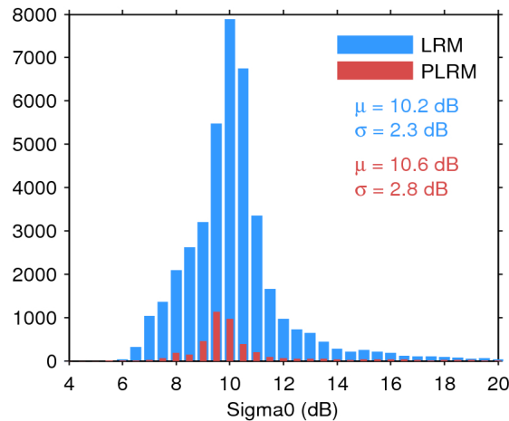
Figure 25. Histogram of flag-valid sigma0 over oceans and lakes for LRM (blue) and PLRM (red) for 16/06/2016. The mean ( \mu ) and standard deviation ( \sigma ) are also shown. Note that values outside [4 20] dB are excluded from the histogram for the sake of readability but not from the computation of \mu and \sigma .
