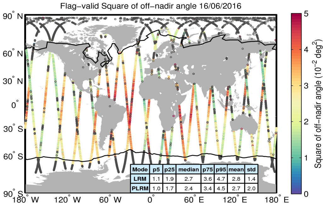
Figure 37. Geographical distribution of flag-valid mispointing data over oceans and lakes for 16/06/2016. The statistical values shown in the table refer to the mispointing in 10^{-2} deg 2 and are calculated separately for LRM and PLRM regions. Measurements taken over polar polygons have been excluded from the computation of the statistical values. The black lines mark the outer limit of the Arctic and Antarctic polar polygons. Gray circles denote negative values.
