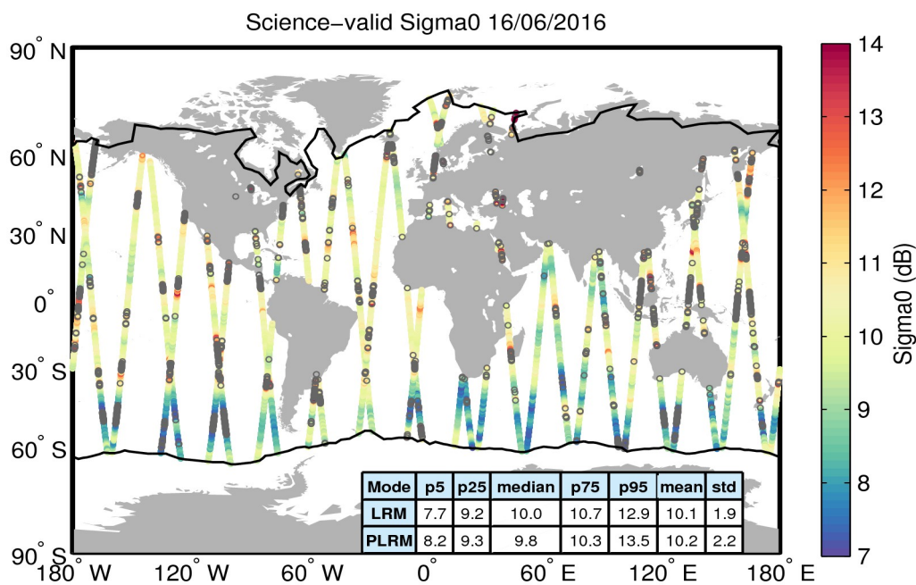
Figure 27. Geographical distribution of science-valid sigma0 data over oceans and lakes for 16/06/2016. The statistical values shown in the table refer to the sigma0 in dB and are calculated separately for LRM and PLRM regions. The black lines mark the outer limit of the Arctic and Antarctic polar polygons. Gray circles denote records that have been rejected based on the editing criteria described in Table 4.
