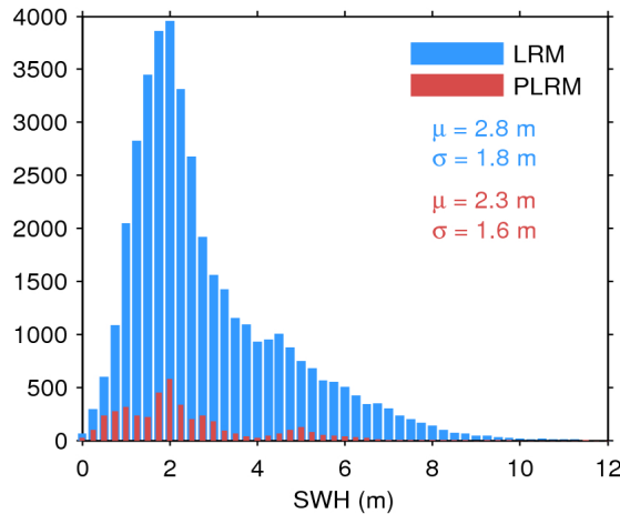
Figure 17. Histogram of flag-valid SWH over oceans and lakes for LRM (blue) and PLRM (red) for 16/06/2016. The mean ( \mu ) and standard deviation ( \sigma ) are also shown. Note that values larger than 12 m are excluded from the histogram for the sake of readability but not from the computation of \mu and \sigma .
