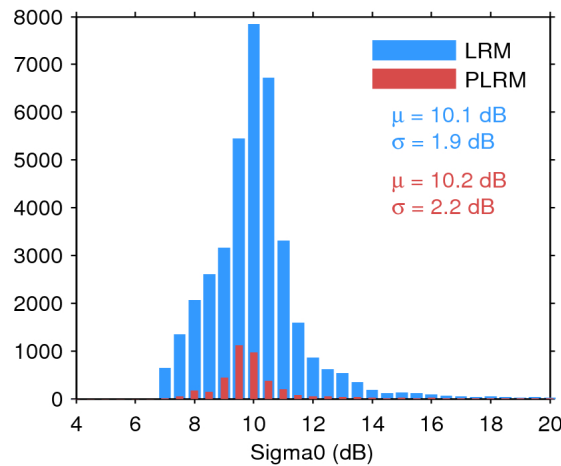
Figure 28. Histogram of science-valid sigma0 over oceans and lakes for LRM (blue) and PLRM (red) for 16/06/2016. The mean ( \mu ) and standard deviation ( \sigma ) are also shown. Note that values outside [4 20] dB are excluded from the histogram for the sake of readability but not from the computation of \mu and \sigma .
