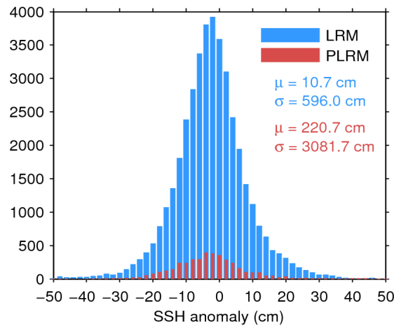
Figure 7. Histogram of flag-valid SSH anomaly over oceans and lakes for LRM (blue) and PLRM (red) for 16/06/2016. The mean ( \mu ) and standard deviation ( \sigma ) are also shown. Note that values outside [-50 \ 50] cm are excluded from the histogram for the sake of readability but not from the computation of \mu and \sigma .
