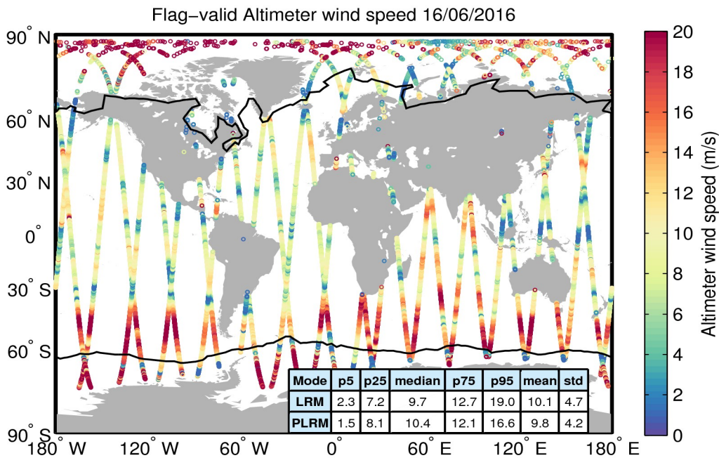
Figure 31. Geographical distribution of flag-valid wind data over oceans and lakes for 16/06/2016. The statistical values shown in the table refer to the wind in m/s and are calculated separately for LRM and PLRM regions. Measurements taken over polar polygons have been excluded from the computation of the statistical values. The black lines mark the outer limit of the Arctic and Antarctic polar polygons.
