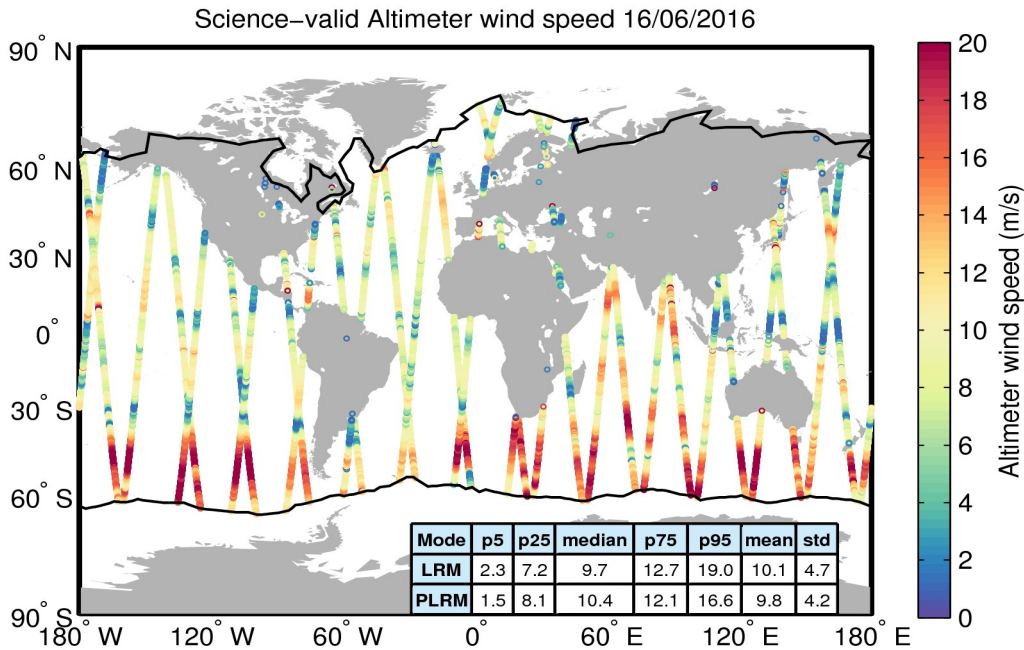
Figure 34. Geographical distribution of science-valid wind data over oceans and lakes for 16/06/2016. The statistical values shown in the table refer to the wind in m/s and are calculated separately for LRM and PLRM regions. The black lines mark the outer limit of the Arctic and Antarctic polar polygons. Gray circles denote records that have been rejected based on the editing criteria described in Table 5.
