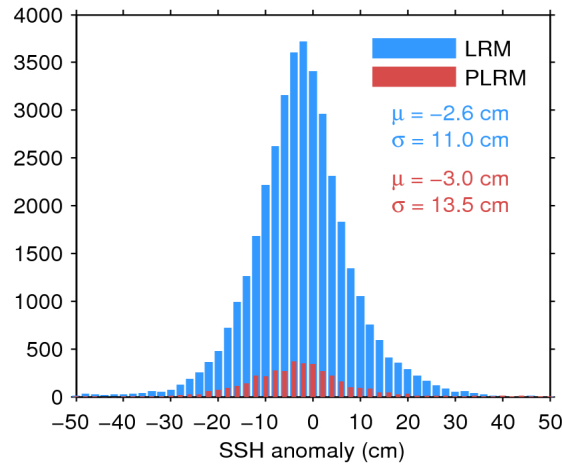
Figure 11. Histogram of science-valid SSH anomaly over oceans and lakes for LRM (blue) and PLRM (red) for 16/06/2016. The mean ( \mu ) and standard deviation ( \sigma ) are also shown. Note that values outside [-50 50] cm are excluded from the histogram for the sake of readability but not from the computation of \mu and \sigma .
