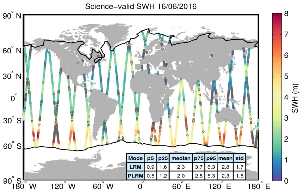
Figure 19. Geographical distribution of science-valid SWH data over oceans and lakes for 16/06/2016. The statistical values shown in the table refer to the SWH in m and are calculated separately for LRM and PLRM regions. The black lines mark the outer limit of the Arctic and Antarctic polar polygons. Gray circles denote records that have been rejected based on the editing criteria described in Table 3.
