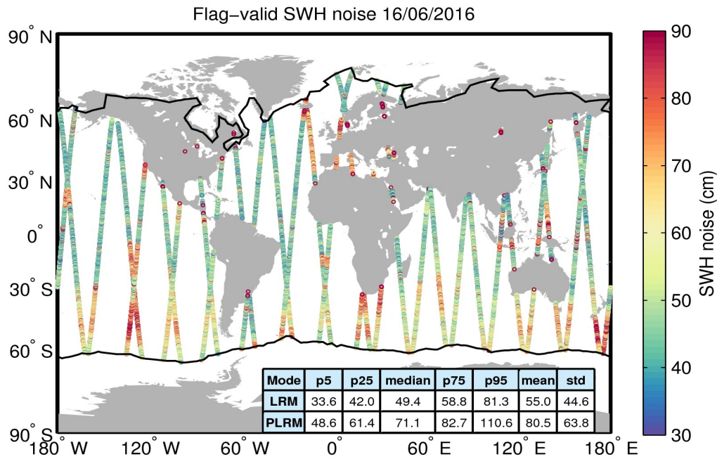
Figure 18. Geographical distribution of flag-valid 20-Hz SWH measurement noise over oceans and lakes for 16/06/2016. The statistical values shown in the table refer to the SWH noise and are calculated separately for LRM and PLRM regions. Measurements taken over polar polygons have been excluded from the computation of the statistical values. The black lines mark the outer limit of the Arctic and Antarctic polar polygons.
