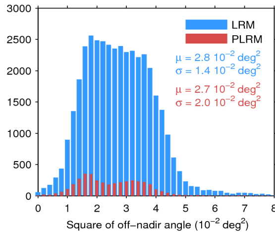
Figure 39. Histogram of flag-valid mispointing over oceans and lakes for LRM (blue) and PLRM (red) for 16/06/2016. Only positive values have been considered. The mean ( \mu ) and standard deviation ( \sigma ) are also shown. Note that values larger than 8 \cdot 10^{-2} \text{ deg}^2 are excluded from the histogram for the sake of readability but not from the computation of \mu and \sigma .
