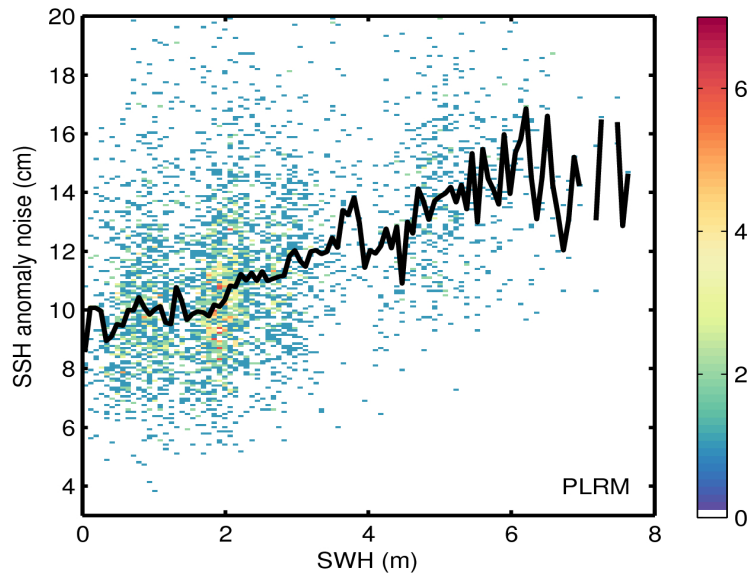
Figure 9. 2D histogram showing flag-valid SSH anomaly noise as a function of SWH for LRM (top) and PLRM (bottom) for 16/06/2016. The black line denotes the median SSH anomaly noise as a function of SWH.
