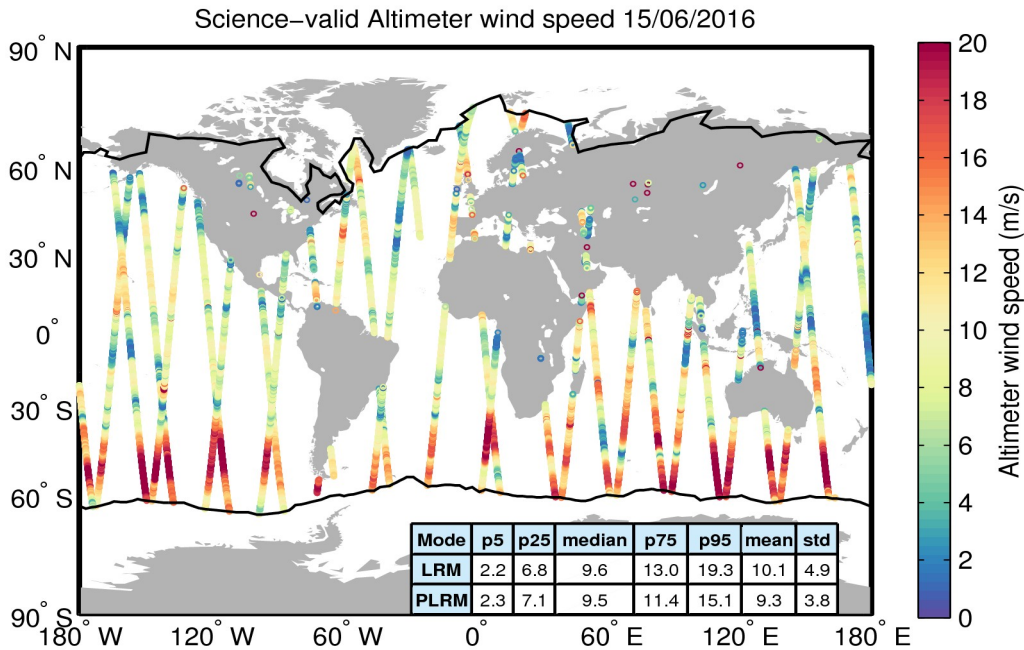
Figure 34. Geographical distribution of science-valid wind data over oceans and lakes for 15/06/2016. The statistical values shown in the table refer to the wind in m/s and are calculated separately for LRM and PLRM regions. The black lines mark the outer limit of the Arctic and Antarctic polar polygons. Gray circles denote records that have been rejected based on the editing criteria described in Table 5.
