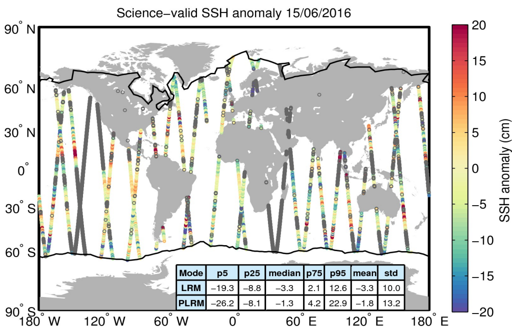
Figure 10. Geographical distribution of science-valid SSH anomaly data over oceans and lakes for 15/06/2016. The statistical values shown in the table refer to the SSH anomaly in cm and are calculated separately for LRM and PLRM regions. The black lines mark the outer limit of the Arctic and Antarctic polar polygons. Gray circles denote records that have been rejected based on the editing criteria described in Table 2.
