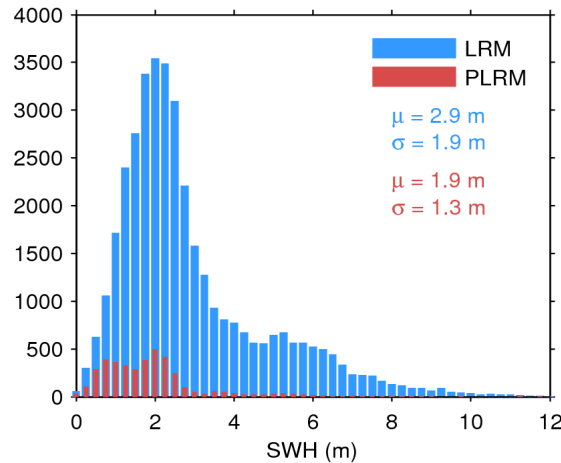
Figure 17. Histogram of flag-valid SWH over oceans and lakes for LRM (blue) and PLRM (red) for 15/06/2016. The mean ( \mu ) and standard deviation ( \sigma ) are also shown. Note that values larger than 12 m are excluded from the histogram for the sake of readability but not from the computation of \mu and \sigma .
