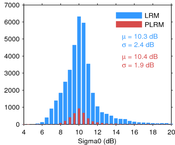
Figure 25. Histogram of flag-valid sigma0 over oceans and lakes for LRM (blue) and PLRM (red) for 15/06/2016. The mean ( \mu ) and standard deviation ( \sigma ) are also shown. Note that values outside [4 20] dB are excluded from the histogram for the sake of readability but not from the computation of \mu and \sigma .
