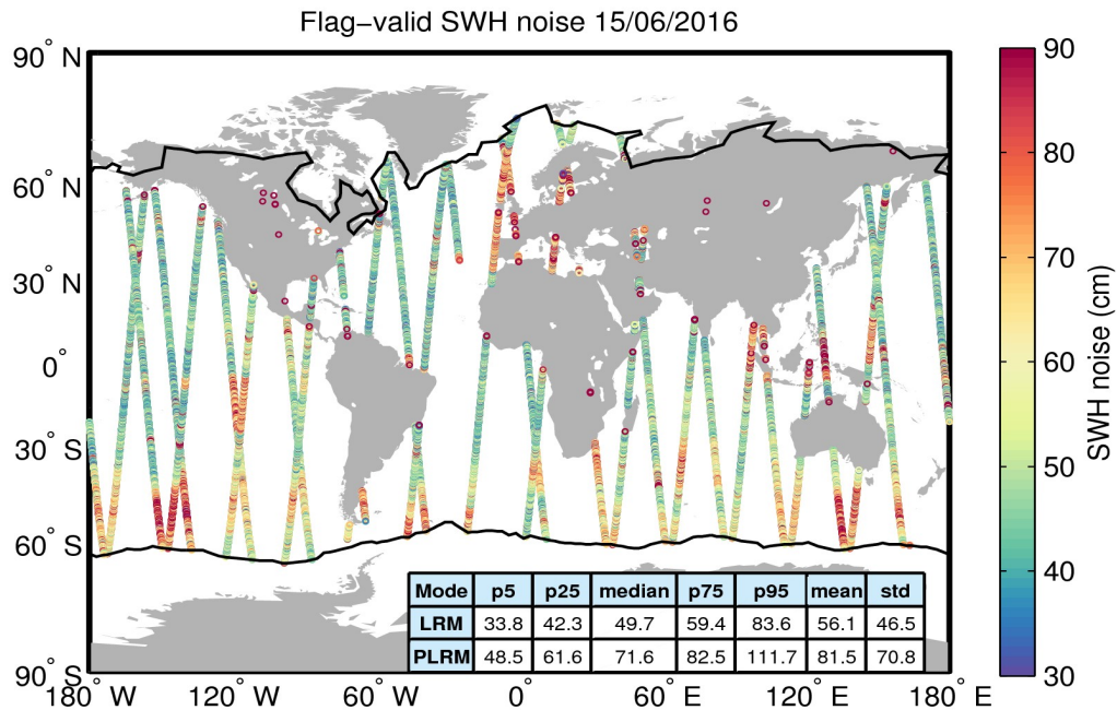
Figure 18. Geographical distribution of flag-valid 20-Hz SWH measurement noise over oceans and lakes for 15/06/2016. The statistical values shown in the table refer to the SWH noise and are calculated separately for LRM and PLRM regions. Measurements taken over polar polygons have been excluded from the computation of the statistical values. The black lines mark the outer limit of the Arctic and Antarctic polar polygons.
