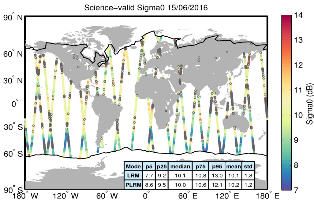
Figure 27. Geographical distribution of science-valid sigma0 data over oceans and lakes for 15/06/2016. The statistical values shown in the table refer to the sigma0 in dB and are calculated separately for LRM and PLRM regions. The black lines mark the outer limit of the Arctic and Antarctic polar polygons. Gray circles denote records that have been rejected based on the editing criteria described in Table 4.
