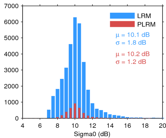
Figure 28. Histogram of science-valid sigma0 over oceans and lakes for LRM (blue) and PLRM (red) for 15/06/2016. The mean ( \mu ) and standard deviation ( \sigma ) are also shown. Note that values outside [4 20] dB are excluded from the histogram for the sake of readability but not from the computation of \mu and \sigma .
