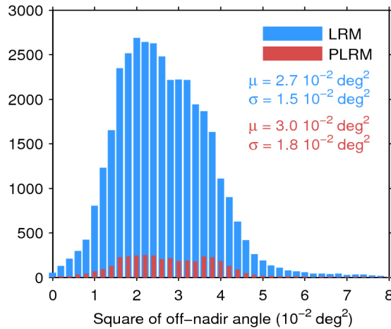
Figure 39. Histogram of flag-valid mispointing over oceans and lakes for LRM (blue) and PLRM (red) for 15/06/2016. Only positive values have been considered. The mean ( \mu ) and standard deviation ( \sigma ) are also shown. Note that values larger than 8 \cdot 10^{-2} \text{ deg}^2 are excluded from the histogram for the sake of readability but not from the computation of \mu and \sigma .
