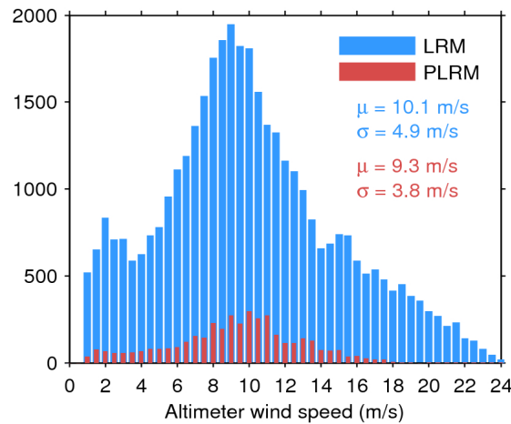
Figure 33. Histogram of flag-valid wind over oceans and lakes for LRM (blue) and PLRM (red) for 15/06/2016. The mean ( \mu ) and standard deviation ( \sigma ) are also shown. Note that values larger than 24 m/s are excluded from the histogram for the sake of readability but not from the computation of \mu and \sigma .
