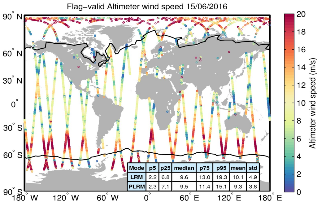
Figure 31. Geographical distribution of flag-valid wind data over oceans and lakes for 15/06/2016. The statistical values shown in the table refer to the wind in m/s and are calculated separately for LRM and PLRM regions. Measurements taken over polar polygons have been excluded from the computation of the statistical values. The black lines mark the outer limit of the Arctic and Antarctic polar polygons.
