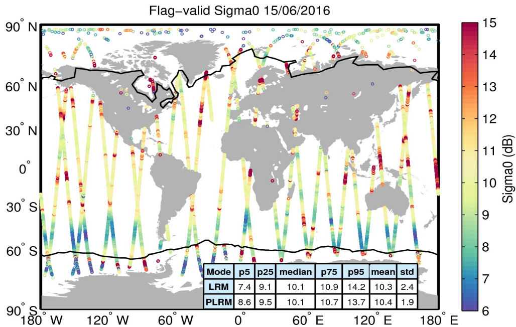
Figure 23. Geographical distribution of flag-valid sigma0 data over oceans and lakes for 15/06/2016. The statistical values shown in the table refer to the sigma0 in dB and are calculated separately for LRM and PLRM regions. Measurements taken over polar polygons have been excluded from the computation of the statistical values. The black lines mark the outer limit of the Arctic and Antarctic polar polygons.
