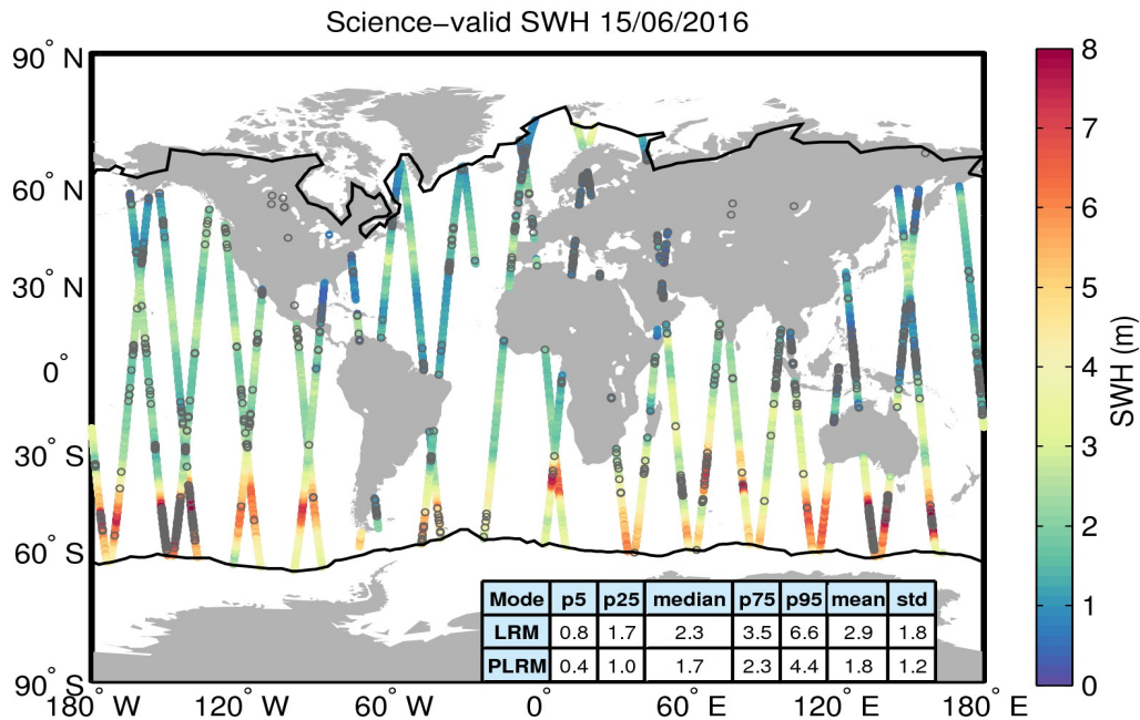
Figure 19. Geographical distribution of science-valid SWH data over oceans and lakes for 15/06/2016. The statistical values shown in the table refer to the SWH in m and are calculated separately for LRM and PLRM regions. The black lines mark the outer limit of the Arctic and Antarctic polar polygons. Gray circles denote records that have been rejected based on the editing criteria described in Table 3.
