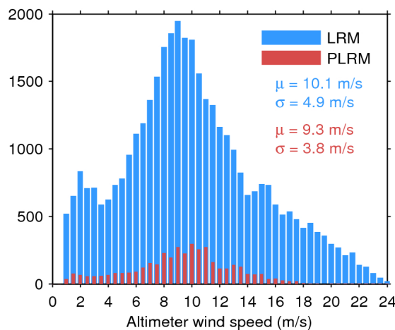
Figure 35. Histogram of science-valid wind over oceans and lakes for LRM (blue) and PLRM (red) for 15/06/2016. The mean ( \mu ) and standard deviation ( \sigma ) are also shown. Note that values larger than 24 m/s are excluded from the histogram for the sake of readability but not from the computation of \mu and \sigma .
