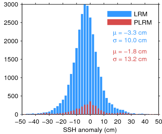
Figure 11. Histogram of science-valid SSH anomaly over oceans and lakes for LRM (blue) and PLRM (red) for 15/06/2016. The mean ( \mu ) and standard deviation ( \sigma ) are also shown. Note that values outside [-50 50] cm are excluded from the histogram for the sake of readability but not from the computation of \mu and \sigma .
