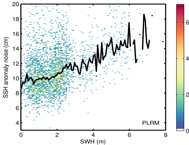
Figure 9. 2D histogram showing flag-valid SSH anomaly noise as a function of SWH for LRM (top) and PLRM (bottom) for 15/06/2016. The black line denotes the median SSH anomaly noise as a function of SWH.
