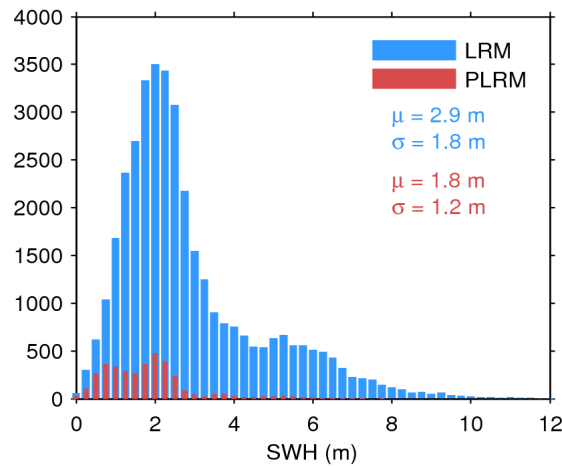
Figure 20. Histogram of science-valid SWH over oceans and lakes for LRM (blue) and PLRM (red) for 15/06/2016. The mean ( \mu ) and standard deviation ( \sigma ) are also shown. Note that values larger than 12 m are excluded from the histogram for the sake of readability but not from the computation of \mu and \sigma .
