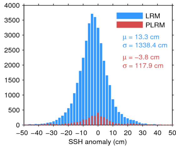
Figure 7. Histogram of flag-valid SSH anomaly over oceans and lakes for LRM (blue) and PLRM (red) for 15/06/2016. The mean ( \mu ) and standard deviation ( \sigma ) are also shown. Note that values outside [-50 50] cm are excluded from the histogram for the sake of readability but not from the computation of \mu and \sigma .
