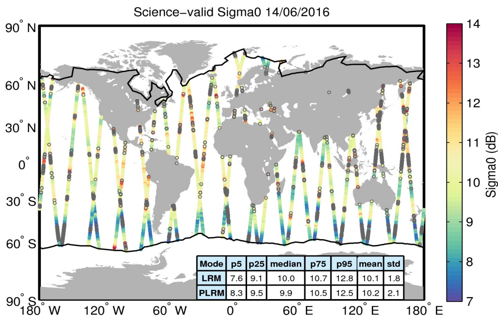
Figure 27. Geographical distribution of science-valid sigma0 data over oceans and lakes for 14/06/2016. The statistical values shown in the table refer to the sigma0 in dB and are calculated separately for LRM and PLRM regions. The black lines mark the outer limit of the Arctic and Antarctic polar polygons. Gray circles denote records that have been rejected based on the editing criteria described in Table 4.
