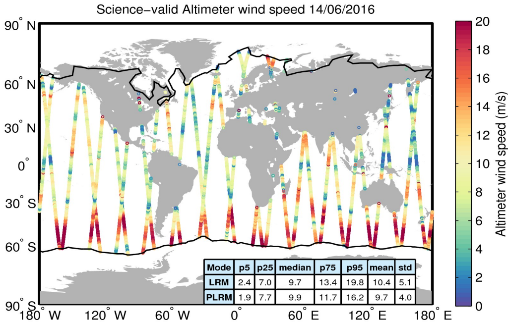
Figure 34. Geographical distribution of science-valid wind data over oceans and lakes for 14/06/2016. The statistical values shown in the table refer to the wind in m/s and are calculated separately for LRM and PLRM regions. The black lines mark the outer limit of the Arctic and Antarctic polar polygons. Gray circles denote records that have been rejected based on the editing criteria described in Table 5.
