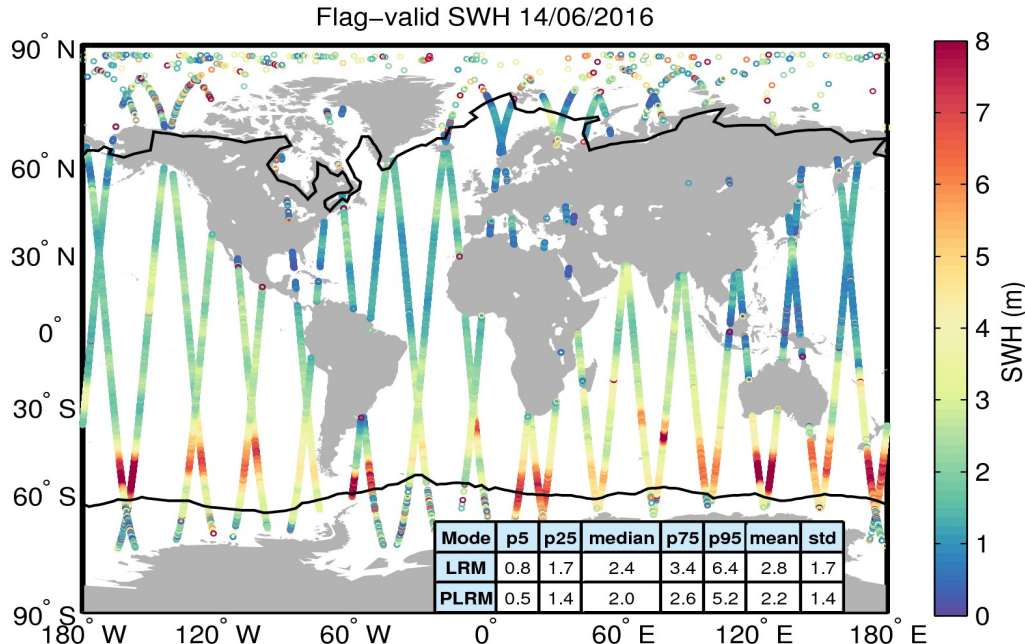
Figure 15. Geographical distribution of flag-valid SWH data over oceans and lakes for 14/06/2016. The statistical values shown in the table refer to the SWH in m and are calculated separately for LRM and PLRM regions. Measurements taken over polar polygons have been excluded from the computation of the statistical values. The black lines mark the outer limit of the Arctic and Antarctic polar polygons.
