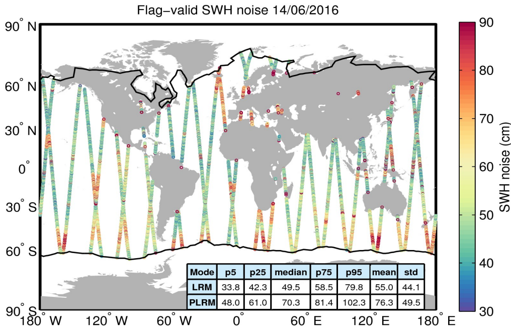
Figure 18. Geographical distribution of flag-valid 20-Hz SWH measurement noise over oceans and lakes for 14/06/2016. The statistical values shown in the table refer to the SWH noise and are calculated separately for LRM and PLRM regions. Measurements taken over polar polygons have been excluded from the computation of the statistical values. The black lines mark the outer limit of the Arctic and Antarctic polar polygons.
