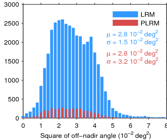
Figure 39. Histogram of flag-valid mispointing over oceans and lakes for LRM (blue) and PLRM (red) for 14/06/2016. Only positive values have been considered. The mean ( \mu ) and standard deviation ( \sigma ) are also shown. Note that values larger than 8 \cdot 10^{-2} \text{ deg}^2 are excluded from the histogram for the sake of readability but not from the computation of \mu and \sigma .
