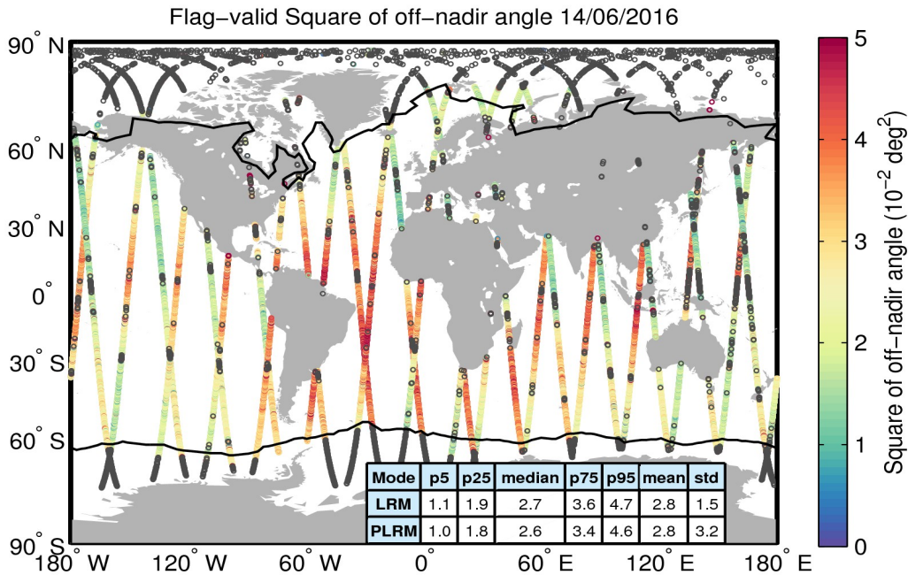
Figure 37. Geographical distribution of flag-valid mispointing data over oceans and lakes for 14/06/2016. The statistical values shown in the table refer to the mispointing in 10^{-2} deg 2 and are calculated separately for LRM and PLRM regions. Measurements taken over polar polygons have been excluded from the computation of the statistical values. The black lines mark the outer limit of the Arctic and Antarctic polar polygons. Gray circles denote negative values.
