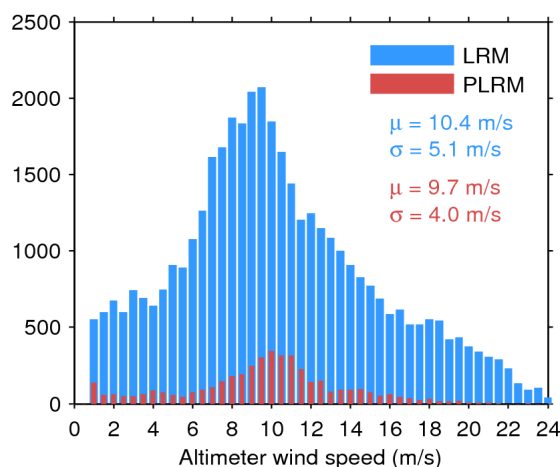
Figure 33. Histogram of flag-valid wind over oceans and lakes for LRM (blue) and PLRM (red) for 14/06/2016. The mean ( \mu ) and standard deviation ( \sigma ) are also shown. Note that values larger than 24 m/s are excluded from the histogram for the sake of readability but not from the computation of \mu and \sigma .
