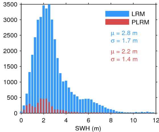
Figure 17. Histogram of flag-valid SWH over oceans and lakes for LRM (blue) and PLRM (red) for 14/06/2016. The mean ( \mu ) and standard deviation ( \sigma ) are also shown. Note that values larger than 12 m are excluded from the histogram for the sake of readability but not from the computation of \mu and \sigma .
