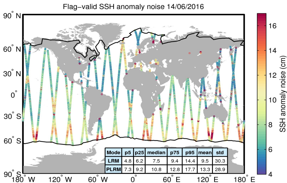
Figure 8. Geographical distribution of flag-valid 20-Hz SSH anomaly measurement noise over oceans and lakes for 14/06/2016. The statistical values shown in the table refer to the SSH anomaly noise and are calculated separately for LRM and PLRM regions. Measurements taken over polar polygons have been excluded from the computation of the statistical values. The black lines mark the outer limit of the Arctic and Antarctic polar polygons.
