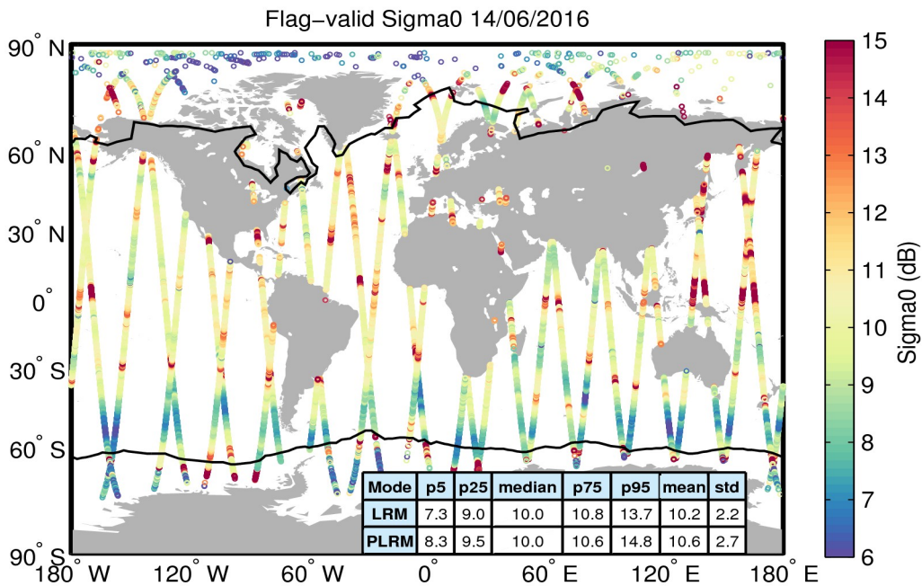
Figure 23. Geographical distribution of flag-valid sigma0 data over oceans and lakes for 14/06/2016. The statistical values shown in the table refer to the sigma0 in dB and are calculated separately for LRM and PLRM regions. Measurements taken over polar polygons have been excluded from the computation of the statistical values. The black lines mark the outer limit of the Arctic and Antarctic polar polygons.
