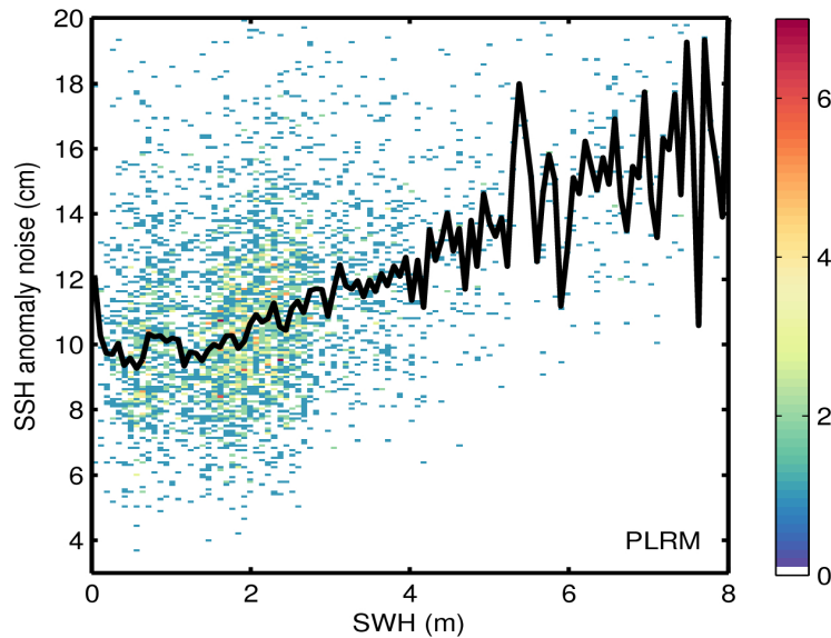
Figure 9. 2D histogram showing flag-valid SSH anomaly noise as a function of SWH for LRM (top) and PLRM (bottom) for 14/06/2016. The black line denotes the median SSH anomaly noise as a function of SWH.
