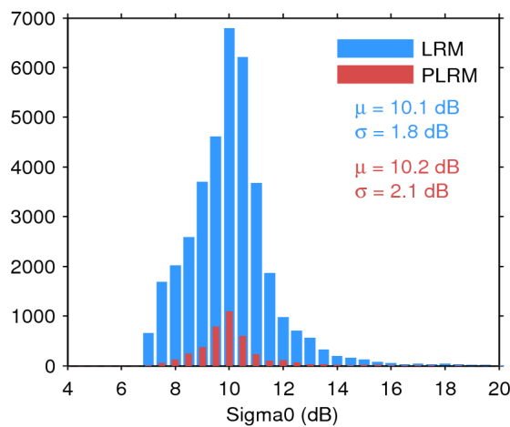
Figure 28. Histogram of science-valid sigma0 over oceans and lakes for LRM (blue) and PLRM (red) for 14/06/2016. The mean ( \mu ) and standard deviation ( \sigma ) are also shown. Note that values outside [4 20] dB are excluded from the histogram for the sake of readability but not from the computation of \mu and \sigma .
