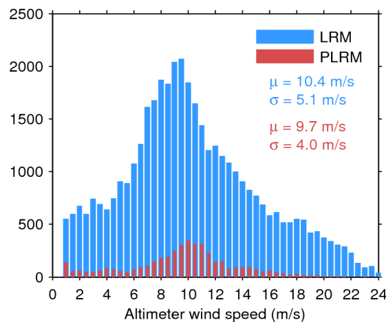
Figure 35. Histogram of science-valid wind over oceans and lakes for LRM (blue) and PLRM (red) for 14/06/2016. The mean ( \mu ) and standard deviation ( \sigma ) are also shown. Note that values larger than 24 m/s are excluded from the histogram for the sake of readability but not from the computation of \mu and \sigma .
