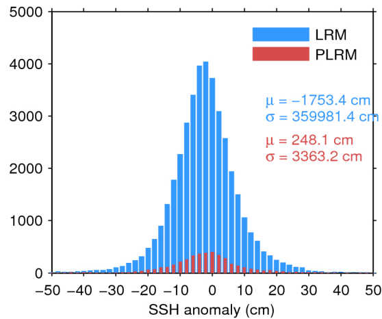
Figure 7. Histogram of flag-valid SSH anomaly over oceans and lakes for LRM (blue) and PLRM (red) for 14/06/2016. The mean ( \mu ) and standard deviation ( \sigma ) are also shown. Note that values outside [-50 50] cm are excluded from the histogram for the sake of readability but not from the computation of \mu and \sigma .
