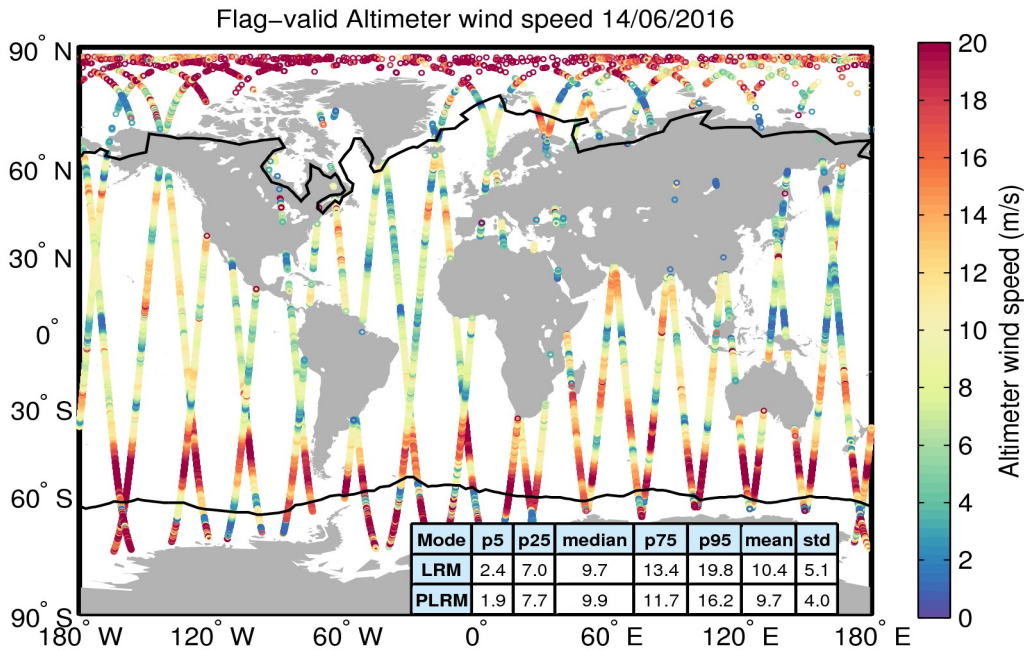
Figure 31. Geographical distribution of flag-valid wind data over oceans and lakes for 14/06/2016. The statistical values shown in the table refer to the wind in m/s and are calculated separately for LRM and PLRM regions. Measurements taken over polar polygons have been excluded from the computation of the statistical values. The black lines mark the outer limit of the Arctic and Antarctic polar polygons.
