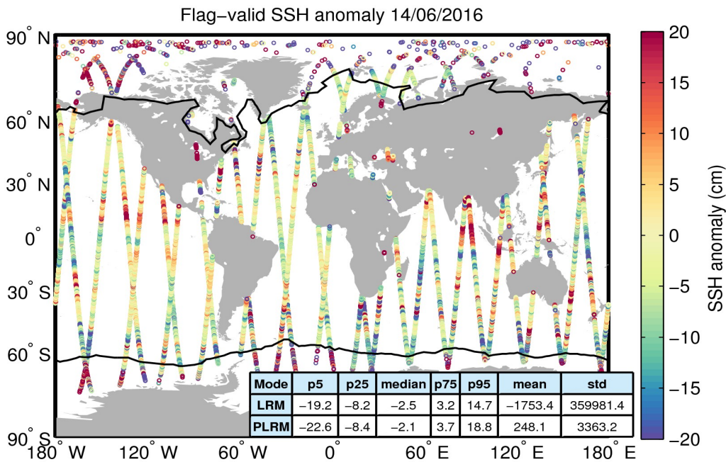
Figure 5. Geographical distribution of flag-valid 1-Hz SSH anomaly data over oceans and lakes for 14/06/2016. The statistical values shown in the table refer to the SSH anomaly in cm and are calculated separately for LRM and PLRM regions. Measurements taken over polar polygons have been excluded from the computation of the statistical values. The black lines mark the outer limit of the Arctic and Antarctic polar polygons.
