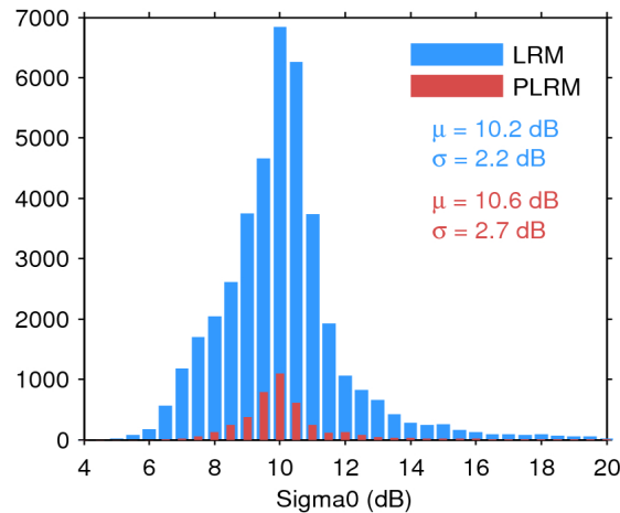
Figure 25. Histogram of flag-valid sigma0 over oceans and lakes for LRM (blue) and PLRM (red) for 14/06/2016. The mean ( \mu ) and standard deviation ( \sigma ) are also shown. Note that values outside [4 20] dB are excluded from the histogram for the sake of readability but not from the computation of \mu and \sigma .
