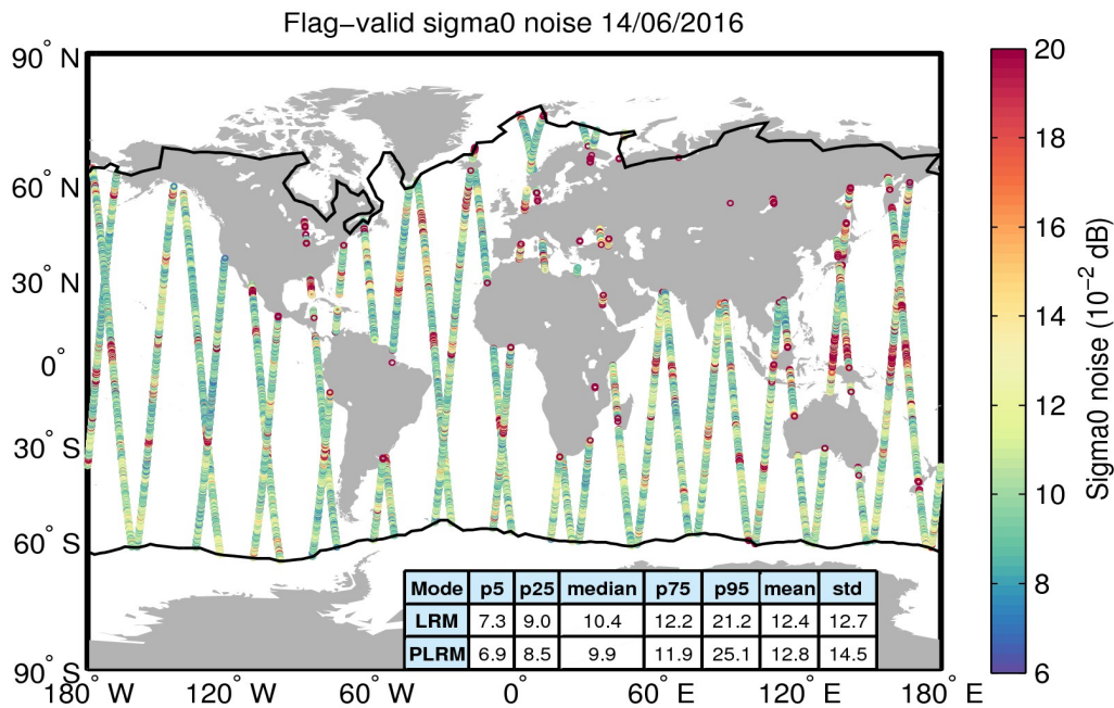
Figure 26. Geographical distribution of flag-valid 20-Hz sigma0 measurement noise over oceans and lakes for 14/06/2016. The statistical values shown in the table refer to the sigma0 noise and are calculated separately for LRM and PLRM regions. Measurements taken over polar polygons have been excluded from the computation of the statistical values. The black lines mark the outer limit of the Arctic and Antarctic polar polygons.
