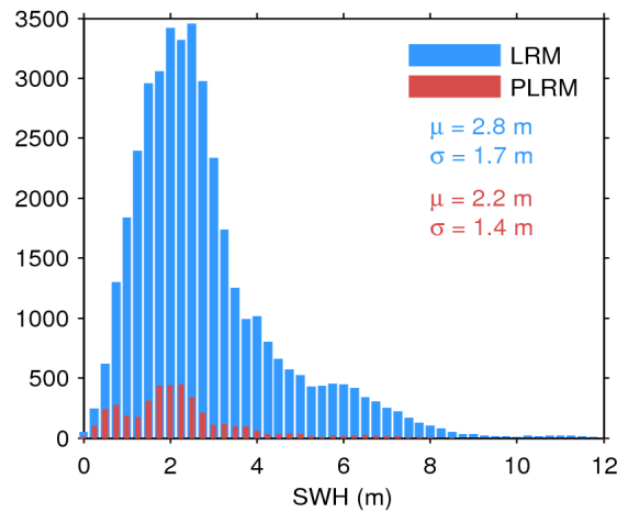
Figure 20. Histogram of science-valid SWH over oceans and lakes for LRM (blue) and PLRM (red) for 14/06/2016. The mean ( \mu ) and standard deviation ( \sigma ) are also shown. Note that values larger than 12 m are excluded from the histogram for the sake of readability but not from the computation of \mu and \sigma .
