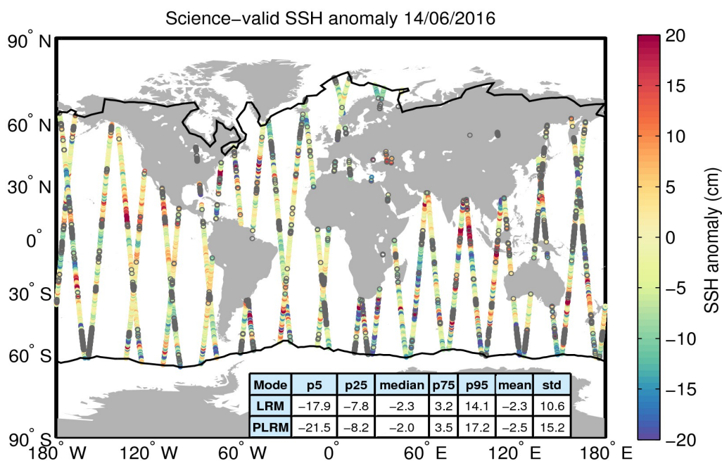
Figure 10. Geographical distribution of science-valid SSH anomaly data over oceans and lakes for 14/06/2016. The statistical values shown in the table refer to the SSH anomaly in cm and are calculated separately for LRM and PLRM regions. The black lines mark the outer limit of the Arctic and Antarctic polar polygons. Gray circles denote records that have been rejected based on the editing criteria described in Table 2.
