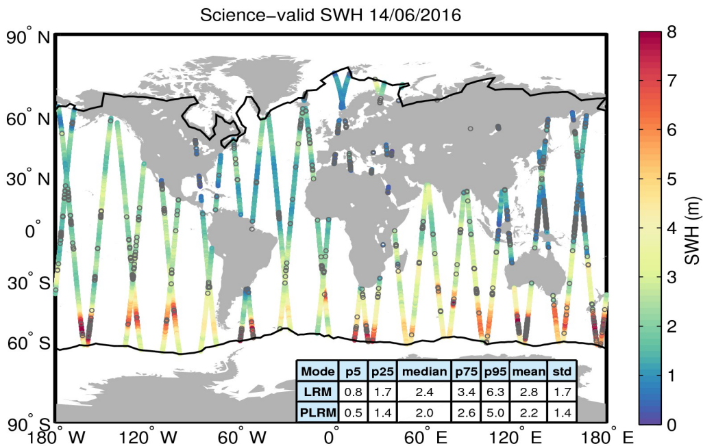
Figure 19. Geographical distribution of science-valid SWH data over oceans and lakes for 14/06/2016. The statistical values shown in the table refer to the SWH in m and are calculated separately for LRM and PLRM regions. The black lines mark the outer limit of the Arctic and Antarctic polar polygons. Gray circles denote records that have been rejected based on the editing criteria described in Table 3.
