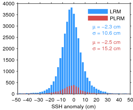
Figure 11. Histogram of science-valid SSH anomaly over oceans and lakes for LRM (blue) and PLRM (red) for 14/06/2016. The mean ( \mu ) and standard deviation ( \sigma ) are also shown. Note that values outside [-50 50] cm are excluded from the histogram for the sake of readability but not from the computation of \mu and \sigma .
