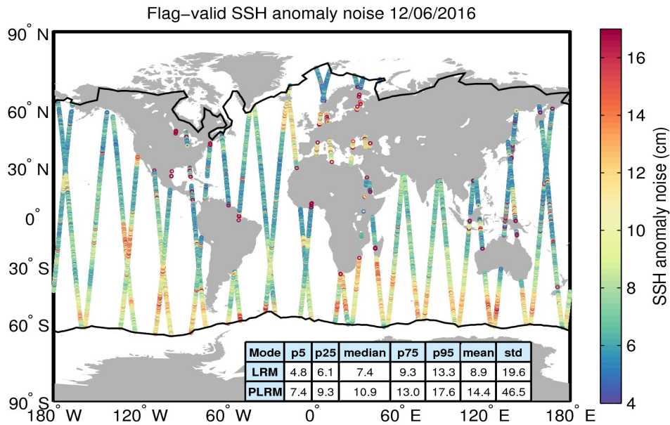
Figure 8. Geographical distribution of flag-valid 20-Hz SSH anomaly measurement noise over oceans and lakes for 12/06/2016. The statistical values shown in the table refer to the SSH anomaly noise and are calculated separately for LRM and PLRM regions. Measurements taken over polar polygons have been excluded from the computation of the statistical values. The black lines mark the outer limit of the Arctic and Antarctic polar polygons.
