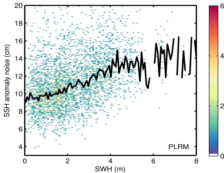
Figure 9. 2D histogram showing flag-valid SSH anomaly noise as a function of SWH for LRM (top) and PLRM (bottom) for 12/06/2016. The black line denotes the median SSH anomaly noise as a function of SWH.
