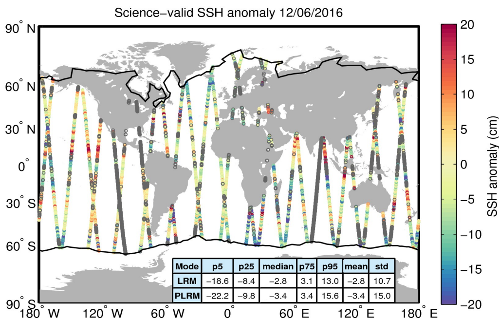
Figure 10. Geographical distribution of science-valid SSH anomaly data over oceans and lakes for 12/06/2016. The statistical values shown in the table refer to the SSH anomaly in cm and are calculated separately for LRM and PLRM regions. The black lines mark the outer limit of the Arctic and Antarctic polar polygons. Gray circles denote records that have been rejected based on the editing criteria described in Table 2.
