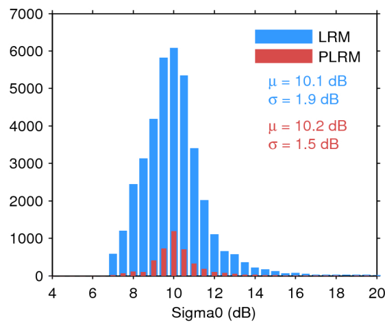
Figure 28. Histogram of science-valid sigma0 over oceans and lakes for LRM (blue) and PLRM (red) for 12/06/2016. The mean ( \mu ) and standard deviation ( \sigma ) are also shown. Note that values outside [4 20] dB are excluded from the histogram for the sake of readability but not from the computation of \mu and \sigma .
