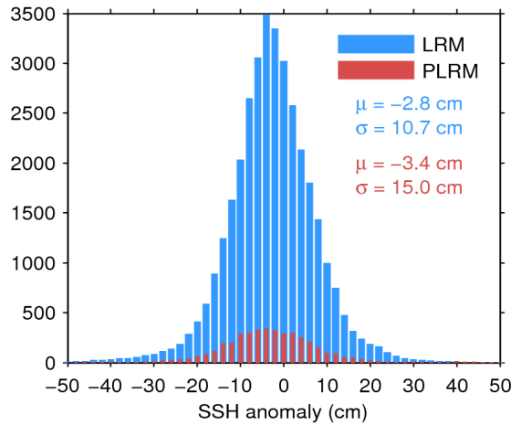
Figure 11. Histogram of science-valid SSH anomaly over oceans and lakes for LRM (blue) and PLRM (red) for 12/06/2016. The mean ( \mu ) and standard deviation ( \sigma ) are also shown. Note that values outside [-50 50] cm are excluded from the histogram for the sake of readability but not from the computation of \mu and \sigma .
