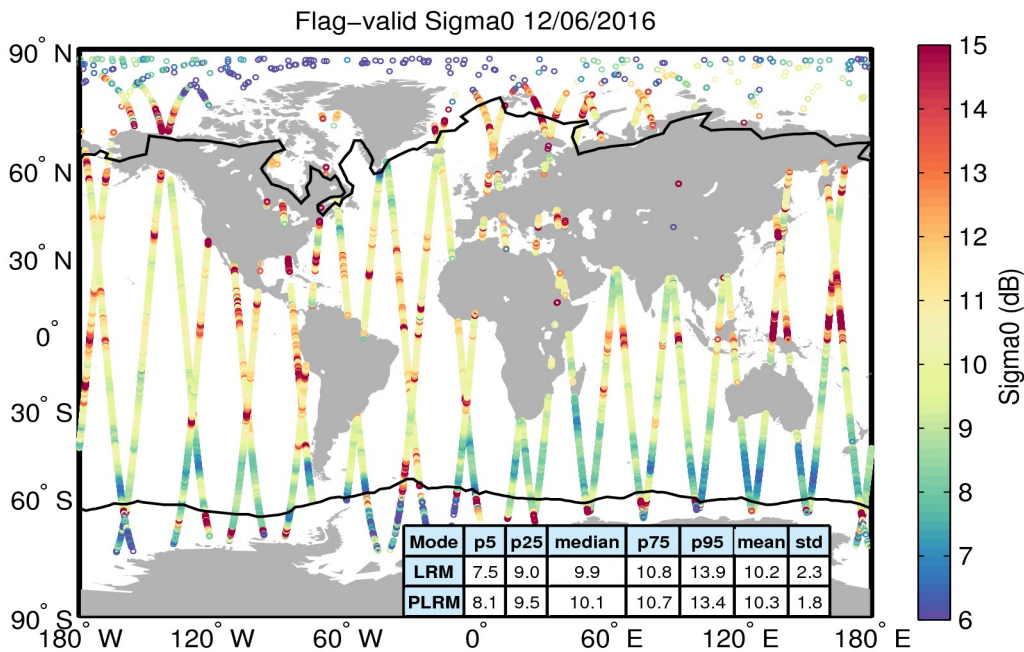
Figure 23. Geographical distribution of flag-valid sigma0 data over oceans and lakes for 12/06/2016. The statistical values shown in the table refer to the sigma0 in dB and are calculated separately for LRM and PLRM regions. Measurements taken over polar polygons have been excluded from the computation of the statistical values. The black lines mark the outer limit of the Arctic and Antarctic polar polygons.
