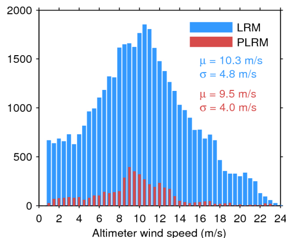
Figure 35. Histogram of science-valid wind over oceans and lakes for LRM (blue) and PLRM (red) for 12/06/2016. The mean ( \mu ) and standard deviation ( \sigma ) are also shown. Note that values larger than 24 m/s are excluded from the histogram for the sake of readability but not from the computation of \mu and \sigma .
