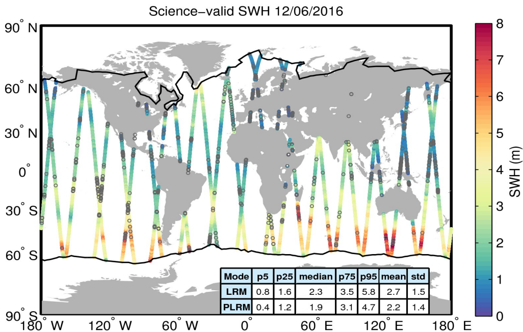
Figure 19. Geographical distribution of science-valid SWH data over oceans and lakes for 12/06/2016. The statistical values shown in the table refer to the SWH in m and are calculated separately for LRM and PLRM regions. The black lines mark the outer limit of the Arctic and Antarctic polar polygons. Gray circles denote records that have been rejected based on the editing criteria described in Table 3.
