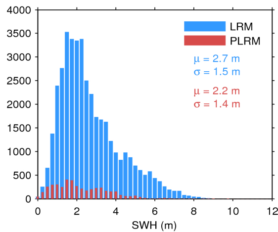
Figure 20. Histogram of science-valid SWH over oceans and lakes for LRM (blue) and PLRM (red) for 12/06/2016. The mean ( \mu ) and standard deviation ( \sigma ) are also shown. Note that values larger than 12 m are excluded from the histogram for the sake of readability but not from the computation of \mu and \sigma .
