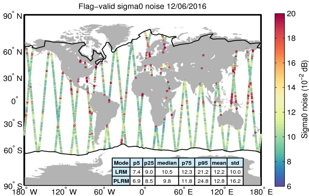
Figure 26. Geographical distribution of flag-valid 20-Hz sigma0 measurement noise over oceans and lakes for 12/06/2016. The statistical values shown in the table refer to the sigma0 noise and are calculated separately for LRM and PLRM regions. Measurements taken over polar polygons have been excluded from the computation of the statistical values. The black lines mark the outer limit of the Arctic and Antarctic polar polygons.
