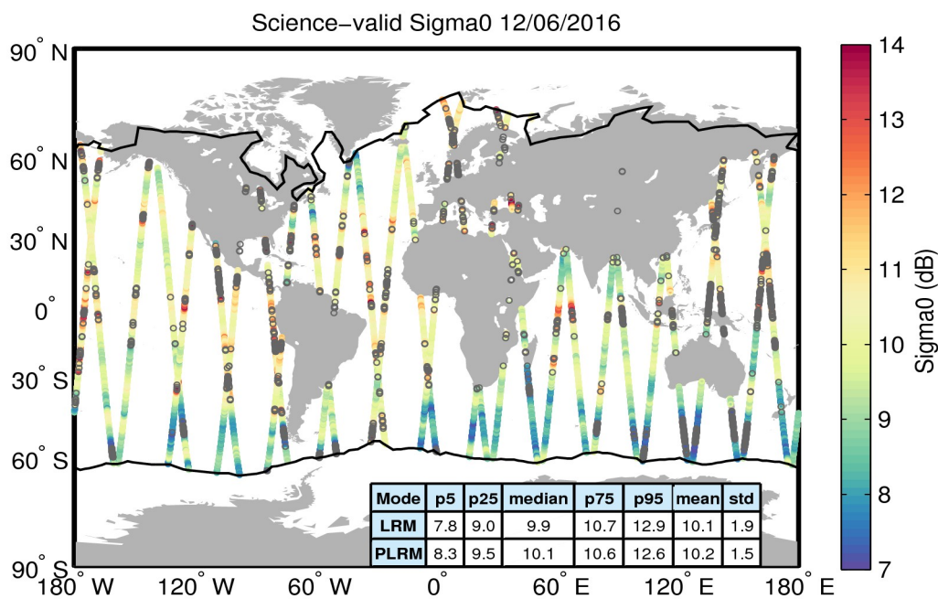
Figure 27. Geographical distribution of science-valid sigma0 data over oceans and lakes for 12/06/2016. The statistical values shown in the table refer to the sigma0 in dB and are calculated separately for LRM and PLRM regions. The black lines mark the outer limit of the Arctic and Antarctic polar polygons. Gray circles denote records that have been rejected based on the editing criteria described in Table 4.
