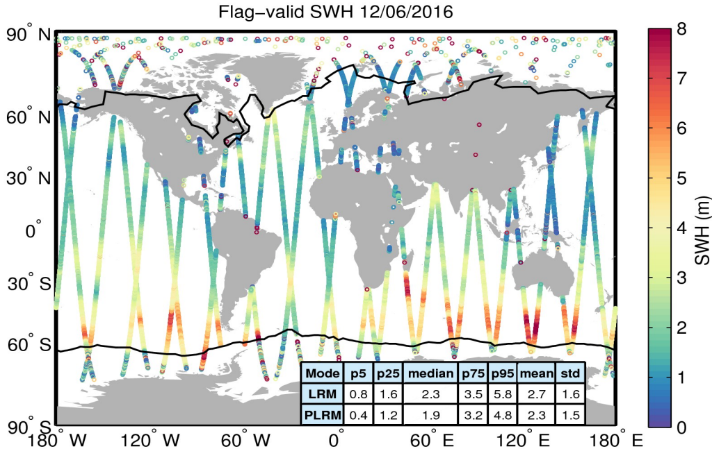
Figure 15. Geographical distribution of flag-valid SWH data over oceans and lakes for 12/06/2016. The statistical values shown in the table refer to the SWH in m and are calculated separately for LRM and PLRM regions. Measurements taken over polar polygons have been excluded from the computation of the statistical values. The black lines mark the outer limit of the Arctic and Antarctic polar polygons.
