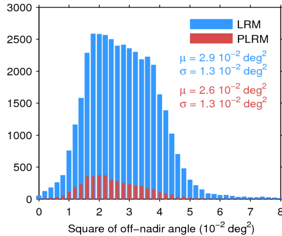
Figure 39. Histogram of flag-valid mispointing over oceans and lakes for LRM (blue) and PLRM (red) for 12/06/2016. Only positive values have been considered. The mean ( \mu ) and standard deviation ( \sigma ) are also shown. Note that values larger than 8 \cdot 10^{-2} \text{ deg}^2 are excluded from the histogram for the sake of readability but not from the computation of \mu and \sigma .
