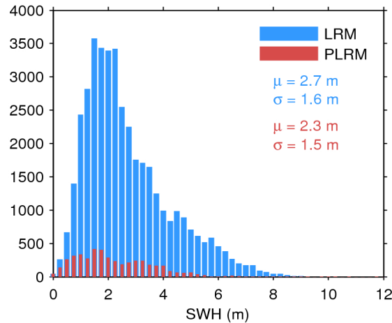
Figure 17. Histogram of flag-valid SWH over oceans and lakes for LRM (blue) and PLRM (red) for 12/06/2016. The mean ( \mu ) and standard deviation ( \sigma ) are also shown. Note that values larger than 12 m are excluded from the histogram for the sake of readability but not from the computation of \mu and \sigma .
