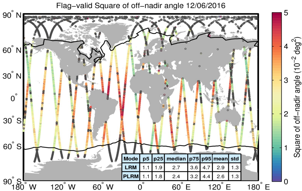
Figure 37. Geographical distribution of flag-valid mispointing data over oceans and lakes for 12/06/2016. The statistical values shown in the table refer to the mispointing in 10^{-2} deg 2 and are calculated separately for LRM and PLRM regions. Measurements taken over polar polygons have been excluded from the computation of the statistical values. The black lines mark the outer limit of the Arctic and Antarctic polar polygons. Gray circles denote negative values.
