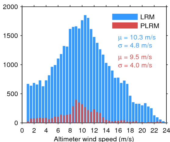
Figure 33. Histogram of flag-valid wind over oceans and lakes for LRM (blue) and PLRM (red) for 12/06/2016. The mean ( \mu ) and standard deviation ( \sigma ) are also shown. Note that values larger than 24 m/s are excluded from the histogram for the sake of readability but not from the computation of \mu and \sigma .
