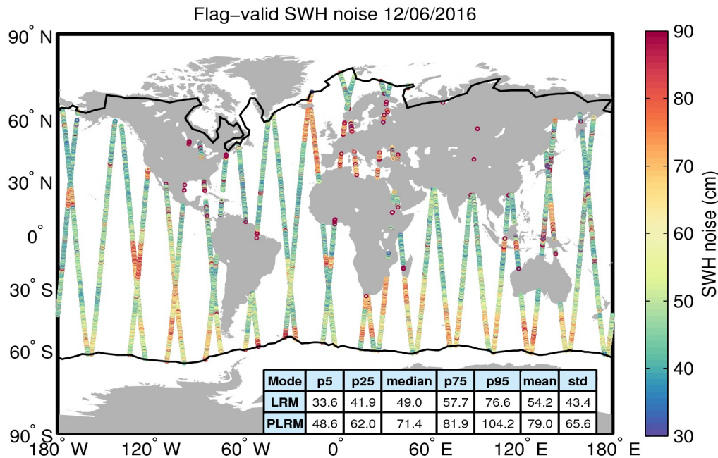
Figure 18. Geographical distribution of flag-valid 20-Hz SWH measurement noise over oceans and lakes for 12/06/2016. The statistical values shown in the table refer to the SWH noise and are calculated separately for LRM and PLRM regions. Measurements taken over polar polygons have been excluded from the computation of the statistical values. The black lines mark the outer limit of the Arctic and Antarctic polar polygons.
