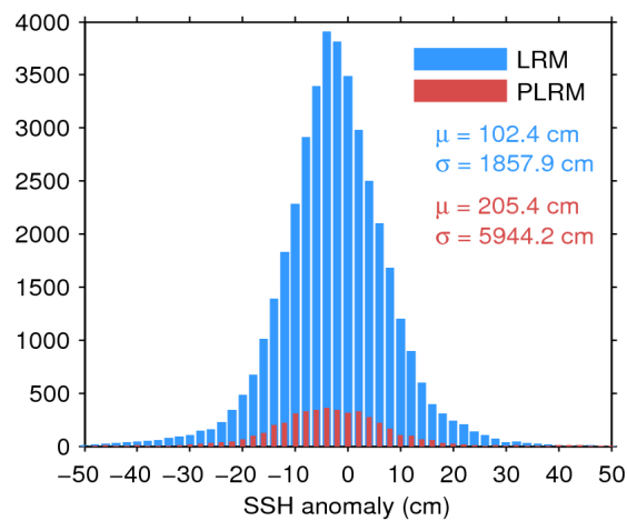
Figure 7. Histogram of flag-valid SSH anomaly over oceans and lakes for LRM (blue) and PLRM (red) for 12/06/2016. The mean ( \mu ) and standard deviation ( \sigma ) are also shown. Note that values outside [-50 50] cm are excluded from the histogram for the sake of readability but not from the computation of \mu and \sigma .
