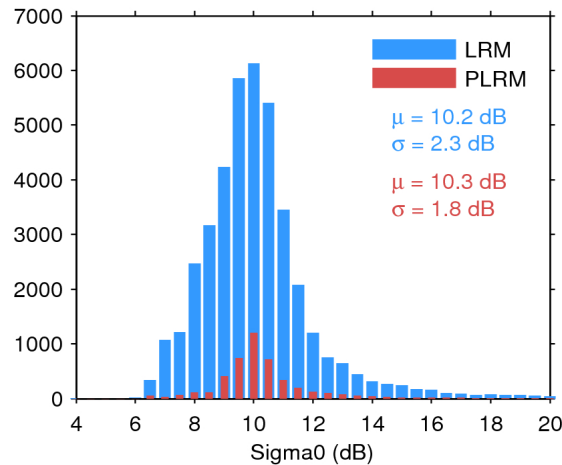
Figure 25. Histogram of flag-valid sigma0 over oceans and lakes for LRM (blue) and PLRM (red) for 12/06/2016. The mean ( \mu ) and standard deviation ( \sigma ) are also shown. Note that values outside [4 20] dB are excluded from the histogram for the sake of readability but not from the computation of \mu and \sigma .
