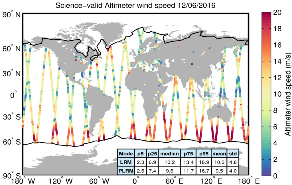
Figure 34. Geographical distribution of science-valid wind data over oceans and lakes for 12/06/2016. The statistical values shown in the table refer to the wind in m/s and are calculated separately for LRM and PLRM regions. The black lines mark the outer limit of the Arctic and Antarctic polar polygons. Gray circles denote records that have been rejected based on the editing criteria described in Table 5.
