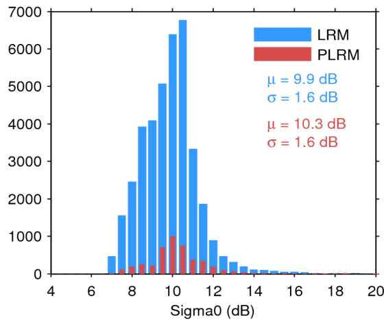
Figure 28. Histogram of science-valid sigma0 over oceans and lakes for LRM (blue) and PLRM (red) for 10/06/2016. The mean ( \mu ) and standard deviation ( \sigma ) are also shown. Note that values outside [4 20] dB are excluded from the histogram for the sake of readability but not from the computation of \mu and \sigma .
