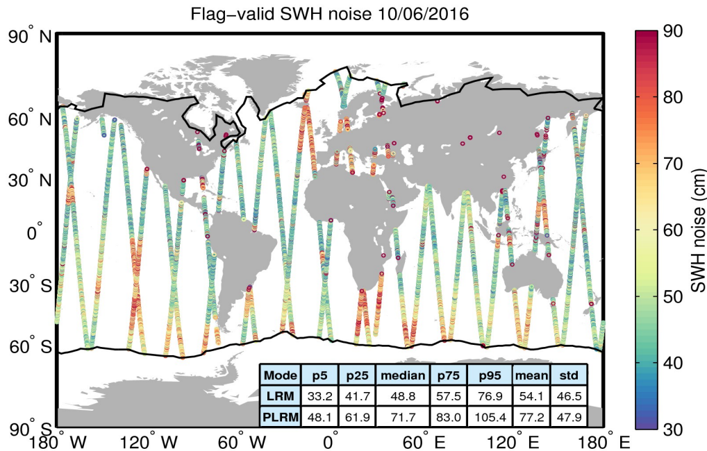
Figure 18. Geographical distribution of flag-valid 20-Hz SWH measurement noise over oceans and lakes for 10/06/2016. The statistical values shown in the table refer to the SWH noise and are calculated separately for LRM and PLRM regions. Measurements taken over polar polygons have been excluded from the computation of the statistical values. The black lines mark the outer limit of the Arctic and Antarctic polar polygons.
