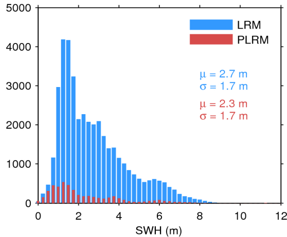
Figure 17. Histogram of flag-valid SWH over oceans and lakes for LRM (blue) and PLRM (red) for 10/06/2016. The mean ( \mu ) and standard deviation ( \sigma ) are also shown. Note that values larger than 12 m are excluded from the histogram for the sake of readability but not from the computation of \mu and \sigma .
