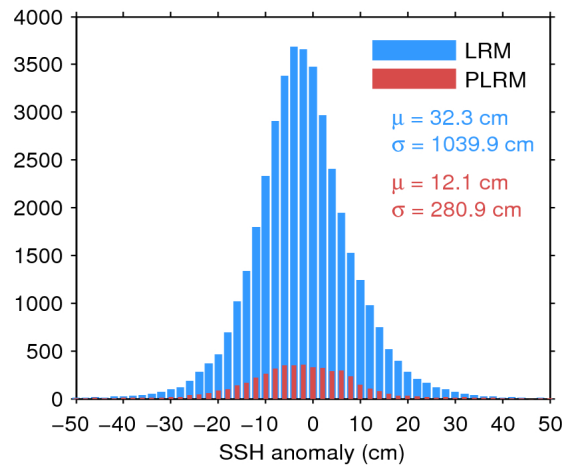
Figure 7. Histogram of flag-valid SSH anomaly over oceans and lakes for LRM (blue) and PLRM (red) for 10/06/2016. The mean ( \mu ) and standard deviation ( \sigma ) are also shown. Note that values outside [-50 50] cm are excluded from the histogram for the sake of readability but not from the computation of \mu and \sigma .
