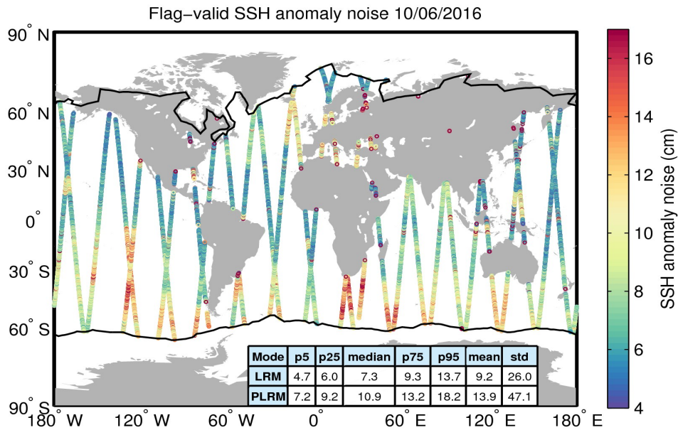
Figure 8. Geographical distribution of flag-valid 20-Hz SSH anomaly measurement noise over oceans and lakes for 10/06/2016. The statistical values shown in the table refer to the SSH anomaly noise and are calculated separately for LRM and PLRM regions. Measurements taken over polar polygons have been excluded from the computation of the statistical values. The black lines mark the outer limit of the Arctic and Antarctic polar polygons.
