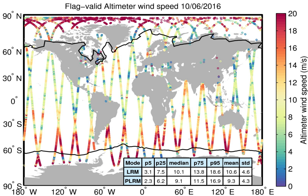
Figure 31. Geographical distribution of flag-valid wind data over oceans and lakes for 10/06/2016. The statistical values shown in the table refer to the wind in m/s and are calculated separately for LRM and PLRM regions. Measurements taken over polar polygons have been excluded from the computation of the statistical values. The black lines mark the outer limit of the Arctic and Antarctic polar polygons.
