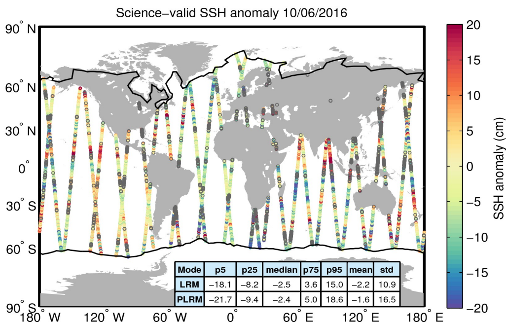
Figure 10. Geographical distribution of science-valid SSH anomaly data over oceans and lakes for 10/06/2016. The statistical values shown in the table refer to the SSH anomaly in cm and are calculated separately for LRM and PLRM regions. The black lines mark the outer limit of the Arctic and Antarctic polar polygons. Gray circles denote records that have been rejected based on the editing criteria described in Table 2.
