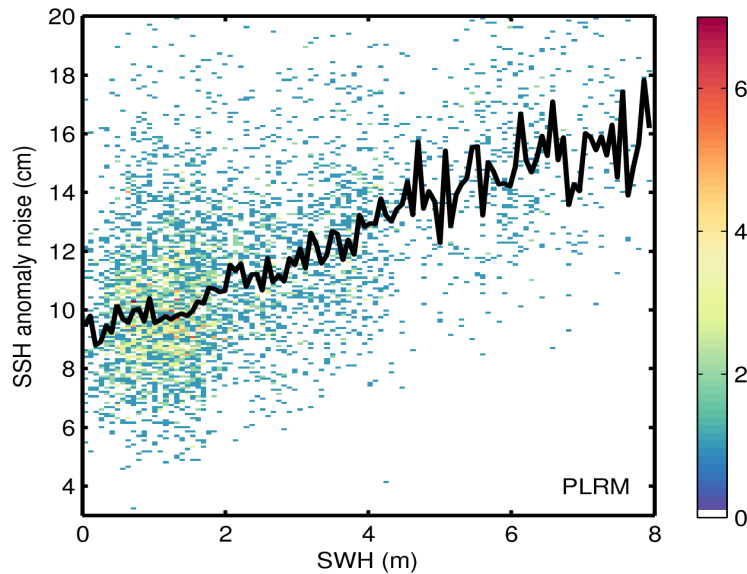
Figure 9. 2D histogram showing flag-valid SSH anomaly noise as a function of SWH for LRM (top) and PLRM (bottom) for 10/06/2016. The black line denotes the median SSH anomaly noise as a function of SWH.
