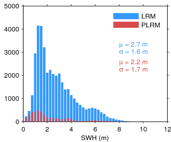
Figure 20. Histogram of science-valid SWH over oceans and lakes for LRM (blue) and PLRM (red) for 10/06/2016. The mean ( \mu ) and standard deviation ( \sigma ) are also shown. Note that values larger than 12 m are excluded from the histogram for the sake of readability but not from the computation of \mu and \sigma .
