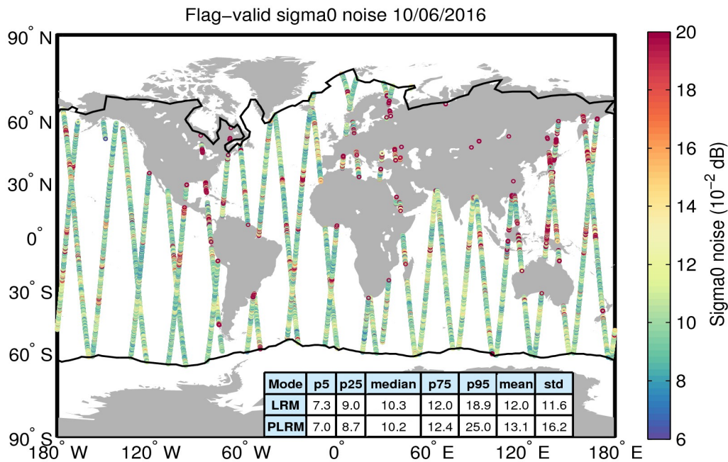
Figure 26. Geographical distribution of flag-valid 20-Hz sigma0 measurement noise over oceans and lakes for 10/06/2016. The statistical values shown in the table refer to the sigma0 noise and are calculated separately for LRM and PLRM regions. Measurements taken over polar polygons have been excluded from the computation of the statistical values. The black lines mark the outer limit of the Arctic and Antarctic polar polygons.
