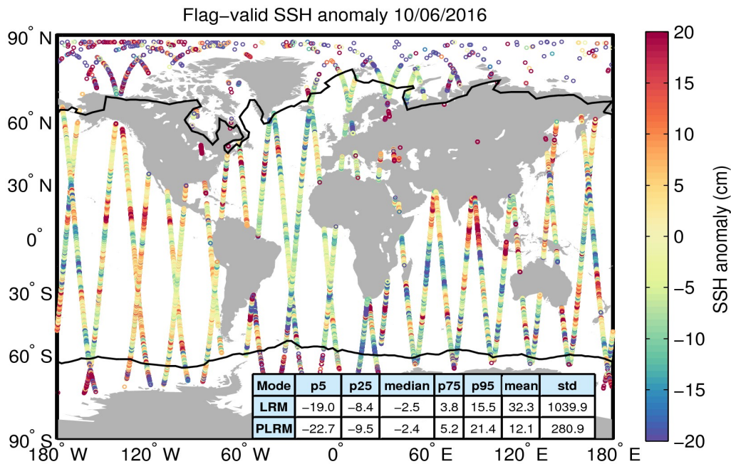
Figure 5. Geographical distribution of flag-valid 1-Hz SSH anomaly data over oceans and lakes for 10/06/2016. The statistical values shown in the table refer to the SSH anomaly in cm and are calculated separately for LRM and PLRM regions. Measurements taken over polar polygons have been excluded from the computation of the statistical values. The black lines mark the outer limit of the Arctic and Antarctic polar polygons.
