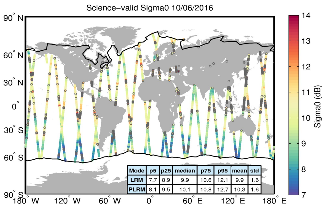
Figure 27. Geographical distribution of science-valid sigma0 data over oceans and lakes for 10/06/2016. The statistical values shown in the table refer to the sigma0 in dB and are calculated separately for LRM and PLRM regions. The black lines mark the outer limit of the Arctic and Antarctic polar polygons. Gray circles denote records that have been rejected based on the editing criteria described in Table 4.
