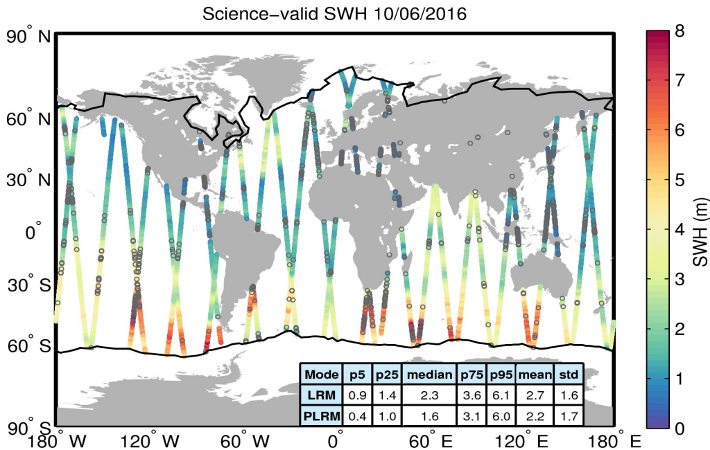
Figure 19. Geographical distribution of science-valid SWH data over oceans and lakes for 10/06/2016. The statistical values shown in the table refer to the SWH in m and are calculated separately for LRM and PLRM regions. The black lines mark the outer limit of the Arctic and Antarctic polar polygons. Gray circles denote records that have been rejected based on the editing criteria described in Table 3.
