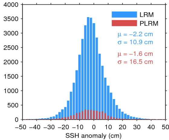
Figure 11. Histogram of science-valid SSH anomaly over oceans and lakes for LRM (blue) and PLRM (red) for 10/06/2016. The mean ( \mu ) and standard deviation ( \sigma ) are also shown. Note that values outside [-50 50] cm are excluded from the histogram for the sake of readability but not from the computation of \mu and \sigma .
