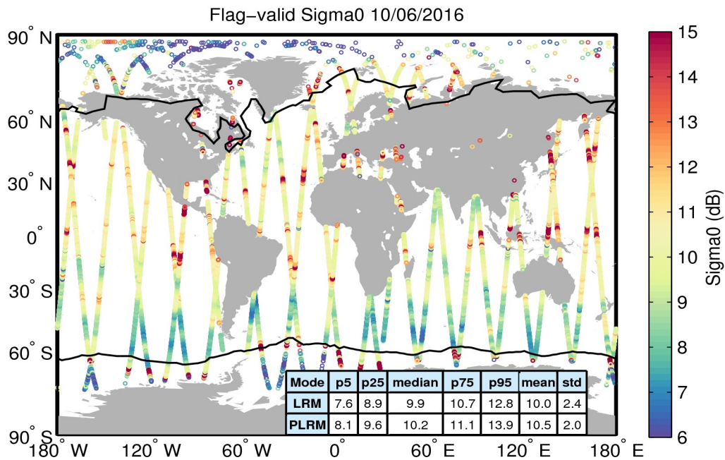
Figure 23. Geographical distribution of flag-valid sigma0 data over oceans and lakes for 10/06/2016. The statistical values shown in the table refer to the sigma0 in dB and are calculated separately for LRM and PLRM regions. Measurements taken over polar polygons have been excluded from the computation of the statistical values. The black lines mark the outer limit of the Arctic and Antarctic polar polygons.
