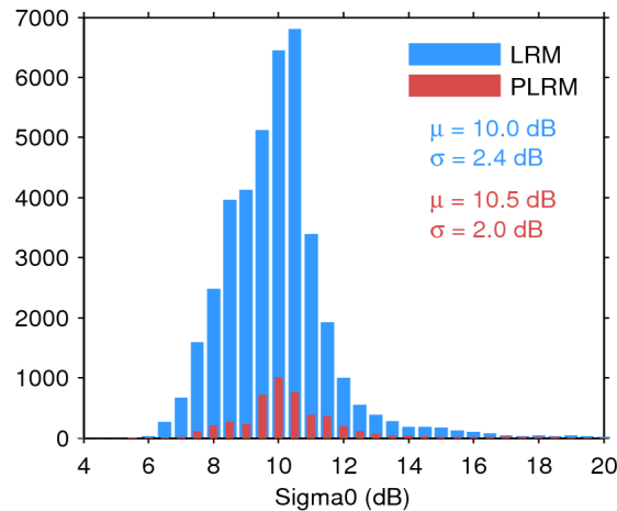
Figure 25. Histogram of flag-valid sigma0 over oceans and lakes for LRM (blue) and PLRM (red) for 10/06/2016. The mean ( \mu ) and standard deviation ( \sigma ) are also shown. Note that values outside [4 20] dB are excluded from the histogram for the sake of readability but not from the computation of \mu and \sigma .
