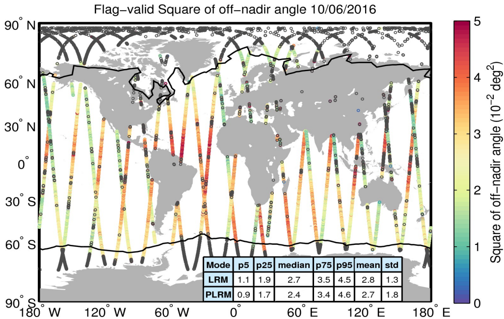
Figure 37. Geographical distribution of flag-valid mispointing data over oceans and lakes for 10/06/2016. The statistical values shown in the table refer to the mispointing in 10^{-2} deg 2 and are calculated separately for LRM and PLRM regions. Measurements taken over polar polygons have been excluded from the computation of the statistical values. The black lines mark the outer limit of the Arctic and Antarctic polar polygons. Gray circles denote negative values.
