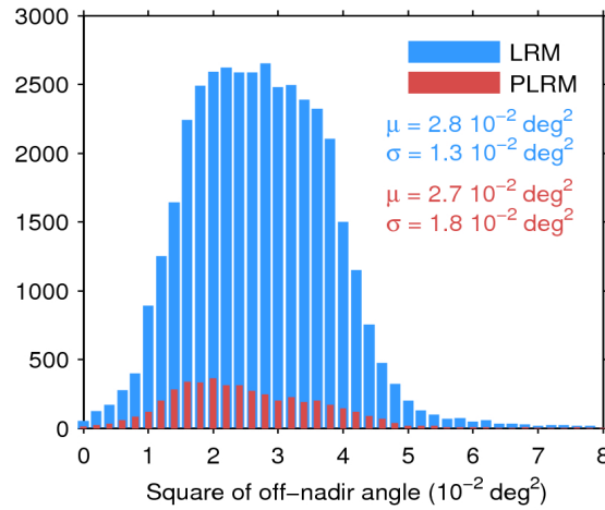
Figure 39. Histogram of flag-valid mispointing over oceans and lakes for LRM (blue) and PLRM (red) for 10/06/2016. Only positive values have been considered. The mean ( \mu ) and standard deviation ( \sigma ) are also shown. Note that values larger than 8 \times 10^{-2} \text{ deg}^2 are excluded from the histogram for the sake of readability but not from the computation of \mu and \sigma .
