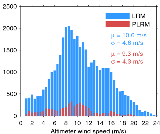
Figure 33. Histogram of flag-valid wind over oceans and lakes for LRM (blue) and PLRM (red) for 10/06/2016. The mean ( \mu ) and standard deviation ( \sigma ) are also shown. Note that values larger than 24 m/s are excluded from the histogram for the sake of readability but not from the computation of \mu and \sigma .
