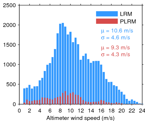
Figure 35. Histogram of science-valid wind over oceans and lakes for LRM (blue) and PLRM (red) for 10/06/2016. The mean ( \mu ) and standard deviation ( \sigma ) are also shown. Note that values larger than 24 m/s are excluded from the histogram for the sake of readability but not from the computation of \mu and \sigma .
