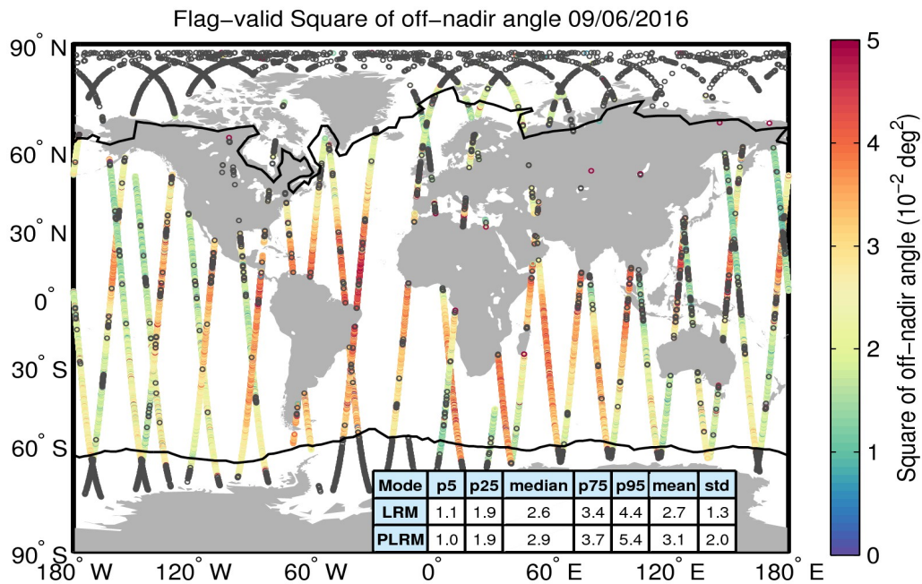
Figure 37. Geographical distribution of flag-valid mispointing data over oceans and lakes for 09/06/2016. The statistical values shown in the table refer to the mispointing in 10^{-2} deg 2 and are calculated separately for LRM and PLRM regions. Measurements taken over polar polygons have been excluded from the computation of the statistical values. The black lines mark the outer limit of the Arctic and Antarctic polar polygons. Gray circles denote negative values.
