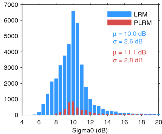
Figure 25. Histogram of flag-valid sigma0 over oceans and lakes for LRM (blue) and PLRM (red) for 09/06/2016. The mean ( \mu ) and standard deviation ( \sigma ) are also shown. Note that values outside [4 20] dB are excluded from the histogram for the sake of readability but not from the computation of \mu and \sigma .
