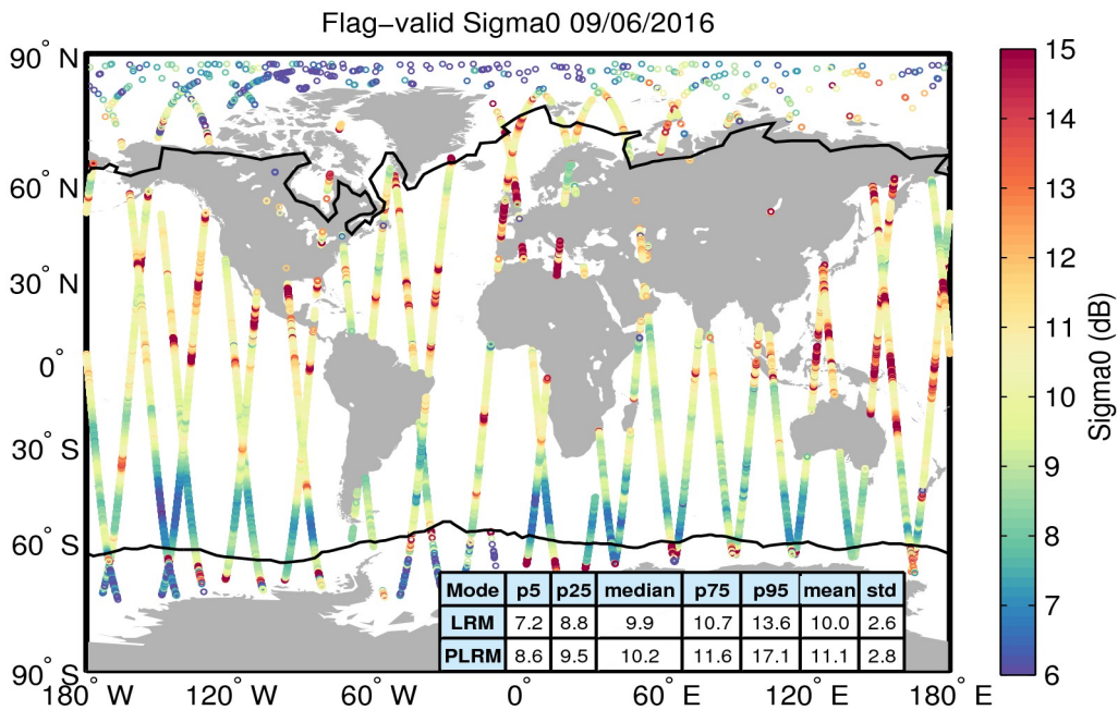
Figure 23. Geographical distribution of flag-valid sigma0 data over oceans and lakes for 09/06/2016. The statistical values shown in the table refer to the sigma0 in dB and are calculated separately for LRM and PLRM regions. Measurements taken over polar polygons have been excluded from the computation of the statistical values. The black lines mark the outer limit of the Arctic and Antarctic polar polygons.
