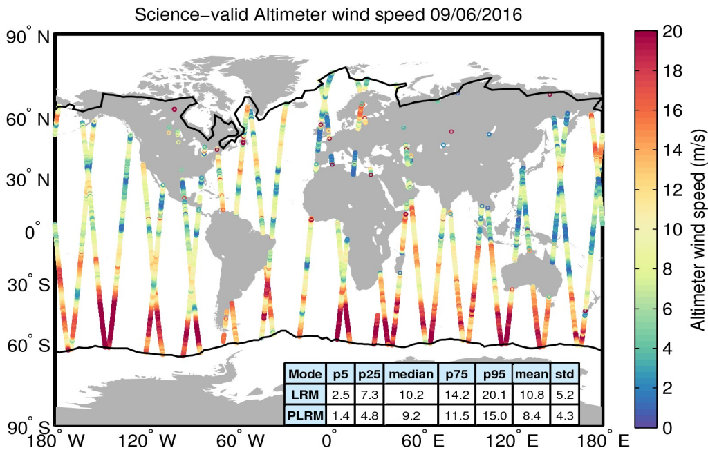
Figure 34. Geographical distribution of science-valid wind data over oceans and lakes for 09/06/2016. The statistical values shown in the table refer to the wind in m/s and are calculated separately for LRM and PLRM regions. The black lines mark the outer limit of the Arctic and Antarctic polar polygons. Gray circles denote records that have been rejected based on the editing criteria described in Table 5.
