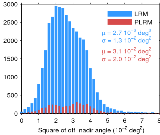
Figure 39. Histogram of flag-valid mispointing over oceans and lakes for LRM (blue) and PLRM (red) for 09/06/2016. Only positive values have been considered. The mean ( \mu ) and standard deviation ( \sigma ) are also shown. Note that values larger than 8 \cdot 10^{-2} \text{ deg}^2 are excluded from the histogram for the sake of readability but not from the computation of \mu and \sigma .
