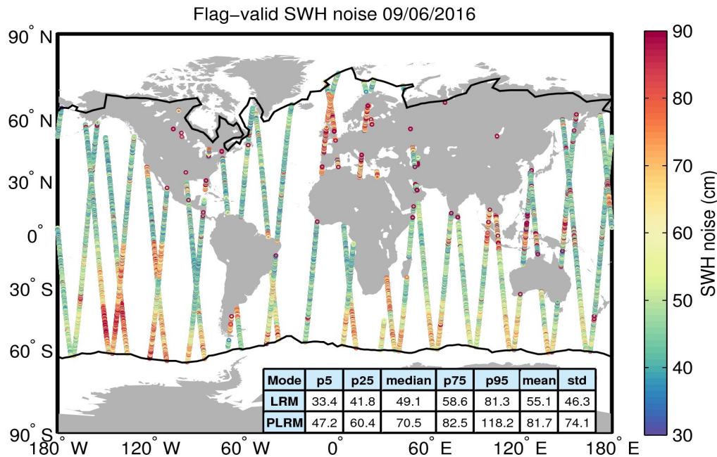
Figure 18. Geographical distribution of flag-valid 20-Hz SWH measurement noise over oceans and lakes for 09/06/2016. The statistical values shown in the table refer to the SWH noise and are calculated separately for LRM and PLRM regions. Measurements taken over polar polygons have been excluded from the computation of the statistical values. The black lines mark the outer limit of the Arctic and Antarctic polar polygons.
