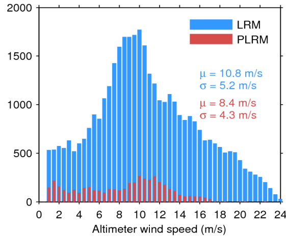
Figure 33. Histogram of flag-valid wind over oceans and lakes for LRM (blue) and PLRM (red) for 09/06/2016. The mean ( \mu ) and standard deviation ( \sigma ) are also shown. Note that values larger than 24 m/s are excluded from the histogram for the sake of readability but not from the computation of \mu and \sigma .
