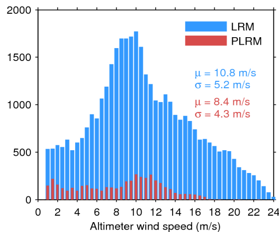
Figure 35. Histogram of science-valid wind over oceans and lakes for LRM (blue) and PLRM (red) for 09/06/2016. The mean ( \mu ) and standard deviation ( \sigma ) are also shown. Note that values larger than 24 m/s are excluded from the histogram for the sake of readability but not from the computation of \mu and \sigma .
