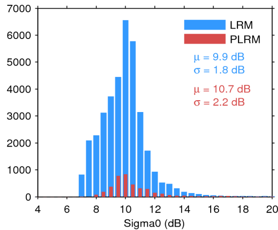
Figure 28. Histogram of science-valid sigma0 over oceans and lakes for LRM (blue) and PLRM (red) for 09/06/2016. The mean ( \mu ) and standard deviation ( \sigma ) are also shown. Note that values outside [4 20] dB are excluded from the histogram for the sake of readability but not from the computation of \mu and \sigma .
