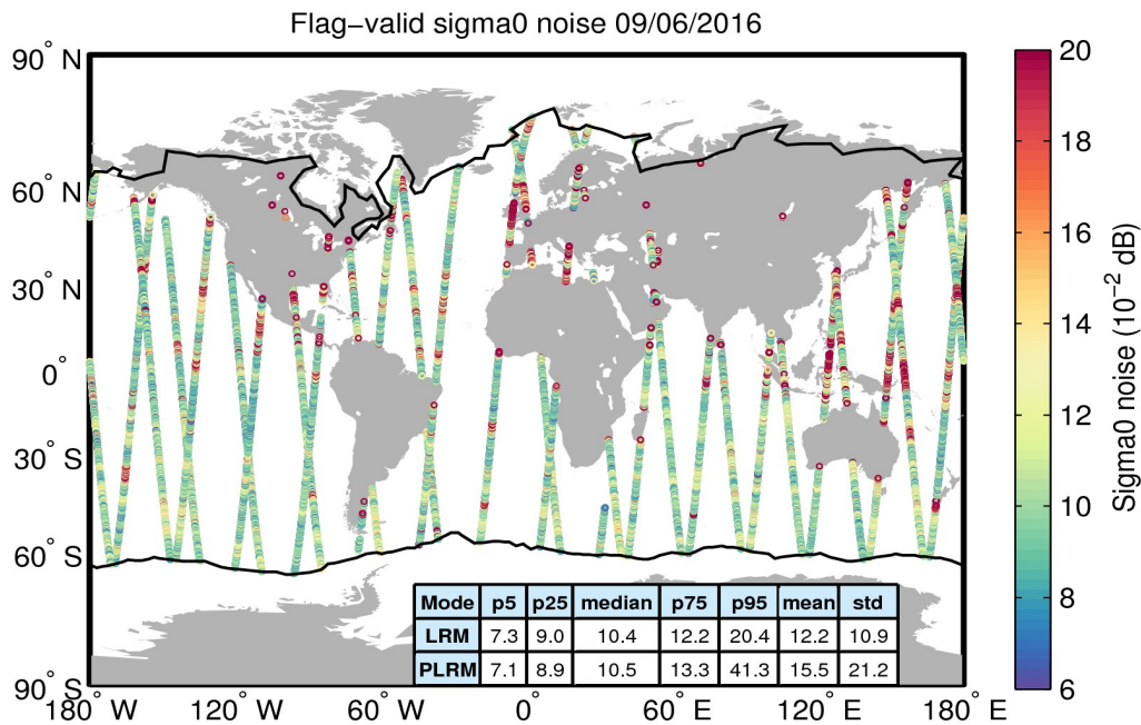
Figure 26. Geographical distribution of flag-valid 20-Hz sigma0 measurement noise over oceans and lakes for 09/06/2016. The statistical values shown in the table refer to the sigma0 noise and are calculated separately for LRM and PLRM regions. Measurements taken over polar polygons have been excluded from the computation of the statistical values. The black lines mark the outer limit of the Arctic and Antarctic polar polygons.
