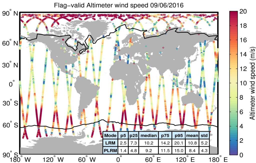
Figure 31. Geographical distribution of flag-valid wind data over oceans and lakes for 09/06/2016. The statistical values shown in the table refer to the wind in m/s and are calculated separately for LRM and PLRM regions. Measurements taken over polar polygons have been excluded from the computation of the statistical values. The black lines mark the outer limit of the Arctic and Antarctic polar polygons.
