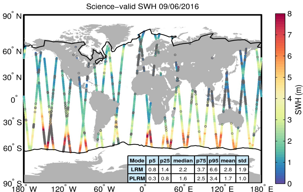
Figure 19. Geographical distribution of science-valid SWH data over oceans and lakes for 09/06/2016. The statistical values shown in the table refer to the SWH in m and are calculated separately for LRM and PLRM regions. The black lines mark the outer limit of the Arctic and Antarctic polar polygons. Gray circles denote records that have been rejected based on the editing criteria described in Table 3.
