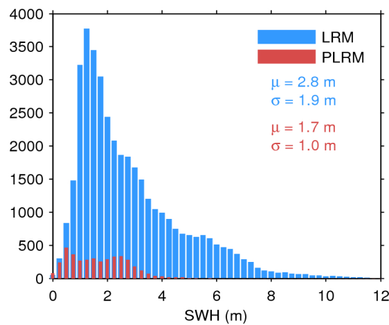
Figure 20. Histogram of science-valid SWH over oceans and lakes for LRM (blue) and PLRM (red) for 09/06/2016. The mean ( \mu ) and standard deviation ( \sigma ) are also shown. Note that values larger than 12 m are excluded from the histogram for the sake of readability but not from the computation of \mu and \sigma .
