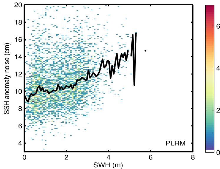
Figure 9. 2D histogram showing flag-valid SSH anomaly noise as a function of SWH for LRM (top) and PLRM (bottom) for 09/06/2016. The black line denotes the median SSH anomaly noise as a function of SWH.
