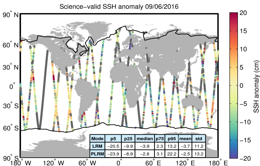
Figure 10. Geographical distribution of science-valid SSH anomaly data over oceans and lakes for 09/06/2016. The statistical values shown in the table refer to the SSH anomaly in cm and are calculated separately for LRM and PLRM regions. The black lines mark the outer limit of the Arctic and Antarctic polar polygons. Gray circles denote records that have been rejected based on the editing criteria described in Table 2.
