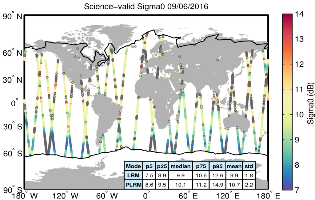
Figure 27. Geographical distribution of science-valid sigma0 data over oceans and lakes for 09/06/2016. The statistical values shown in the table refer to the sigma0 in dB and are calculated separately for LRM and PLRM regions. The black lines mark the outer limit of the Arctic and Antarctic polar polygons. Gray circles denote records that have been rejected based on the editing criteria described in Table 4.
