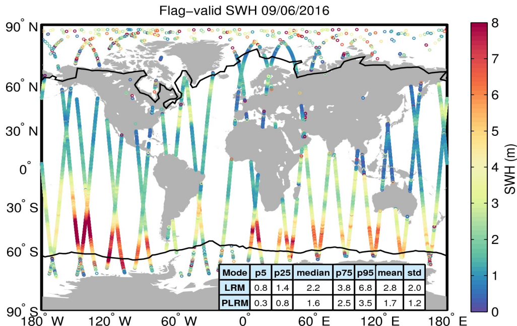
Figure 15. Geographical distribution of flag-valid SWH data over oceans and lakes for 09/06/2016. The statistical values shown in the table refer to the SWH in m and are calculated separately for LRM and PLRM regions. Measurements taken over polar polygons have been excluded from the computation of the statistical values. The black lines mark the outer limit of the Arctic and Antarctic polar polygons.
