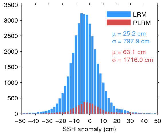
Figure 7. Histogram of flag-valid SSH anomaly over oceans and lakes for LRM (blue) and PLRM (red) for 09/06/2016. The mean ( \mu ) and standard deviation ( \sigma ) are also shown. Note that values outside [-50 50] cm are excluded from the histogram for the sake of readability but not from the computation of \mu and \sigma .
