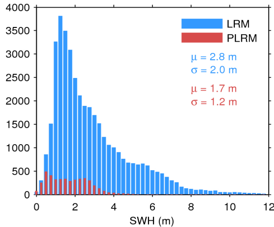
Figure 17. Histogram of flag-valid SWH over oceans and lakes for LRM (blue) and PLRM (red) for 09/06/2016. The mean ( \mu ) and standard deviation ( \sigma ) are also shown. Note that values larger than 12 m are excluded from the histogram for the sake of readability but not from the computation of \mu and \sigma .
