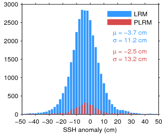
Figure 11. Histogram of science-valid SSH anomaly over oceans and lakes for LRM (blue) and PLRM (red) for 09/06/2016. The mean ( \mu ) and standard deviation ( \sigma ) are also shown. Note that values outside [-50\ 50] cm are excluded from the histogram for the sake of readability but not from the computation of \mu and \sigma .
