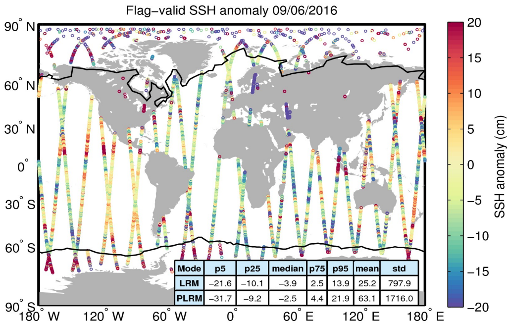
Figure 5. Geographical distribution of flag-valid 1-Hz SSH anomaly data over oceans and lakes for 09/06/2016. The statistical values shown in the table refer to the SSH anomaly in cm and are calculated separately for LRM and PLRM regions. Measurements taken over polar polygons have been excluded from the computation of the statistical values. The black lines mark the outer limit of the Arctic and Antarctic polar polygons.
