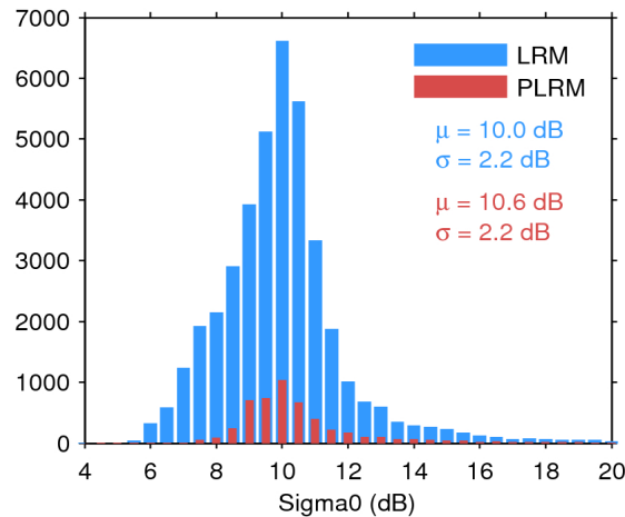
Figure 25. Histogram of flag-valid sigma0 over oceans and lakes for LRM (blue) and PLRM (red) for 08/06/2016. The mean ( \mu ) and standard deviation ( \sigma ) are also shown. Note that values outside [4 20] dB are excluded from the histogram for the sake of readability but not from the computation of \mu and \sigma .
