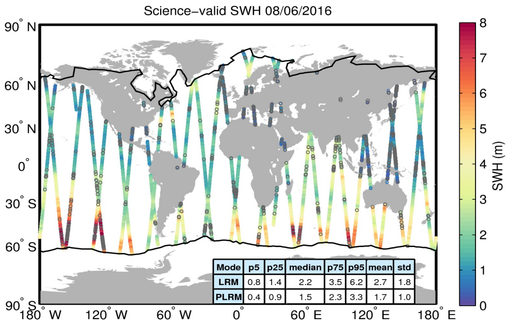
Figure 19. Geographical distribution of science-valid SWH data over oceans and lakes for 08/06/2016. The statistical values shown in the table refer to the SWH in m and are calculated separately for LRM and PLRM regions. The black lines mark the outer limit of the Arctic and Antarctic polar polygons. Gray circles denote records that have been rejected based on the editing criteria described in Table 3.
