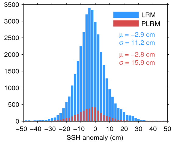
Figure 11. Histogram of science-valid SSH anomaly over oceans and lakes for LRM (blue) and PLRM (red) for 08/06/2016. The mean ( \mu ) and standard deviation ( \sigma ) are also shown. Note that values outside [-50\ 50] cm are excluded from the histogram for the sake of readability but not from the computation of \mu and \sigma .
