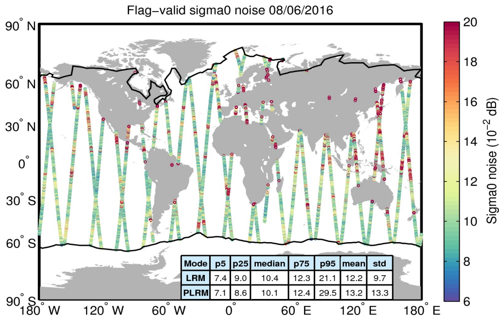
Figure 26. Geographical distribution of flag-valid 20-Hz sigma0 measurement noise over oceans and lakes for 08/06/2016. The statistical values shown in the table refer to the sigma0 noise and are calculated separately for LRM and PLRM regions. Measurements taken over polar polygons have been excluded from the computation of the statistical values. The black lines mark the outer limit of the Arctic and Antarctic polar polygons.
