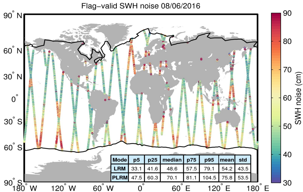
Figure 18. Geographical distribution of flag-valid 20-Hz SWH measurement noise over oceans and lakes for 08/06/2016. The statistical values shown in the table refer to the SWH noise and are calculated separately for LRM and PLRM regions. Measurements taken over polar polygons have been excluded from the computation of the statistical values. The black lines mark the outer limit of the Arctic and Antarctic polar polygons.
