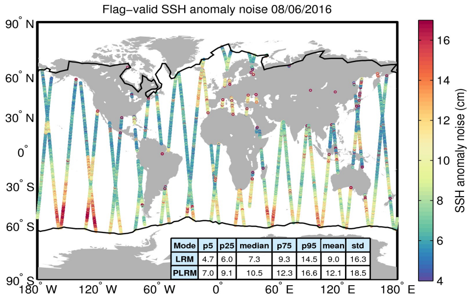
Figure 8. Geographical distribution of flag-valid 20-Hz SSH anomaly measurement noise over oceans and lakes for 08/06/2016. The statistical values shown in the table refer to the SSH anomaly noise and are calculated separately for LRM and PLRM regions. Measurements taken over polar polygons have been excluded from the computation of the statistical values. The black lines mark the outer limit of the Arctic and Antarctic polar polygons.
