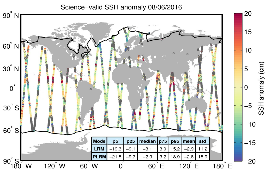
Figure 10. Geographical distribution of science-valid SSH anomaly data over oceans and lakes for 08/06/2016. The statistical values shown in the table refer to the SSH anomaly in cm and are calculated separately for LRM and PLRM regions. The black lines mark the outer limit of the Arctic and Antarctic polar polygons. Gray circles denote records that have been rejected based on the editing criteria described in Table 2.
