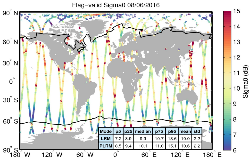
Figure 23. Geographical distribution of flag-valid sigma0 data over oceans and lakes for 08/06/2016. The statistical values shown in the table refer to the sigma0 in dB and are calculated separately for LRM and PLRM regions. Measurements taken over polar polygons have been excluded from the computation of the statistical values. The black lines mark the outer limit of the Arctic and Antarctic polar polygons.
