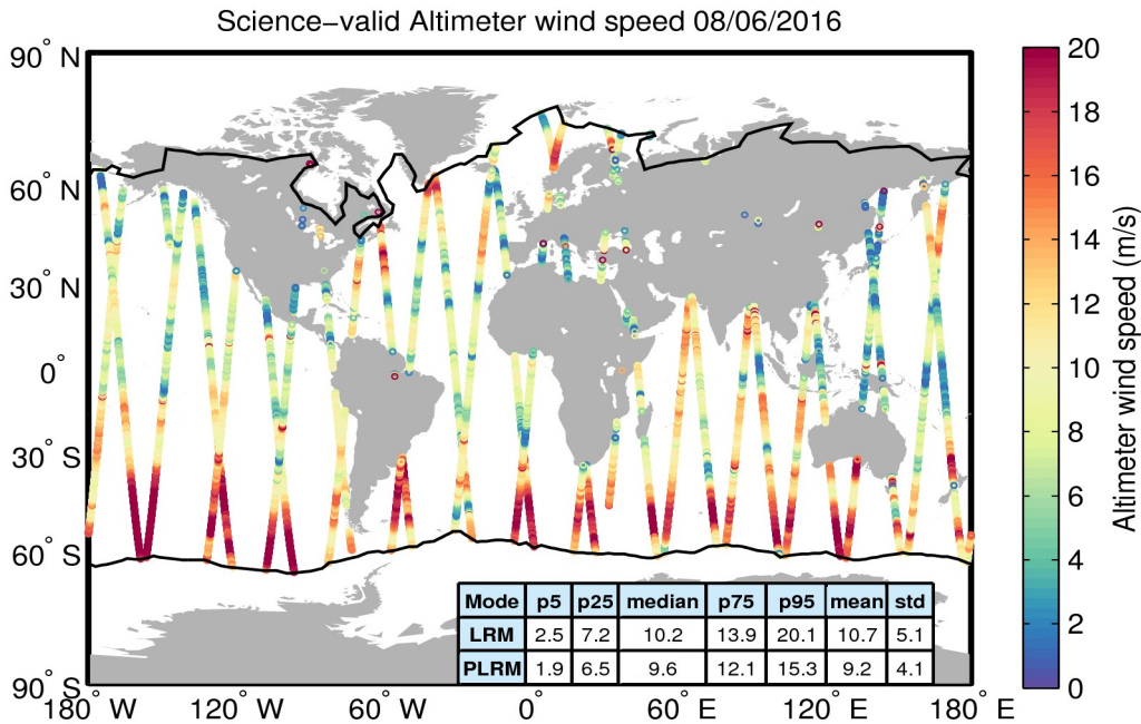
Figure 34. Geographical distribution of science-valid wind data over oceans and lakes for 08/06/2016. The statistical values shown in the table refer to the wind in m/s and are calculated separately for LRM and PLRM regions. The black lines mark the outer limit of the Arctic and Antarctic polar polygons. Gray circles denote records that have been rejected based on the editing criteria described in Table 5.
