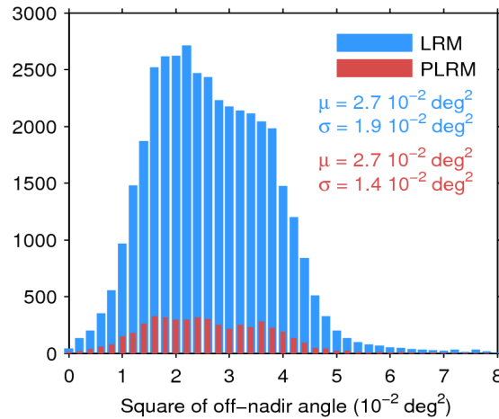
Figure 39. Histogram of flag-valid mispointing over oceans and lakes for LRM (blue) and PLRM (red) for 08/06/2016. Only positive values have been considered. The mean ( \mu ) and standard deviation ( \sigma ) are also shown. Note that values larger than 8 \cdot 10^{-2} \text{ deg}^2 are excluded from the histogram for the sake of readability but not from the computation of \mu and \sigma .
