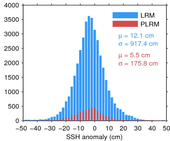
Figure 7. Histogram of flag-valid SSH anomaly over oceans and lakes for LRM (blue) and PLRM (red) for 08/06/2016. The mean ( \mu ) and standard deviation ( \sigma ) are also shown. Note that values outside [-50\ 50] cm are excluded from the histogram for the sake of readability but not from the computation of \mu and \sigma .
