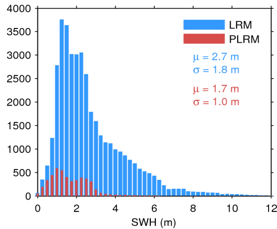
Figure 20. Histogram of science-valid SWH over oceans and lakes for LRM (blue) and PLRM (red) for 08/06/2016. The mean ( \mu ) and standard deviation ( \sigma ) are also shown. Note that values larger than 12 m are excluded from the histogram for the sake of readability but not from the computation of \mu and \sigma .
