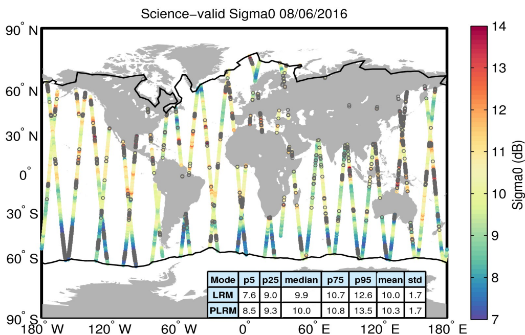
Figure 27. Geographical distribution of science-valid sigma0 data over oceans and lakes for 08/06/2016. The statistical values shown in the table refer to the sigma0 in dB and are calculated separately for LRM and PLRM regions. The black lines mark the outer limit of the Arctic and Antarctic polar polygons. Gray circles denote records that have been rejected based on the editing criteria described in Table 4.
