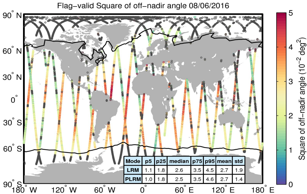
Figure 37. Geographical distribution of flag-valid mispointing data over oceans and lakes for 08/06/2016. The statistical values shown in the table refer to the mispointing in 10^{-2} \text{ deg}^2 and are calculated separately for LRM and PLRM regions. Measurements taken over polar polygons have been excluded from the computation of the statistical values. The black lines mark the outer limit of the Arctic and Antarctic polar polygons. Gray circles denote negative values.
