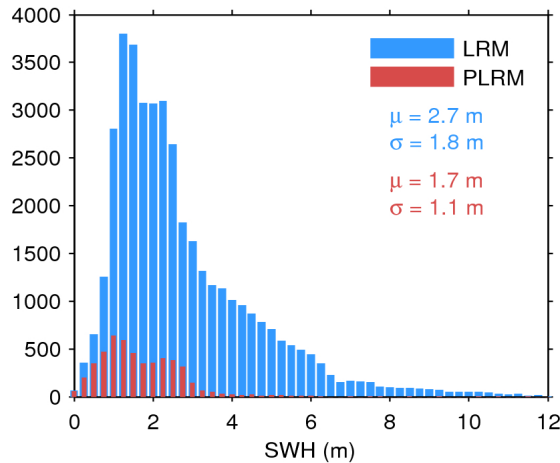
Figure 17. Histogram of flag-valid SWH over oceans and lakes for LRM (blue) and PLRM (red) for 08/06/2016. The mean ( \mu ) and standard deviation ( \sigma ) are also shown. Note that values larger than 12 m are excluded from the histogram for the sake of readability but not from the computation of \mu and \sigma .
