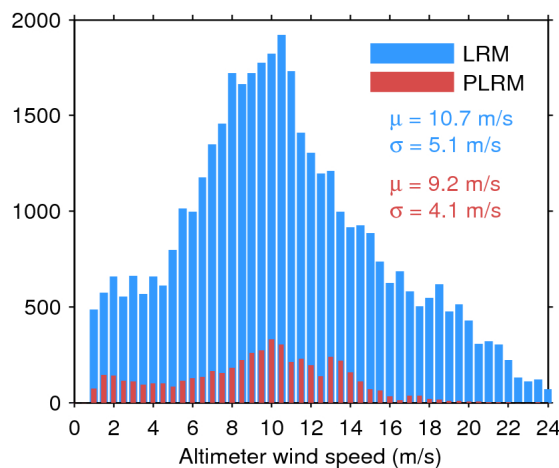
Figure 35. Histogram of science-valid wind over oceans and lakes for LRM (blue) and PLRM (red) for 08/06/2016. The mean ( \mu ) and standard deviation ( \sigma ) are also shown. Note that values larger than 24 m/s are excluded from the histogram for the sake of readability but not from the computation of \mu and \sigma .
