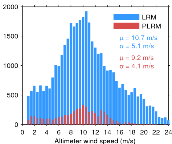
Figure 33. Histogram of flag-valid wind over oceans and lakes for LRM (blue) and PLRM (red) for 08/06/2016. The mean ( \mu ) and standard deviation ( \sigma ) are also shown. Note that values larger than 24 m/s are excluded from the histogram for the sake of readability but not from the computation of \mu and \sigma .
