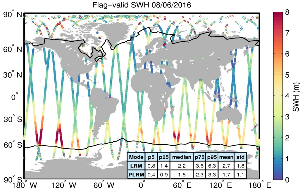
Figure 15. Geographical distribution of flag-valid SWH data over oceans and lakes for 08/06/2016. The statistical values shown in the table refer to the SWH in m and are calculated separately for LRM and PLRM regions. Measurements taken over polar polygons have been excluded from the computation of the statistical values. The black lines mark the outer limit of the Arctic and Antarctic polar polygons.
