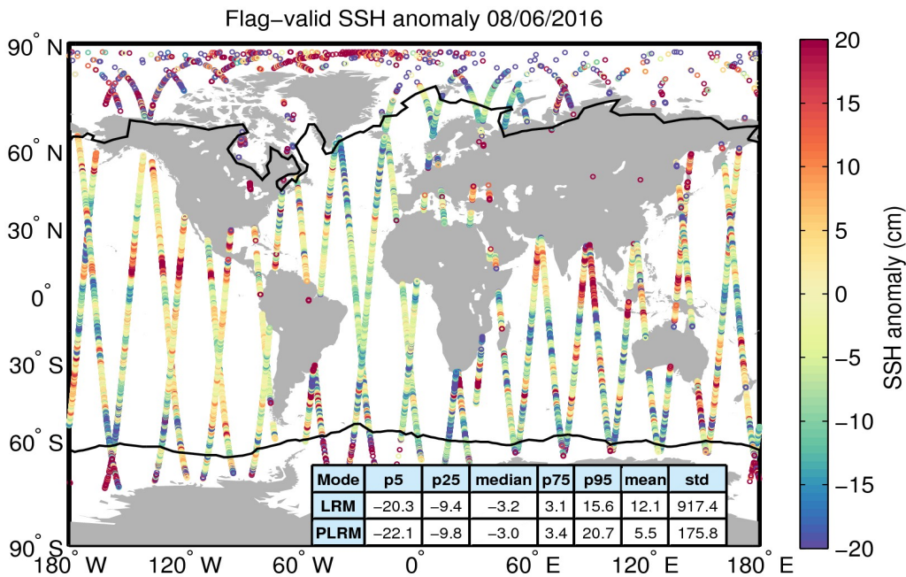
Figure 5. Geographical distribution of flag-valid 1-Hz SSH anomaly data over oceans and lakes for 08/06/2016. The statistical values shown in the table refer to the SSH anomaly in cm and are calculated separately for LRM and PLRM regions. Measurements taken over polar polygons have been excluded from the computation of the statistical values. The black lines mark the outer limit of the Arctic and Antarctic polar polygons.
