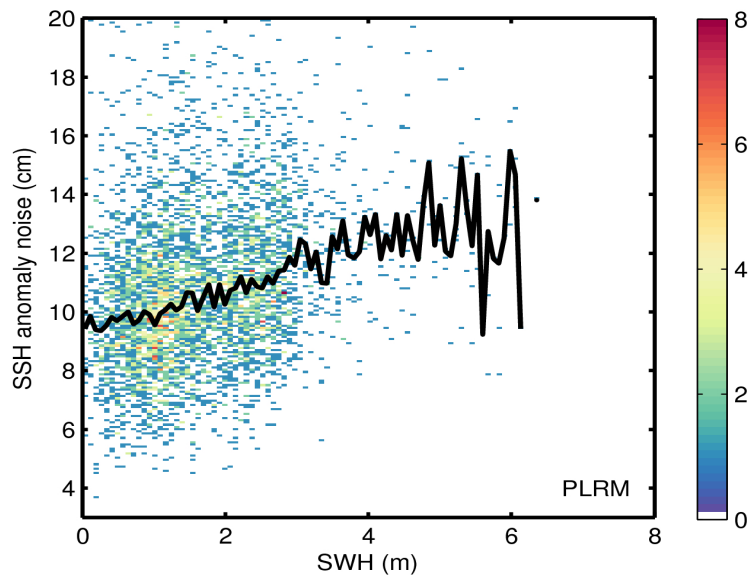
Figure 9. 2D histogram showing flag-valid SSH anomaly noise as a function of SWH for LRM (top) and PLRM (bottom) for 08/06/2016. The black line denotes the median SSH anomaly noise as a function of SWH.
