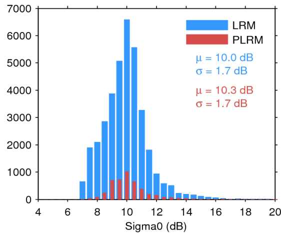
Figure 28. Histogram of science-valid sigma0 over oceans and lakes for LRM (blue) and PLRM (red) for 08/06/2016. The mean ( \mu ) and standard deviation ( \sigma ) are also shown. Note that values outside [4 20] dB are excluded from the histogram for the sake of readability but not from the computation of \mu and \sigma .
