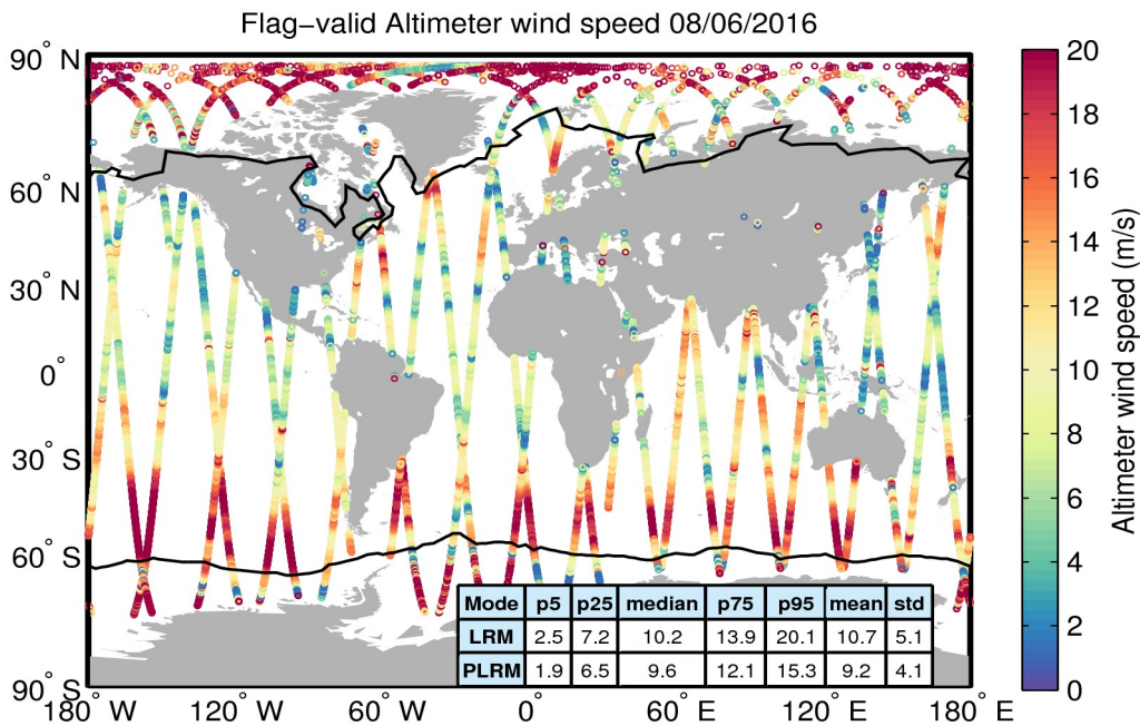
Figure 31. Geographical distribution of flag-valid wind data over oceans and lakes for 08/06/2016. The statistical values shown in the table refer to the wind in m/s and are calculated separately for LRM and PLRM regions. Measurements taken over polar polygons have been excluded from the computation of the statistical values. The black lines mark the outer limit of the Arctic and Antarctic polar polygons.
