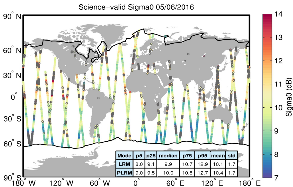
Figure 27. Geographical distribution of science-valid sigma0 data over oceans and lakes for 05/06/2016. The statistical values shown in the table refer to the sigma0 in dB and are calculated separately for LRM and PLRM regions. The black lines mark the outer limit of the Arctic and Antarctic polar polygons. Gray circles denote records that have been rejected based on the editing criteria described in Table 4.
