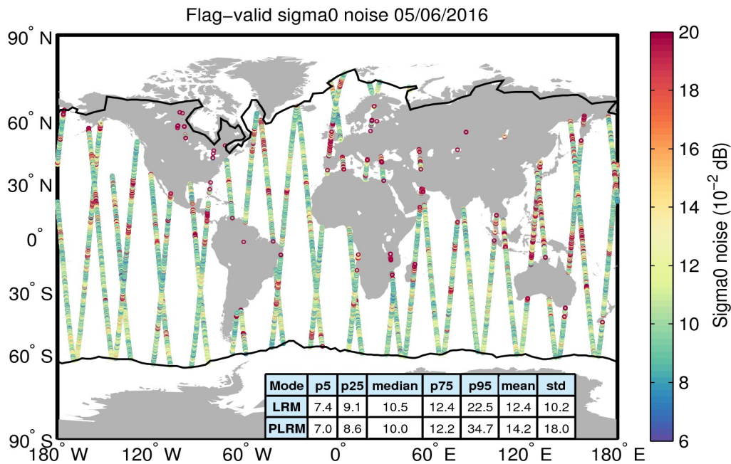
Figure 26. Geographical distribution of flag-valid 20-Hz sigma0 measurement noise over oceans and lakes for 05/06/2016. The statistical values shown in the table refer to the sigma0 noise and are calculated separately for LRM and PLRM regions. Measurements taken over polar polygons have been excluded from the computation of the statistical values. The black lines mark the outer limit of the Arctic and Antarctic polar polygons.
