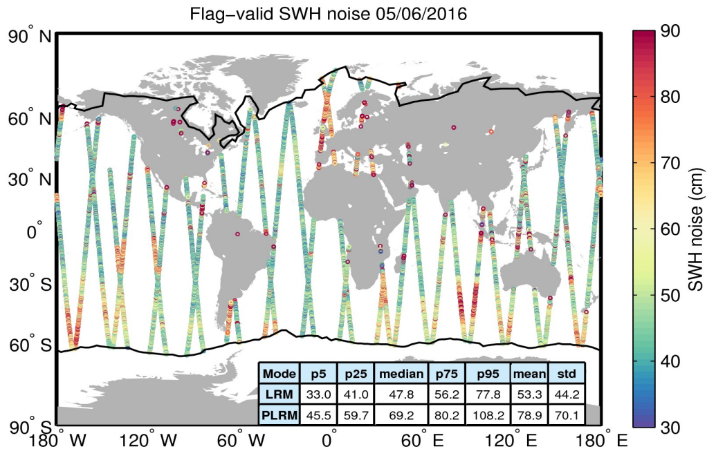
Figure 18. Geographical distribution of flag-valid 20-Hz SWH measurement noise over oceans and lakes for 05/06/2016. The statistical values shown in the table refer to the SWH noise and are calculated separately for LRM and PLRM regions. Measurements taken over polar polygons have been excluded from the computation of the statistical values. The black lines mark the outer limit of the Arctic and Antarctic polar polygons.
