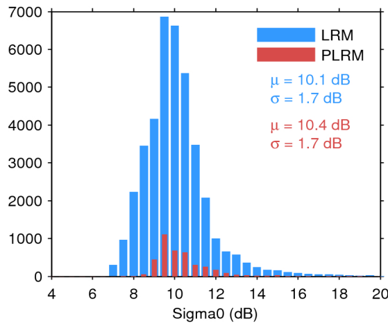
Figure 28. Histogram of science-valid sigma0 over oceans and lakes for LRM (blue) and PLRM (red) for 05/06/2016. The mean ( \mu ) and standard deviation ( \sigma ) are also shown. Note that values outside [4 20] dB are excluded from the histogram for the sake of readability but not from the computation of \mu and \sigma .
