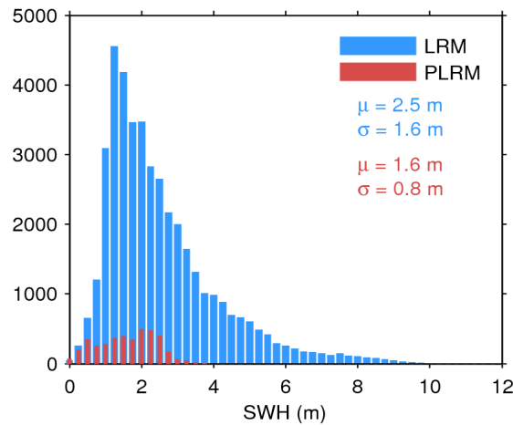
Figure 20. Histogram of science-valid SWH over oceans and lakes for LRM (blue) and PLRM (red) for 05/06/2016. The mean ( \mu ) and standard deviation ( \sigma ) are also shown. Note that values larger than 12 m are excluded from the histogram for the sake of readability but not from the computation of \mu and \sigma .
