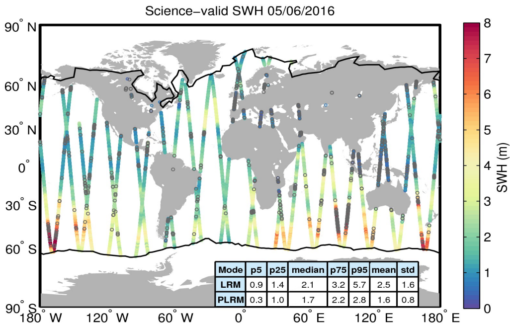
Figure 19. Geographical distribution of science-valid SWH data over oceans and lakes for 05/06/2016. The statistical values shown in the table refer to the SWH in m and are calculated separately for LRM and PLRM regions. The black lines mark the outer limit of the Arctic and Antarctic polar polygons. Gray circles denote records that have been rejected based on the editing criteria described in Table 3.
