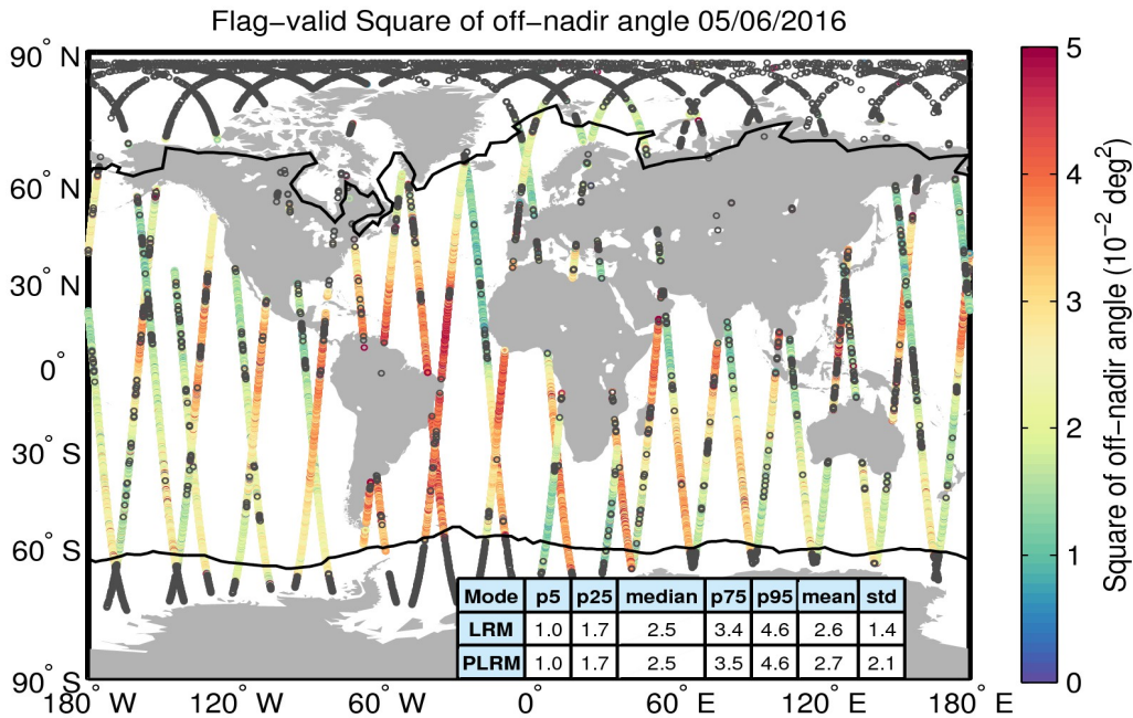
Figure 37. Geographical distribution of flag-valid mispointing data over oceans and lakes for 05/06/2016. The statistical values shown in the table refer to the mispointing in 10^{-2} deg 2 and are calculated separately for LRM and PLRM regions. Measurements taken over polar polygons have been excluded from the computation of the statistical values. The black lines mark the outer limit of the Arctic and Antarctic polar polygons. Gray circles denote negative values.
