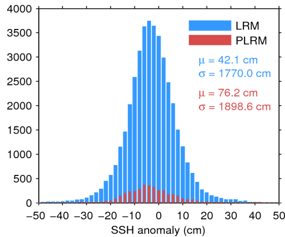
Figure 7. Histogram of flag-valid SSH anomaly over oceans and lakes for LRM (blue) and PLRM (red) for 05/06/2016. The mean ( \mu ) and standard deviation ( \sigma ) are also shown. Note that values outside [-50\ 50] cm are excluded from the histogram for the sake of readability but not from the computation of \mu and \sigma .
