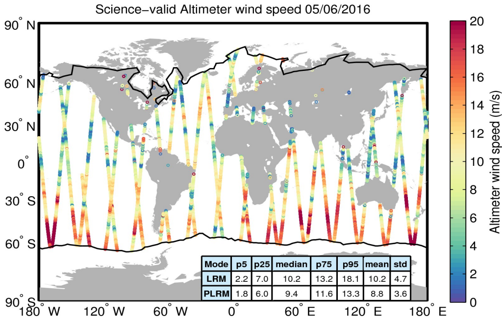
Figure 34. Geographical distribution of science-valid wind data over oceans and lakes for 05/06/2016. The statistical values shown in the table refer to the wind in m/s and are calculated separately for LRM and PLRM regions. The black lines mark the outer limit of the Arctic and Antarctic polar polygons. Gray circles denote records that have been rejected based on the editing criteria described in Table 5.
