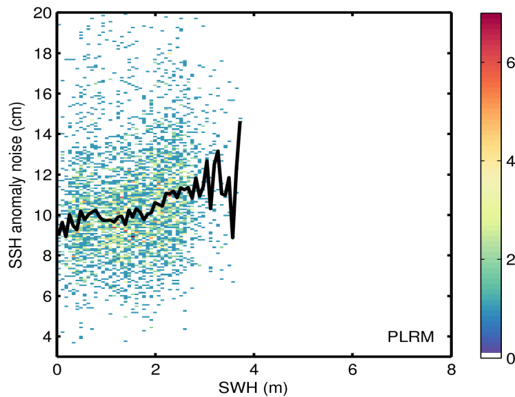
Figure 9. 2D histogram showing flag-valid SSH anomaly noise as a function of SWH for LRM (top) and PLRM (bottom) for 05/06/2016. The black line denotes the median SSH anomaly noise as a function of SWH.
