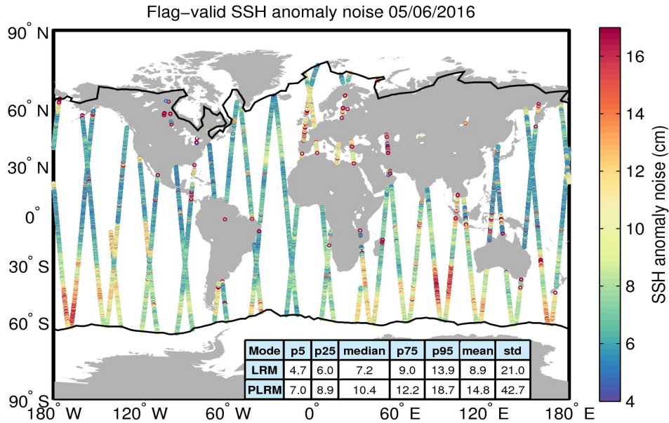
Figure 8. Geographical distribution of flag-valid 20-Hz SSH anomaly measurement noise over oceans and lakes for 05/06/2016. The statistical values shown in the table refer to the SSH anomaly noise and are calculated separately for LRM and PLRM regions. Measurements taken over polar polygons have been excluded from the computation of the statistical values. The black lines mark the outer limit of the Arctic and Antarctic polar polygons.
