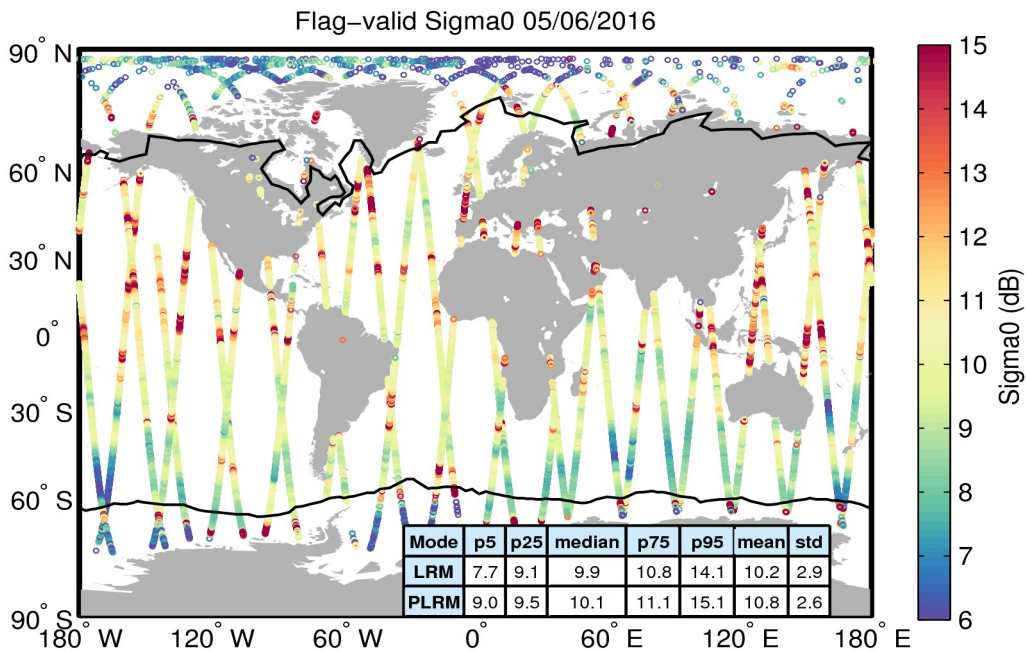
Figure 23. Geographical distribution of flag-valid sigma0 data over oceans and lakes for 05/06/2016. The statistical values shown in the table refer to the sigma0 in dB and are calculated separately for LRM and PLRM regions. Measurements taken over polar polygons have been excluded from the computation of the statistical values. The black lines mark the outer limit of the Arctic and Antarctic polar polygons.
