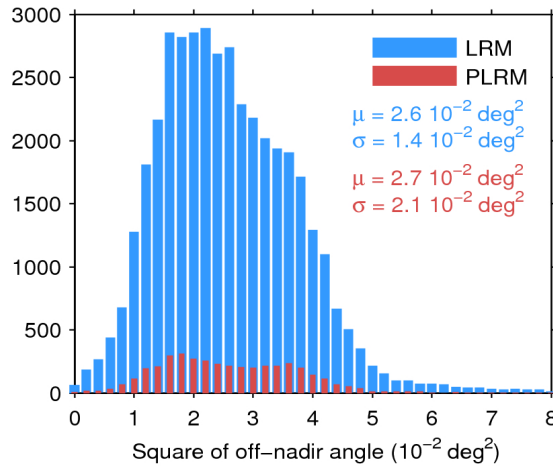
Figure 39. Histogram of flag-valid mispointing over oceans and lakes for LRM (blue) and PLRM (red) for 05/06/2016. Only positive values have been considered. The mean ( \mu ) and standard deviation ( \sigma ) are also shown. Note that values larger than 8 \cdot 10^{-2} \text{ deg}^2 are excluded from the histogram for the sake of readability but not from the computation of \mu and \sigma .
