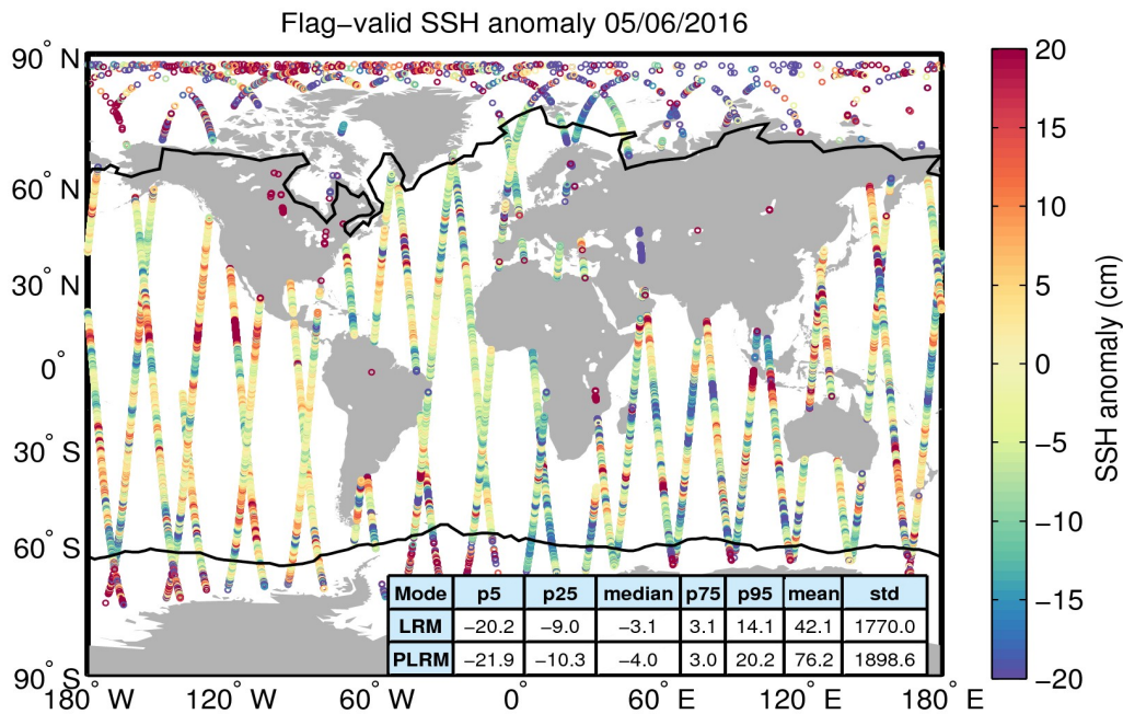
Figure 5. Geographical distribution of flag-valid 1-Hz SSH anomaly data over oceans and lakes for 05/06/2016. The statistical values shown in the table refer to the SSH anomaly in cm and are calculated separately for LRM and PLRM regions. Measurements taken over polar polygons have been excluded from the computation of the statistical values. The black lines mark the outer limit of the Arctic and Antarctic polar polygons.
