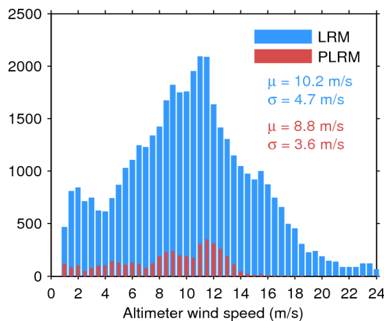
Figure 35. Histogram of science-valid wind over oceans and lakes for LRM (blue) and PLRM (red) for 05/06/2016. The mean ( \mu ) and standard deviation ( \sigma ) are also shown. Note that values larger than 24 m/s are excluded from the histogram for the sake of readability but not from the computation of \mu and \sigma .
