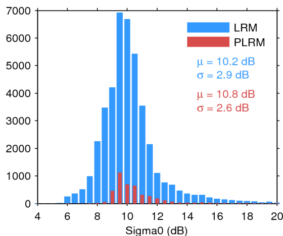
Figure 25. Histogram of flag-valid sigma0 over oceans and lakes for LRM (blue) and PLRM (red) for 05/06/2016. The mean ( \mu ) and standard deviation ( \sigma ) are also shown. Note that values outside [4 20] dB are excluded from the histogram for the sake of readability but not from the computation of \mu and \sigma .
