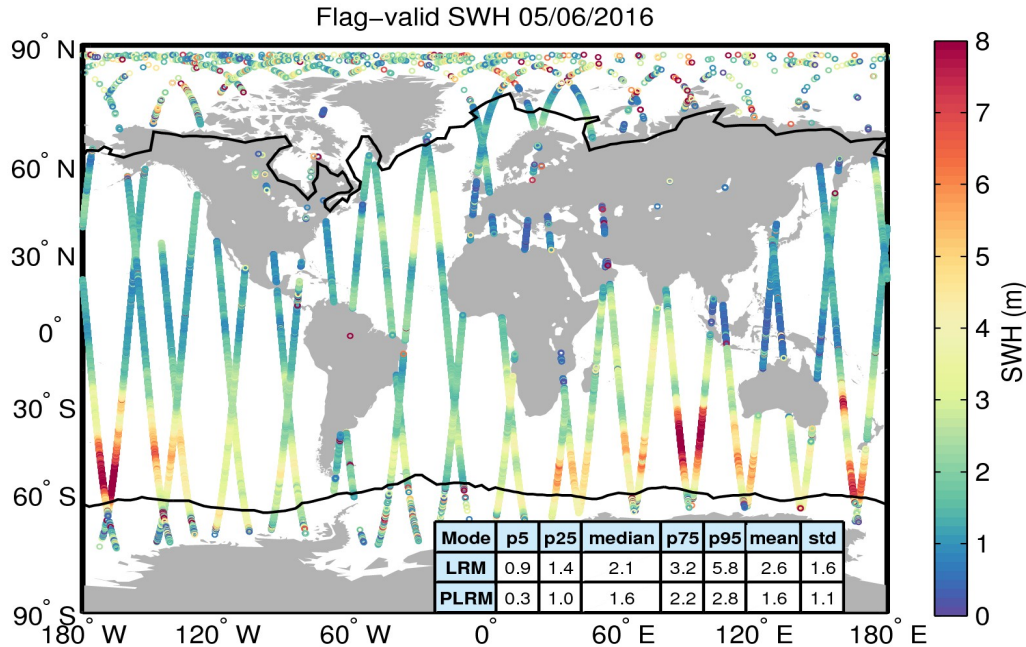
Figure 15. Geographical distribution of flag-valid SWH data over oceans and lakes for 05/06/2016. The statistical values shown in the table refer to the SWH in m and are calculated separately for LRM and PLRM regions. Measurements taken over polar polygons have been excluded from the computation of the statistical values. The black lines mark the outer limit of the Arctic and Antarctic polar polygons.
