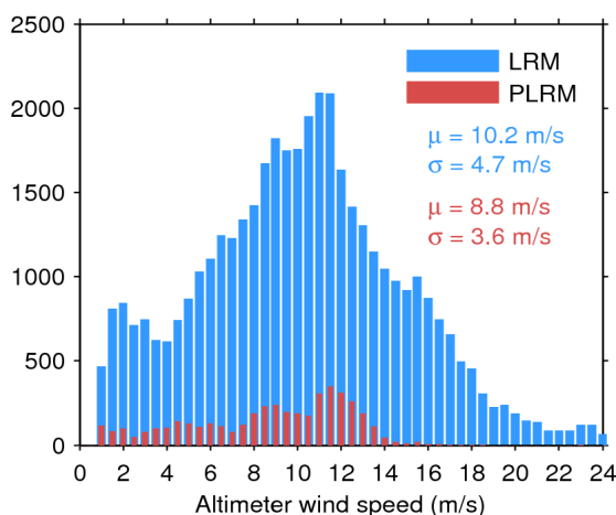
Figure 33. Histogram of flag-valid wind over oceans and lakes for LRM (blue) and PLRM (red) for 05/06/2016. The mean ( \mu ) and standard deviation ( \sigma ) are also shown. Note that values larger than 24 m/s are excluded from the histogram for the sake of readability but not from the computation of \mu and \sigma .
