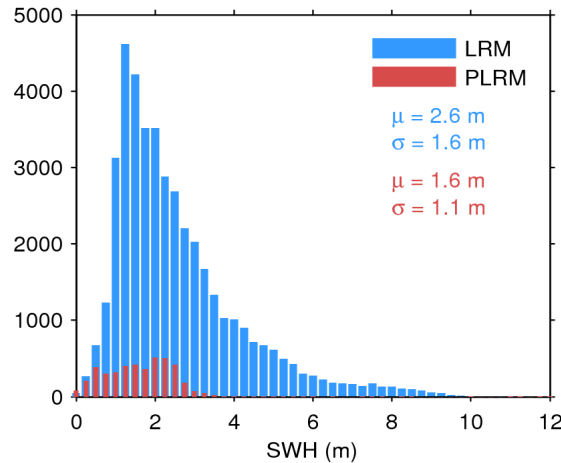
Figure 17. Histogram of flag-valid SWH over oceans and lakes for LRM (blue) and PLRM (red) for 05/06/2016. The mean ( \mu ) and standard deviation ( \sigma ) are also shown. Note that values larger than 12 m are excluded from the histogram for the sake of readability but not from the computation of \mu and \sigma .
