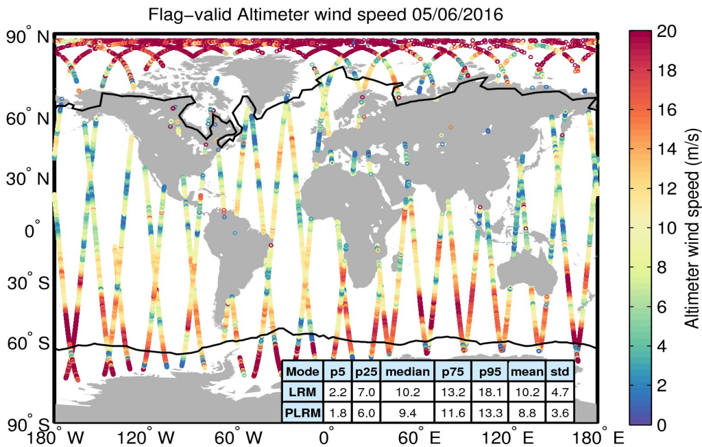
Figure 31. Geographical distribution of flag-valid wind data over oceans and lakes for 05/06/2016. The statistical values shown in the table refer to the wind in m/s and are calculated separately for LRM and PLRM regions. Measurements taken over polar polygons have been excluded from the computation of the statistical values. The black lines mark the outer limit of the Arctic and Antarctic polar polygons.
