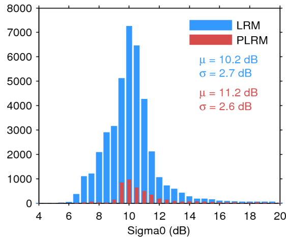
Figure 25. Histogram of flag-valid sigma0 over oceans and lakes for LRM (blue) and PLRM (red) for 04/06/2016. The mean ( \mu ) and standard deviation ( \sigma ) are also shown. Note that values outside [4 20] dB are excluded from the histogram for the sake of readability but not from the computation of \mu and \sigma .
