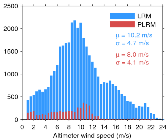
Figure 35. Histogram of science-valid wind over oceans and lakes for LRM (blue) and PLRM (red) for 04/06/2016. The mean ( \mu ) and standard deviation ( \sigma ) are also shown. Note that values larger than 24 m/s are excluded from the histogram for the sake of readability but not from the computation of \mu and \sigma .
