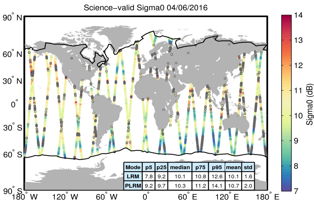
Figure 27. Geographical distribution of science-valid sigma0 data over oceans and lakes for 04/06/2016. The statistical values shown in the table refer to the sigma0 in dB and are calculated separately for LRM and PLRM regions. The black lines mark the outer limit of the Arctic and Antarctic polar polygons. Gray circles denote records that have been rejected based on the editing criteria described in Table 4.
