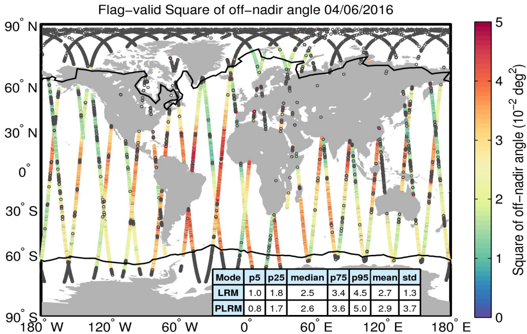
Figure 37. Geographical distribution of flag-valid mispointing data over oceans and lakes for 04/06/2016. The statistical values shown in the table refer to the mispointing in 10^{-2} deg 2 and are calculated separately for LRM and PLRM regions. Measurements taken over polar polygons have been excluded from the computation of the statistical values. The black lines mark the outer limit of the Arctic and Antarctic polar polygons. Gray circles denote negative values.
