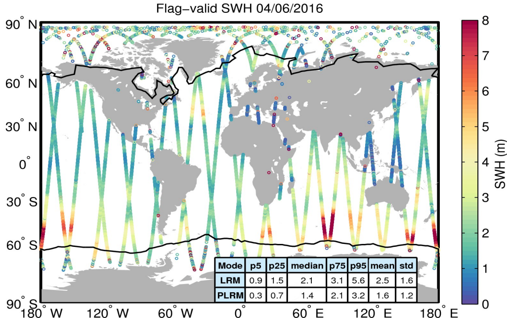
Figure 15. Geographical distribution of flag-valid SWH data over oceans and lakes for 04/06/2016. The statistical values shown in the table refer to the SWH in m and are calculated separately for LRM and PLRM regions. Measurements taken over polar polygons have been excluded from the computation of the statistical values. The black lines mark the outer limit of the Arctic and Antarctic polar polygons.
