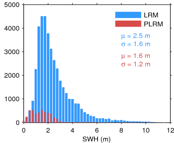
Figure 17. Histogram of flag-valid SWH over oceans and lakes for LRM (blue) and PLRM (red) for 04/06/2016. The mean ( \mu ) and standard deviation ( \sigma ) are also shown. Note that values larger than 12 m are excluded from the histogram for the sake of readability but not from the computation of \mu and \sigma .
