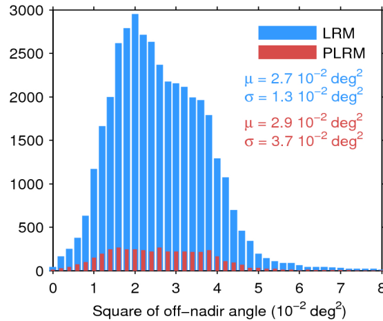
Figure 39. Histogram of flag-valid mispointing over oceans and lakes for LRM (blue) and PLRM (red) for 04/06/2016. Only positive values have been considered. The mean ( \mu ) and standard deviation ( \sigma ) are also shown. Note that values larger than 8 \cdot 10^{-2} \text{ deg}^2 are excluded from the histogram for the sake of readability but not from the computation of \mu and \sigma .
