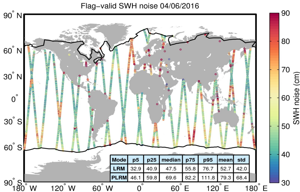
Figure 18. Geographical distribution of flag-valid 20-Hz SWH measurement noise over oceans and lakes for 04/06/2016. The statistical values shown in the table refer to the SWH noise and are calculated separately for LRM and PLRM regions. Measurements taken over polar polygons have been excluded from the computation of the statistical values. The black lines mark the outer limit of the Arctic and Antarctic polar polygons.
