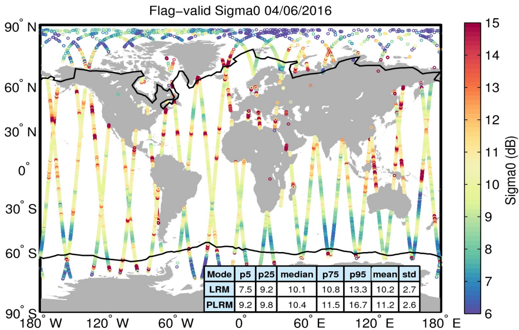
Figure 23. Geographical distribution of flag-valid sigma0 data over oceans and lakes for 04/06/2016. The statistical values shown in the table refer to the sigma0 in dB and are calculated separately for LRM and PLRM regions. Measurements taken over polar polygons have been excluded from the computation of the statistical values. The black lines mark the outer limit of the Arctic and Antarctic polar polygons.
