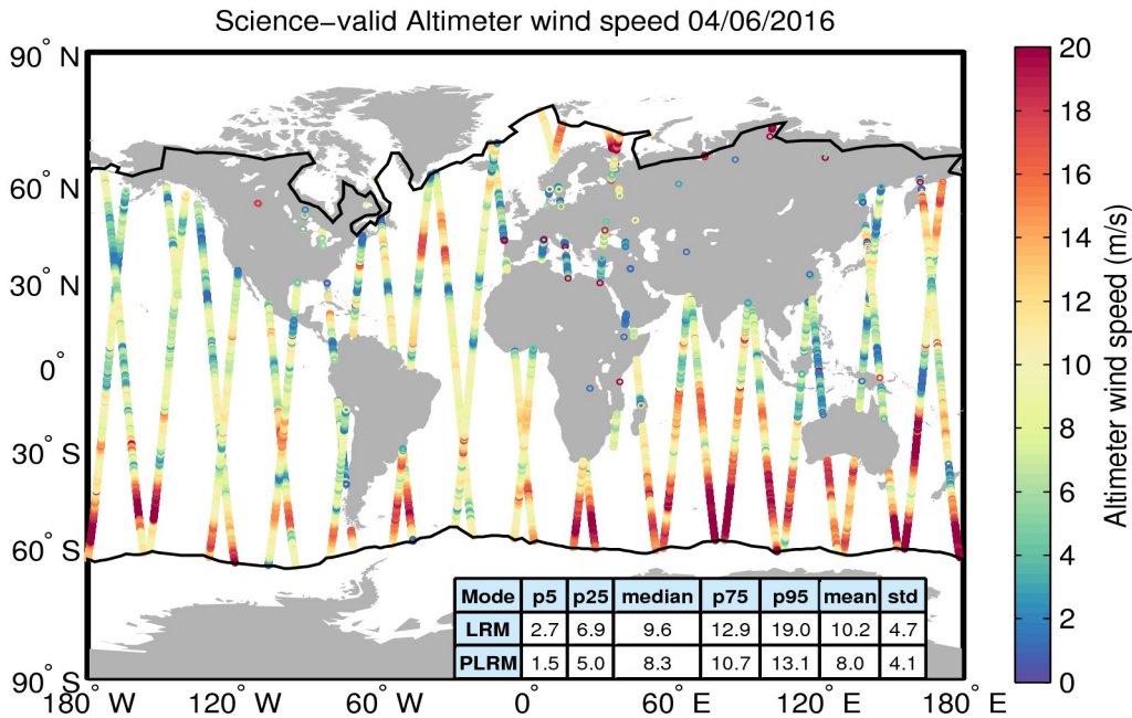
Figure 34. Geographical distribution of science-valid wind data over oceans and lakes for 04/06/2016. The statistical values shown in the table refer to the wind in m/s and are calculated separately for LRM and PLRM regions. The black lines mark the outer limit of the Arctic and Antarctic polar polygons. Gray circles denote records that have been rejected based on the editing criteria described in Table 5.
