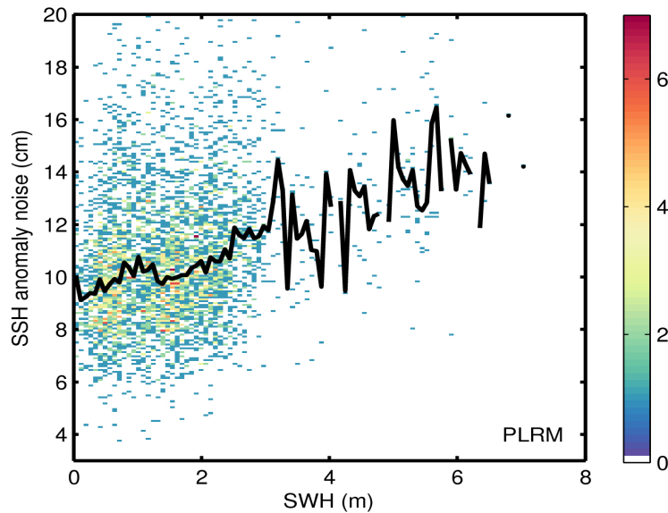
Figure 9. 2D histogram showing flag-valid SSH anomaly noise as a function of SWH for LRM (top) and PLRM (bottom) for 04/06/2016. The black line denotes the median SSH anomaly noise as a function of SWH.
