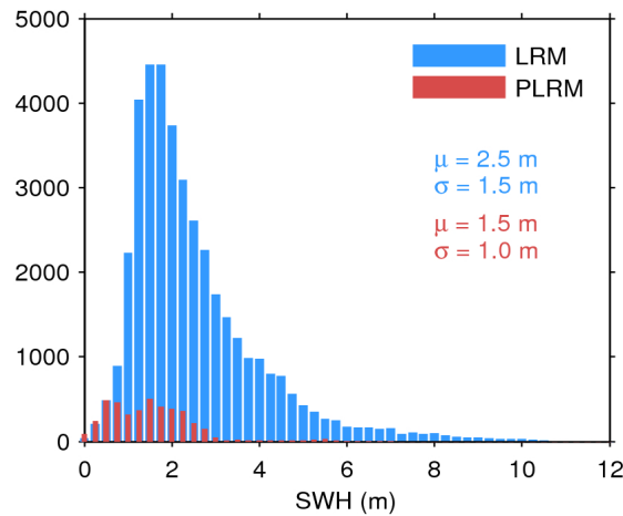
Figure 20. Histogram of science-valid SWH over oceans and lakes for LRM (blue) and PLRM (red) for 04/06/2016. The mean ( \mu ) and standard deviation ( \sigma ) are also shown. Note that values larger than 12 m are excluded from the histogram for the sake of readability but not from the computation of \mu and \sigma .
