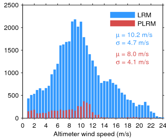
Figure 33. Histogram of flag-valid wind over oceans and lakes for LRM (blue) and PLRM (red) for 04/06/2016. The mean ( \mu ) and standard deviation ( \sigma ) are also shown. Note that values larger than 24 m/s are excluded from the histogram for the sake of readability but not from the computation of \mu and \sigma .
