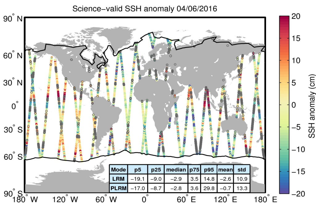
Figure 10. Geographical distribution of science-valid SSH anomaly data over oceans and lakes for 04/06/2016. The statistical values shown in the table refer to the SSH anomaly in cm and are calculated separately for LRM and PLRM regions. The black lines mark the outer limit of the Arctic and Antarctic polar polygons. Gray circles denote records that have been rejected based on the editing criteria described in Table 2.
