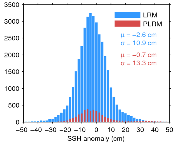
Figure 11. Histogram of science-valid SSH anomaly over oceans and lakes for LRM (blue) and PLRM (red) for 04/06/2016. The mean ( \mu ) and standard deviation ( \sigma ) are also shown. Note that values outside [-50\ 50] cm are excluded from the histogram for the sake of readability but not from the computation of \mu and \sigma .
