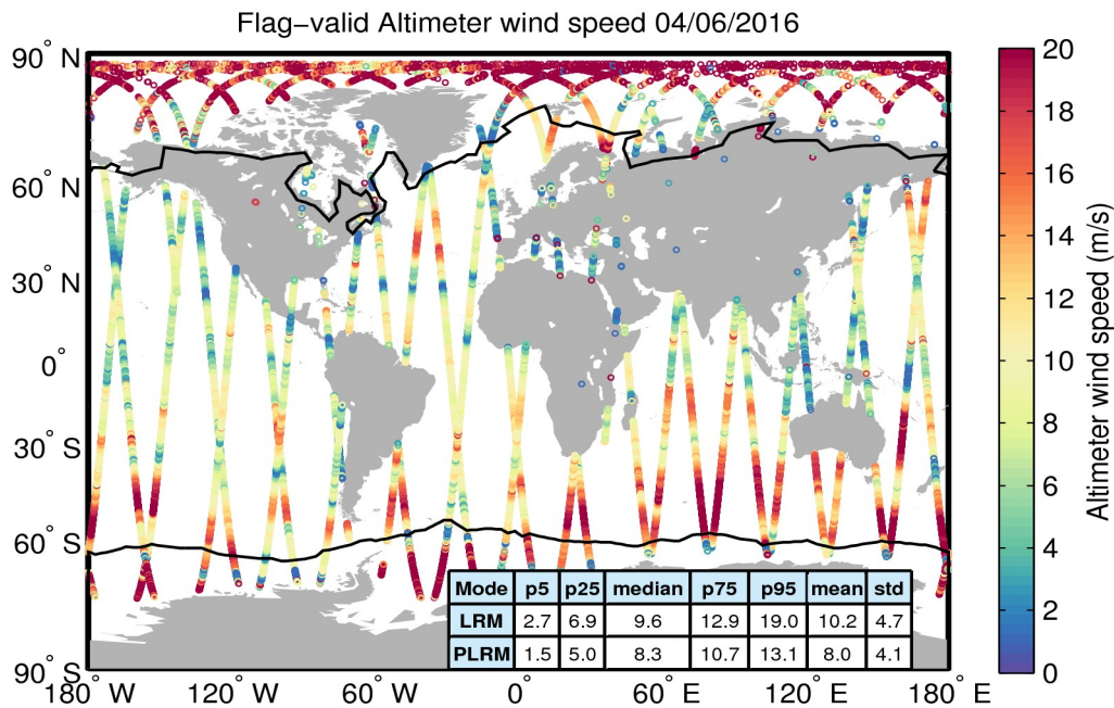
Figure 31. Geographical distribution of flag-valid wind data over oceans and lakes for 04/06/2016. The statistical values shown in the table refer to the wind in m/s and are calculated separately for LRM and PLRM regions. Measurements taken over polar polygons have been excluded from the computation of the statistical values. The black lines mark the outer limit of the Arctic and Antarctic polar polygons.
