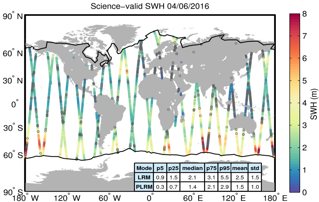
Figure 19. Geographical distribution of science-valid SWH data over oceans and lakes for 04/06/2016. The statistical values shown in the table refer to the SWH in m and are calculated separately for LRM and PLRM regions. The black lines mark the outer limit of the Arctic and Antarctic polar polygons. Gray circles denote records that have been rejected based on the editing criteria described in Table 3.
