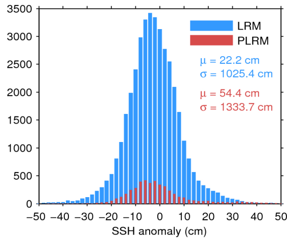
Figure 7. Histogram of flag-valid SSH anomaly over oceans and lakes for LRM (blue) and PLRM (red) for 04/06/2016. The mean ( \mu ) and standard deviation ( \sigma ) are also shown. Note that values outside [-50 50] cm are excluded from the histogram for the sake of readability but not from the computation of \mu and \sigma .
