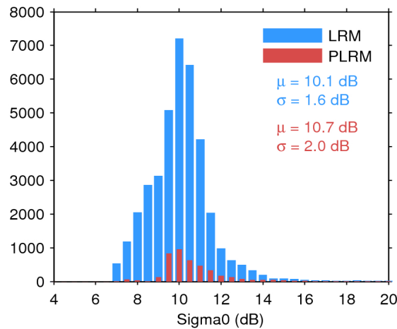
Figure 28. Histogram of science-valid sigma0 over oceans and lakes for LRM (blue) and PLRM (red) for 04/06/2016. The mean ( \mu ) and standard deviation ( \sigma ) are also shown. Note that values outside [4 20] dB are excluded from the histogram for the sake of readability but not from the computation of \mu and \sigma .
