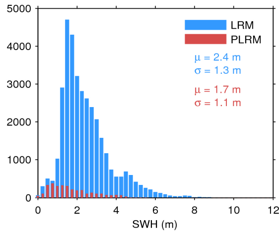
Figure 20. Histogram of science-valid SWH over oceans and lakes for LRM (blue) and PLRM (red) for 02/06/2016. The mean ( \mu ) and standard deviation ( \sigma ) are also shown. Note that values larger than 12 m are excluded from the histogram for the sake of readability but not from the computation of \mu and \sigma .
