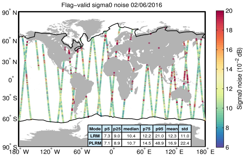
Figure 26. Geographical distribution of flag-valid 20-Hz sigma0 measurement noise over oceans and lakes for 02/06/2016. The statistical values shown in the table refer to the sigma0 noise and are calculated separately for LRM and PLRM regions. Measurements taken over polar polygons have been excluded from the computation of the statistical values. The black lines mark the outer limit of the Arctic and Antarctic polar polygons.
