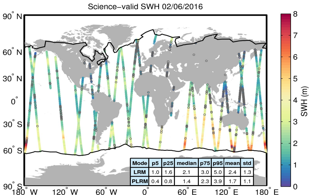
Figure 19. Geographical distribution of science-valid SWH data over oceans and lakes for 02/06/2016. The statistical values shown in the table refer to the SWH in m and are calculated separately for LRM and PLRM regions. The black lines mark the outer limit of the Arctic and Antarctic polar polygons. Gray circles denote records that have been rejected based on the editing criteria described in Table 3.
