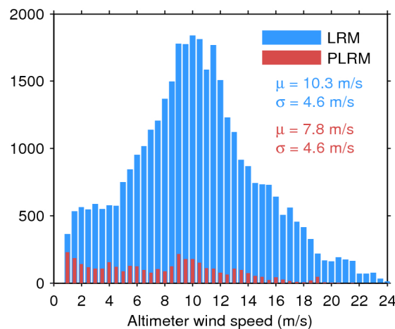
Figure 35. Histogram of science-valid wind over oceans and lakes for LRM (blue) and PLRM (red) for 02/06/2016. The mean ( \mu ) and standard deviation ( \sigma ) are also shown. Note that values larger than 24 m/s are excluded from the histogram for the sake of readability but not from the computation of \mu and \sigma .
