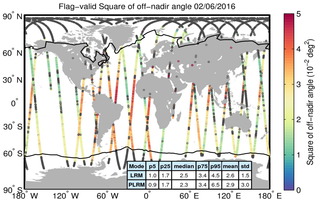
Figure 37. Geographical distribution of flag-valid mispointing data over oceans and lakes for 02/06/2016. The statistical values shown in the table refer to the mispointing in 10^{-2} deg 2 and are calculated separately for LRM and PLRM regions. Measurements taken over polar polygons have been excluded from the computation of the statistical values. The black lines mark the outer limit of the Arctic and Antarctic polar polygons. Gray circles denote negative values.
