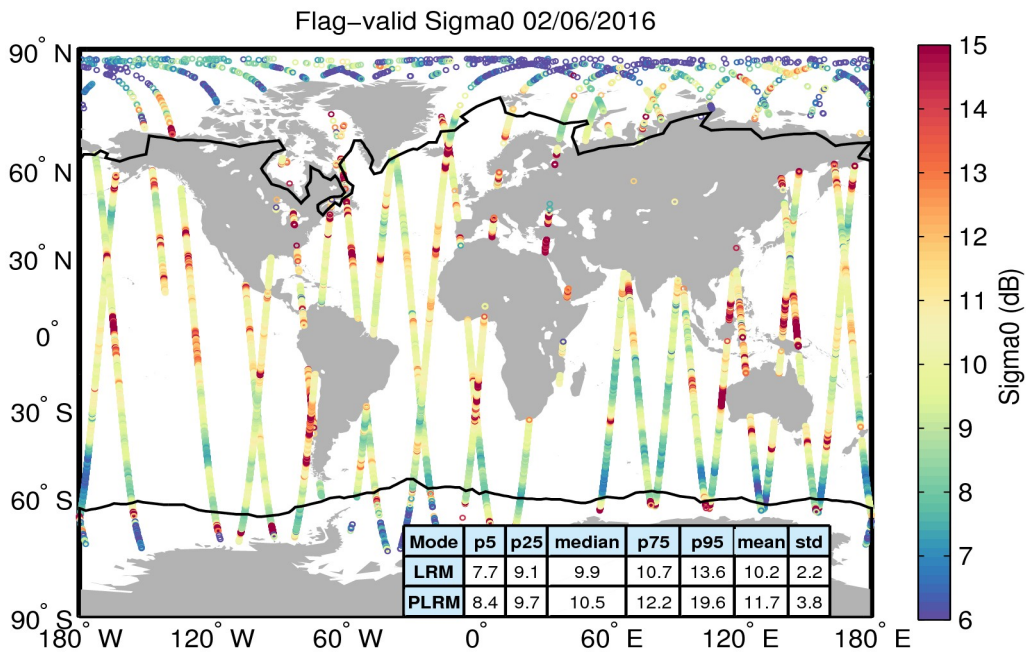
Figure 23. Geographical distribution of flag-valid sigma0 data over oceans and lakes for 02/06/2016. The statistical values shown in the table refer to the sigma0 in dB and are calculated separately for LRM and PLRM regions. Measurements taken over polar polygons have been excluded from the computation of the statistical values. The black lines mark the outer limit of the Arctic and Antarctic polar polygons.
