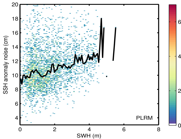
Figure 9. 2D histogram showing flag-valid SSH anomaly noise as a function of SWH for LRM (top) and PLRM (bottom) for 02/06/2016. The black line denotes the median SSH anomaly noise as a function of SWH.
