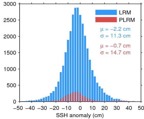
Figure 11. Histogram of science-valid SSH anomaly over oceans and lakes for LRM (blue) and PLRM (red) for 02/06/2016. The mean ( \mu ) and standard deviation ( \sigma ) are also shown. Note that values outside [-50 50] cm are excluded from the histogram for the sake of readability but not from the computation of \mu and \sigma .
