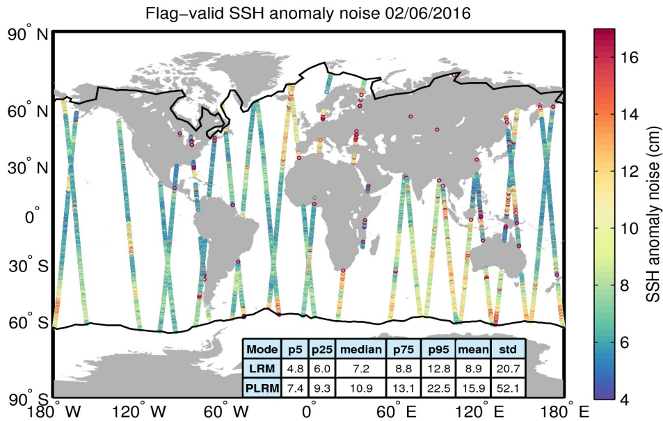
Figure 8. Geographical distribution of flag-valid 20-Hz SSH anomaly measurement noise over oceans and lakes for 02/06/2016. The statistical values shown in the table refer to the SSH anomaly noise and are calculated separately for LRM and PLRM regions. Measurements taken over polar polygons have been excluded from the computation of the statistical values. The black lines mark the outer limit of the Arctic and Antarctic polar polygons.
