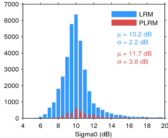
Figure 25. Histogram of flag-valid sigma0 over oceans and lakes for LRM (blue) and PLRM (red) for 02/06/2016. The mean ( \mu ) and standard deviation ( \sigma ) are also shown. Note that values outside [4 20] dB are excluded from the histogram for the sake of readability but not from the computation of \mu and \sigma .
