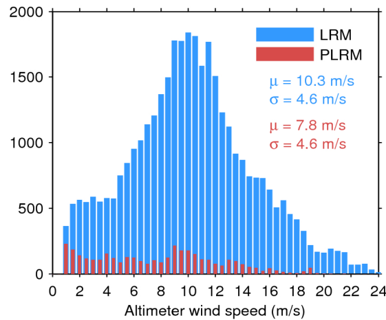
Figure 33. Histogram of flag-valid wind over oceans and lakes for LRM (blue) and PLRM (red) for 02/06/2016. The mean ( \mu ) and standard deviation ( \sigma ) are also shown. Note that values larger than 24 m/s are excluded from the histogram for the sake of readability but not from the computation of \mu and \sigma .
