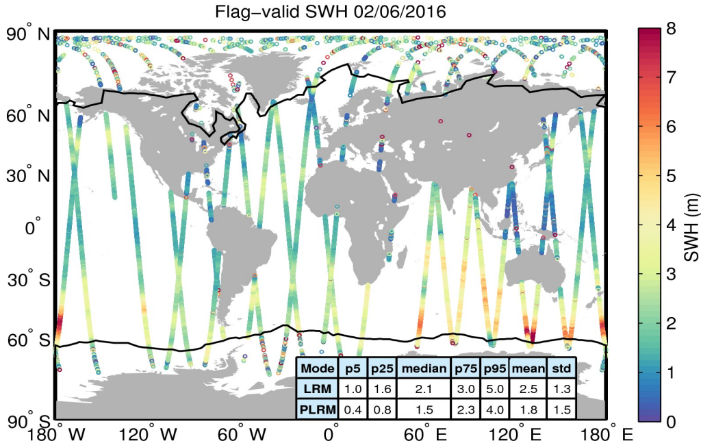
Figure 15. Geographical distribution of flag-valid SWH data over oceans and lakes for 02/06/2016. The statistical values shown in the table refer to the SWH in m and are calculated separately for LRM and PLRM regions. Measurements taken over polar polygons have been excluded from the computation of the statistical values. The black lines mark the outer limit of the Arctic and Antarctic polar polygons.
