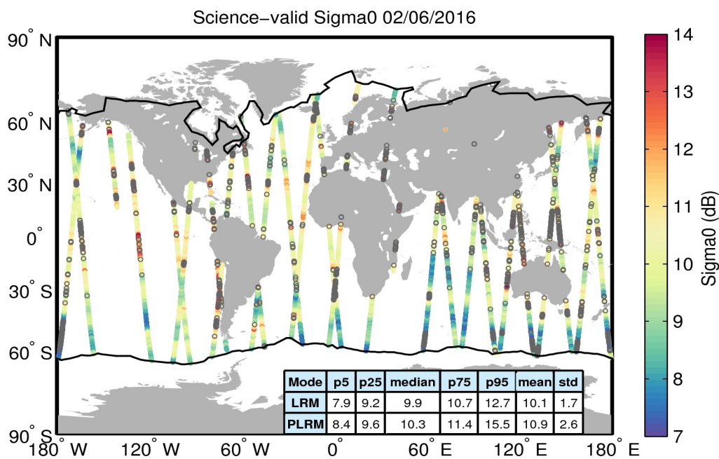
Figure 27. Geographical distribution of science-valid sigma0 data over oceans and lakes for 02/06/2016. The statistical values shown in the table refer to the sigma0 in dB and are calculated separately for LRM and PLRM regions. The black lines mark the outer limit of the Arctic and Antarctic polar polygons. Gray circles denote records that have been rejected based on the editing criteria described in Table 4.
