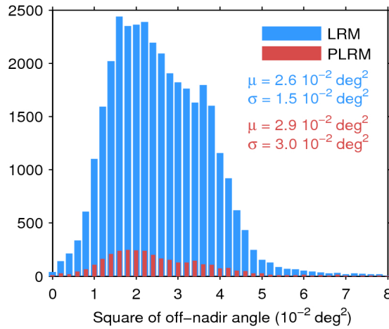
Figure 39. Histogram of flag-valid mispointing over oceans and lakes for LRM (blue) and PLRM (red) for 02/06/2016. Only positive values have been considered. The mean ( \mu ) and standard deviation ( \sigma ) are also shown. Note that values larger than 8 \cdot 10^{-2} \text{ deg}^2 are excluded from the histogram for the sake of readability but not from the computation of \mu and \sigma .
