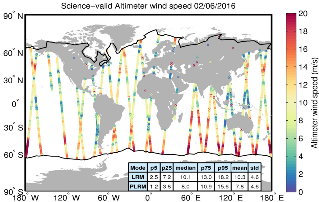
Figure 34. Geographical distribution of science-valid wind data over oceans and lakes for 02/06/2016. The statistical values shown in the table refer to the wind in m/s and are calculated separately for LRM and PLRM regions. The black lines mark the outer limit of the Arctic and Antarctic polar polygons. Gray circles denote records that have been rejected based on the editing criteria described in Table 5.
