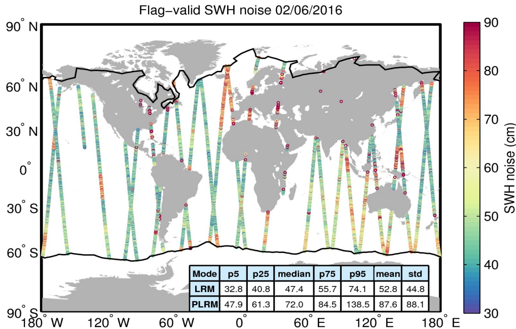
Figure 18. Geographical distribution of flag-valid 20-Hz SWH measurement noise over oceans and lakes for 02/06/2016. The statistical values shown in the table refer to the SWH noise and are calculated separately for LRM and PLRM regions. Measurements taken over polar polygons have been excluded from the computation of the statistical values. The black lines mark the outer limit of the Arctic and Antarctic polar polygons.
