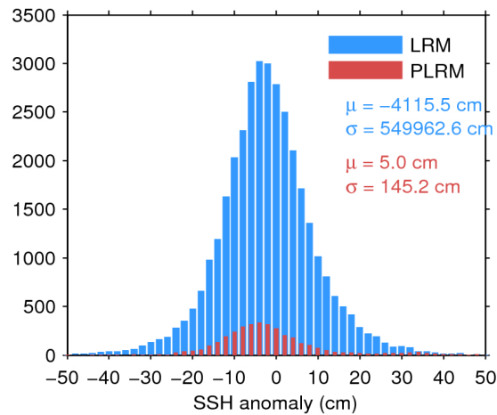
Figure 7. Histogram of flag-valid SSH anomaly over oceans and lakes for LRM (blue) and PLRM (red) for 02/06/2016. The mean ( \mu ) and standard deviation ( \sigma ) are also shown. Note that values outside [-50 50] cm are excluded from the histogram for the sake of readability but not from the computation of \mu and \sigma .
