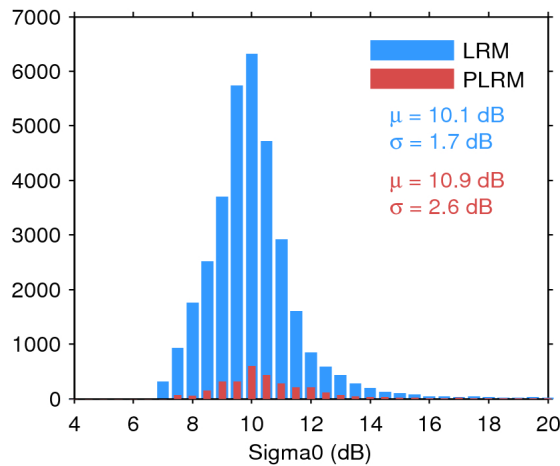
Figure 28. Histogram of science-valid sigma0 over oceans and lakes for LRM (blue) and PLRM (red) for 02/06/2016. The mean ( \mu ) and standard deviation ( \sigma ) are also shown. Note that values outside [4 20] dB are excluded from the histogram for the sake of readability but not from the computation of \mu and \sigma .
