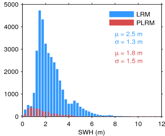
Figure 17. Histogram of flag-valid SWH over oceans and lakes for LRM (blue) and PLRM (red) for 02/06/2016. The mean ( \mu ) and standard deviation ( \sigma ) are also shown. Note that values larger than 12 m are excluded from the histogram for the sake of readability but not from the computation of \mu and \sigma .
