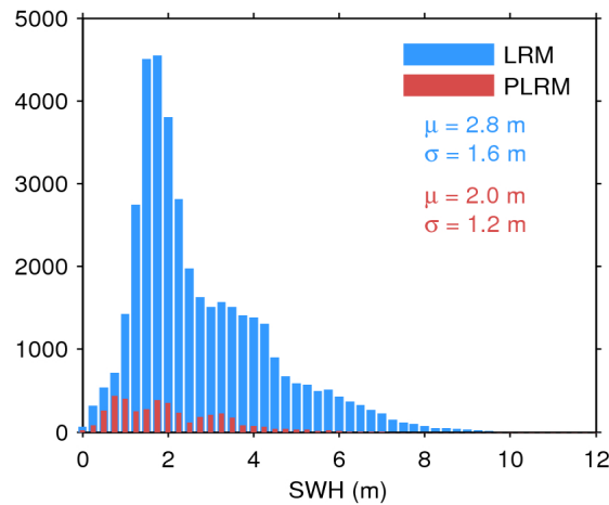
Figure 20. Histogram of science-valid SWH over oceans and lakes for LRM (blue) and PLRM (red) for 25/05/2016. The mean ( \mu ) and standard deviation ( \sigma ) are also shown. Note that values larger than 12 m are excluded from the histogram for the sake of readability but not from the computation of \mu and \sigma .
