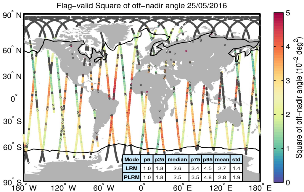
Figure 37. Geographical distribution of flag-valid mispointing data over oceans and lakes for 25/05/2016. The statistical values shown in the table refer to the mispointing in 10^{-2} deg 2 and are calculated separately for LRM and PLRM regions. Measurements taken over polar polygons have been excluded from the computation of the statistical values. The black lines mark the outer limit of the Arctic and Antarctic polar polygons. Gray circles denote negative values.
