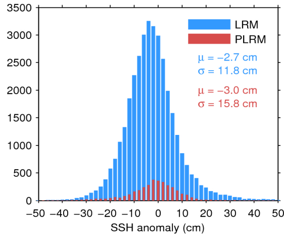
Figure 11. Histogram of science-valid SSH anomaly over oceans and lakes for LRM (blue) and PLRM (red) for 25/05/2016. The mean ( \mu ) and standard deviation ( \sigma ) are also shown. Note that values outside [-50 50] cm are excluded from the histogram for the sake of readability but not from the computation of \mu and \sigma .
