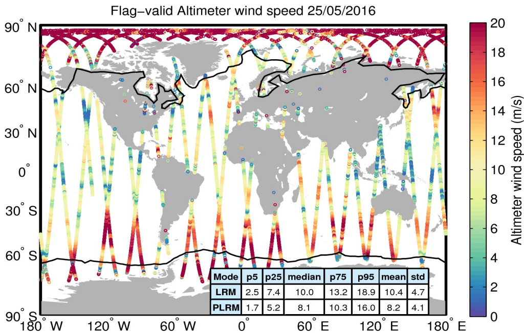
Figure 31. Geographical distribution of flag-valid wind data over oceans and lakes for 25/05/2016. The statistical values shown in the table refer to the wind in m/s and are calculated separately for LRM and PLRM regions. Measurements taken over polar polygons have been excluded from the computation of the statistical values. The black lines mark the outer limit of the Arctic and Antarctic polar polygons.
