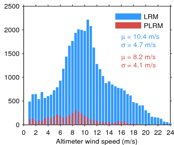
Figure 35. Histogram of science-valid wind over oceans and lakes for LRM (blue) and PLRM (red) for 25/05/2016. The mean ( \mu ) and standard deviation ( \sigma ) are also shown. Note that values larger than 24 m/s are excluded from the histogram for the sake of readability but not from the computation of \mu and \sigma .
