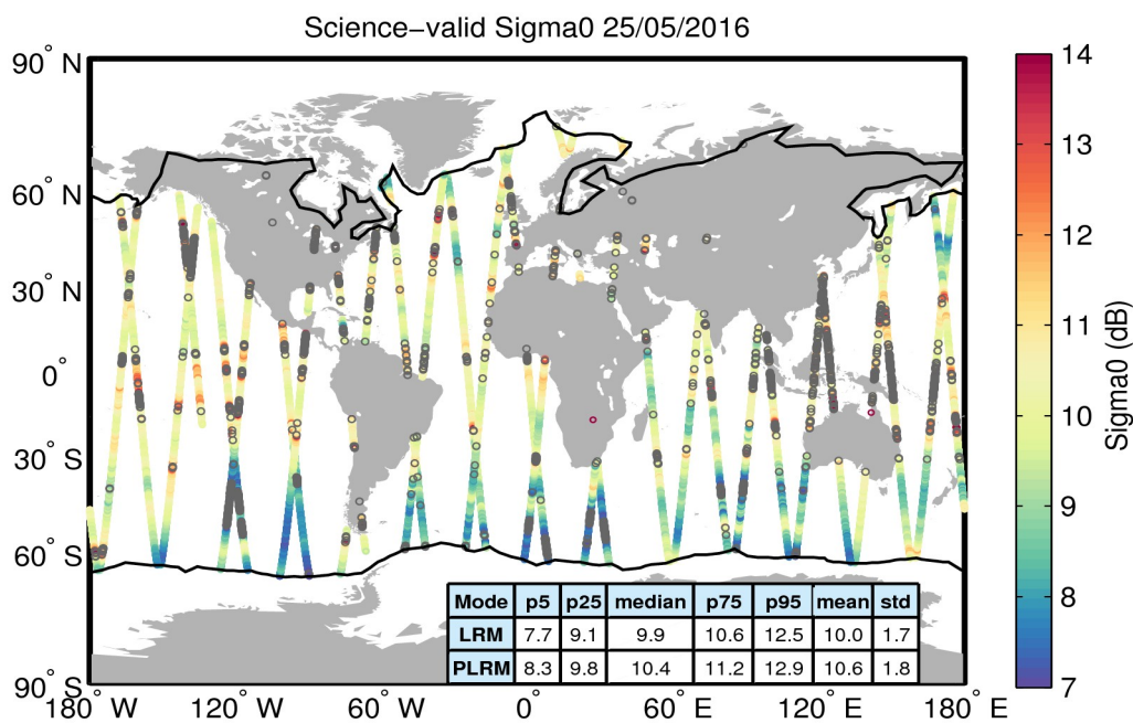
Figure 27. Geographical distribution of science-valid sigma0 data over oceans and lakes for 25/05/2016. The statistical values shown in the table refer to the sigma0 in dB and are calculated separately for LRM and PLRM regions. The black lines mark the outer limit of the Arctic and Antarctic polar polygons. Gray circles denote records that have been rejected based on the editing criteria described in Table 4.
