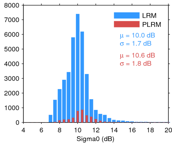
Figure 28. Histogram of science-valid sigma0 over oceans and lakes for LRM (blue) and PLRM (red) for 25/05/2016. The mean ( \mu ) and standard deviation ( \sigma ) are also shown. Note that values outside [4 20] dB are excluded from the histogram for the sake of readability but not from the computation of \mu and \sigma .
