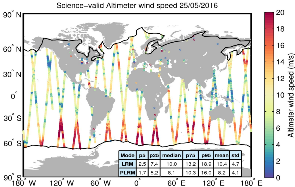
Figure 34. Geographical distribution of science-valid wind data over oceans and lakes for 25/05/2016. The statistical values shown in the table refer to the wind in m/s and are calculated separately for LRM and PLRM regions. The black lines mark the outer limit of the Arctic and Antarctic polar polygons. Gray circles denote records that have been rejected based on the editing criteria described in Table 5.
