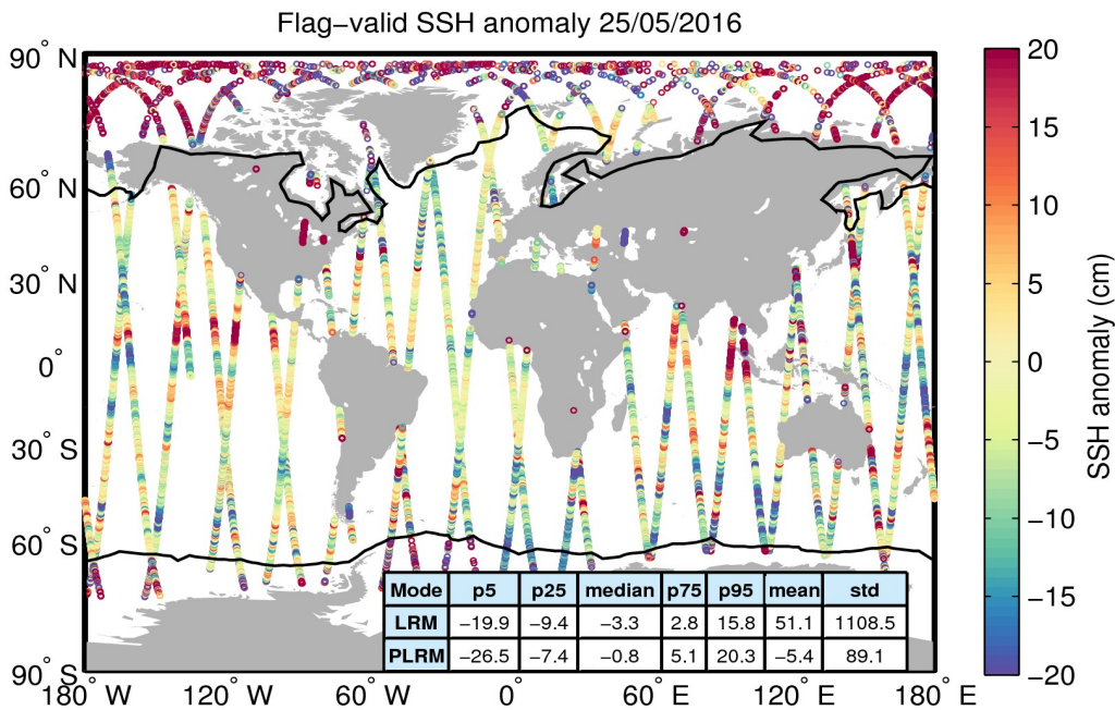
Figure 5. Geographical distribution of flag-valid 1-Hz SSH anomaly data over oceans and lakes for 25/05/2016. The statistical values shown in the table refer to the SSH anomaly in cm and are calculated separately for LRM and PLRM regions. Measurements taken over polar polygons have been excluded from the computation of the statistical values. The black lines mark the outer limit of the Arctic and Antarctic polar polygons.
