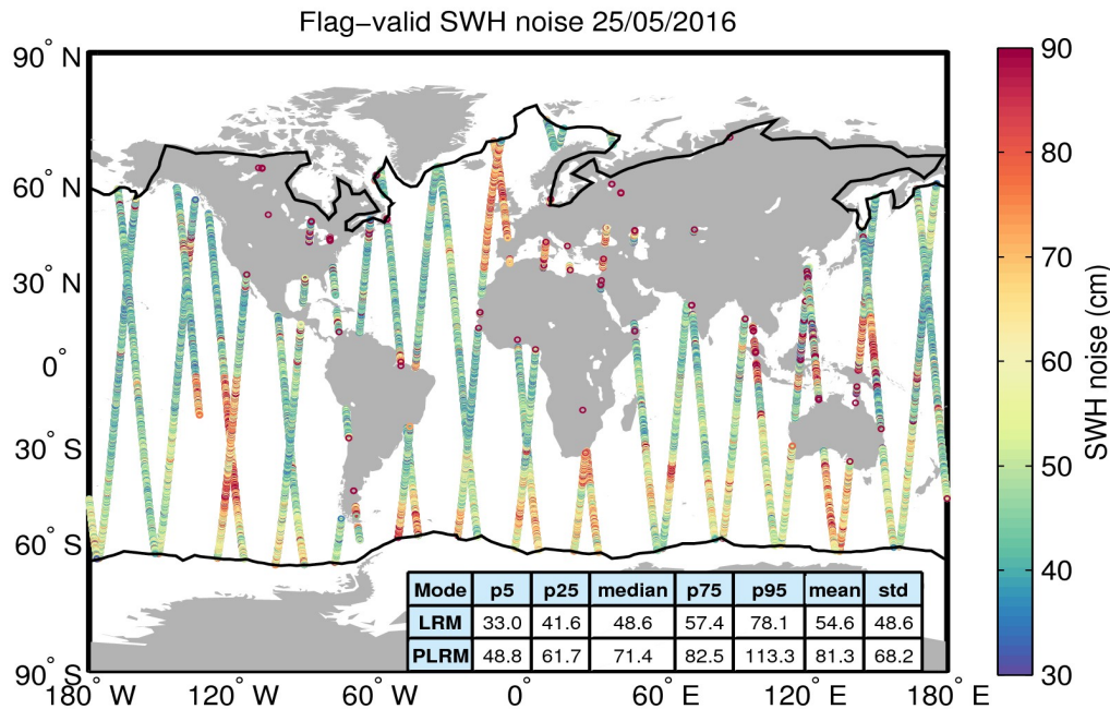
Figure 18. Geographical distribution of flag-valid 20-Hz SWH measurement noise over oceans and lakes for 25/05/2016. The statistical values shown in the table refer to the SWH noise and are calculated separately for LRM and PLRM regions. Measurements taken over polar polygons have been excluded from the computation of the statistical values. The black lines mark the outer limit of the Arctic and Antarctic polar polygons.
