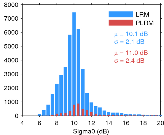
Figure 25. Histogram of flag-valid sigma0 over oceans and lakes for LRM (blue) and PLRM (red) for 25/05/2016. The mean ( \mu ) and standard deviation ( \sigma ) are also shown. Note that values outside [4 20] dB are excluded from the histogram for the sake of readability but not from the computation of \mu and \sigma .
