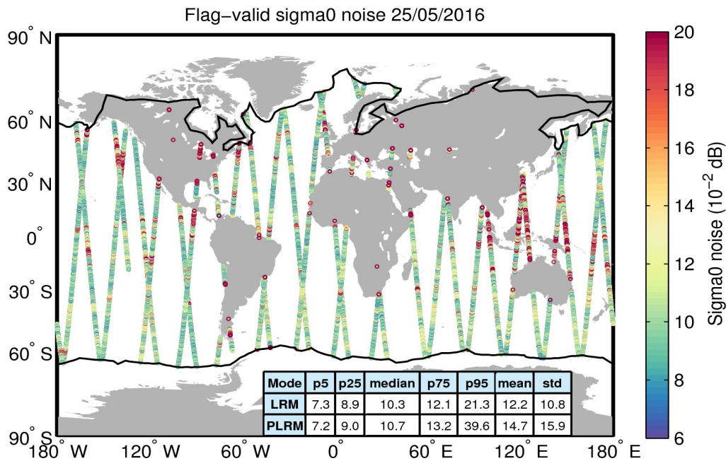
Figure 26. Geographical distribution of flag-valid 20-Hz sigma0 measurement noise over oceans and lakes for 25/05/2016. The statistical values shown in the table refer to the sigma0 noise and are calculated separately for LRM and PLRM regions. Measurements taken over polar polygons have been excluded from the computation of the statistical values. The black lines mark the outer limit of the Arctic and Antarctic polar polygons.
