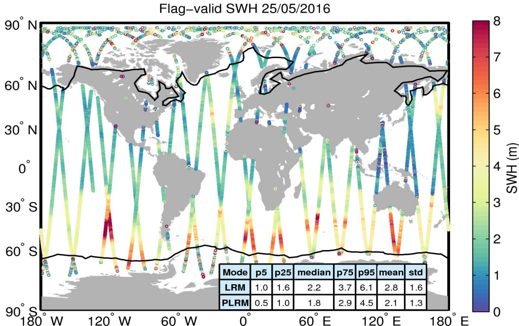
Figure 15. Geographical distribution of flag-valid SWH data over oceans and lakes for 25/05/2016. The statistical values shown in the table refer to the SWH in m and are calculated separately for LRM and PLRM regions. Measurements taken over polar polygons have been excluded from the computation of the statistical values. The black lines mark the outer limit of the Arctic and Antarctic polar polygons.
