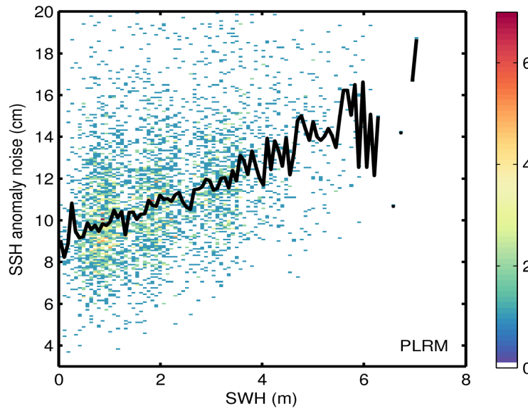
Figure 9. 2D histogram showing flag-valid SSH anomaly noise as a function of SWH for LRM (top) and PLRM (bottom) for 25/05/2016. The black line denotes the median SSH anomaly noise as a function of SWH.
