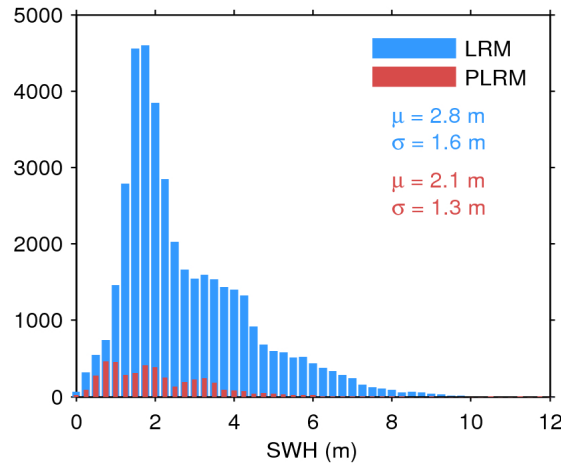
Figure 17. Histogram of flag-valid SWH over oceans and lakes for LRM (blue) and PLRM (red) for 25/05/2016. The mean ( \mu ) and standard deviation ( \sigma ) are also shown. Note that values larger than 12 m are excluded from the histogram for the sake of readability but not from the computation of \mu and \sigma .
