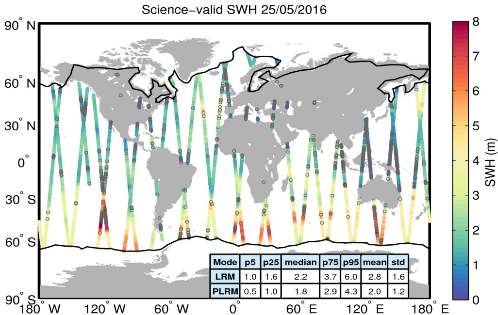
Figure 19. Geographical distribution of science-valid SWH data over oceans and lakes for 25/05/2016. The statistical values shown in the table refer to the SWH in m and are calculated separately for LRM and PLRM regions. The black lines mark the outer limit of the Arctic and Antarctic polar polygons. Gray circles denote records that have been rejected based on the editing criteria described in Table 3.
