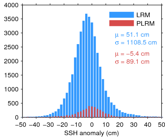
Figure 7. Histogram of flag-valid SSH anomaly over oceans and lakes for LRM (blue) and PLRM (red) for 25/05/2016. The mean ( \mu ) and standard deviation ( \sigma ) are also shown. Note that values outside [-50 50] cm are excluded from the histogram for the sake of readability but not from the computation of \mu and \sigma .
