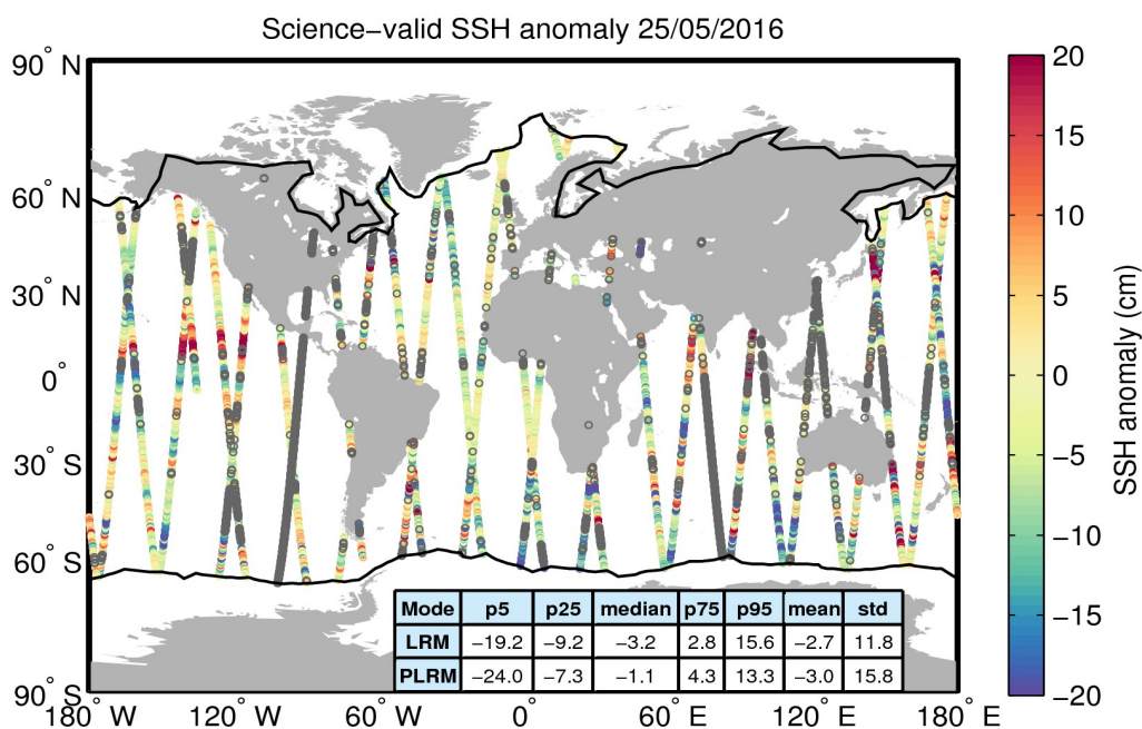
Figure 10. Geographical distribution of science-valid SSH anomaly data over oceans and lakes for 25/05/2016. The statistical values shown in the table refer to the SSH anomaly in cm and are calculated separately for LRM and PLRM regions. The black lines mark the outer limit of the Arctic and Antarctic polar polygons. Gray circles denote records that have been rejected based on the editing criteria described in Table 2.
