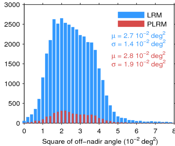
Figure 39. Histogram of flag-valid mispointing over oceans and lakes for LRM (blue) and PLRM (red) for 25/05/2016. Only positive values have been considered. The mean ( \mu ) and standard deviation ( \sigma ) are also shown. Note that values larger than 8 \cdot 10^{-2} \text{ deg}^2 are excluded from the histogram for the sake of readability but not from the computation of \mu and \sigma .
