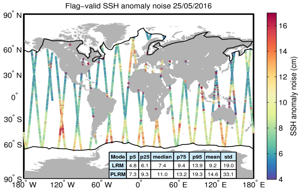
Figure 8. Geographical distribution of flag-valid 20-Hz SSH anomaly measurement noise over oceans and lakes for 25/05/2016. The statistical values shown in the table refer to the SSH anomaly noise and are calculated separately for LRM and PLRM regions. Measurements taken over polar polygons have been excluded from the computation of the statistical values. The black lines mark the outer limit of the Arctic and Antarctic polar polygons.
