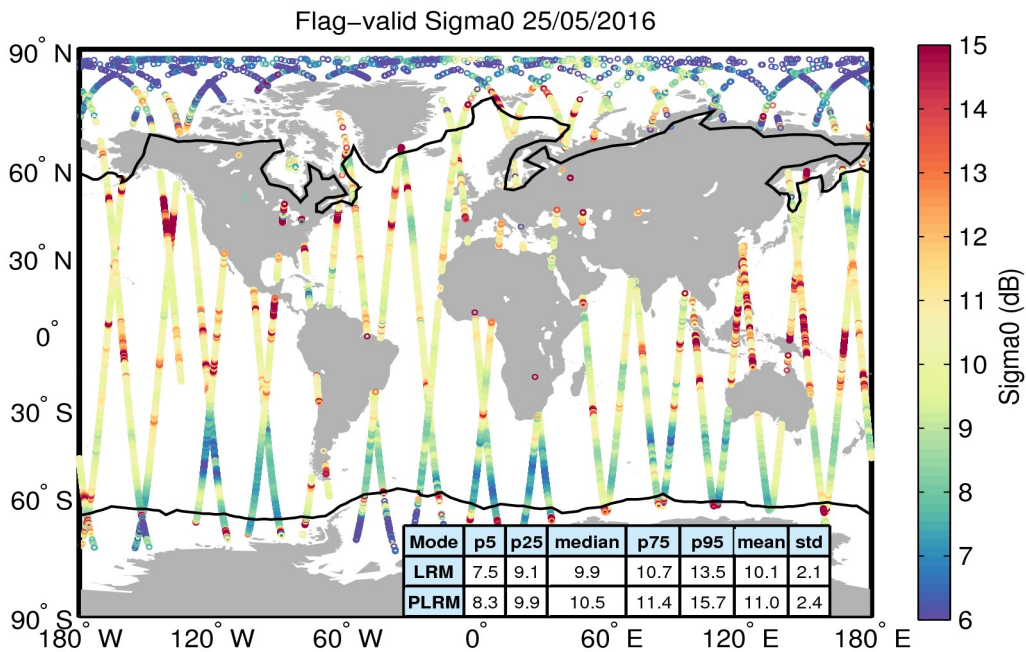
Figure 23. Geographical distribution of flag-valid sigma0 data over oceans and lakes for 25/05/2016. The statistical values shown in the table refer to the sigma0 in dB and are calculated separately for LRM and PLRM regions. Measurements taken over polar polygons have been excluded from the computation of the statistical values. The black lines mark the outer limit of the Arctic and Antarctic polar polygons.
