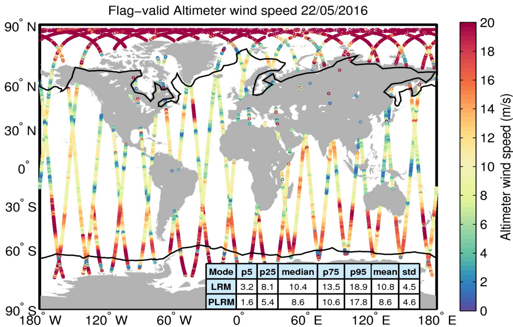
Figure 31. Geographical distribution of flag-valid wind data over oceans and lakes for 22/05/2016. The statistical values shown in the table refer to the wind in m/s and are calculated separately for LRM and PLRM regions. Measurements taken over polar polygons have been excluded from the computation of the statistical values. The black lines mark the outer limit of the Arctic and Antarctic polar polygons.
