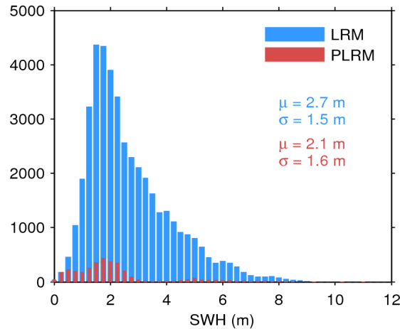
Figure 17. Histogram of flag-valid SWH over oceans and lakes for LRM (blue) and PLRM (red) for 22/05/2016. The mean ( \mu ) and standard deviation ( \sigma ) are also shown. Note that values larger than 12 m are excluded from the histogram for the sake of readability but not from the computation of \mu and \sigma .
