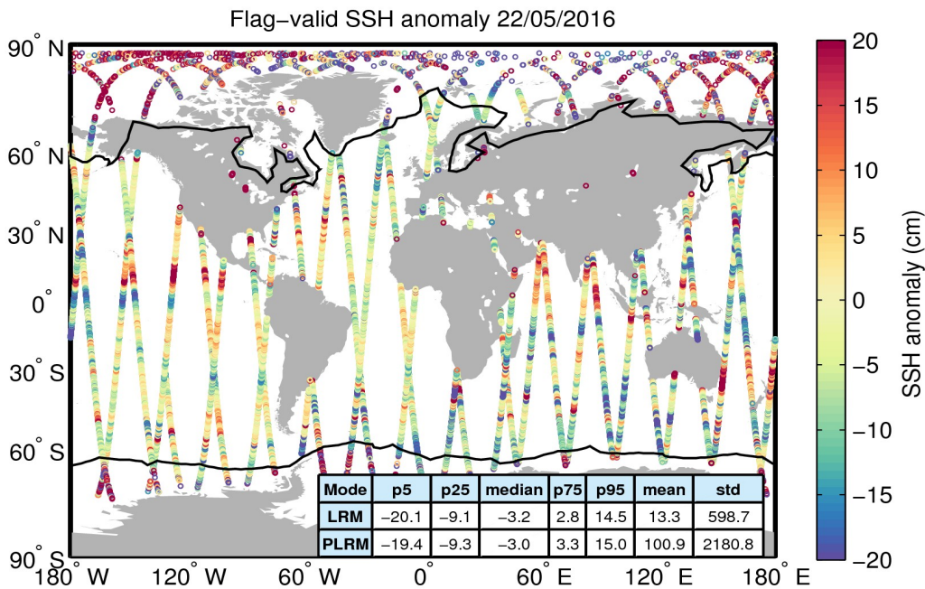
Figure 5. Geographical distribution of flag-valid 1-Hz SSH anomaly data over oceans and lakes for 22/05/2016. The statistical values shown in the table refer to the SSH anomaly in cm and are calculated separately for LRM and PLRM regions. Measurements taken over polar polygons have been excluded from the computation of the statistical values. The black lines mark the outer limit of the Arctic and Antarctic polar polygons.
