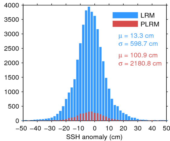
Figure 7. Histogram of flag-valid SSH anomaly over oceans and lakes for LRM (blue) and PLRM (red) for 22/05/2016. The mean ( \mu ) and standard deviation ( \sigma ) are also shown. Note that values outside [-50 50] cm are excluded from the histogram for the sake of readability but not from the computation of \mu and \sigma .
