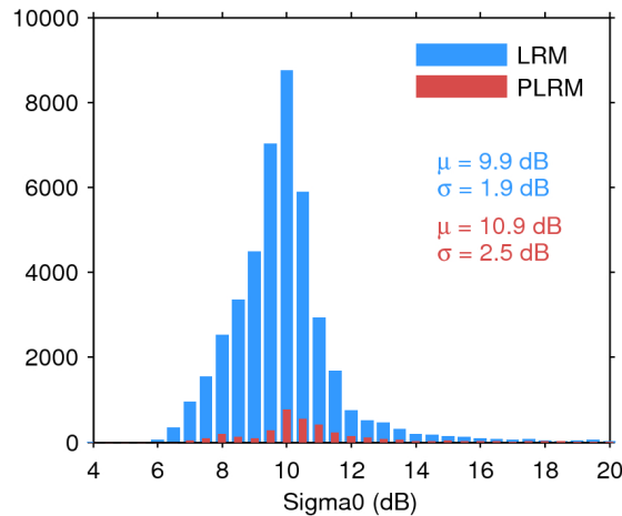
Figure 25. Histogram of flag-valid sigma0 over oceans and lakes for LRM (blue) and PLRM (red) for 22/05/2016. The mean ( \mu ) and standard deviation ( \sigma ) are also shown. Note that values outside [4 20] dB are excluded from the histogram for the sake of readability but not from the computation of \mu and \sigma .
