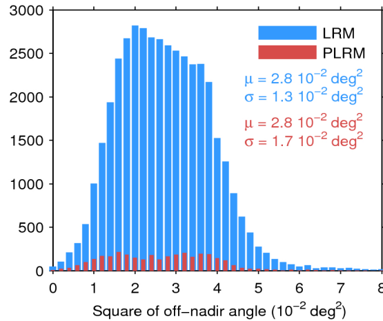
Figure 39. Histogram of flag-valid mispointing over oceans and lakes for LRM (blue) and PLRM (red) for 22/05/2016. Only positive values have been considered. The mean ( \mu ) and standard deviation ( \sigma ) are also shown. Note that values larger than 8 \cdot 10^{-2} \text{ deg}^2 are excluded from the histogram for the sake of readability but not from the computation of \mu and \sigma .
