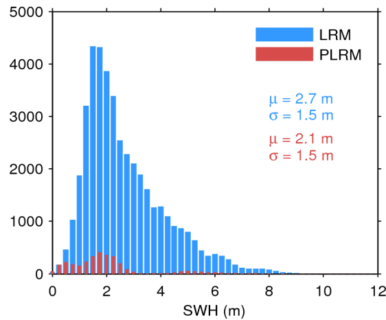
Figure 20. Histogram of science-valid SWH over oceans and lakes for LRM (blue) and PLRM (red) for 22/05/2016. The mean ( \mu ) and standard deviation ( \sigma ) are also shown. Note that values larger than 12 m are excluded from the histogram for the sake of readability but not from the computation of \mu and \sigma .
