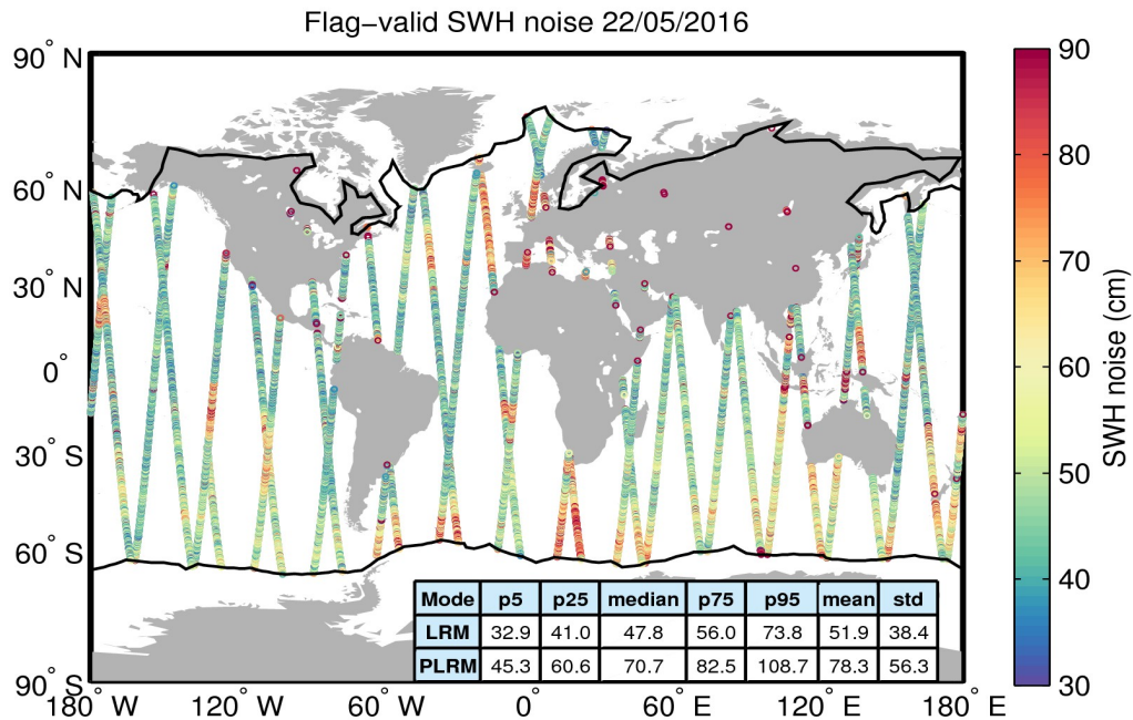
Figure 18. Geographical distribution of flag-valid 20-Hz SWH measurement noise over oceans and lakes for 22/05/2016. The statistical values shown in the table refer to the SWH noise and are calculated separately for LRM and PLRM regions. Measurements taken over polar polygons have been excluded from the computation of the statistical values. The black lines mark the outer limit of the Arctic and Antarctic polar polygons.
