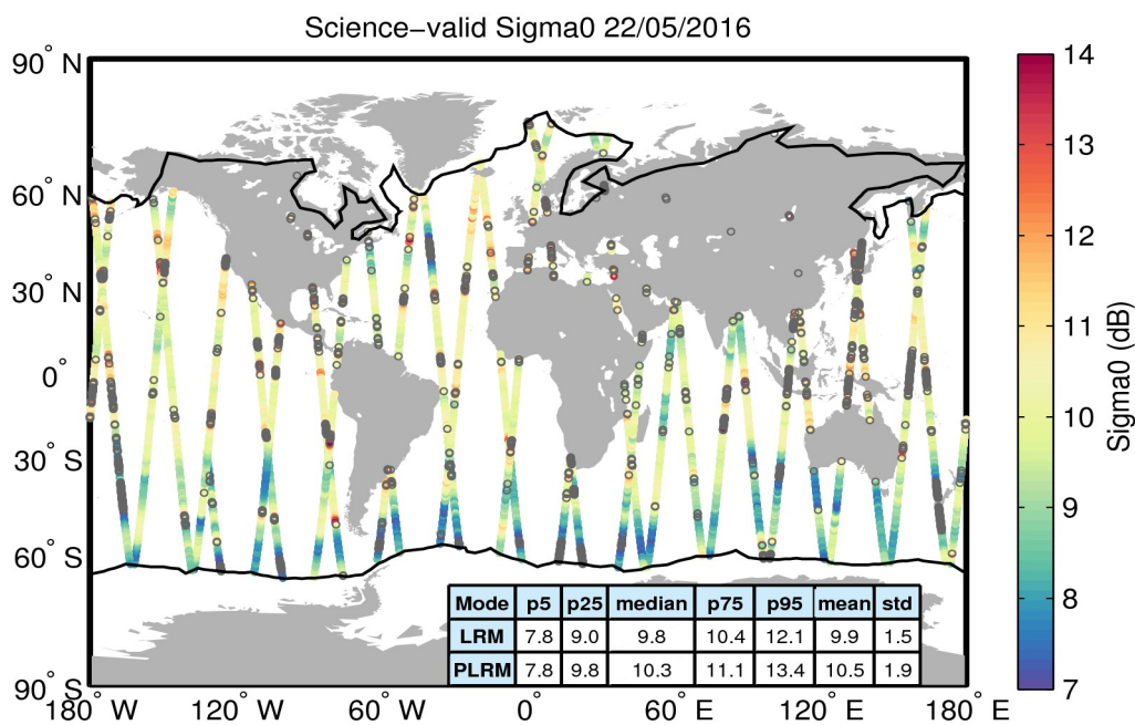
Figure 27. Geographical distribution of science-valid sigma0 data over oceans and lakes for 22/05/2016. The statistical values shown in the table refer to the sigma0 in dB and are calculated separately for LRM and PLRM regions. The black lines mark the outer limit of the Arctic and Antarctic polar polygons. Gray circles denote records that have been rejected based on the editing criteria described in Table 4.
