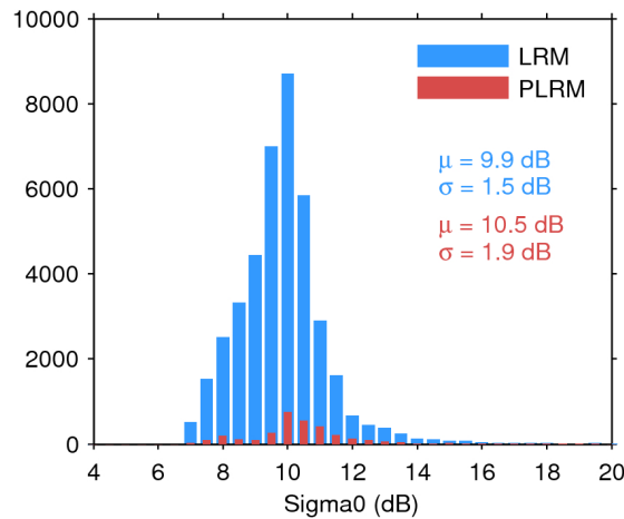
Figure 28. Histogram of science-valid sigma0 over oceans and lakes for LRM (blue) and PLRM (red) for 22/05/2016. The mean ( \mu ) and standard deviation ( \sigma ) are also shown. Note that values outside [4 20] dB are excluded from the histogram for the sake of readability but not from the computation of \mu and \sigma .
