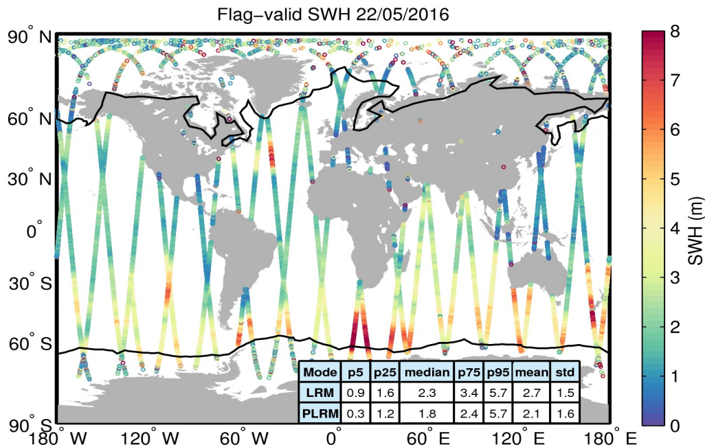
Figure 15. Geographical distribution of flag-valid SWH data over oceans and lakes for 22/05/2016. The statistical values shown in the table refer to the SWH in m and are calculated separately for LRM and PLRM regions. Measurements taken over polar polygons have been excluded from the computation of the statistical values. The black lines mark the outer limit of the Arctic and Antarctic polar polygons.
