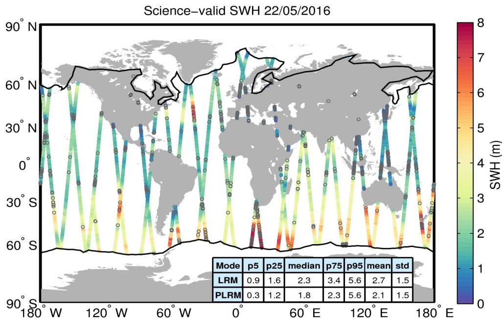
Figure 19. Geographical distribution of science-valid SWH data over oceans and lakes for 22/05/2016. The statistical values shown in the table refer to the SWH in m and are calculated separately for LRM and PLRM regions. The black lines mark the outer limit of the Arctic and Antarctic polar polygons. Gray circles denote records that have been rejected based on the editing criteria described in Table 3.
