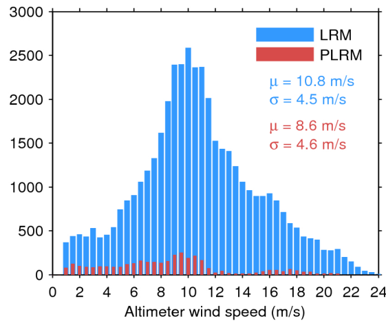
Figure 33. Histogram of flag-valid wind over oceans and lakes for LRM (blue) and PLRM (red) for 22/05/2016. The mean ( \mu ) and standard deviation ( \sigma ) are also shown. Note that values larger than 24 m/s are excluded from the histogram for the sake of readability but not from the computation of \mu and \sigma .
