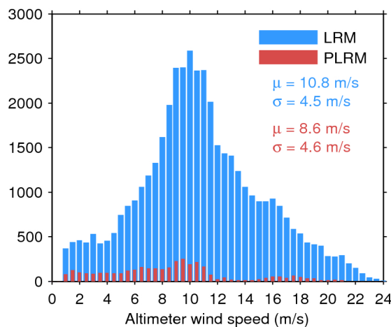
Figure 35. Histogram of science-valid wind over oceans and lakes for LRM (blue) and PLRM (red) for 22/05/2016. The mean ( \mu ) and standard deviation ( \sigma ) are also shown. Note that values larger than 24 m/s are excluded from the histogram for the sake of readability but not from the computation of \mu and \sigma .
