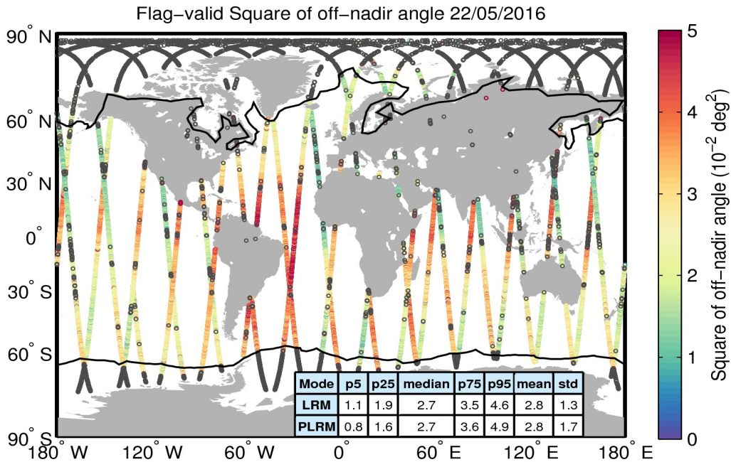
Figure 37. Geographical distribution of flag-valid mispointing data over oceans and lakes for 22/05/2016. The statistical values shown in the table refer to the mispointing in 10^{-2} \text{ deg}^2 and are calculated separately for LRM and PLRM regions. Measurements taken over polar polygons have been excluded from the computation of the statistical values. The black lines mark the outer limit of the Arctic and Antarctic polar polygons. Gray circles denote negative values.
