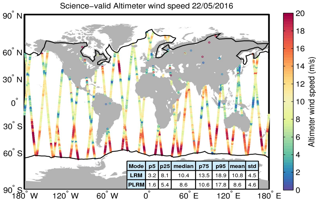
Figure 34. Geographical distribution of science-valid wind data over oceans and lakes for 22/05/2016. The statistical values shown in the table refer to the wind in m/s and are calculated separately for LRM and PLRM regions. The black lines mark the outer limit of the Arctic and Antarctic polar polygons. Gray circles denote records that have been rejected based on the editing criteria described in Table 5.
