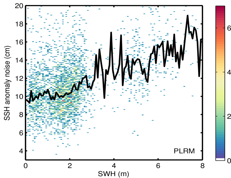
Figure 9. 2D histogram showing flag-valid SSH anomaly noise as a function of SWH for LRM (top) and PLRM (bottom) for 22/05/2016. The black line denotes the median SSH anomaly noise as a function of SWH.
