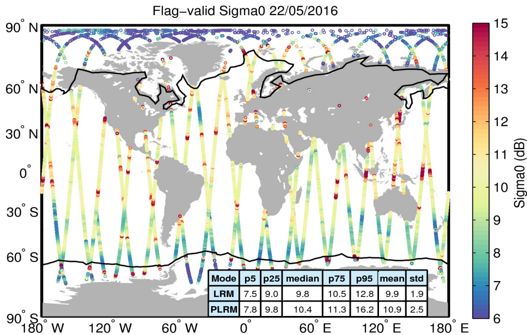
Figure 23. Geographical distribution of flag-valid sigma0 data over oceans and lakes for 22/05/2016. The statistical values shown in the table refer to the sigma0 in dB and are calculated separately for LRM and PLRM regions. Measurements taken over polar polygons have been excluded from the computation of the statistical values. The black lines mark the outer limit of the Arctic and Antarctic polar polygons.
