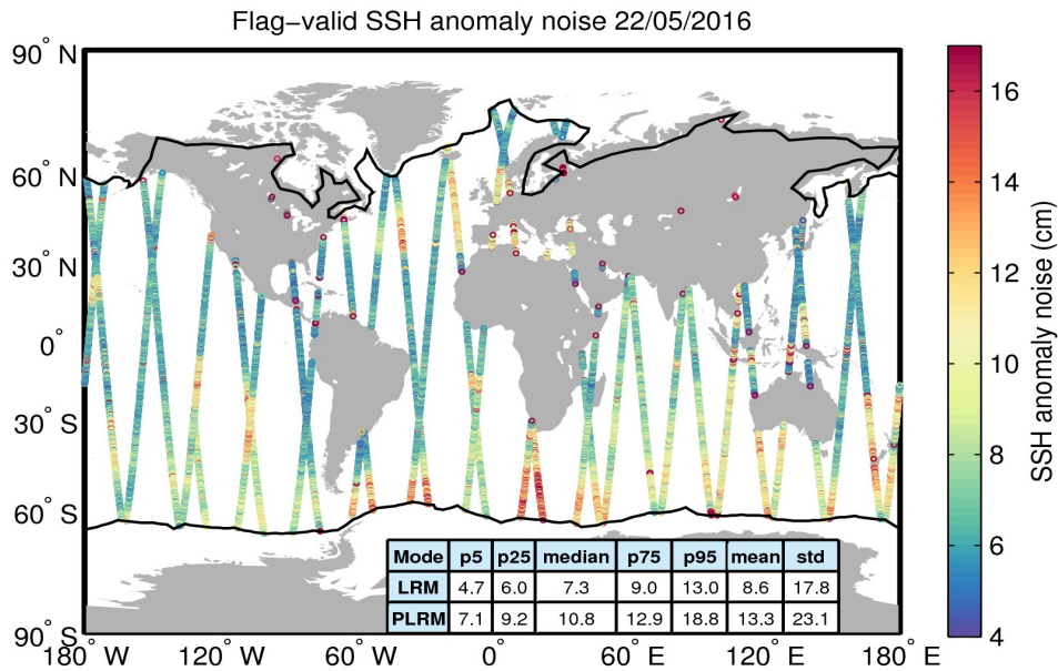
Figure 8. Geographical distribution of flag-valid 20-Hz SSH anomaly measurement noise over oceans and lakes for 22/05/2016. The statistical values shown in the table refer to the SSH anomaly noise and are calculated separately for LRM and PLRM regions. Measurements taken over polar polygons have been excluded from the computation of the statistical values. The black lines mark the outer limit of the Arctic and Antarctic polar polygons.
