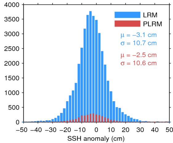
Figure 11. Histogram of science-valid SSH anomaly over oceans and lakes for LRM (blue) and PLRM (red) for 22/05/2016. The mean ( \mu ) and standard deviation ( \sigma ) are also shown. Note that values outside [-50 50] cm are excluded from the histogram for the sake of readability but not from the computation of \mu and \sigma .
