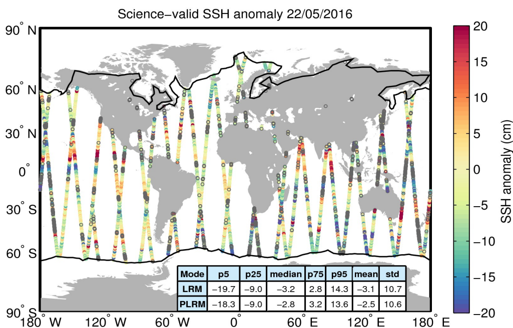
Figure 10. Geographical distribution of science-valid SSH anomaly data over oceans and lakes for 22/05/2016. The statistical values shown in the table refer to the SSH anomaly in cm and are calculated separately for LRM and PLRM regions. The black lines mark the outer limit of the Arctic and Antarctic polar polygons. Gray circles denote records that have been rejected based on the editing criteria described in Table 2.
