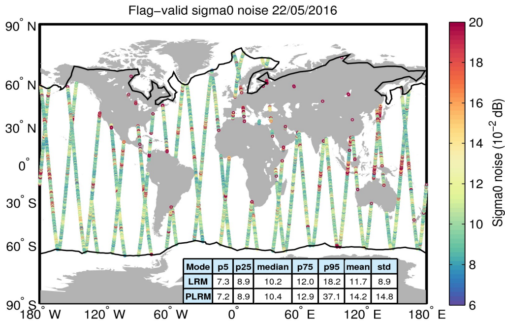
Figure 26. Geographical distribution of flag-valid 20-Hz sigma0 measurement noise over oceans and lakes for 22/05/2016. The statistical values shown in the table refer to the sigma0 noise and are calculated separately for LRM and PLRM regions. Measurements taken over polar polygons have been excluded from the computation of the statistical values. The black lines mark the outer limit of the Arctic and Antarctic polar polygons.
