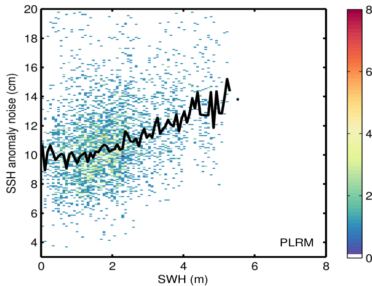
Figure 9. 2D histogram showing flag-valid SSH anomaly noise as a function of SWH for LRM (top) and PLRM (bottom) for 20/05/2016. The black line denotes the median SSH anomaly noise as a function of SWH.
