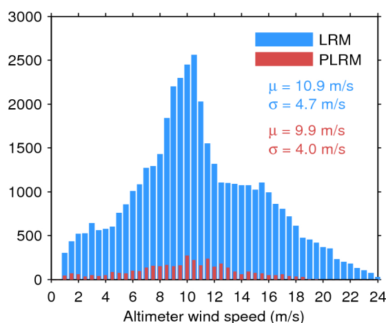
Figure 33. Histogram of flag-valid wind over oceans and lakes for LRM (blue) and PLRM (red) for 20/05/2016. The mean ( \mu ) and standard deviation ( \sigma ) are also shown. Note that values larger than 24 m/s are excluded from the histogram for the sake of readability but not from the computation of \mu and \sigma .
