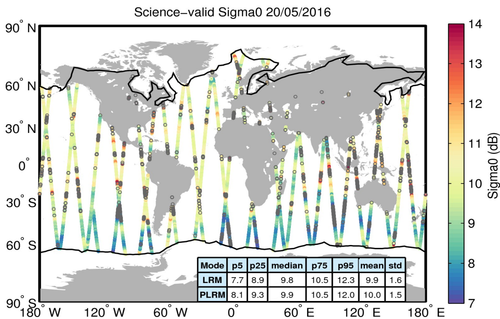
Figure 27. Geographical distribution of science-valid sigma0 data over oceans and lakes for 20/05/2016. The statistical values shown in the table refer to the sigma0 in dB and are calculated separately for LRM and PLRM regions. The black lines mark the outer limit of the Arctic and Antarctic polar polygons. Gray circles denote records that have been rejected based on the editing criteria described in Table 4.
