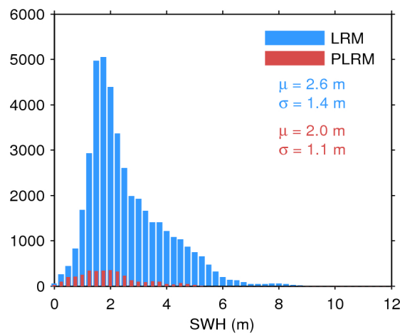
Figure 20. Histogram of science-valid SWH over oceans and lakes for LRM (blue) and PLRM (red) for 20/05/2016. The mean ( \mu ) and standard deviation ( \sigma ) are also shown. Note that values larger than 12 m are excluded from the histogram for the sake of readability but not from the computation of \mu and \sigma .
