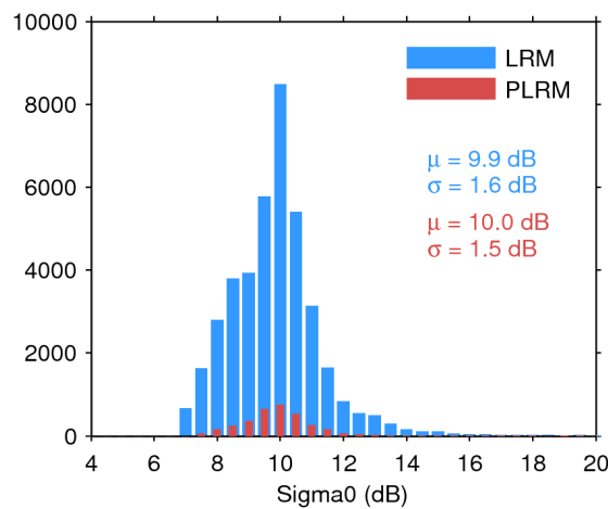
Figure 28. Histogram of science-valid sigma0 over oceans and lakes for LRM (blue) and PLRM (red) for 20/05/2016. The mean ( \mu ) and standard deviation ( \sigma ) are also shown. Note that values outside [4 20] dB are excluded from the histogram for the sake of readability but not from the computation of \mu and \sigma .
