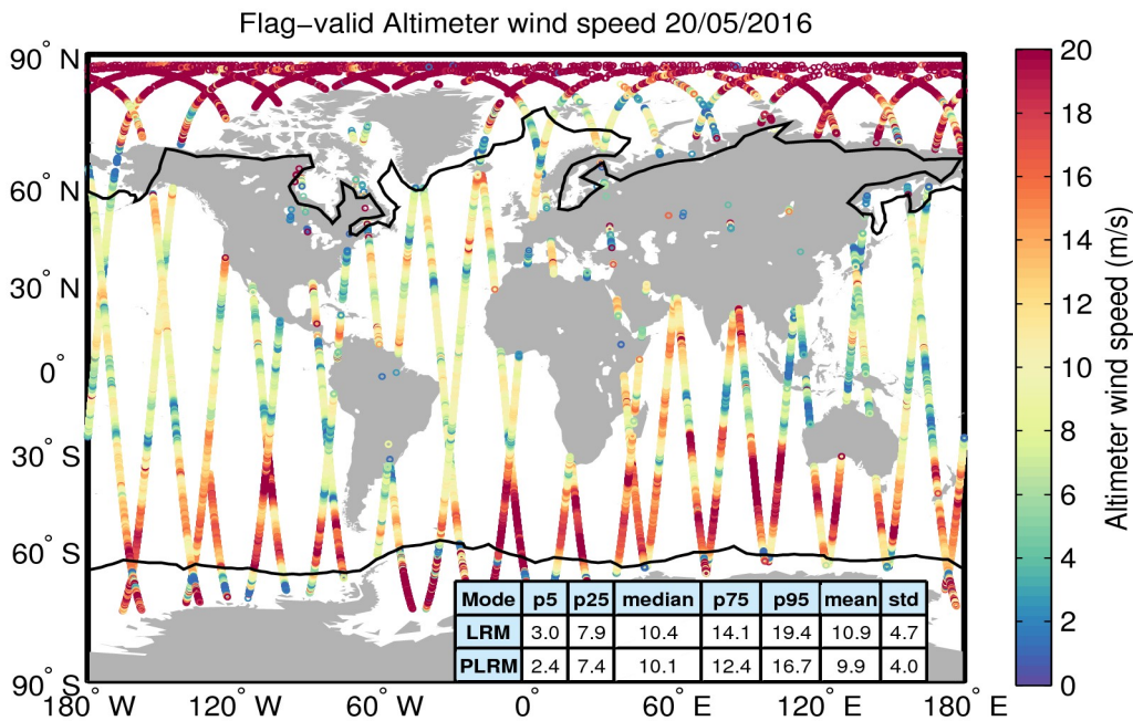
Figure 31. Geographical distribution of flag-valid wind data over oceans and lakes for 20/05/2016. The statistical values shown in the table refer to the wind in m/s and are calculated separately for LRM and PLRM regions. Measurements taken over polar polygons have been excluded from the computation of the statistical values. The black lines mark the outer limit of the Arctic and Antarctic polar polygons.
