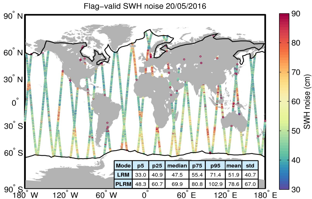
Figure 18. Geographical distribution of flag-valid 20-Hz SWH measurement noise over oceans and lakes for 20/05/2016. The statistical values shown in the table refer to the SWH noise and are calculated separately for LRM and PLRM regions. Measurements taken over polar polygons have been excluded from the computation of the statistical values. The black lines mark the outer limit of the Arctic and Antarctic polar polygons.
