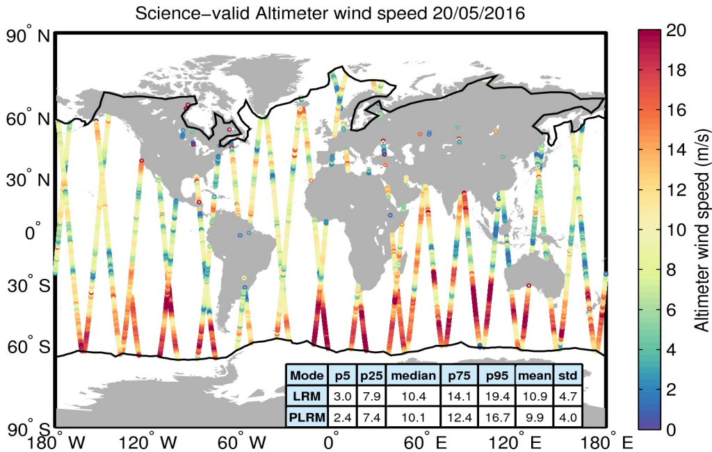
Figure 34. Geographical distribution of science-valid wind data over oceans and lakes for 20/05/2016. The statistical values shown in the table refer to the wind in m/s and are calculated separately for LRM and PLRM regions. The black lines mark the outer limit of the Arctic and Antarctic polar polygons. Gray circles denote records that have been rejected based on the editing criteria described in Table 5.
