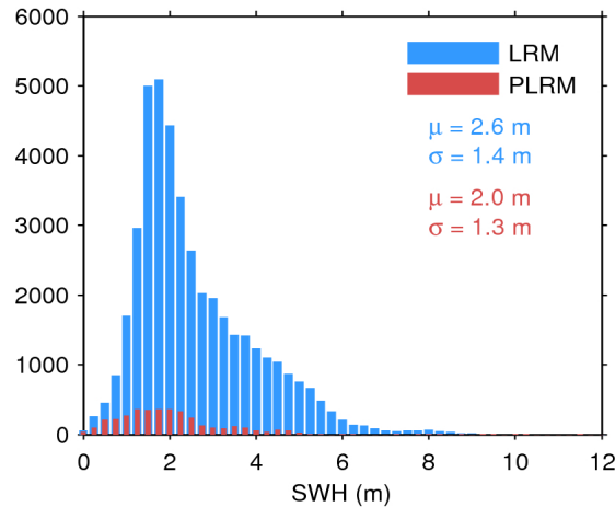
Figure 17. Histogram of flag-valid SWH over oceans and lakes for LRM (blue) and PLRM (red) for 20/05/2016. The mean ( \mu ) and standard deviation ( \sigma ) are also shown. Note that values larger than 12 m are excluded from the histogram for the sake of readability but not from the computation of \mu and \sigma .
