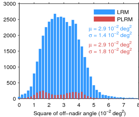
Figure 39. Histogram of flag-valid mispointing over oceans and lakes for LRM (blue) and PLRM (red) for 20/05/2016. Only positive values have been considered. The mean ( \mu ) and standard deviation ( \sigma ) are also shown. Note that values larger than 8 \cdot 10^{-2} \text{ deg}^2 are excluded from the histogram for the sake of readability but not from the computation of \mu and \sigma .
