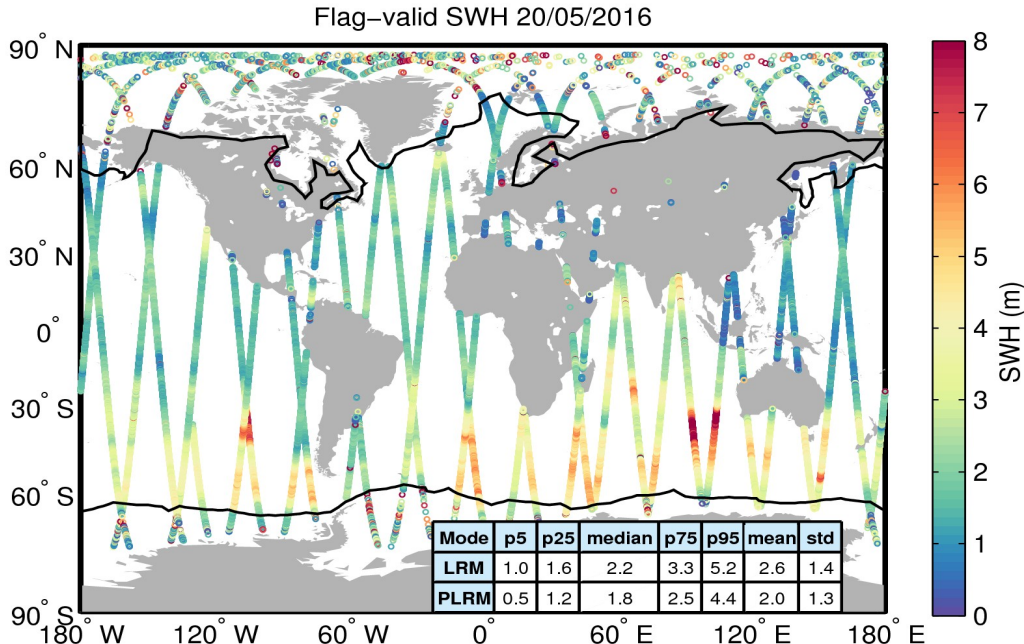
Figure 15. Geographical distribution of flag-valid SWH data over oceans and lakes for 20/05/2016. The statistical values shown in the table refer to the SWH in m and are calculated separately for LRM and PLRM regions. Measurements taken over polar polygons have been excluded from the computation of the statistical values. The black lines mark the outer limit of the Arctic and Antarctic polar polygons.
