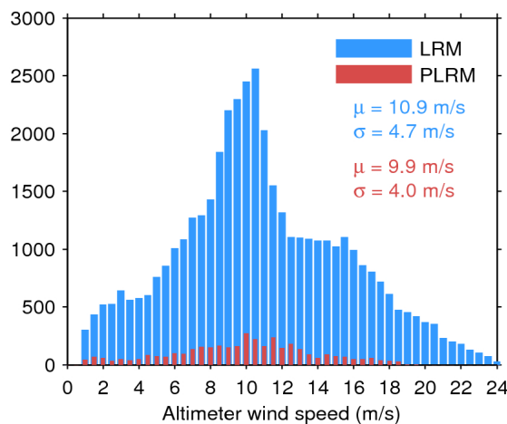
Figure 35. Histogram of science-valid wind over oceans and lakes for LRM (blue) and PLRM (red) for 20/05/2016. The mean ( \mu ) and standard deviation ( \sigma ) are also shown. Note that values larger than 24 m/s are excluded from the histogram for the sake of readability but not from the computation of \mu and \sigma .
