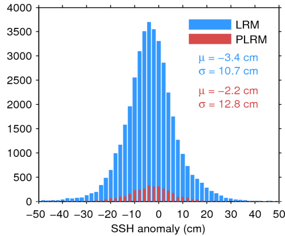
Figure 11. Histogram of science-valid SSH anomaly over oceans and lakes for LRM (blue) and PLRM (red) for 20/05/2016. The mean ( \mu ) and standard deviation ( \sigma ) are also shown. Note that values outside [-50 50] cm are excluded from the histogram for the sake of readability but not from the computation of \mu and \sigma .
