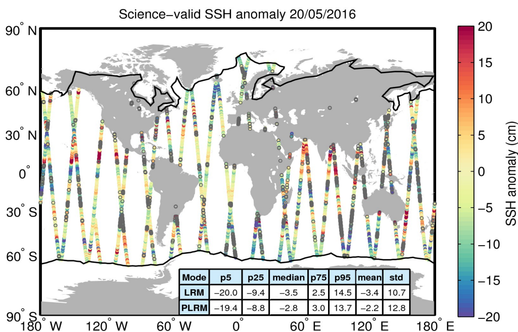
Figure 10. Geographical distribution of science-valid SSH anomaly data over oceans and lakes for 20/05/2016. The statistical values shown in the table refer to the SSH anomaly in cm and are calculated separately for LRM and PLRM regions. The black lines mark the outer limit of the Arctic and Antarctic polar polygons. Gray circles denote records that have been rejected based on the editing criteria described in Table 2.
