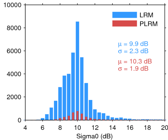
Figure 25. Histogram of flag-valid sigma0 over oceans and lakes for LRM (blue) and PLRM (red) for 20/05/2016. The mean ( \mu ) and standard deviation ( \sigma ) are also shown. Note that values outside [4 20] dB are excluded from the histogram for the sake of readability but not from the computation of \mu and \sigma .
