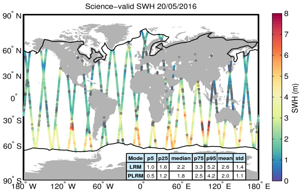
Figure 19. Geographical distribution of science-valid SWH data over oceans and lakes for 20/05/2016. The statistical values shown in the table refer to the SWH in m and are calculated separately for LRM and PLRM regions. The black lines mark the outer limit of the Arctic and Antarctic polar polygons. Gray circles denote records that have been rejected based on the editing criteria described in Table 3.
