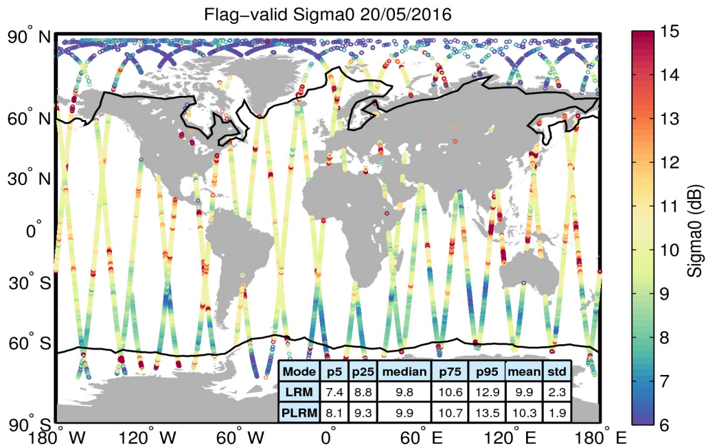
Figure 23. Geographical distribution of flag-valid sigma0 data over oceans and lakes for 20/05/2016. The statistical values shown in the table refer to the sigma0 in dB and are calculated separately for LRM and PLRM regions. Measurements taken over polar polygons have been excluded from the computation of the statistical values. The black lines mark the outer limit of the Arctic and Antarctic polar polygons.
