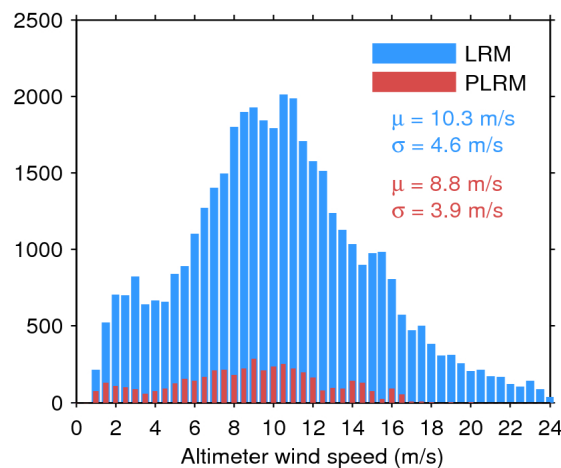
Figure 35. Histogram of science-valid wind over oceans and lakes for LRM (blue) and PLRM (red) for 17/05/2016. The mean ( \mu ) and standard deviation ( \sigma ) are also shown. Note that values larger than 24 m/s are excluded from the histogram for the sake of readability but not from the computation of \mu and \sigma .
