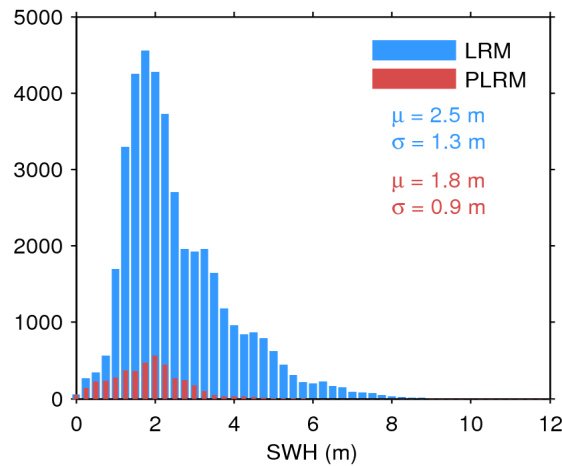
Figure 20. Histogram of science-valid SWH over oceans and lakes for LRM (blue) and PLRM (red) for 17/05/2016. The mean ( \mu ) and standard deviation ( \sigma ) are also shown. Note that values larger than 12 m are excluded from the histogram for the sake of readability but not from the computation of \mu and \sigma .
