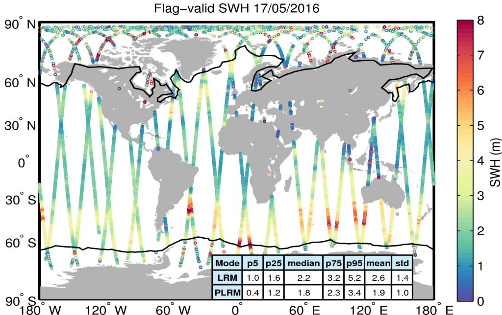
Figure 15. Geographical distribution of flag-valid SWH data over oceans and lakes for 17/05/2016. The statistical values shown in the table refer to the SWH in m and are calculated separately for LRM and PLRM regions. Measurements taken over polar polygons have been excluded from the computation of the statistical values. The black lines mark the outer limit of the Arctic and Antarctic polar polygons.
