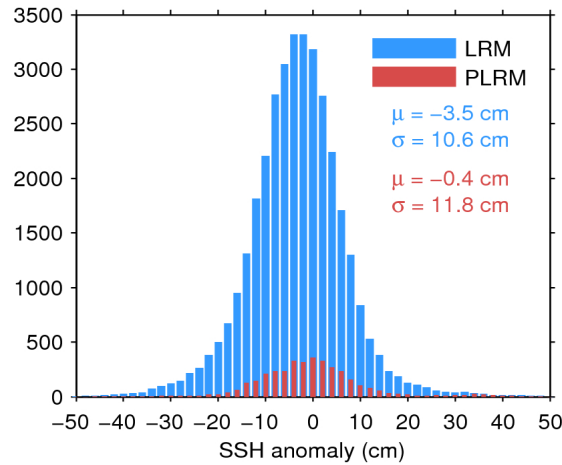
Figure 11. Histogram of science-valid SSH anomaly over oceans and lakes for LRM (blue) and PLRM (red) for 17/05/2016. The mean ( \mu ) and standard deviation ( \sigma ) are also shown. Note that values outside [-50 50] cm are excluded from the histogram for the sake of readability but not from the computation of \mu and \sigma .
