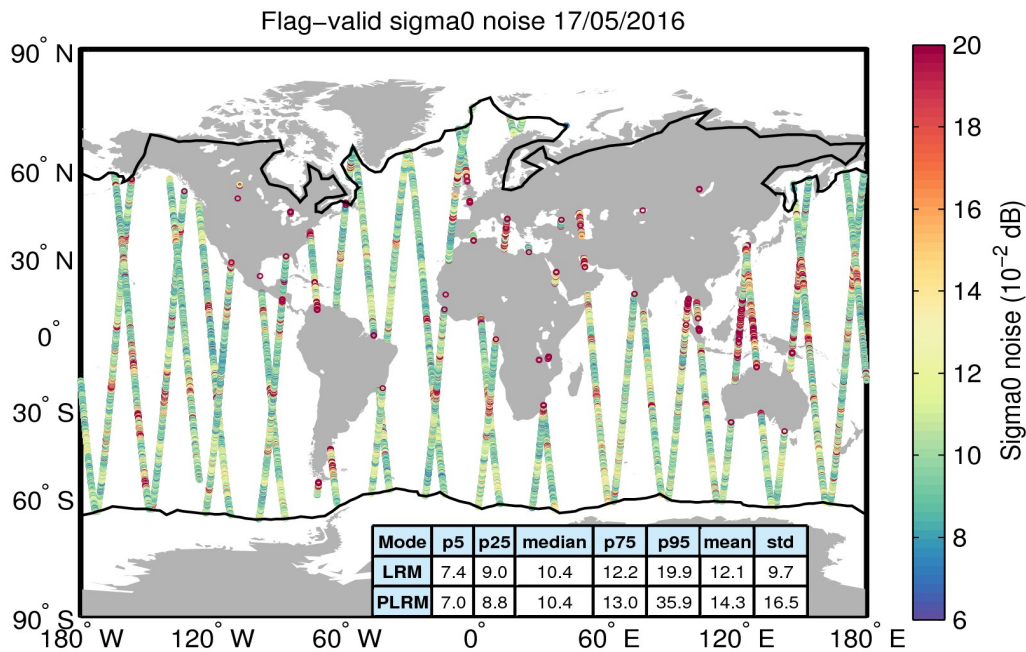
Figure 26. Geographical distribution of flag-valid 20-Hz sigma0 measurement noise over oceans and lakes for 17/05/2016. The statistical values shown in the table refer to the sigma0 noise and are calculated separately for LRM and PLRM regions. Measurements taken over polar polygons have been excluded from the computation of the statistical values. The black lines mark the outer limit of the Arctic and Antarctic polar polygons.
