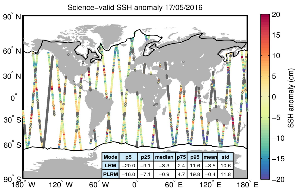
Figure 10. Geographical distribution of science-valid SSH anomaly data over oceans and lakes for 17/05/2016. The statistical values shown in the table refer to the SSH anomaly in cm and are calculated separately for LRM and PLRM regions. The black lines mark the outer limit of the Arctic and Antarctic polar polygons. Gray circles denote records that have been rejected based on the editing criteria described in Table 2.
