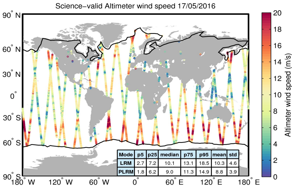
Figure 34. Geographical distribution of science-valid wind data over oceans and lakes for 17/05/2016. The statistical values shown in the table refer to the wind in m/s and are calculated separately for LRM and PLRM regions. The black lines mark the outer limit of the Arctic and Antarctic polar polygons. Gray circles denote records that have been rejected based on the editing criteria described in Table 5.
