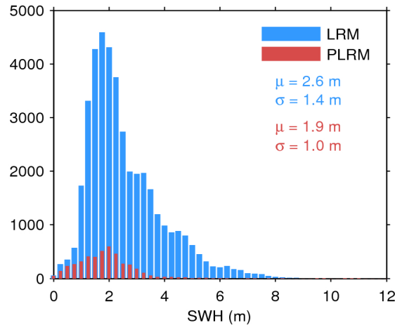
Figure 17. Histogram of flag-valid SWH over oceans and lakes for LRM (blue) and PLRM (red) for 17/05/2016. The mean ( \mu ) and standard deviation ( \sigma ) are also shown. Note that values larger than 12 m are excluded from the histogram for the sake of readability but not from the computation of \mu and \sigma .
