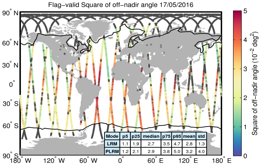
Figure 37. Geographical distribution of flag-valid mispointing data over oceans and lakes for 17/05/2016. The statistical values shown in the table refer to the mispointing in 10^{-2} deg 2 and are calculated separately for LRM and PLRM regions. Measurements taken over polar polygons have been excluded from the computation of the statistical values. The black lines mark the outer limit of the Arctic and Antarctic polar polygons. Gray circles denote negative values.
