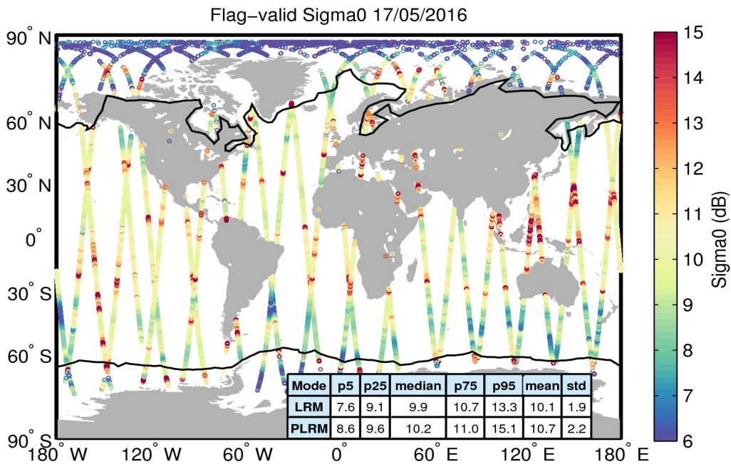
Figure 23. Geographical distribution of flag-valid sigma0 data over oceans and lakes for 17/05/2016. The statistical values shown in the table refer to the sigma0 in dB and are calculated separately for LRM and PLRM regions. Measurements taken over polar polygons have been excluded from the computation of the statistical values. The black lines mark the outer limit of the Arctic and Antarctic polar polygons.
