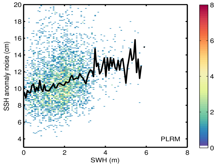
Figure 9. 2D histogram showing flag-valid SSH anomaly noise as a function of SWH for LRM (top) and PLRM (bottom) for 17/05/2016. The black line denotes the median SSH anomaly noise as a function of SWH.
