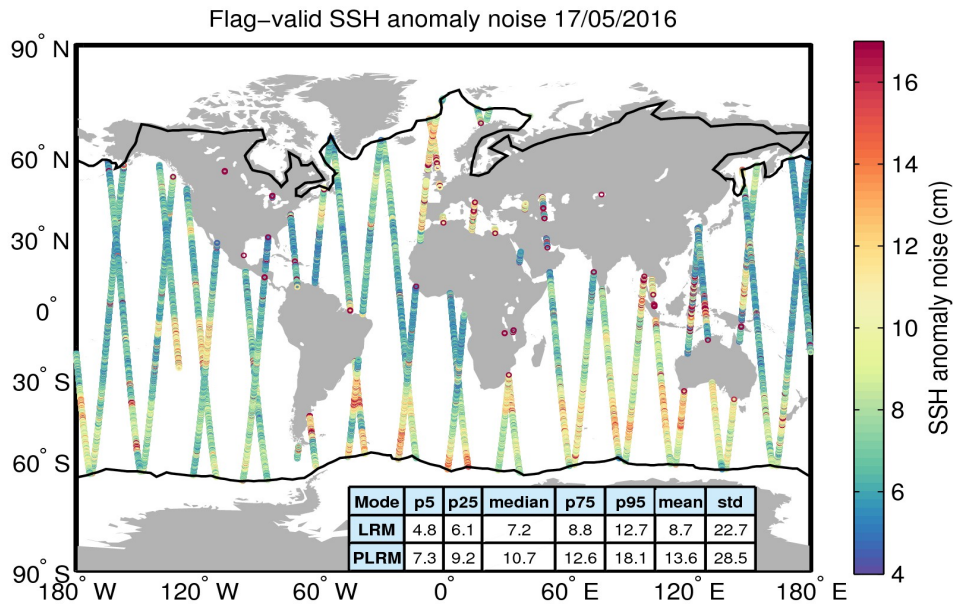
Figure 8. Geographical distribution of flag-valid 20-Hz SSH anomaly measurement noise over oceans and lakes for 17/05/2016. The statistical values shown in the table refer to the SSH anomaly noise and are calculated separately for LRM and PLRM regions. Measurements taken over polar polygons have been excluded from the computation of the statistical values. The black lines mark the outer limit of the Arctic and Antarctic polar polygons.
