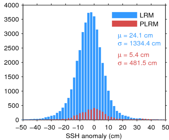
Figure 7. Histogram of flag-valid SSH anomaly over oceans and lakes for LRM (blue) and PLRM (red) for 17/05/2016. The mean ( \mu ) and standard deviation ( \sigma ) are also shown. Note that values outside [-50\ 50] cm are excluded from the histogram for the sake of readability but not from the computation of \mu and \sigma .
