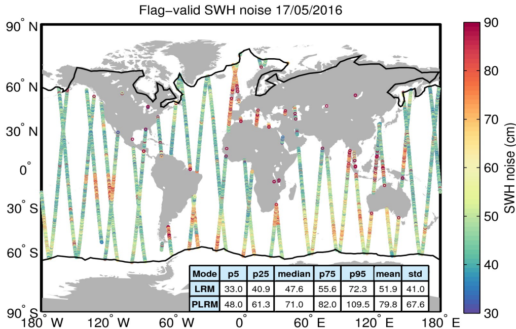
Figure 18. Geographical distribution of flag-valid 20-Hz SWH measurement noise over oceans and lakes for 17/05/2016. The statistical values shown in the table refer to the SWH noise and are calculated separately for LRM and PLRM regions. Measurements taken over polar polygons have been excluded from the computation of the statistical values. The black lines mark the outer limit of the Arctic and Antarctic polar polygons.
