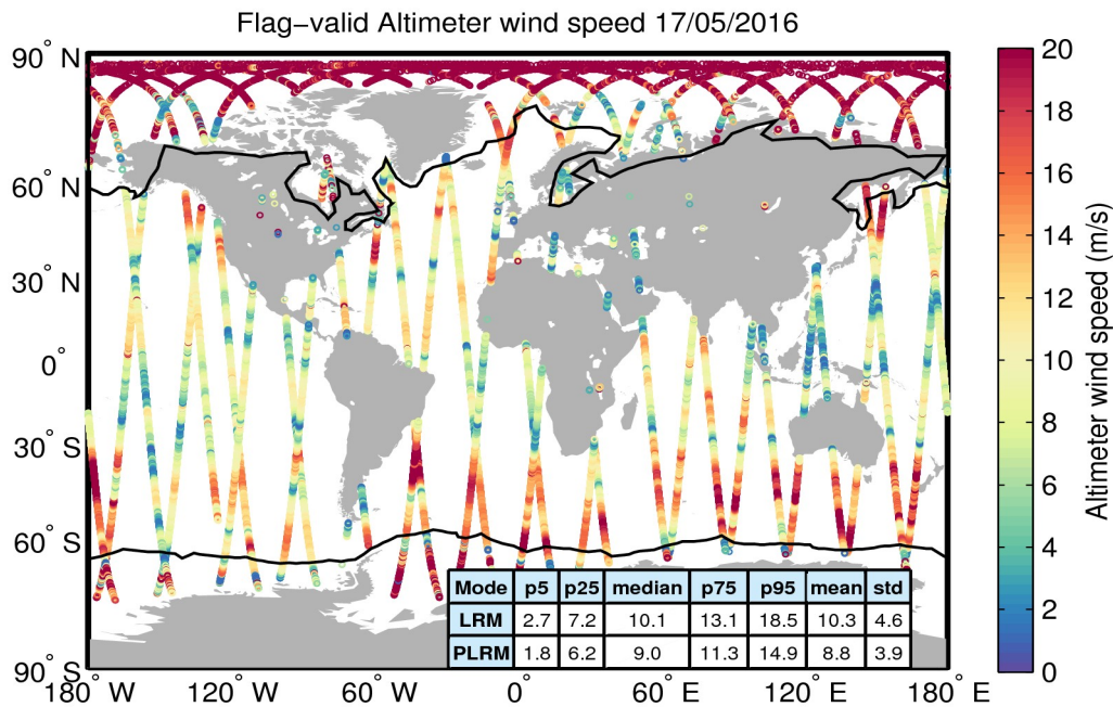
Figure 31. Geographical distribution of flag-valid wind data over oceans and lakes for 17/05/2016. The statistical values shown in the table refer to the wind in m/s and are calculated separately for LRM and PLRM regions. Measurements taken over polar polygons have been excluded from the computation of the statistical values. The black lines mark the outer limit of the Arctic and Antarctic polar polygons.
