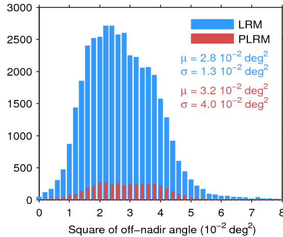
Figure 39. Histogram of flag-valid mispointing over oceans and lakes for LRM (blue) and PLRM (red) for 17/05/2016. Only positive values have been considered. The mean ( \mu ) and standard deviation ( \sigma ) are also shown. Note that values larger than 8 \cdot 10^{-2} \text{ deg}^2 are excluded from the histogram for the sake of readability but not from the computation of \mu and \sigma .
