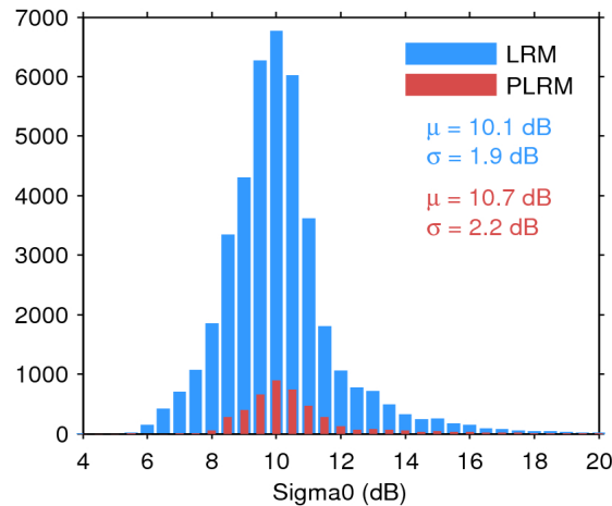
Figure 25. Histogram of flag-valid sigma0 over oceans and lakes for LRM (blue) and PLRM (red) for 17/05/2016. The mean ( \mu ) and standard deviation ( \sigma ) are also shown. Note that values outside [4 20] dB are excluded from the histogram for the sake of readability but not from the computation of \mu and \sigma .
