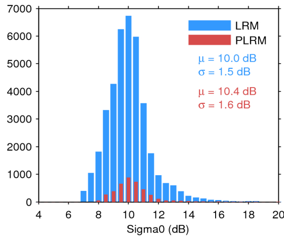
Figure 28. Histogram of science-valid sigma0 over oceans and lakes for LRM (blue) and PLRM (red) for 17/05/2016. The mean ( \mu ) and standard deviation ( \sigma ) are also shown. Note that values outside [4 20] dB are excluded from the histogram for the sake of readability but not from the computation of \mu and \sigma .
