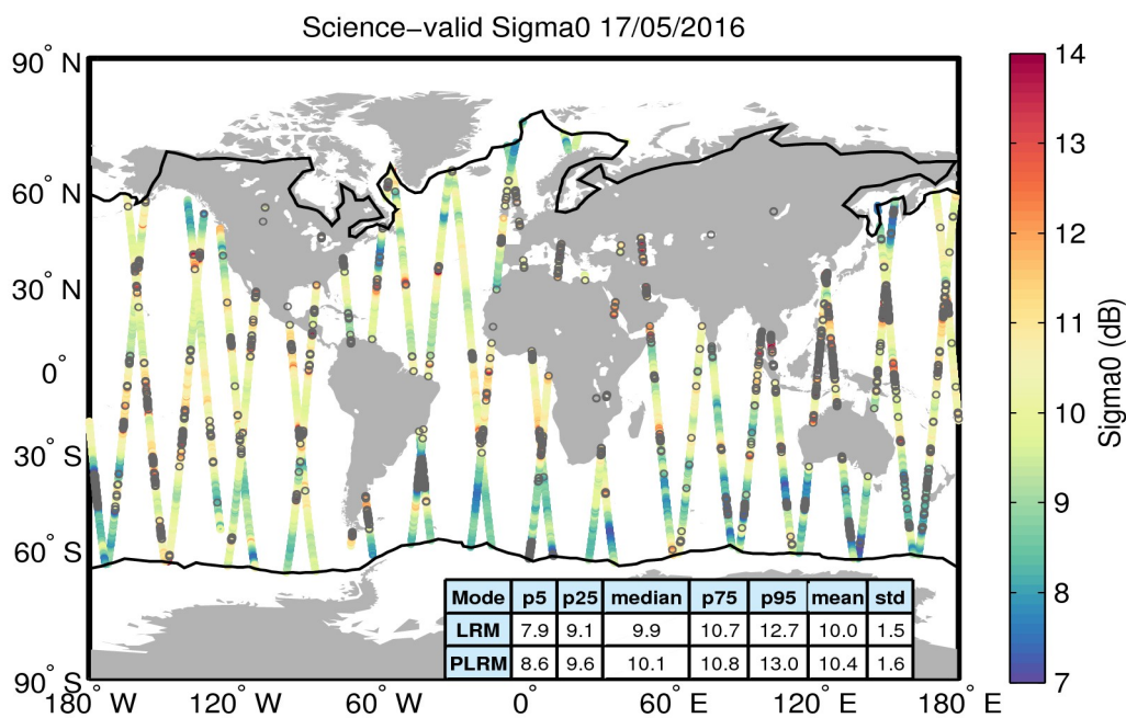
Figure 27. Geographical distribution of science-valid sigma0 data over oceans and lakes for 17/05/2016. The statistical values shown in the table refer to the sigma0 in dB and are calculated separately for LRM and PLRM regions. The black lines mark the outer limit of the Arctic and Antarctic polar polygons. Gray circles denote records that have been rejected based on the editing criteria described in Table 4.
