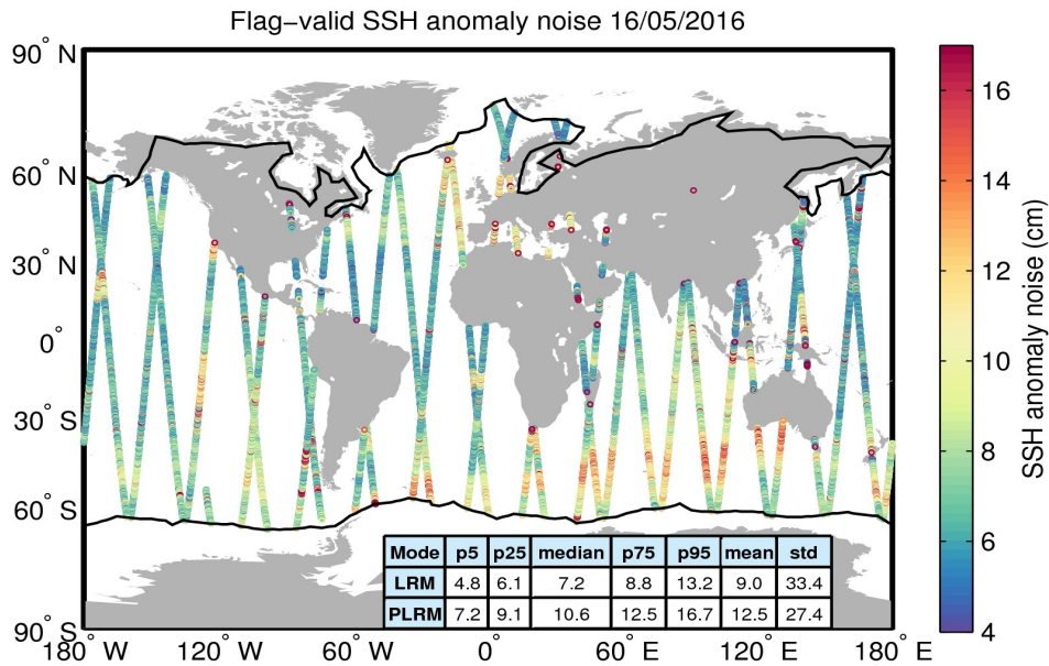
Figure 8. Geographical distribution of flag-valid 20-Hz SSH anomaly measurement noise over oceans and lakes for 16/05/2016. The statistical values shown in the table refer to the SSH anomaly noise and are calculated separately for LRM and PLRM regions. Measurements taken over polar polygons have been excluded from the computation of the statistical values. The black lines mark the outer limit of the Arctic and Antarctic polar polygons.
