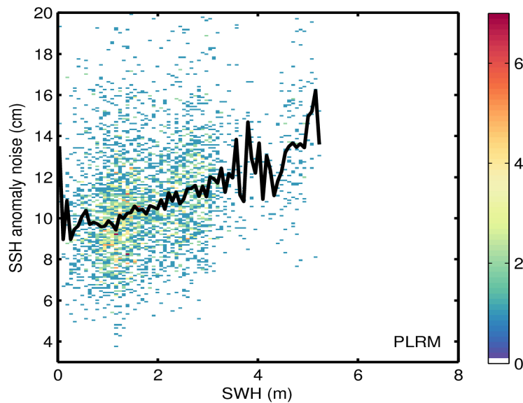
Figure 9. 2D histogram showing flag-valid SSH anomaly noise as a function of SWH for LRM (top) and PLRM (bottom) for 16/05/2016. The black line denotes the median SSH anomaly noise as a function of SWH.
