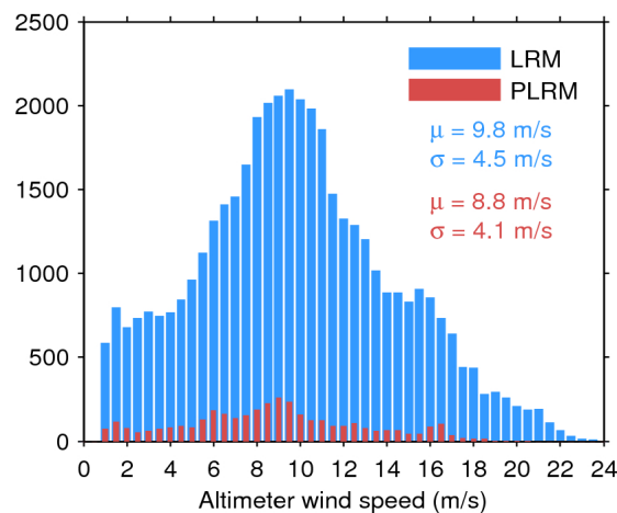
Figure 35. Histogram of science-valid wind over oceans and lakes for LRM (blue) and PLRM (red) for 16/05/2016. The mean ( \mu ) and standard deviation ( \sigma ) are also shown. Note that values larger than 24 m/s are excluded from the histogram for the sake of readability but not from the computation of \mu and \sigma .
