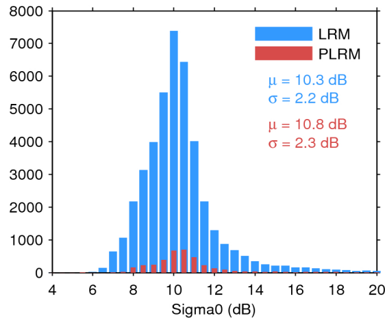
Figure 25. Histogram of flag-valid sigma0 over oceans and lakes for LRM (blue) and PLRM (red) for 16/05/2016. The mean ( \mu ) and standard deviation ( \sigma ) are also shown. Note that values outside [4 20] dB are excluded from the histogram for the sake of readability but not from the computation of \mu and \sigma .
