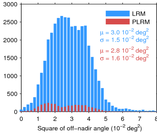
Figure 39. Histogram of flag-valid mispointing over oceans and lakes for LRM (blue) and PLRM (red) for 16/05/2016. Only positive values have been considered. The mean ( \mu ) and standard deviation ( \sigma ) are also shown. Note that values larger than 8 \cdot 10^{-2} \text{ deg}^2 are excluded from the histogram for the sake of readability but not from the computation of \mu and \sigma .
