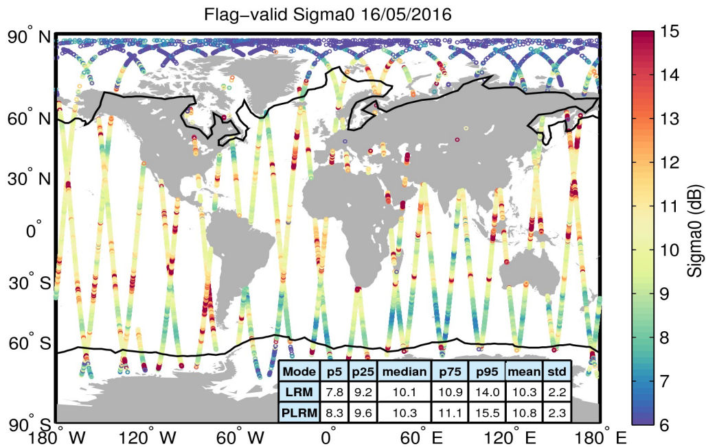
Figure 23. Geographical distribution of flag-valid sigma0 data over oceans and lakes for 16/05/2016. The statistical values shown in the table refer to the sigma0 in dB and are calculated separately for LRM and PLRM regions. Measurements taken over polar polygons have been excluded from the computation of the statistical values. The black lines mark the outer limit of the Arctic and Antarctic polar polygons.
