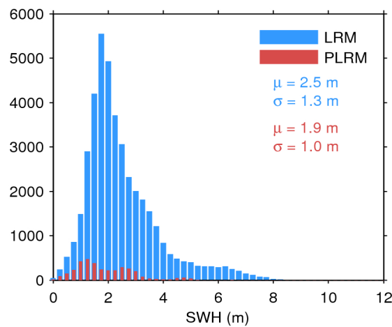
Figure 20. Histogram of science-valid SWH over oceans and lakes for LRM (blue) and PLRM (red) for 16/05/2016. The mean ( \mu ) and standard deviation ( \sigma ) are also shown. Note that values larger than 12 m are excluded from the histogram for the sake of readability but not from the computation of \mu and \sigma .
