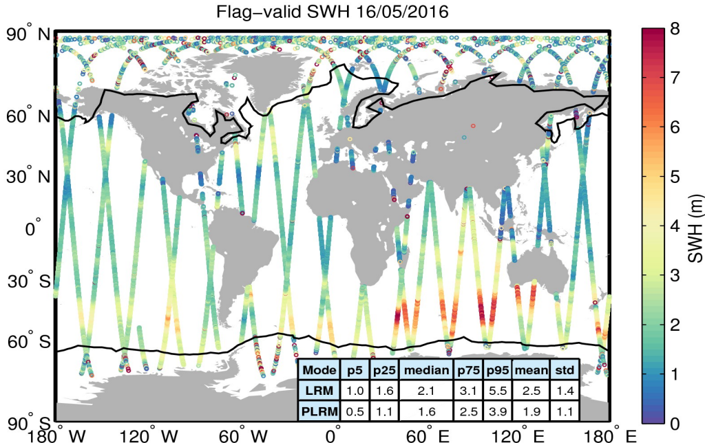
Figure 15. Geographical distribution of flag-valid SWH data over oceans and lakes for 16/05/2016. The statistical values shown in the table refer to the SWH in m and are calculated separately for LRM and PLRM regions. Measurements taken over polar polygons have been excluded from the computation of the statistical values. The black lines mark the outer limit of the Arctic and Antarctic polar polygons.
