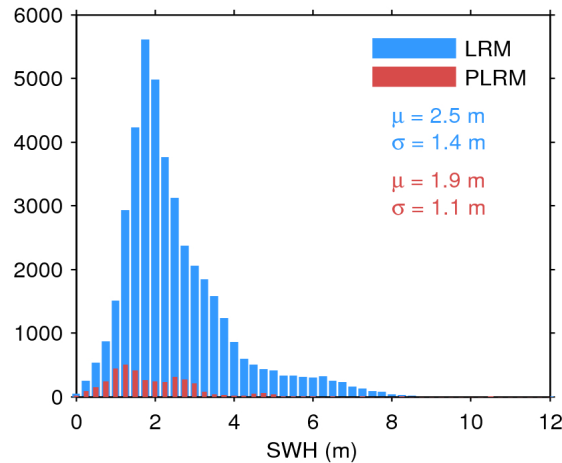
Figure 17. Histogram of flag-valid SWH over oceans and lakes for LRM (blue) and PLRM (red) for 16/05/2016. The mean ( \mu ) and standard deviation ( \sigma ) are also shown. Note that values larger than 12 m are excluded from the histogram for the sake of readability but not from the computation of \mu and \sigma .
