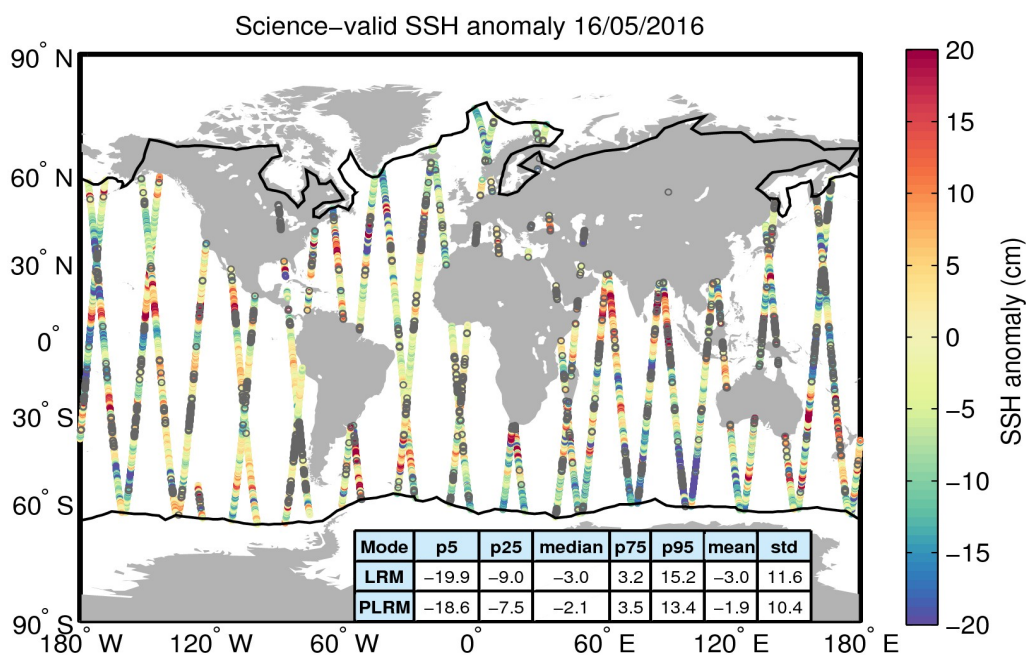
Figure 10. Geographical distribution of science-valid SSH anomaly data over oceans and lakes for 16/05/2016. The statistical values shown in the table refer to the SSH anomaly in cm and are calculated separately for LRM and PLRM regions. The black lines mark the outer limit of the Arctic and Antarctic polar polygons. Gray circles denote records that have been rejected based on the editing criteria described in Table 2.
