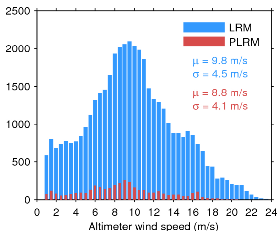
Figure 33. Histogram of flag-valid wind over oceans and lakes for LRM (blue) and PLRM (red) for 16/05/2016. The mean ( \mu ) and standard deviation ( \sigma ) are also shown. Note that values larger than 24 m/s are excluded from the histogram for the sake of readability but not from the computation of \mu and \sigma .
