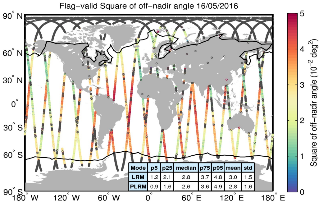
Figure 37. Geographical distribution of flag-valid mispointing data over oceans and lakes for 16/05/2016. The statistical values shown in the table refer to the mispointing in 10^{-2} deg 2 and are calculated separately for LRM and PLRM regions. Measurements taken over polar polygons have been excluded from the computation of the statistical values. The black lines mark the outer limit of the Arctic and Antarctic polar polygons. Gray circles denote negative values.
