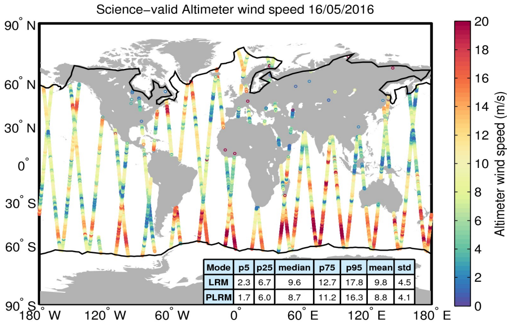
Figure 34. Geographical distribution of science-valid wind data over oceans and lakes for 16/05/2016. The statistical values shown in the table refer to the wind in m/s and are calculated separately for LRM and PLRM regions. The black lines mark the outer limit of the Arctic and Antarctic polar polygons. Gray circles denote records that have been rejected based on the editing criteria described in Table 5.
