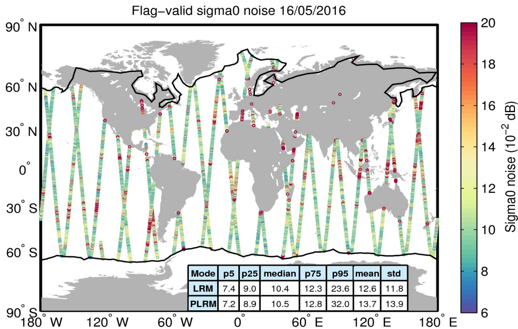
Figure 26. Geographical distribution of flag-valid 20-Hz sigma0 measurement noise over oceans and lakes for 16/05/2016. The statistical values shown in the table refer to the sigma0 noise and are calculated separately for LRM and PLRM regions. Measurements taken over polar polygons have been excluded from the computation of the statistical values. The black lines mark the outer limit of the Arctic and Antarctic polar polygons.
