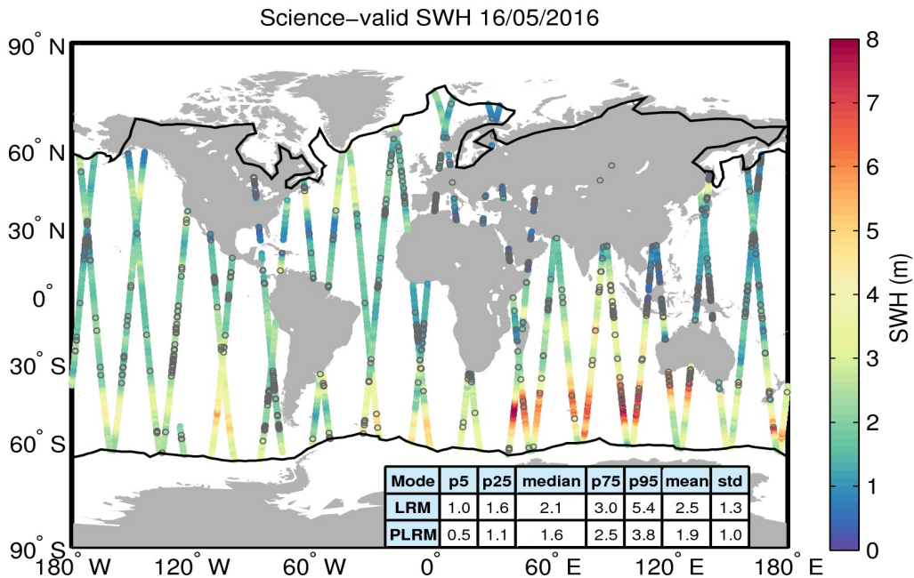
Figure 19. Geographical distribution of science-valid SWH data over oceans and lakes for 16/05/2016. The statistical values shown in the table refer to the SWH in m and are calculated separately for LRM and PLRM regions. The black lines mark the outer limit of the Arctic and Antarctic polar polygons. Gray circles denote records that have been rejected based on the editing criteria described in Table 3.
