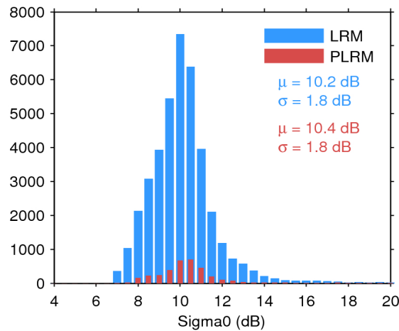
Figure 28. Histogram of science-valid sigma0 over oceans and lakes for LRM (blue) and PLRM (red) for 16/05/2016. The mean ( \mu ) and standard deviation ( \sigma ) are also shown. Note that values outside [4 20] dB are excluded from the histogram for the sake of readability but not from the computation of \mu and \sigma .
