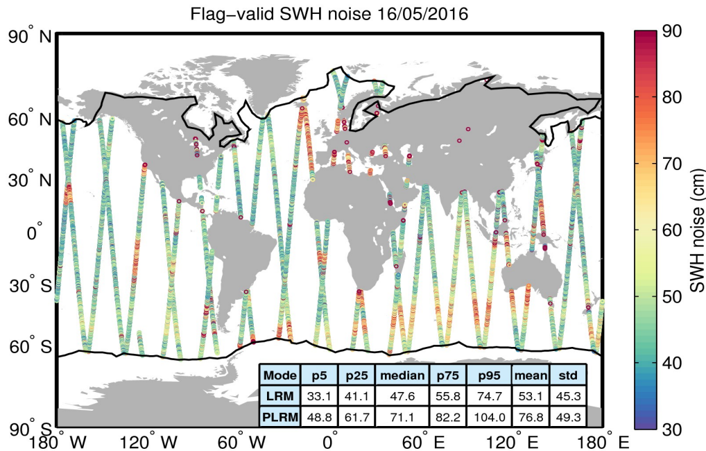
Figure 18. Geographical distribution of flag-valid 20-Hz SWH measurement noise over oceans and lakes for 16/05/2016. The statistical values shown in the table refer to the SWH noise and are calculated separately for LRM and PLRM regions. Measurements taken over polar polygons have been excluded from the computation of the statistical values. The black lines mark the outer limit of the Arctic and Antarctic polar polygons.
