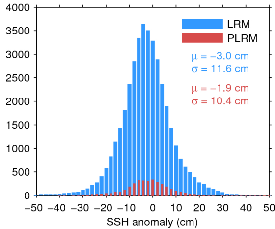
Figure 11. Histogram of science-valid SSH anomaly over oceans and lakes for LRM (blue) and PLRM (red) for 16/05/2016. The mean ( \mu ) and standard deviation ( \sigma ) are also shown. Note that values outside [-50 50] cm are excluded from the histogram for the sake of readability but not from the computation of \mu and \sigma .
