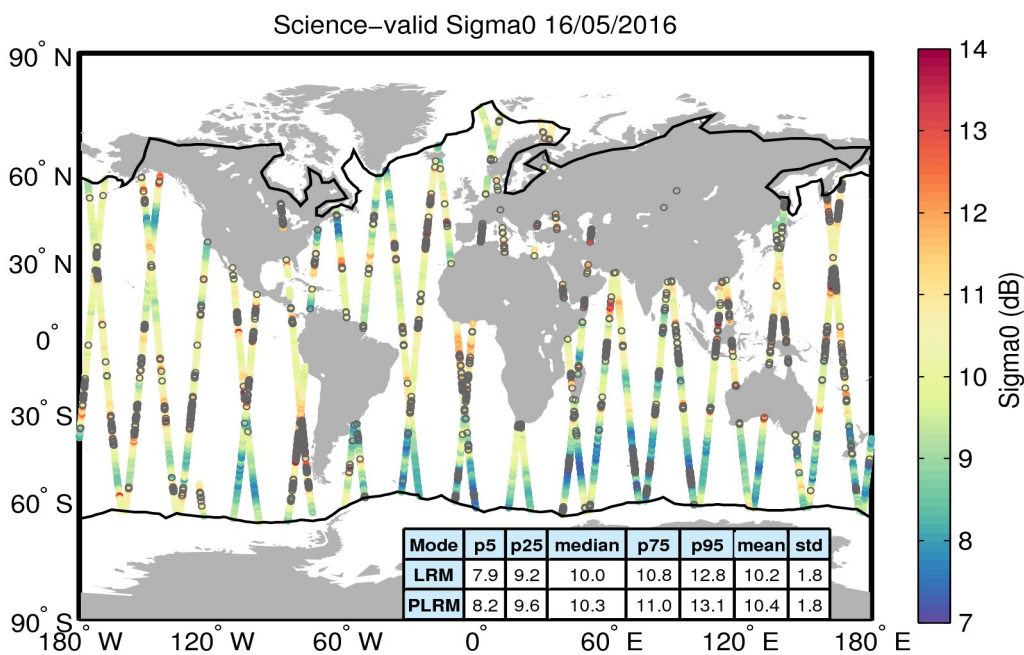
Figure 27. Geographical distribution of science-valid sigma0 data over oceans and lakes for 16/05/2016. The statistical values shown in the table refer to the sigma0 in dB and are calculated separately for LRM and PLRM regions. The black lines mark the outer limit of the Arctic and Antarctic polar polygons. Gray circles denote records that have been rejected based on the editing criteria described in Table 4.
