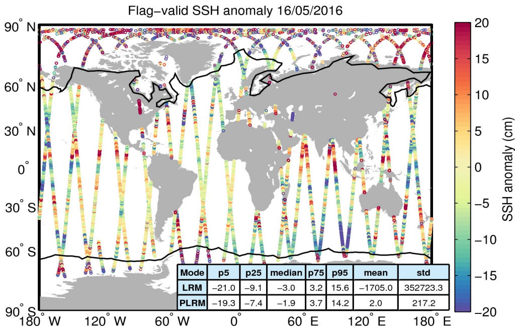
Figure 5. Geographical distribution of flag-valid 1-Hz SSH anomaly data over oceans and lakes for 16/05/2016. The statistical values shown in the table refer to the SSH anomaly in cm and are calculated separately for LRM and PLRM regions. Measurements taken over polar polygons have been excluded from the computation of the statistical values. The black lines mark the outer limit of the Arctic and Antarctic polar polygons.
