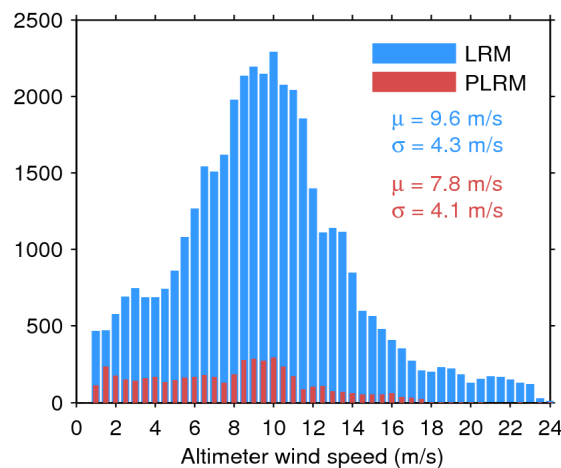
Figure 35. Histogram of science-valid wind over oceans and lakes for LRM (blue) and PLRM (red) for 15/05/2016. The mean ( \mu ) and standard deviation ( \sigma ) are also shown. Note that values larger than 24 m/s are excluded from the histogram for the sake of readability but not from the computation of \mu and \sigma .
