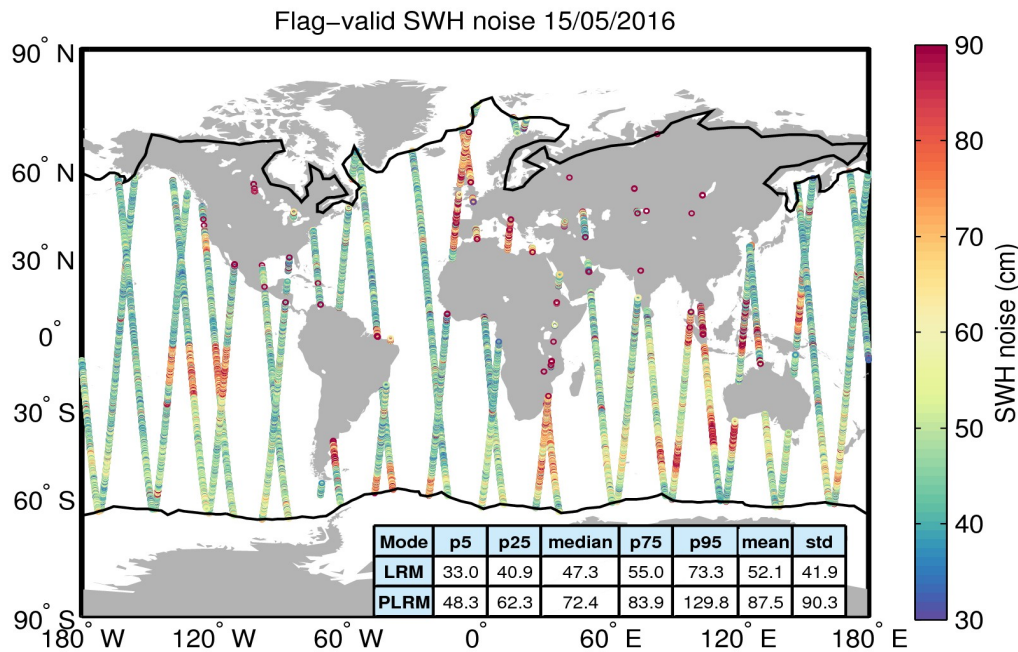
Figure 18. Geographical distribution of flag-valid 20-Hz SWH measurement noise over oceans and lakes for 15/05/2016. The statistical values shown in the table refer to the SWH noise and are calculated separately for LRM and PLRM regions. Measurements taken over polar polygons have been excluded from the computation of the statistical values. The black lines mark the outer limit of the Arctic and Antarctic polar polygons.
