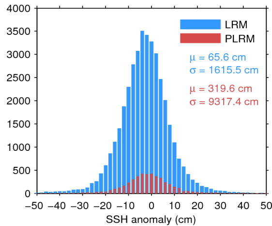
Figure 7. Histogram of flag-valid SSH anomaly over oceans and lakes for LRM (blue) and PLRM (red) for 15/05/2016. The mean ( \mu ) and standard deviation ( \sigma ) are also shown. Note that values outside [-50\ 50] cm are excluded from the histogram for the sake of readability but not from the computation of \mu and \sigma .
