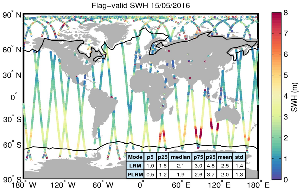
Figure 15. Geographical distribution of flag-valid SWH data over oceans and lakes for 15/05/2016. The statistical values shown in the table refer to the SWH in m and are calculated separately for LRM and PLRM regions. Measurements taken over polar polygons have been excluded from the computation of the statistical values. The black lines mark the outer limit of the Arctic and Antarctic polar polygons.
