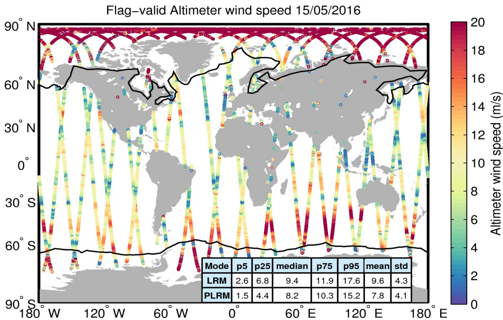
Figure 31. Geographical distribution of flag-valid wind data over oceans and lakes for 15/05/2016. The statistical values shown in the table refer to the wind in m/s and are calculated separately for LRM and PLRM regions. Measurements taken over polar polygons have been excluded from the computation of the statistical values. The black lines mark the outer limit of the Arctic and Antarctic polar polygons.
