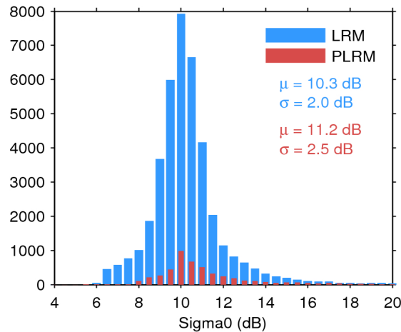
Figure 25. Histogram of flag-valid sigma0 over oceans and lakes for LRM (blue) and PLRM (red) for 15/05/2016. The mean ( \mu ) and standard deviation ( \sigma ) are also shown. Note that values outside [4 20] dB are excluded from the histogram for the sake of readability but not from the computation of \mu and \sigma .
