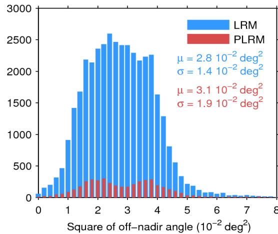
Figure 39. Histogram of flag-valid mispointing over oceans and lakes for LRM (blue) and PLRM (red) for 15/05/2016. Only positive values have been considered. The mean ( \mu ) and standard deviation ( \sigma ) are also shown. Note that values larger than 8 \cdot 10^{-2} \text{ deg}^2 are excluded from the histogram for the sake of readability but not from the computation of \mu and \sigma .
