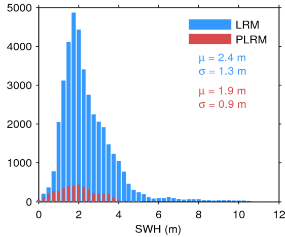
Figure 20. Histogram of science-valid SWH over oceans and lakes for LRM (blue) and PLRM (red) for 15/05/2016. The mean ( \mu ) and standard deviation ( \sigma ) are also shown. Note that values larger than 12 m are excluded from the histogram for the sake of readability but not from the computation of \mu and \sigma .
