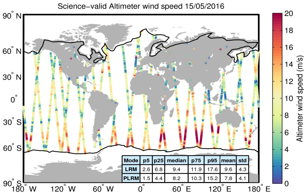
Figure 34. Geographical distribution of science-valid wind data over oceans and lakes for 15/05/2016. The statistical values shown in the table refer to the wind in m/s and are calculated separately for LRM and PLRM regions. The black lines mark the outer limit of the Arctic and Antarctic polar polygons. Gray circles denote records that have been rejected based on the editing criteria described in Table 5.
