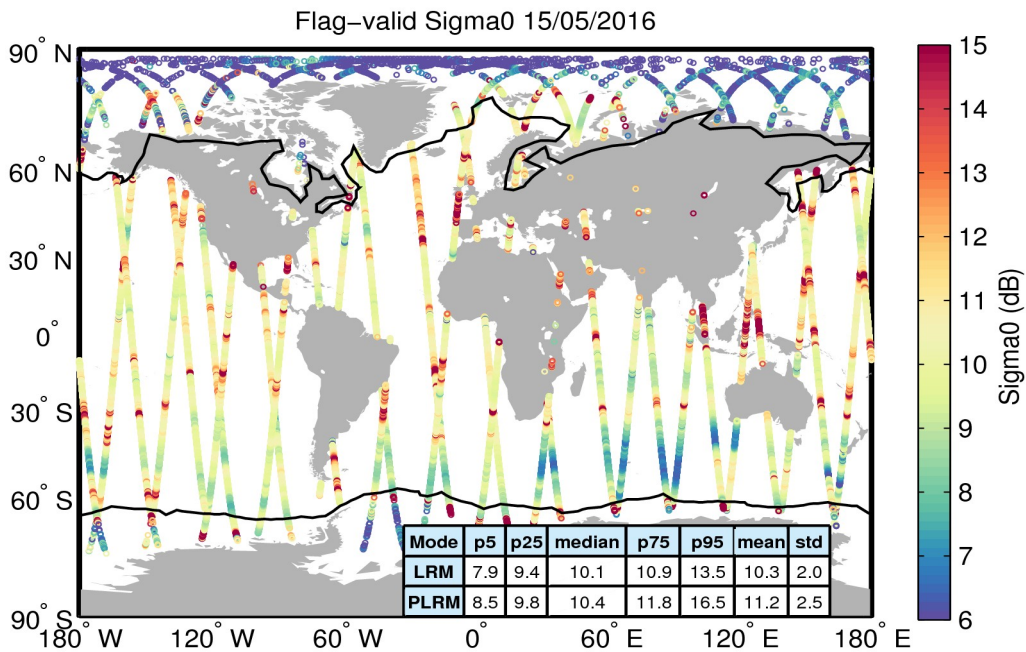
Figure 23. Geographical distribution of flag-valid sigma0 data over oceans and lakes for 15/05/2016. The statistical values shown in the table refer to the sigma0 in dB and are calculated separately for LRM and PLRM regions. Measurements taken over polar polygons have been excluded from the computation of the statistical values. The black lines mark the outer limit of the Arctic and Antarctic polar polygons.
