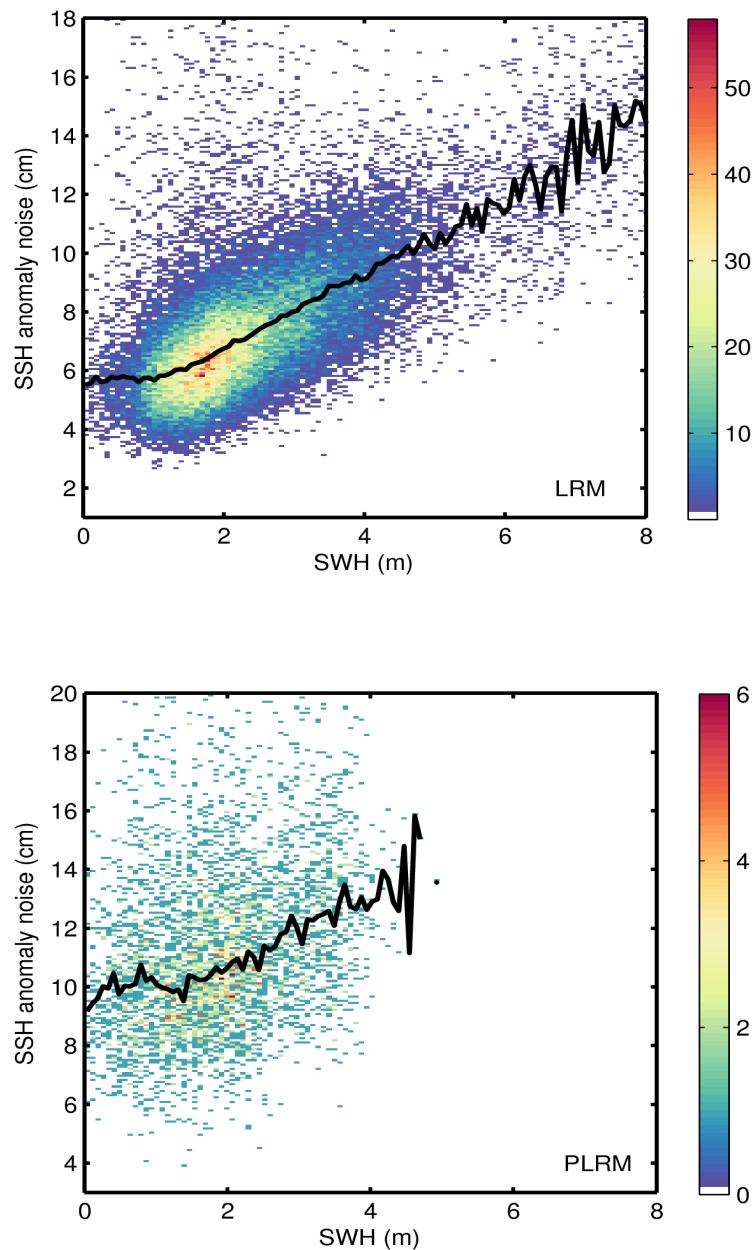
Figure 9. 2D histogram showing flag-valid SSH anomaly noise as a function of SWH for LRM (top) and PLRM (bottom) for 15/05/2016. The black line denotes the median SSH anomaly noise as a function of SWH.
