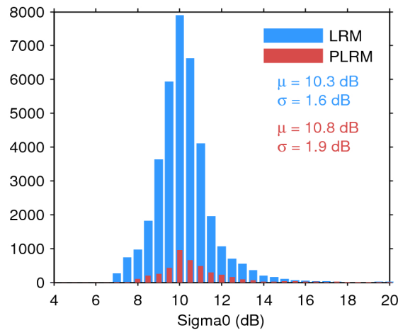
Figure 28. Histogram of science-valid sigma0 over oceans and lakes for LRM (blue) and PLRM (red) for 15/05/2016. The mean ( \mu ) and standard deviation ( \sigma ) are also shown. Note that values outside [4 20] dB are excluded from the histogram for the sake of readability but not from the computation of \mu and \sigma .
