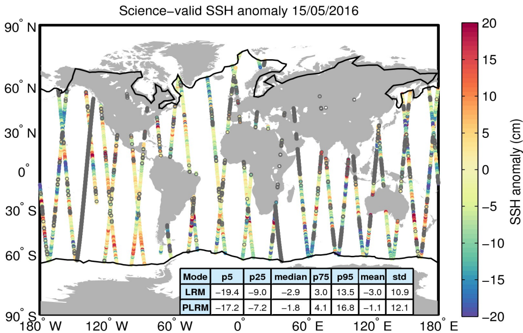
Figure 10. Geographical distribution of science-valid SSH anomaly data over oceans and lakes for 15/05/2016. The statistical values shown in the table refer to the SSH anomaly in cm and are calculated separately for LRM and PLRM regions. The black lines mark the outer limit of the Arctic and Antarctic polar polygons. Gray circles denote records that have been rejected based on the editing criteria described in Table 2.
