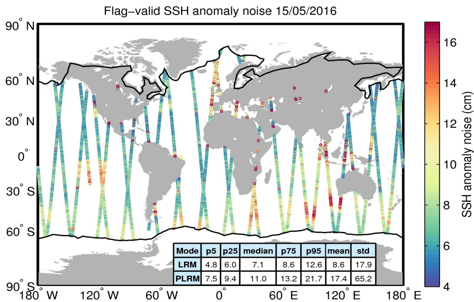
Figure 8. Geographical distribution of flag-valid 20-Hz SSH anomaly measurement noise over oceans and lakes for 15/05/2016. The statistical values shown in the table refer to the SSH anomaly noise and are calculated separately for LRM and PLRM regions. Measurements taken over polar polygons have been excluded from the computation of the statistical values. The black lines mark the outer limit of the Arctic and Antarctic polar polygons.
