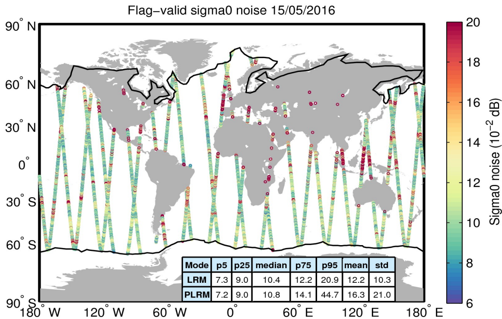
Figure 26. Geographical distribution of flag-valid 20-Hz sigma0 measurement noise over oceans and lakes for 15/05/2016. The statistical values shown in the table refer to the sigma0 noise and are calculated separately for LRM and PLRM regions. Measurements taken over polar polygons have been excluded from the computation of the statistical values. The black lines mark the outer limit of the Arctic and Antarctic polar polygons.
