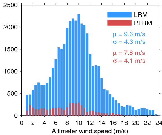
Figure 33. Histogram of flag-valid wind over oceans and lakes for LRM (blue) and PLRM (red) for 15/05/2016. The mean ( \mu ) and standard deviation ( \sigma ) are also shown. Note that values larger than 24 m/s are excluded from the histogram for the sake of readability but not from the computation of \mu and \sigma .
