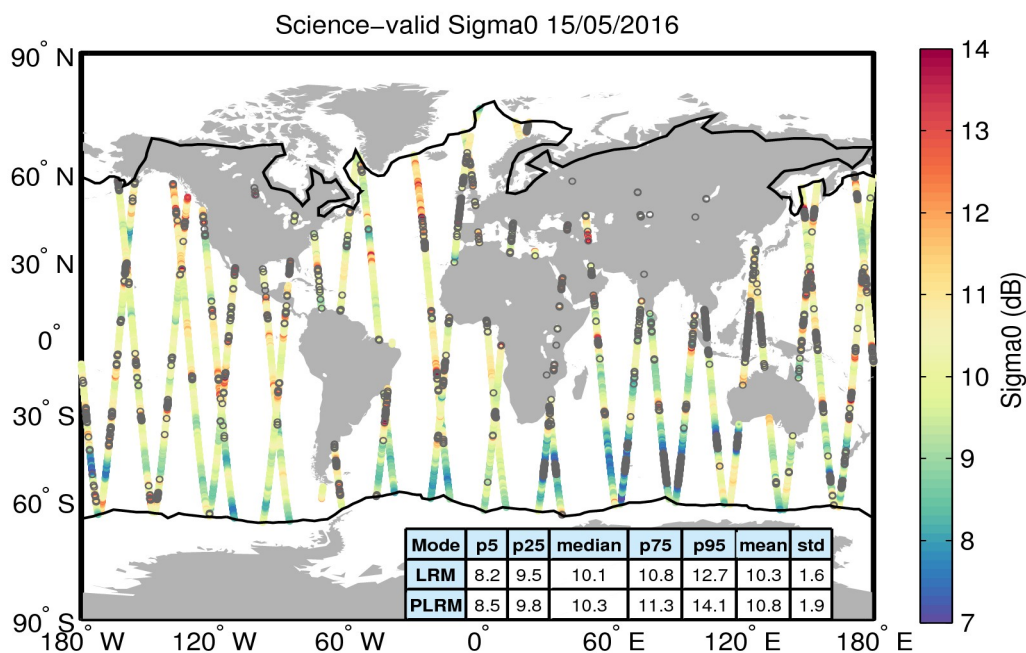
Figure 27. Geographical distribution of science-valid sigma0 data over oceans and lakes for 15/05/2016. The statistical values shown in the table refer to the sigma0 in dB and are calculated separately for LRM and PLRM regions. The black lines mark the outer limit of the Arctic and Antarctic polar polygons. Gray circles denote records that have been rejected based on the editing criteria described in Table 4.
