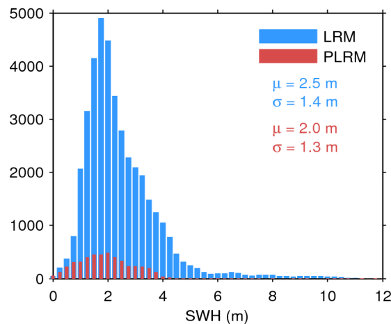
Figure 17. Histogram of flag-valid SWH over oceans and lakes for LRM (blue) and PLRM (red) for 15/05/2016. The mean ( \mu ) and standard deviation ( \sigma ) are also shown. Note that values larger than 12 m are excluded from the histogram for the sake of readability but not from the computation of \mu and \sigma .
