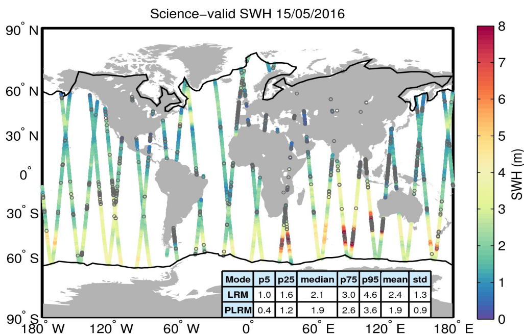
Figure 19. Geographical distribution of science-valid SWH data over oceans and lakes for 15/05/2016. The statistical values shown in the table refer to the SWH in m and are calculated separately for LRM and PLRM regions. The black lines mark the outer limit of the Arctic and Antarctic polar polygons. Gray circles denote records that have been rejected based on the editing criteria described in Table 3.
