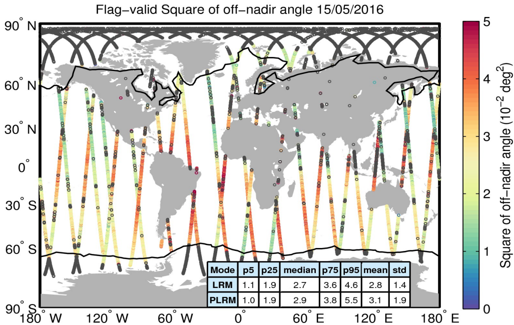
Figure 37. Geographical distribution of flag-valid mispointing data over oceans and lakes for 15/05/2016. The statistical values shown in the table refer to the mispointing in 10^{-2} deg 2 and are calculated separately for LRM and PLRM regions. Measurements taken over polar polygons have been excluded from the computation of the statistical values. The black lines mark the outer limit of the Arctic and Antarctic polar polygons. Gray circles denote negative values.
