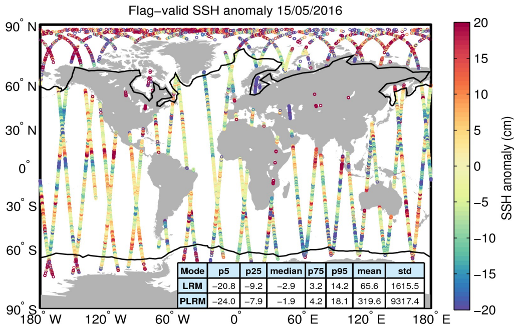
Figure 5. Geographical distribution of flag-valid 1-Hz SSH anomaly data over oceans and lakes for 15/05/2016. The statistical values shown in the table refer to the SSH anomaly in cm and are calculated separately for LRM and PLRM regions. Measurements taken over polar polygons have been excluded from the computation of the statistical values. The black lines mark the outer limit of the Arctic and Antarctic polar polygons.
