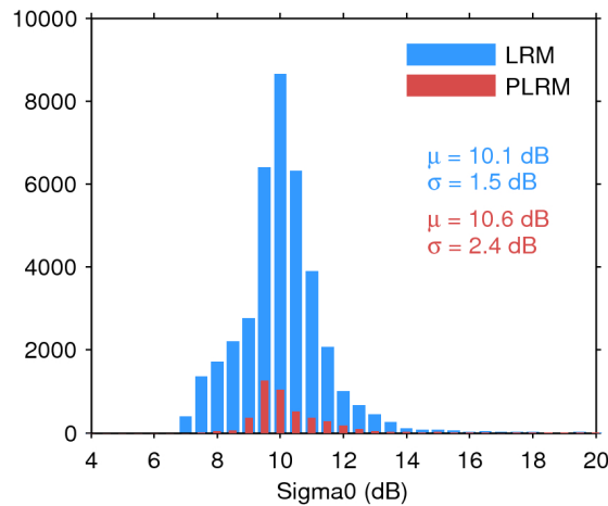
Figure 28. Histogram of science-valid sigma0 over oceans and lakes for LRM (blue) and PLRM (red) for 11/05/2016. The mean ( \mu ) and standard deviation ( \sigma ) are also shown. Note that values outside [4 20] dB are excluded from the histogram for the sake of readability but not from the computation of \mu and \sigma .
