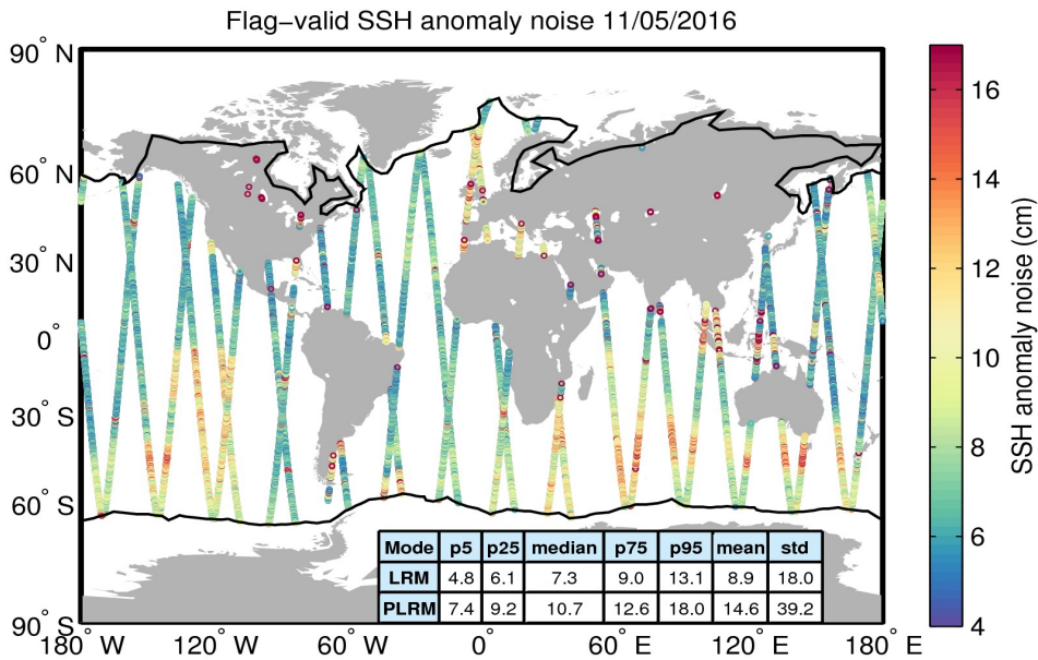
Figure 8. Geographical distribution of flag-valid 20-Hz SSH anomaly measurement noise over oceans and lakes for 11/05/2016. The statistical values shown in the table refer to the SSH anomaly noise and are calculated separately for LRM and PLRM regions. Measurements taken over polar polygons have been excluded from the computation of the statistical values. The black lines mark the outer limit of the Arctic and Antarctic polar polygons.
