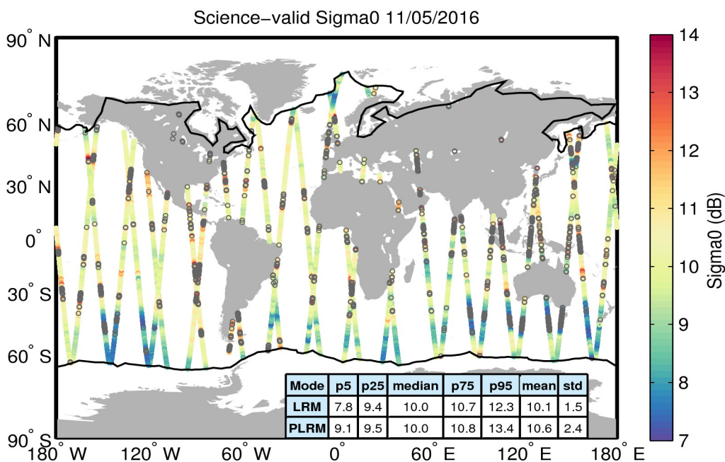
Figure 27. Geographical distribution of science-valid sigma0 data over oceans and lakes for 11/05/2016. The statistical values shown in the table refer to the sigma0 in dB and are calculated separately for LRM and PLRM regions. The black lines mark the outer limit of the Arctic and Antarctic polar polygons. Gray circles denote records that have been rejected based on the editing criteria described in Table 4.
