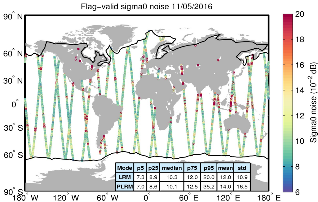
Figure 26. Geographical distribution of flag-valid 20-Hz sigma0 measurement noise over oceans and lakes for 11/05/2016. The statistical values shown in the table refer to the sigma0 noise and are calculated separately for LRM and PLRM regions. Measurements taken over polar polygons have been excluded from the computation of the statistical values. The black lines mark the outer limit of the Arctic and Antarctic polar polygons.
