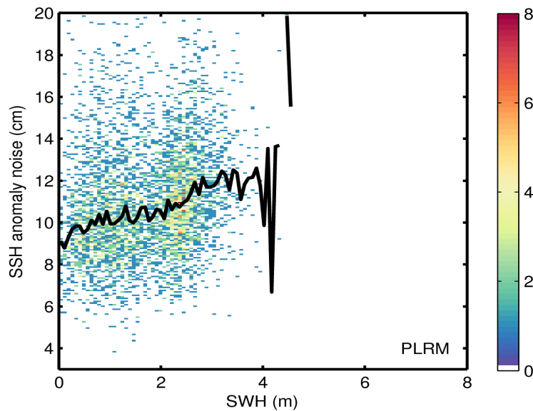
Figure 9. 2D histogram showing flag-valid SSH anomaly noise as a function of SWH for LRM (top) and PLRM (bottom) for 11/05/2016. The black line denotes the median SSH anomaly noise as a function of SWH.
