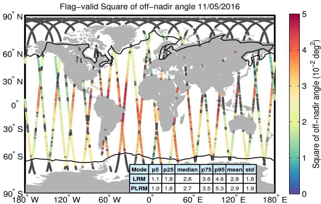
Figure 37. Geographical distribution of flag-valid mispointing data over oceans and lakes for 11/05/2016. The statistical values shown in the table refer to the mispointing in 10^{-2} deg 2 and are calculated separately for LRM and PLRM regions. Measurements taken over polar polygons have been excluded from the computation of the statistical values. The black lines mark the outer limit of the Arctic and Antarctic polar polygons. Gray circles denote negative values.
