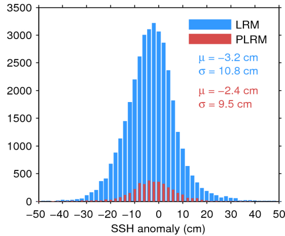
Figure 11. Histogram of science-valid SSH anomaly over oceans and lakes for LRM (blue) and PLRM (red) for 11/05/2016. The mean ( \mu ) and standard deviation ( \sigma ) are also shown. Note that values outside [-50 50] cm are excluded from the histogram for the sake of readability but not from the computation of \mu and \sigma .
