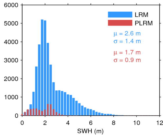
Figure 20. Histogram of science-valid SWH over oceans and lakes for LRM (blue) and PLRM (red) for 11/05/2016. The mean ( \mu ) and standard deviation ( \sigma ) are also shown. Note that values larger than 12 m are excluded from the histogram for the sake of readability but not from the computation of \mu and \sigma .
