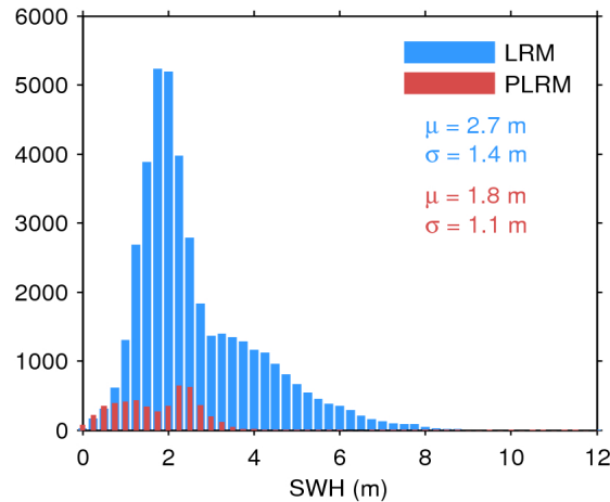
Figure 17. Histogram of flag-valid SWH over oceans and lakes for LRM (blue) and PLRM (red) for 11/05/2016. The mean ( \mu ) and standard deviation ( \sigma ) are also shown. Note that values larger than 12 m are excluded from the histogram for the sake of readability but not from the computation of \mu and \sigma .
