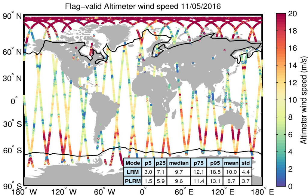
Figure 31. Geographical distribution of flag-valid wind data over oceans and lakes for 11/05/2016. The statistical values shown in the table refer to the wind in m/s and are calculated separately for LRM and PLRM regions. Measurements taken over polar polygons have been excluded from the computation of the statistical values. The black lines mark the outer limit of the Arctic and Antarctic polar polygons.
