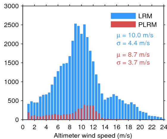
Figure 35. Histogram of science-valid wind over oceans and lakes for LRM (blue) and PLRM (red) for 11/05/2016. The mean ( \mu ) and standard deviation ( \sigma ) are also shown. Note that values larger than 24 m/s are excluded from the histogram for the sake of readability but not from the computation of \mu and \sigma .
