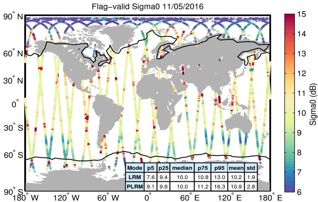
Figure 23. Geographical distribution of flag-valid sigma0 data over oceans and lakes for 11/05/2016. The statistical values shown in the table refer to the sigma0 in dB and are calculated separately for LRM and PLRM regions. Measurements taken over polar polygons have been excluded from the computation of the statistical values. The black lines mark the outer limit of the Arctic and Antarctic polar polygons.
