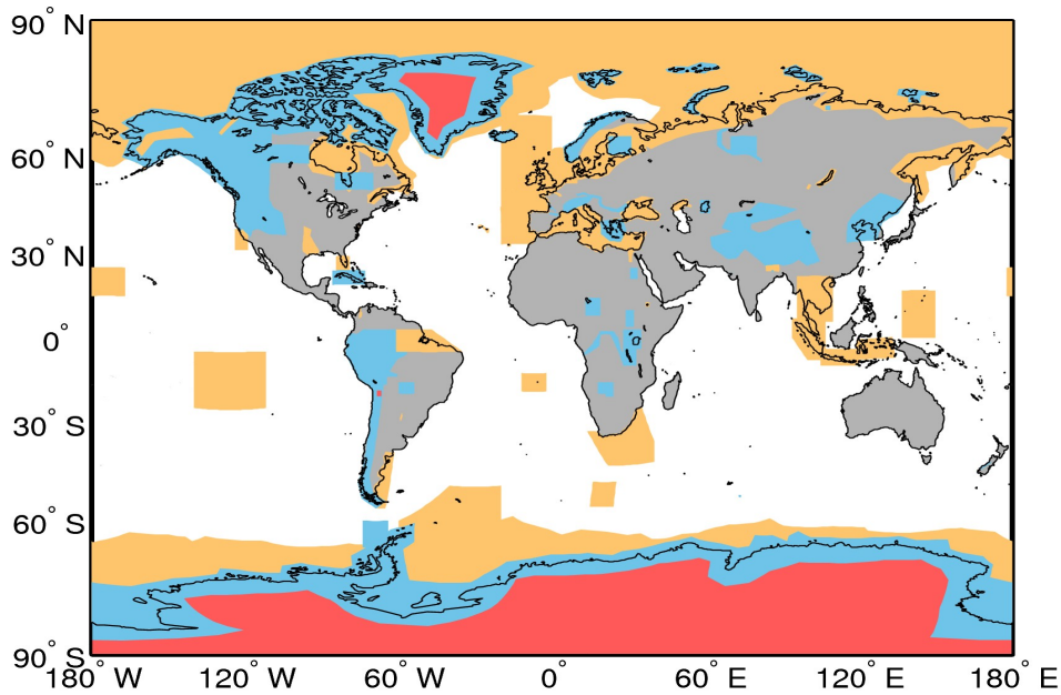
Figure A1. Extent of the regions defining the geographical mode mask for 11/05/2016. The regions where SAR, and SARIn are operated are denoted by the orange and blue polygons, respectively. LRM is operated over areas of the continental ice sheets (red polygons) and over oceans and land not covered by other modes.
