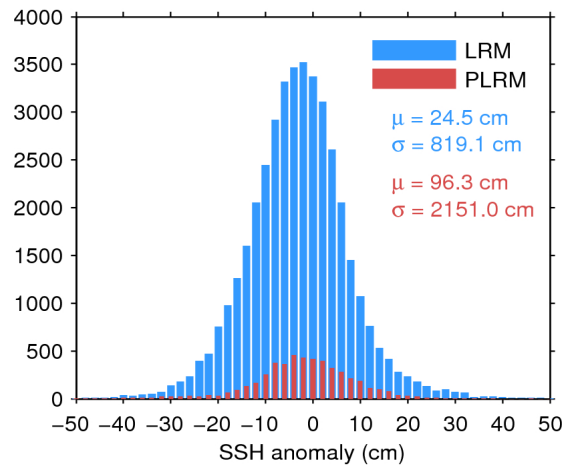
Figure 7. Histogram of flag-valid SSH anomaly over oceans and lakes for LRM (blue) and PLRM (red) for 11/05/2016. The mean ( \mu ) and standard deviation ( \sigma ) are also shown. Note that values outside [-50 50] cm are excluded from the histogram for the sake of readability but not from the computation of \mu and \sigma .
