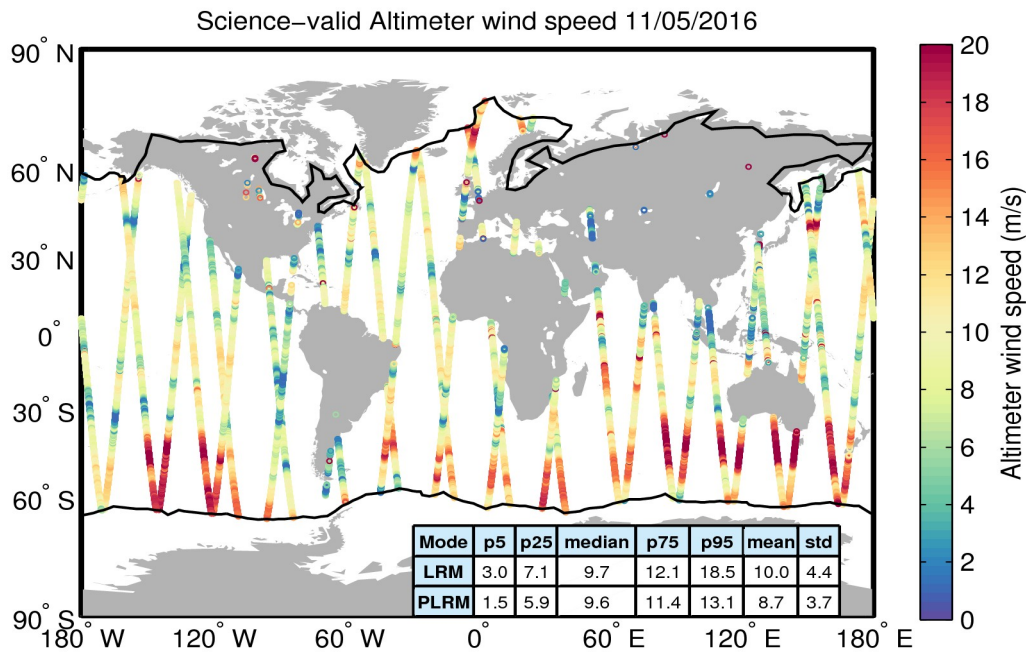
Figure 34. Geographical distribution of science-valid wind data over oceans and lakes for 11/05/2016. The statistical values shown in the table refer to the wind in m/s and are calculated separately for LRM and PLRM regions. The black lines mark the outer limit of the Arctic and Antarctic polar polygons. Gray circles denote records that have been rejected based on the editing criteria described in Table 5.
