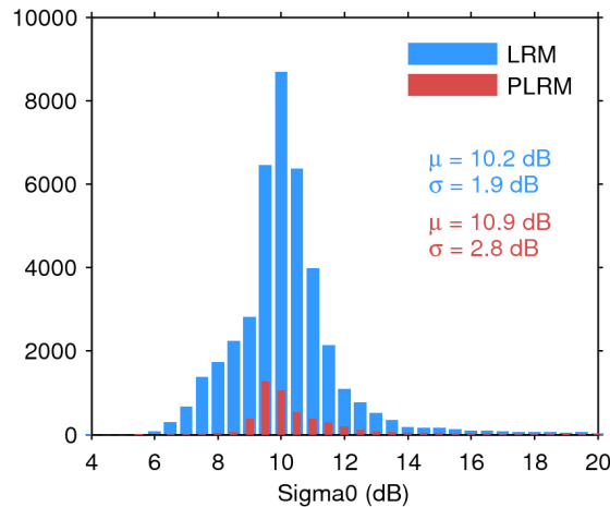
Figure 25. Histogram of flag-valid sigma0 over oceans and lakes for LRM (blue) and PLRM (red) for 11/05/2016. The mean ( \mu ) and standard deviation ( \sigma ) are also shown. Note that values outside [4 20] dB are excluded from the histogram for the sake of readability but not from the computation of \mu and \sigma .
