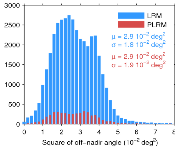
Figure 39. Histogram of flag-valid mispointing over oceans and lakes for LRM (blue) and PLRM (red) for 11/05/2016. Only positive values have been considered. The mean ( \mu ) and standard deviation ( \sigma ) are also shown. Note that values larger than 8 \cdot 10^{-2} \text{ deg}^2 are excluded from the histogram for the sake of readability but not from the computation of \mu and \sigma .
