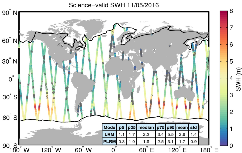
Figure 19. Geographical distribution of science-valid SWH data over oceans and lakes for 11/05/2016. The statistical values shown in the table refer to the SWH in m and are calculated separately for LRM and PLRM regions. The black lines mark the outer limit of the Arctic and Antarctic polar polygons. Gray circles denote records that have been rejected based on the editing criteria described in Table 3.
