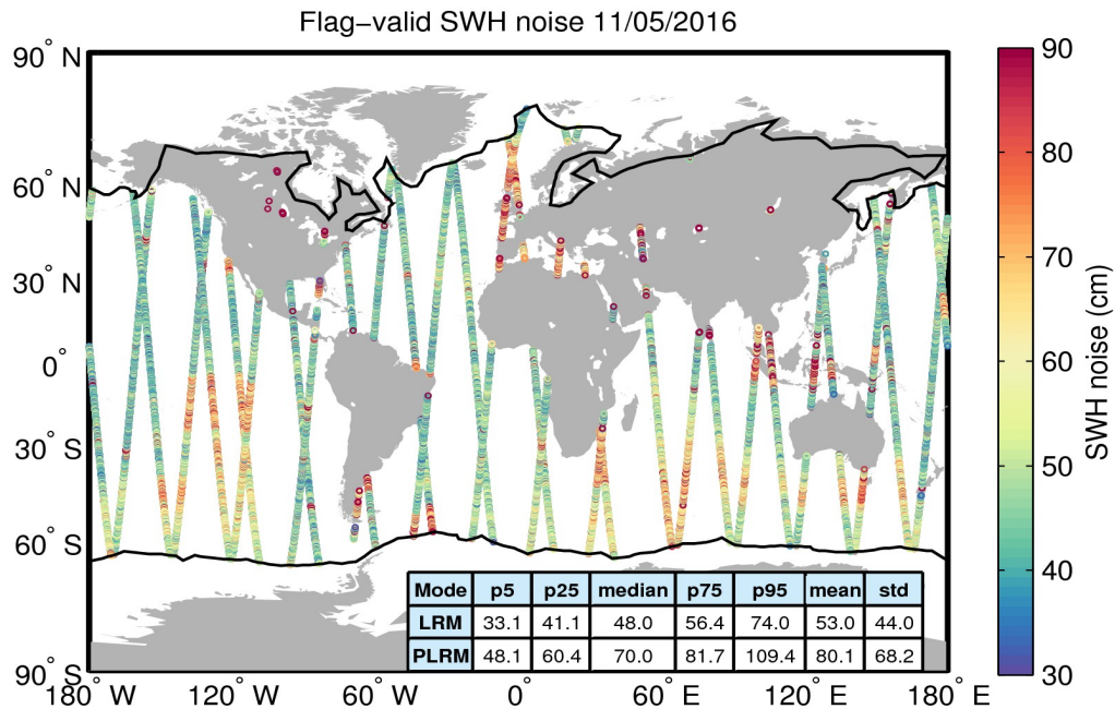
Figure 18. Geographical distribution of flag-valid 20-Hz SWH measurement noise over oceans and lakes for 11/05/2016. The statistical values shown in the table refer to the SWH noise and are calculated separately for LRM and PLRM regions. Measurements taken over polar polygons have been excluded from the computation of the statistical values. The black lines mark the outer limit of the Arctic and Antarctic polar polygons.
