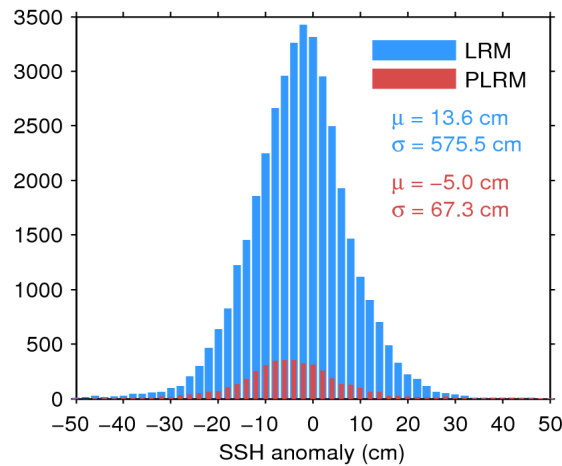
Figure 7. Histogram of flag-valid SSH anomaly over oceans and lakes for LRM (blue) and PLRM (red) for 10/05/2016. The mean ( \mu ) and standard deviation ( \sigma ) are also shown. Note that values outside [-50 50] cm are excluded from the histogram for the sake of readability but not from the computation of \mu and \sigma .
