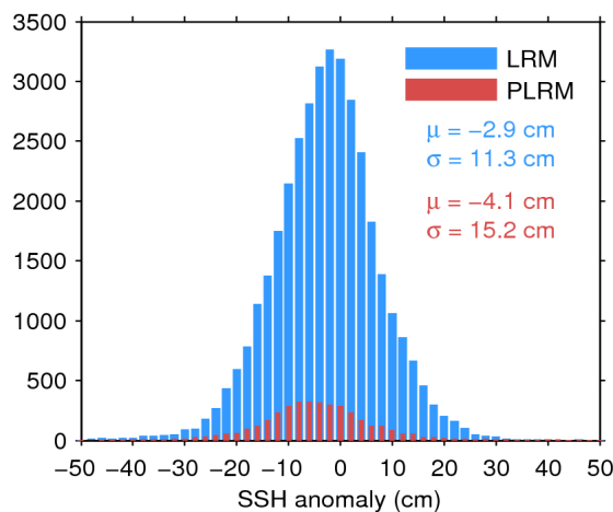
Figure 11. Histogram of science-valid SSH anomaly over oceans and lakes for LRM (blue) and PLRM (red) for 10/05/2016. The mean ( \mu ) and standard deviation ( \sigma ) are also shown. Note that values outside [-50 50] cm are excluded from the histogram for the sake of readability but not from the computation of \mu and \sigma .
