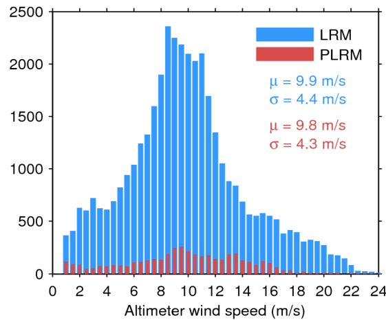
Figure 33. Histogram of flag-valid wind over oceans and lakes for LRM (blue) and PLRM (red) for 10/05/2016. The mean ( \mu ) and standard deviation ( \sigma ) are also shown. Note that values larger than 24 m/s are excluded from the histogram for the sake of readability but not from the computation of \mu and \sigma .
