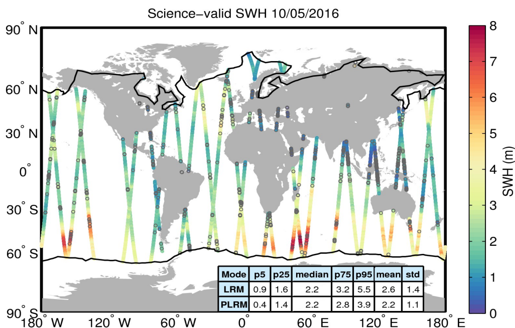
Figure 19. Geographical distribution of science-valid SWH data over oceans and lakes for 10/05/2016. The statistical values shown in the table refer to the SWH in m and are calculated separately for LRM and PLRM regions. The black lines mark the outer limit of the Arctic and Antarctic polar polygons. Gray circles denote records that have been rejected based on the editing criteria described in Table 3.
