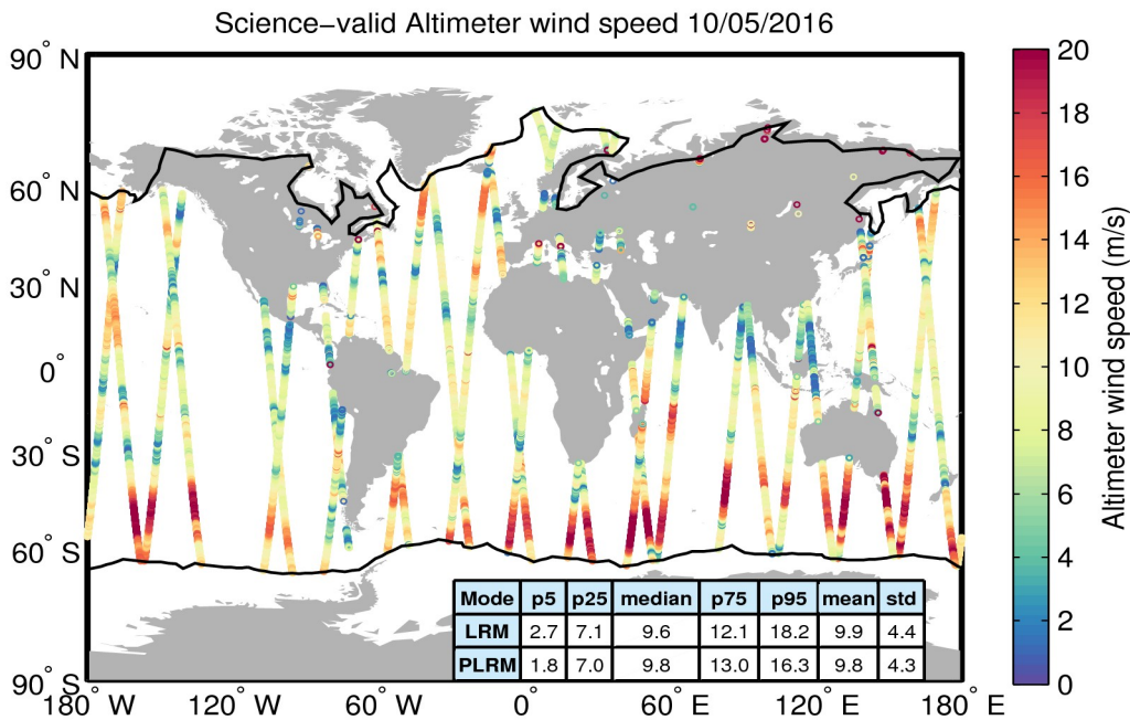
Figure 34. Geographical distribution of science-valid wind data over oceans and lakes for 10/05/2016. The statistical values shown in the table refer to the wind in m/s and are calculated separately for LRM and PLRM regions. The black lines mark the outer limit of the Arctic and Antarctic polar polygons. Gray circles denote records that have been rejected based on the editing criteria described in Table 5.
