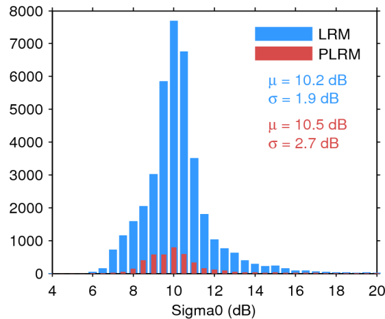
Figure 25. Histogram of flag-valid sigma0 over oceans and lakes for LRM (blue) and PLRM (red) for 10/05/2016. The mean ( \mu ) and standard deviation ( \sigma ) are also shown. Note that values outside [4 20] dB are excluded from the histogram for the sake of readability but not from the computation of \mu and \sigma .
