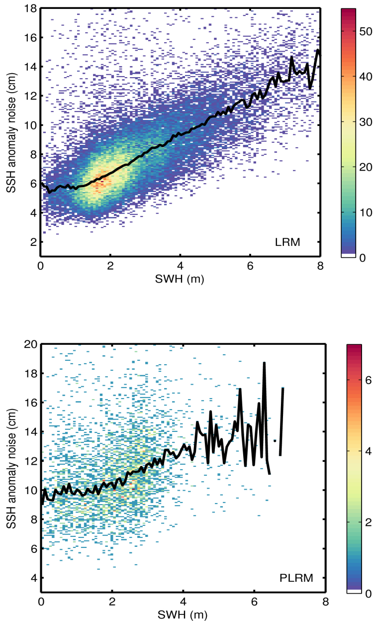
Figure 9. 2D histogram showing flag-valid SSH anomaly noise as a function of SWH for LRM (top) and PLRM (bottom) for 10/05/2016. The black line denotes the median SSH anomaly noise as a function of SWH.
