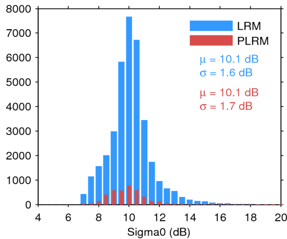
Figure 28. Histogram of science-valid sigma0 over oceans and lakes for LRM (blue) and PLRM (red) for 10/05/2016. The mean ( \mu ) and standard deviation ( \sigma ) are also shown. Note that values outside [4 20] dB are excluded from the histogram for the sake of readability but not from the computation of \mu and \sigma .
