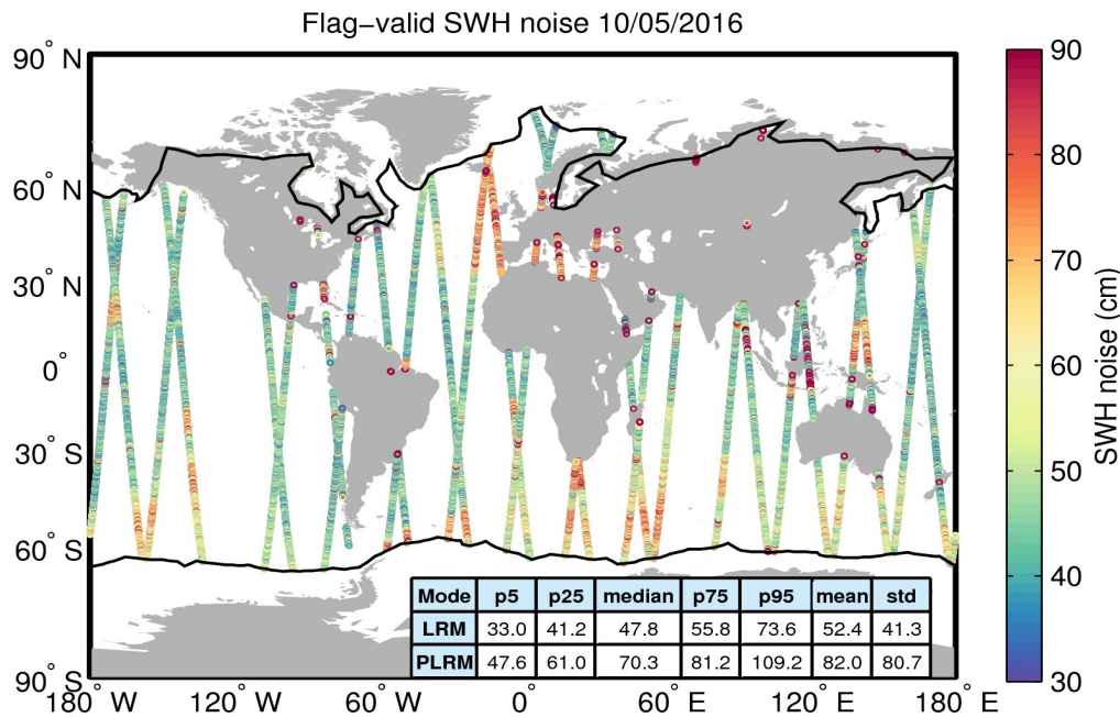
Figure 18. Geographical distribution of flag-valid 20-Hz SWH measurement noise over oceans and lakes for 10/05/2016. The statistical values shown in the table refer to the SWH noise and are calculated separately for LRM and PLRM regions. Measurements taken over polar polygons have been excluded from the computation of the statistical values. The black lines mark the outer limit of the Arctic and Antarctic polar polygons.
