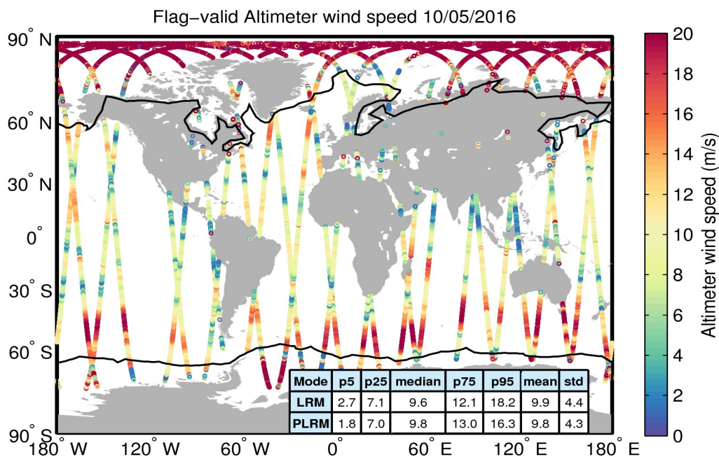
Figure 31. Geographical distribution of flag-valid wind data over oceans and lakes for 10/05/2016. The statistical values shown in the table refer to the wind in m/s and are calculated separately for LRM and PLRM regions. Measurements taken over polar polygons have been excluded from the computation of the statistical values. The black lines mark the outer limit of the Arctic and Antarctic polar polygons.
