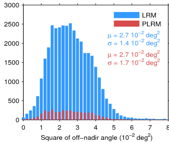
Figure 39. Histogram of flag-valid mispointing over oceans and lakes for LRM (blue) and PLRM (red) for 10/05/2016. Only positive values have been considered. The mean ( \mu ) and standard deviation ( \sigma ) are also shown. Note that values larger than 8 \cdot 10^{-2} \text{ deg}^2 are excluded from the histogram for the sake of readability but not from the computation of \mu and \sigma .
