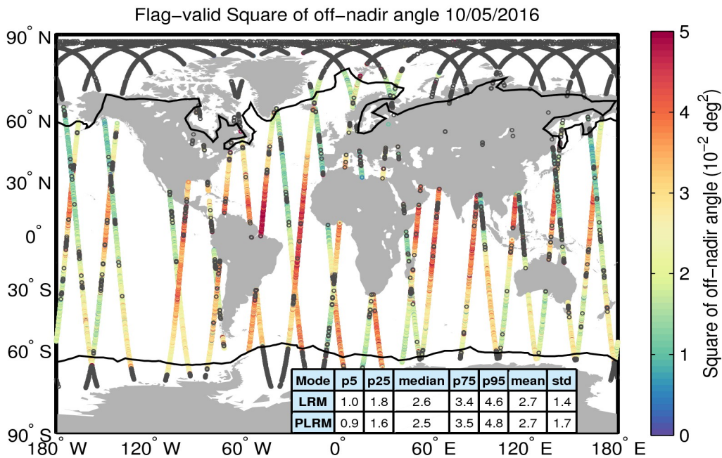
Figure 37. Geographical distribution of flag-valid mispointing data over oceans and lakes for 10/05/2016. The statistical values shown in the table refer to the mispointing in 10^{-2} \text{ deg}^2 and are calculated separately for LRM and PLRM regions. Measurements taken over polar polygons have been excluded from the computation of the statistical values. The black lines mark the outer limit of the Arctic and Antarctic polar polygons. Gray circles denote negative values.
