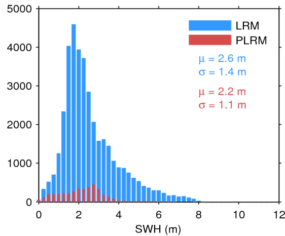
Figure 20. Histogram of science-valid SWH over oceans and lakes for LRM (blue) and PLRM (red) for 10/05/2016. The mean ( \mu ) and standard deviation ( \sigma ) are also shown. Note that values larger than 12 m are excluded from the histogram for the sake of readability but not from the computation of \mu and \sigma .
