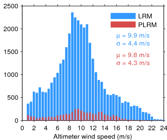
Figure 35. Histogram of science-valid wind over oceans and lakes for LRM (blue) and PLRM (red) for 10/05/2016. The mean ( \mu ) and standard deviation ( \sigma ) are also shown. Note that values larger than 24 m/s are excluded from the histogram for the sake of readability but not from the computation of \mu and \sigma .
