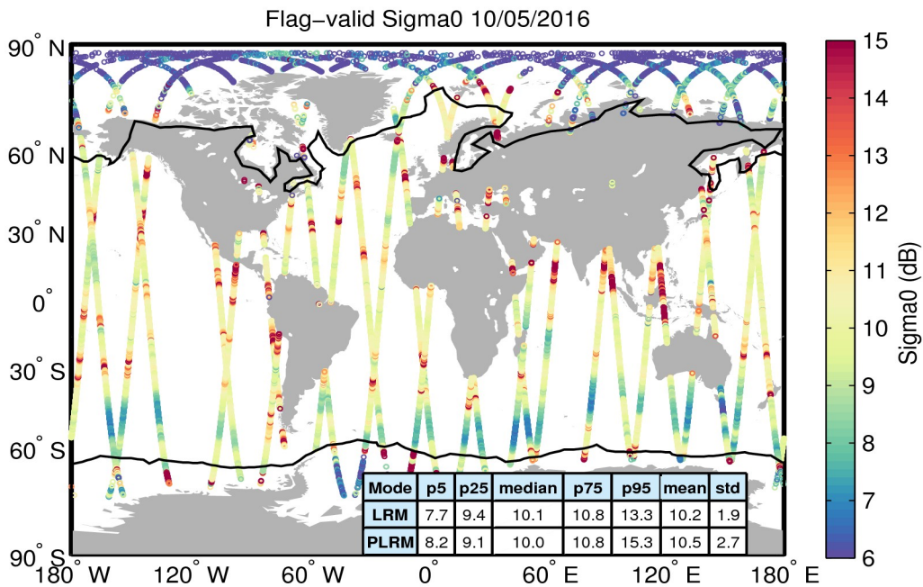
Figure 23. Geographical distribution of flag-valid sigma0 data over oceans and lakes for 10/05/2016. The statistical values shown in the table refer to the sigma0 in dB and are calculated separately for LRM and PLRM regions. Measurements taken over polar polygons have been excluded from the computation of the statistical values. The black lines mark the outer limit of the Arctic and Antarctic polar polygons.
