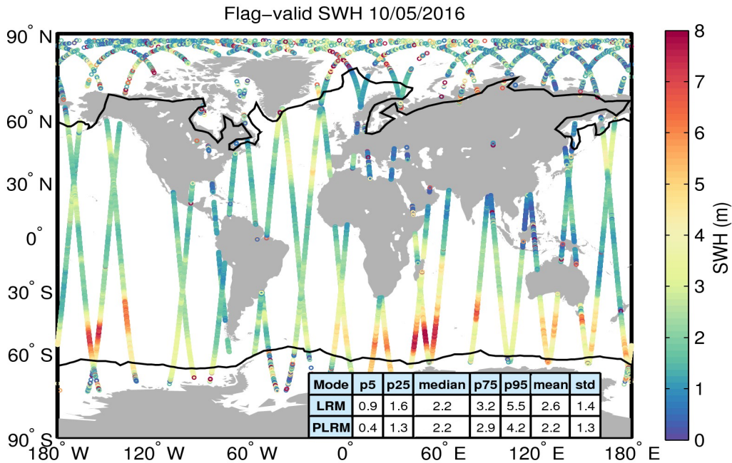
Figure 15. Geographical distribution of flag-valid SWH data over oceans and lakes for 10/05/2016. The statistical values shown in the table refer to the SWH in m and are calculated separately for LRM and PLRM regions. Measurements taken over polar polygons have been excluded from the computation of the statistical values. The black lines mark the outer limit of the Arctic and Antarctic polar polygons.
