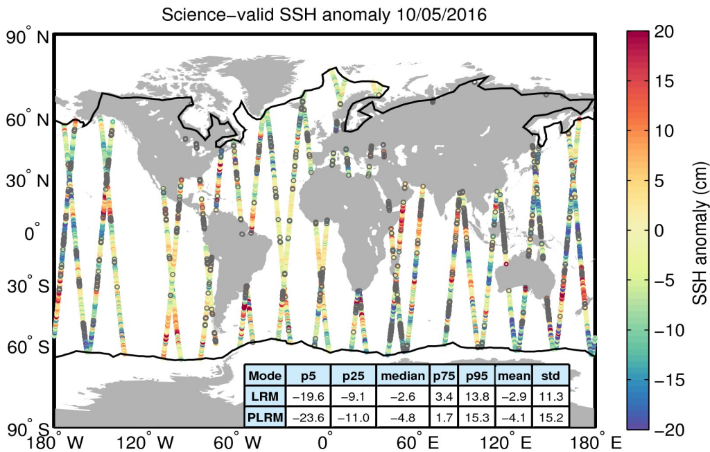
Figure 10. Geographical distribution of science-valid SSH anomaly data over oceans and lakes for 10/05/2016. The statistical values shown in the table refer to the SSH anomaly in cm and are calculated separately for LRM and PLRM regions. The black lines mark the outer limit of the Arctic and Antarctic polar polygons. Gray circles denote records that have been rejected based on the editing criteria described in Table 2.
