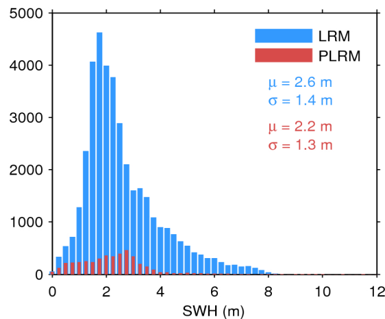
Figure 17. Histogram of flag-valid SWH over oceans and lakes for LRM (blue) and PLRM (red) for 10/05/2016. The mean ( \mu ) and standard deviation ( \sigma ) are also shown. Note that values larger than 12 m are excluded from the histogram for the sake of readability but not from the computation of \mu and \sigma .
