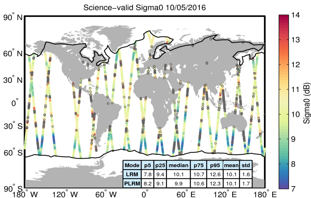
Figure 27. Geographical distribution of science-valid sigma0 data over oceans and lakes for 10/05/2016. The statistical values shown in the table refer to the sigma0 in dB and are calculated separately for LRM and PLRM regions. The black lines mark the outer limit of the Arctic and Antarctic polar polygons. Gray circles denote records that have been rejected based on the editing criteria described in Table 4.
