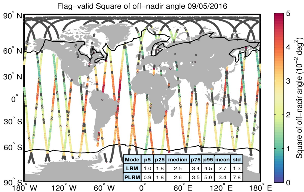
Figure 37. Geographical distribution of flag-valid mispointing data over oceans and lakes for 09/05/2016. The statistical values shown in the table refer to the mispointing in 10^{-2} deg 2 and are calculated separately for LRM and PLRM regions. Measurements taken over polar polygons have been excluded from the computation of the statistical values. The black lines mark the outer limit of the Arctic and Antarctic polar polygons. Gray circles denote negative values.
