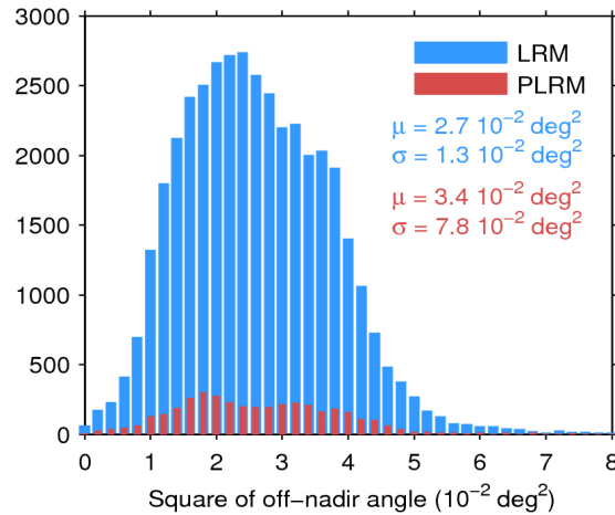
Figure 39. Histogram of flag-valid mispointing over oceans and lakes for LRM (blue) and PLRM (red) for 09/05/2016. Only positive values have been considered. The mean ( \mu ) and standard deviation ( \sigma ) are also shown. Note that values larger than 8 \cdot 10^{-2} \text{ deg}^2 are excluded from the histogram for the sake of readability but not from the computation of \mu and \sigma .
