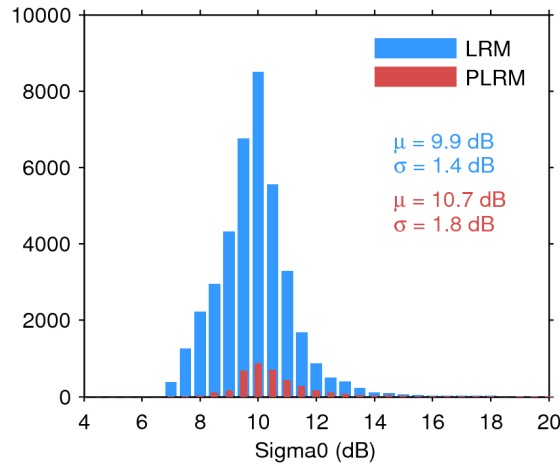
Figure 28. Histogram of science-valid sigma0 over oceans and lakes for LRM (blue) and PLRM (red) for 09/05/2016. The mean ( \mu ) and standard deviation ( \sigma ) are also shown. Note that values outside [4 20] dB are excluded from the histogram for the sake of readability but not from the computation of \mu and \sigma .
