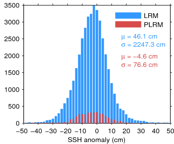
Figure 7. Histogram of flag-valid SSH anomaly over oceans and lakes for LRM (blue) and PLRM (red) for 09/05/2016. The mean ( \mu ) and standard deviation ( \sigma ) are also shown. Note that values outside [-50 50] cm are excluded from the histogram for the sake of readability but not from the computation of \mu and \sigma .
