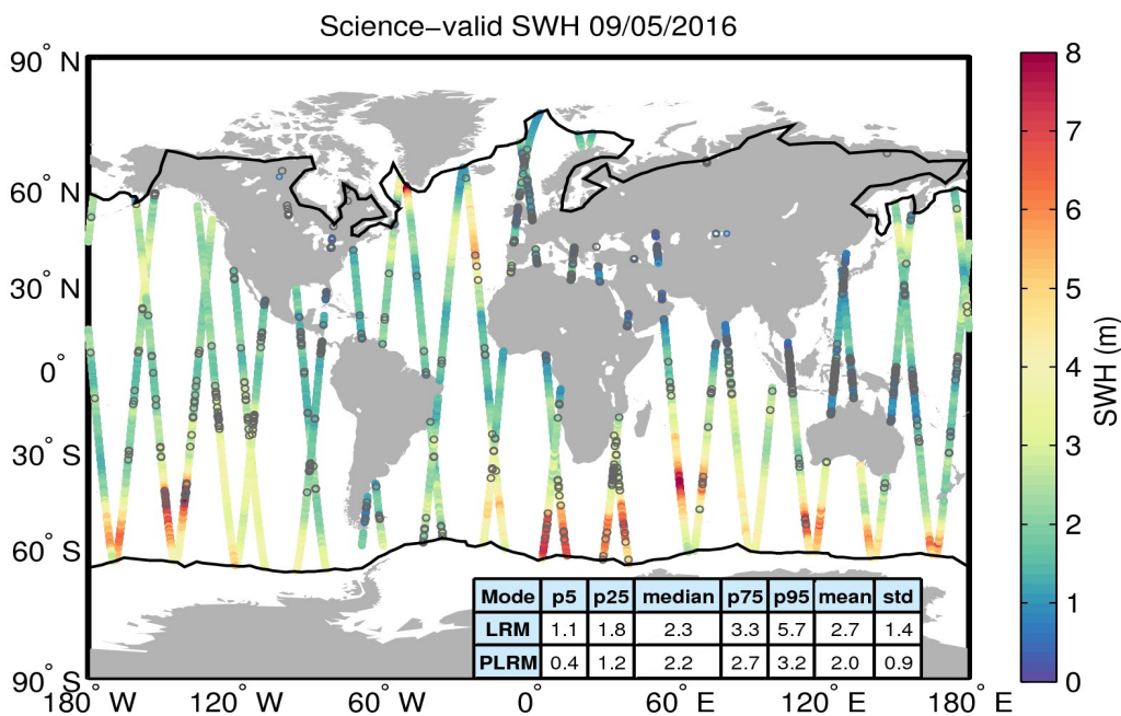
Figure 19. Geographical distribution of science-valid SWH data over oceans and lakes for 09/05/2016. The statistical values shown in the table refer to the SWH in m and are calculated separately for LRM and PLRM regions. The black lines mark the outer limit of the Arctic and Antarctic polar polygons. Gray circles denote records that have been rejected based on the editing criteria described in Table 3.
