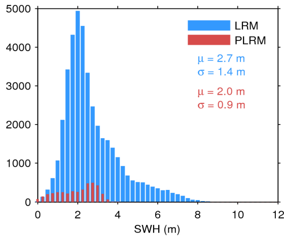
Figure 20. Histogram of science-valid SWH over oceans and lakes for LRM (blue) and PLRM (red) for 09/05/2016. The mean ( \mu ) and standard deviation ( \sigma ) are also shown. Note that values larger than 12 m are excluded from the histogram for the sake of readability but not from the computation of \mu and \sigma .
