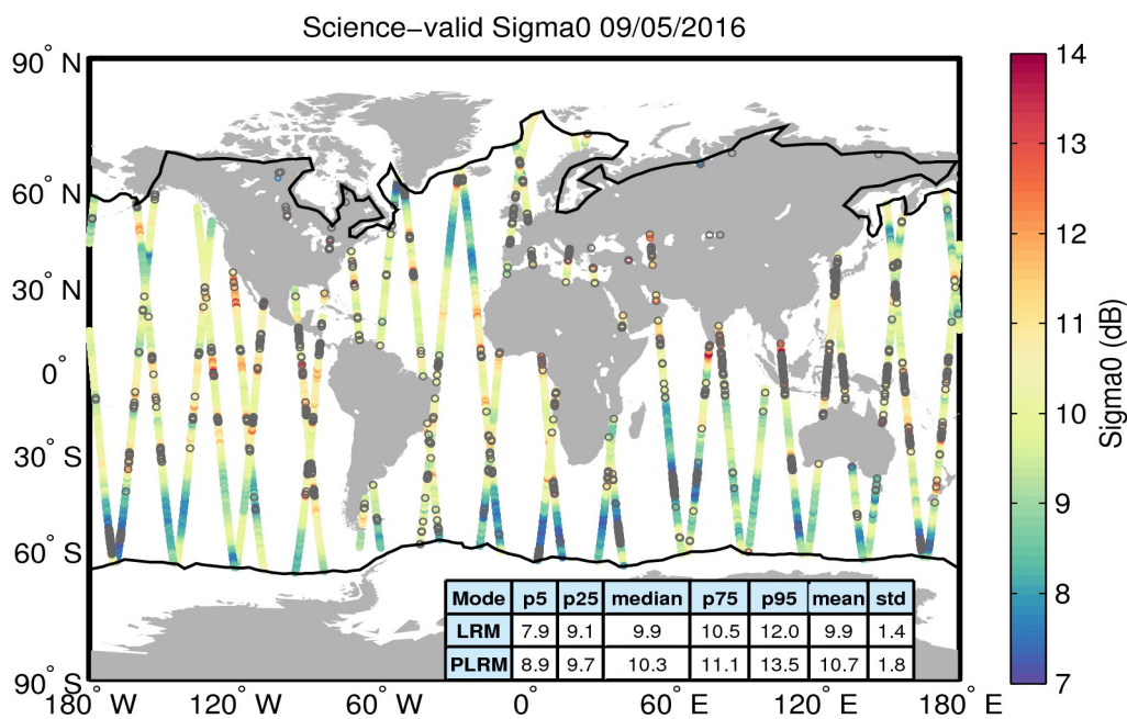
Figure 27. Geographical distribution of science-valid sigma0 data over oceans and lakes for 09/05/2016. The statistical values shown in the table refer to the sigma0 in dB and are calculated separately for LRM and PLRM regions. The black lines mark the outer limit of the Arctic and Antarctic polar polygons. Gray circles denote records that have been rejected based on the editing criteria described in Table 4.
