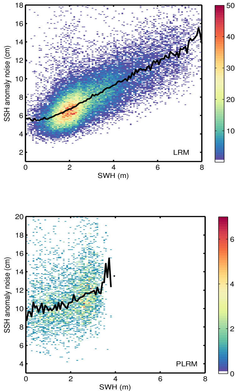
Figure 9. 2D histogram showing flag-valid SSH anomaly noise as a function of SWH for LRM (top) and PLRM (bottom) for 09/05/2016. The black line denotes the median SSH anomaly noise as a function of SWH.
