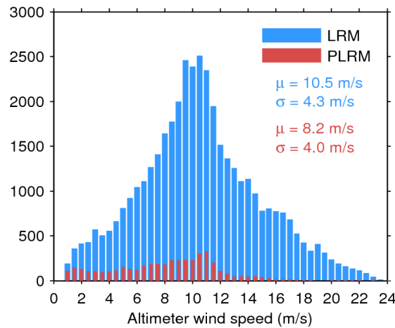
Figure 33. Histogram of flag-valid wind over oceans and lakes for LRM (blue) and PLRM (red) for 09/05/2016. The mean ( \mu ) and standard deviation ( \sigma ) are also shown. Note that values larger than 24 m/s are excluded from the histogram for the sake of readability but not from the computation of \mu and \sigma .
