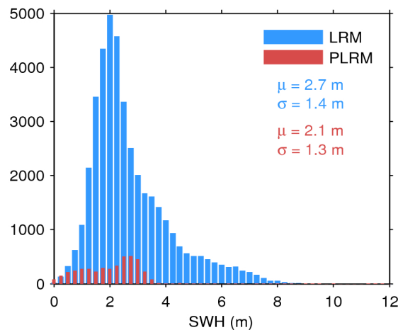
Figure 17. Histogram of flag-valid SWH over oceans and lakes for LRM (blue) and PLRM (red) for 09/05/2016. The mean ( \mu ) and standard deviation ( \sigma ) are also shown. Note that values larger than 12 m are excluded from the histogram for the sake of readability but not from the computation of \mu and \sigma .
