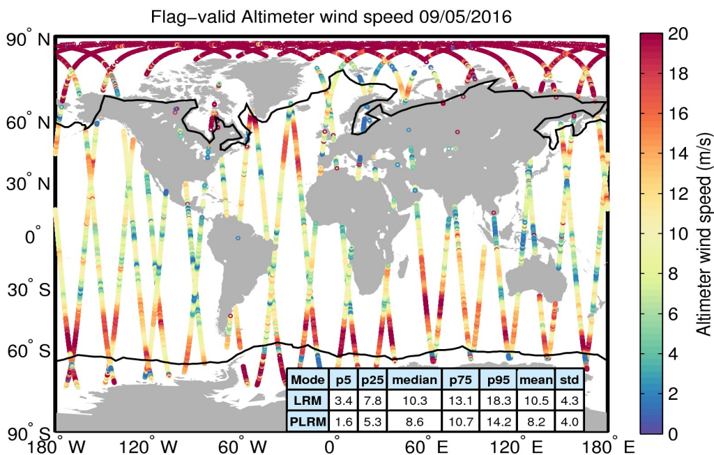
Figure 31. Geographical distribution of flag-valid wind data over oceans and lakes for 09/05/2016. The statistical values shown in the table refer to the wind in m/s and are calculated separately for LRM and PLRM regions. Measurements taken over polar polygons have been excluded from the computation of the statistical values. The black lines mark the outer limit of the Arctic and Antarctic polar polygons.
