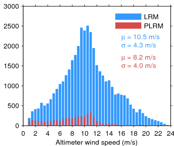
Figure 35. Histogram of science-valid wind over oceans and lakes for LRM (blue) and PLRM (red) for 09/05/2016. The mean ( \mu ) and standard deviation ( \sigma ) are also shown. Note that values larger than 24 m/s are excluded from the histogram for the sake of readability but not from the computation of \mu and \sigma .
