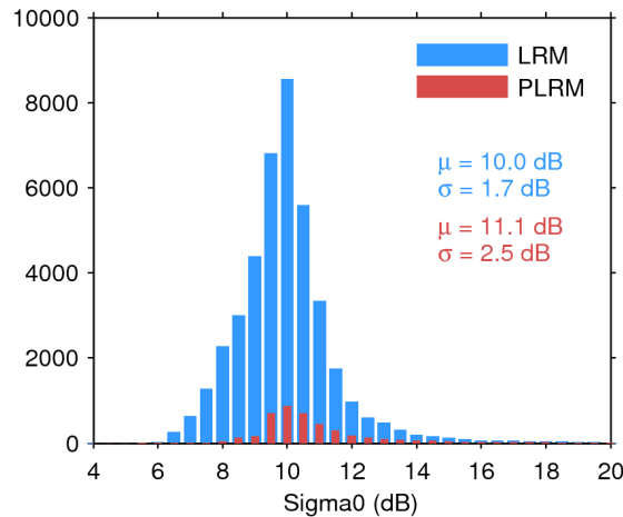
Figure 25. Histogram of flag-valid sigma0 over oceans and lakes for LRM (blue) and PLRM (red) for 09/05/2016. The mean ( \mu ) and standard deviation ( \sigma ) are also shown. Note that values outside [4 20] dB are excluded from the histogram for the sake of readability but not from the computation of \mu and \sigma .
