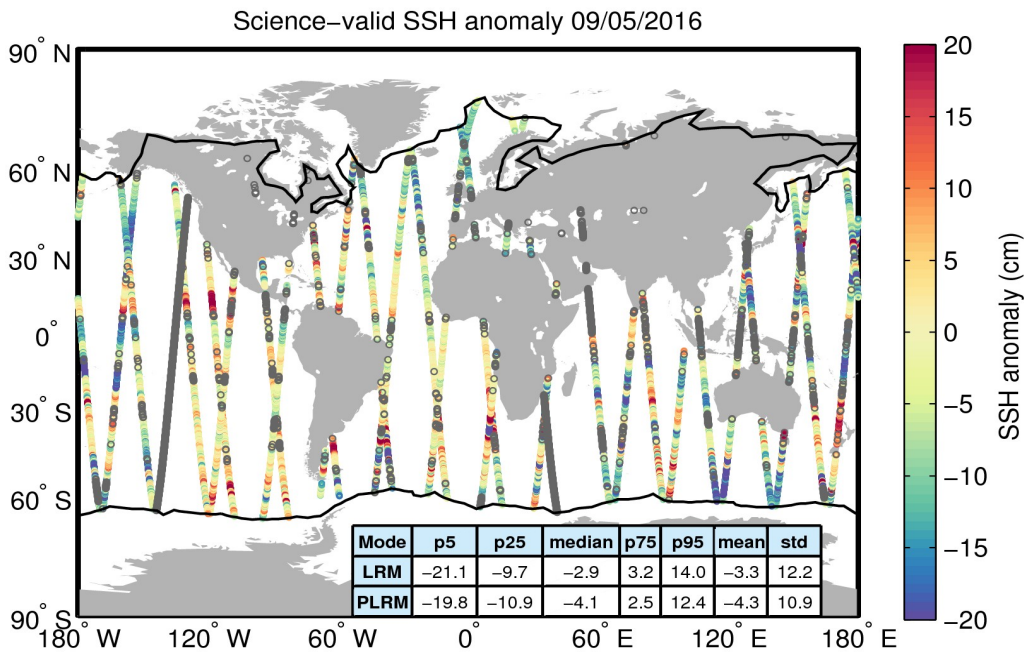
Figure 10. Geographical distribution of science-valid SSH anomaly data over oceans and lakes for 09/05/2016. The statistical values shown in the table refer to the SSH anomaly in cm and are calculated separately for LRM and PLRM regions. The black lines mark the outer limit of the Arctic and Antarctic polar polygons. Gray circles denote records that have been rejected based on the editing criteria described in Table 2.
