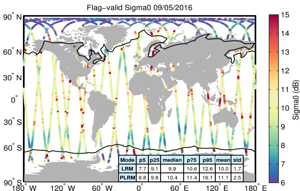
Figure 23. Geographical distribution of flag-valid sigma0 data over oceans and lakes for 09/05/2016. The statistical values shown in the table refer to the sigma0 in dB and are calculated separately for LRM and PLRM regions. Measurements taken over polar polygons have been excluded from the computation of the statistical values. The black lines mark the outer limit of the Arctic and Antarctic polar polygons.
