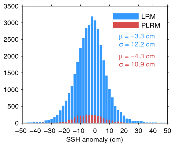
Figure 11. Histogram of science-valid SSH anomaly over oceans and lakes for LRM (blue) and PLRM (red) for 09/05/2016. The mean ( \mu ) and standard deviation ( \sigma ) are also shown. Note that values outside [-50 50] cm are excluded from the histogram for the sake of readability but not from the computation of \mu and \sigma .
