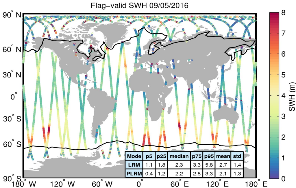
Figure 15. Geographical distribution of flag-valid SWH data over oceans and lakes for 09/05/2016. The statistical values shown in the table refer to the SWH in m and are calculated separately for LRM and PLRM regions. Measurements taken over polar polygons have been excluded from the computation of the statistical values. The black lines mark the outer limit of the Arctic and Antarctic polar polygons.
