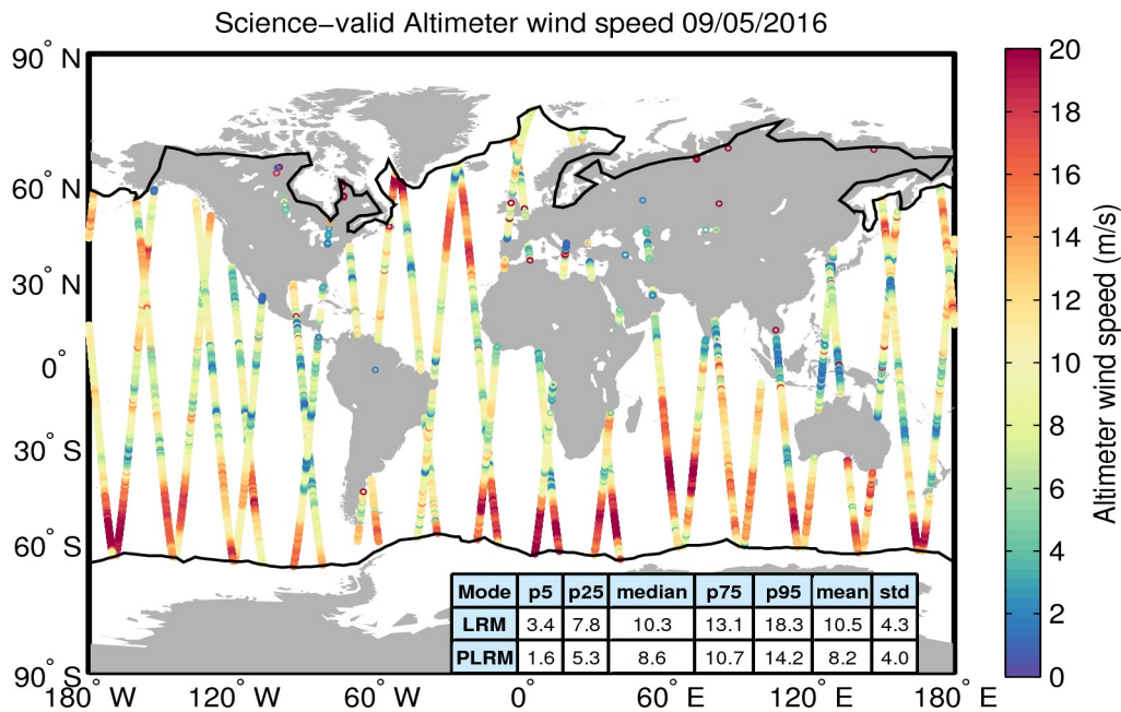
Figure 34. Geographical distribution of science-valid wind data over oceans and lakes for 09/05/2016. The statistical values shown in the table refer to the wind in m/s and are calculated separately for LRM and PLRM regions. The black lines mark the outer limit of the Arctic and Antarctic polar polygons. Gray circles denote records that have been rejected based on the editing criteria described in Table 5.
