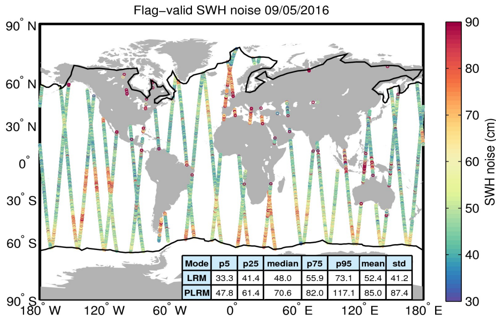
Figure 18. Geographical distribution of flag-valid 20-Hz SWH measurement noise over oceans and lakes for 09/05/2016. The statistical values shown in the table refer to the SWH noise and are calculated separately for LRM and PLRM regions. Measurements taken over polar polygons have been excluded from the computation of the statistical values. The black lines mark the outer limit of the Arctic and Antarctic polar polygons.
