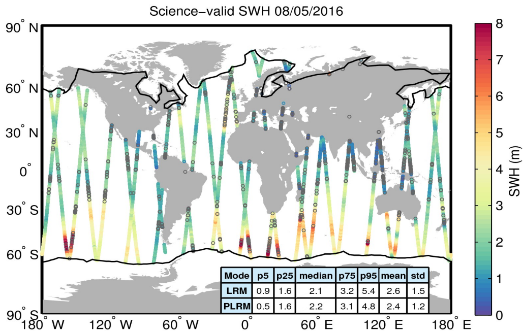
Figure 19. Geographical distribution of science-valid SWH data over oceans and lakes for 08/05/2016. The statistical values shown in the table refer to the SWH in m and are calculated separately for LRM and PLRM regions. The black lines mark the outer limit of the Arctic and Antarctic polar polygons. Gray circles denote records that have been rejected based on the editing criteria described in Table 3.
