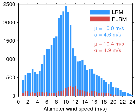
Figure 33. Histogram of flag-valid wind over oceans and lakes for LRM (blue) and PLRM (red) for 08/05/2016. The mean ( \mu ) and standard deviation ( \sigma ) are also shown. Note that values larger than 24 m/s are excluded from the histogram for the sake of readability but not from the computation of \mu and \sigma .
