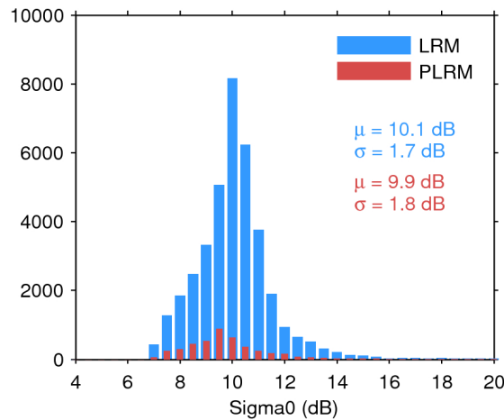
Figure 28. Histogram of science-valid sigma0 over oceans and lakes for LRM (blue) and PLRM (red) for 08/05/2016. The mean ( \mu ) and standard deviation ( \sigma ) are also shown. Note that values outside [4 20] dB are excluded from the histogram for the sake of readability but not from the computation of \mu and \sigma .
