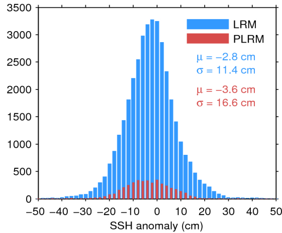
Figure 11. Histogram of science-valid SSH anomaly over oceans and lakes for LRM (blue) and PLRM (red) for 08/05/2016. The mean ( \mu ) and standard deviation ( \sigma ) are also shown. Note that values outside [-50 50] cm are excluded from the histogram for the sake of readability but not from the computation of \mu and \sigma .
