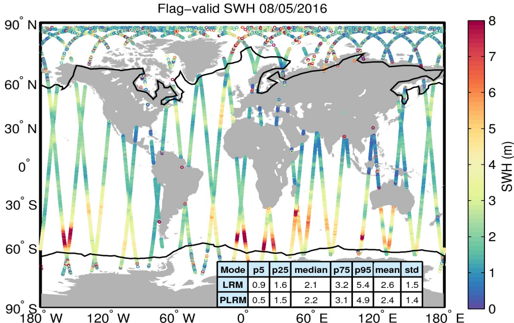
Figure 15. Geographical distribution of flag-valid SWH data over oceans and lakes for 08/05/2016. The statistical values shown in the table refer to the SWH in m and are calculated separately for LRM and PLRM regions. Measurements taken over polar polygons have been excluded from the computation of the statistical values. The black lines mark the outer limit of the Arctic and Antarctic polar polygons.
