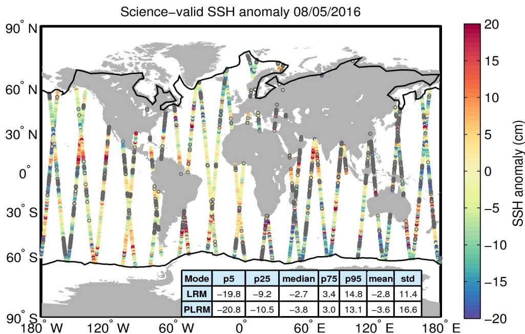
Figure 10. Geographical distribution of science-valid SSH anomaly data over oceans and lakes for 08/05/2016. The statistical values shown in the table refer to the SSH anomaly in cm and are calculated separately for LRM and PLRM regions. The black lines mark the outer limit of the Arctic and Antarctic polar polygons. Gray circles denote records that have been rejected based on the editing criteria described in Table 2.
