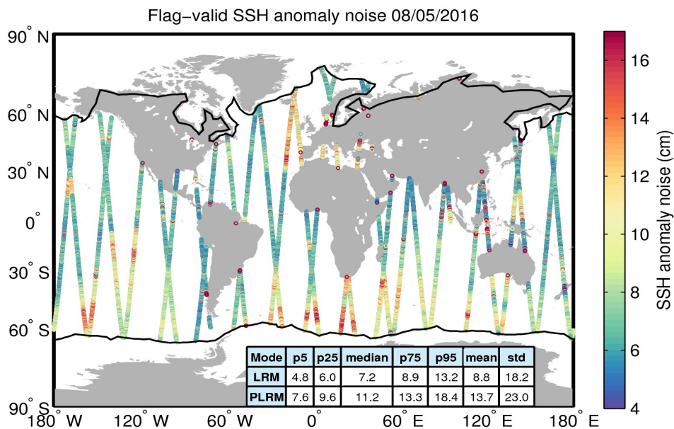
Figure 8. Geographical distribution of flag-valid 20-Hz SSH anomaly measurement noise over oceans and lakes for 08/05/2016. The statistical values shown in the table refer to the SSH anomaly noise and are calculated separately for LRM and PLRM regions. Measurements taken over polar polygons have been excluded from the computation of the statistical values. The black lines mark the outer limit of the Arctic and Antarctic polar polygons.
