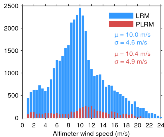
Figure 35. Histogram of science-valid wind over oceans and lakes for LRM (blue) and PLRM (red) for 08/05/2016. The mean ( \mu ) and standard deviation ( \sigma ) are also shown. Note that values larger than 24 m/s are excluded from the histogram for the sake of readability but not from the computation of \mu and \sigma .
