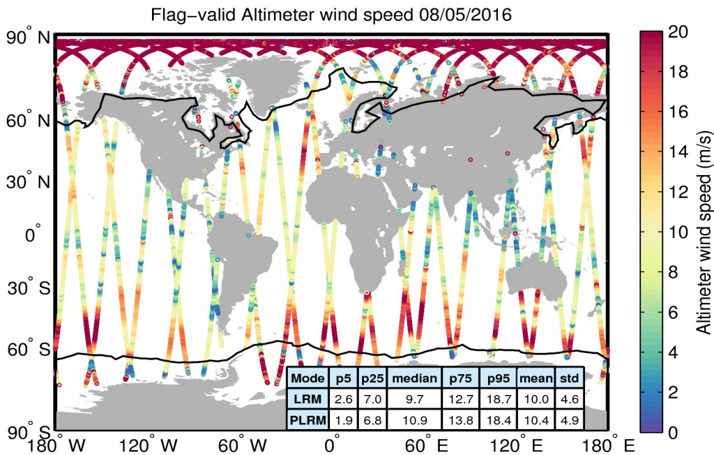
Figure 31. Geographical distribution of flag-valid wind data over oceans and lakes for 08/05/2016. The statistical values shown in the table refer to the wind in m/s and are calculated separately for LRM and PLRM regions. Measurements taken over polar polygons have been excluded from the computation of the statistical values. The black lines mark the outer limit of the Arctic and Antarctic polar polygons.
