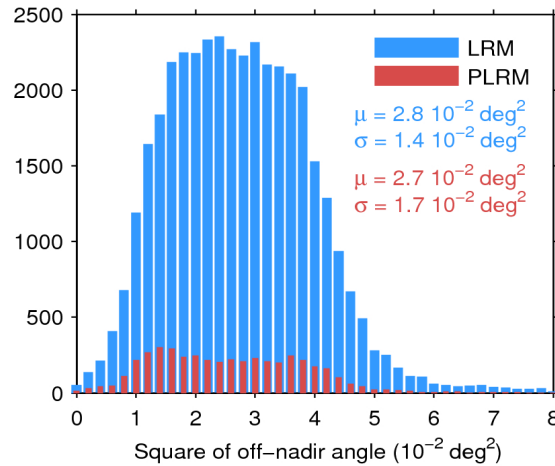
Figure 39. Histogram of flag-valid mispointing over oceans and lakes for LRM (blue) and PLRM (red) for 08/05/2016. Only positive values have been considered. The mean ( \mu ) and standard deviation ( \sigma ) are also shown. Note that values larger than 8 \cdot 10^{-2} \text{ deg}^2 are excluded from the histogram for the sake of readability but not from the computation of \mu and \sigma .
