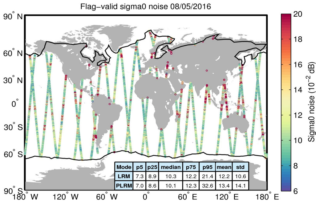
Figure 26. Geographical distribution of flag-valid 20-Hz sigma0 measurement noise over oceans and lakes for 08/05/2016. The statistical values shown in the table refer to the sigma0 noise and are calculated separately for LRM and PLRM regions. Measurements taken over polar polygons have been excluded from the computation of the statistical values. The black lines mark the outer limit of the Arctic and Antarctic polar polygons.
