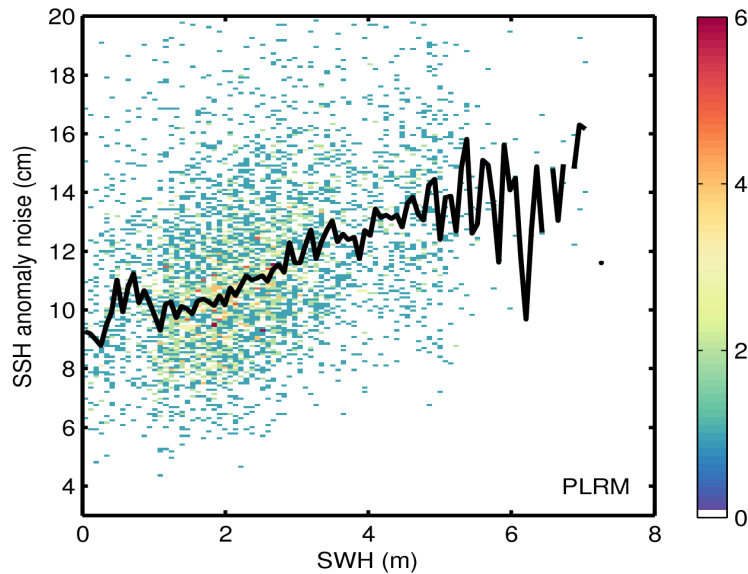
Figure 9. 2D histogram showing flag-valid SSH anomaly noise as a function of SWH for LRM (top) and PLRM (bottom) for 08/05/2016. The black line denotes the median SSH anomaly noise as a function of SWH.
