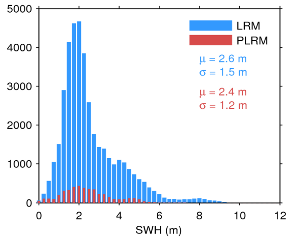
Figure 20. Histogram of science-valid SWH over oceans and lakes for LRM (blue) and PLRM (red) for 08/05/2016. The mean ( \mu ) and standard deviation ( \sigma ) are also shown. Note that values larger than 12 m are excluded from the histogram for the sake of readability but not from the computation of \mu and \sigma .
