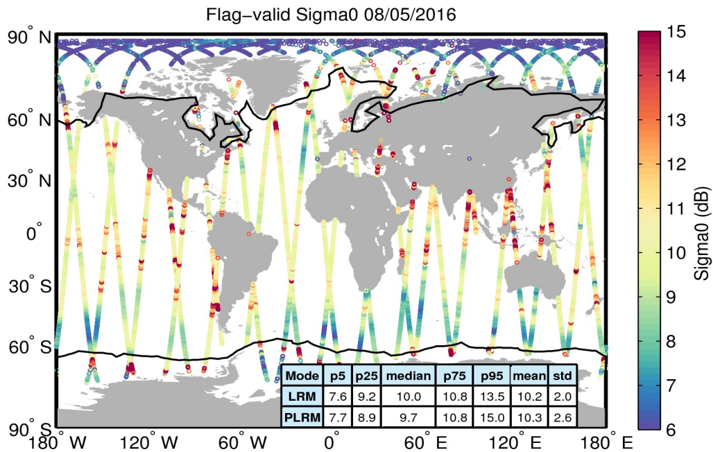
Figure 23. Geographical distribution of flag-valid sigma0 data over oceans and lakes for 08/05/2016. The statistical values shown in the table refer to the sigma0 in dB and are calculated separately for LRM and PLRM regions. Measurements taken over polar polygons have been excluded from the computation of the statistical values. The black lines mark the outer limit of the Arctic and Antarctic polar polygons.
