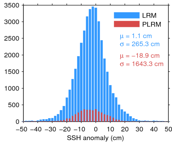
Figure 7. Histogram of flag-valid SSH anomaly over oceans and lakes for LRM (blue) and PLRM (red) for 08/05/2016. The mean ( \mu ) and standard deviation ( \sigma ) are also shown. Note that values outside [-50 50] cm are excluded from the histogram for the sake of readability but not from the computation of \mu and \sigma .
