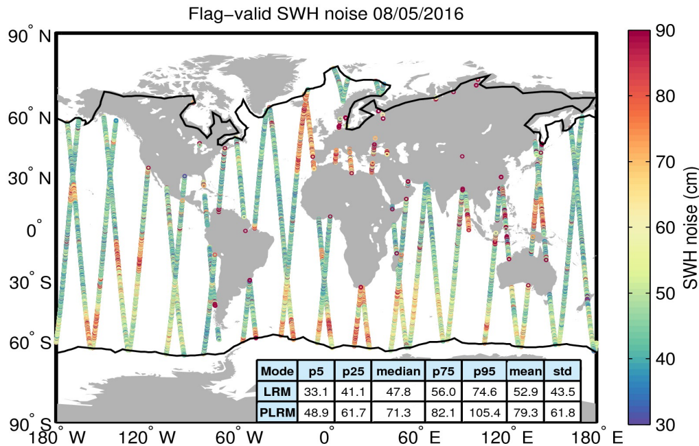
Figure 18. Geographical distribution of flag-valid 20-Hz SWH measurement noise over oceans and lakes for 08/05/2016. The statistical values shown in the table refer to the SWH noise and are calculated separately for LRM and PLRM regions. Measurements taken over polar polygons have been excluded from the computation of the statistical values. The black lines mark the outer limit of the Arctic and Antarctic polar polygons.
