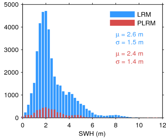
Figure 17. Histogram of flag-valid SWH over oceans and lakes for LRM (blue) and PLRM (red) for 08/05/2016. The mean ( \mu ) and standard deviation ( \sigma ) are also shown. Note that values larger than 12 m are excluded from the histogram for the sake of readability but not from the computation of \mu and \sigma .
