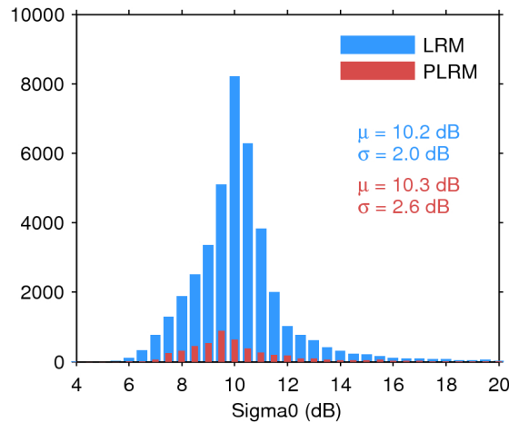
Figure 25. Histogram of flag-valid sigma0 over oceans and lakes for LRM (blue) and PLRM (red) for 08/05/2016. The mean ( \mu ) and standard deviation ( \sigma ) are also shown. Note that values outside [4 20] dB are excluded from the histogram for the sake of readability but not from the computation of \mu and \sigma .
