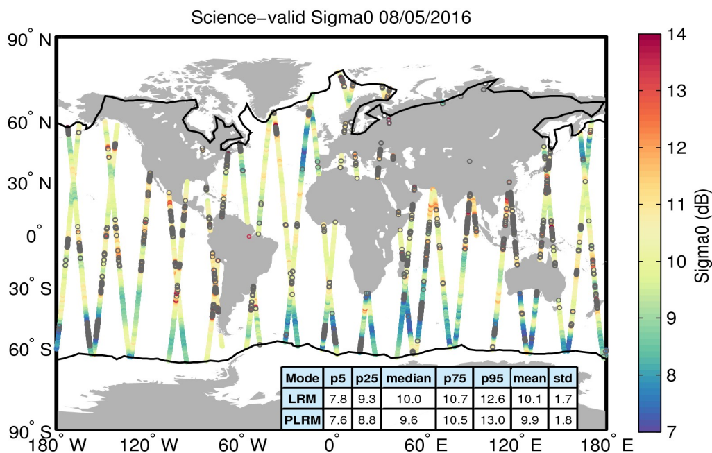
Figure 27. Geographical distribution of science-valid sigma0 data over oceans and lakes for 08/05/2016. The statistical values shown in the table refer to the sigma0 in dB and are calculated separately for LRM and PLRM regions. The black lines mark the outer limit of the Arctic and Antarctic polar polygons. Gray circles denote records that have been rejected based on the editing criteria described in Table 4.
