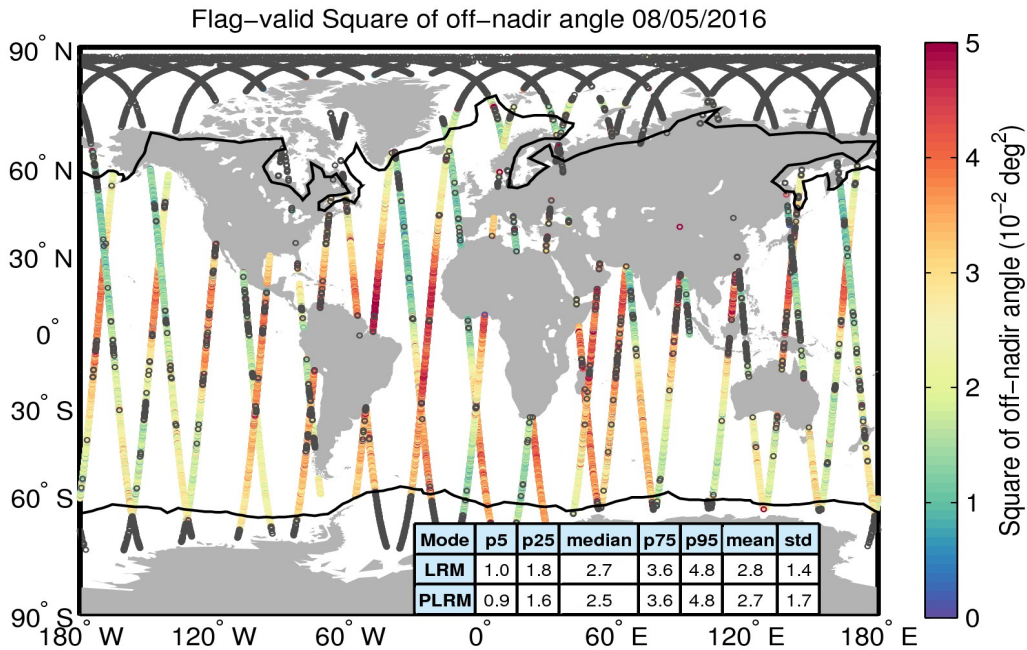
Figure 37. Geographical distribution of flag-valid mispointing data over oceans and lakes for 08/05/2016. The statistical values shown in the table refer to the mispointing in 10^{-2} deg 2 and are calculated separately for LRM and PLRM regions. Measurements taken over polar polygons have been excluded from the computation of the statistical values. The black lines mark the outer limit of the Arctic and Antarctic polar polygons. Gray circles denote negative values.
