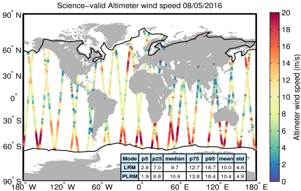
Figure 34. Geographical distribution of science-valid wind data over oceans and lakes for 08/05/2016. The statistical values shown in the table refer to the wind in m/s and are calculated separately for LRM and PLRM regions. The black lines mark the outer limit of the Arctic and Antarctic polar polygons. Gray circles denote records that have been rejected based on the editing criteria described in Table 5.
