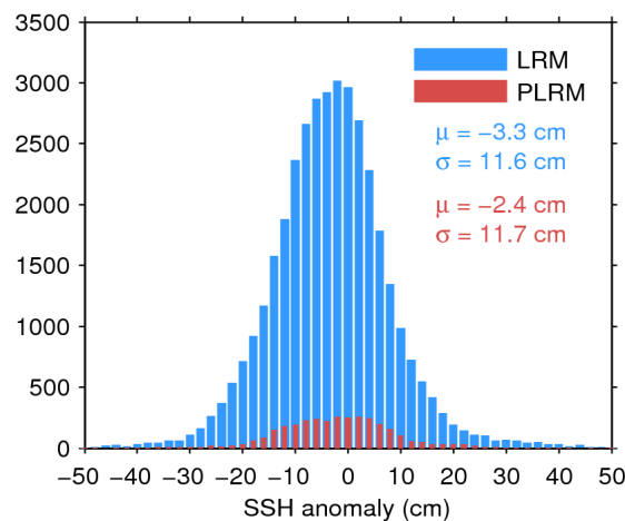
Figure 11. Histogram of science-valid SSH anomaly over oceans and lakes for LRM (blue) and PLRM (red) for 07/05/2016. The mean ( \mu ) and standard deviation ( \sigma ) are also shown. Note that values outside [-50 50] cm are excluded from the histogram for the sake of readability but not from the computation of \mu and \sigma .
