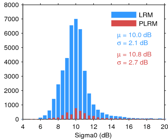
Figure 25. Histogram of flag-valid sigma0 over oceans and lakes for LRM (blue) and PLRM (red) for 07/05/2016. The mean ( \mu ) and standard deviation ( \sigma ) are also shown. Note that values outside [4 20] dB are excluded from the histogram for the sake of readability but not from the computation of \mu and \sigma .
