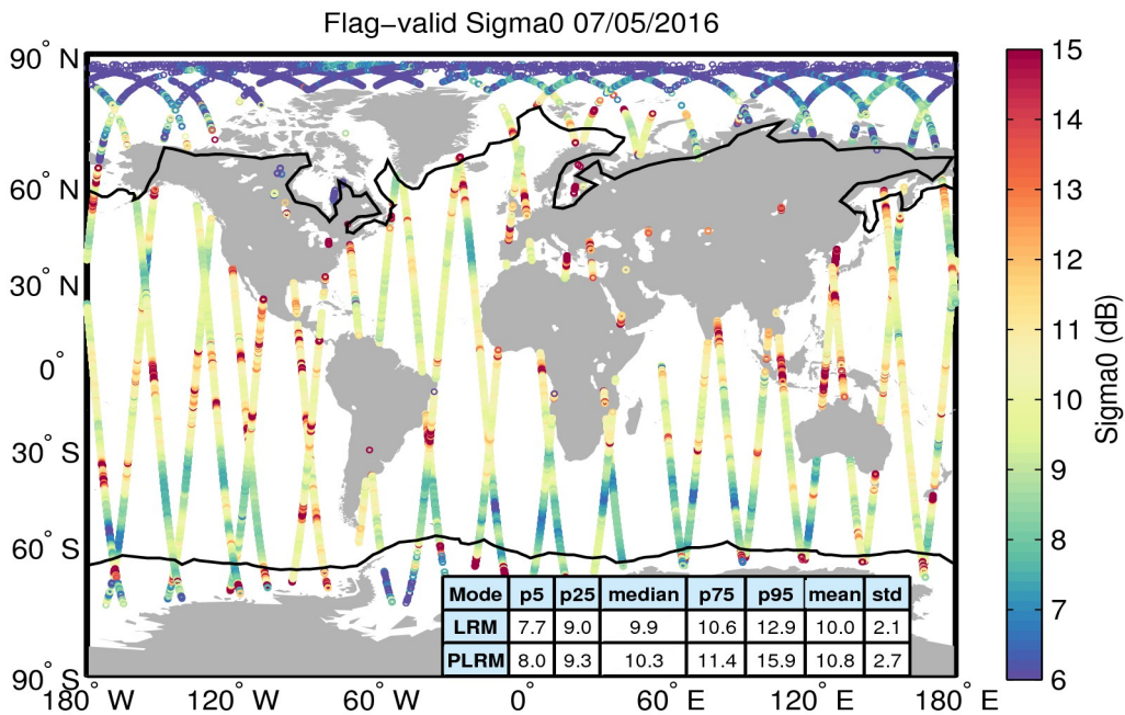
Figure 23. Geographical distribution of flag-valid sigma0 data over oceans and lakes for 07/05/2016. The statistical values shown in the table refer to the sigma0 in dB and are calculated separately for LRM and PLRM regions. Measurements taken over polar polygons have been excluded from the computation of the statistical values. The black lines mark the outer limit of the Arctic and Antarctic polar polygons.
