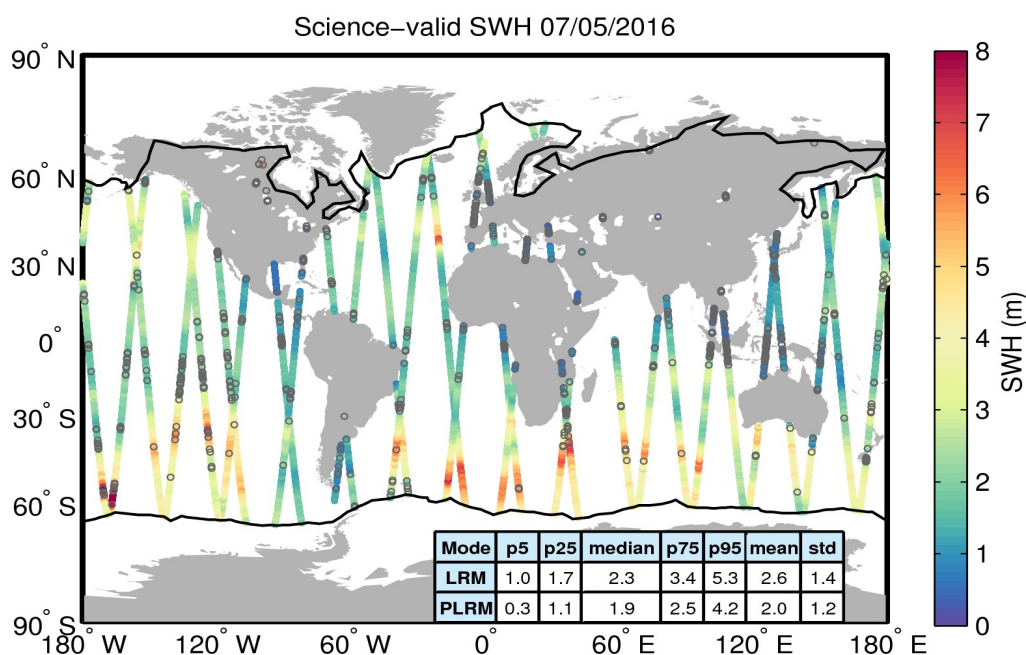
Figure 19. Geographical distribution of science-valid SWH data over oceans and lakes for 07/05/2016. The statistical values shown in the table refer to the SWH in m and are calculated separately for LRM and PLRM regions. The black lines mark the outer limit of the Arctic and Antarctic polar polygons. Gray circles denote records that have been rejected based on the editing criteria described in Table 3.
