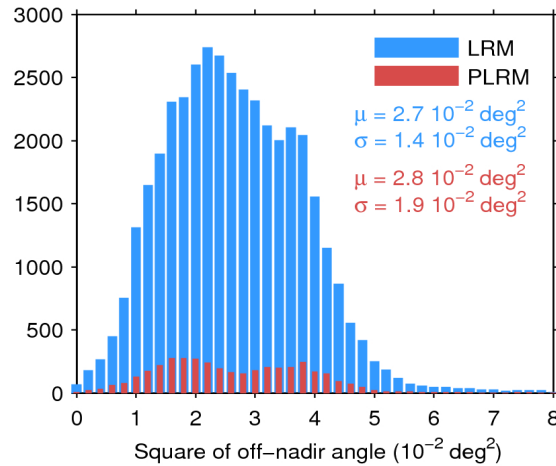
Figure 39. Histogram of flag-valid mispointing over oceans and lakes for LRM (blue) and PLRM (red) for 07/05/2016. Only positive values have been considered. The mean ( \mu ) and standard deviation ( \sigma ) are also shown. Note that values larger than 8 \cdot 10^{-2} \text{ deg}^2 are excluded from the histogram for the sake of readability but not from the computation of \mu and \sigma .
