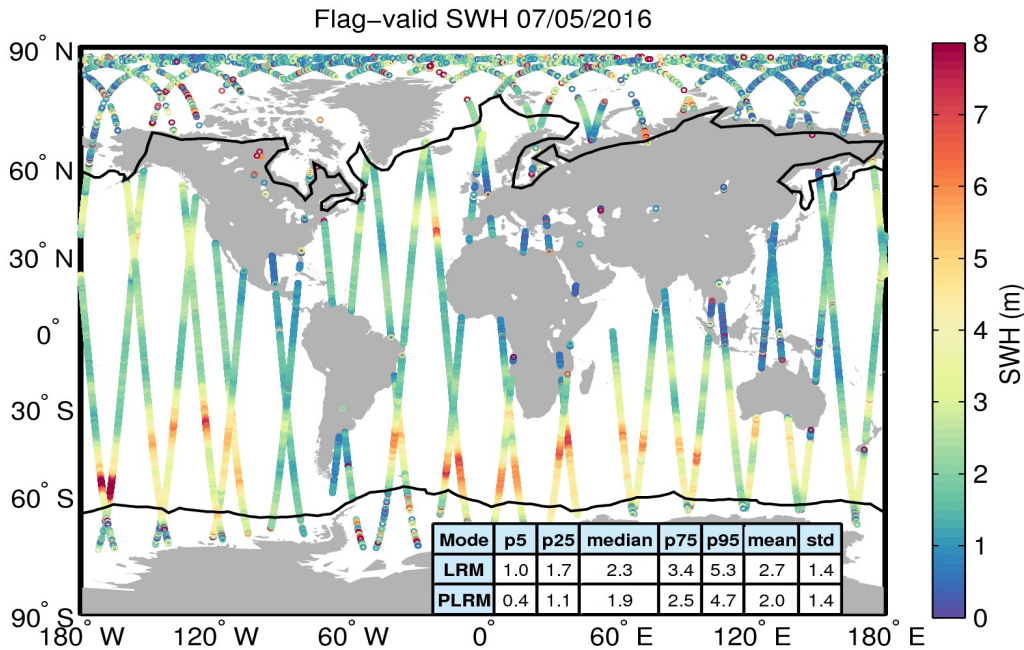
Figure 15. Geographical distribution of flag-valid SWH data over oceans and lakes for 07/05/2016. The statistical values shown in the table refer to the SWH in m and are calculated separately for LRM and PLRM regions. Measurements taken over polar polygons have been excluded from the computation of the statistical values. The black lines mark the outer limit of the Arctic and Antarctic polar polygons.
