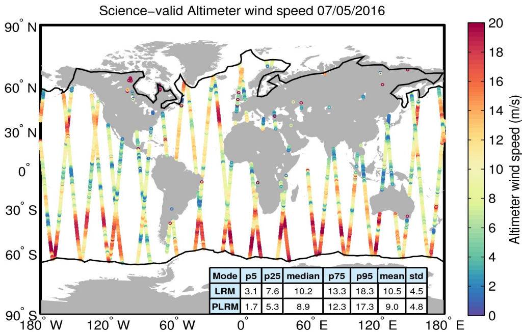
Figure 34. Geographical distribution of science-valid wind data over oceans and lakes for 07/05/2016. The statistical values shown in the table refer to the wind in m/s and are calculated separately for LRM and PLRM regions. The black lines mark the outer limit of the Arctic and Antarctic polar polygons. Gray circles denote records that have been rejected based on the editing criteria described in Table 5.
