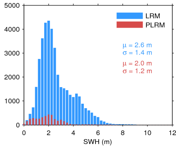
Figure 20. Histogram of science-valid SWH over oceans and lakes for LRM (blue) and PLRM (red) for 07/05/2016. The mean ( \mu ) and standard deviation ( \sigma ) are also shown. Note that values larger than 12 m are excluded from the histogram for the sake of readability but not from the computation of \mu and \sigma .
