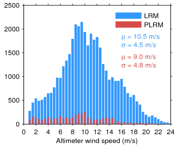
Figure 33. Histogram of flag-valid wind over oceans and lakes for LRM (blue) and PLRM (red) for 07/05/2016. The mean ( \mu ) and standard deviation ( \sigma ) are also shown. Note that values larger than 24 m/s are excluded from the histogram for the sake of readability but not from the computation of \mu and \sigma .
