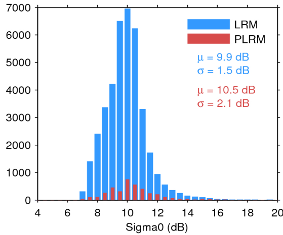
Figure 28. Histogram of science-valid sigma0 over oceans and lakes for LRM (blue) and PLRM (red) for 07/05/2016. The mean ( \mu ) and standard deviation ( \sigma ) are also shown. Note that values outside [4 20] dB are excluded from the histogram for the sake of readability but not from the computation of \mu and \sigma .
