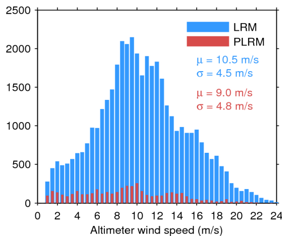
Figure 35. Histogram of science-valid wind over oceans and lakes for LRM (blue) and PLRM (red) for 07/05/2016. The mean ( \mu ) and standard deviation ( \sigma ) are also shown. Note that values larger than 24 m/s are excluded from the histogram for the sake of readability but not from the computation of \mu and \sigma .
