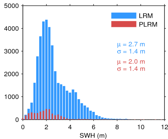
Figure 17. Histogram of flag-valid SWH over oceans and lakes for LRM (blue) and PLRM (red) for 07/05/2016. The mean ( \mu ) and standard deviation ( \sigma ) are also shown. Note that values larger than 12 m are excluded from the histogram for the sake of readability but not from the computation of \mu and \sigma .
