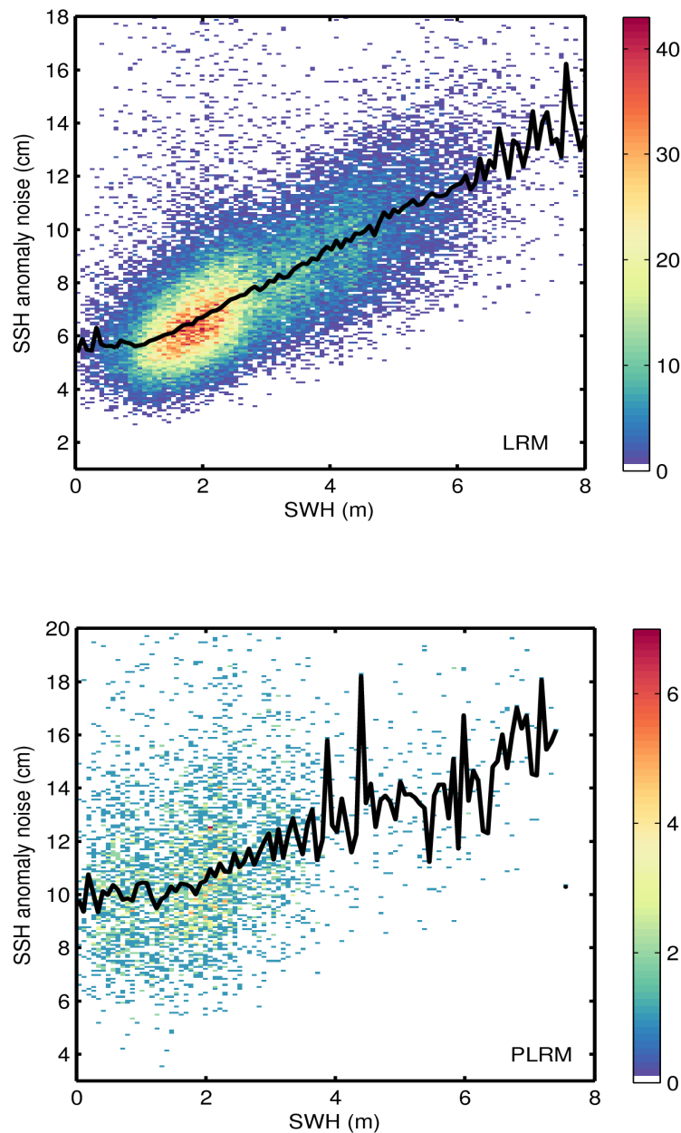
Figure 9. 2D histogram showing flag-valid SSH anomaly noise as a function of SWH for LRM (top) and PLRM (bottom) for 07/05/2016. The black line denotes the median SSH anomaly noise as a function of SWH.
