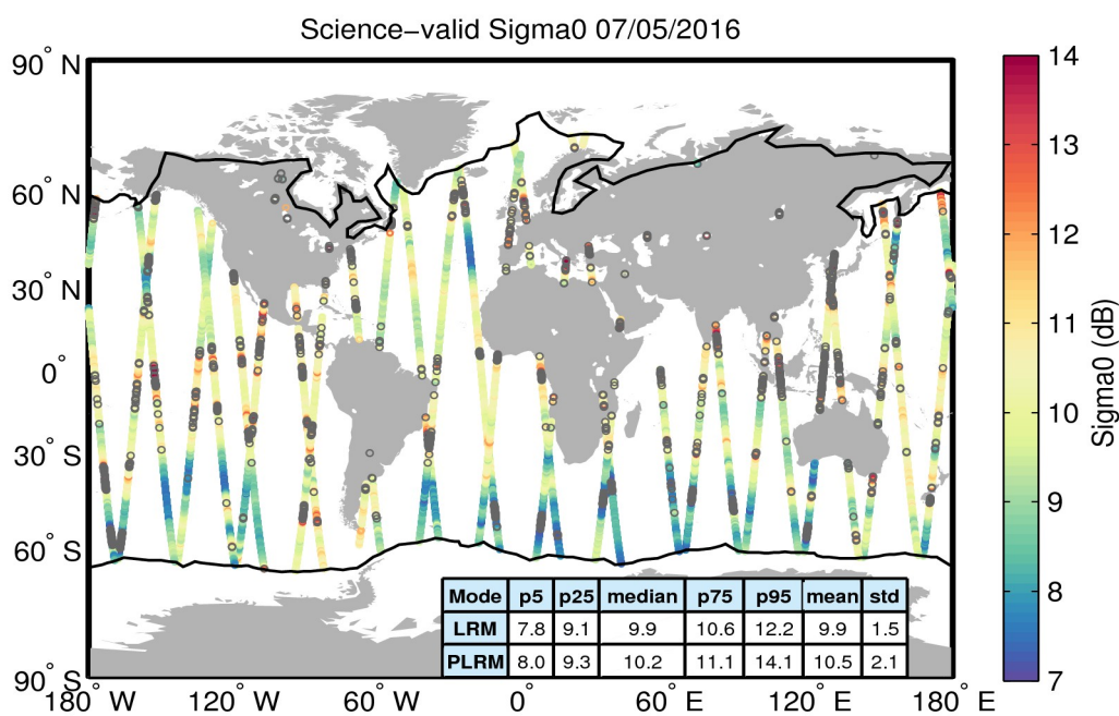
Figure 27. Geographical distribution of science-valid sigma0 data over oceans and lakes for 07/05/2016. The statistical values shown in the table refer to the sigma0 in dB and are calculated separately for LRM and PLRM regions. The black lines mark the outer limit of the Arctic and Antarctic polar polygons. Gray circles denote records that have been rejected based on the editing criteria described in Table 4.
