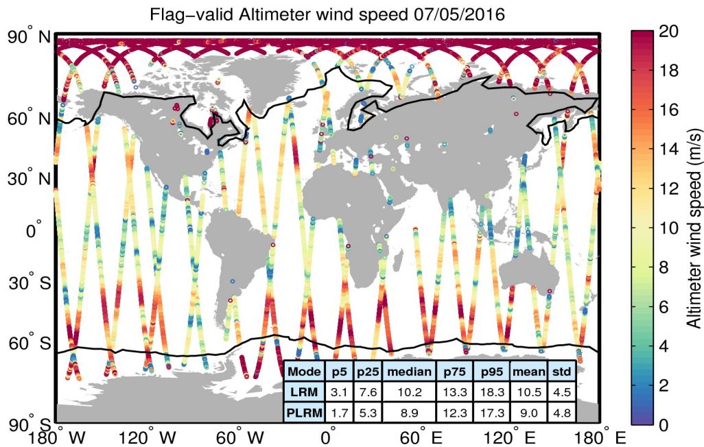
Figure 31. Geographical distribution of flag-valid wind data over oceans and lakes for 07/05/2016. The statistical values shown in the table refer to the wind in m/s and are calculated separately for LRM and PLRM regions. Measurements taken over polar polygons have been excluded from the computation of the statistical values. The black lines mark the outer limit of the Arctic and Antarctic polar polygons.
