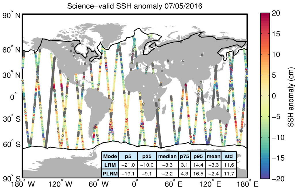
Figure 10. Geographical distribution of science-valid SSH anomaly data over oceans and lakes for 07/05/2016. The statistical values shown in the table refer to the SSH anomaly in cm and are calculated separately for LRM and PLRM regions. The black lines mark the outer limit of the Arctic and Antarctic polar polygons. Gray circles denote records that have been rejected based on the editing criteria described in Table 2.
