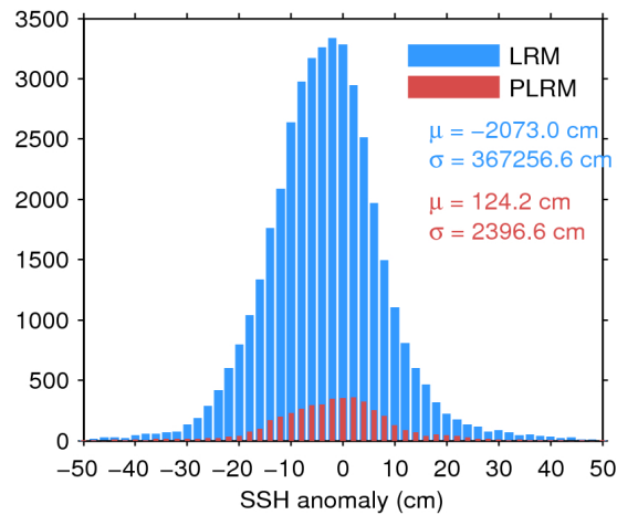
Figure 7. Histogram of flag-valid SSH anomaly over oceans and lakes for LRM (blue) and PLRM (red) for 07/05/2016. The mean ( \mu ) and standard deviation ( \sigma ) are also shown. Note that values outside [-50 50] cm are excluded from the histogram for the sake of readability but not from the computation of \mu and \sigma .
