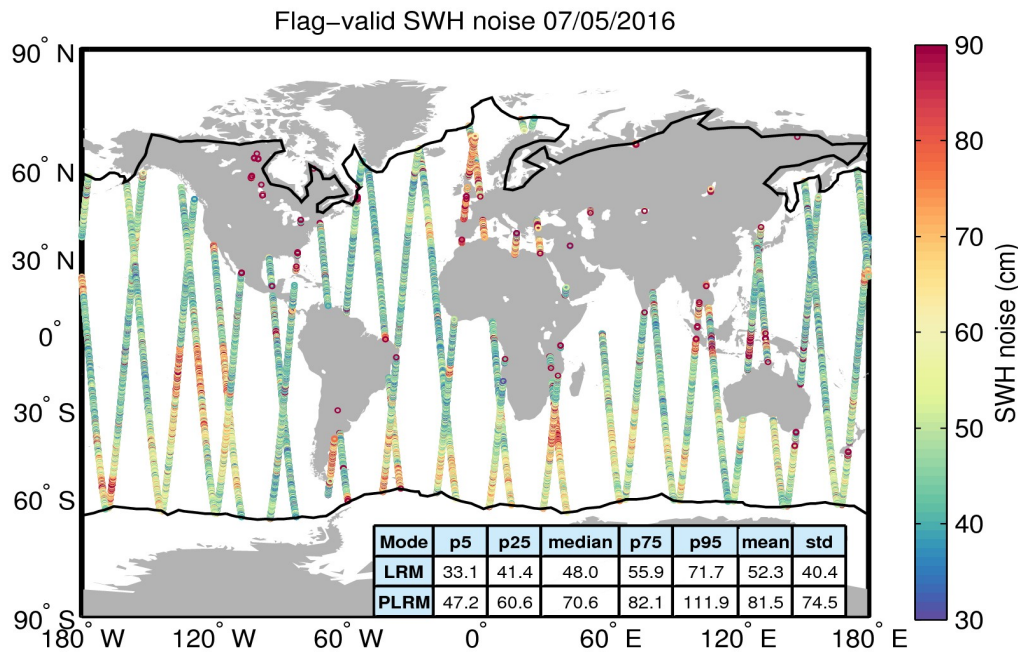
Figure 18. Geographical distribution of flag-valid 20-Hz SWH measurement noise over oceans and lakes for 07/05/2016. The statistical values shown in the table refer to the SWH noise and are calculated separately for LRM and PLRM regions. Measurements taken over polar polygons have been excluded from the computation of the statistical values. The black lines mark the outer limit of the Arctic and Antarctic polar polygons.
