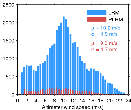
Figure 35. Histogram of science-valid wind over oceans and lakes for LRM (blue) and PLRM (red) for 28/04/2016. The mean ( \mu ) and standard deviation ( \sigma ) are also shown. Note that values larger than 24 m/s are excluded from the histogram for the sake of readability but not from the computation of \mu and \sigma .
