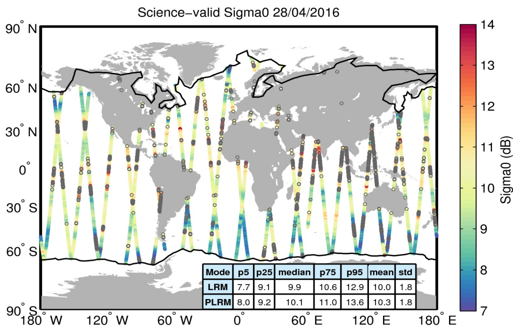
Figure 27. Geographical distribution of science-valid sigma0 data over oceans and lakes for 28/04/2016. The statistical values shown in the table refer to the sigma0 in dB and are calculated separately for LRM and PLRM regions. The black lines mark the outer limit of the Arctic and Antarctic polar polygons. Gray circles denote records that have been rejected based on the editing criteria described in Table 4.
