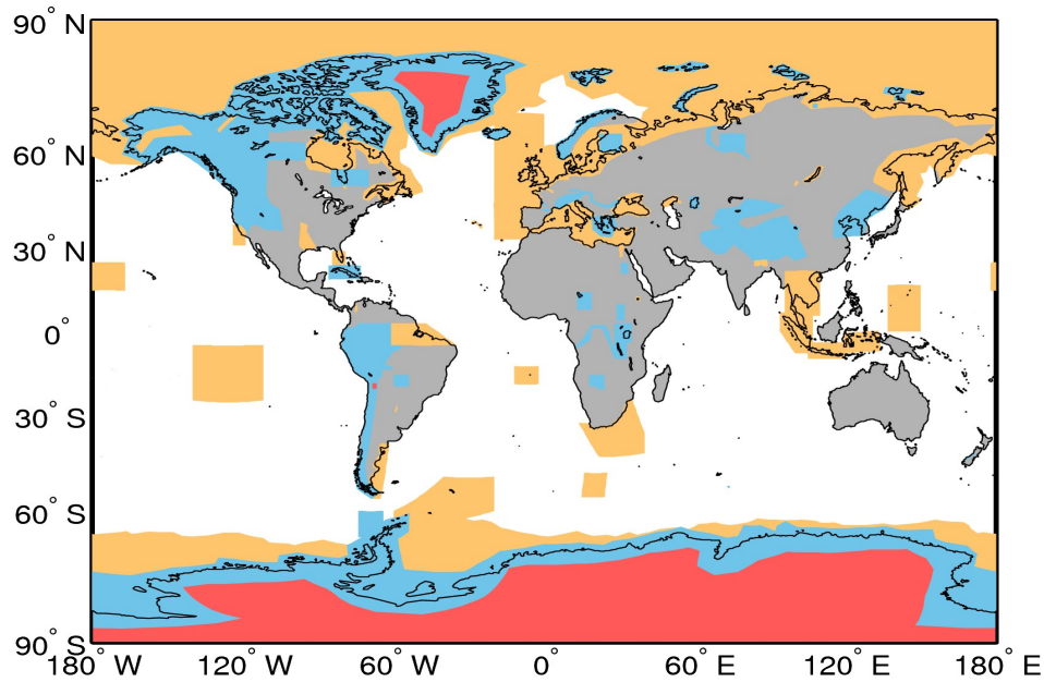
Figure A1. Extent of the regions defining the geographical mode mask for 28/04/2016. The regions where SAR, and SARIn are operated are denoted by the orange and blue polygons, respectively. LRM is operated over areas of the continental ice sheets (red polygons) and over oceans and land not covered by other modes.
