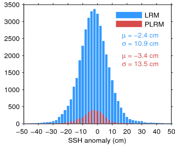
Figure 11. Histogram of science-valid SSH anomaly over oceans and lakes for LRM (blue) and PLRM (red) for 28/04/2016. The mean ( \mu ) and standard deviation ( \sigma ) are also shown. Note that values outside [-50\ 50] cm are excluded from the histogram for the sake of readability but not from the computation of \mu and \sigma .
