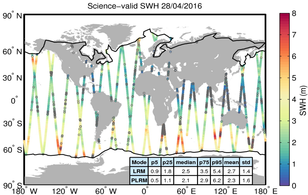
Figure 19. Geographical distribution of science-valid SWH data over oceans and lakes for 28/04/2016. The statistical values shown in the table refer to the SWH in m and are calculated separately for LRM and PLRM regions. The black lines mark the outer limit of the Arctic and Antarctic polar polygons. Gray circles denote records that have been rejected based on the editing criteria described in Table 3.
