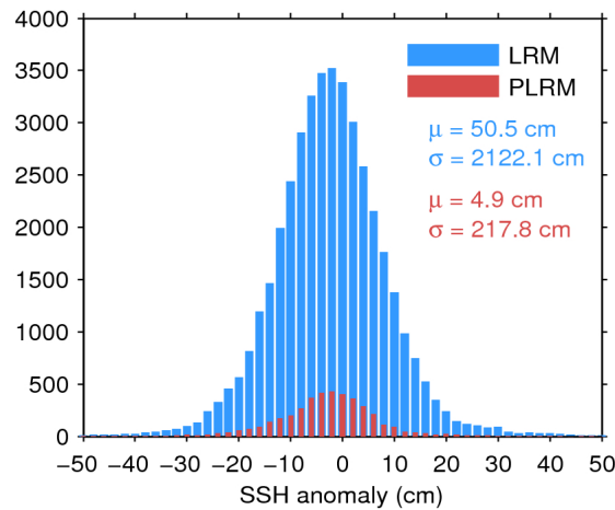
Figure 7. Histogram of flag-valid SSH anomaly over oceans and lakes for LRM (blue) and PLRM (red) for 28/04/2016. The mean ( \mu ) and standard deviation ( \sigma ) are also shown. Note that values outside [-50 50] cm are excluded from the histogram for the sake of readability but not from the computation of \mu and \sigma .
