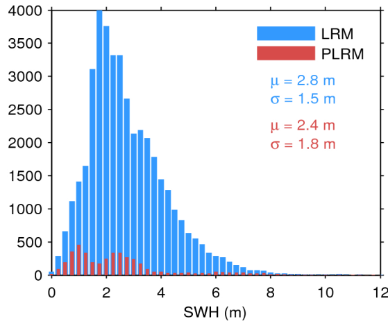
Figure 17. Histogram of flag-valid SWH over oceans and lakes for LRM (blue) and PLRM (red) for 28/04/2016. The mean ( \mu ) and standard deviation ( \sigma ) are also shown. Note that values larger than 12 m are excluded from the histogram for the sake of readability but not from the computation of \mu and \sigma .
