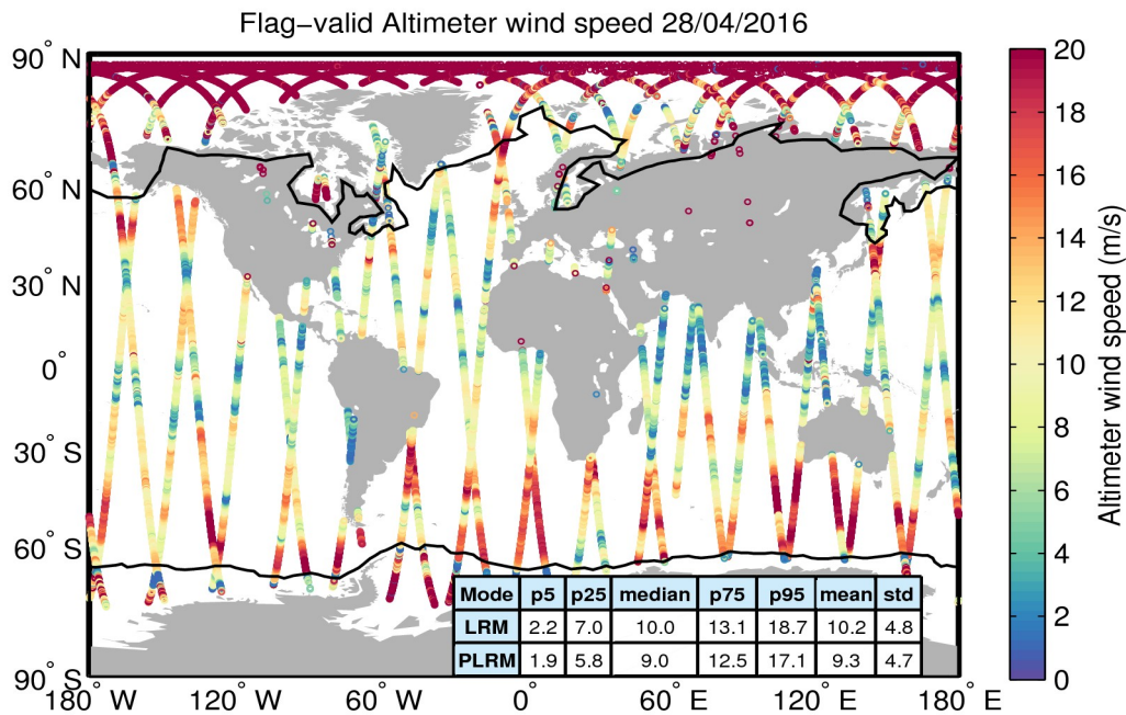
Figure 31. Geographical distribution of flag-valid wind data over oceans and lakes for 28/04/2016. The statistical values shown in the table refer to the wind in m/s and are calculated separately for LRM and PLRM regions. Measurements taken over polar polygons have been excluded from the computation of the statistical values. The black lines mark the outer limit of the Arctic and Antarctic polar polygons.
