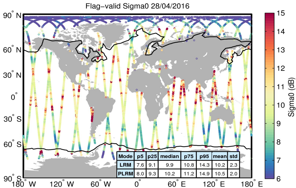
Figure 23. Geographical distribution of flag-valid sigma0 data over oceans and lakes for 28/04/2016. The statistical values shown in the table refer to the sigma0 in dB and are calculated separately for LRM and PLRM regions. Measurements taken over polar polygons have been excluded from the computation of the statistical values. The black lines mark the outer limit of the Arctic and Antarctic polar polygons.
