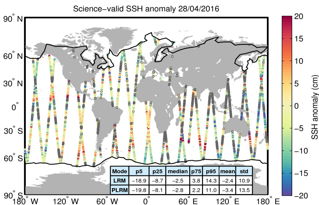
Figure 10. Geographical distribution of science-valid SSH anomaly data over oceans and lakes for 28/04/2016. The statistical values shown in the table refer to the SSH anomaly in cm and are calculated separately for LRM and PLRM regions. The black lines mark the outer limit of the Arctic and Antarctic polar polygons. Gray circles denote records that have been rejected based on the editing criteria described in Table 2.
