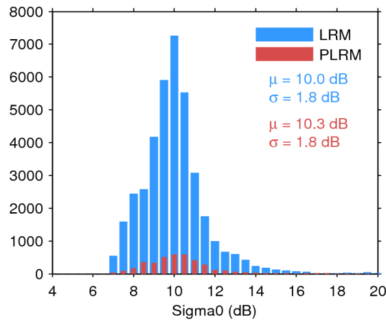
Figure 28. Histogram of science-valid sigma0 over oceans and lakes for LRM (blue) and PLRM (red) for 28/04/2016. The mean ( \mu ) and standard deviation ( \sigma ) are also shown. Note that values outside [4 20] dB are excluded from the histogram for the sake of readability but not from the computation of \mu and \sigma .
