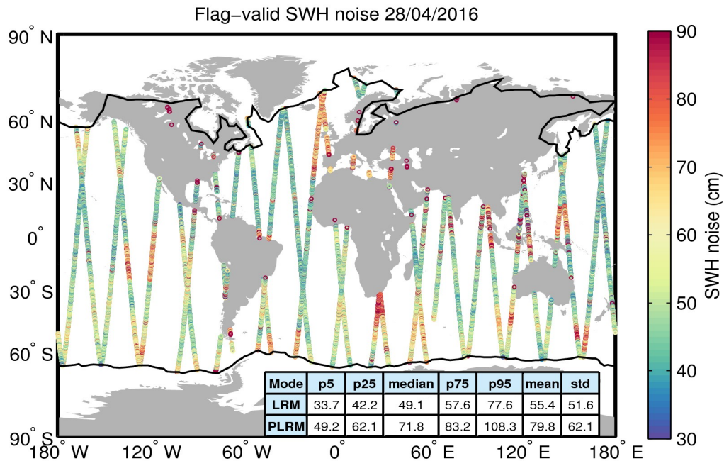
Figure 18. Geographical distribution of flag-valid 20-Hz SWH measurement noise over oceans and lakes for 28/04/2016. The statistical values shown in the table refer to the SWH noise and are calculated separately for LRM and PLRM regions. Measurements taken over polar polygons have been excluded from the computation of the statistical values. The black lines mark the outer limit of the Arctic and Antarctic polar polygons.
