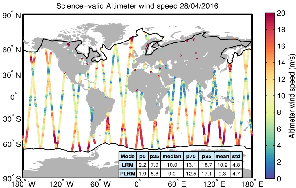
Figure 34. Geographical distribution of science-valid wind data over oceans and lakes for 28/04/2016. The statistical values shown in the table refer to the wind in m/s and are calculated separately for LRM and PLRM regions. The black lines mark the outer limit of the Arctic and Antarctic polar polygons. Gray circles denote records that have been rejected based on the editing criteria described in Table 5.
