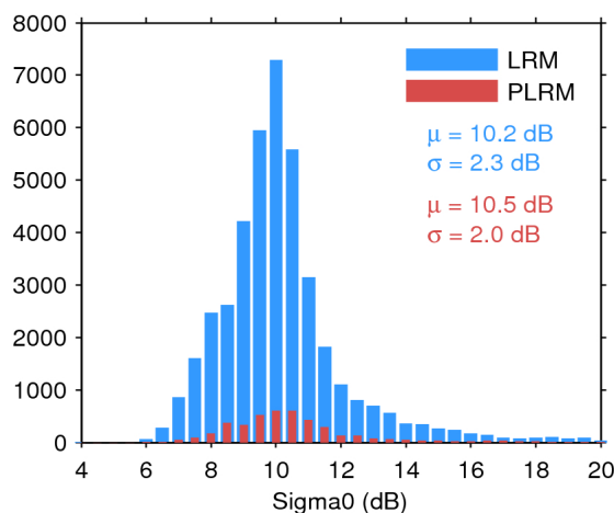
Figure 25. Histogram of flag-valid sigma0 over oceans and lakes for LRM (blue) and PLRM (red) for 28/04/2016. The mean ( \mu ) and standard deviation ( \sigma ) are also shown. Note that values outside [4 20] dB are excluded from the histogram for the sake of readability but not from the computation of \mu and \sigma .
