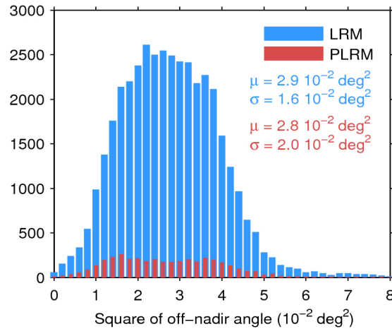
Figure 39. Histogram of flag-valid mispointing over oceans and lakes for LRM (blue) and PLRM (red) for 28/04/2016. Only positive values have been considered. The mean ( \mu ) and standard deviation ( \sigma ) are also shown. Note that values larger than 8 \cdot 10^{-2} \text{ deg}^2 are excluded from the histogram for the sake of readability but not from the computation of \mu and \sigma .
