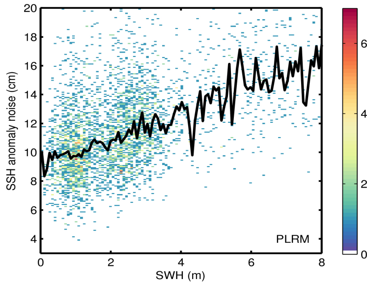
Figure 9. 2D histogram showing flag-valid SSH anomaly noise as a function of SWH for LRM (top) and PLRM (bottom) for 28/04/2016. The black line denotes the median SSH anomaly noise as a function of SWH.
