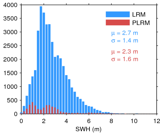
Figure 20. Histogram of science-valid SWH over oceans and lakes for LRM (blue) and PLRM (red) for 28/04/2016. The mean ( \mu ) and standard deviation ( \sigma ) are also shown. Note that values larger than 12 m are excluded from the histogram for the sake of readability but not from the computation of \mu and \sigma .
