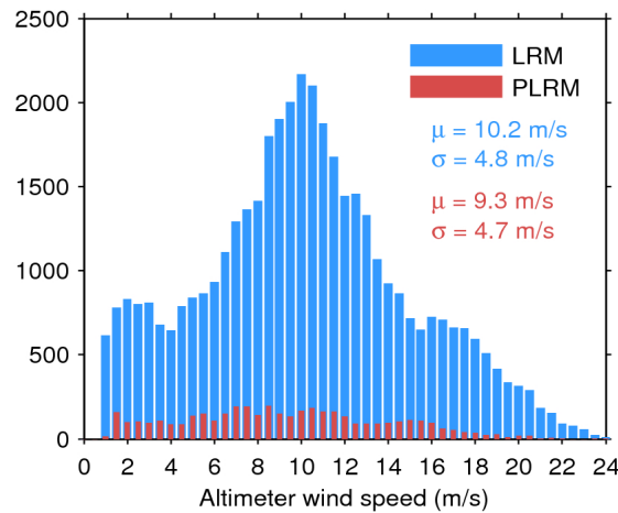
Figure 33. Histogram of flag-valid wind over oceans and lakes for LRM (blue) and PLRM (red) for 28/04/2016. The mean ( \mu ) and standard deviation ( \sigma ) are also shown. Note that values larger than 24 m/s are excluded from the histogram for the sake of readability but not from the computation of \mu and \sigma .
