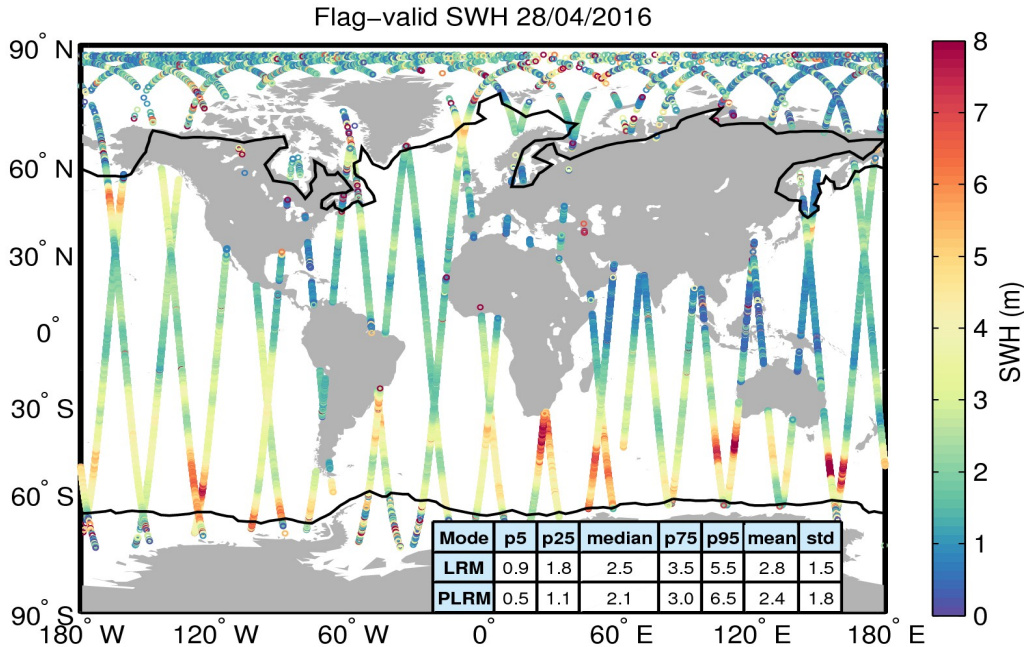
Figure 15. Geographical distribution of flag-valid SWH data over oceans and lakes for 28/04/2016. The statistical values shown in the table refer to the SWH in m and are calculated separately for LRM and PLRM regions. Measurements taken over polar polygons have been excluded from the computation of the statistical values. The black lines mark the outer limit of the Arctic and Antarctic polar polygons.
